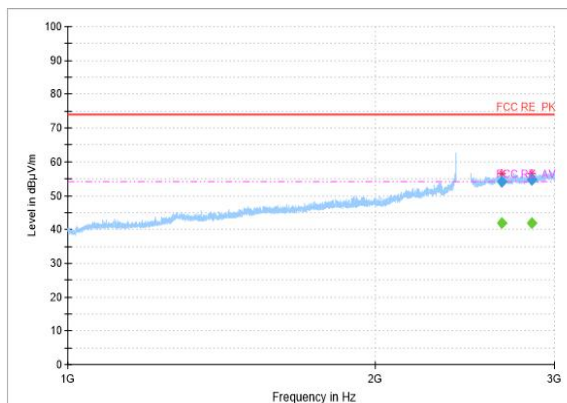
RSE-2M-CH19-1GHz-3GHz
