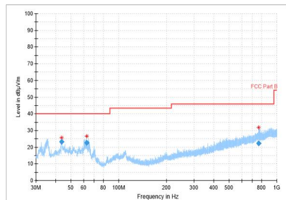
RSE-2M-CH19-30MHz-1GHz
