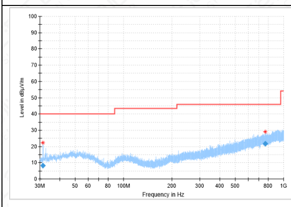
RSE-11A-CH140-30MHz-1GHz
