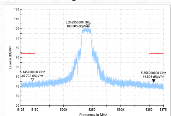
Bandedge-11A-CH48-PK
