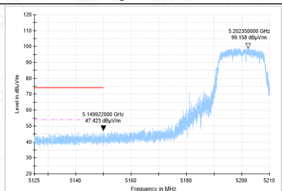
Bandedge-11A-CH40-PK
