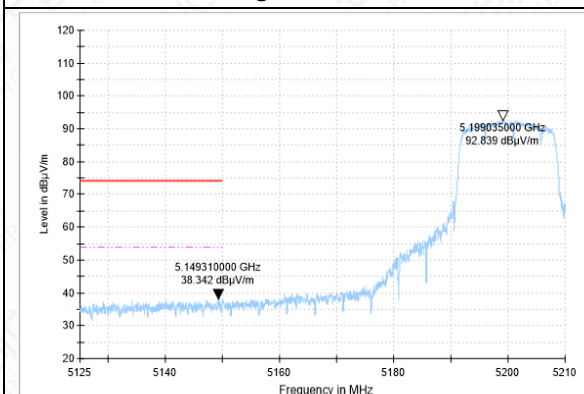
Bandedge-11A-CH40-AV
