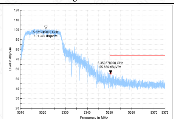
Bandedge-11A-CH64-PK
