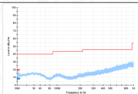
RSE-11A-CH52-30MHz-1GHz
