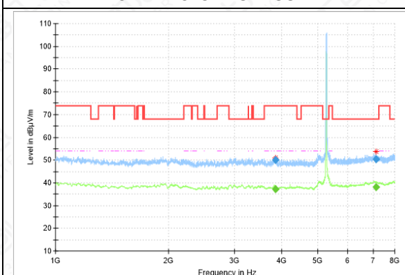
RSE-11A-CH52-1GHz-8GHz
