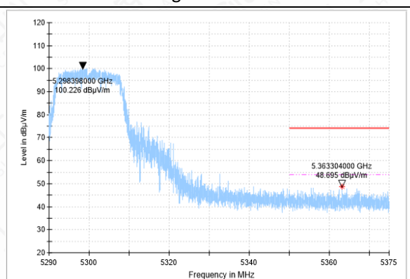
Bandedge-11A-CH60-PK
