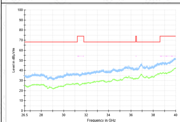
RSE-11A-CH48-26.5GHz-40GHz
