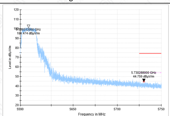
Bandedge-11A-CH120-PK
