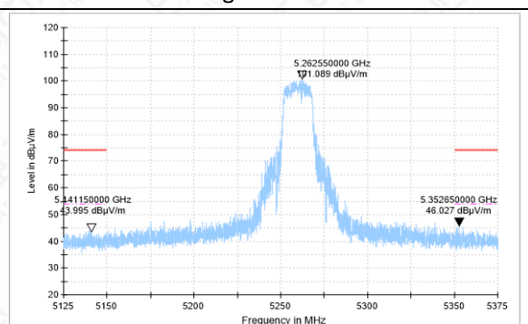
Bandedge-11A-CH52-PK
