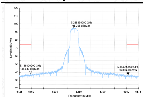
Bandedge-11A-CH48-AV
