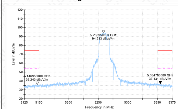
Bandedge-11A-CH52-AV
