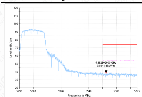
Bandedge-11A-CH60-AV
