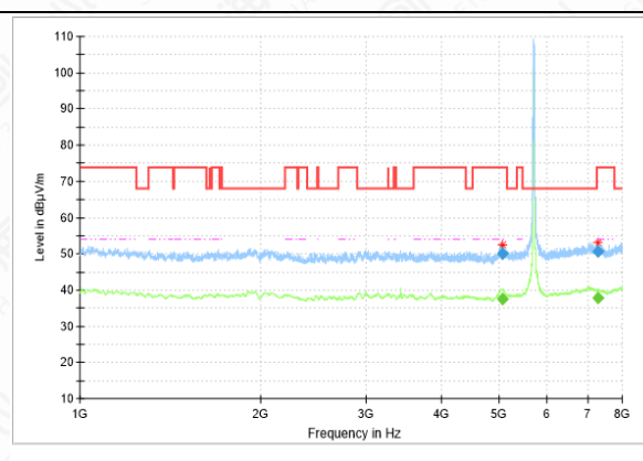
RSE-11A-CH140-1GHz-8GHz
