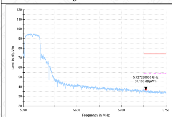
Bandedge-11A-CH120-AV
