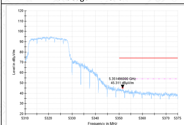
Bandedge-11A-CH64-AV
