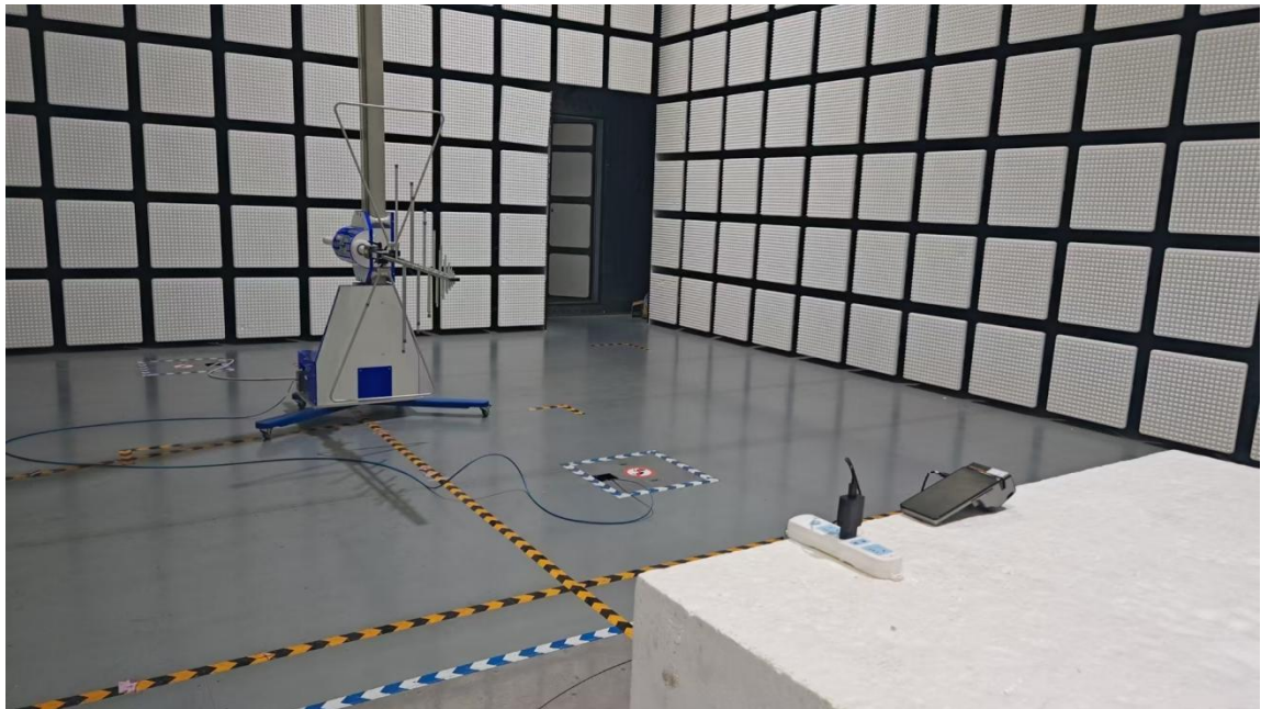
Description: Back view of Radiated Emission Test Setup (Below 1GHz)
