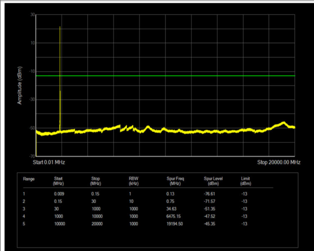
Band2 QPSK BW=15MHz Channel=18675 RB Size=1 Position=#0
