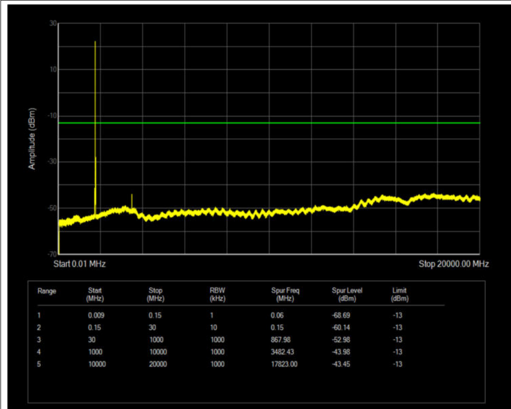
Band4 QPSK BW=15MHz Channel=20325 RB Size=1 Position=#0
