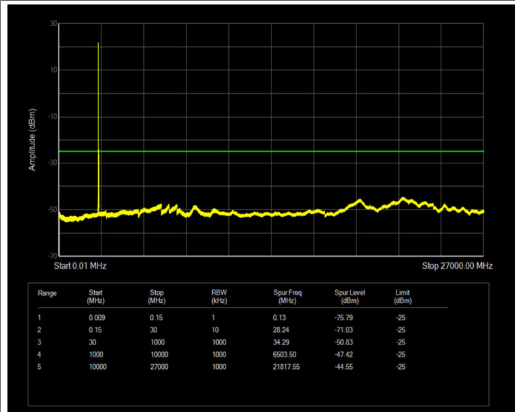
Band7 QPSK BW=20MHz Channel=20850 RB Size=1 Position=#0
