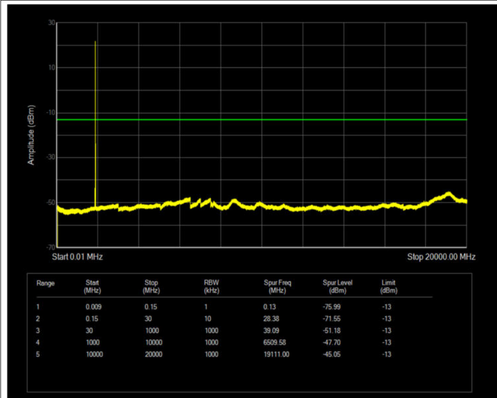
Band2 QPSK BW=10MHz Channel=18900 RB Size=1 Position=#0
