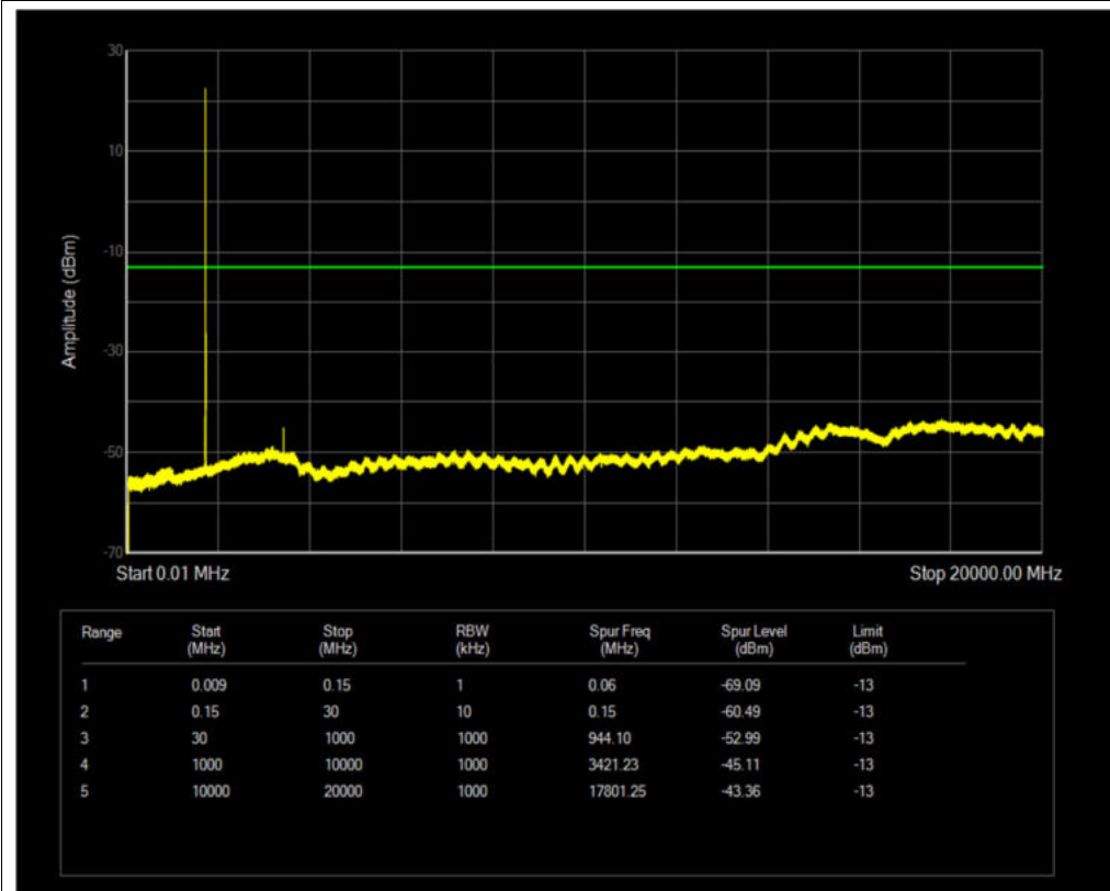
Band4 QPSK BW=5MHz Channel=19975 RB Size=1 Position=#0
