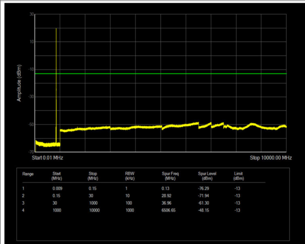
Band5 QPSK BW=5MHz Channel=20625 RB Size=1 Position=#0
