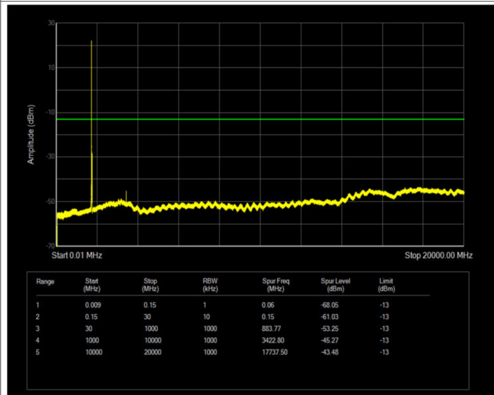
Band4 QPSK BW=20MHz Channel=20050 RB Size=1 Position=#0
