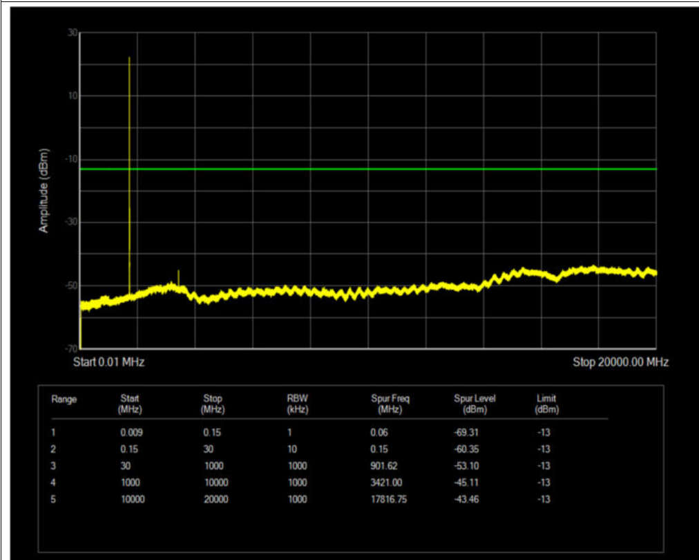
Band4 QPSK BW=3MHz Channel=19965 RB Size=1 Position=#0
