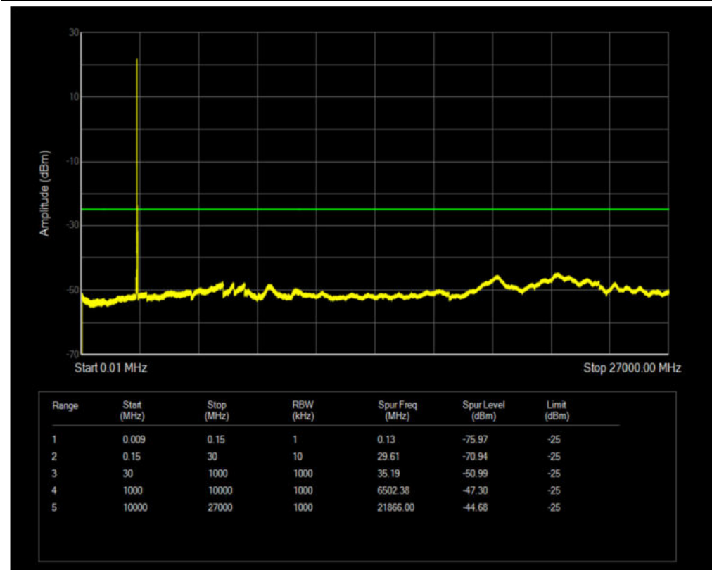
Band7 QPSK BW=20MHz Channel=21350 RB Size=1 Position=#0
