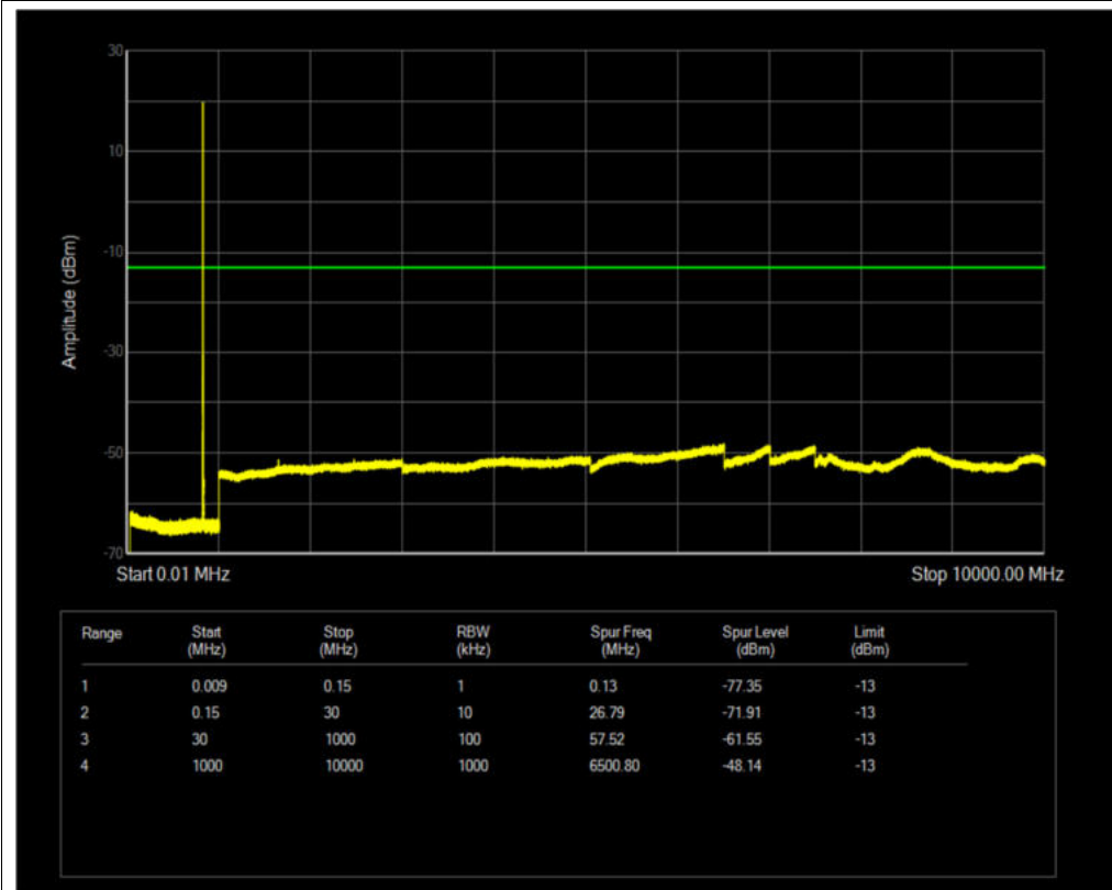
Band5 QPSK BW=3MHz Channel=20415 RB Size=1 Position=#0
