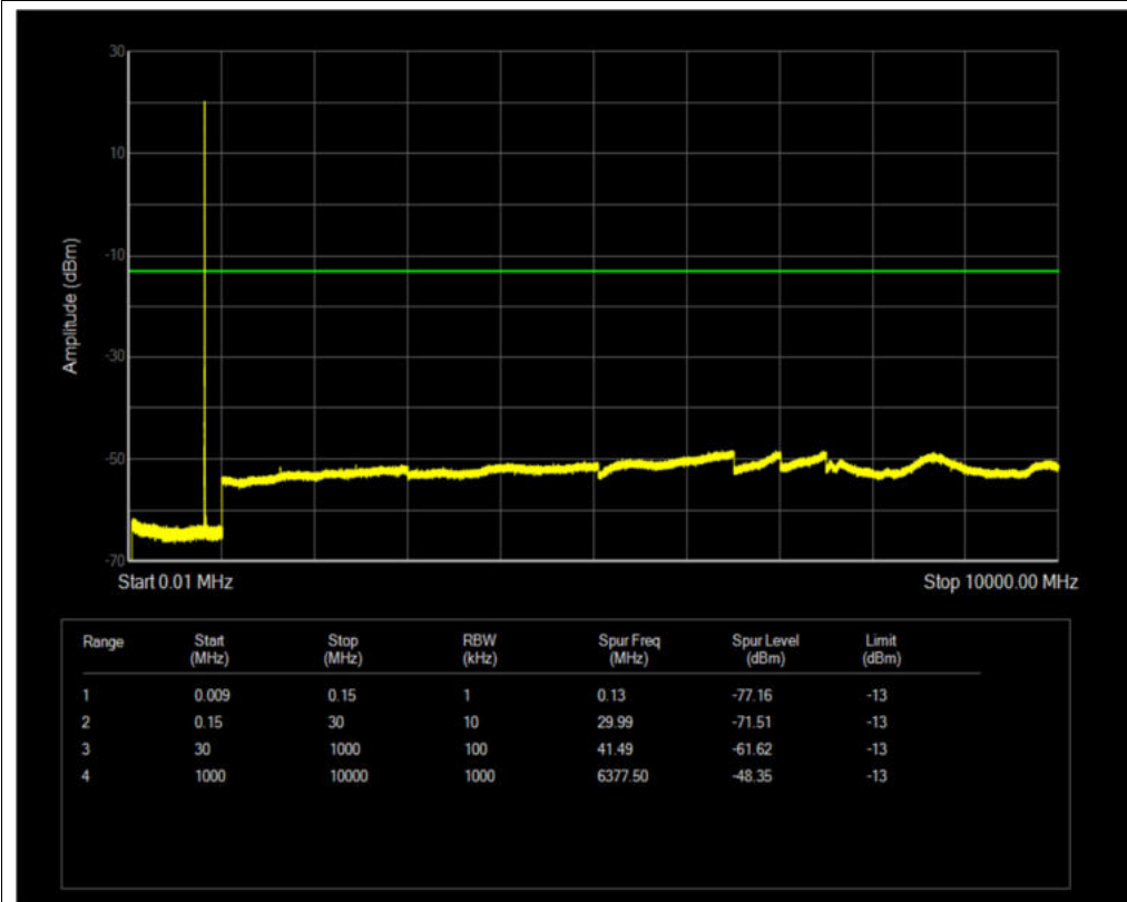
Band26(814-824) QPSK BW=1.4MHz Channel=26697 RB Size=1 Position=#0
