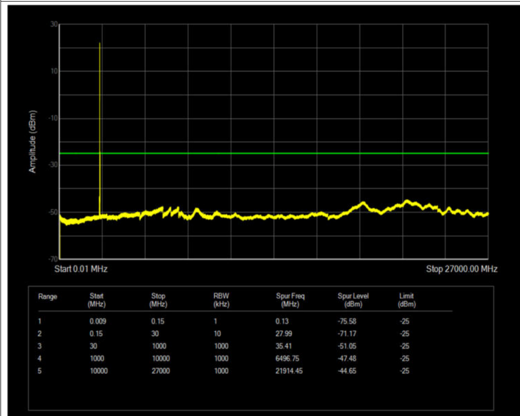
Band7 QPSK BW=10MHz Channel=21100 RB Size=1 Position=#0
