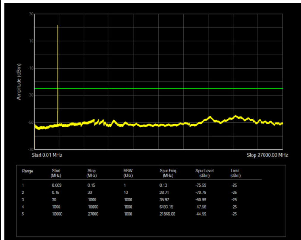
Band7 QPSK BW=5MHz Channel=21100 RB Size=1 Position=#0
