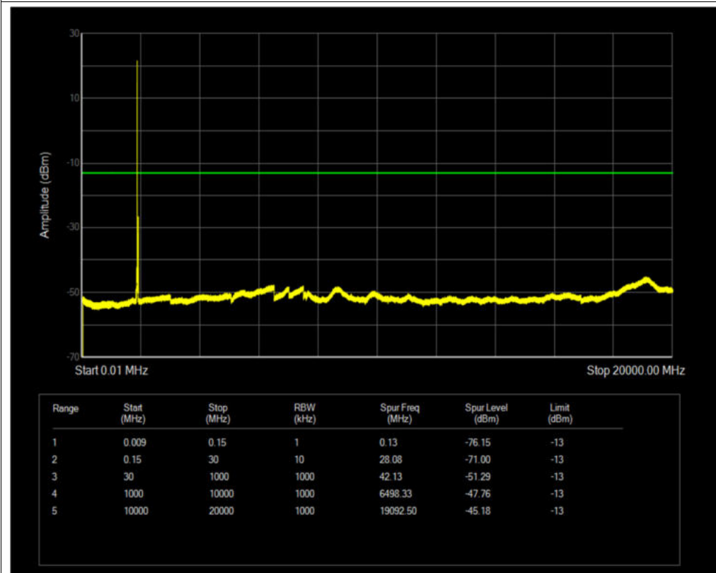
Band2 QPSK BW=20MHz Channel=18900 RB Size=1 Position=#0
