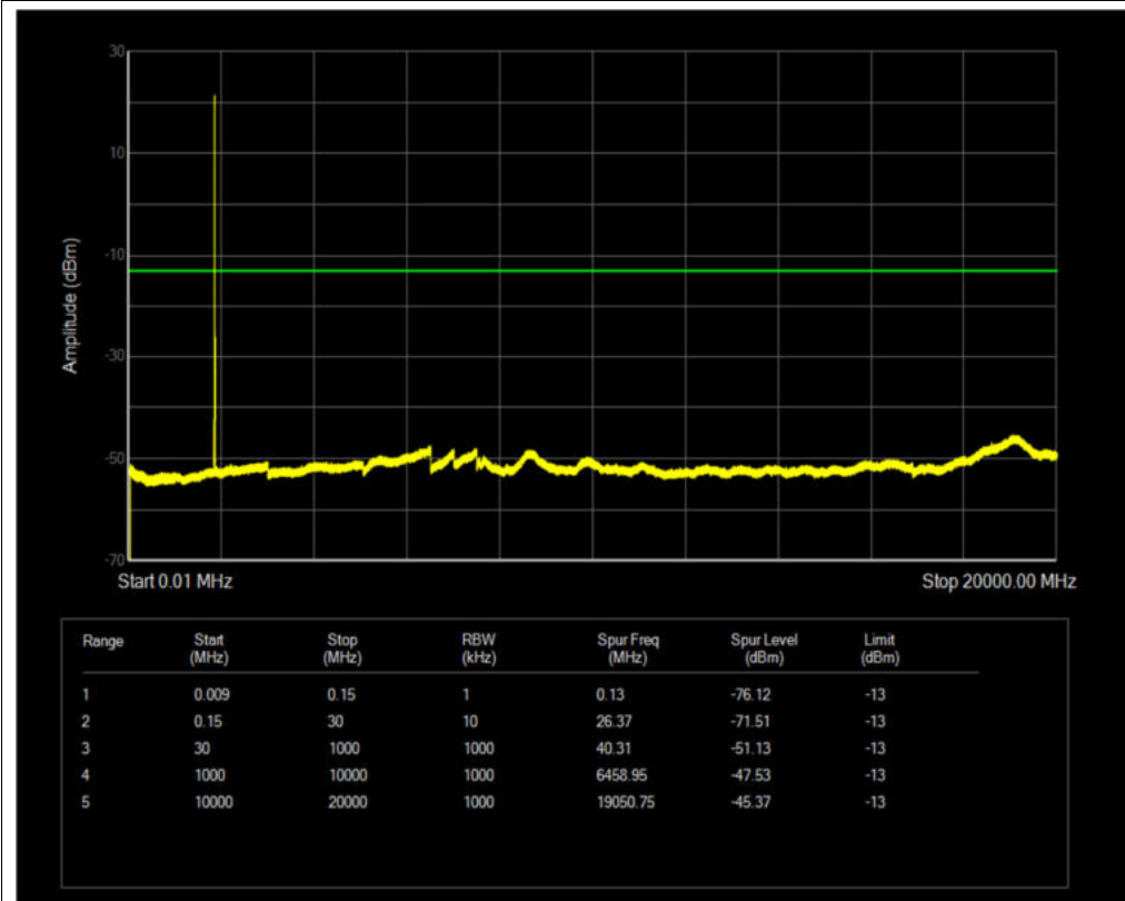
Band2 QPSK BW=5MHz Channel=18625 RB Size=1 Position=#0
