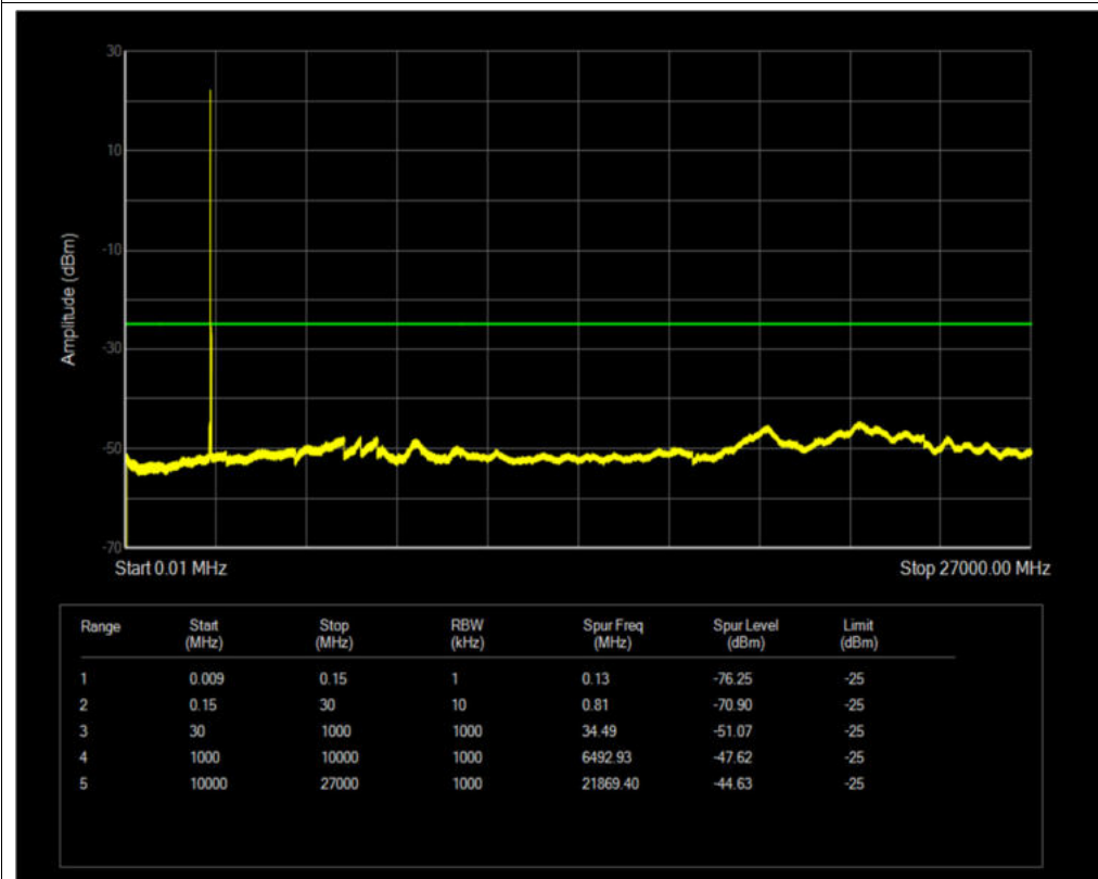
Band7 QPSK BW=20MHz Channel=21100 RB Size=1 Position=#0
