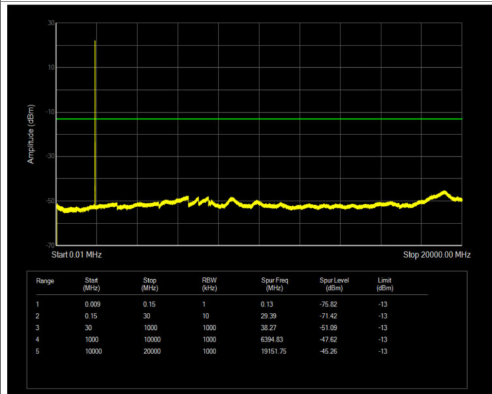
Band2 QPSK BW=3MHz Channel=19185 RB Size=1 Position=#0
