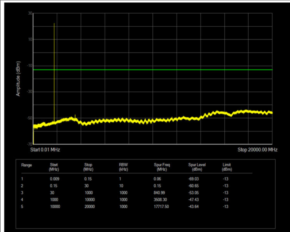
Band4 QPSK BW=1.4MHz Channel=20393 RB Size=1 Position=#0
