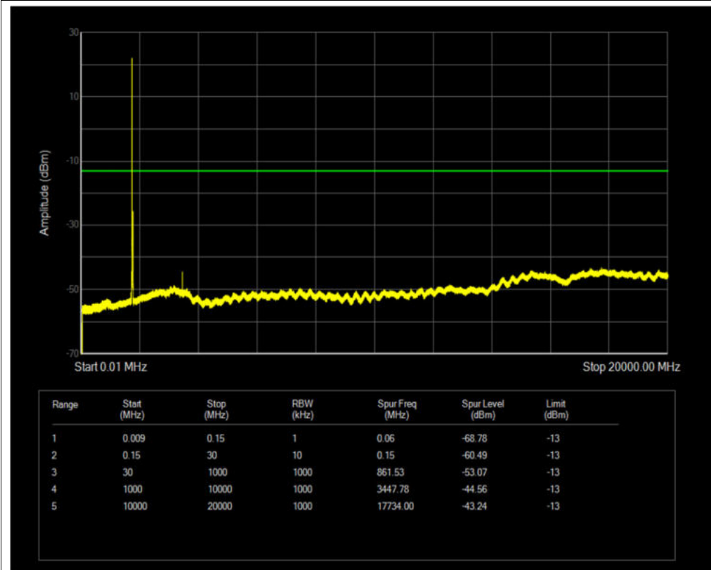
Band4 QPSK BW=20MHz Channel=20175 RB Size=1 Position=#0
