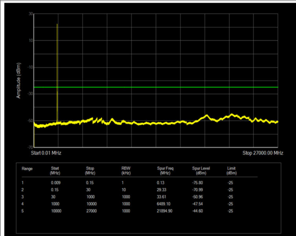
Band7 QPSK BW=5MHz Channel=21425 RB Size=1 Position=#0
