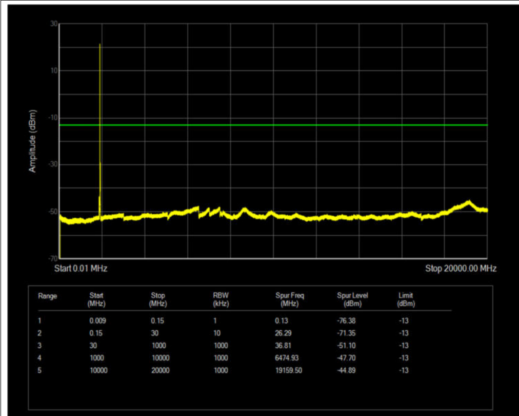
Band2 QPSK BW=20MHz Channel=19100 RB Size=1 Position=#0
