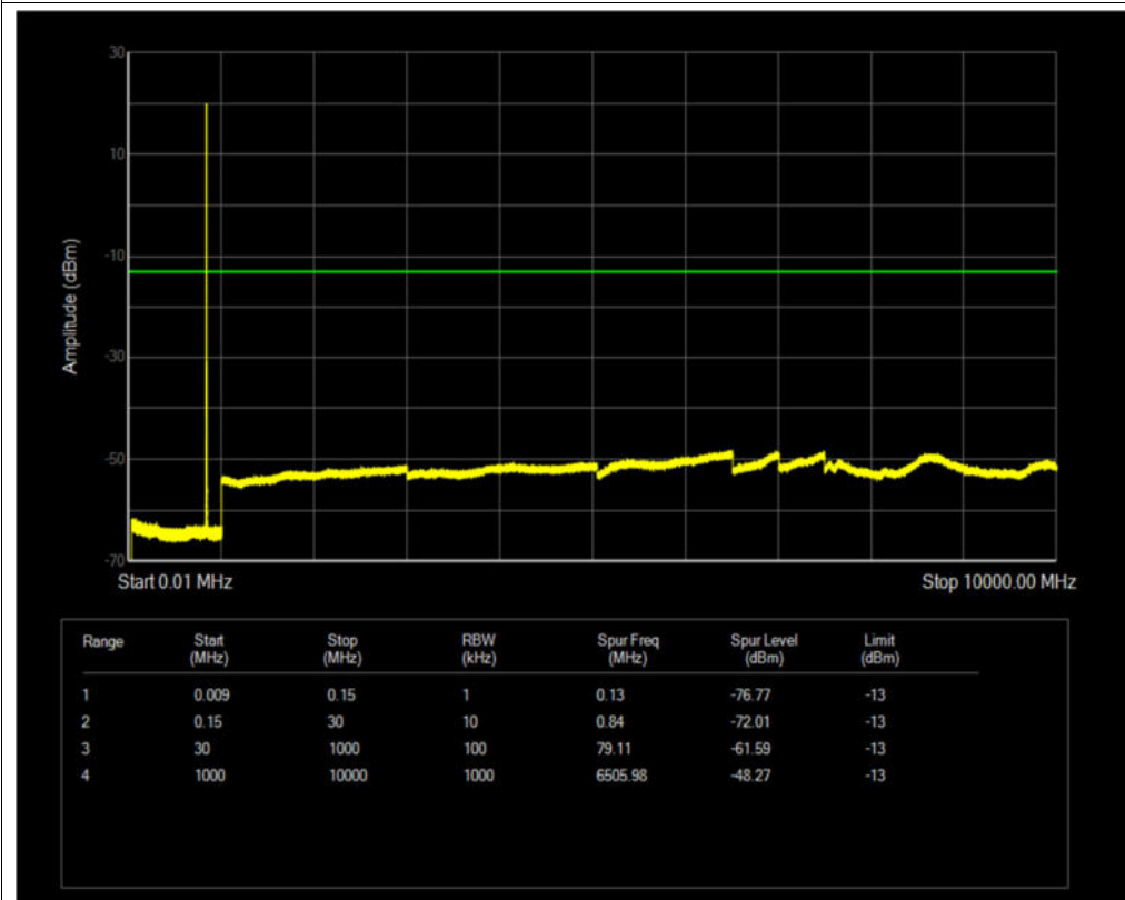
Band5 QPSK BW=3MHz Channel=20525 RB Size=1 Position=#0
