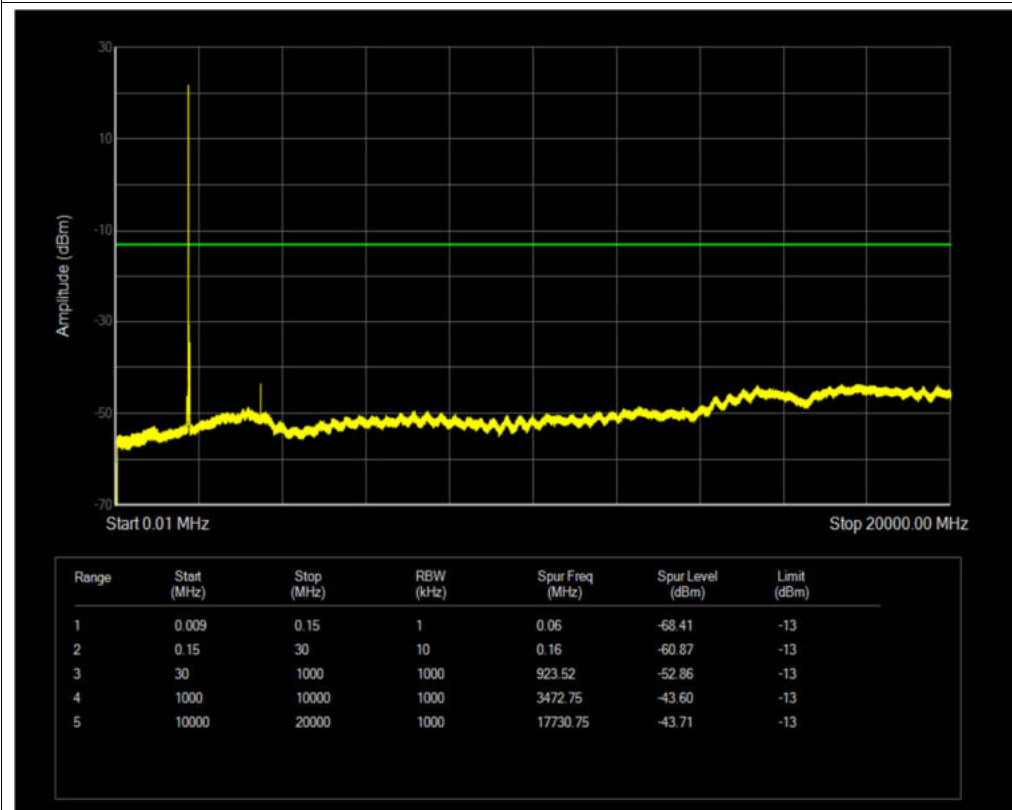
Band4 QPSK BW=20MHz Channel=20300 RB Size=1 Position=#0
