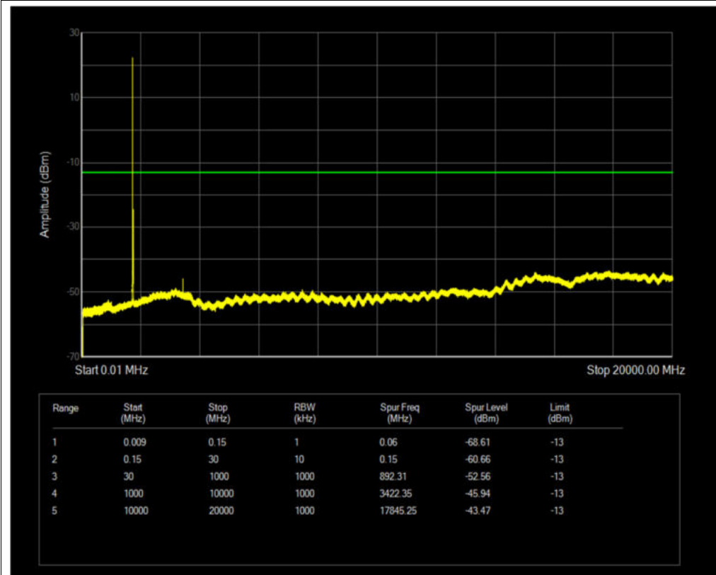
Band4 QPSK BW=15MHz Channel=20025 RB Size=1 Position=#0
