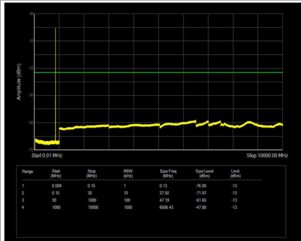
Band5 QPSK BW=3MHz Channel=20635 RB Size=1 Position=#0
