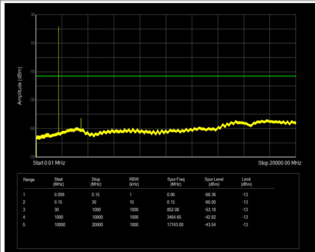
Band4 QPSK BW=1.4MHz Channel=20175 RB Size=1 Position=#0
