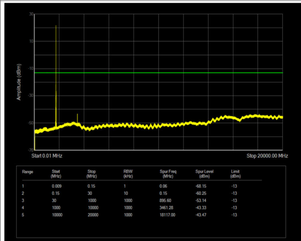
Band4 QPSK BW=5MHz Channel=20175 RB Size=1 Position=#0
