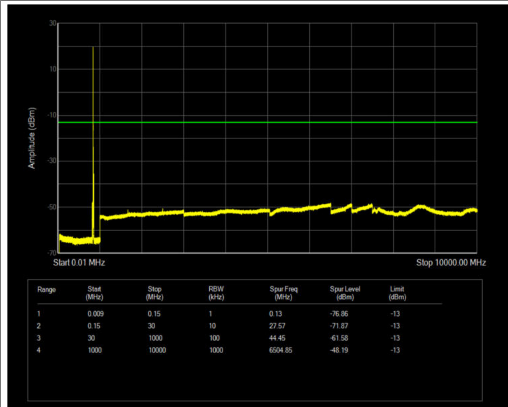
Band5 QPSK BW=10MHz Channel=20525 RB Size=1 Position=#0
