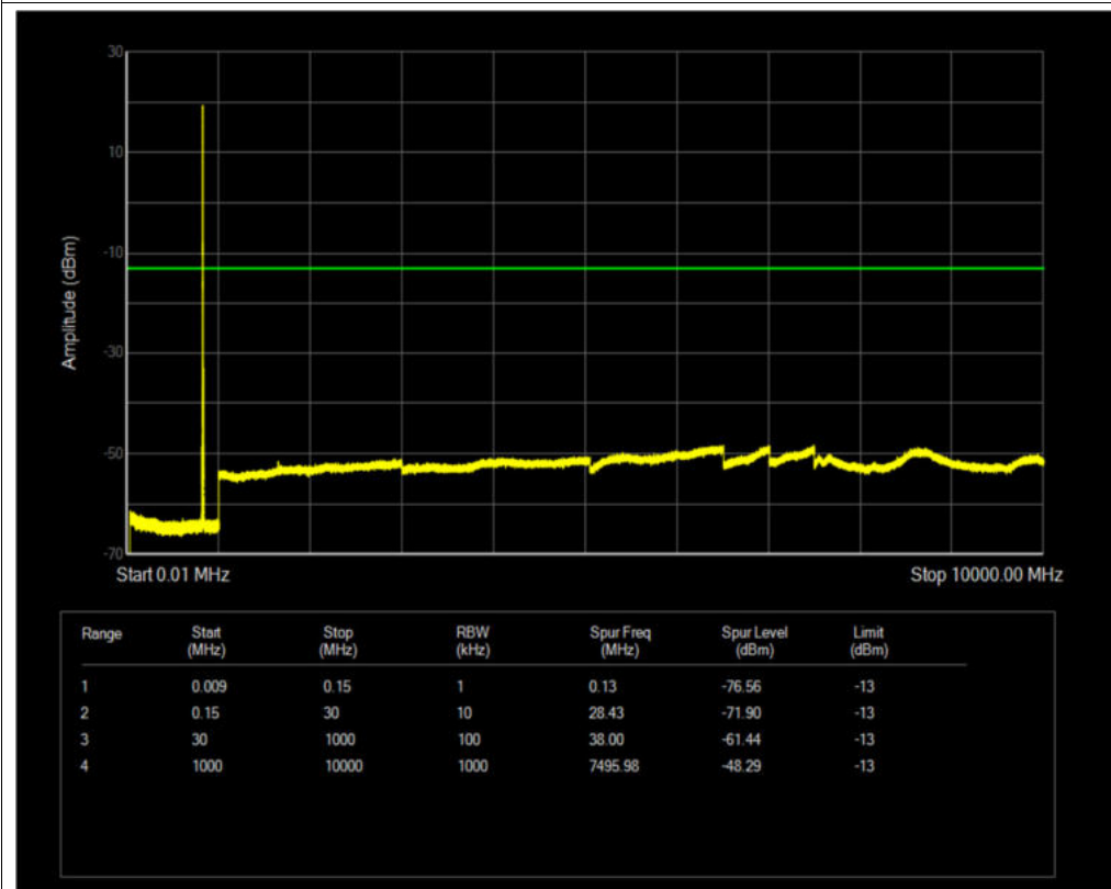
Band5 QPSK BW=5MHz Channel=20425 RB Size=1 Position=#0
