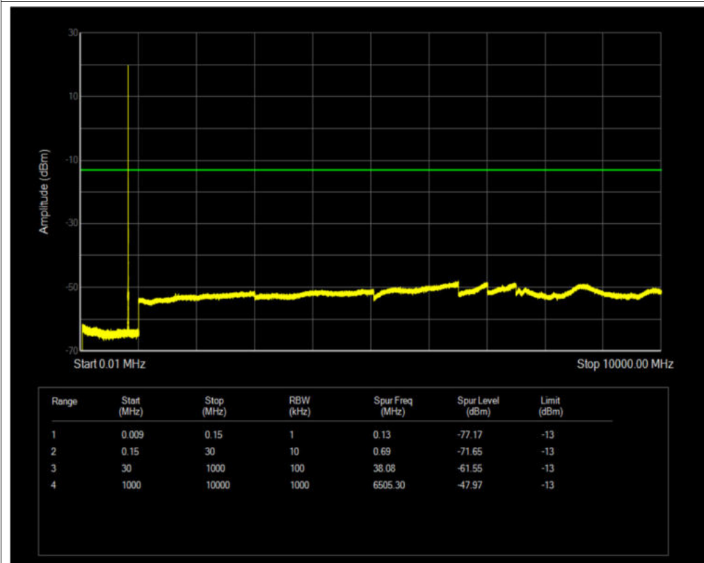
Band26(814-824) QPSK BW=1.4MHz Channel=26740 RB Size=1 Position=#0
