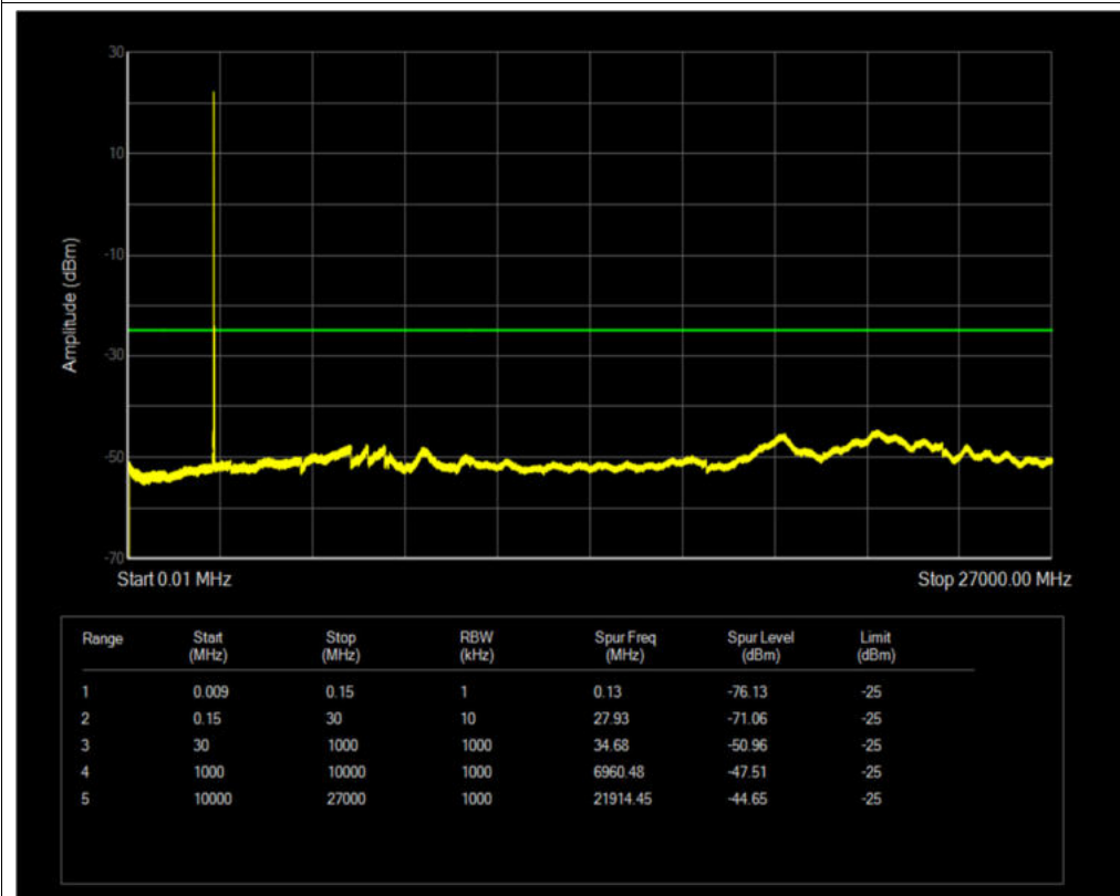
Band7 QPSK BW=15MHz Channel=20825 RB Size=1 Position=#0
