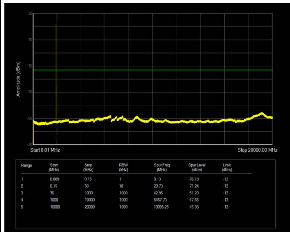
Band2 QPSK BW=5MHz Channel=19175 RB Size=1 Position=#0
