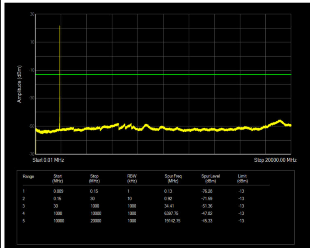
Band2 QPSK BW=10MHz Channel=19150 RB Size=1 Position=#0
