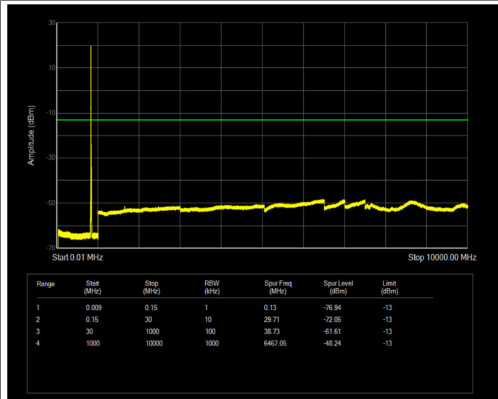
Band5 QPSK BW=10MHz Channel=20450 RB Size=1 Position=#0
