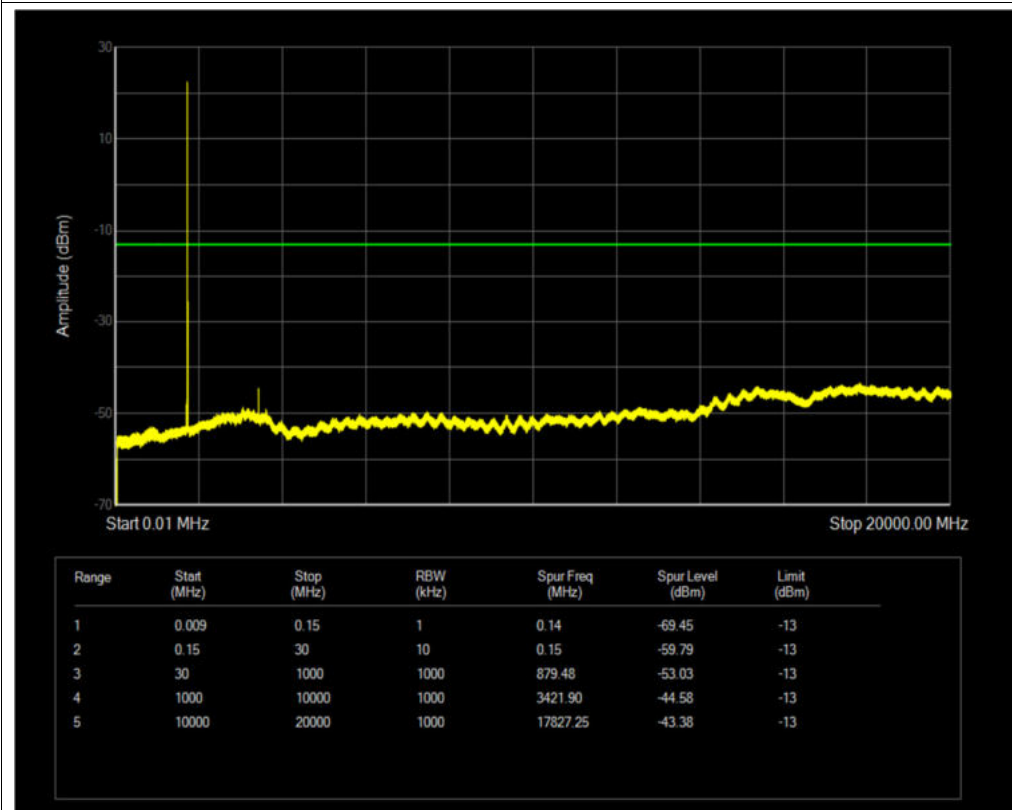
Band4 QPSK BW=10MHz Channel=20000 RB Size=1 Position=#0
