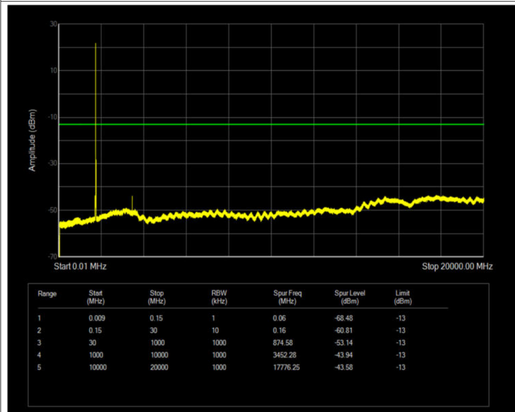
Band4 QPSK BW=15MHz Channel=20175 RB Size=1 Position=#0
