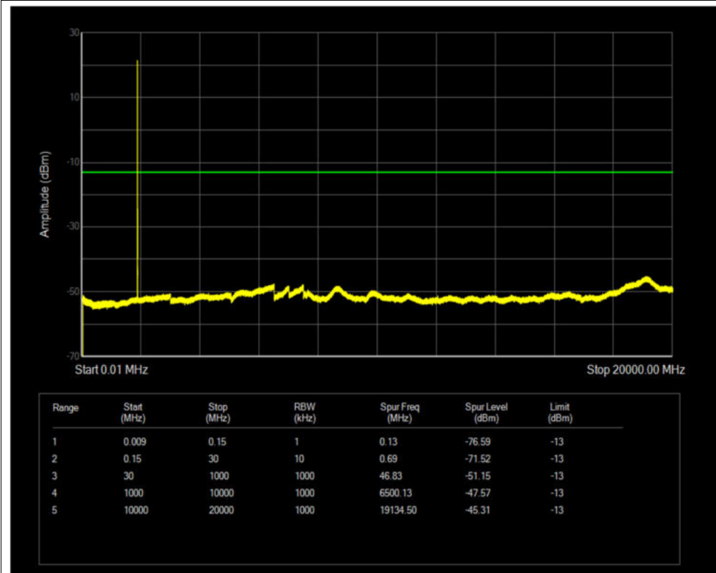
Band2 QPSK BW=3MHz Channel=18900 RB Size=1 Position=#0
