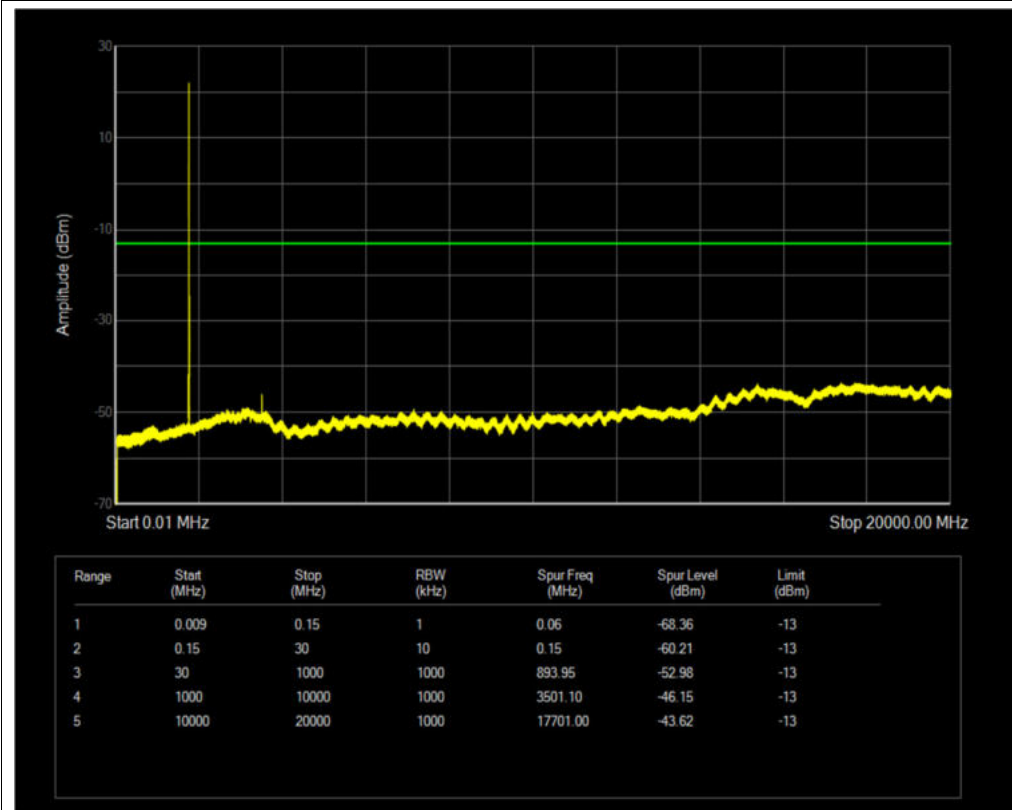
Band4 QPSK BW=5MHz Channel=20375 RB Size=1 Position=#0
