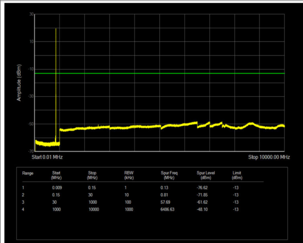
Band5 QPSK BW=1.4MHz Channel=20643 RB Size=1 Position=#0
