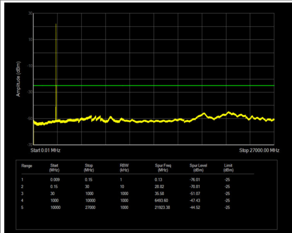
Band7 QPSK BW=15MHz Channel=21100 RB Size=1 Position=#0
