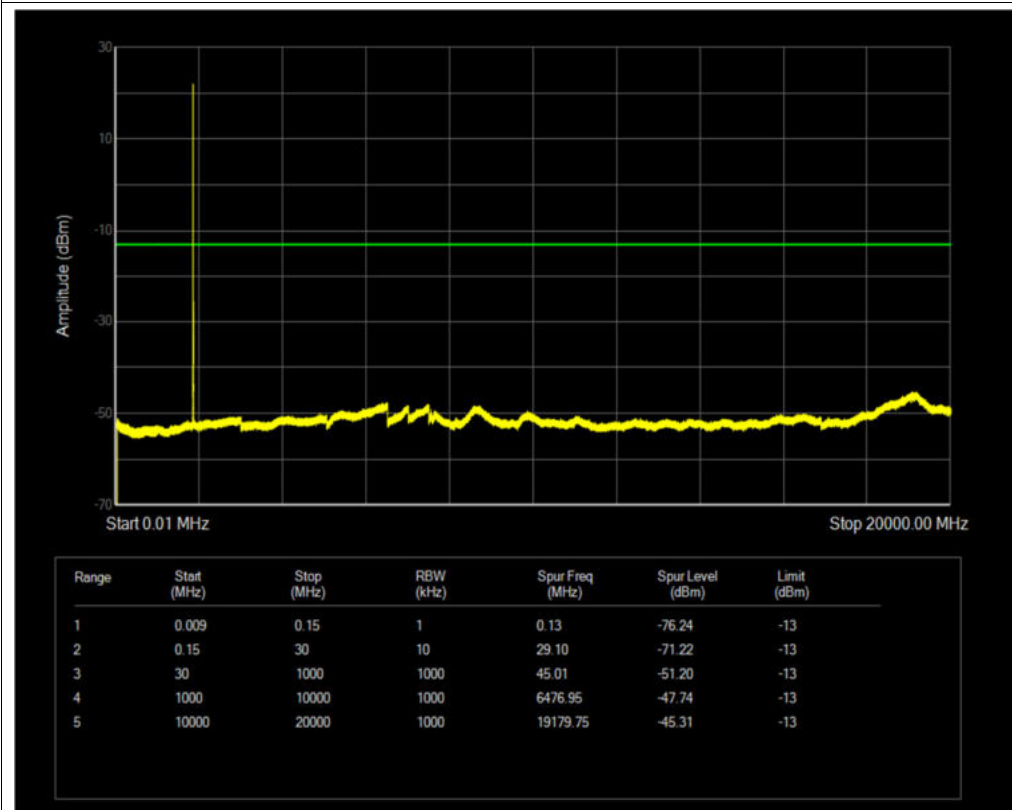
Band2 QPSK BW=3MHz Channel=18615 RB Size=1 Position=#0
