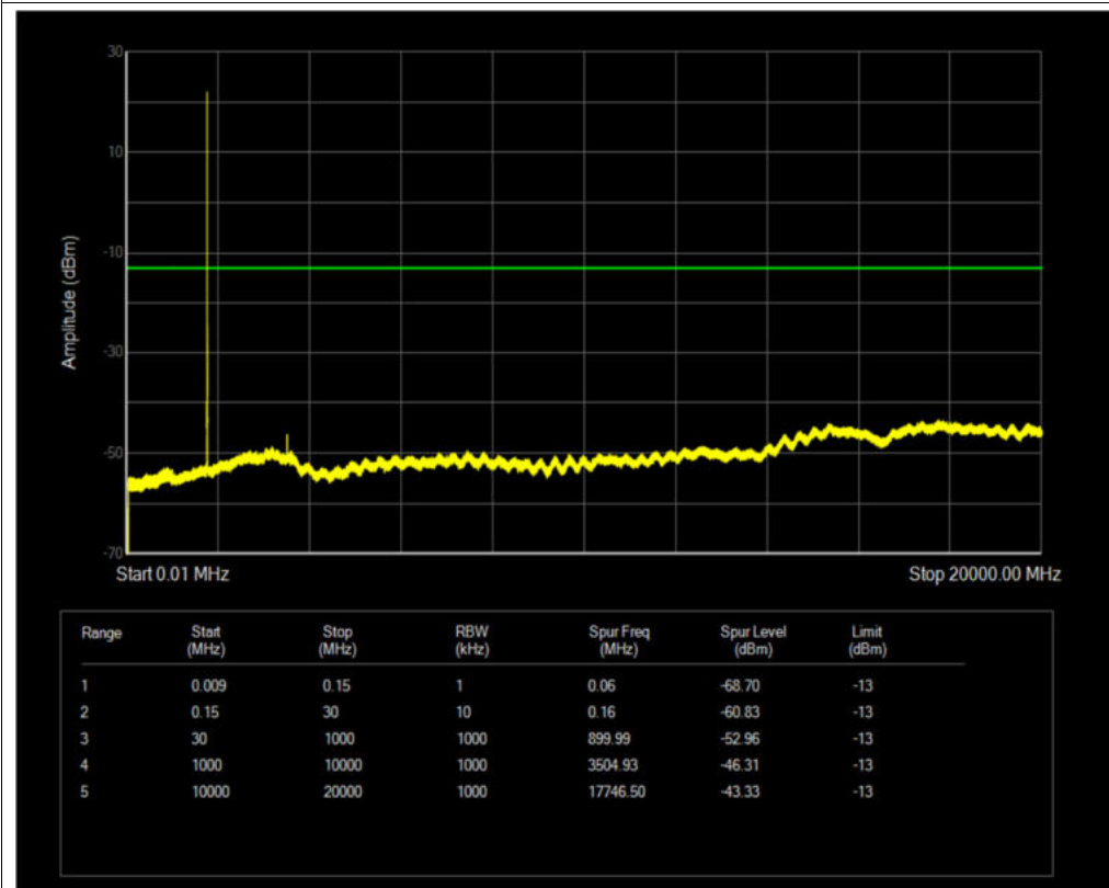
Band4 QPSK BW=3MHz Channel=20385 RB Size=1 Position=#0
