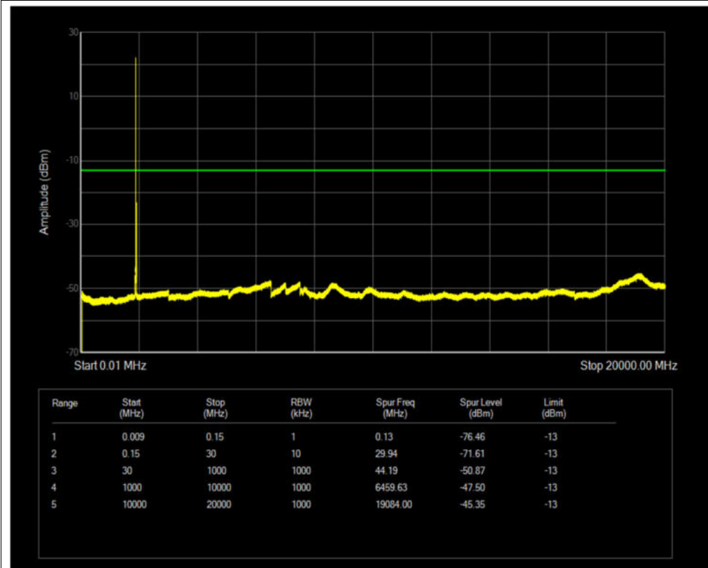
Band2 QPSK BW=15MHz Channel=18900 RB Size=1 Position=#0
