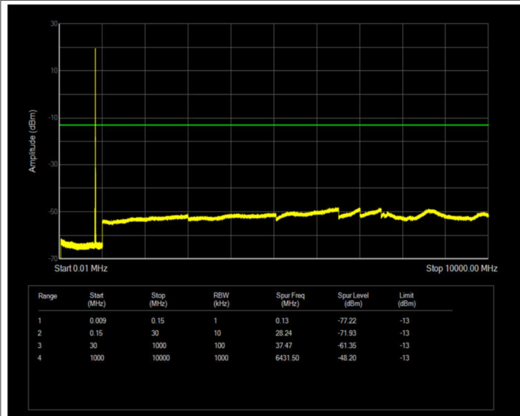
Band5 QPSK BW=5MHz Channel=20525 RB Size=1 Position=#0
