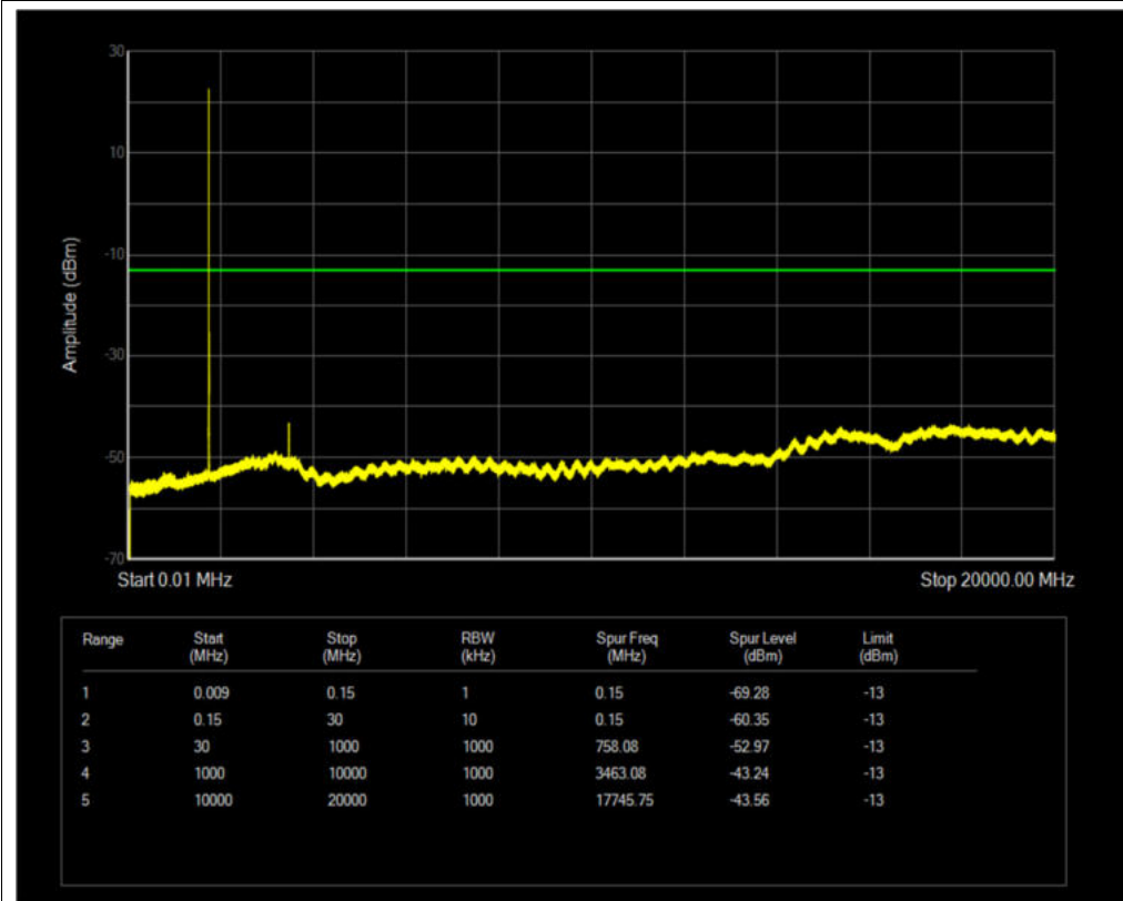
Band4 QPSK BW=3MHz Channel=20175 RB Size=1 Position=#0
