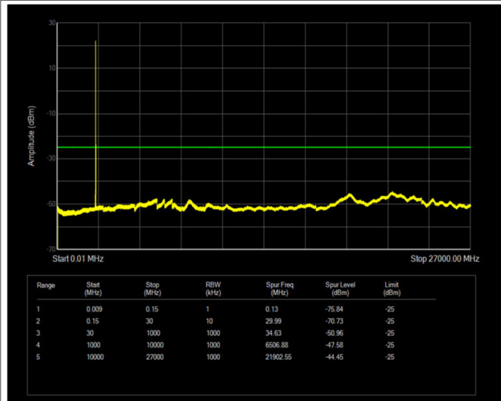
Band7 QPSK BW=10MHz Channel=20800 RB Size=1 Position=#0
