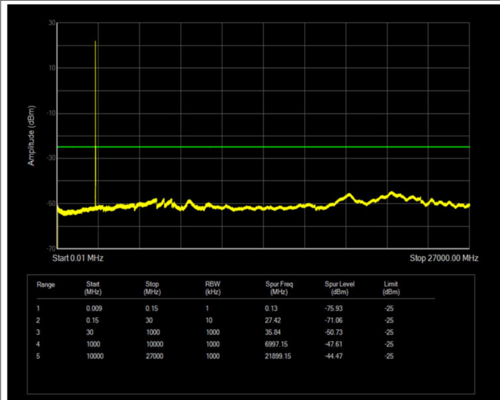
Band7 QPSK BW=5MHz Channel=20775 RB Size=1 Position=#0
