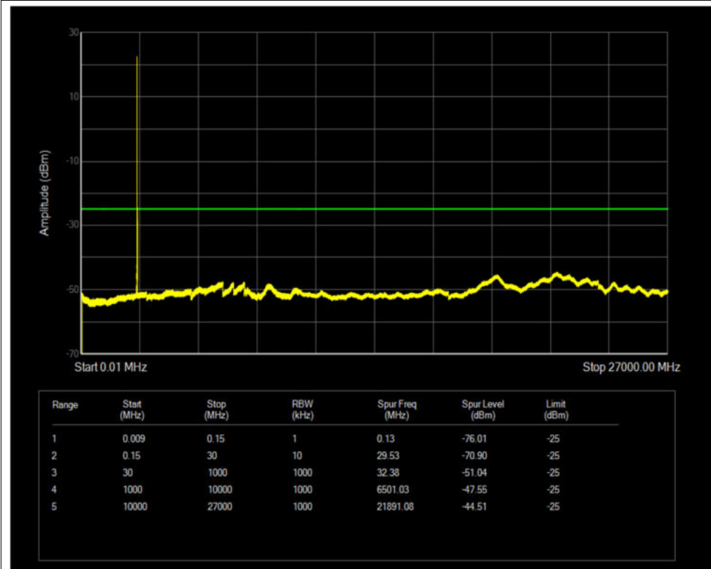
Band7 QPSK BW=10MHz Channel=21400 RB Size=1 Position=#0
