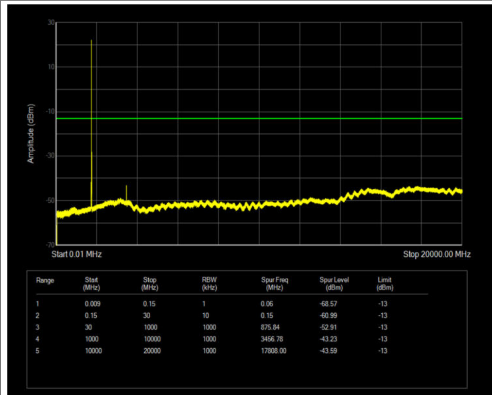
Band4 QPSK BW=10MHz Channel=20175 RB Size=1 Position=#0
