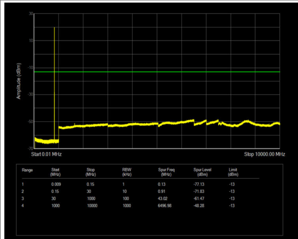
Band5 QPSK BW=1.4MHz Channel=20407 RB Size=1 Position=#0
