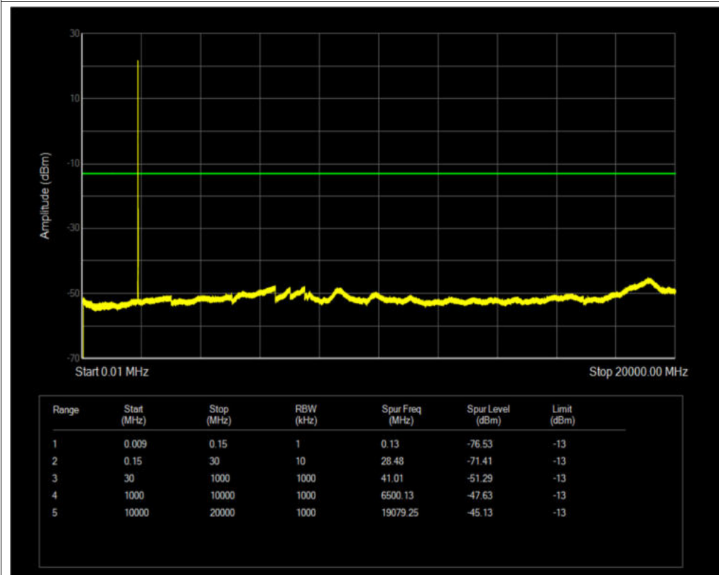
Band2 QPSK BW=5MHz Channel=18900 RB Size=1 Position=#0
