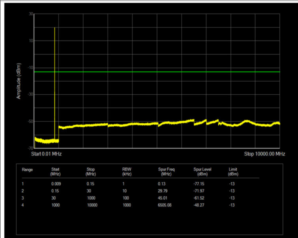
Band5 QPSK BW=1.4MHz Channel=20525 RB Size=1 Position=#0
