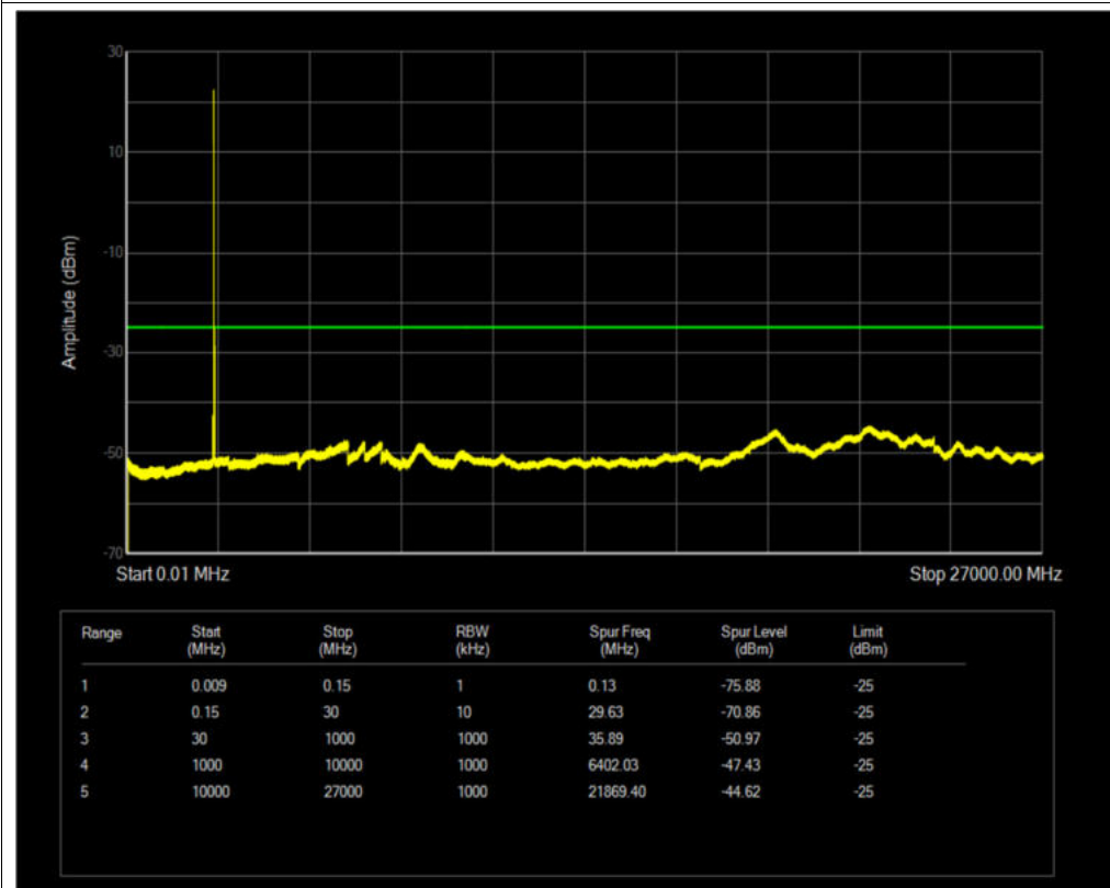
Band7 QPSK BW=15MHz Channel=21375 RB Size=1 Position=#0
