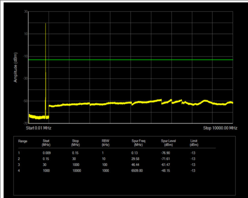
Band5 QPSK BW=10MHz Channel=20600 RB Size=1 Position=#0
