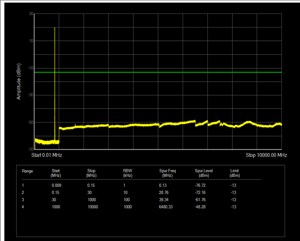
Band26(824-849) QPSK BW=3MHz Channel=26805 RB Size=1 Position=#0
