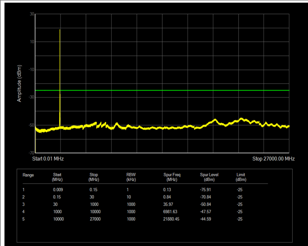
Band38 QPSK BW=15MHz Channel=38175 RB Size=1 Position=#0
