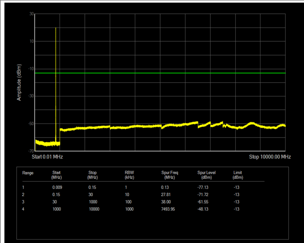
Band26(824-849) QPSK BW=5MHz Channel=26915 RB Size=1 Position=#0
