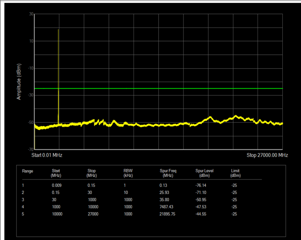
Band38 QPSK BW=10MHz Channel=38000 RB Size=1 Position=#0
