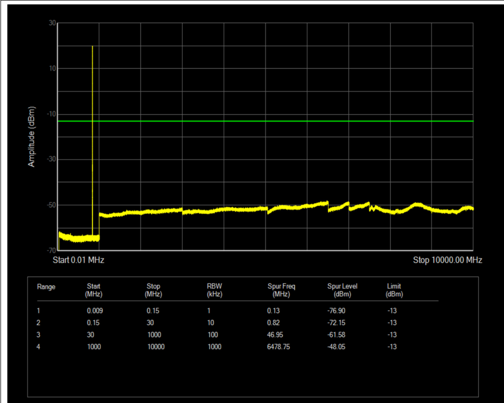
Band26(824-849) QPSK BW=1.4MHz Channel=26915 RB Size=1 Position=#0
