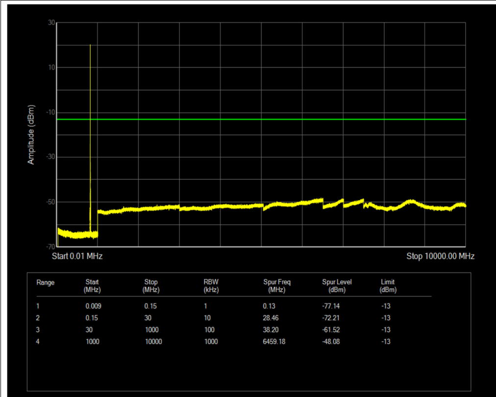
Band26(814-824) QPSK BW=3MHz Channel=26740 RB Size=1 Position=#0
