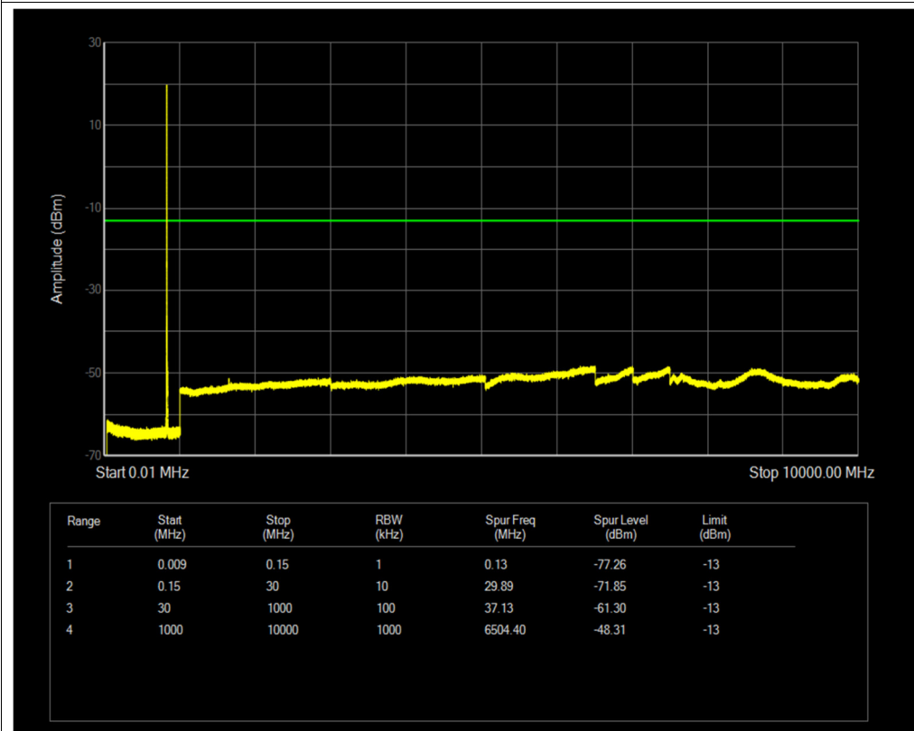
Band26(824-849) QPSK BW=5MHz Channel=26815 RB Size=1 Position=#0
