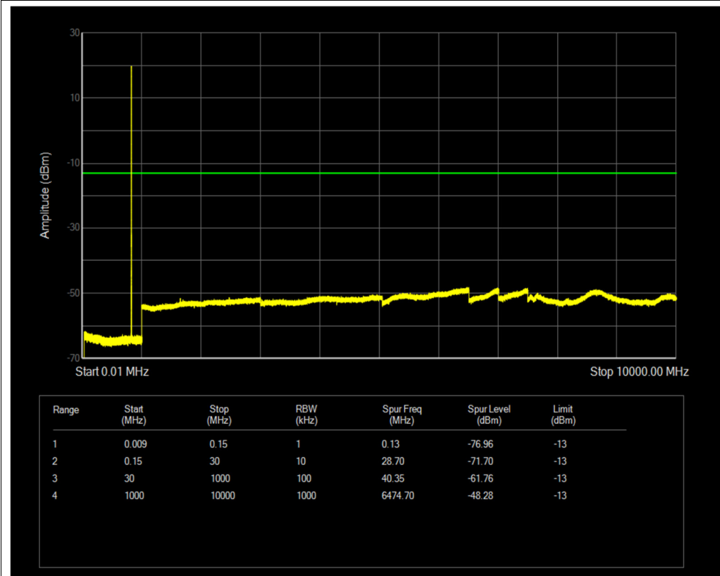
Band26(824-849) QPSK BW=1.4MHz Channel=26797 RB Size=1 Position=#0
