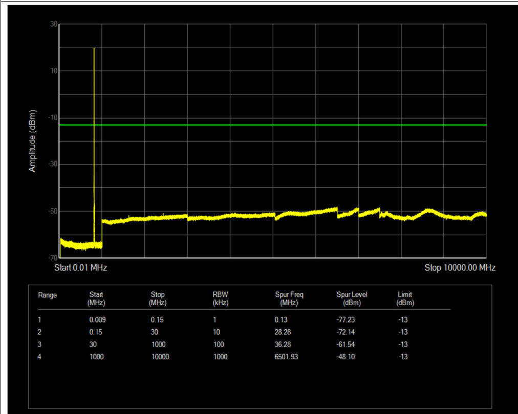
Band26(814-824) QPSK BW=5MHz Channel=26715 RB Size=1 Position=#0
