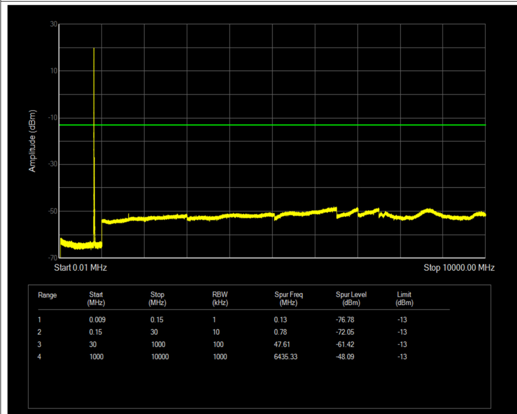
Band26(814-824) QPSK BW=10MHz Channel=26740 RB Size=1 Position=#0
