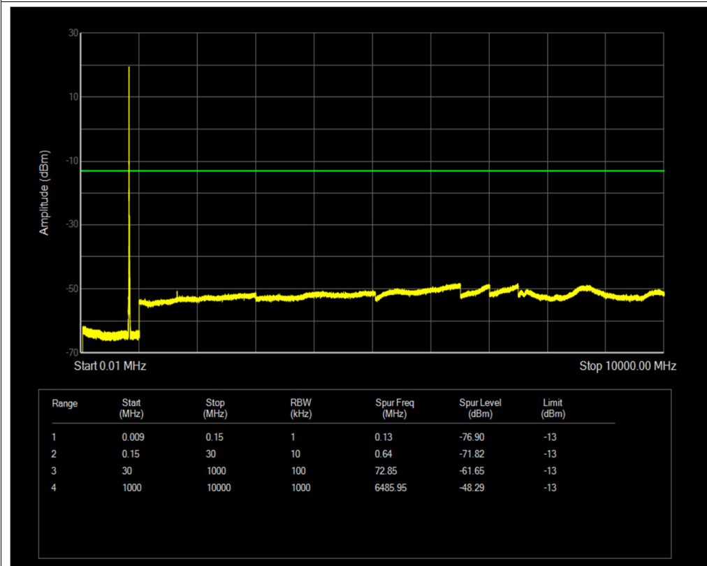
Band26(824-849) QPSK BW=10MHz Channel=26840 RB Size=1 Position=#0
