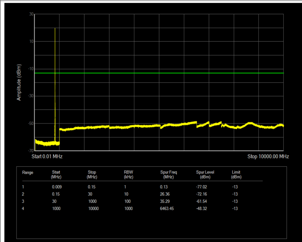
Band26(814-824) QPSK BW=5MHz Channel=26765 RB Size=1 Position=#0
