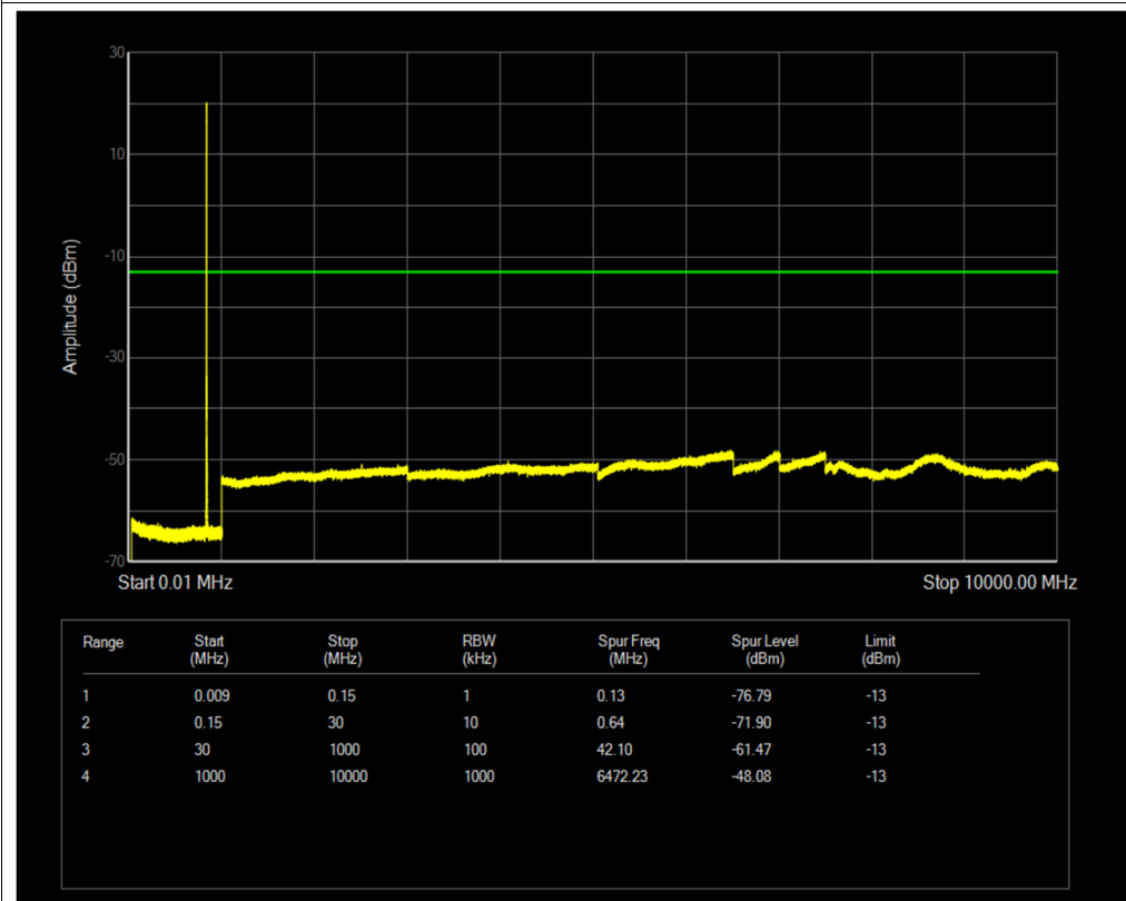
Band26(824-849) QPSK BW=3MHz Channel=26915 RB Size=1 Position=#0
