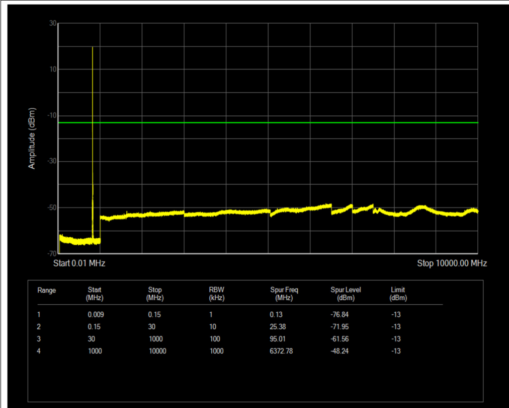
Band26(814-824) QPSK BW=5MHz Channel=26740 RB Size=1 Position=#0
