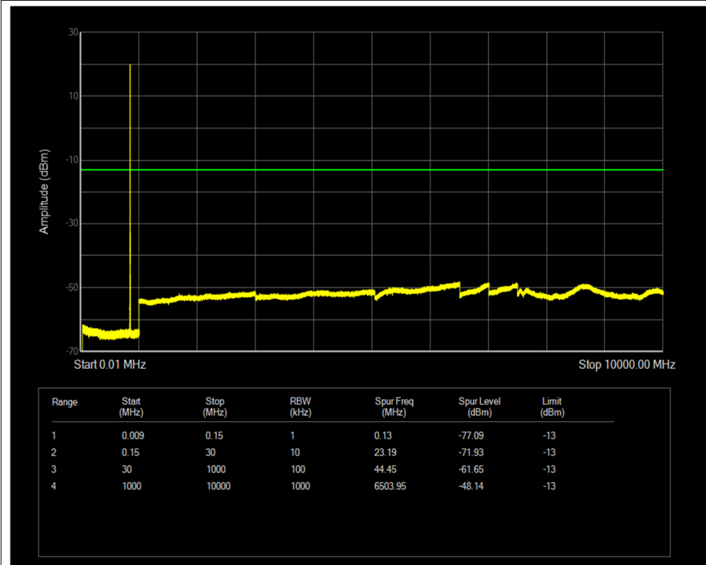
Band26(824-849) QPSK BW=3MHz Channel=27025 RB Size=1 Position=#0
