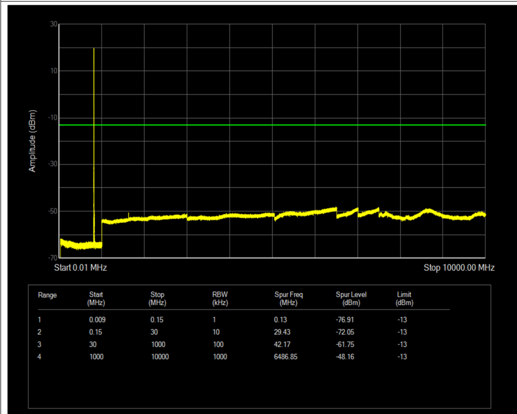
Band26(814-824) QPSK BW=3MHz Channel=26705 RB Size=1 Position=#0
