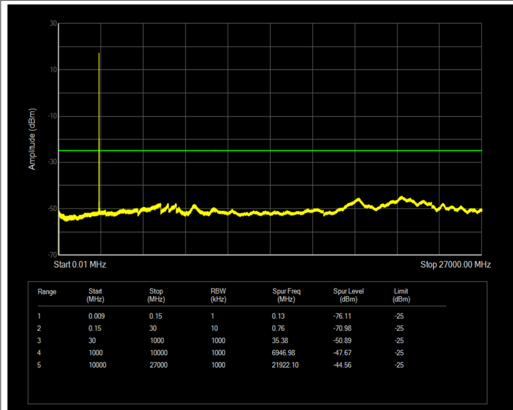
Band38 QPSK BW=10MHz Channel=37800 RB Size=1 Position=#0
