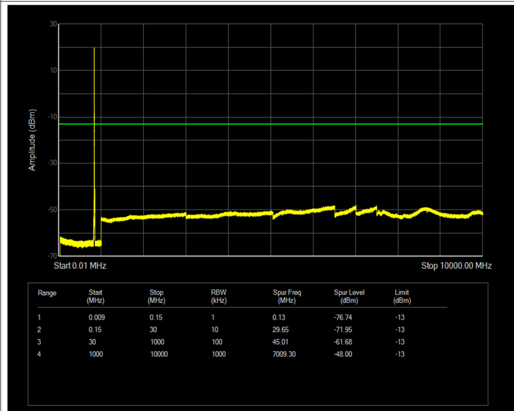
Band26(824-849) QPSK BW=15MHz Channel=26965 RB Size=1 Position=#0
