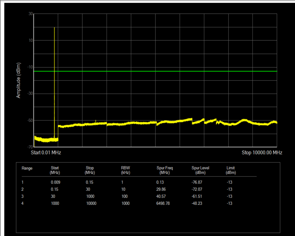
Band26(824-849) QPSK BW=1.4MHz Channel=27033 RB Size=1 Position=#0
