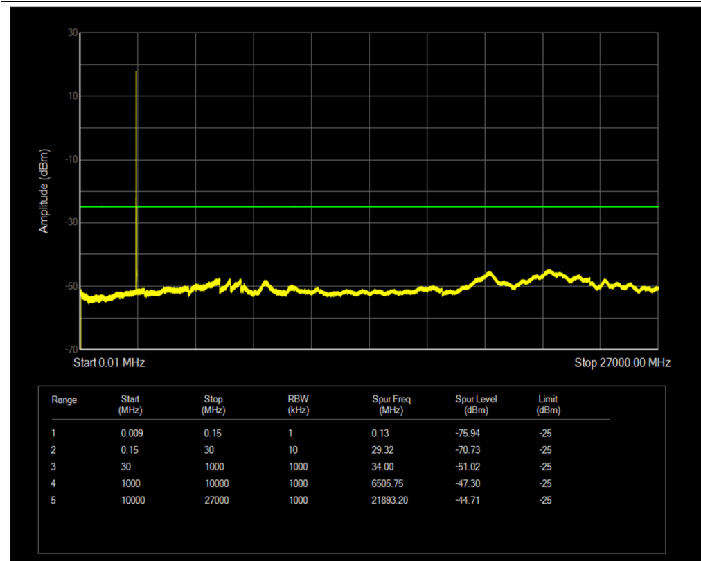
Band38 QPSK BW=10MHz Channel=38200 RB Size=1 Position=#0
