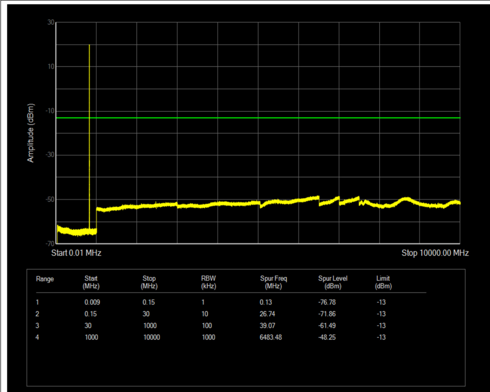
Band26(814-824) QPSK BW=1.4MHz Channel=26783 RB Size=1 Position=#0
