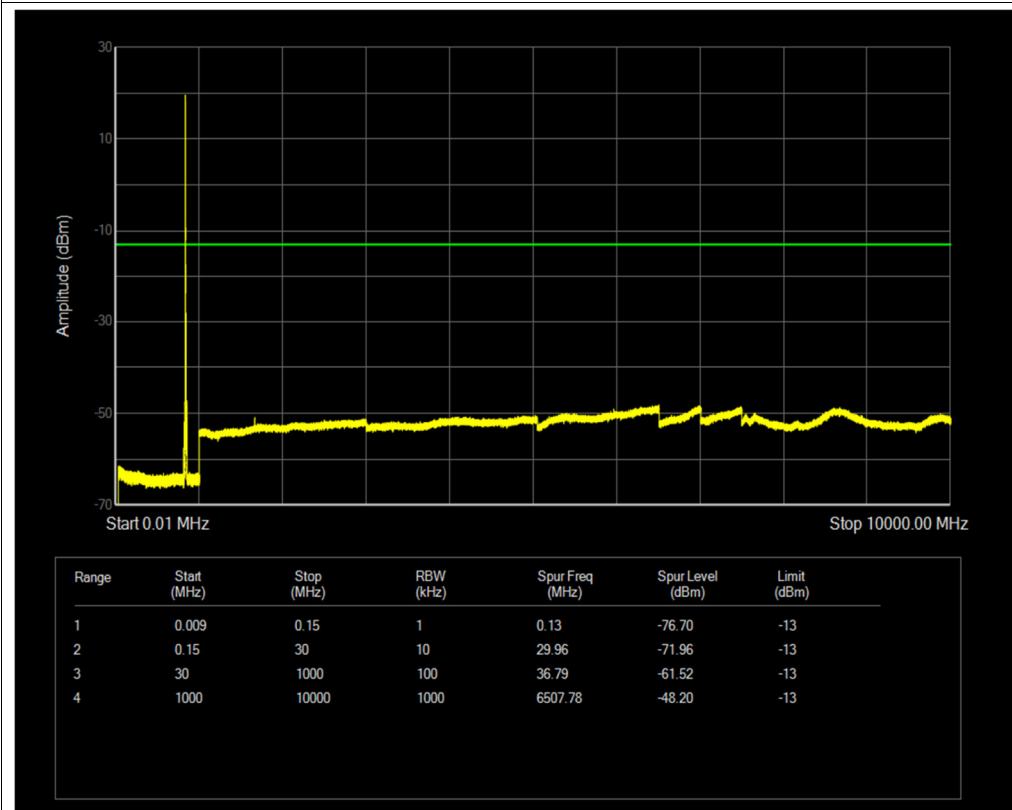
Band26(824-849) QPSK BW=10MHz Channel=26915 RB Size=1 Position=#0
