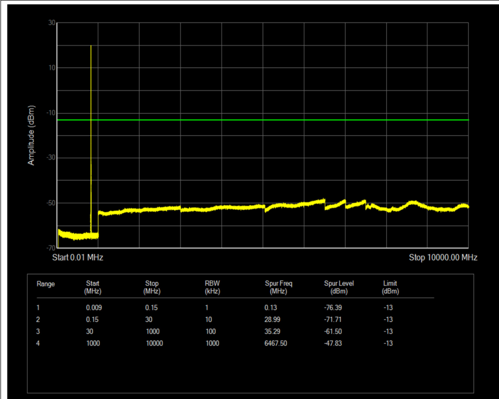
Band26(814-824) QPSK BW=3MHz Channel=26775 RB Size=1 Position=#0
