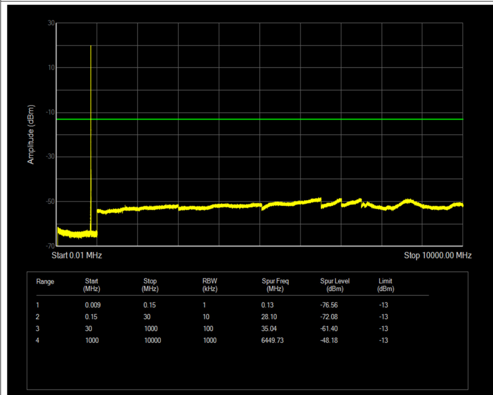
Band26(824-849) QPSK BW=5MHz Channel=27015 RB Size=1 Position=#0
