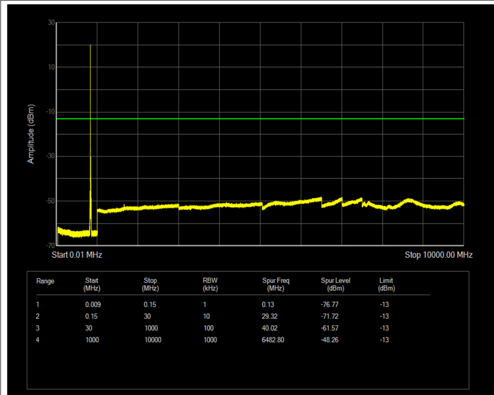
Band26(824-849) QPSK BW=15MHz Channel=26915 RB Size=1 Position=#0
