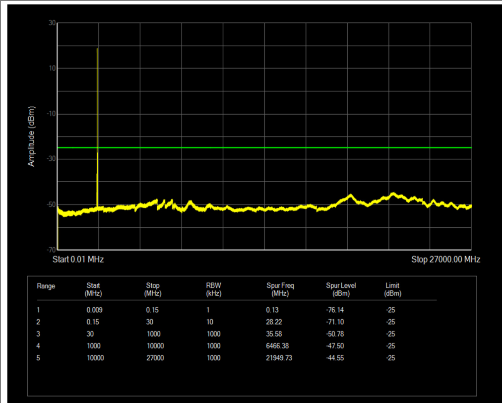
Band38 QPSK BW=15MHz Channel=38000 RB Size=1 Position=#0
