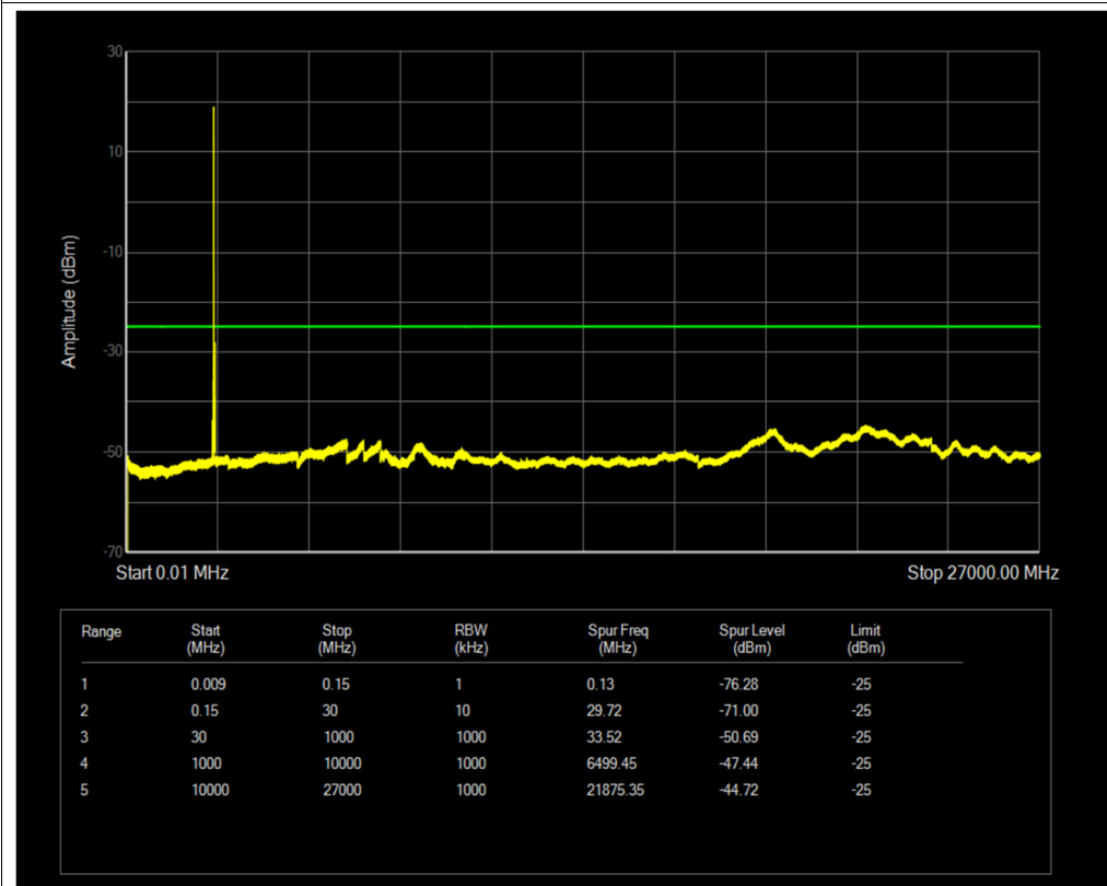
Band38 QPSK BW=20MHz Channel=37850 RB Size=1 Position=#0
