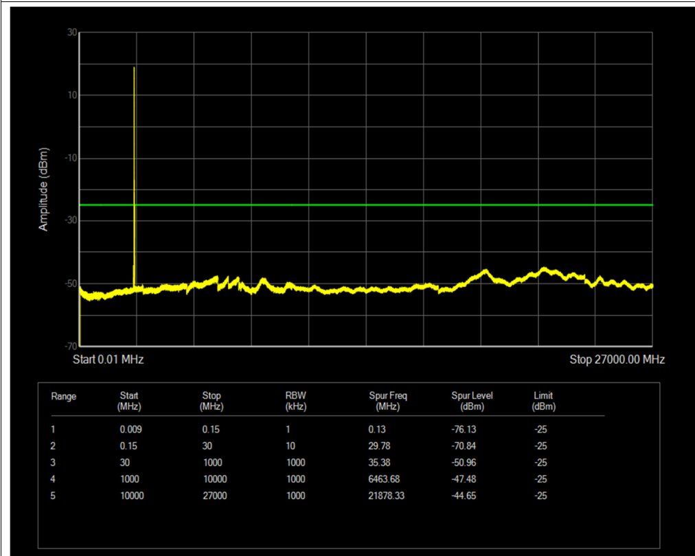
Band38 QPSK BW=15MHz Channel=37825 RB Size=1 Position=#0
