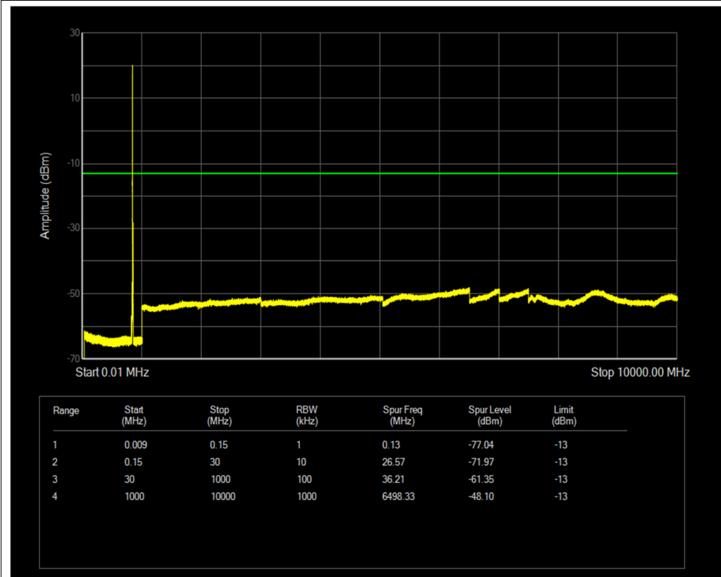
Band26(824-849) QPSK BW=10MHz Channel=26990 RB Size=1 Position=#0
