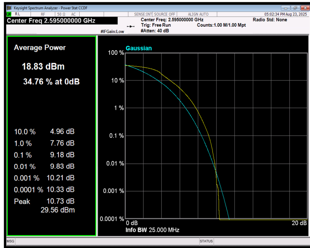
Band38 QPSK BW=5MHz Channel=38000 RB Size=25 Position=#0
