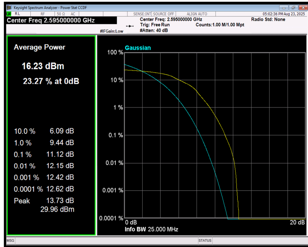
Band38 16QAM BW=5MHz Channel=38000 RB Size=25 Position=#0
