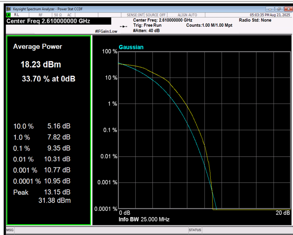
Band38 16QAM BW=20MHz Channel=38150 RB Size=100 Position=#0
