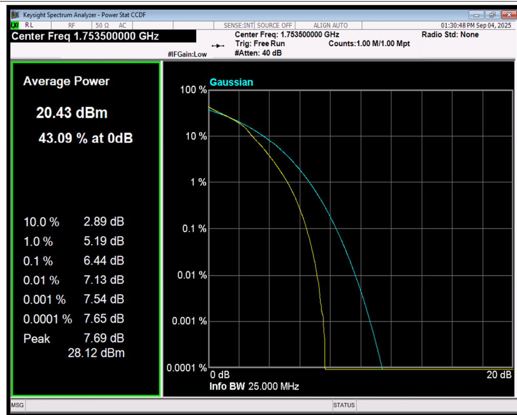
Band4 16QAM BW=3MHz Channel=20385 RB Size=15 Position=#0
