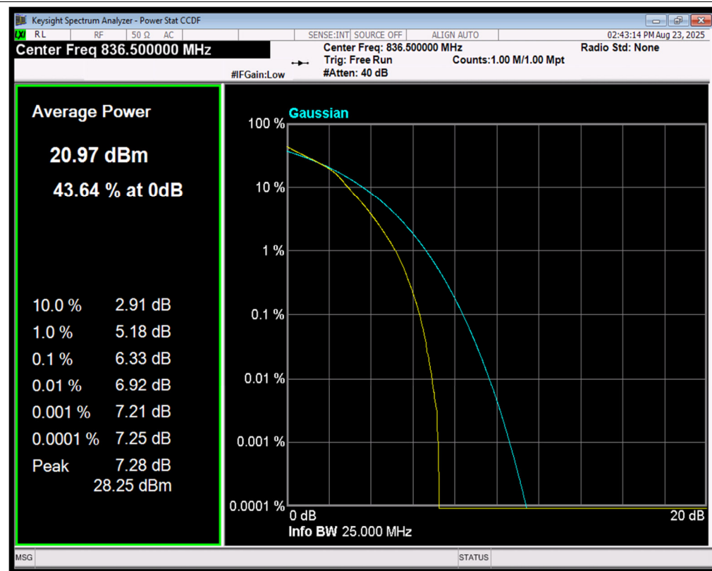
Band5 16QAM BW=3MHz Channel=20525 RB Size=15 Position=#0
