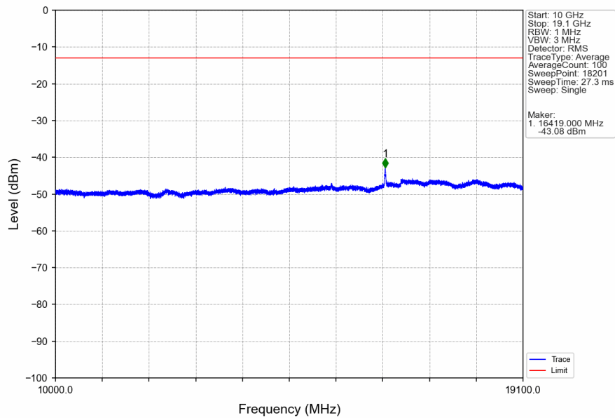
Band2_HSDPA_MCH_1880MHz_Subtest 1_NTNV
