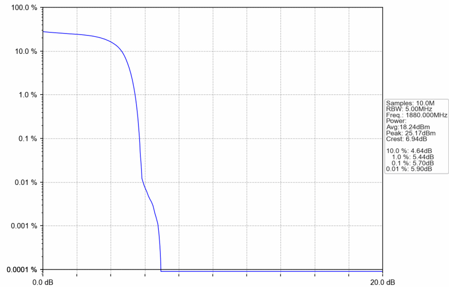
Band2_HSDPA_MCH_1880MHz_Subtest 1_NTNV
