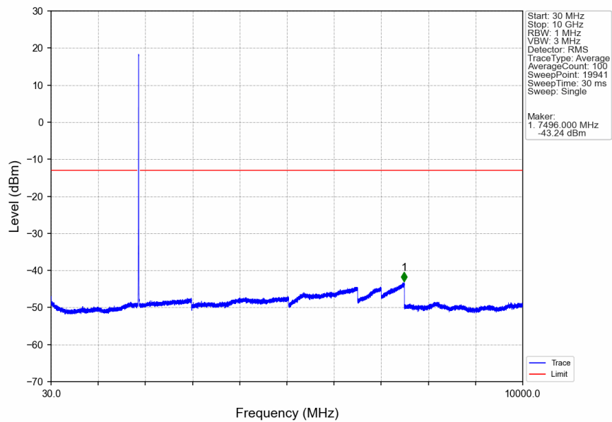
Band2_RMC_MCH_1880MHz_12.2kbps RMC_NTNV
