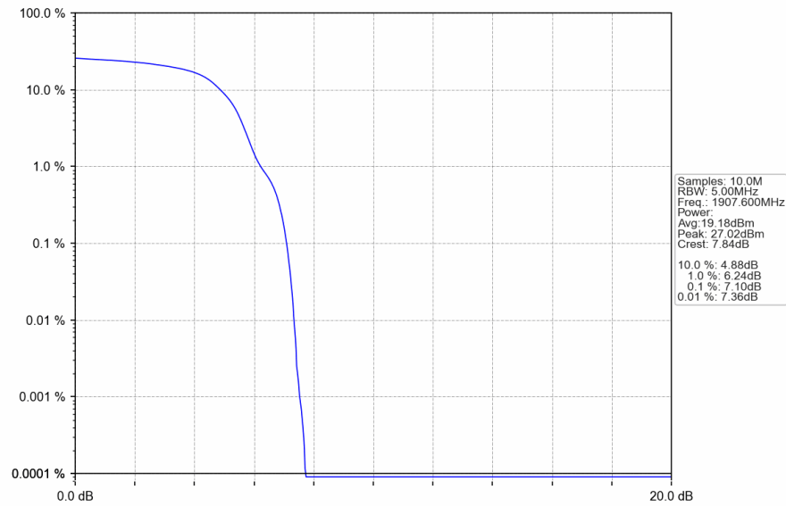
Band2_HSUPA_HCH_1907.6MHz_Subtest 1_NTNV
