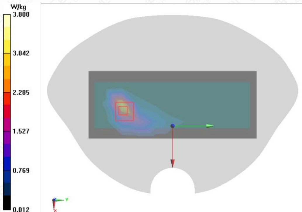
Figure A.1-8 WCDMA BandⅣ Right Side Mode Middle 0mm
