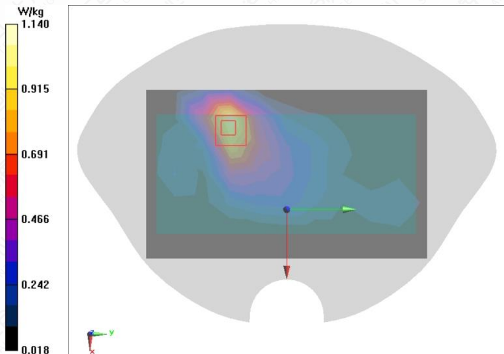
Figure A.1-7 WCDMA BandIV Front Side Mode Middle 5mm
