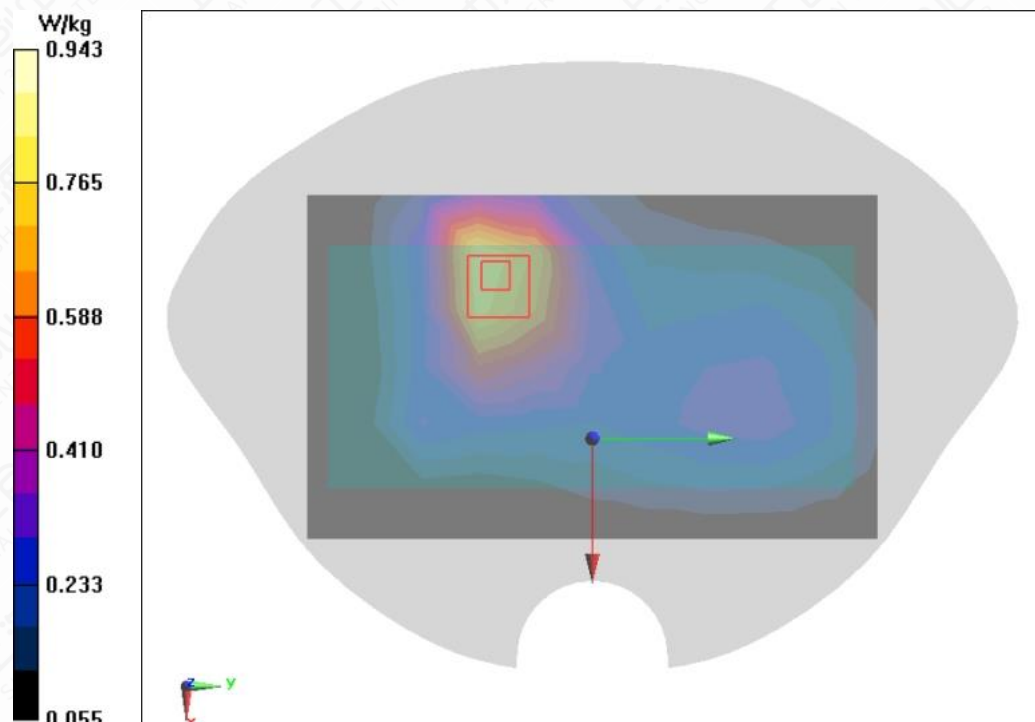
Figure A.1-1 GSM850 GPRS 4TS Front Side Mode Middle 5mm
