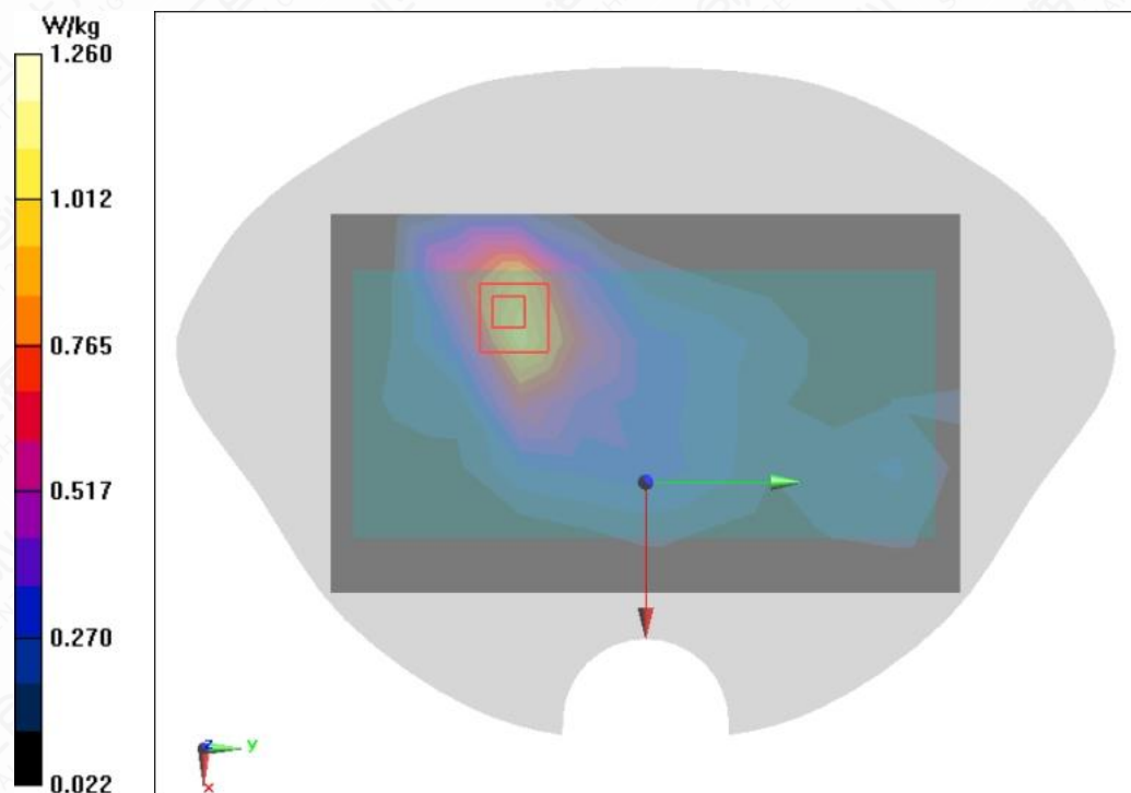
Figure A.1-5 WCDMA Band II Front Side Mode Middle 5mm
