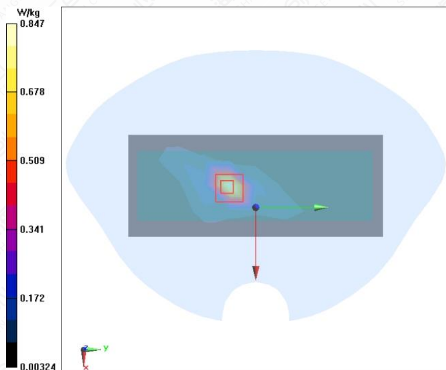
Figure A.1-25 Wi-Fi 2.4G 802.11b Right Side Mode Middle 5mm
