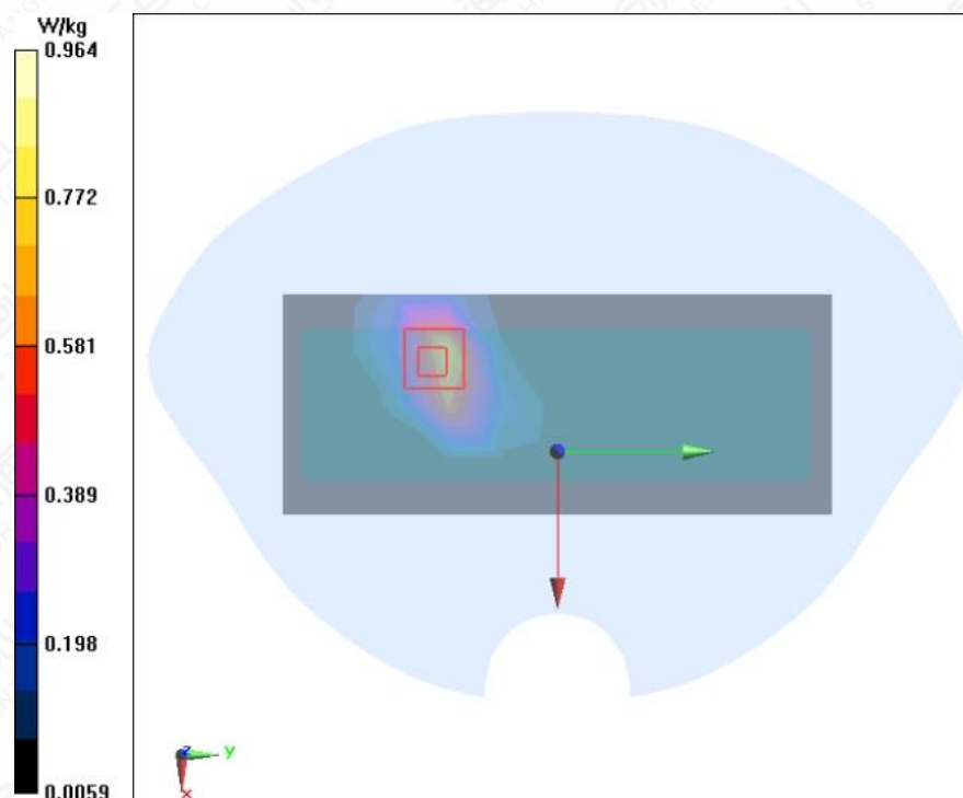
Figure A.1-23 LTE B41 20MHz 1RB 50offset Right Side Mode Low 5mm
