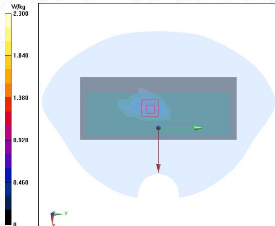
Figure A.1-32 Wi-Fi 5G U-NII-2C 802.11a Right Side Mode High 0mm
