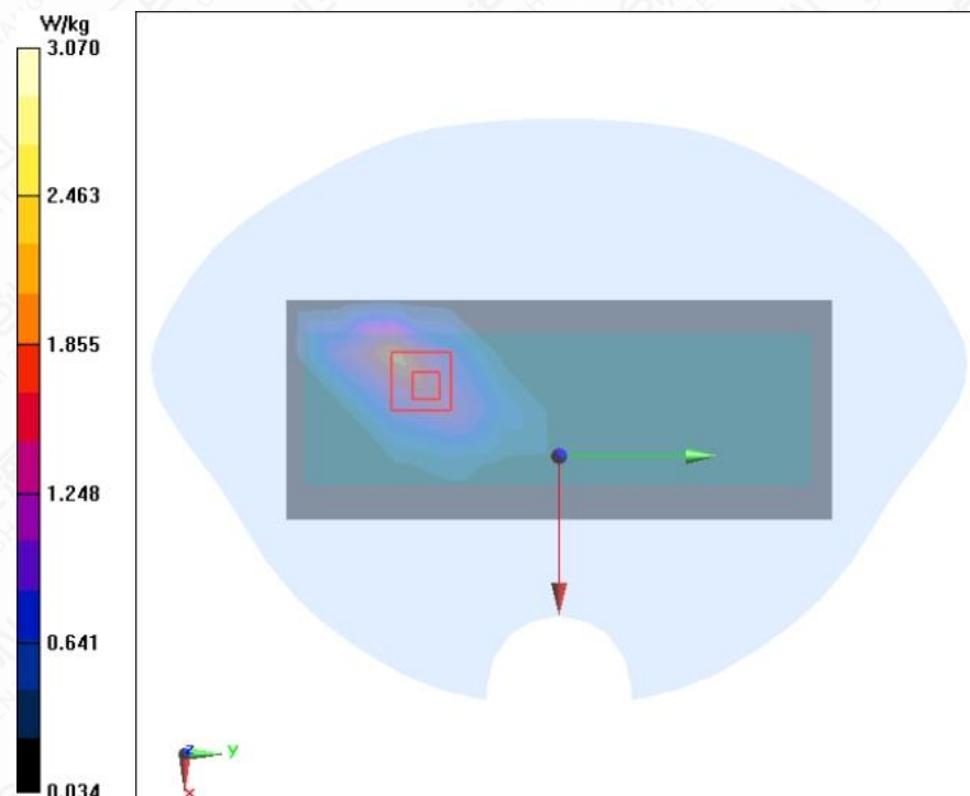
Figure A.1-18 LTE B26 15MHz 36RB 0offset Right Side Mode Middle 0mm
