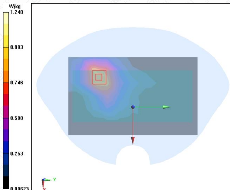
Figure A.1-15 LTE B7 20MHz 50RB 0offset Front Side Mode Low 5mm
