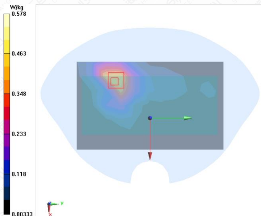
Figure A.1-19 LTE B40 10MHz 1RB 25offset Front Side Mode Middle 5mm
