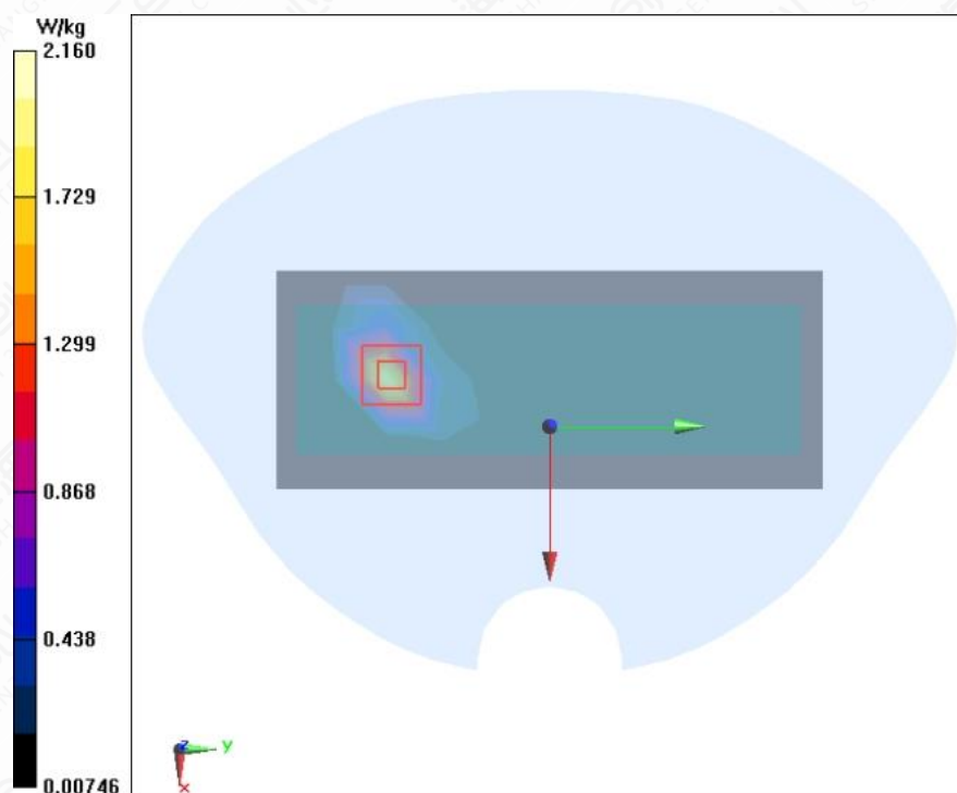
Figure A.1-20 LTE B40 10MHz 1RB 25offset Right Side Mode Middle 0mm
