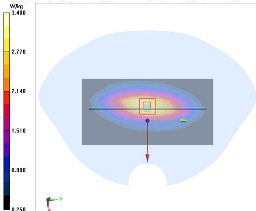
Figure A.2-1 System Check 835MHz
