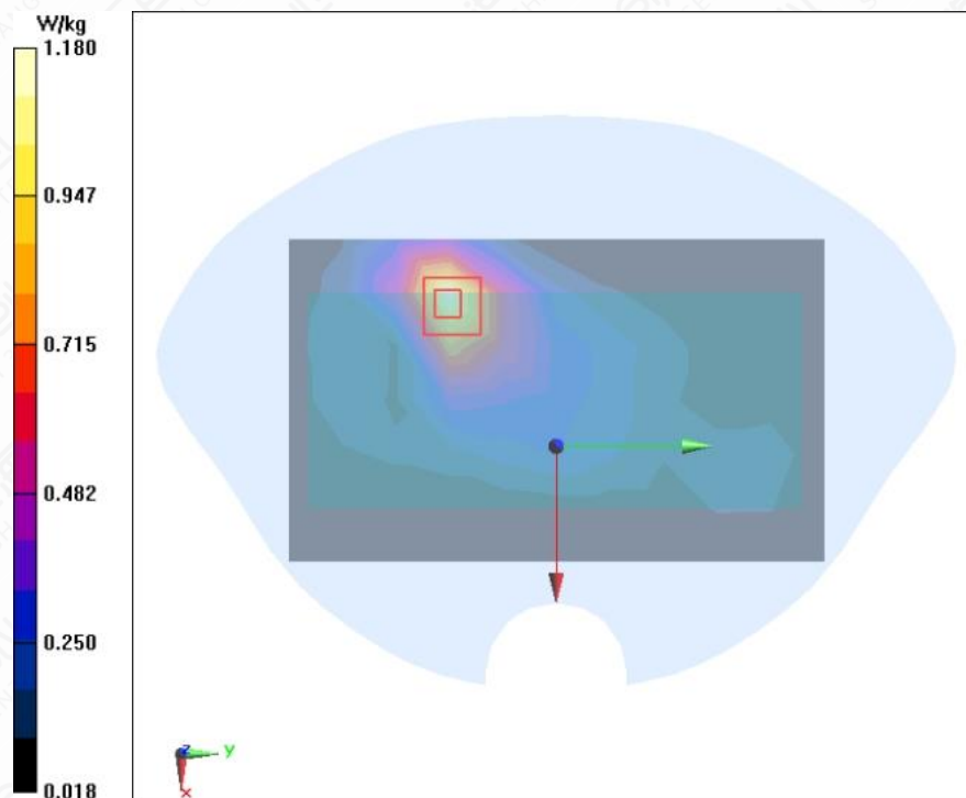
Figure A.1-5 WCDMA Band II RMC Front Side Mode Middle 5mm
