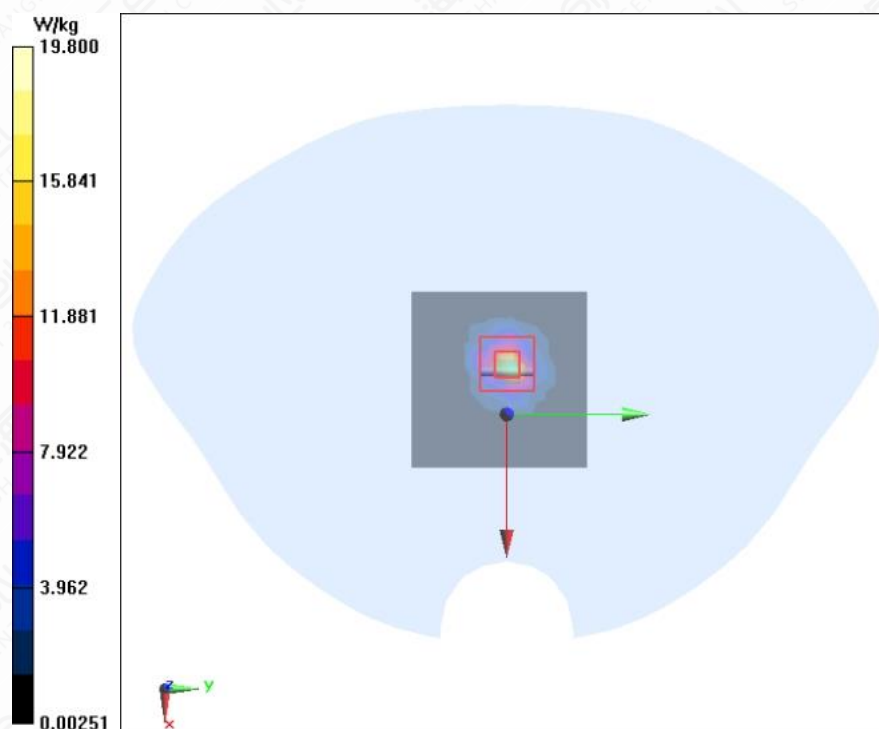
Figure A.2-12 System Check 5300MHz
