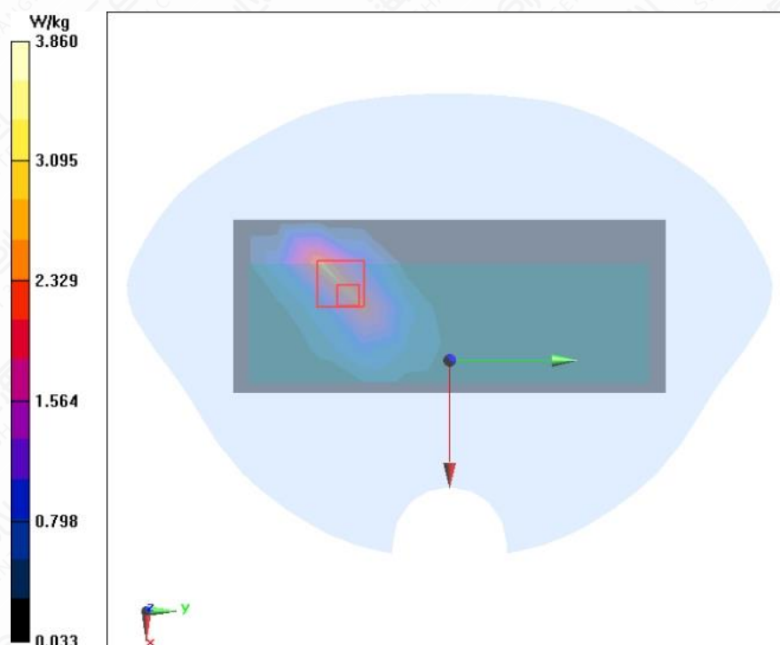
Figure A.1-2 GSM850 GPRS 4TS Right Side Mode Middle 0mm
