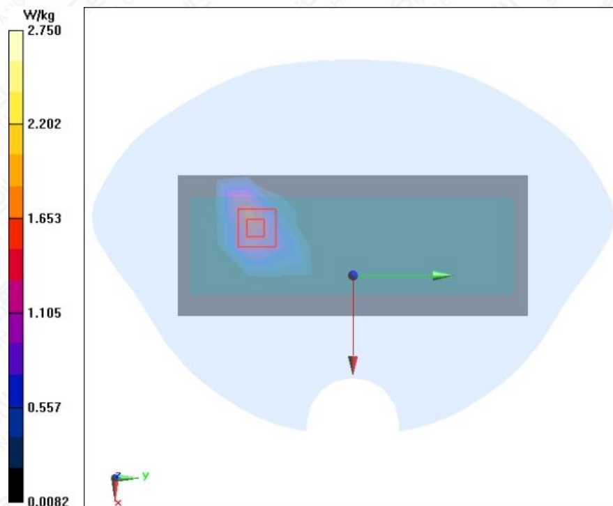
Figure A.1-16 LTE B7 20MHz 1RB 50offset Right Side Mode Middle 0mm
