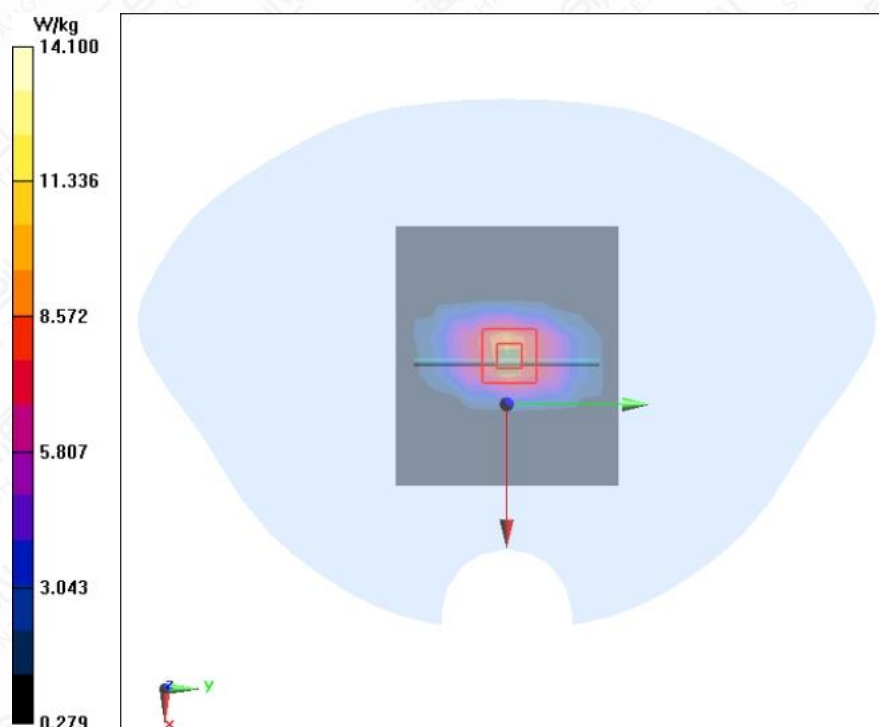
Figure A.2-4 System Check 1750MHz
