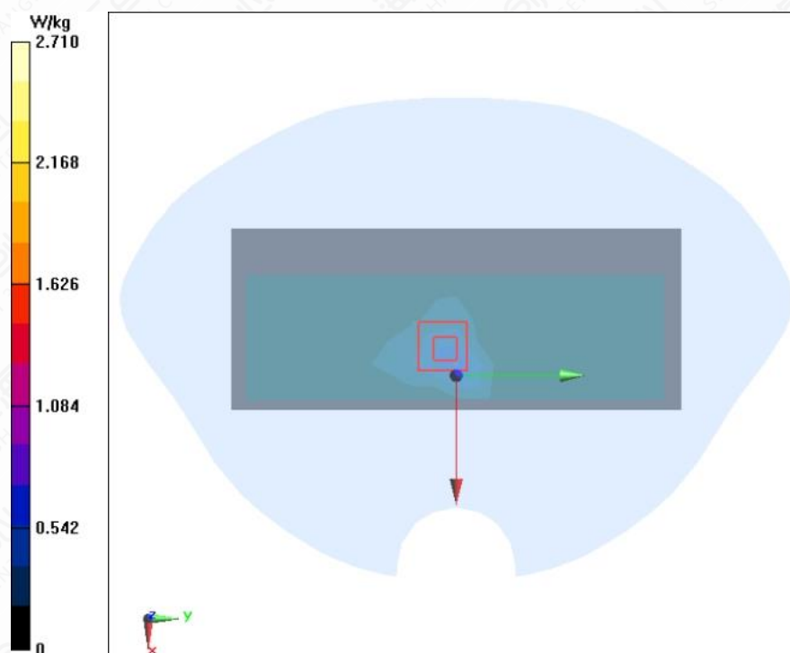
Figure A.1-30 Wi-Fi 5G U-NII-2A 802.11a Right Side Mode High 0mm
