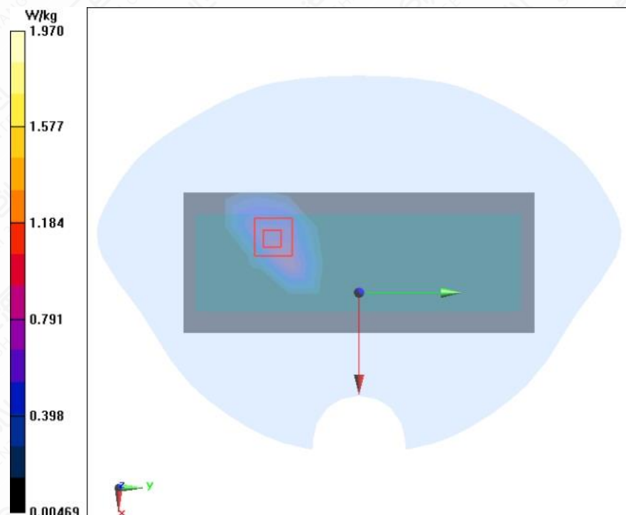
Figure A.1-24 LTE B41 20MHz 1RB 50offset Right Side Mode Middle 0mm
