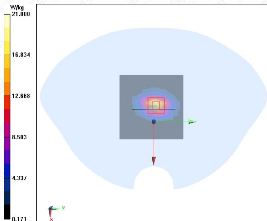
Figure A.2-7 System Check 2300MHz
