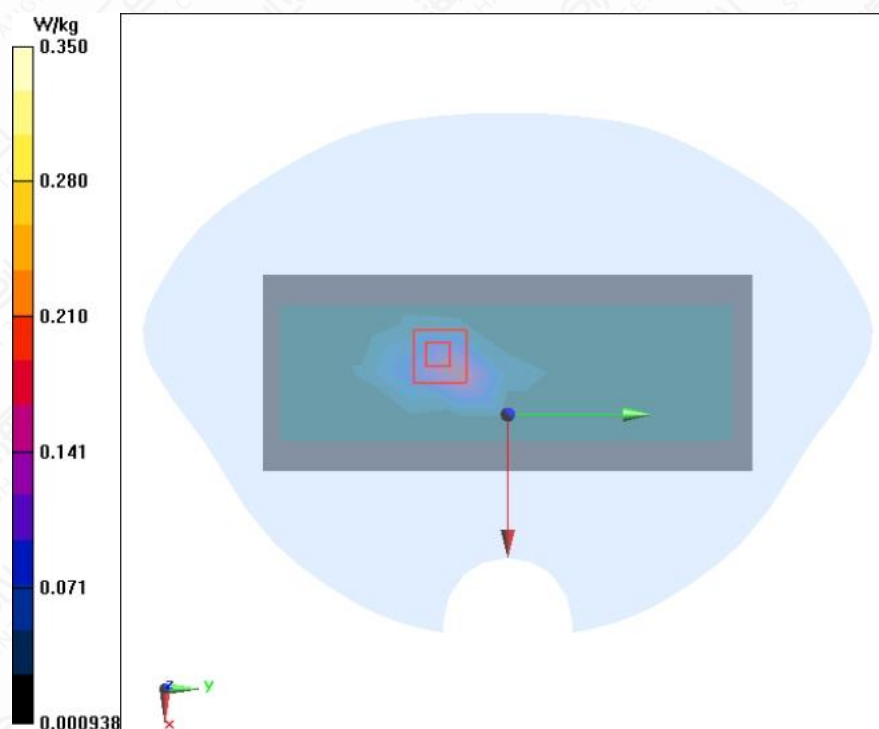
Figure A.1-36 BT DH5 Right Side Mode Middle 0mm
