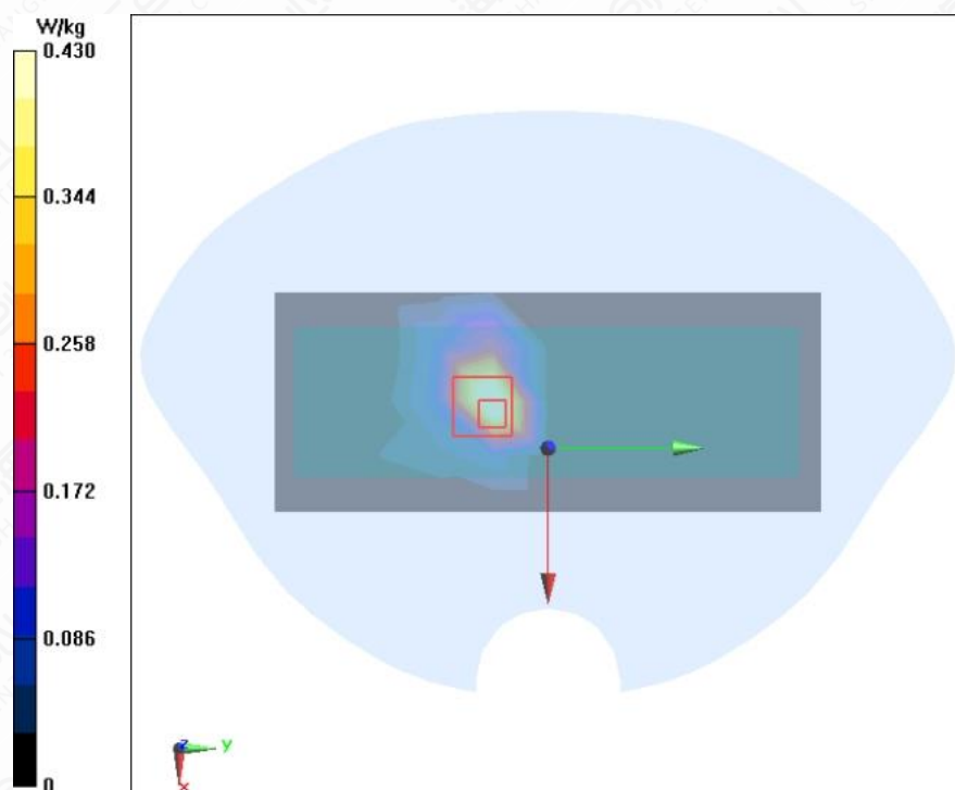
Figure A.1-27 Wi-Fi 5G U-NII-1 802.11a Right Side Mode Middle 5mm
