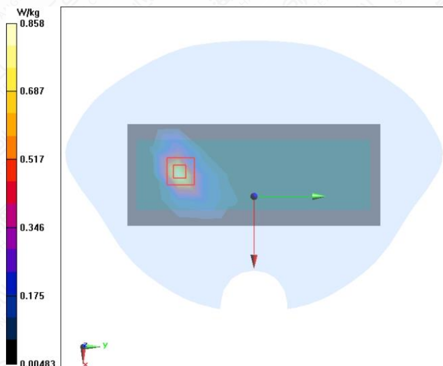
Figure A.1-21 LTE B40 10MHz 1RB 25offset Right Side Mode Middle 5mm
