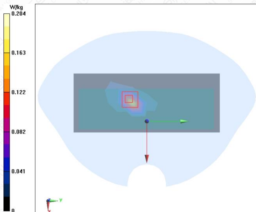
Figure A.1-35 BT DH5 Right Side Mode Middle 5mm
