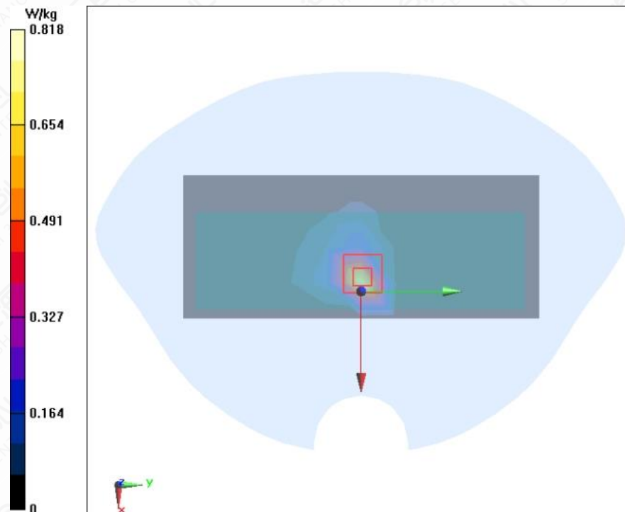
Figure A.1-29 Wi-Fi 5G U-NII-2A 802.11a Right Side Mode High 5mm
