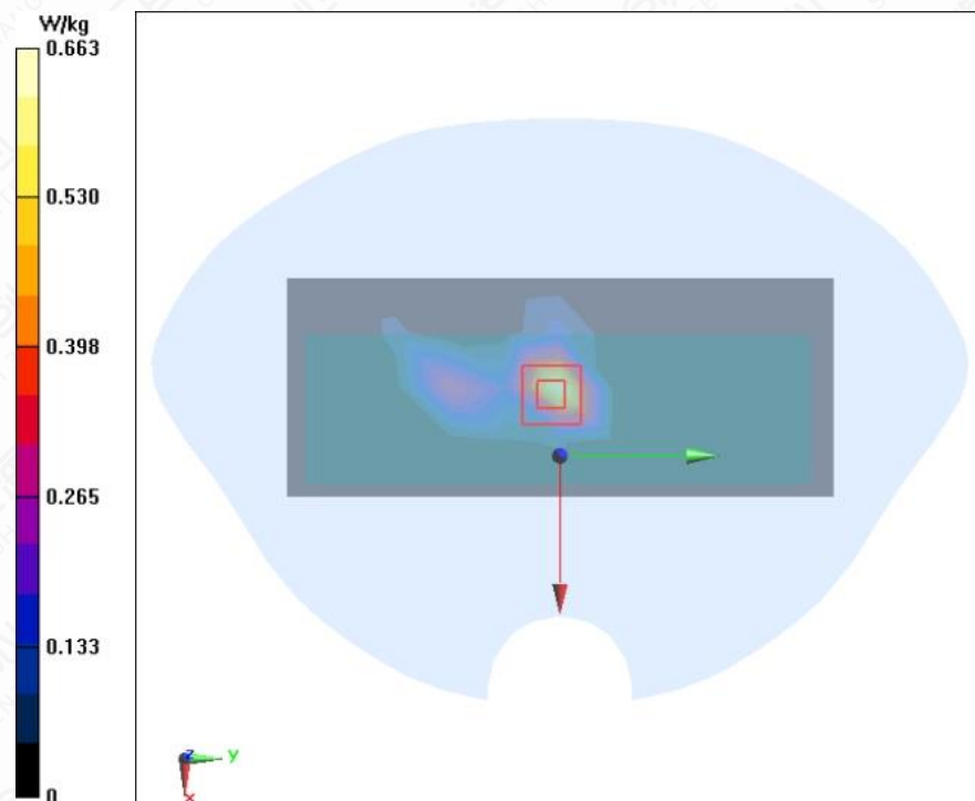
Figure A.1-31 Wi-Fi 5G U-NII-2C 802.11a Right Side Mode High 5mm
