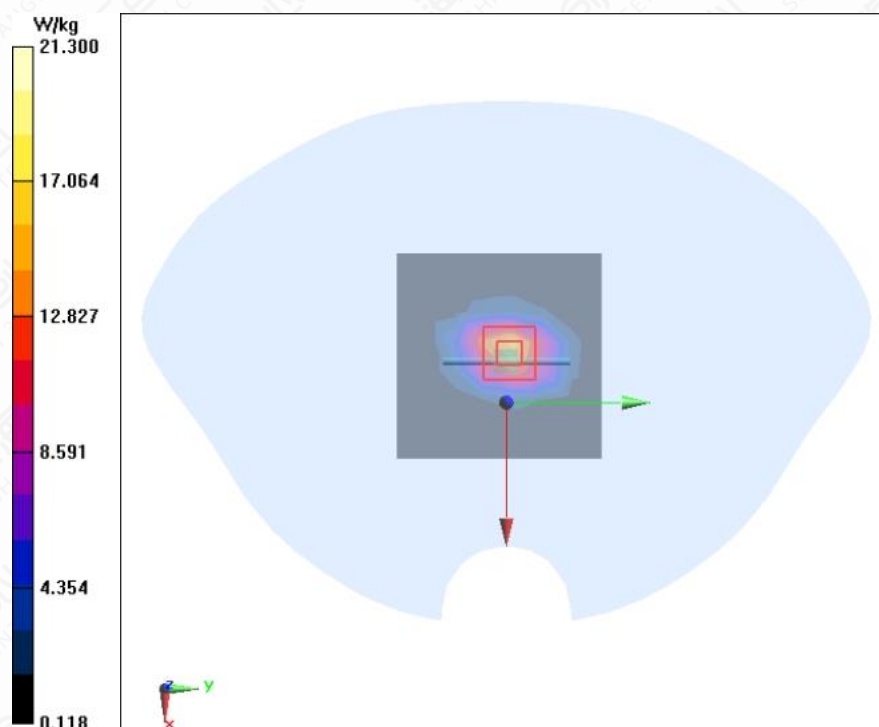
Figure A.2-8 System Check 2450MHz
