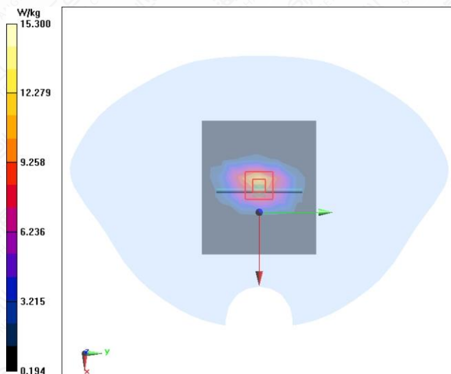
Figure A.2-5 System Check 1900MHz
