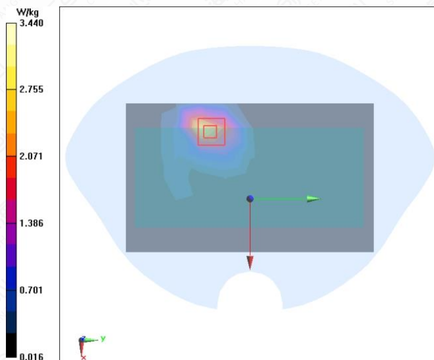
Figure A.1-6 WCDMA Band II RMC Front Side Mode Middle 0mm
