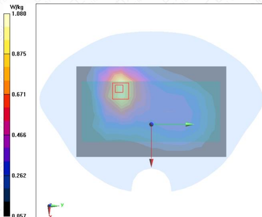
Figure A.1-1 GSM850 GPRS 4TS Front Side Mode Middle 5mm
