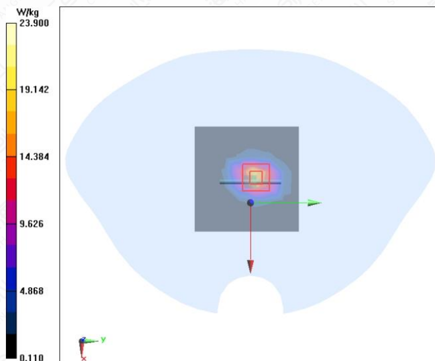
Figure A.2-9 System Check 2600MHz
