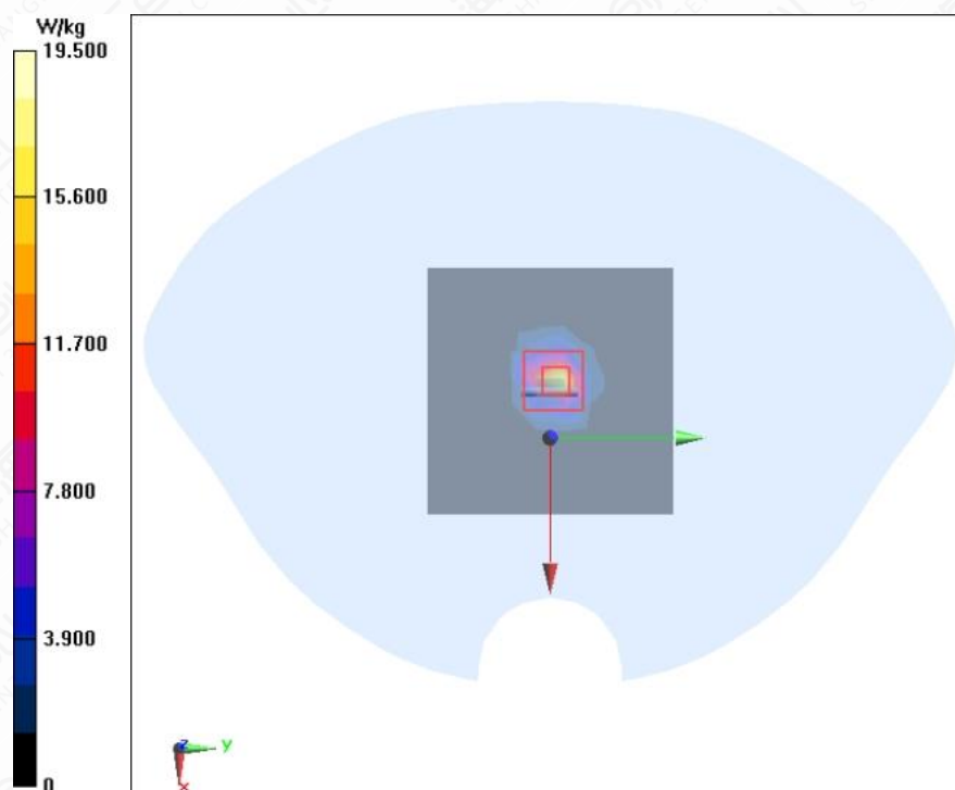
Figure A.2-11 System Check 5200MHz
