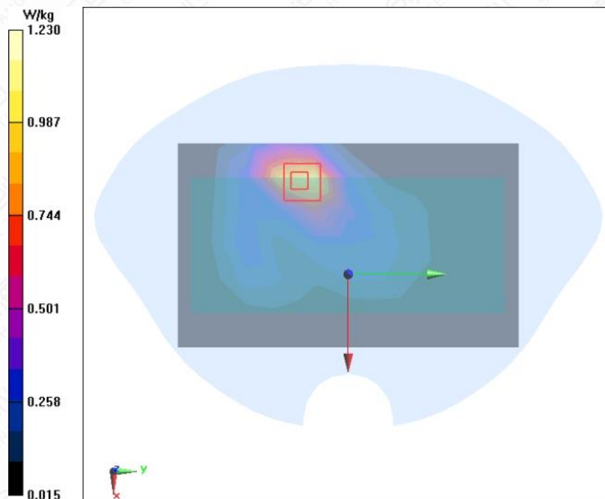
Figure A.1-7 WCDMA BandIV RMC Front Side Mode Middle 5mm
