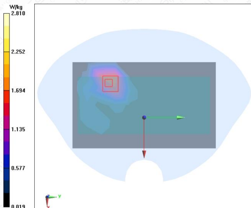
Figure A.1-14 LTE B4 20MHz 1RB 50offset Front Side Mode Middle 0mm
