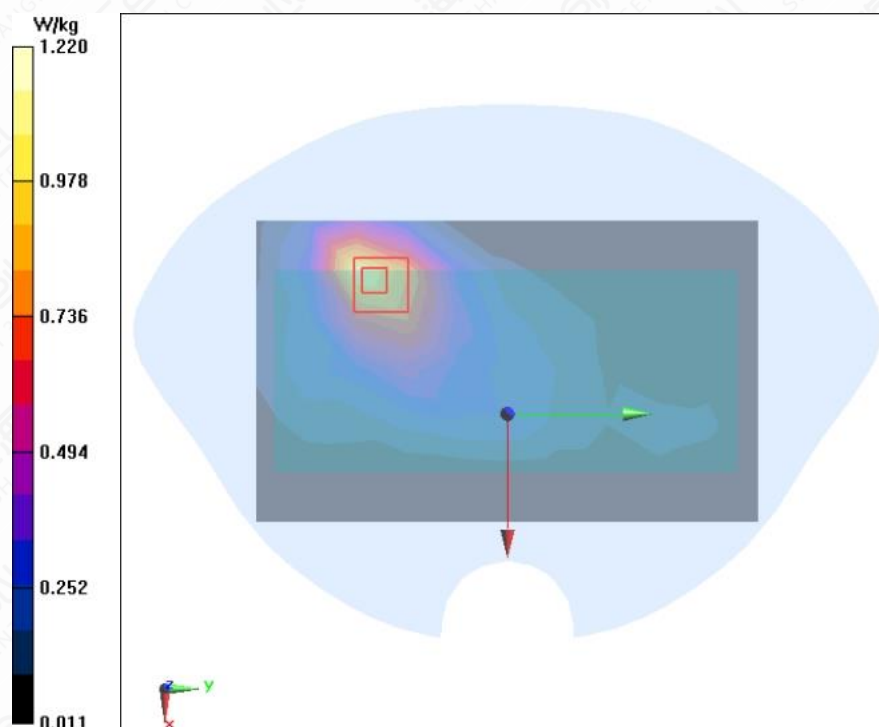
Figure A.1-11 LTE B2 20MHz 1RB 50offset Front Side Mode High 5mm
