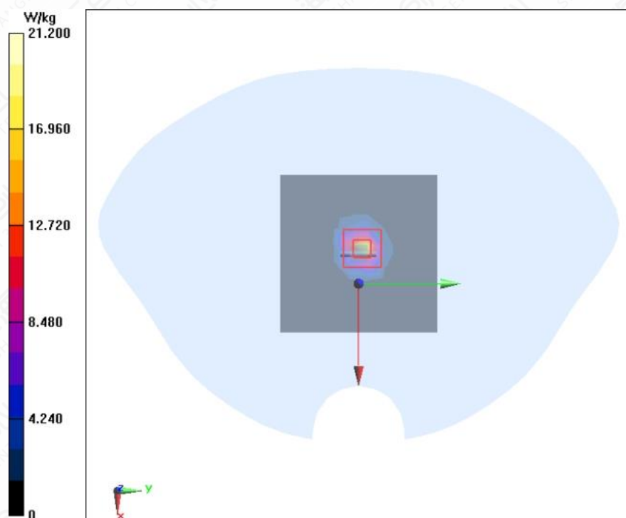
Figure A.2-13 System Check 5600MHz
