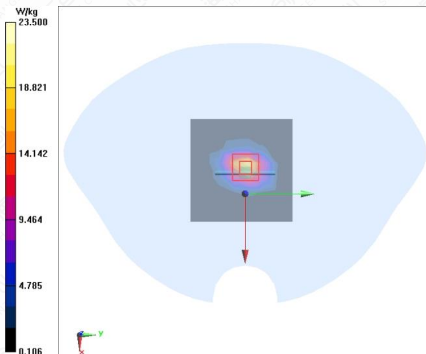
Figure A.2-10 System Check 2600MHz
