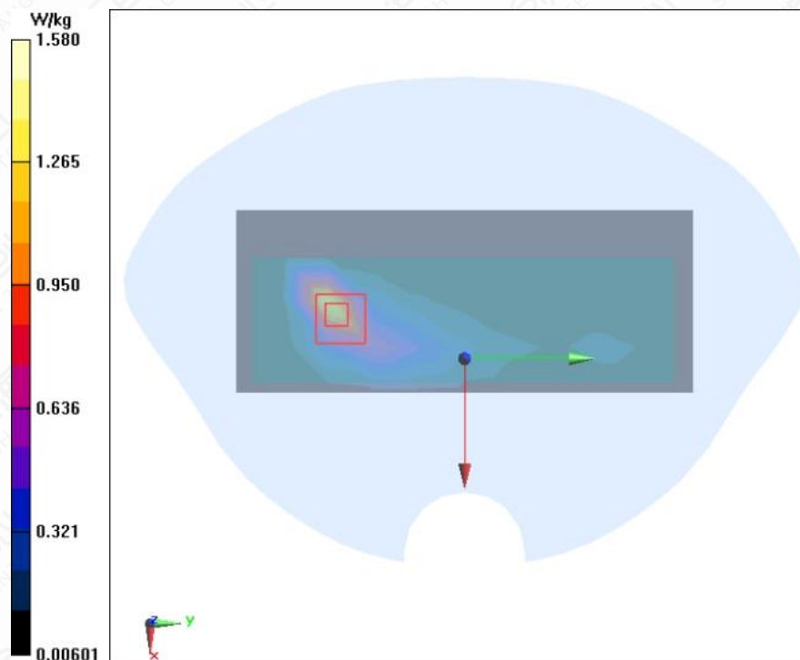
Figure A.1-3 GSM1900 GPRS 4TS Right Side Mode High 5mm
