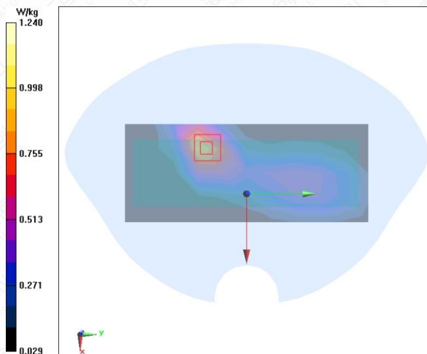
Figure A.1-17 LTE B26 15MHz 1RB 38offset Right Side Mode High 5mm
