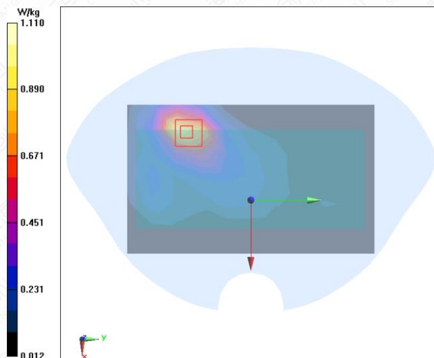
Figure A.1-13 LTE B4 20MHz 1RB 50offset Front Side Mode High 5mm
