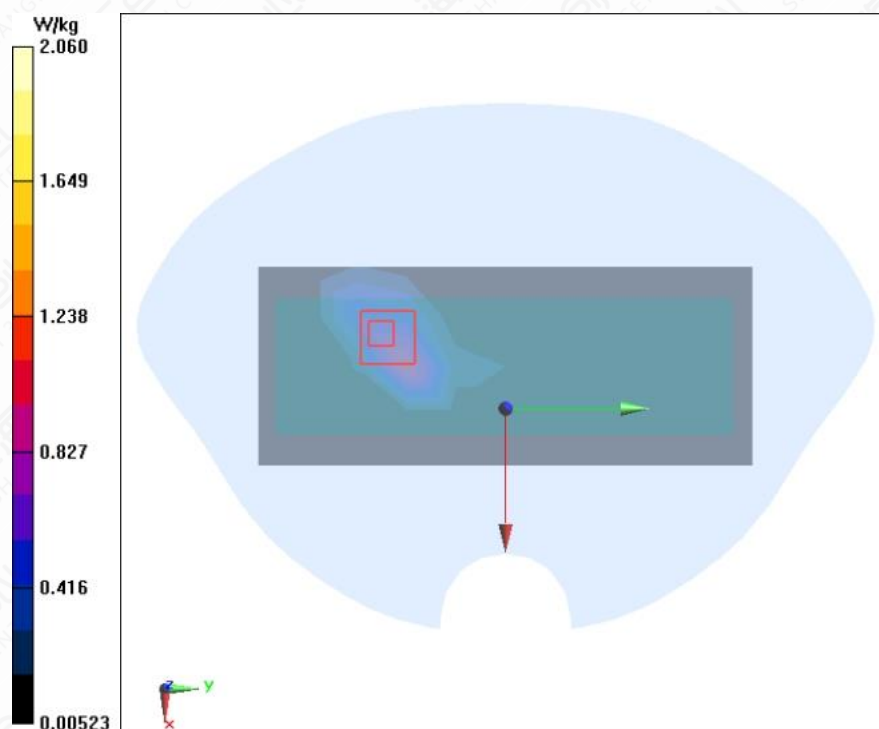
Figure A.1-22 LTE B40 10MHz 1RB 25offset Right Side Mode Middle 0mm
