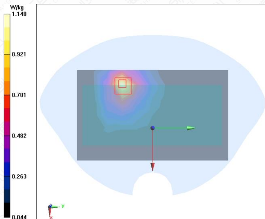
Figure A.1-10 WCDMA Band V RMC Front Side Mode Middle 0mm
