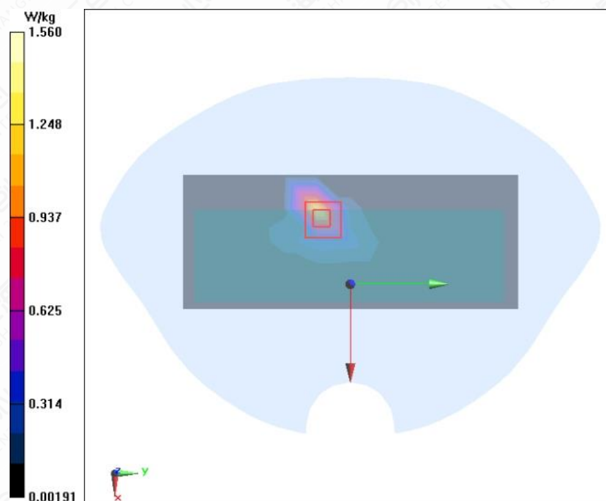
Figure A.1-26 Wi-Fi 2.4G 802.11b Right Side Mode Middle 0mm
