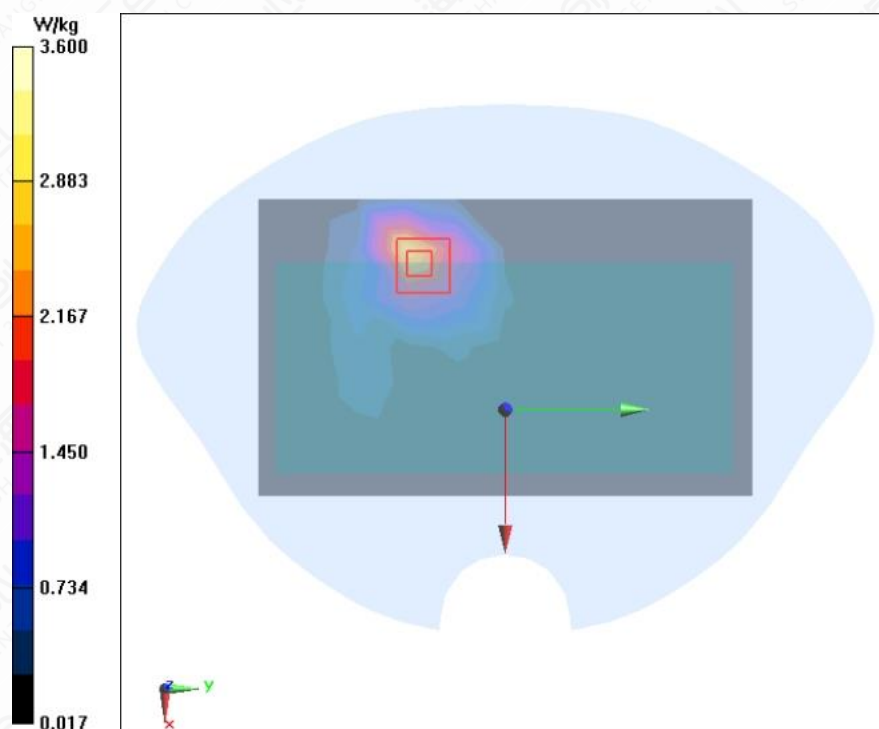
Figure A.1-4 GSM1900 GPRS 4TS Front Side Mode Middle 0mm
