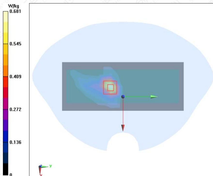
Figure A.1-33 Wi-Fi 5G U-NII-3 802.11a Right Side Mode Middle 5mm
