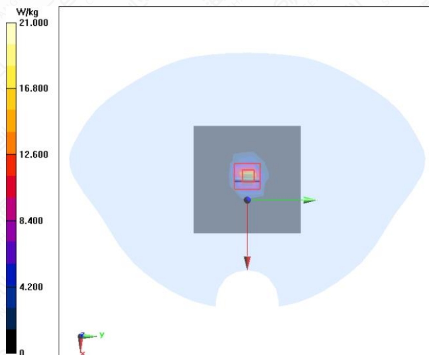
Figure A.2-14 System Check 5800MHz
