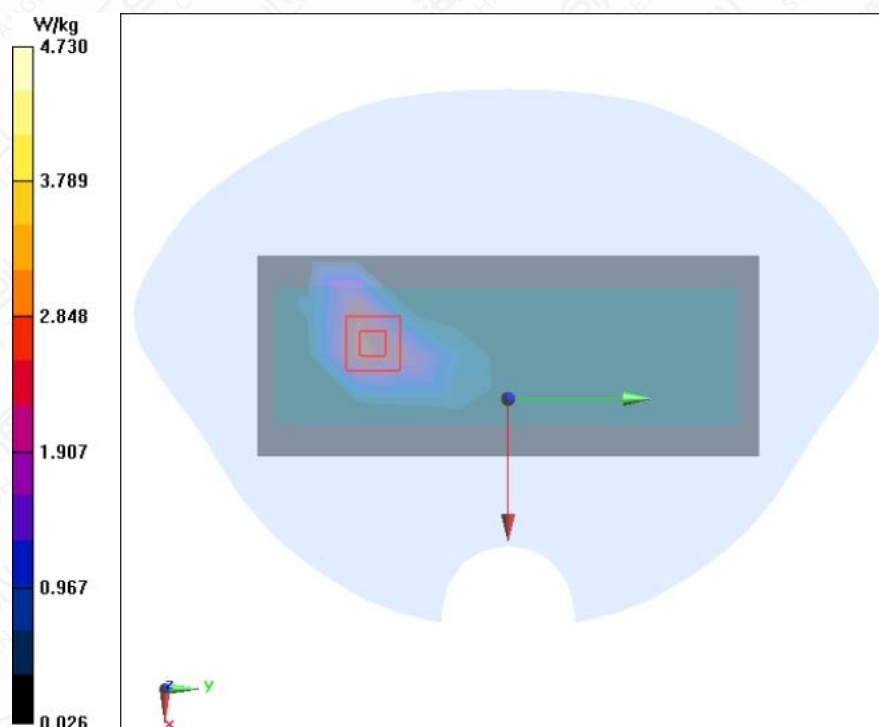
Figure A.1-8 WCDMA BandIV RMC Right Side Mode Middle 0mm
