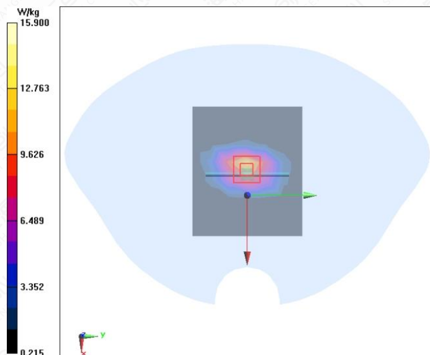
Figure A.2-6 System Check 1900MHz
