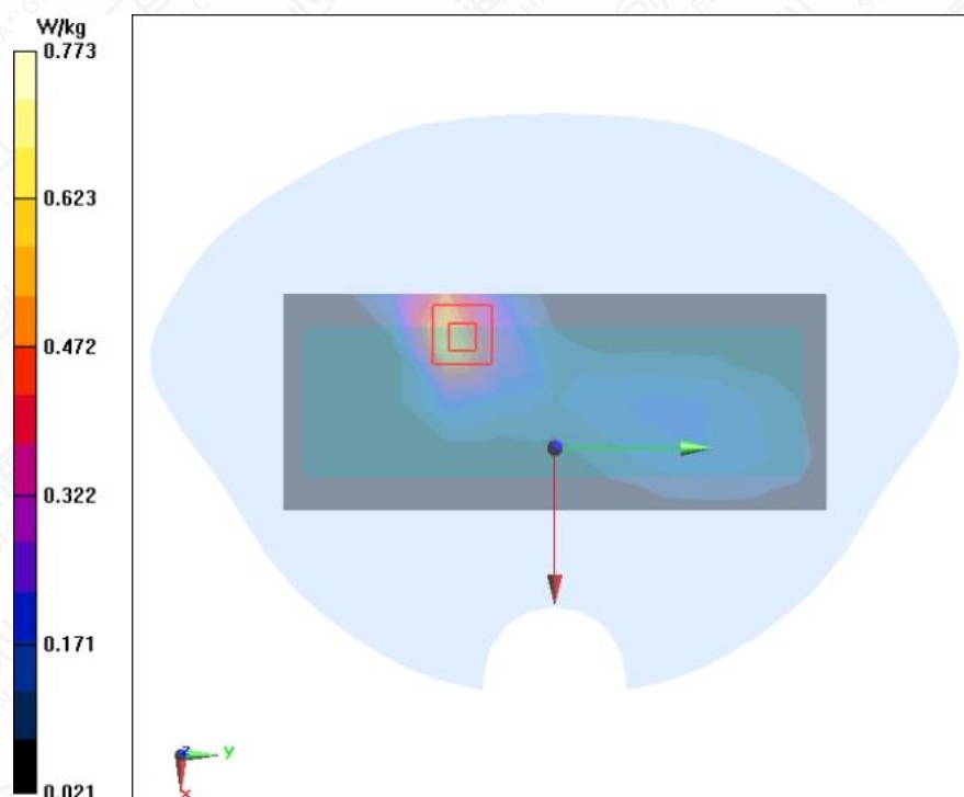
Figure A.1-9 WCDMA Band V RMC Right Side Mode Middle 5mm
