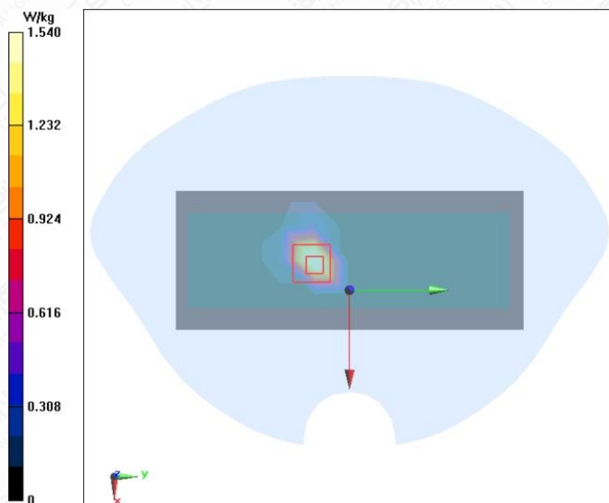
Figure A.1-28 Wi-Fi 5G U-NII-1 802.11a Right Side Mode Middle 0mm
