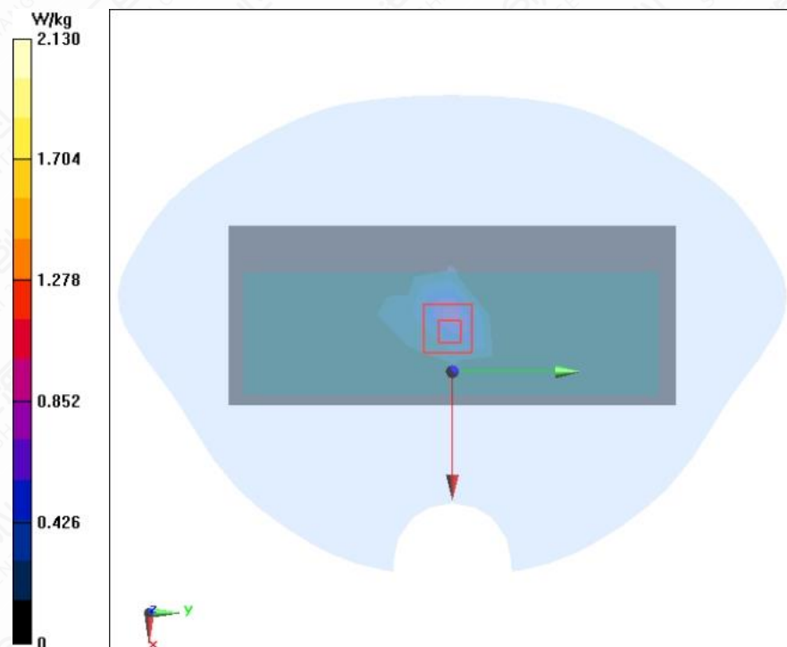
Figure A.1-34 Wi-Fi 5G U-NII-3 802.11a Right Side Mode Middle 0mm
