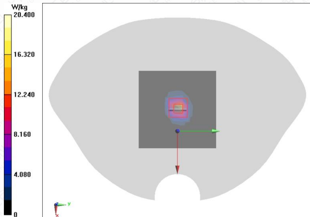
Figure A.2-11 System Check 5800MHz
