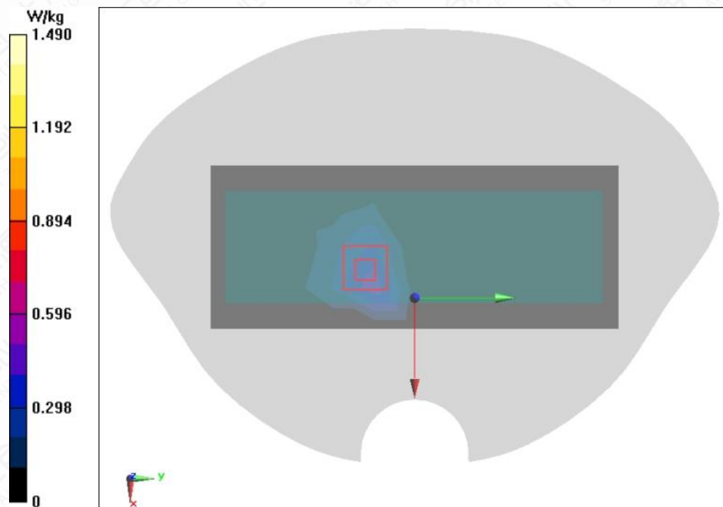
Figure A.1-25 Wi-Fi 5G U-NII-1 802.11a Right Side Mode Middle 0mm
