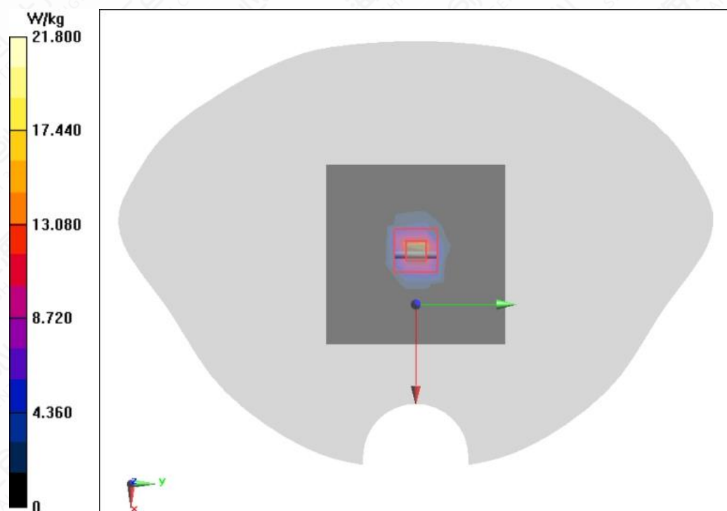
Figure A.2-10 System Check 5600MHz
