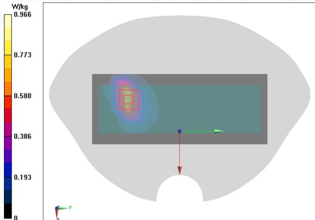
Figure A.1-19 LTE B41 20MHz 1RB 50offset Right Side Mode Middle 5mm
