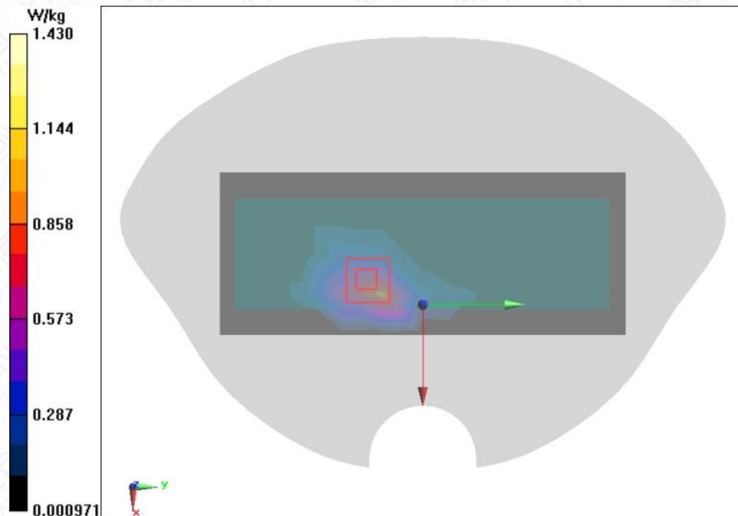
Figure A.1-23 Wi-Fi 2.4G 802.11b Right Side Mode Middle 0mm
