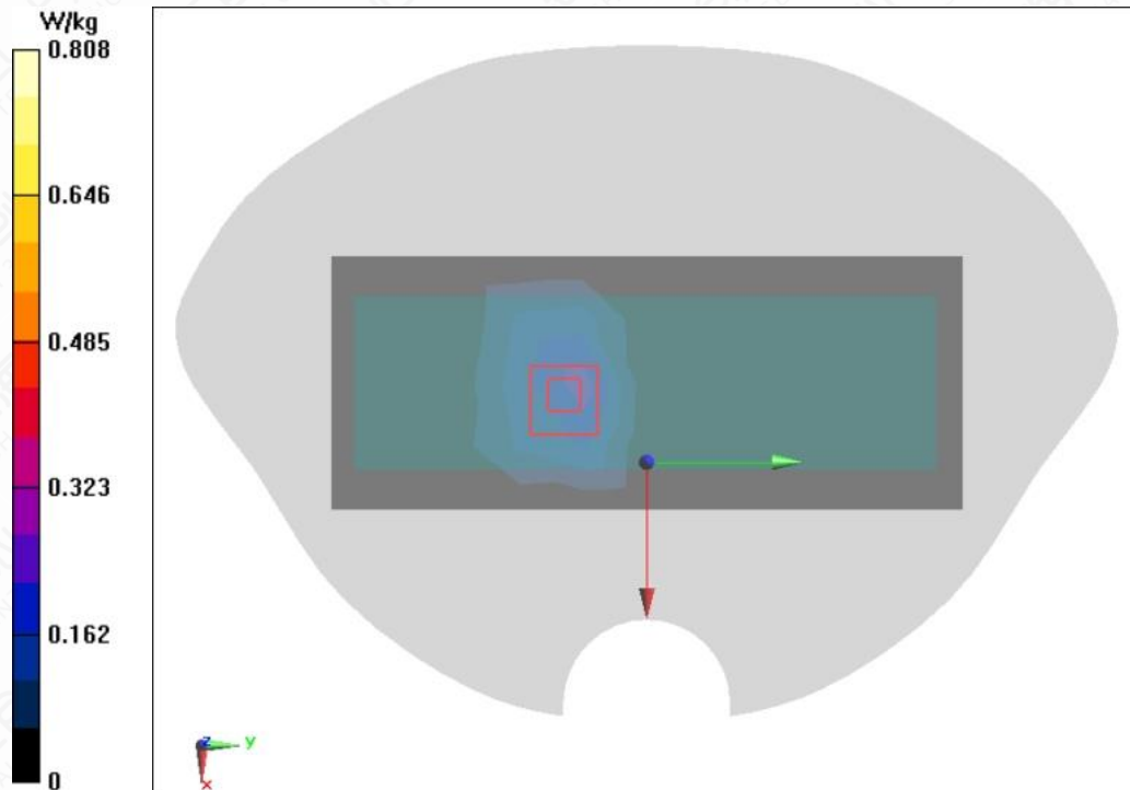
Figure A.1-24 Wi-Fi 5G U-NII-1 802.11a Right Side Mode Middle 5mm
