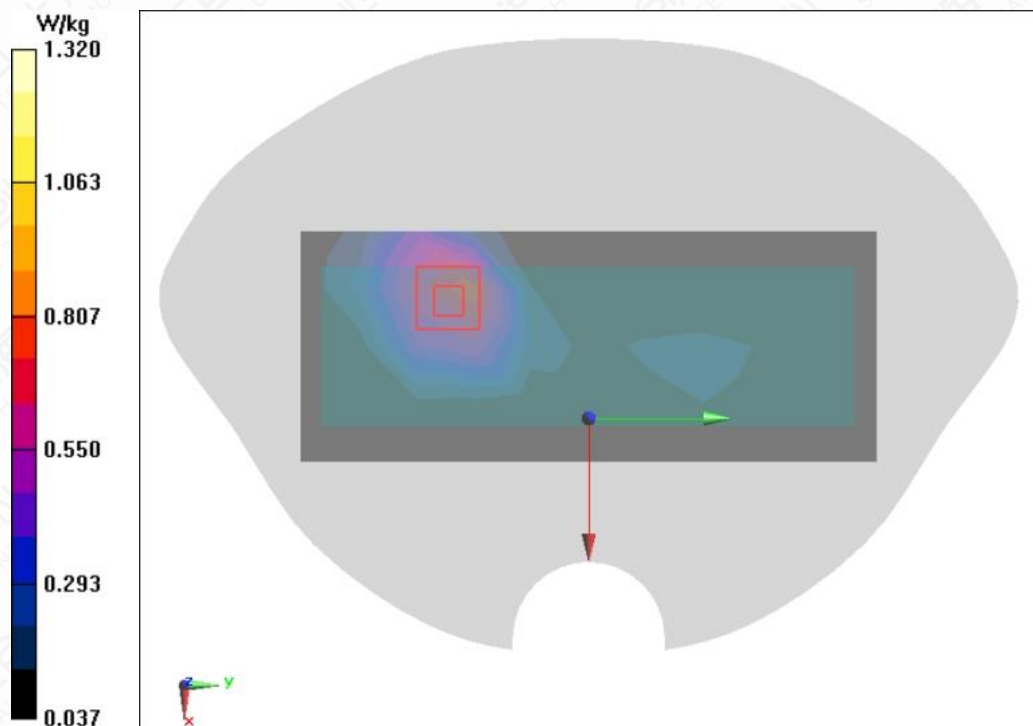
Figure A.1-15 LTE B5 10MHz 25RB 0offset Right Side Mode High 5mm
