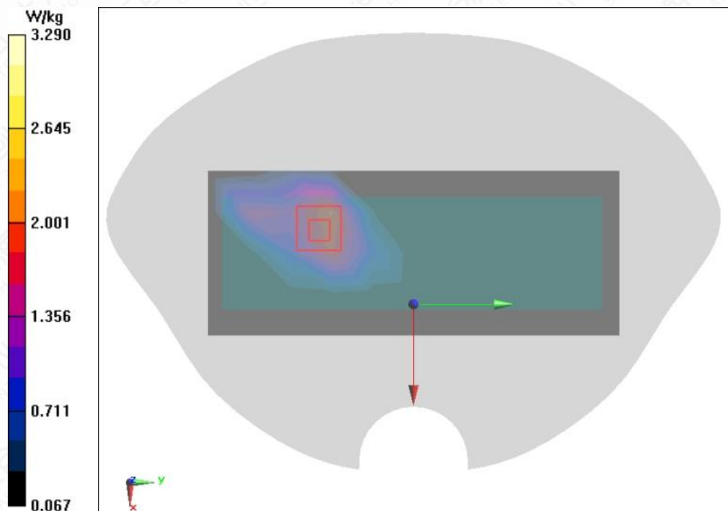
Figure A.1-16 LTE B5 10MHz 1RB 25offset Right Side Mode Middle 0mm
