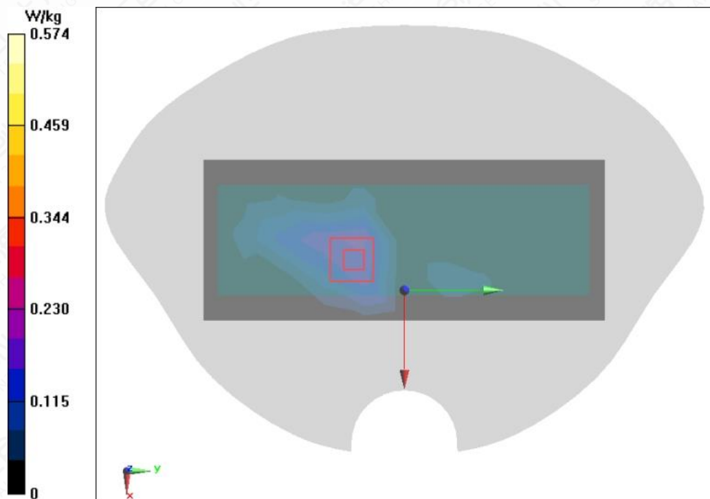
Figure A.1-28 Wi-Fi 5G U-NII-2C 802.11a Right Side Mode High 5mm
