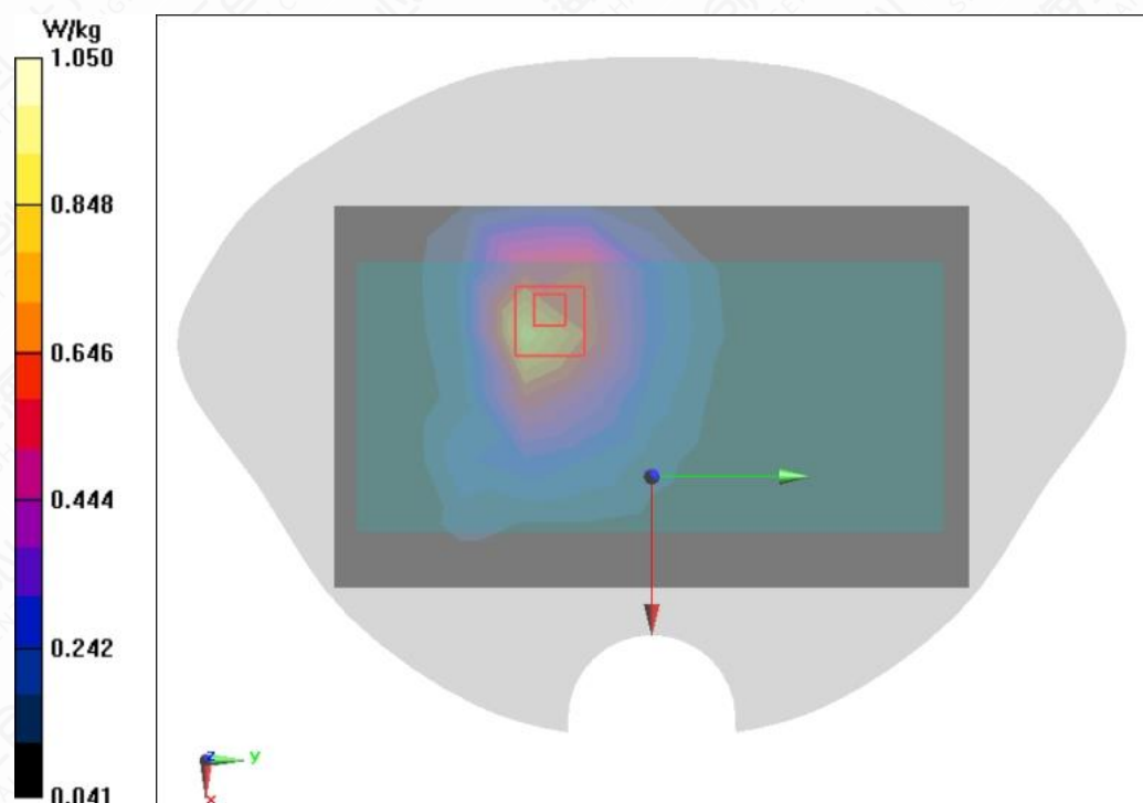
Figure A.1-10 WCDMA Band V Front Side Mode Middle 0mm
