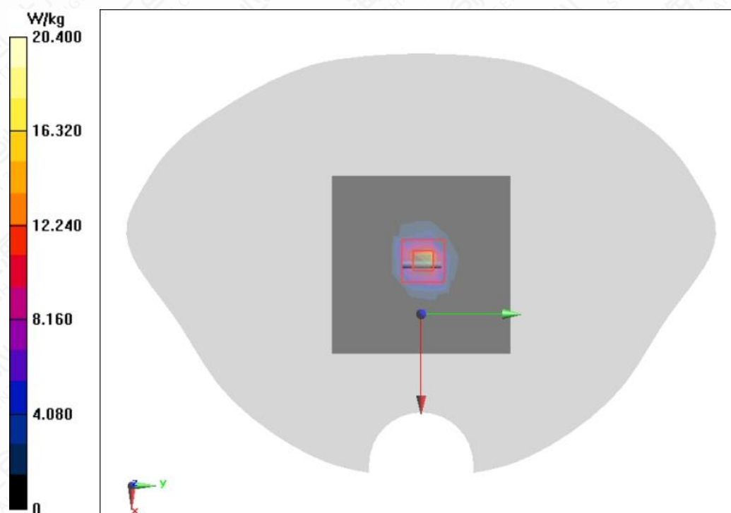
Figure A.2-9 System Check 5300MHz
