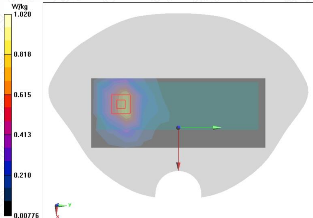
Figure A.1-20 LTE B41 20MHz 1RB 50offset Right Side Mode Middle 16mm
