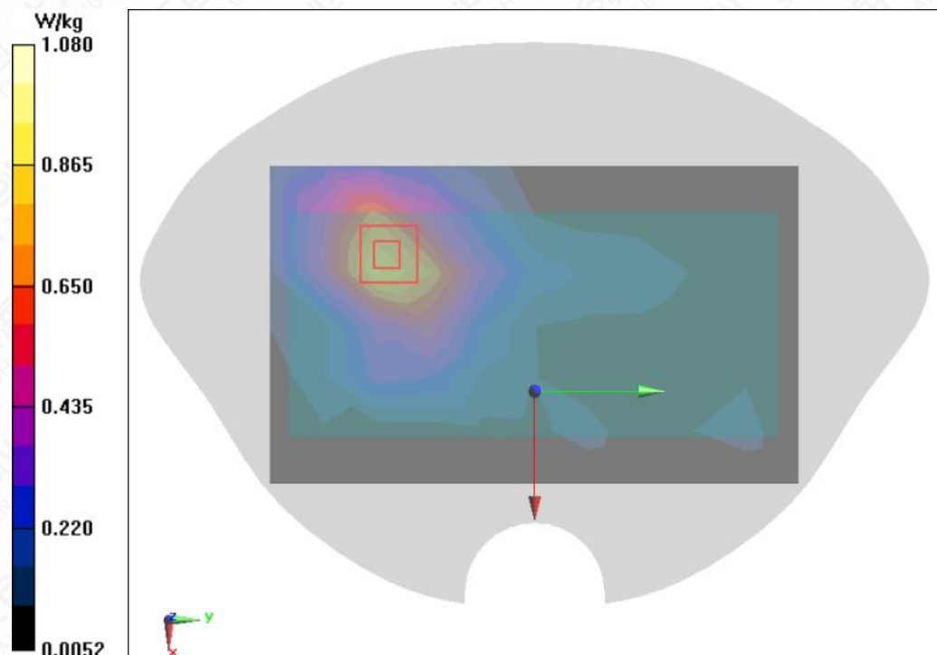
Figure A.1-17 LTE B7 20MHz 1RB 50offset Front Side Mode Low 5mm
