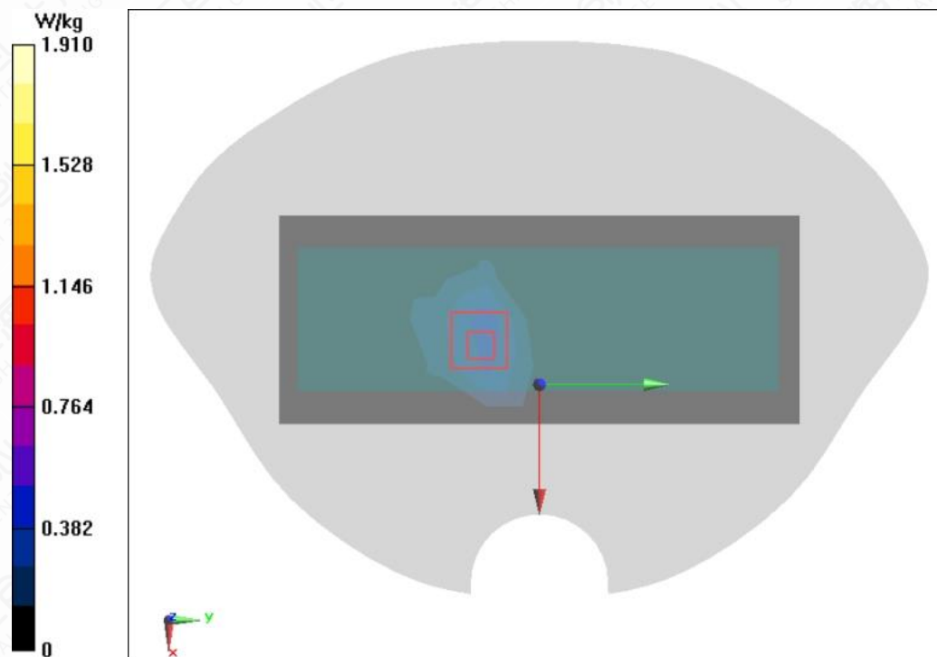
Figure A.1-27 Wi-Fi 5G U-NII-2A 802.11a Right Side Mode High 0mm
