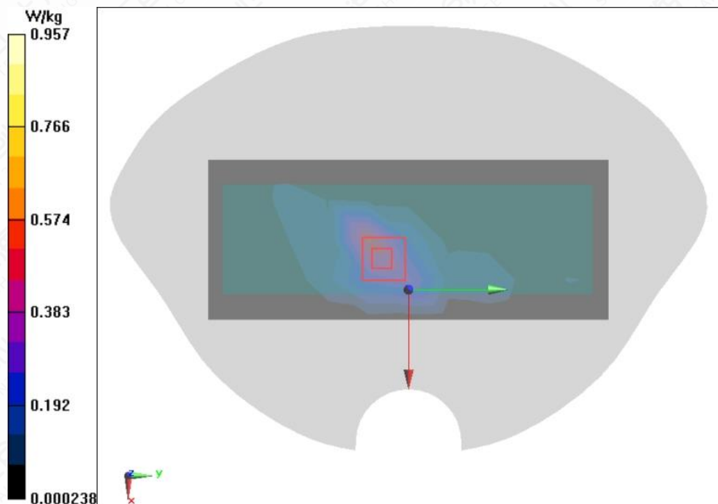
Figure A.1-22 Wi-Fi 2.4G 802.11b Right Side Mode Middle 5mm
