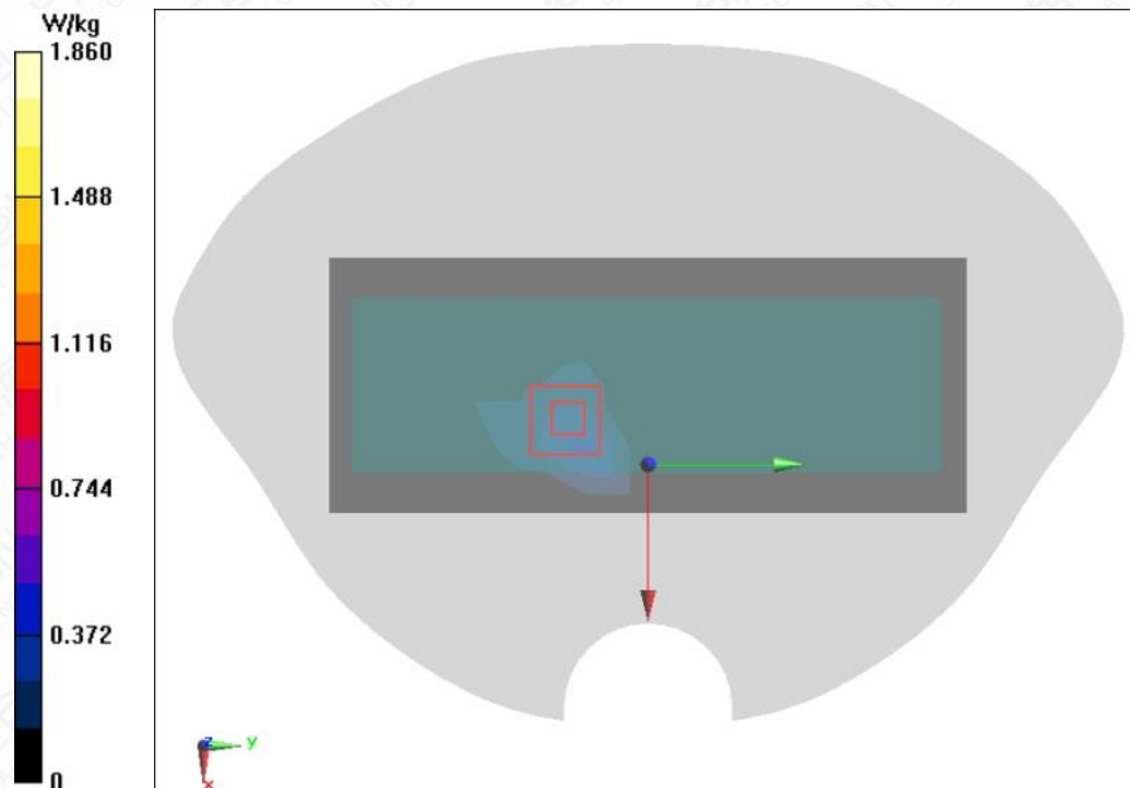
Figure A.1-31 Wi-Fi 5G U-NII-3 802.11a Right Side Mode Low 0mm
