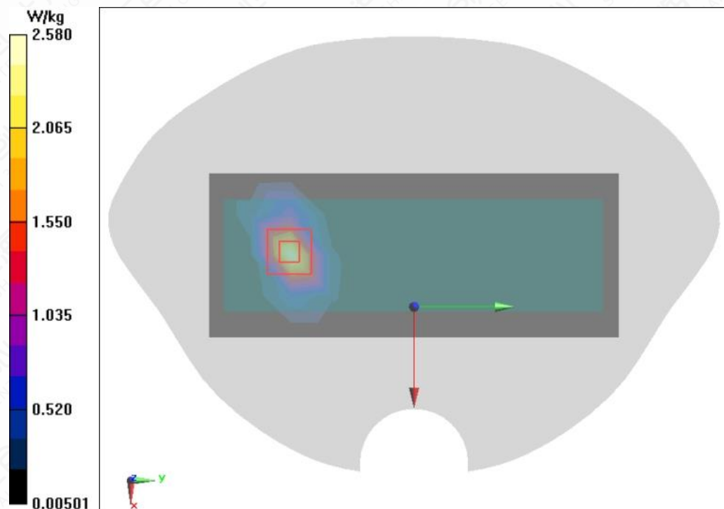
Figure A.1-18 LTE B7 20MHz 1RB 50offset Right Side Mode Middle 0mm
