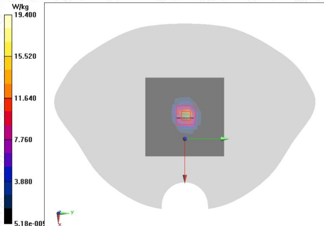
Figure A.2-8 System Check 5200MHz
