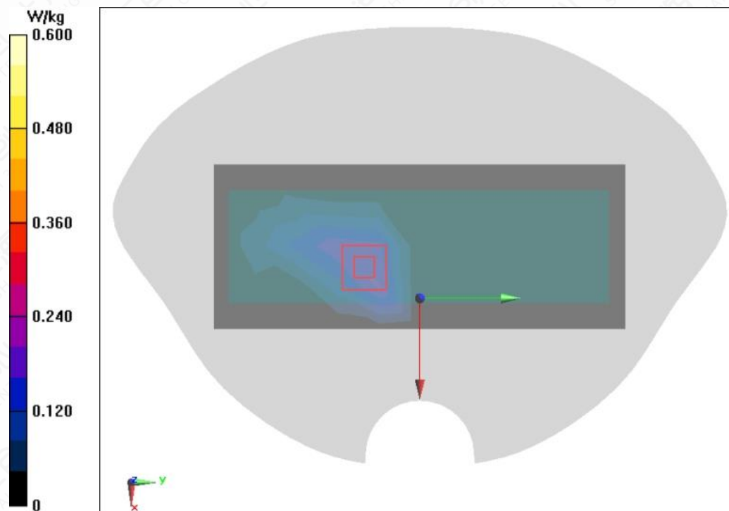
Figure A.1-30 Wi-Fi 5G U-NII-3 802.11a Right Side Mode Low 5mm
