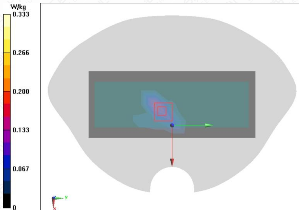
Figure A.1-33 BT DH5 Right Side Mode High 0mm
