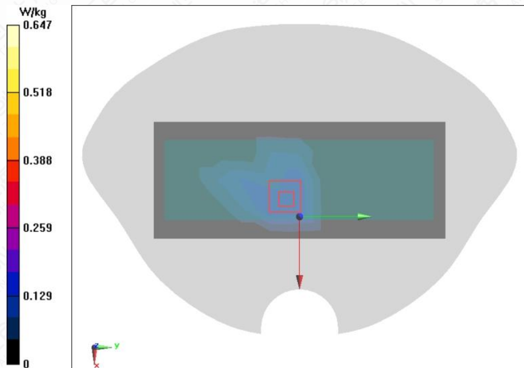
Figure A.1-26 Wi-Fi 5G U-NII-2A 802.11a Right Side Mode High 5mm
