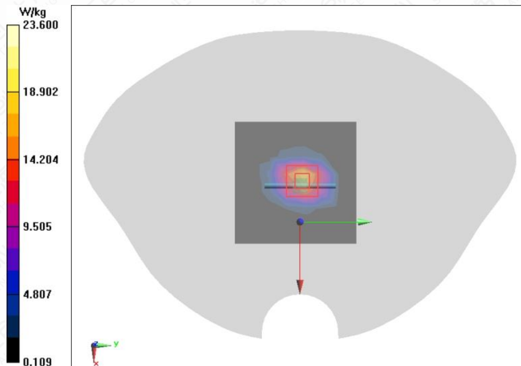
Figure A.2-7 System Check 2600MHz
