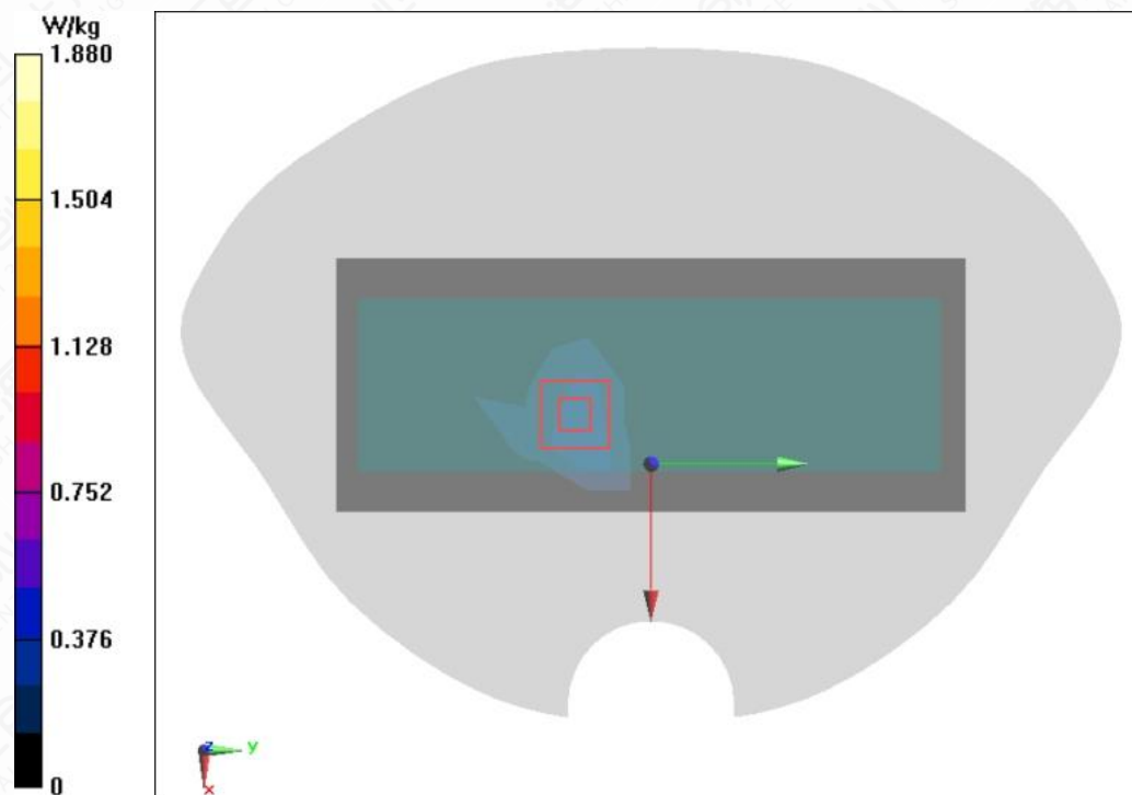
Figure A.1-29 Wi-Fi 5G U-NII-2C 802.11a Right Side Mode High 0mm
