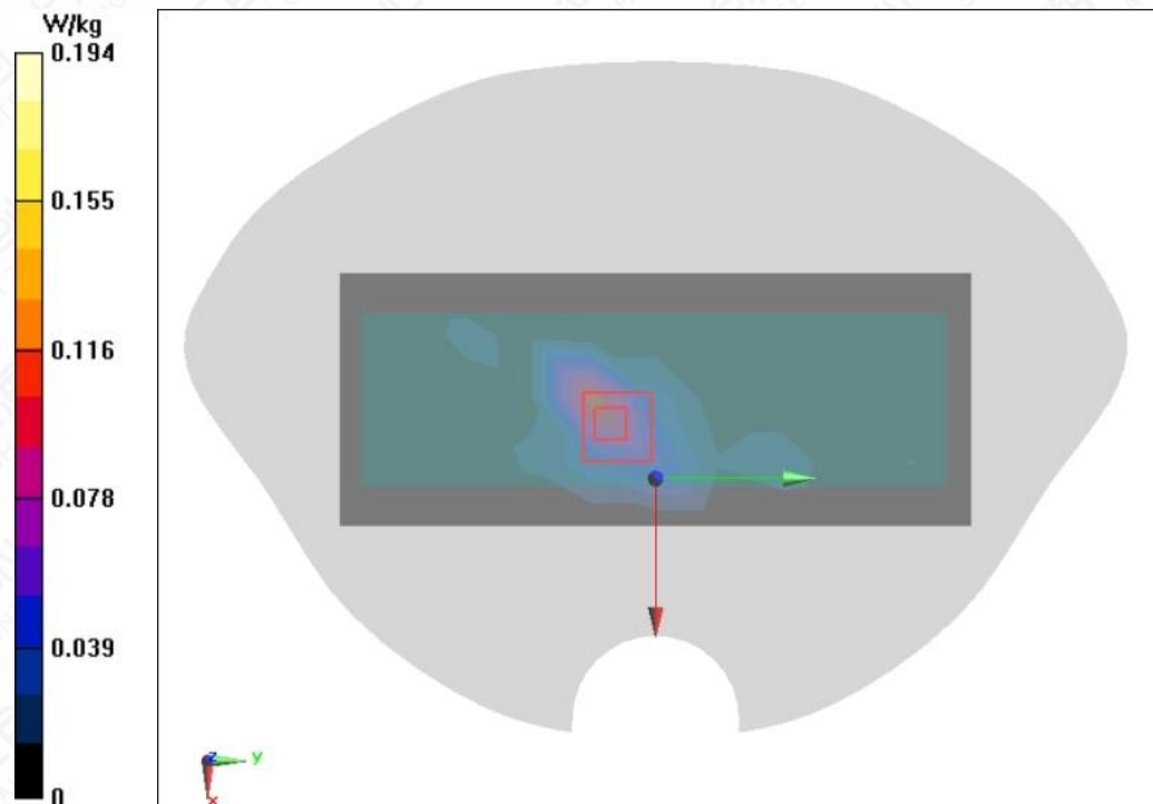
Figure A.1-32 BT DH5 Right Side Mode High 5mm
