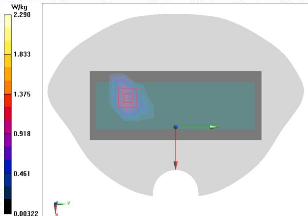
Figure A.1-21 LTE B41 20MHz 1RB 50offset Right Side Mode Middle 0mm
