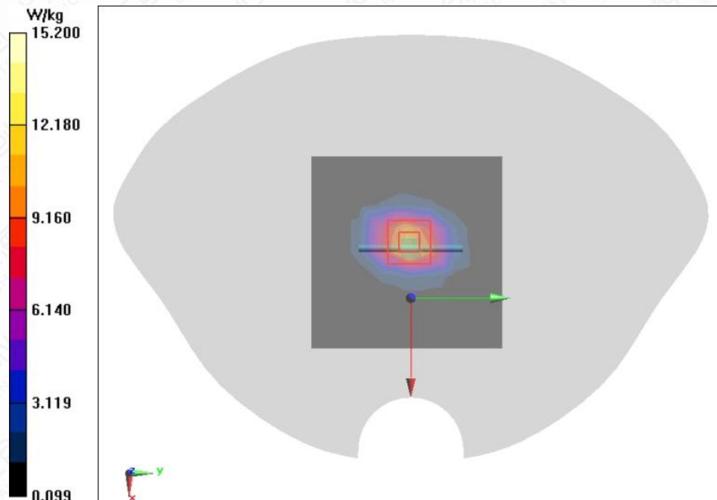
Figure A.2-6 System Check 2450MHz
