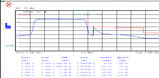
TDD41_Channel High_10MHz_QPSK_FullRB
