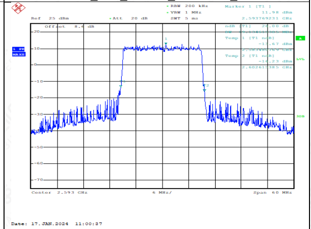
TDD41_Mid_20MHz_2593MHz_Q16
