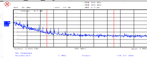
TDD41_Channel High_10_2656000000Hz _1RB_HighOut of Limit Channel Power
