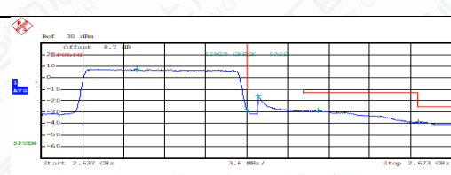
TDD41_Channel High_15MHz_QPSK_FullRB
