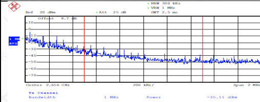
TDD41_Channel High_15_2656000000Hz _1RB_HighOut of Limit Channel Power
