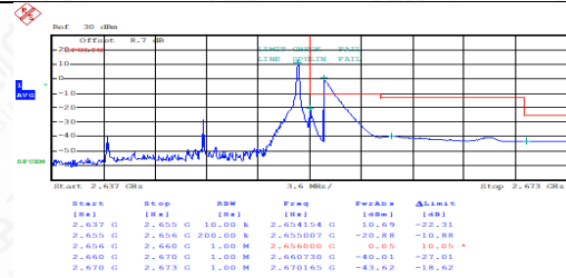
TDD41_Channel High_15MHz_QPSK_1RB_HighRange
