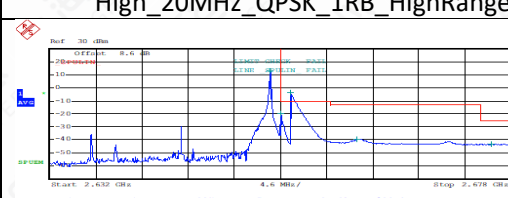
TDD41_Channel High_20MHz_QPSK_1RB_HighRange
