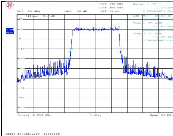
TDD41_Mid_15MHz_2593MHz_QPSK
