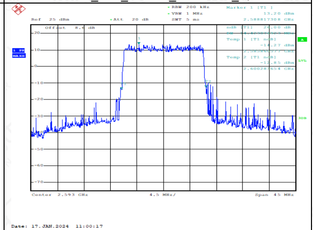
TDD41_Mid_20MHz_2593MHz_Q16
