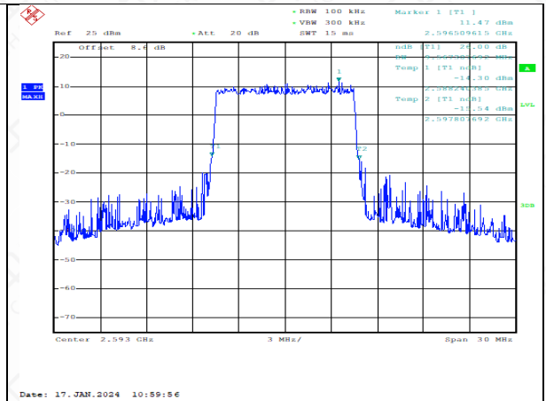
TDD41_Mid_15MHz_2593MHz_Q16
