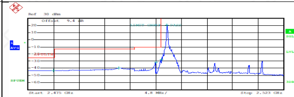
FDD07LowRange_20MHz_QPSK_1RB_LowRange
