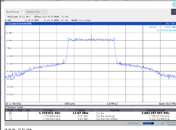
FDD66_MidRange_5_1745_QPSK
