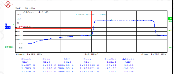
FDD04LowRange_20MHz_QPSK_FullRB_LowRange
