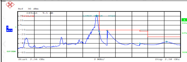
FDD07HighRange_5MHz_QPSK_1RB_HighRange
