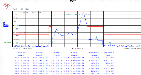
FDD13HighRange_10MHz_QPSK_1RB_HighRange
