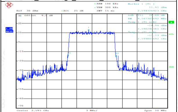
TDD38_MidRange_10MHz_2595MHz_16QAM
