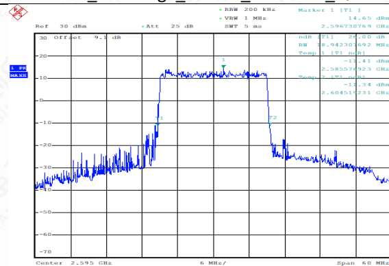
TDD38_MidRange_20MHz_2595MHz_QPSK
