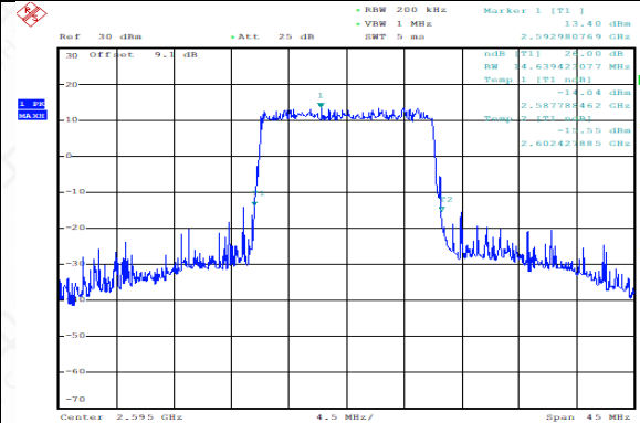
TDD38_MidRange_15MHz_2595MHz_16QAM
