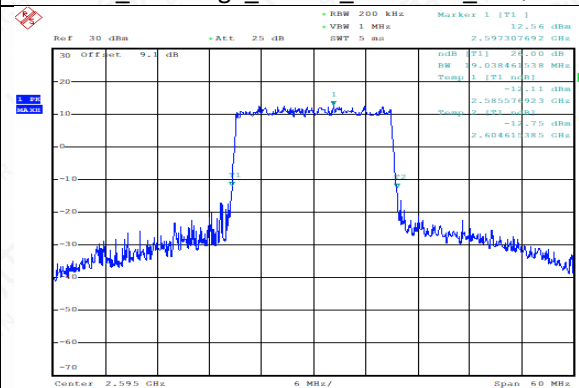
TDD38_MidRange_20MHz_2595MHz_16QAM
