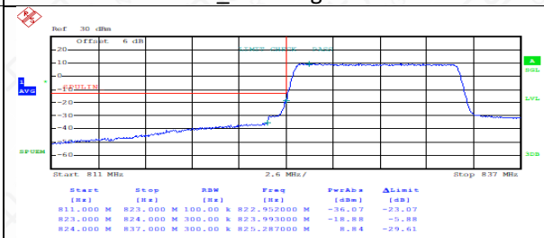
FDD05LowRange_10MHz_QPSK_FullRB_LowRange
