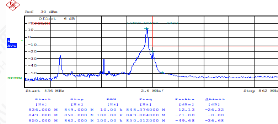
FDD05HighRange_10MHz_QPSK_1RB_HighRange
