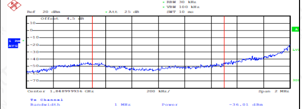
FDD02_LowRange_1.4_1848999936Hz_1RB_LowRangeOut of Limit Channel Power
