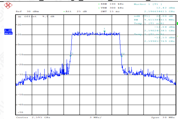
TDD38_MidRange_10MHz_2595MHz_QPSK
