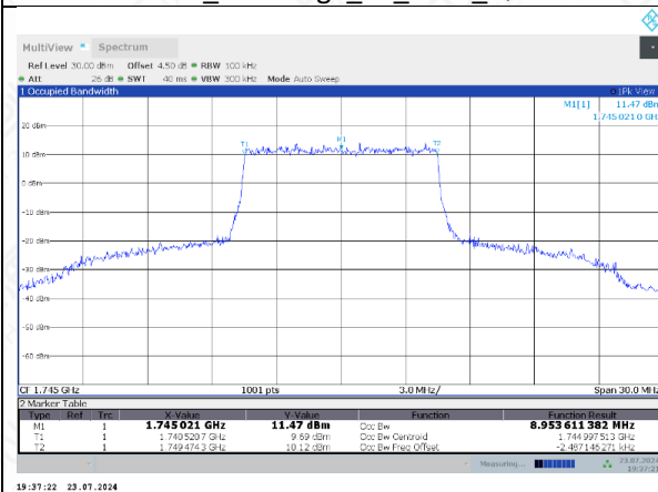
FDD66_MidRange_10_1745_QPSK
