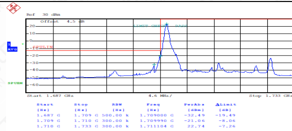
FDD04LowRange_20MHz_QPSK_1RB_LowRange
