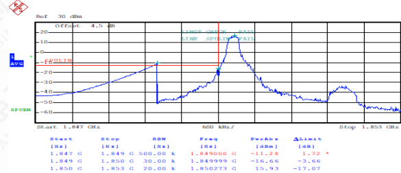
FDD02LowRange_1.4MHz_QPSK_1RB_LowRange
