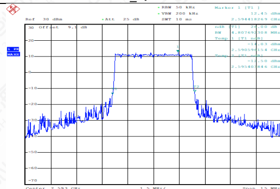
TDD41_MidRange_5MHz_2593MHz_QPSK
