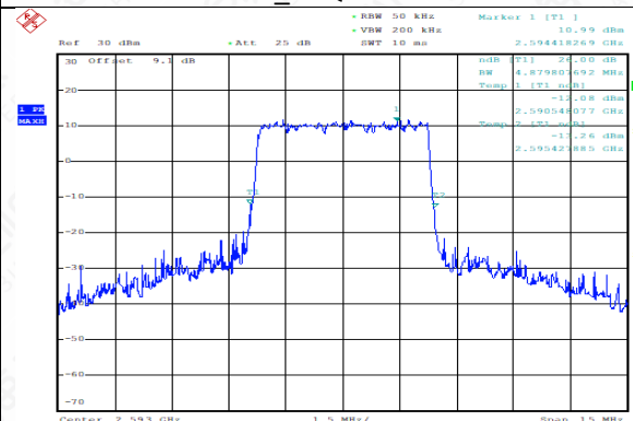
TDD41_MidRange_5MHz_2593MHz_16QAM
