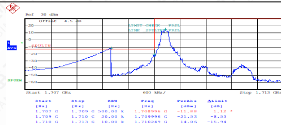
FDD04LowRange_1.4MHz_QPSK_1RB_LowRange
