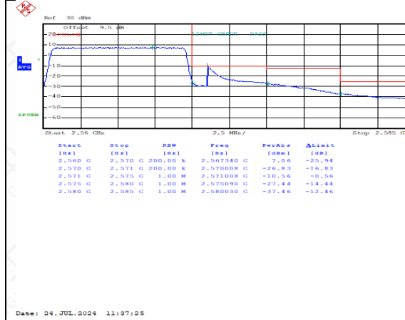
FDD07HighRange_15MHz_QPSK_FullRB_HighRange
