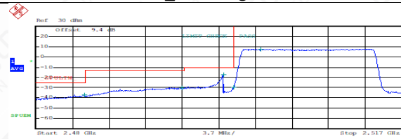
FDD07LowRange_15MHz_QPSK_FullRB _LowRange
