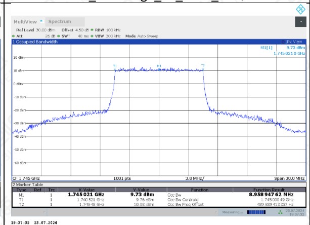
FDD66_MidRange_10_1745_16QAM
