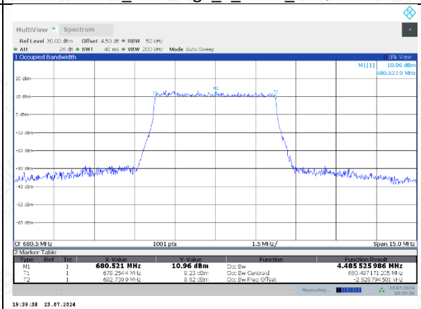
FDD71_MidRange_5_680.5_16QAM
