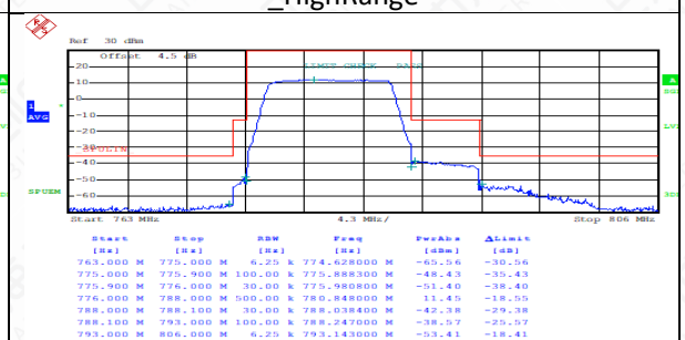
FDD13HighRange_10MHz_QPSK_FullRB_HighRange
