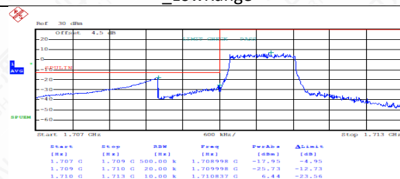
FDD04LowRange_1.4MHz_QPSK_FullRB_LowRange
