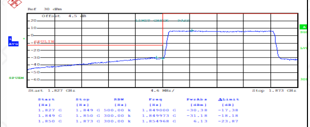
FDD02LowRange_20MHz_QPSK_FullRB_LowRange
