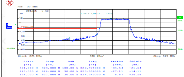
FDD05LowRange_1.4MHz_QPSK_FullRB_LowRange
