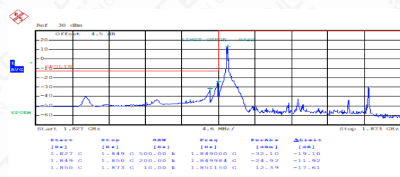
FDD02LowRange_20MHz_QPSK_1RB_LowRange
