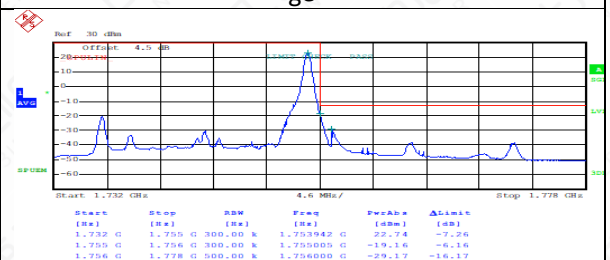
FDD04HighRange_20MHz_QPSK_1RB_HighRange
