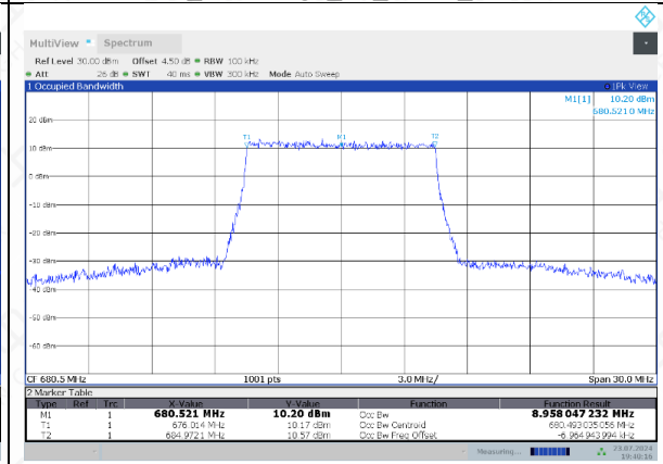
FDD71_MidRange_15_680.5_16QAM
