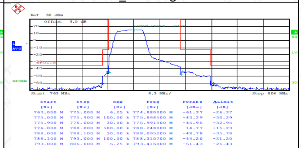
FDD13LowRange_5MHz_QPSK_FullRB_LowRange
