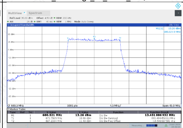
FDD71_MidRange_20_683_16QAM
