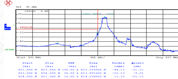
FDD05LowRange_1.4MHz_QPSK_1RB_LowRange
