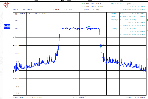
TDD38_MidRange_5MHz_2595MHz_QPSK
