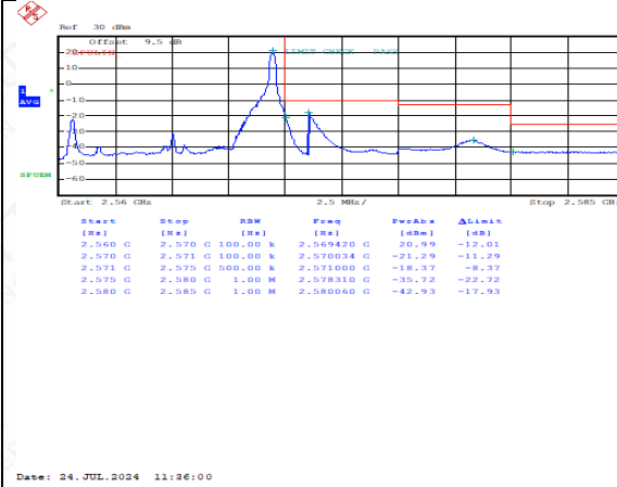
FDD07HighRange_15MHz_QPSK_1RB_HighRange
