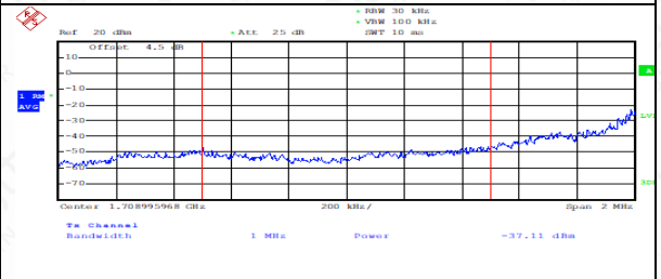
FDD04_LowRange_1.4_1708995968Hz_1RB_LowRangeOut of Limit Channel Power
