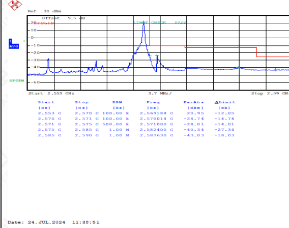
FDD07HighRange_20MHz_QPSK_1RB_HighRange
