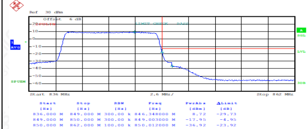
FDD05HighRange_10MHz_QPSK_FullRB_HighRange
