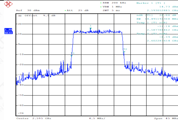
TDD38_MidRange_15MHz_2595MHz_QPSK
