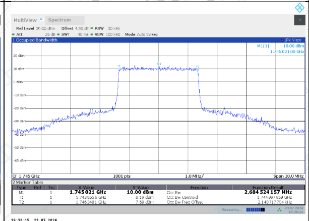
FDD66_MidRange_5_1745_16QAM
