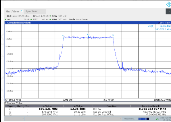
FDD71_MidRange_15_680.5_QPSK
