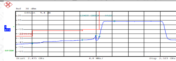
FDD07LowRange_20MHz_QPSK_FullRB _LowRange
