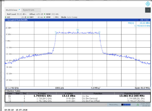
FDD66_MidRange_20_1745_16QAM
