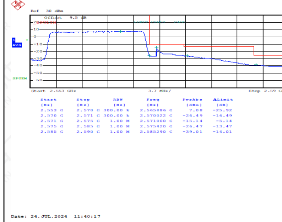
FDD07HighRange_20MHz_QPSK_FullRB_HighRange
