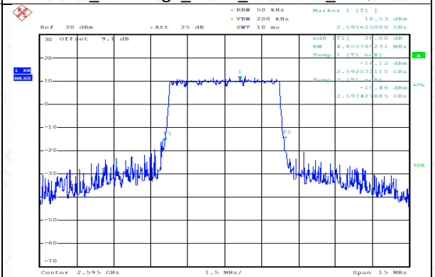
TDD38_MidRange_5MHz_2595MHz_16QAM
