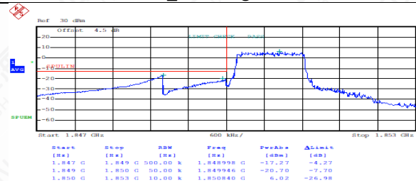
FDD02LowRange_1.4MHz_QPSK_FullRB_LowRange
