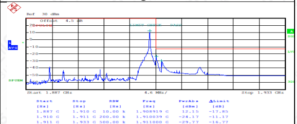
FDD02HighRange_20MHz_QPSK_1RB_HighRange
