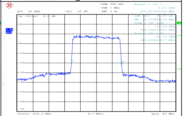
FDD26(PART 22)_MidRange_15MHz_836.5MHz_16QAM
