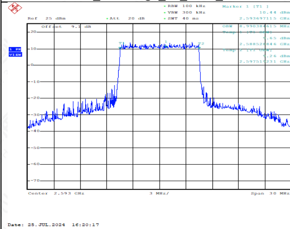
TDD41_MidRange_10_2593_QPSK
