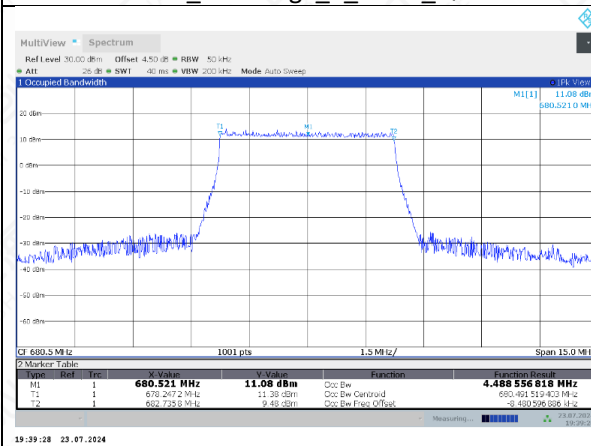
FDD71_MidRange_5_680.5_QPSK
