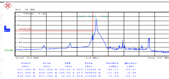
FDD05LowRange_10MHz_QPSK_1RB_LowRange
