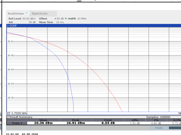
FDD04_MidRange_5MHz_1732.5_fullRB_16QAM
