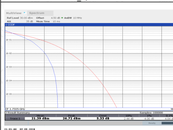
FDD04_MidRange_5MHz_1732.5_fullRB_QPSK
