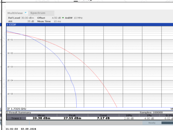
FDD04_MidRange_10MHz_1732.5_fullRB_16QAM
