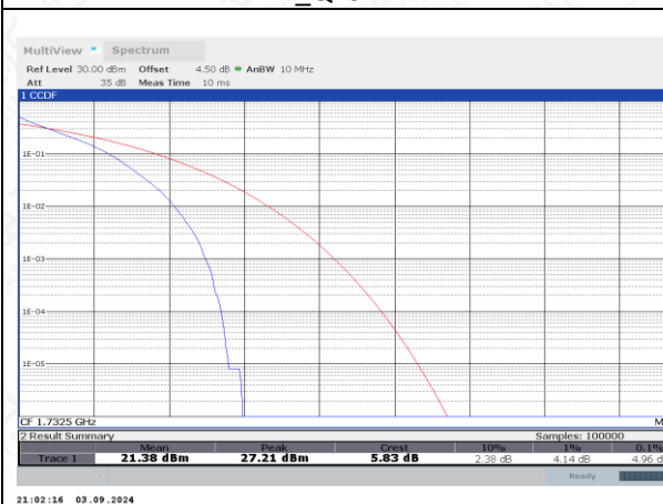
FDD04_MidRange_10MHz_1732.5_fullRB_QPSK
