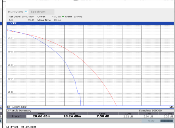
FDD25_MidRange_10MHz_1882.5_fullRB_16QAM
