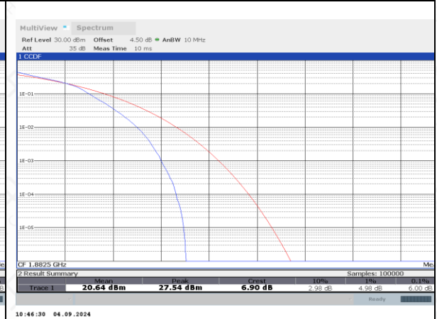
FDD25_MidRange_5MHz_1882.5_fullRB_16QAM
