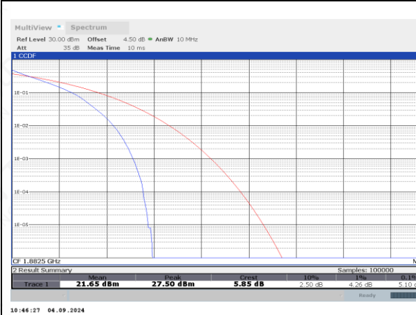
FDD25_MidRange_5MHz_1882.5_fullRB_QPSK
