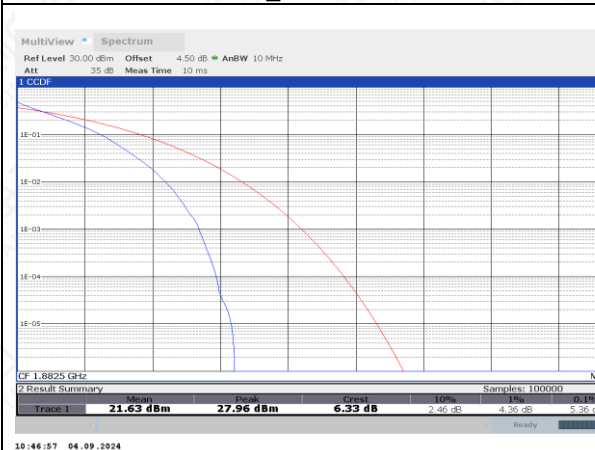
FDD25_MidRange_10MHz_1882.5_fullRB_QPSK
