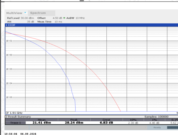
FDD25_HighRange_10MHz_1910_fullRB_QPSK
