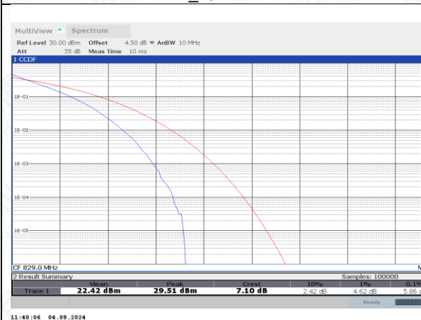
FDD26_22_LowRange_10MHz_829_fullIRB_QPSK
