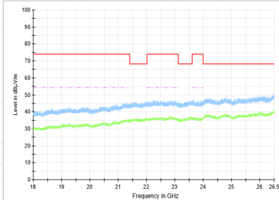
RSE-11AC(20M)-CH157-18GHz-26.5GHz
