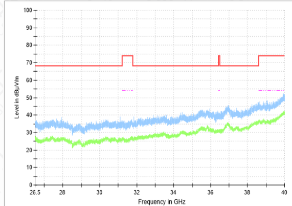
RSE-11AC(20M)-CH157-26.5GHz-40GHz
