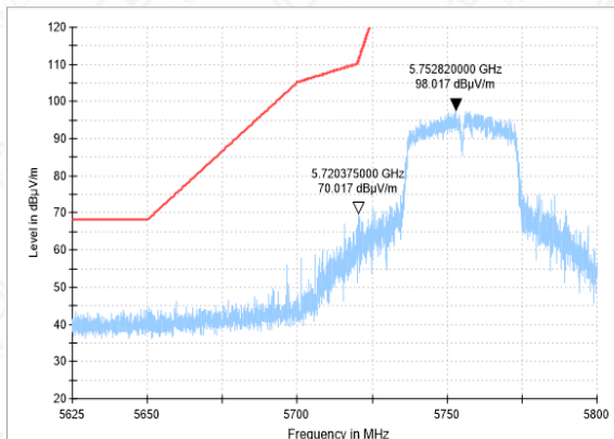
Bandedge-11N(40M)-CH151-PK
