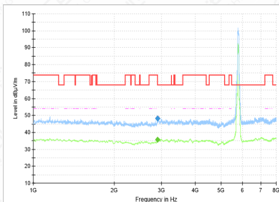
RSE-11AC(80M)-CH155-1GHz-8GHz
