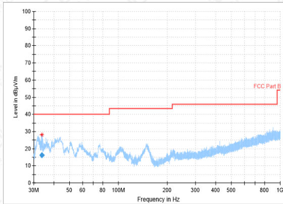
RSE-11AC(40M)-CH159-30MHz-1GHz
