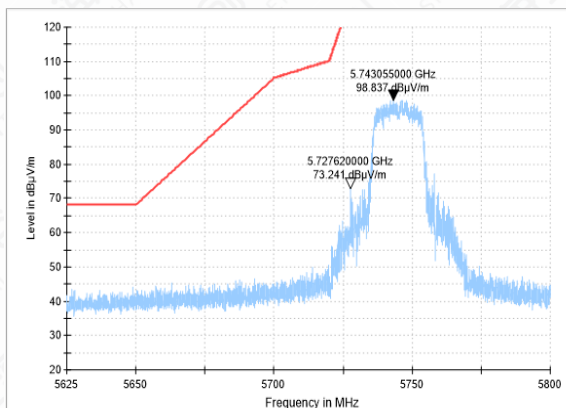
Bandedge-11AC(20M)-CH149-PK
