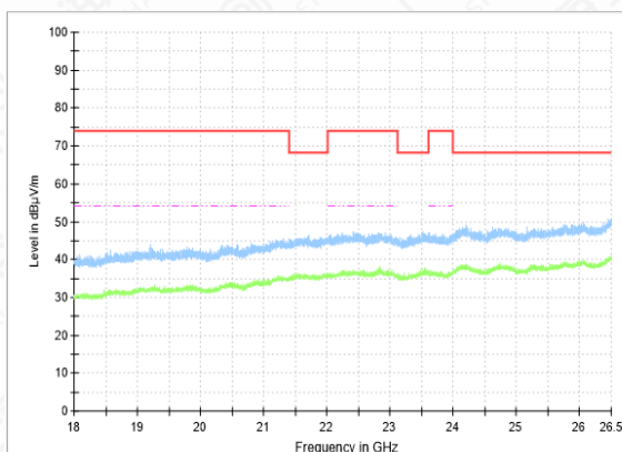
RSE-11AC(80M)-CH155-18GHz-26.5GHz
