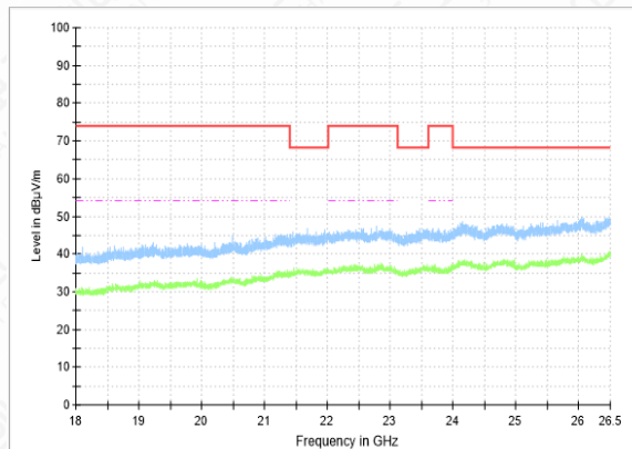
RSE-11AC(40M)-CH159-18GHz-26.5GHz
