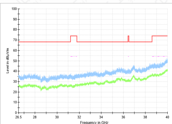
RSE-11AC(80M)-CH155-26.5GHz-40GHz
