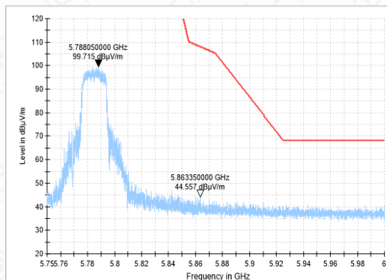
Bandedge-11AC(20M)-CH157-PK
