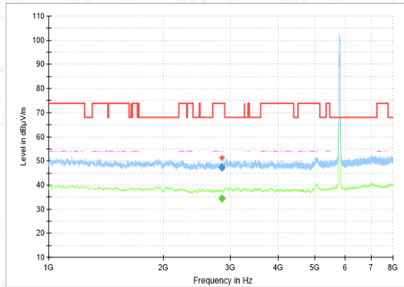
RSE-11AC(40M)-CH159-1GHz-8GHz
