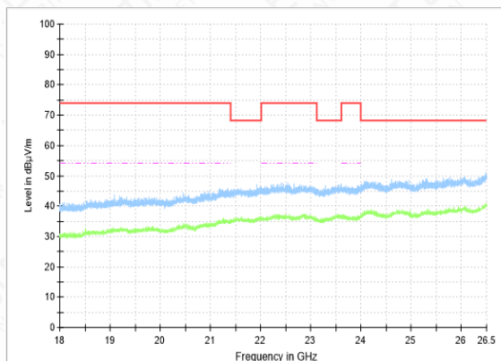
RSE-11N(20M)-CH36-18GHz-26.5GHz
