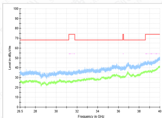
RSE-11A-CH52-26.5GHz-40GHz
