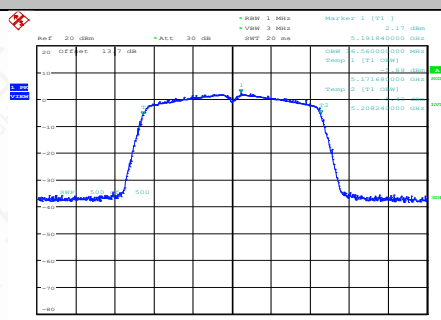
11AC40SISO-Ant1-5190
