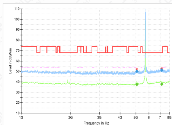
RSE-11A-CH140-1GHz-8GHz
