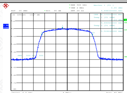
11AC20SISO-Ant1-5500
