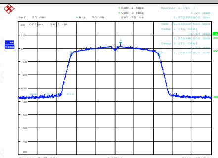
11AC40SISO-Ant1-5270
