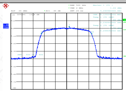
11AC20SISO-Ant1-5240
