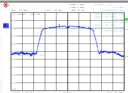
11N40SISO-Ant1-5550
