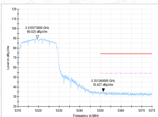
Bandedge-11N(20M)-CH64-AV
