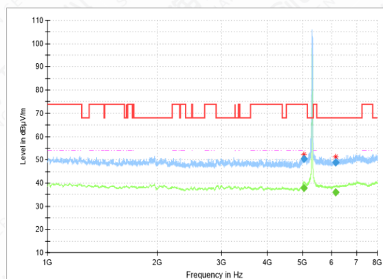
RSE-11N(20M)-CH60-1GHz-8GHz
