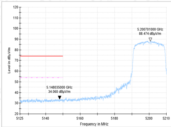
Bandedge-11N(20M)-CH40-AV
