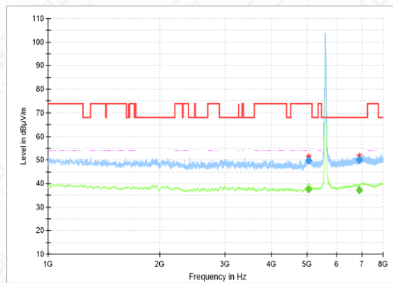
RSE-11N(40M)-CH118-1GHz-8GHz
