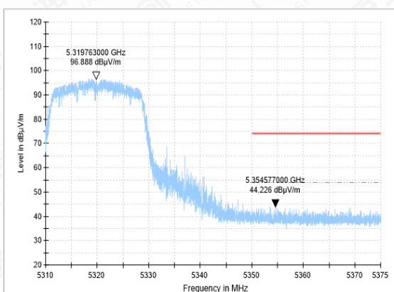
Bandedge-11N(20M)-CH64-PK
