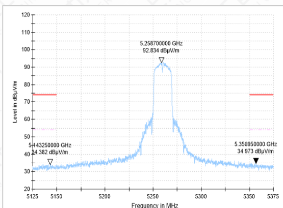
Bandedge-11N(20M)-CH52-AV
