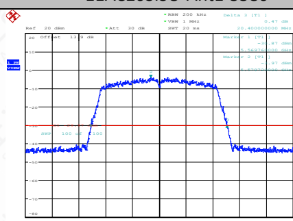
11AC20SISO-Ant1-5580
