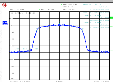
11AC20SISO-Ant1-5320
