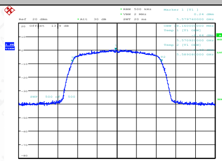
11AC20SISO-Ant1-5580
