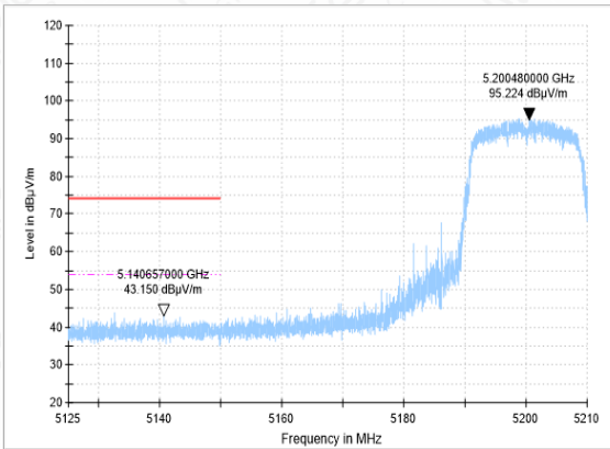
Bandedge-11N(20M)-CH40-PK
