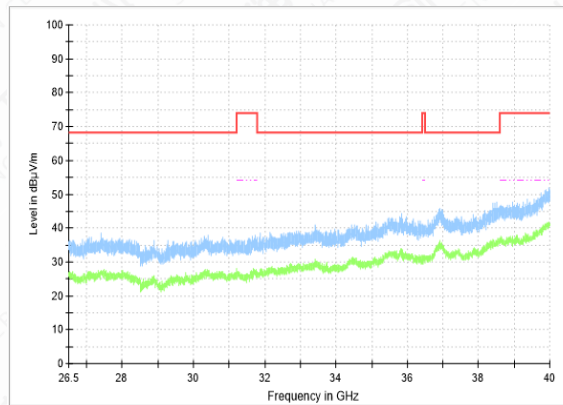
RSE-11N(40M)-CH62-26.5GHz-40GHz
