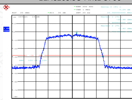
11AC20SISO-Ant1-5700
