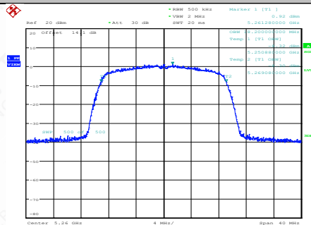
11AC20SISO-Ant1-5260
