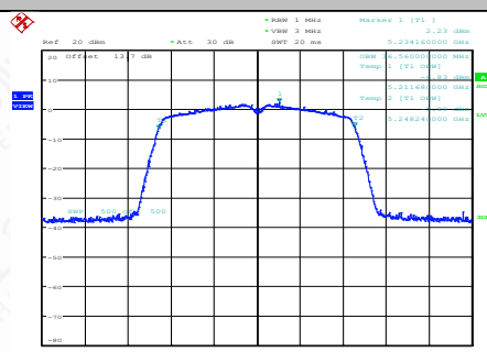
11AC40SISO-Ant1-5230
