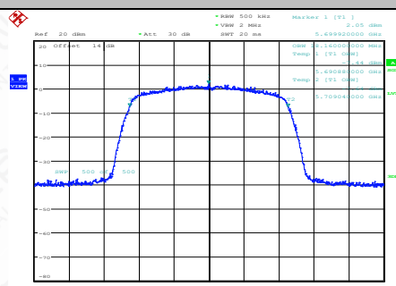
11AC20SISO-Ant1-5700
