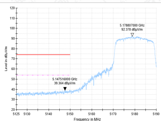
Bandedge-11N(20M)-CH36-AV
