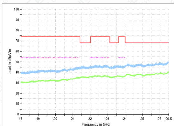
RSE-11A-CH52-18GHz-26.5GHz
