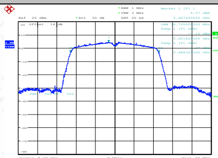
11N40SISO-Ant1-5670
