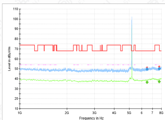
RSE-11N(20M)-CH36-1GHz-8GHz
