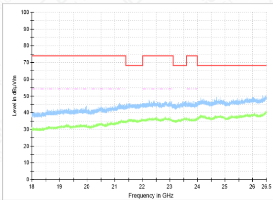
RSE-11N(40M)-CH62-18GHz-26.5GHz
