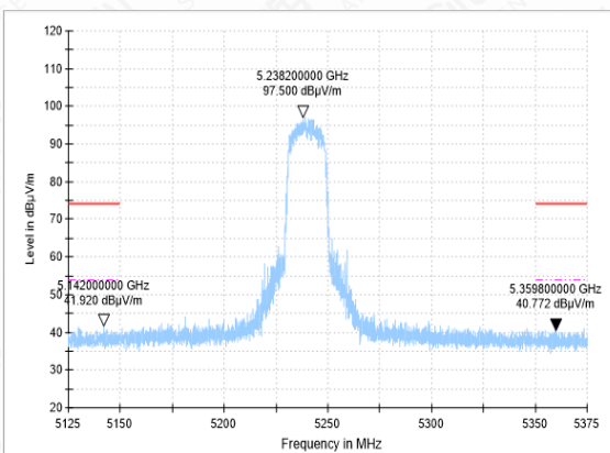
Bandedge-11N(20M)-CH48-PK
