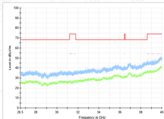
RSE-11N(20M)-CH36-26.5GHz-40GHz
