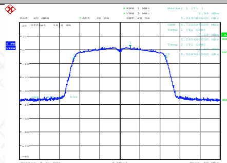
11AC40SISO-Ant1-5310
