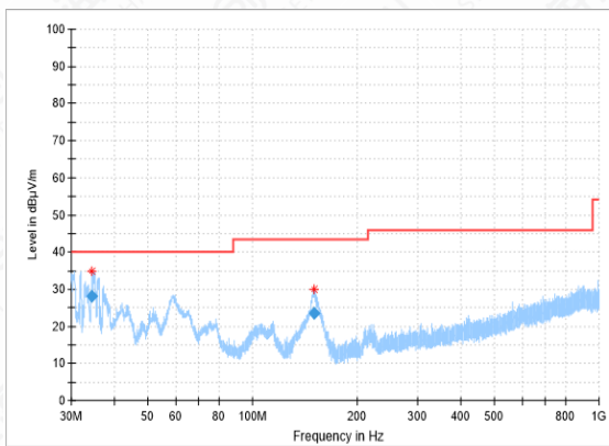
RSE-11N(40M)-CH118-30MHz-1GHz
