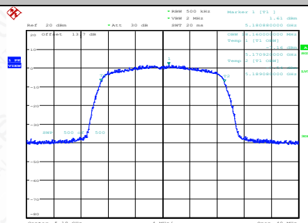
11AC20SISO-Ant1-5180
