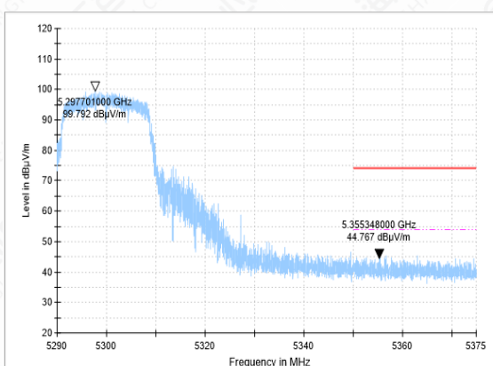
Bandedge-11N(20M)-CH60-PK
