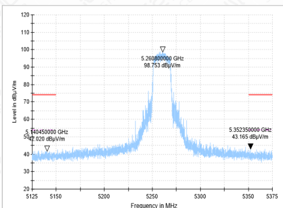
Bandedge-11N(20M)-CH52-PK
