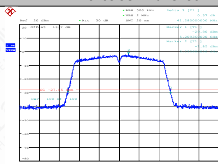
11AC40SISO-Ant1-5230
