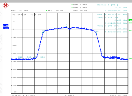
11N40SISO-Ant1-5510
