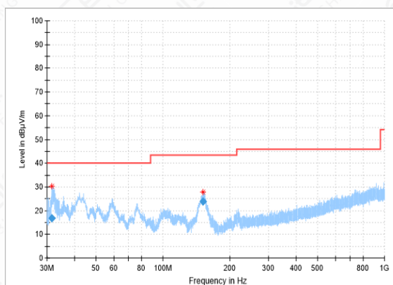
RSE-11N(20M)-CH60-30MHz-1GHz
