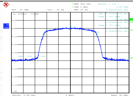
11AC20SISO-Ant1-5280
