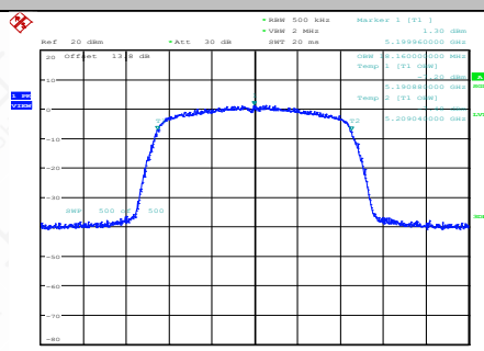
11AC20SISO-Ant1-5200
