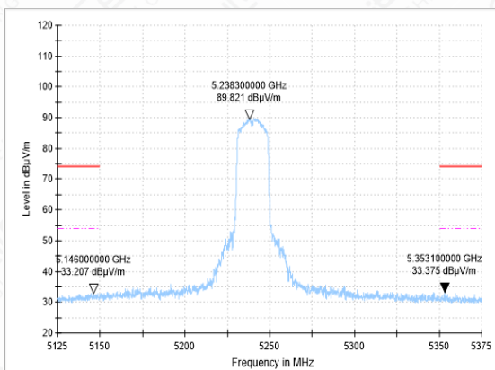
Bandedge-11N(20M)-CH48-AV
