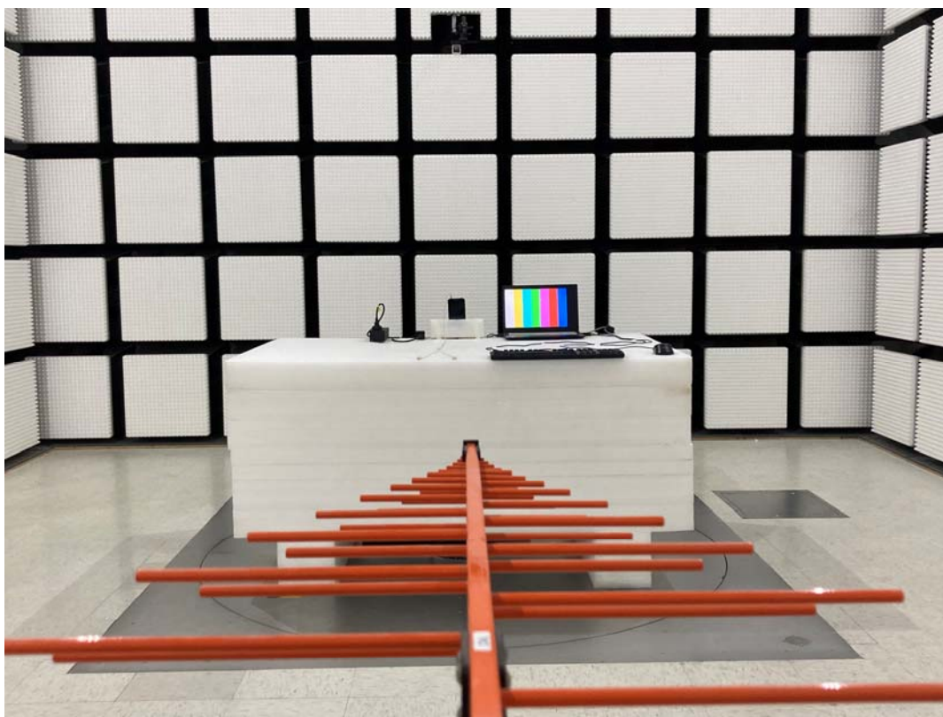
Radiated Emission Below 1G rear View-M3
