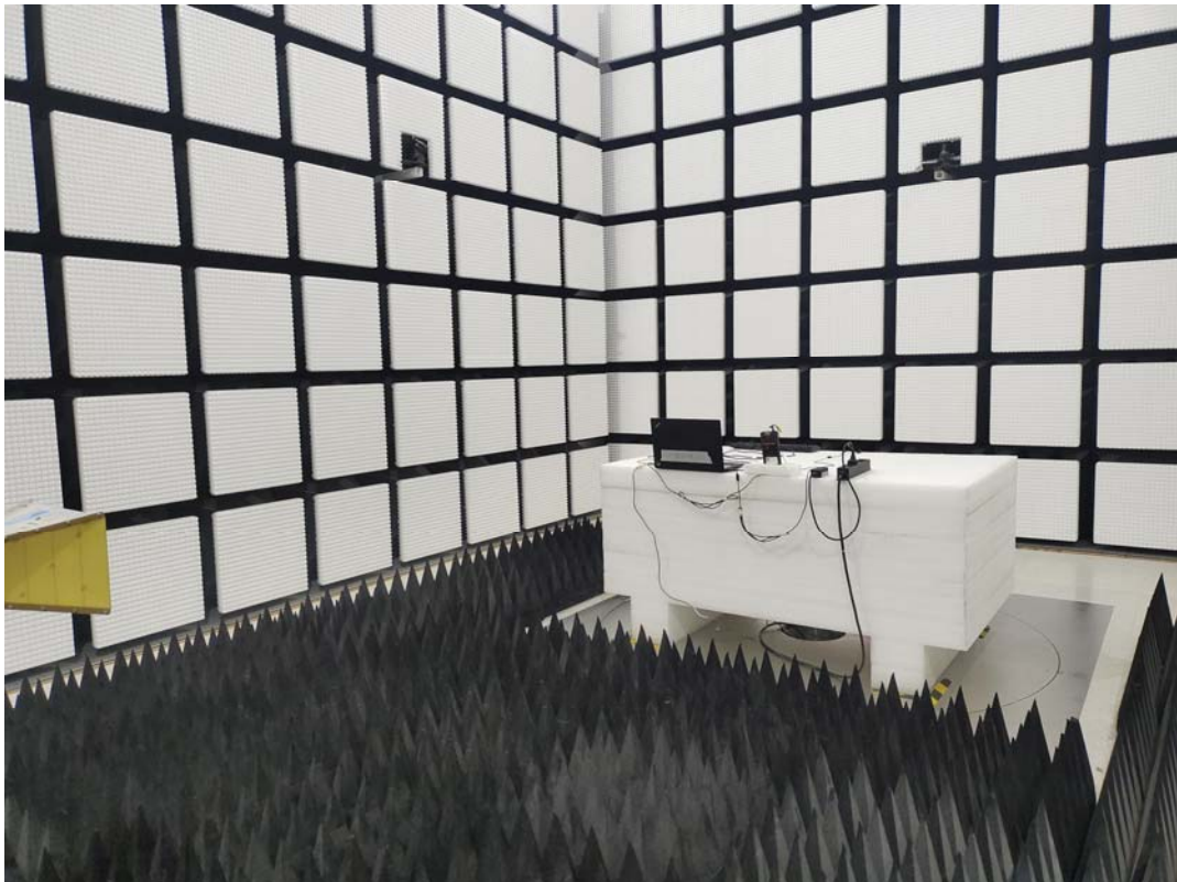
Radiated Emission Above 1G rear View-M3
