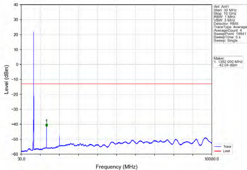
Band71_10MHz_16QAM_HCH_693MHz_RB_1_0_NTNV
