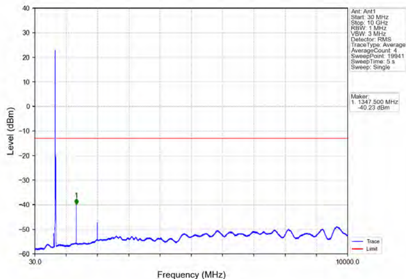
Band71_15MHz_QPSK_MCH_680.5MHz_RB_1_0_NTNV
