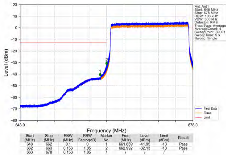
Band71_15MHz_QPSK_LCH_670.5MHz_RB_75_0_NTNV
