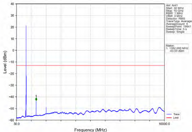
Band71_10MHz_64QAM_MCH_680.5MHz_RB_1_0_NTNV
