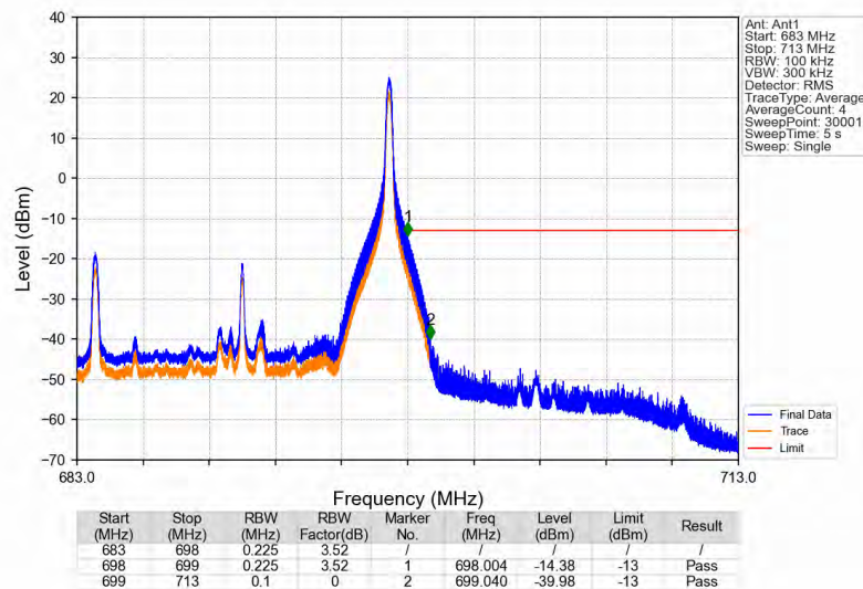
Band71_15MHz_16QAM_HCH_690.5MHz_RB_1_74_NTNV
