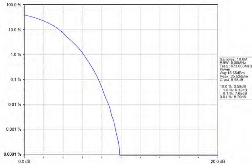
Band71_20MHz_64QAM_LCH_673MHz_RB_100_0_NTNV
