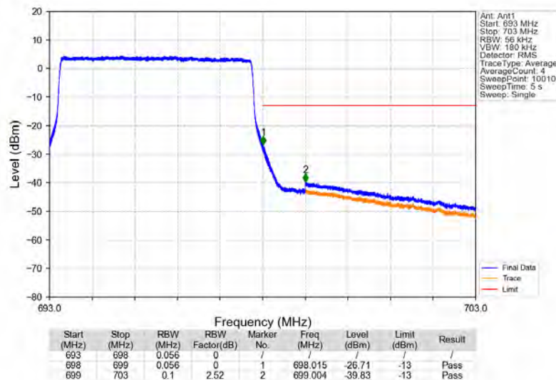
Band71_5MHz_16QAM_HCH_695.5MHz_RB_25_0_NTNV
