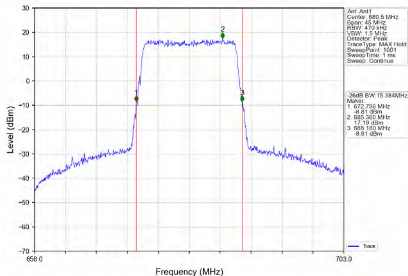
Band71_15MHz_64QAM_MCH_680.5MHz_RB_75_0_NTNV
