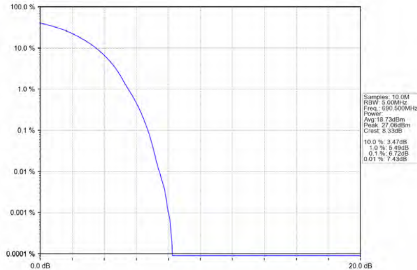
Band71_15MHz_QPSK_HCH_690.5MHz_RB_75_0_NTNV
