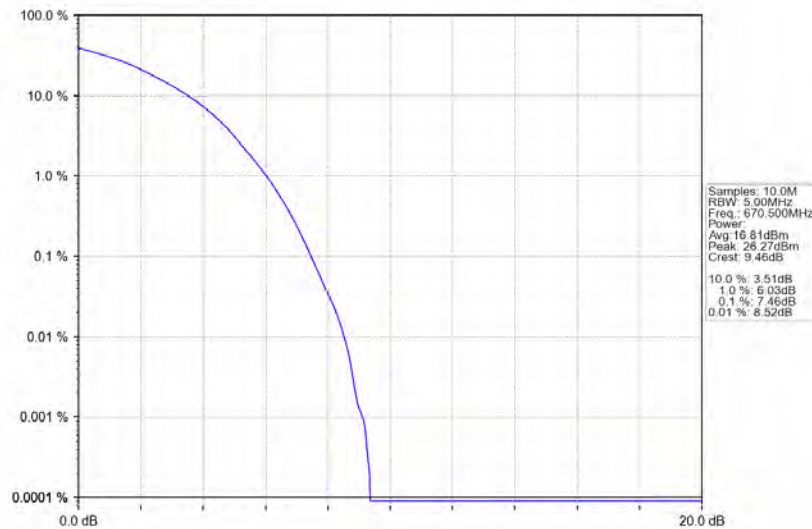
Band71_15MHz_64QAM_LCH_670.5MHz_RB_75_0_NTNV
