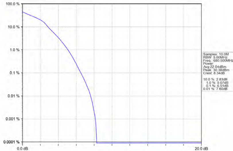
Band71_5MHz_16QAM_MCH_680.5MHz_RB_25_0_NTNV
