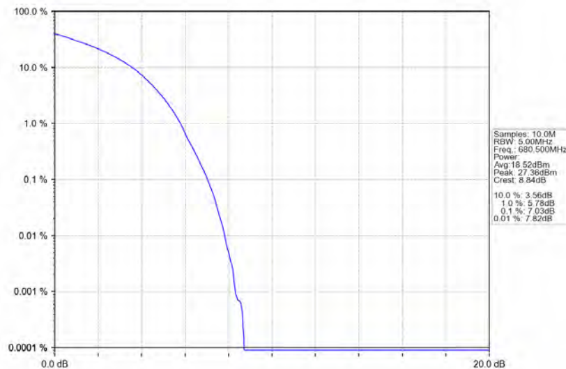
Band71_10MHz_64QAM_MCH_680.5MHz_RB_50_0_NTNV
