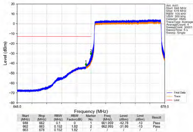
Band71_15MHz_16QAM_LCH_670.5MHz_RB_75_0_NTNV
