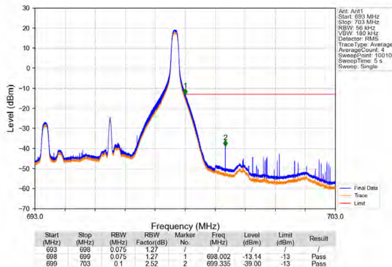
Band71_5MHz_64QAM_HCH_695.5MHz_RB_1_24_NTNV
