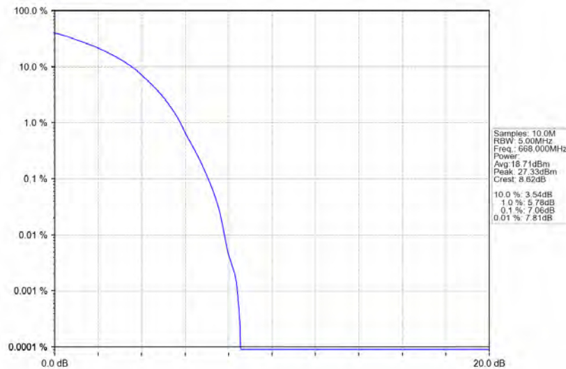
Band71_10MHz_64QAM_LCH_668MHz_RB_50_0_NTNV
