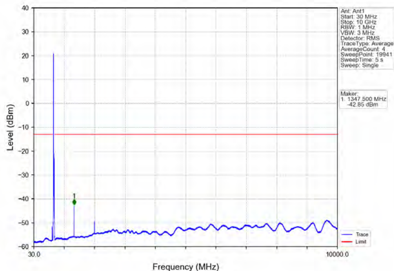
Band71 15MHz 64QAM MCH 680.5MHz RB 1 0 NTNV
