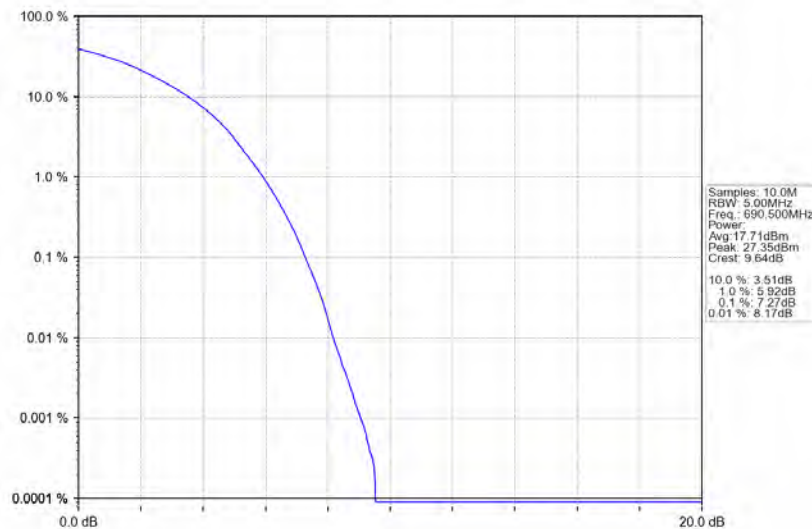
Band71_15MHz_16QAM_HCH_690.5MHz_RB_75_0_NTNV
