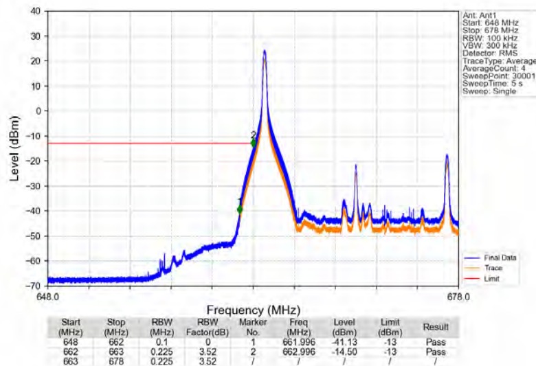
Band71_15MHz_16QAM_LCH_670.5MHz_RB_1_0_NTNV
