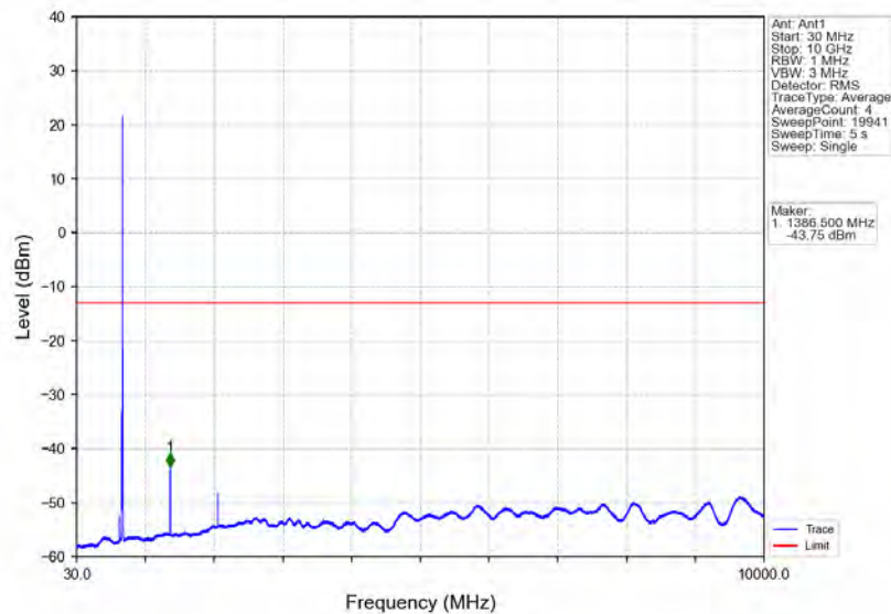
Band71_5MHz_64QAM_HCH_695.5MHz_RB_1_24_NTNV
