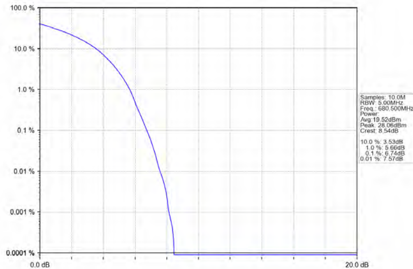
Band71_10MHz_16QAM_MCH_680.5MHz_RB_50_0_NTNV
