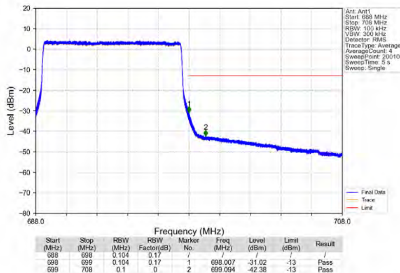
Band71_10MHz_16QAM_HCH_693MHz_RB_50_0_NTNV
