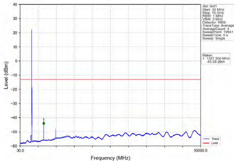
Band71_15MHz_16QAM_LCH_670.5MHz_RB_75_0_NTNV
