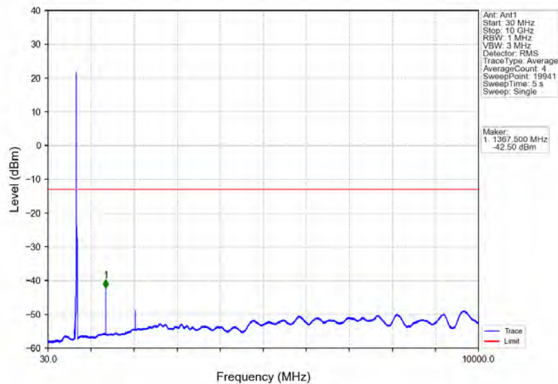
Band71_15MHz_64QAM_HCH_690.5MHz_RB_1_74_NTNV
