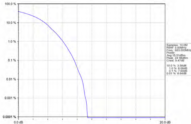
Band71_20MHz_64QAM_MCH_683MHz_RB_100_0_NTNV
