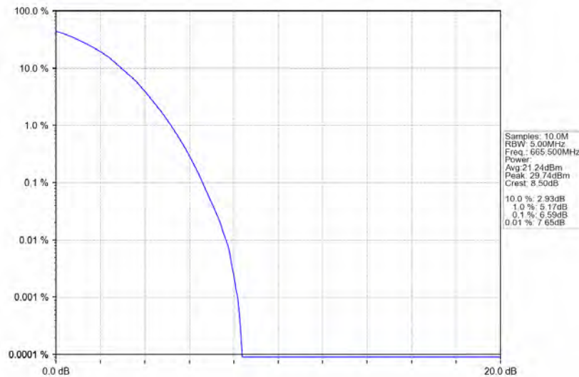
Band71_5MHz_64QAM_LCH_665.5MHz_RB_25_0_NTNV
