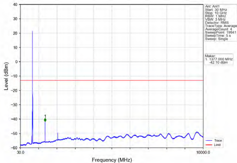
Band71_10MHz_64QAM_HCH_693MHz_RB_1_49_NTNV
