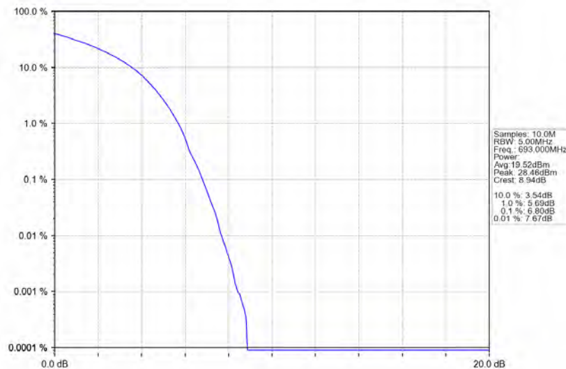
Band71_10MHz_16QAM_HCH_693MHz_RB_50_0_NTNV
