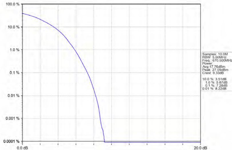
Band71_15MHz_16QAM_LCH_670.5MHz_RB_75_0_NTNV
