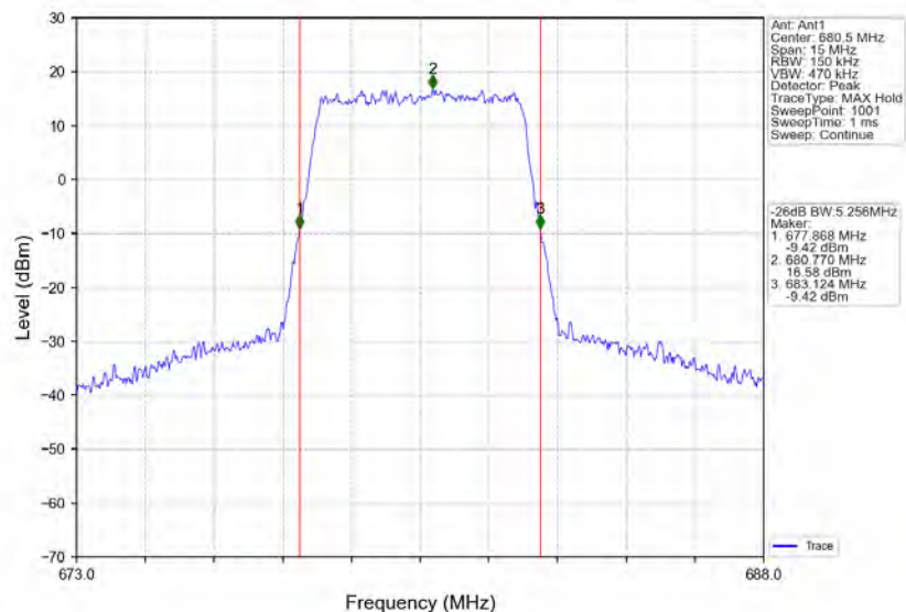
Band71_5MHz_64QAM_MCH_680.5MHz_RB_25_0_NTNV
