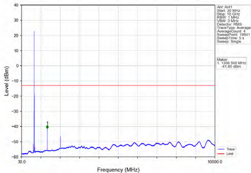
Band71_5MHz_QPSK_MCH_680.5MHz_RB_1_0_NTNV
