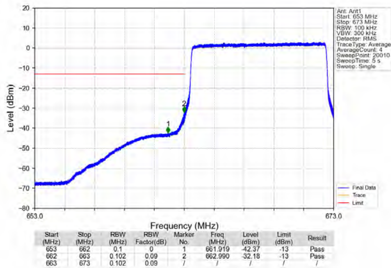
Band71_10MHz_64QAM_LCH_668MHz_RB_50_0_NTNV
