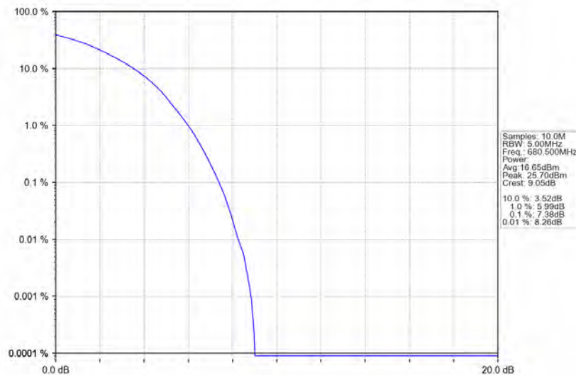
Band71_15MHz_64QAM_MCH_680.5MHz_RB_75_0_NTNV
