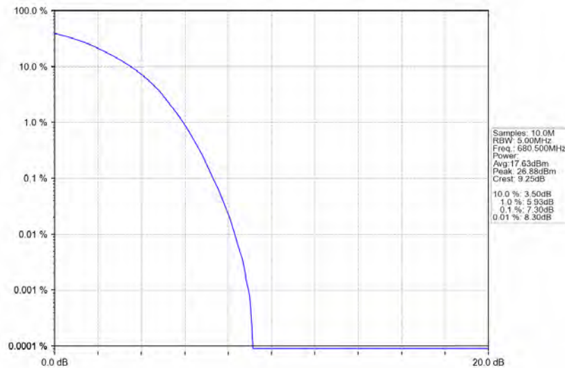
Band71_15MHz_16QAM_MCH_680.5MHz_RB_75_0_NTNV
