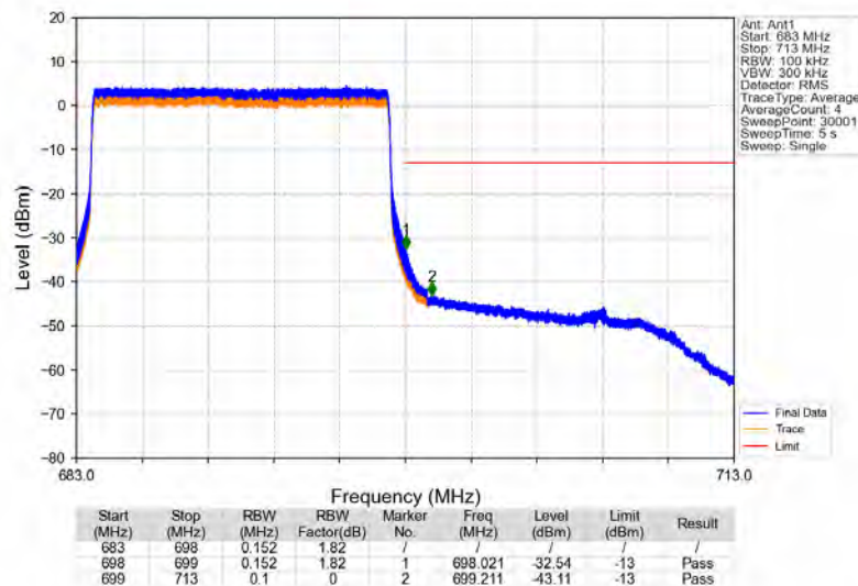
Band71_15MHz_16QAM_HCH_690.5MHz_RB_75_0_NTNV
