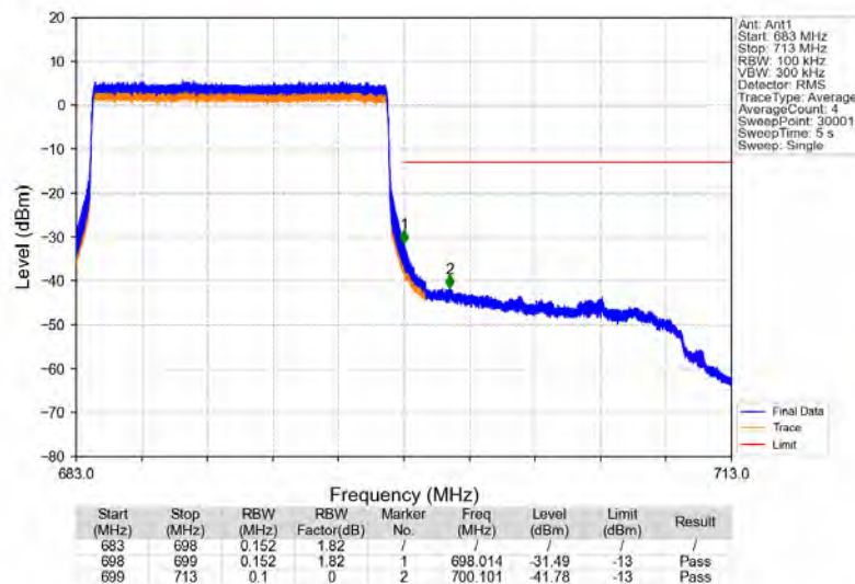
Band71_15MHz_QPSK_HCH_690.5MHz_RB_75_0_NTNV
