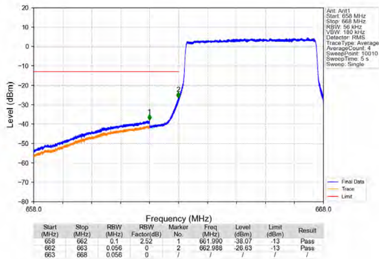
Band71_5MHz_16QAM_LCH_665.5MHz_RB_25_0_NTNV
