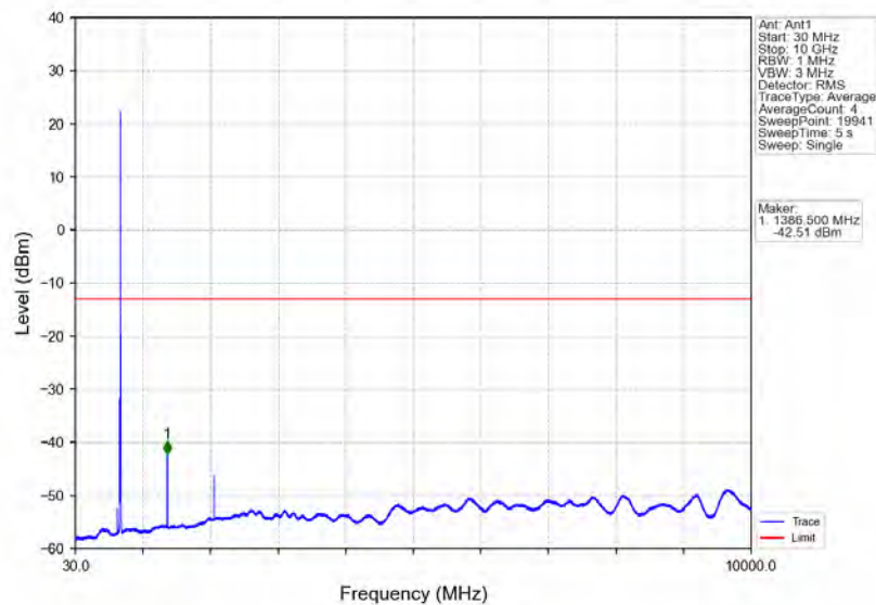
Band71_5MHz_16QAM_HCH_695.5MHz_RB_1_0_NTNV
