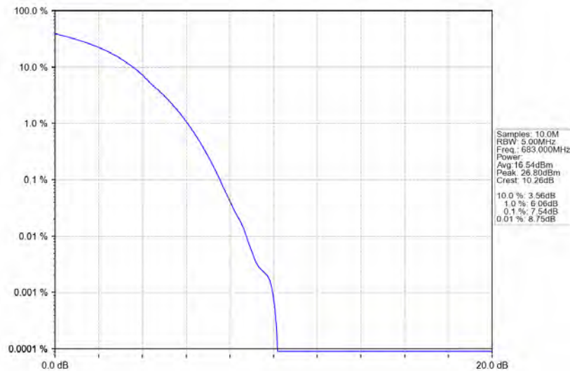
Band71_20MHz_16QAM_MCH_683MHz_RB_100_0_NTNV
