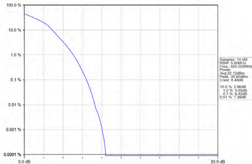
Band71_5MHz_16QAM_LCH_665.5MHz_RB_25_0_NTNV
