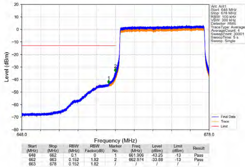
Band71 15MHz 64QAM LCH 670.5MHz RB 75 0 NTNV
