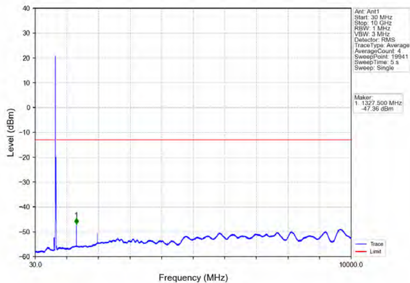
Band71_15MHz_64QAM_LCH_670.5MHz_RB_1_0_NTNV
