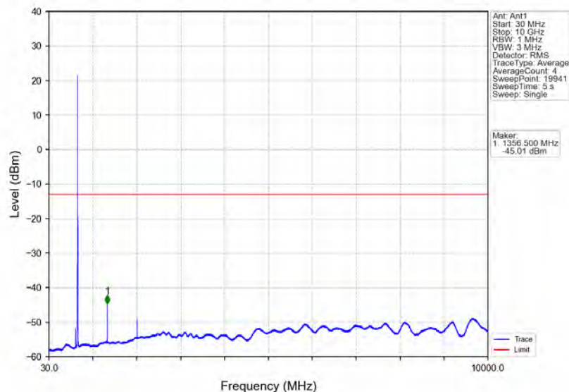
Band71_5MHz_64QAM_MCH_680.5MHz_RB_1_0_NTNV
