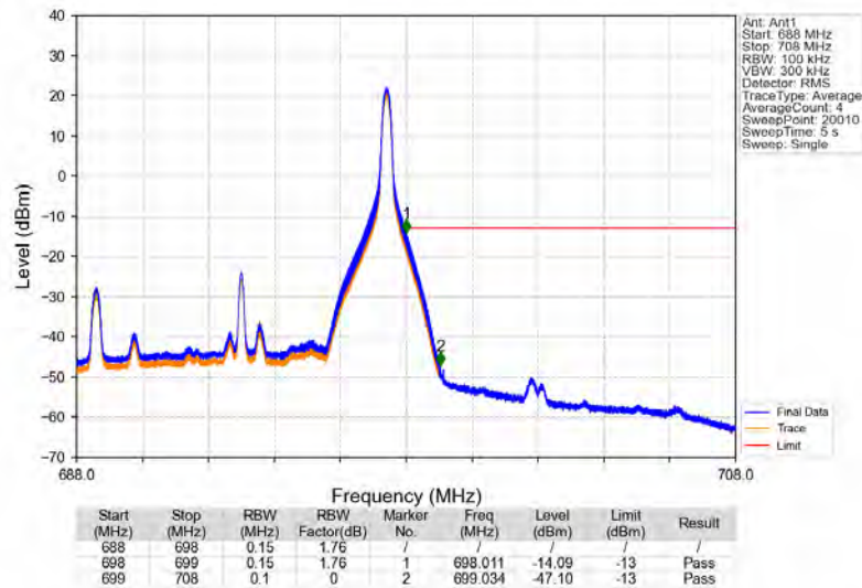
Band71_10MHz_64QAM_HCH_693MHz_RB_1_49_NTNV
