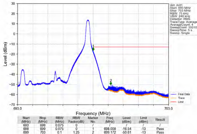
Band71_5MHz_16QAM_HCH_695.5MHz_RB_1_24_NTNV
