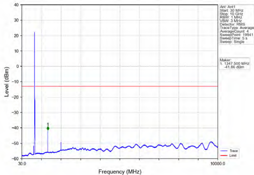
Band71_15MHz_16QAM_HCH_690.5MHz_RB_1_0_NTNV
