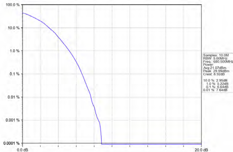
Band71_5MHz_64QAM_MCH_680.5MHz_RB_25_0_NTNV
