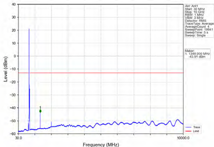
Band71_20MHz_64QAM_MCH_683MHz_RB_1_0_NTNV
