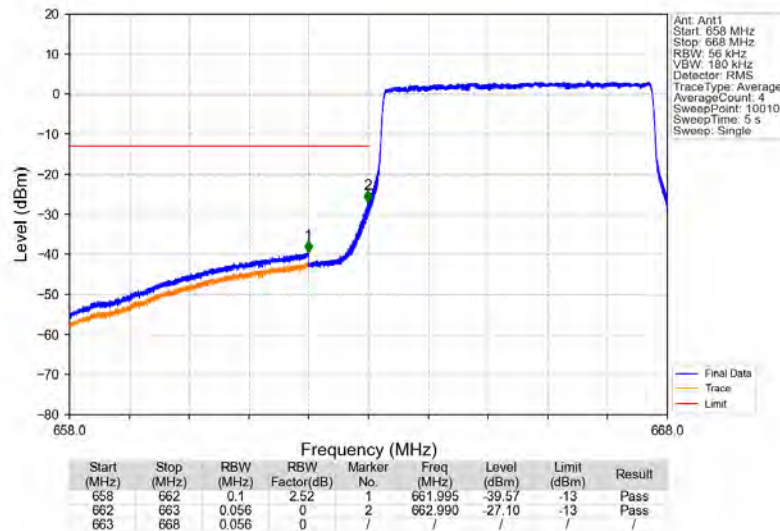
Band71_5MHz_64QAM_LCH_665.5MHz_RB_25_0_NTNV
