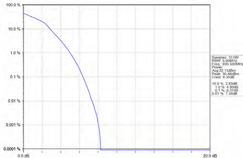
Band71_5MHz_16QAM_HCH_695.5MHz_RB_25_0_NTNV
