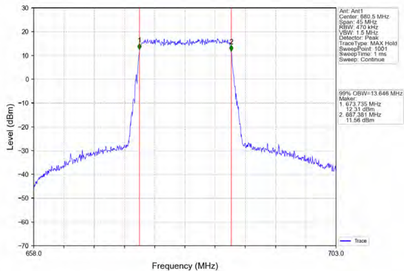
Band71_15MHz_64QAM_MCH_680.5MHz_RB_75_0_NTNV
