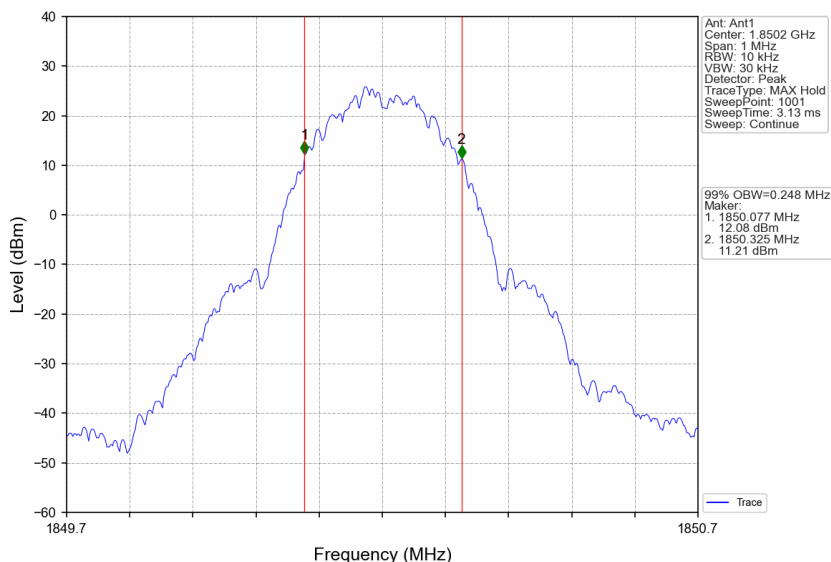
PCS1900_GPRS_LCH_1850.2MHz_1 TX Slot_NTNV
