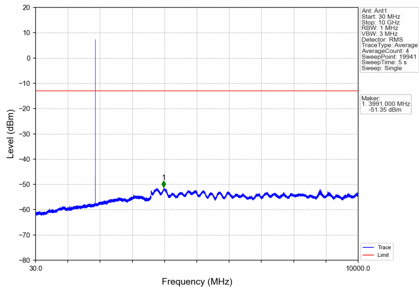
PCS1900_GPRS_MCH_1880MHz_1 TX Slot_NTNV
