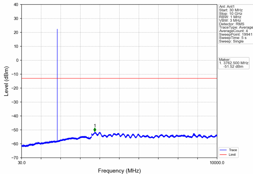
PCS1900_GPRS_LCH_1850.2MHz_1 TX Slot_NTNV
