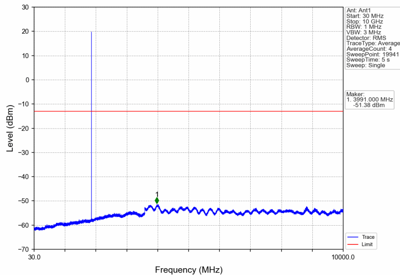
PCS1900_EGPRS_MCH_1880MHz_1 TX Slot_NTNV
