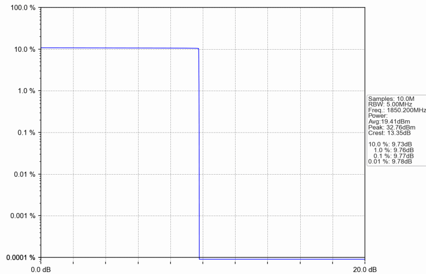
PCS1900_GPRS_LCH_1850.2MHz_4 TX Slots_NTNV
