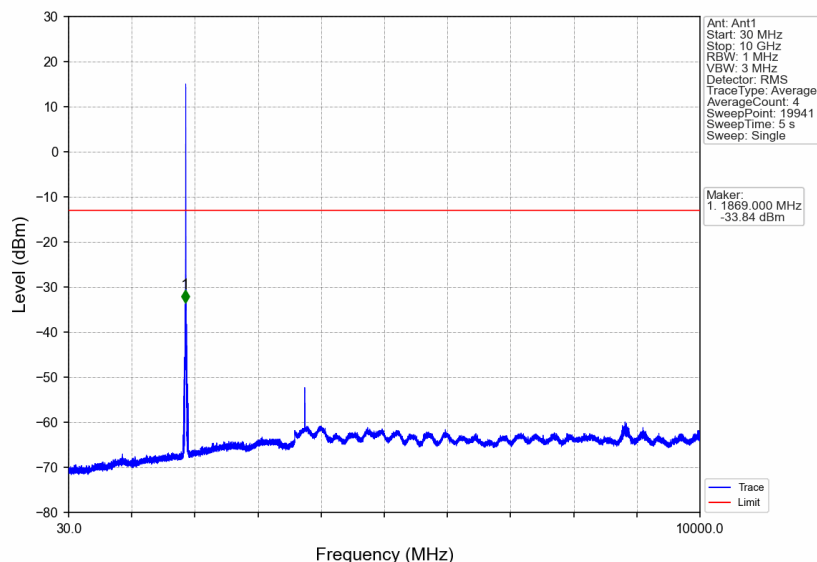
Band2_HSDPA_MCH_1880MHz_Subtest 1_NTNV
