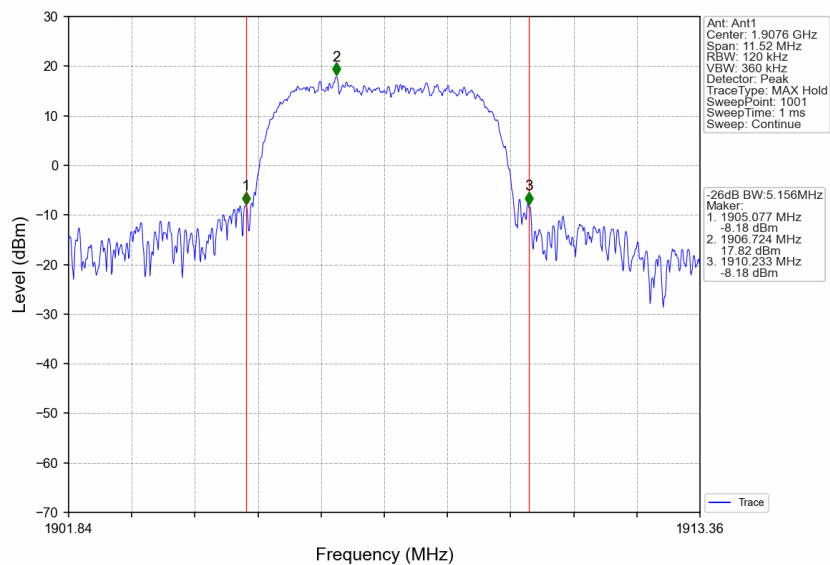
Band2_HSUPA_HCH_1907.6MHz_Subtest 1_NTNV
