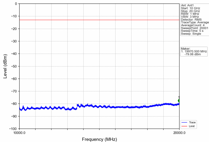
Band2_HSUPA_HCH_1907.6MHz_Subtest 1_NTNV
