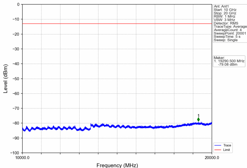
Band2_RMC_MCH_1880MHz_12.2kbps RMC_NTNV
