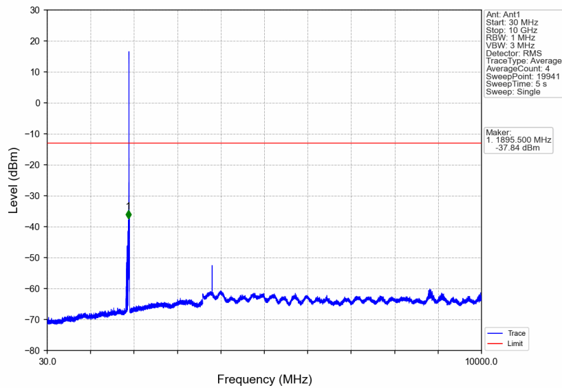
Band2_HSDPA_HCH_1907.6MHz_Subtest 1_NTNV
