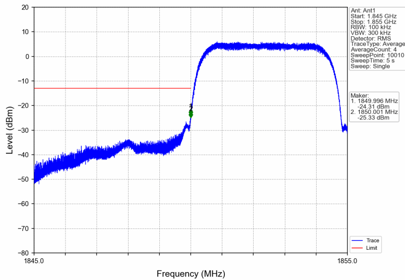
Band2_HSUPA_LCH_1852.4MHz_Subtest 1_NTNV
