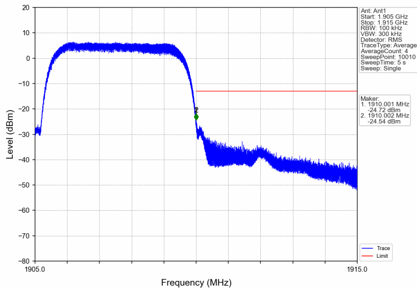
Band2_HSUPA_HCH_1907.6MHz_Subtest 1_NTNV
