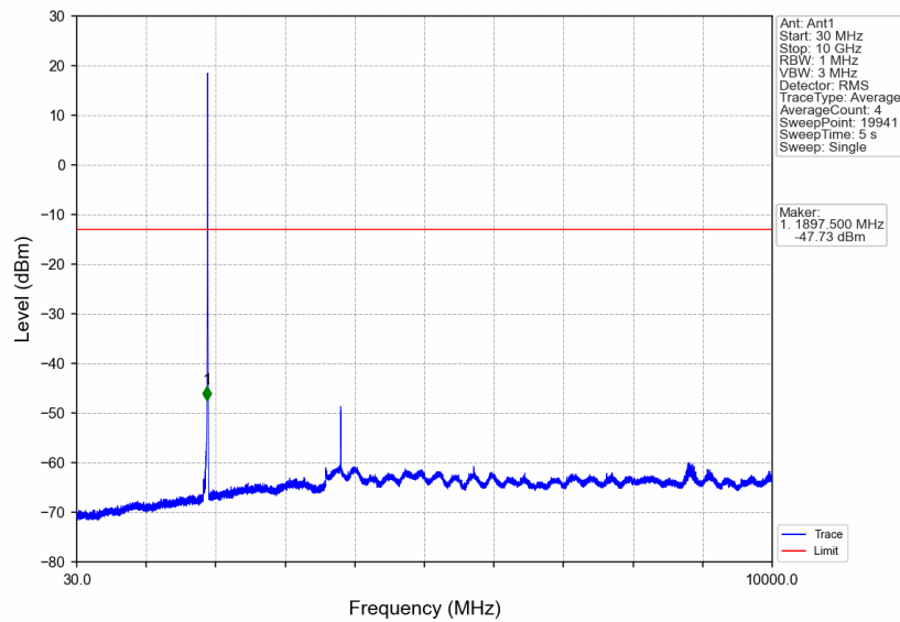
Band2_RMC_HCH_1907.6MHz_12.2kbps RMC_NTNV
