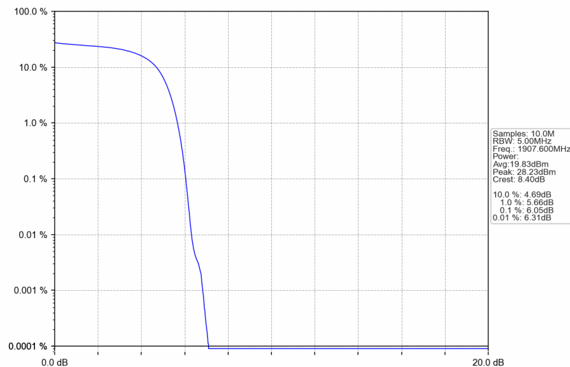
Band2_HSUPA_HCH_1907.6MHz_Subtest 1_NTNV
