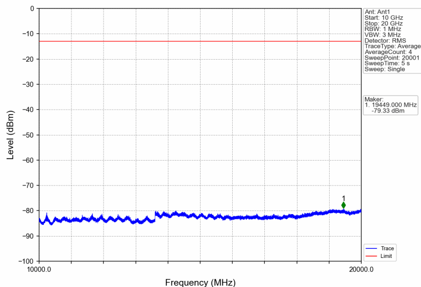
Band2_HSDPA_HCH_1907.6MHz_Subtest 1_NTNV
