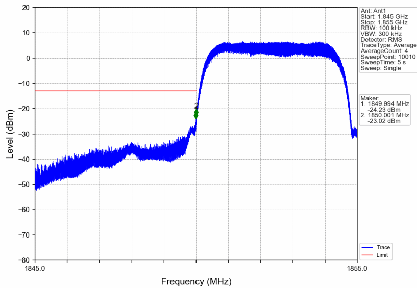
Band2_HSDPA_LCH_1852.4MHz_Subtest 1_NTNV
