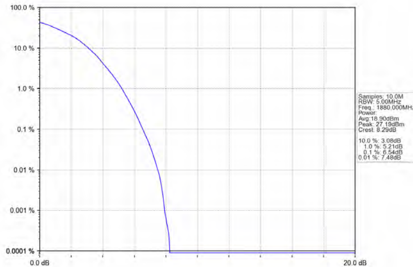
Band2_3MHz_64QAM_MCH_1880MHz_RB_15_0_NTNV
