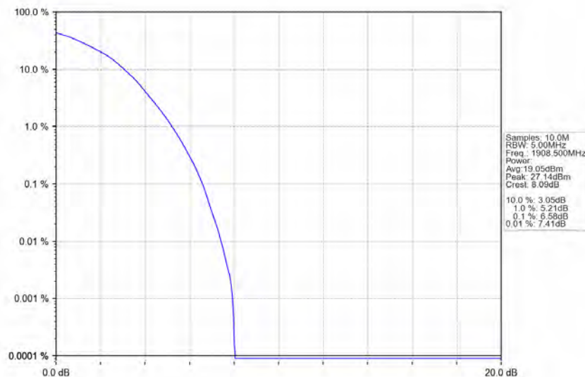
Band2_3MHz_64QAM_HCH_1908.5MHz_RB_15_0_NTNV
