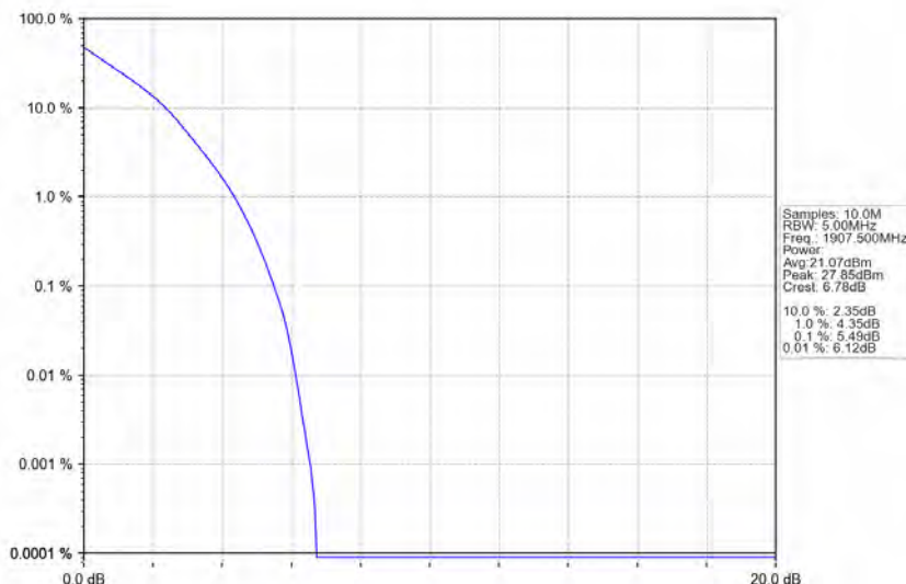
Band2_5MHz_QPSK_HCH_1907.5MHz_RB_25_0_NTNV
