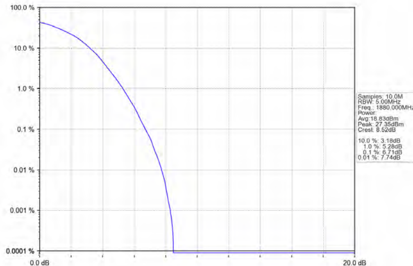
Band2_1.4MHz_64QAM_MCH_1880MHz_RB_6_0_NTNV
