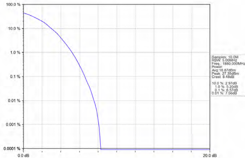
Band2_5MHz_64QAM_MCH_1880MHz_RB_25_0_NTNV
