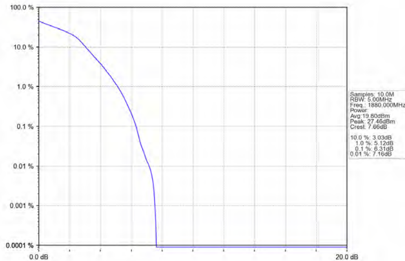
Band2_1.4MHz_16QAM_MCH_1880MHz_RB_6_0_NTNV
