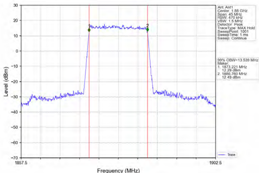
Band2_15MHz_QPSK_MCH_1880MHz_RB_75_0_NTNV
