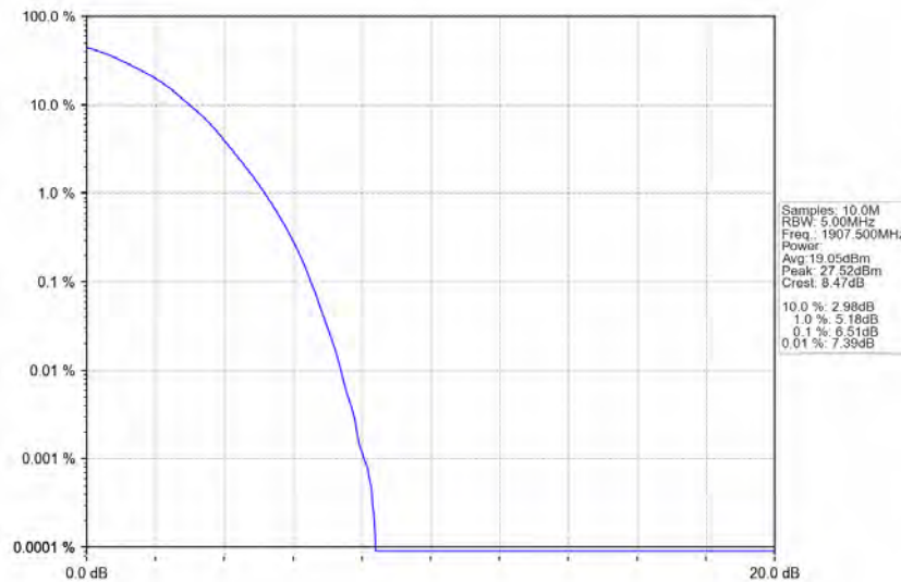
Band2_5MHz_64QAM_HCH_1907.5MHz_RB_25_0_NTNV
