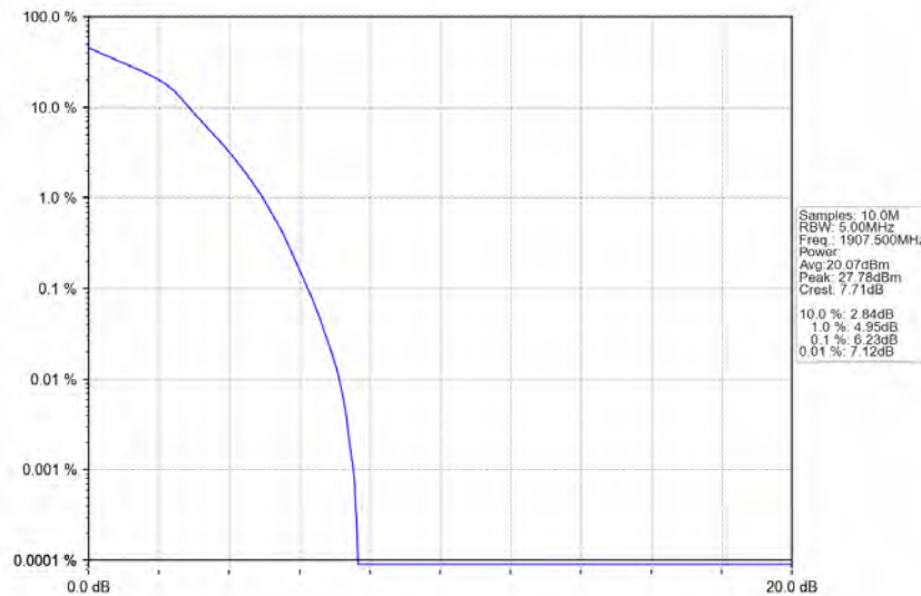
Band2_5MHz_16QAM_HCH_1907.5MHz_RB_25_0_NTNV
