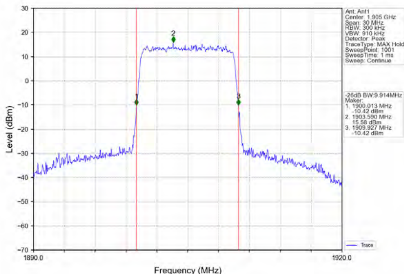
Band2_10MHz_64QAM_HCH_1905MHz_RB_50_0_NTNV
