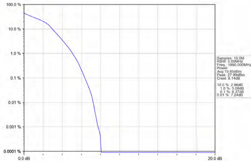
Band2_3MHz_16QAM_MCH_1880MHz_RB_15_0_NTNV
