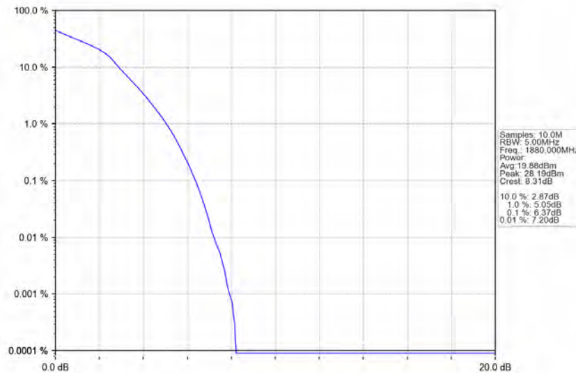
Band2_5MHz_16QAM_MCH_1880MHz_RB_25_0_NTNV
