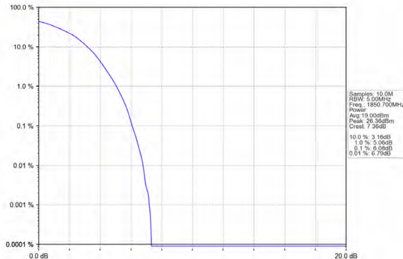
Band2_1.4MHz_64QAM_LCH_1850.7MHz_RB_6_0_NTNV
