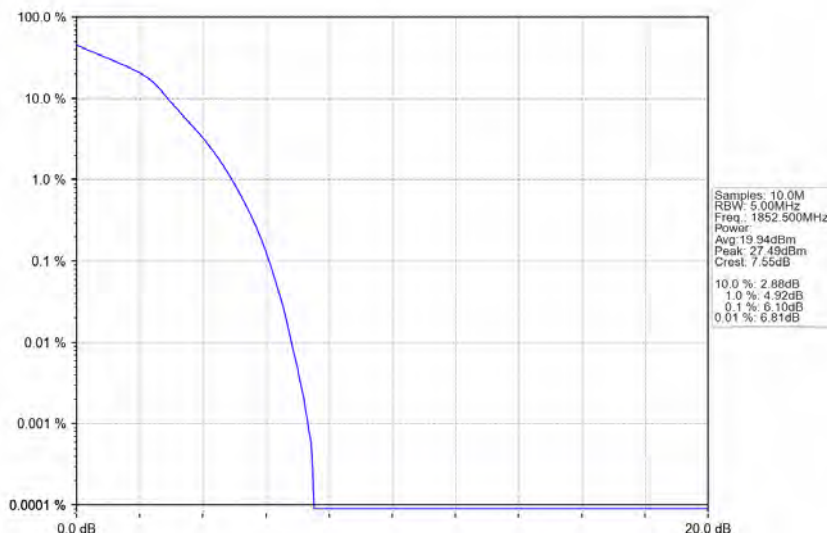
Band2_5MHz_16QAM_LCH_1852.5MHz_RB_25_0_NTNV
