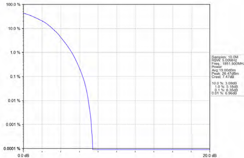
Band2_3MHz_64QAM_LCH_1851.5MHz_RB_15_0_NTNV
