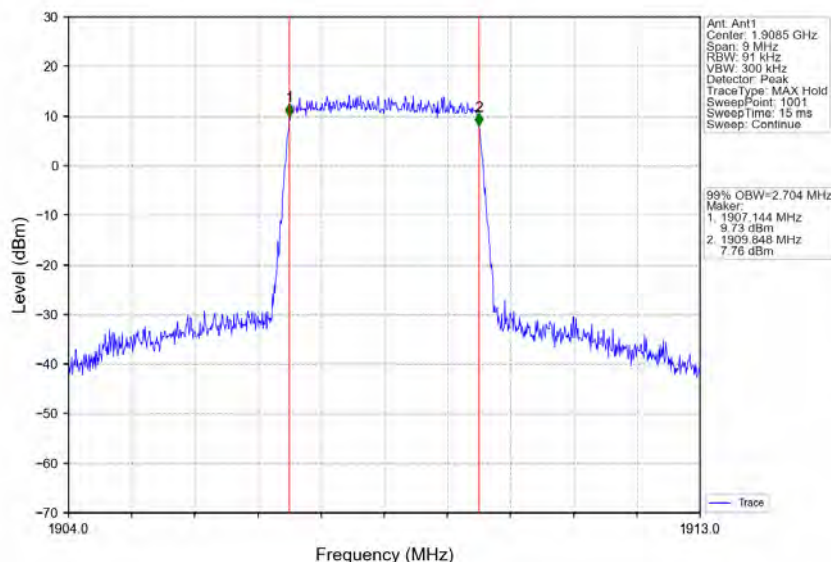
Band2_3MHz_64QAM_HCH_1908.5MHz_RB_15_0_NTNV
