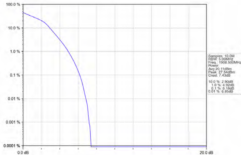
Band2_3MHz_16QAM_HCH_1908.5MHz_RB_15_0_NTNV
