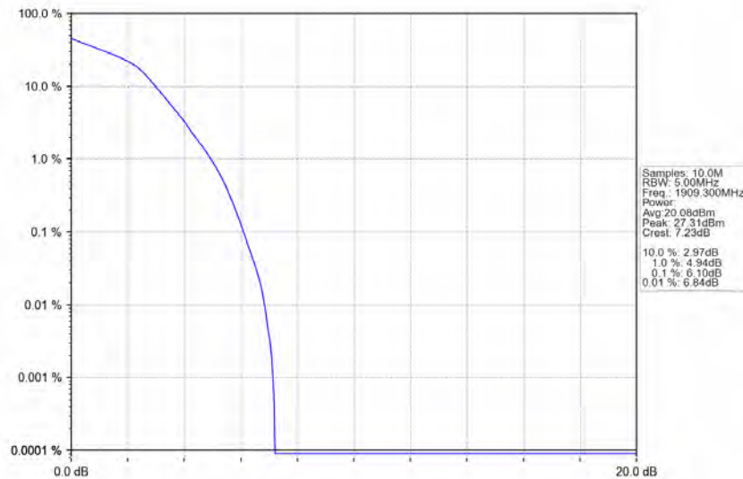
Band2_1.4MHz_16QAM_HCH_1909.3MHz_RB_6_0_NTNV
