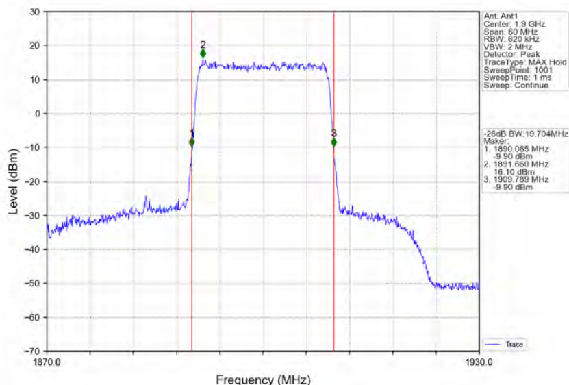
Band2_20MHz_64QAM_HCH_1900MHz_RB_100_0_NTNV
