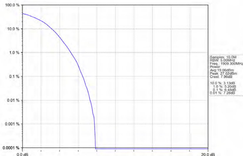
Band2_1.4MHz_64QAM_HCH_1909.3MHz_RB_6_0_NTNV
