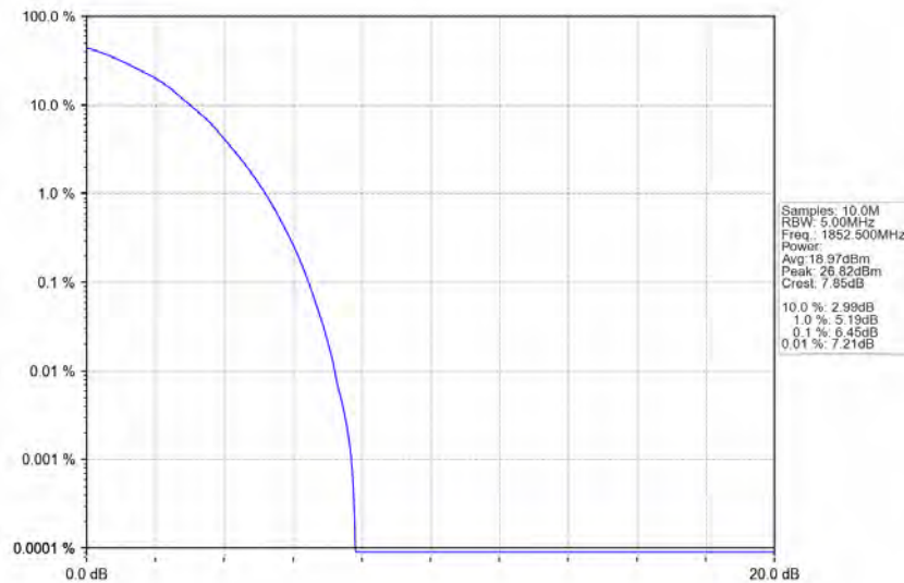
Band2_5MHz_64QAM_LCH_1852.5MHz_RB_25_0_NTNV
