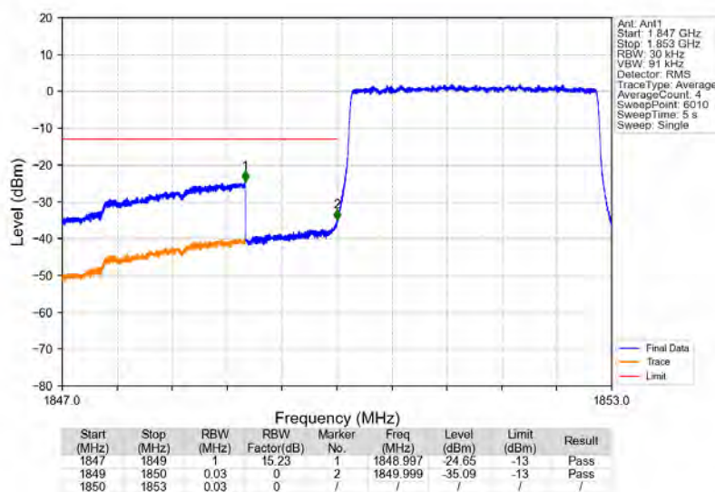
Band2_3MHz_16QAM_LCH_1851.5MHz_RB_15_0_NTNV
