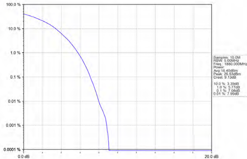
Band2_15MHz_16QAM_MCH_1880MHz_RB_75_0_NTNV
