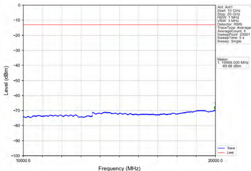
Band2_1.4MHz_QPSK_LCH_1850.7MHz_RB_6_0_NTNV
