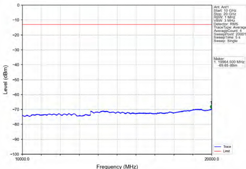
Band2_1.4MHz_64QAM_MCH_1880MHz_RB_1_0_NTNV
