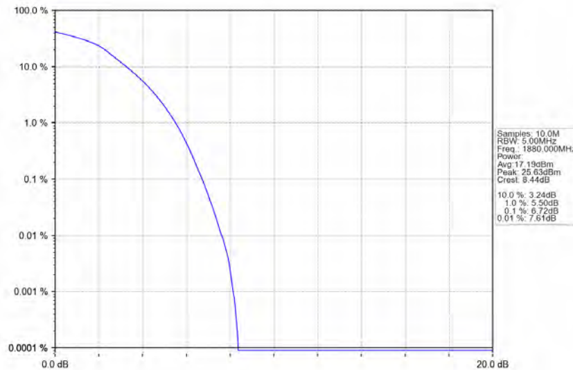
Band2_10MHz_64QAM_MCH_1880MHz_RB_50_0_NTNV
