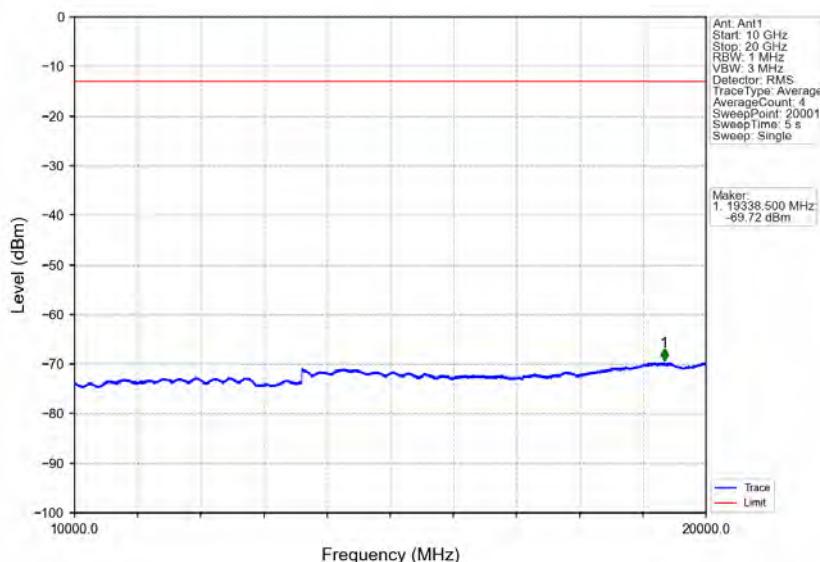
Band2_15MHz_16QAM_HCH_1902.5MHz_RB_1_0_NTNV
