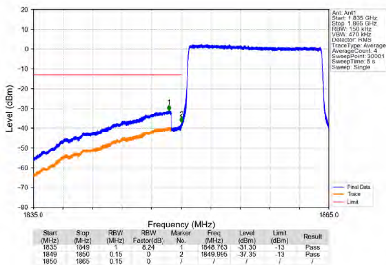
Band2_15MHz_16QAM_LCH_1857.5MHz_RB_75_0_NTNV
