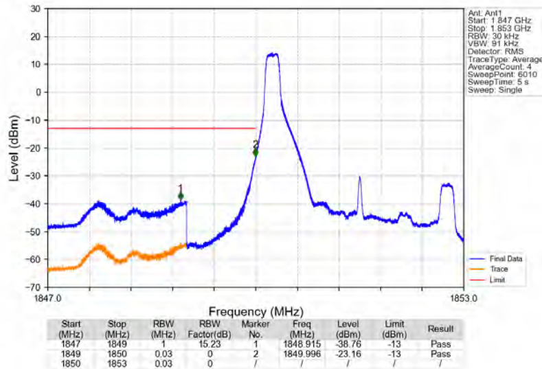
Band2_3MHz_16QAM_LCH_1851.5MHz_RB_1_0_NTNV
