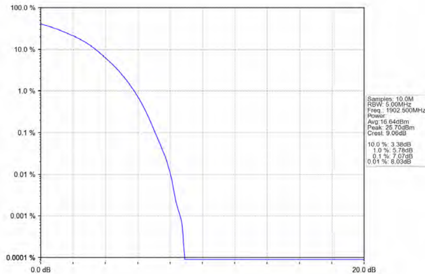
Band2_15MHz_16QAM_HCH_1902.5MHz_RB_75_0_NTNV
