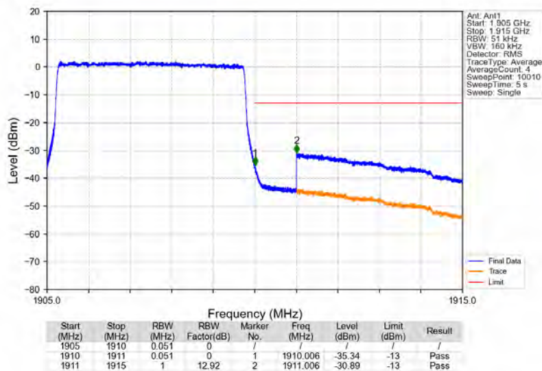
Band2_5MHz_16QAM_HCH_1907.5MHz_RB_25_0_NTNV
