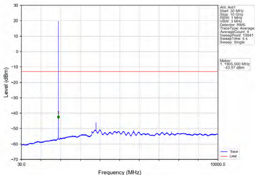
Band2_1.4MHz_64QAM_HCH_1909.3MHz_RB_1_0_NTNV
