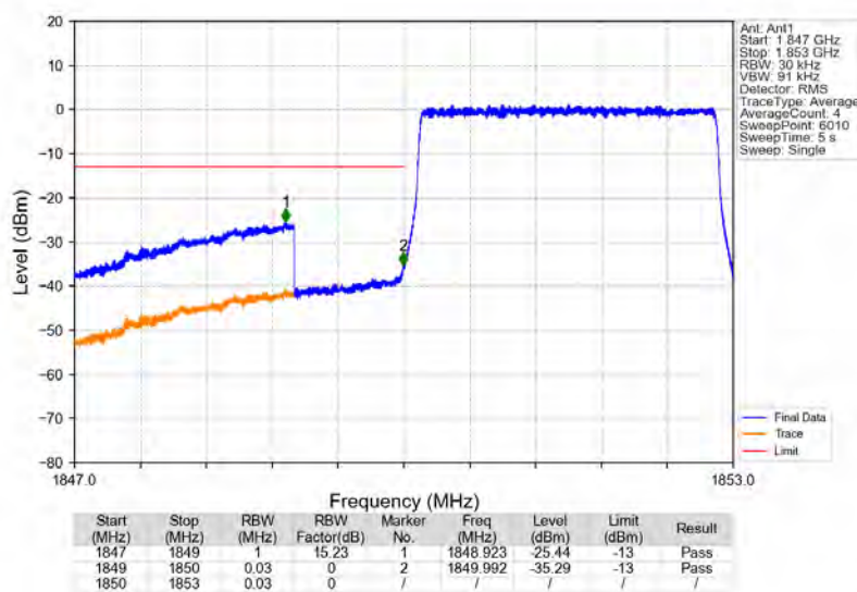
Band2_3MHz_64QAM_LCH_1851.5MHz_RB_15_0_NTNV
