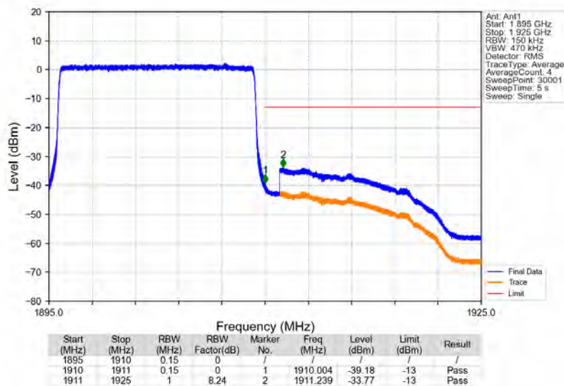
Band2_15MHz_16QAM_HCH_1902.5MHz_RB_75_0_NTNV
