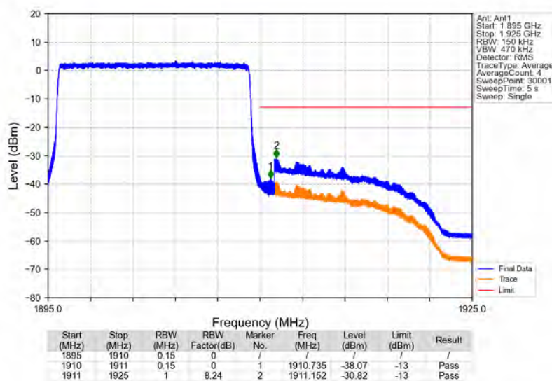
Band2_15MHz_QPSK_HCH_1902.5MHz_RB_75_0_NTNV
