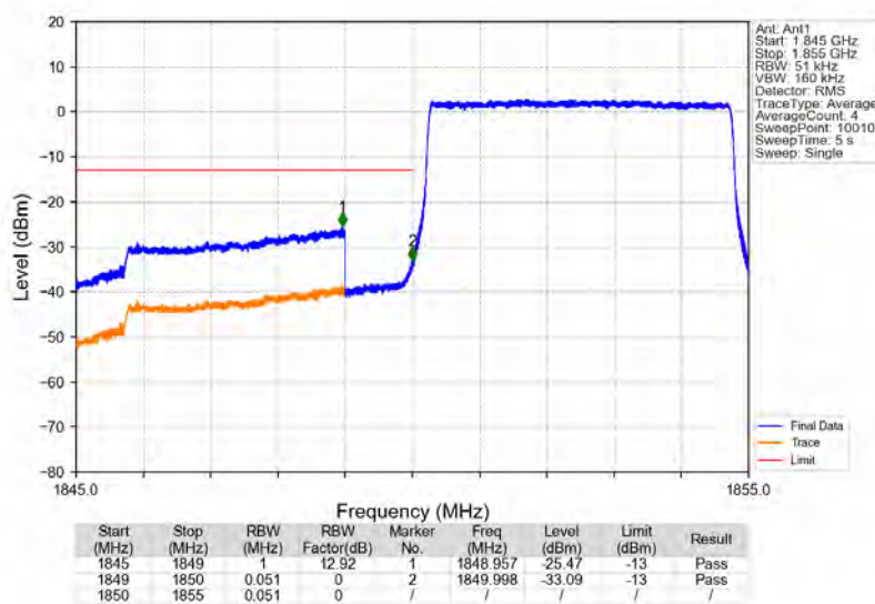
Band2_5MHz_QPSK_LCH_1852.5MHz_RB_25_0_NTNV
