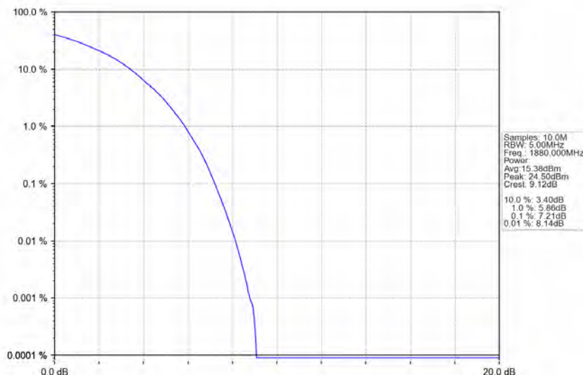
Band2_15MHz_64QAM_MCH_1880MHz_RB_75_0_NTNV
