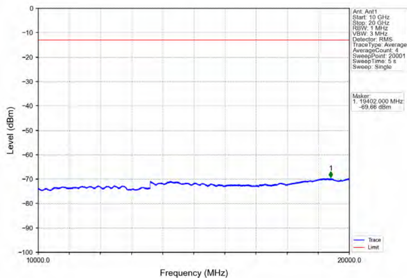
Band2_10MHz_64QAM_MCH_1880MHz_RB_1_0_NTNV
