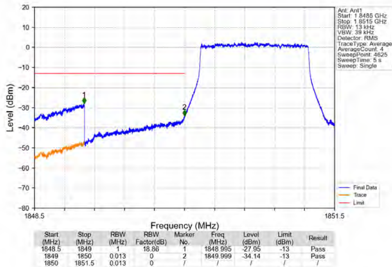
Band2_1.4MHz_16QAM_LCH_1850.7MHz_RB_6_0_NTNV
