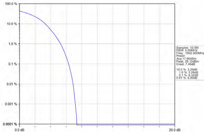
Band2_15MHz_QPSK_HCH_1902.5MHz_RB_75_0_NTNV
