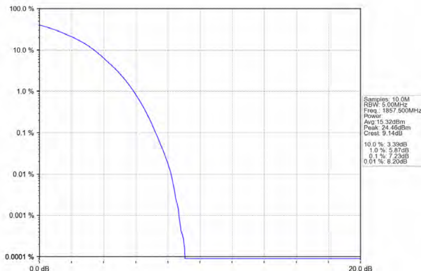
Band2_15MHz_64QAM_LCH_1857.5MHz_RB_75_0_NTNV
