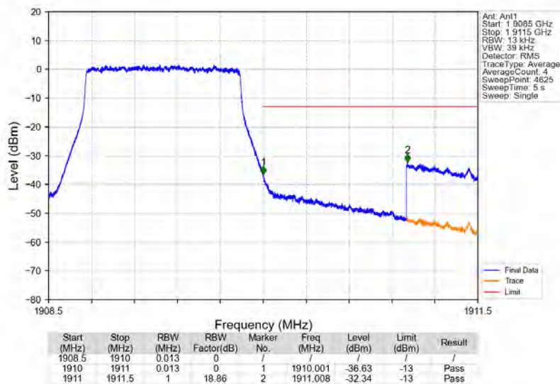
Band2_1.4MHz_64QAM_HCH_1909.3MHz_RB_6_0_NTNV
