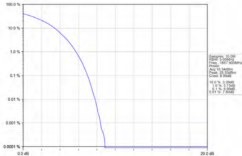
Band2_15MHz_16QAM_LCH_1857.5MHz_RB_75_0_NTNV
