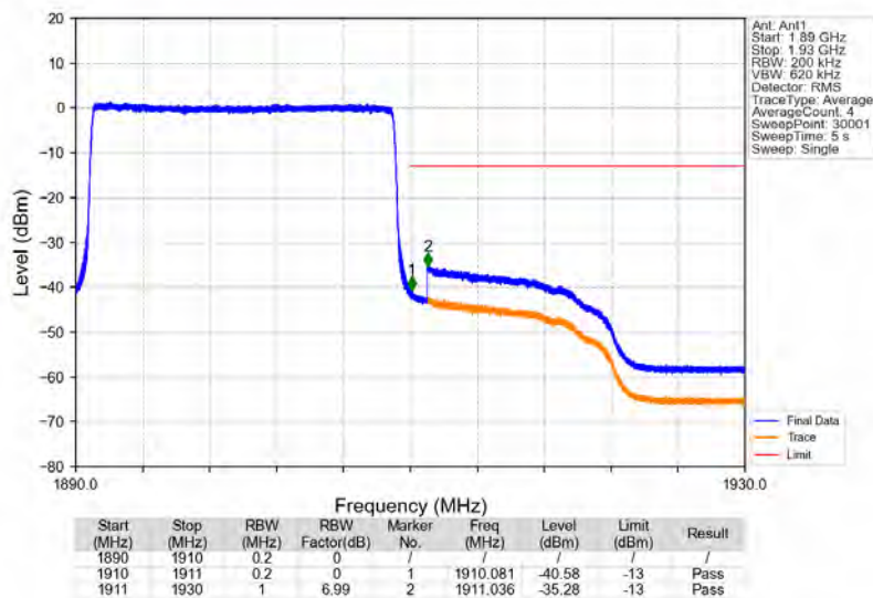
Band2_20MHz_64QAM_HCH_1900MHz_RB_100_0_NTNV
