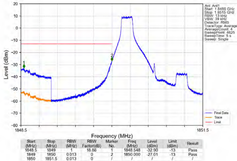
Band2_1.4MHz_64QAM_LCH_1850.7MHz_RB_1_0_NTNV
