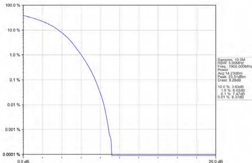
Band2_20MHz_64QAM_HCH_1900MHz_RB_100_0_NTNV
