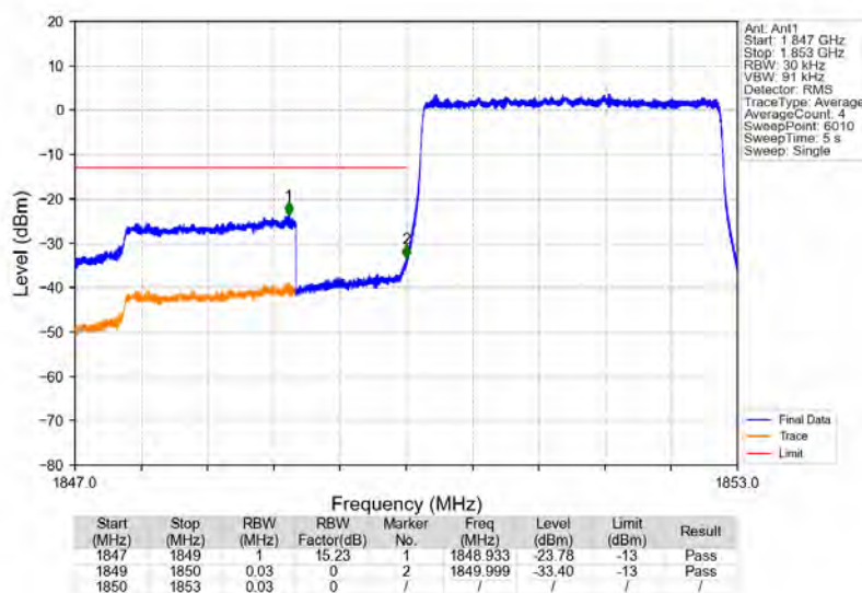
Band2_3MHz_QPSK_LCH_1851.5MHz_RB_15_0_NTNV
