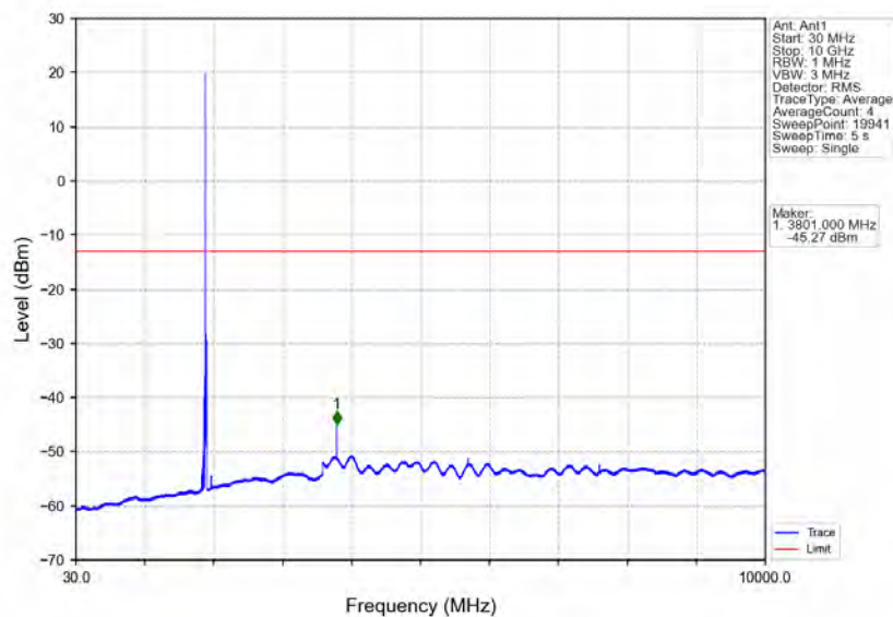
Band2_10MHz_64QAM_HCH_1905MHz_RB_1_0_NTNV
