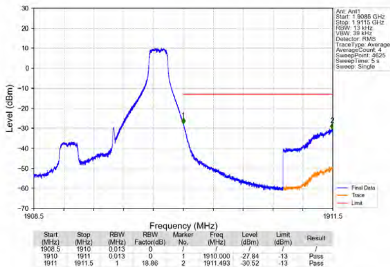
Band2_1.4MHz_64QAM_HCH_1909.3MHz_RB_1_5_NTNV
