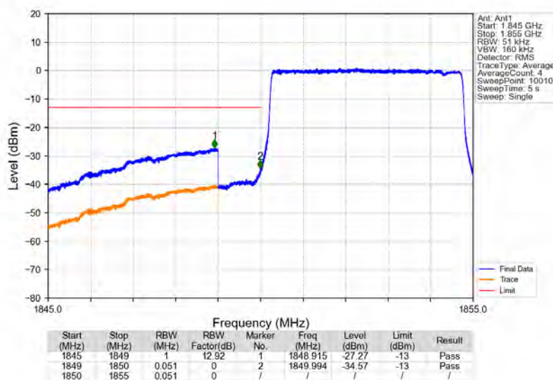
Band2_5MHz_64QAM_LCH_1852.5MHz_RB_25_0_NTNV
