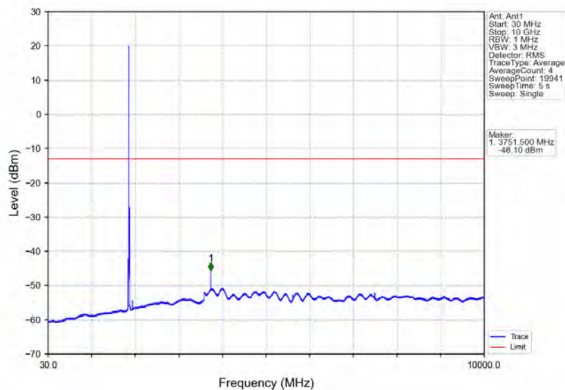
Band2_10MHz_64QAM_MCH_1880MHz_RB_1_0_NTNV
