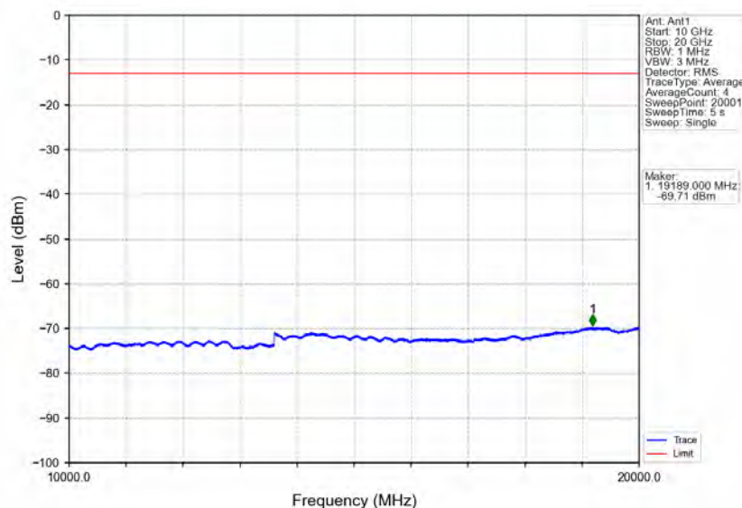
Band2_5MHz_QPSK_LCH_1852.5MHz_RB_25_0_NTNV
