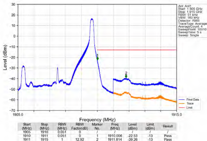
Band2_5MHz_16QAM_HCH_1907.5MHz_RB_1_24_NTNV
