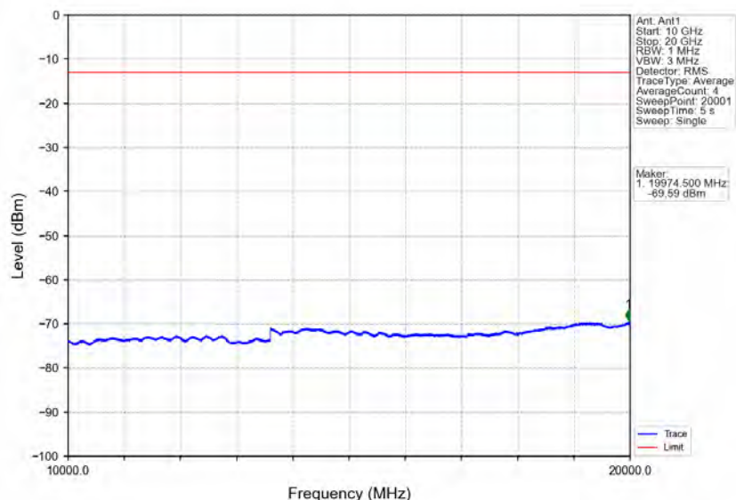
Band2_1.4MHz_64QAM_HCH_1909.3MHz_RB_1_0_NTNV
