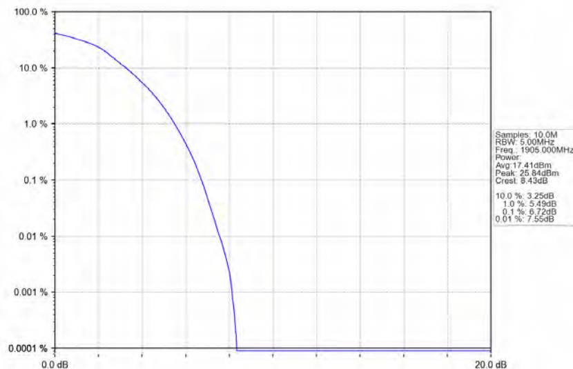
Band2_10MHz_64QAM_HCH_1905MHz_RB_50_0_NTNV
