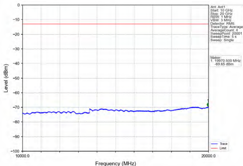
Band2_1.4MHz_64QAM_LCH_1850.7MHz_RB_6_0_NTNV
