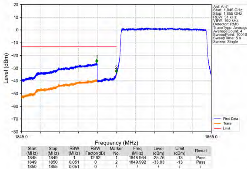
Band2_5MHz_16QAM_LCH_1852.5MHz_RB_25_0_NTNV
