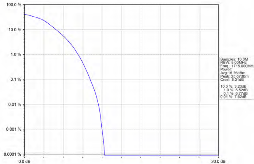
Band4_10MHz_64QAM_LCH_1715MHz_RB_50_0_NTNV
