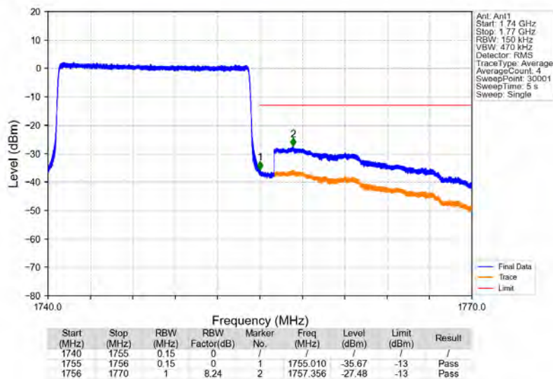
Band4_15MHz_16QAM_HCH_1747.5MHz_RB_75_0_NTNV
