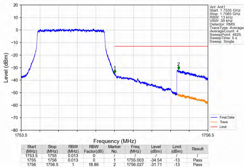
Band4_1.4MHz_64QAM_HCH_1754.3MHz_RB_6_0_NTNV
