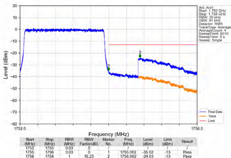
Band4_3MHz_64QAM_HCH_1753.5MHz_RB_15_0_NTNV
