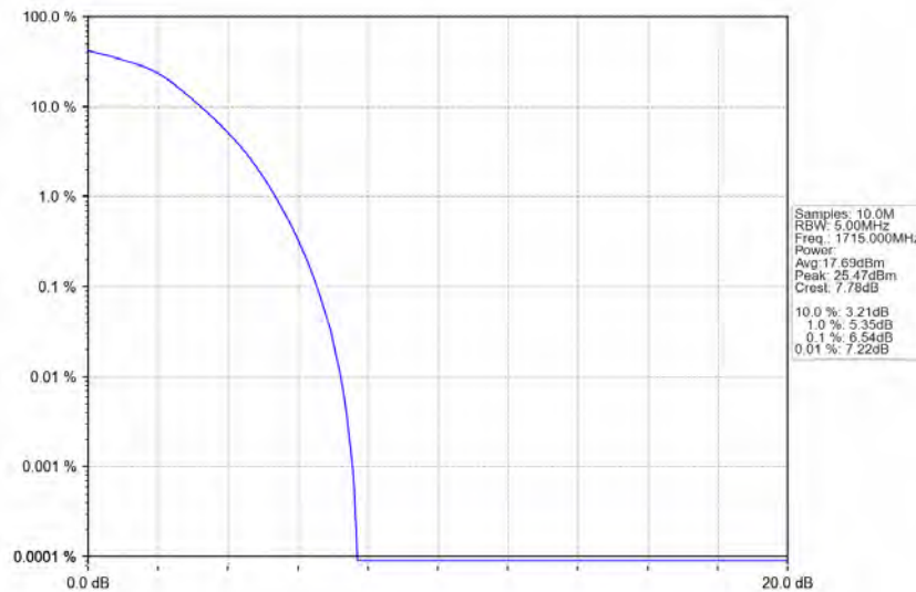
Band4_10MHz_16QAM_LCH_1715MHz_RB_50_0_NTNV
