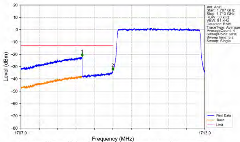
Band4_3MHz_16QAM_LCH_1711.5MHz_RB_15_0_NTNV
