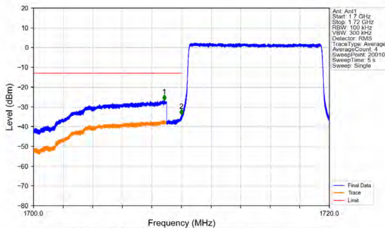
Band4_10MHz_QPSK_LCH_1715MHz_RB_50_0_NTNV
