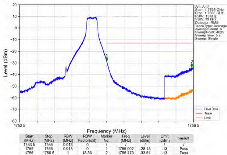
Band4_1.4MHz_64QAM_HCH_1754.3MHz_RB_1_5_NTNV
