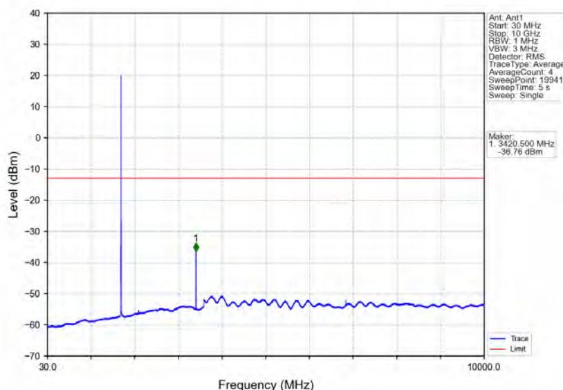
Band4_3MHz_16QAM_LCH_1711.5MHz_RB_1_0_NTNV
