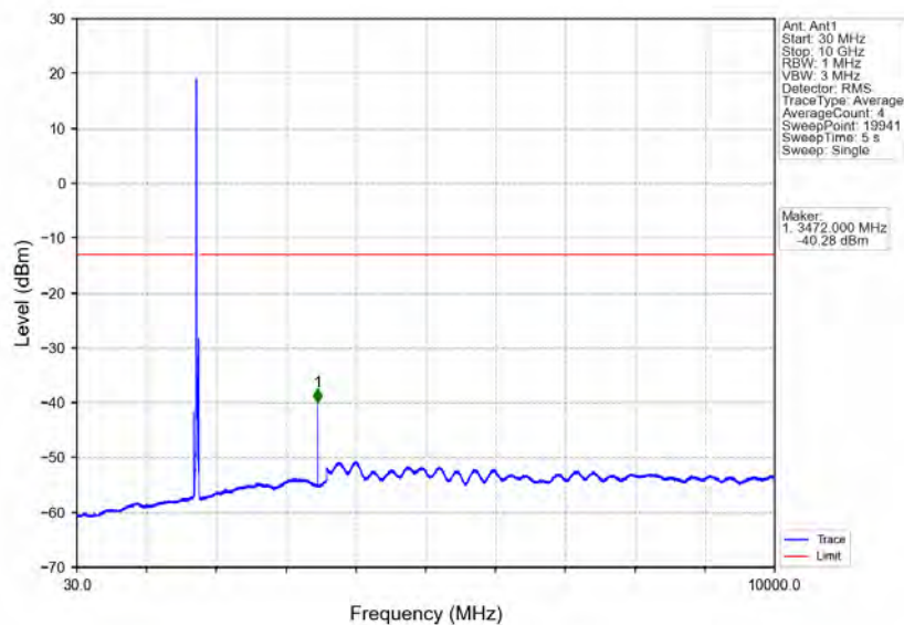
Band4_20MHz_64QAM_HCH_1745MHz_RB_1_0_NTNV
