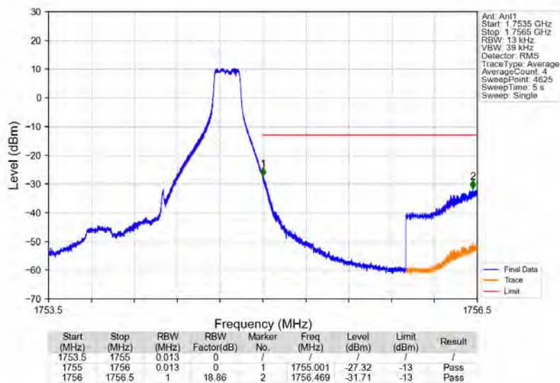
Band4_1.4MHz_16QAM_HCH_1754.3MHz_RB_1_5_NTNV
