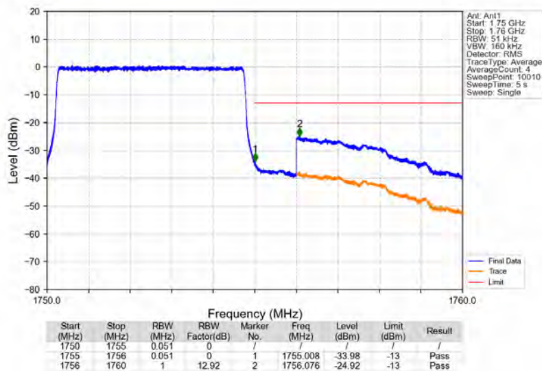
Band4_5MHz_64QAM_HCH_1752.5MHz_RB_25_0_NTNV
