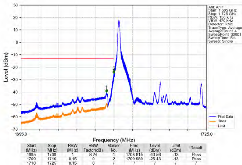
Band4_15MHz_64QAM_LCH_1717.5MHz_RB_1_0_NTNV
