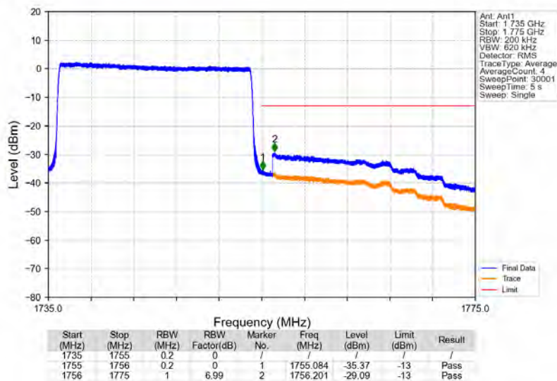
Band4_20MHz_16QAM_HCH_1745MHz_RB_100_0_NTNV
