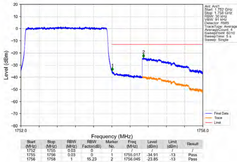
Band4_3MHz_16QAM_HCH_1753.5MHz_RB_15_0_NTNV
