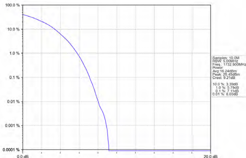
Band4_15MHz_16QAM_MCH_1732.5MHz_RB_75_0_NTNV
