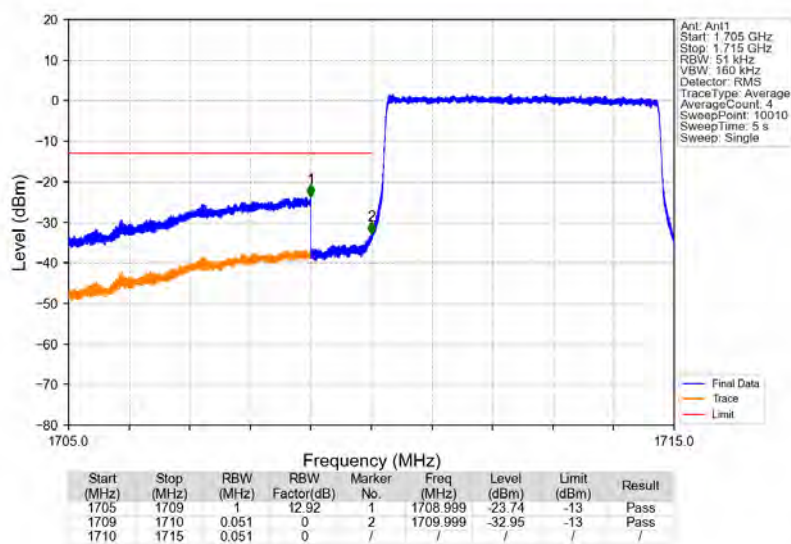
Band4_5MHz_16QAM_LCH_1712.5MHz_RB_25_0_NTNV
