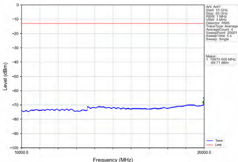
Band4_5MHz_64QAM_MCH_1732.5MHz_RB_1_0_NTNV
