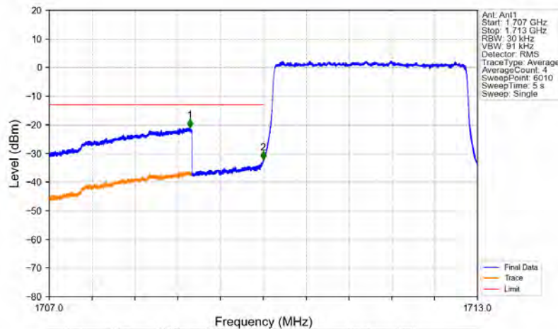
Band4_3MHz_QPSK_LCH_1711.5MHz_RB_15_0_NTNV
