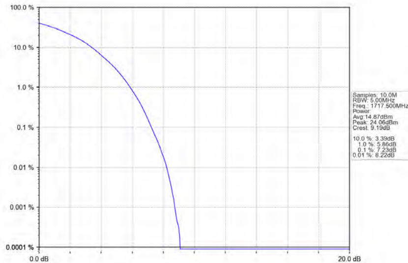
Band4_15MHz_64QAM_LCH_1717.5MHz_RB_75_0_NTNV
