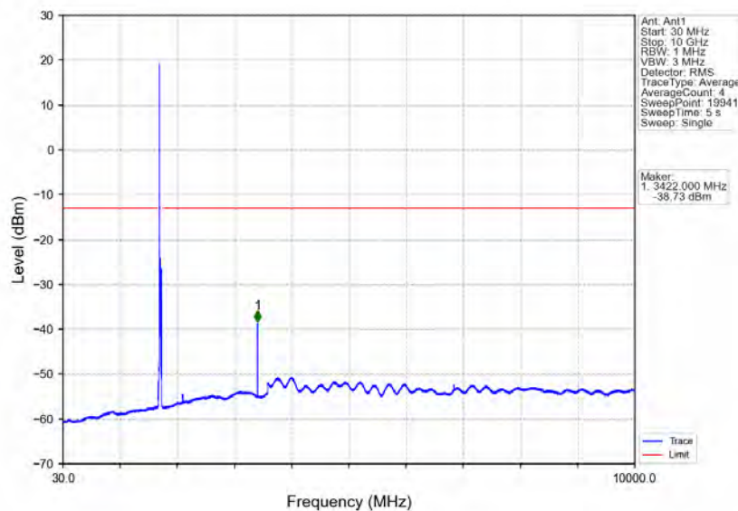
Band4_20MHz_64QAM_LCH_1720MHz_RB_1_0_NTNV
