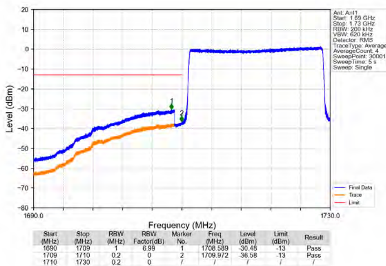
Band4_20MHz_64QAM_LCH_1720MHz_RB_100_0_NTNV
