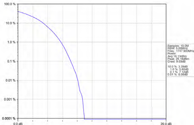
Band4_15MHz_16QAM_HCH_1747.5MHz_RB_75_0_NTNV
