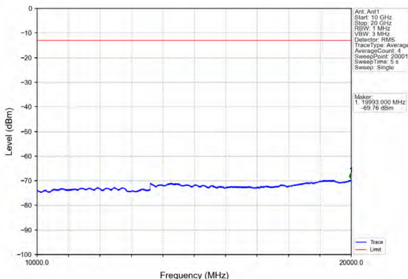
Band4_15MHz_QPSK_HCH_1747.5MHz_RB_1_0_NTNV
