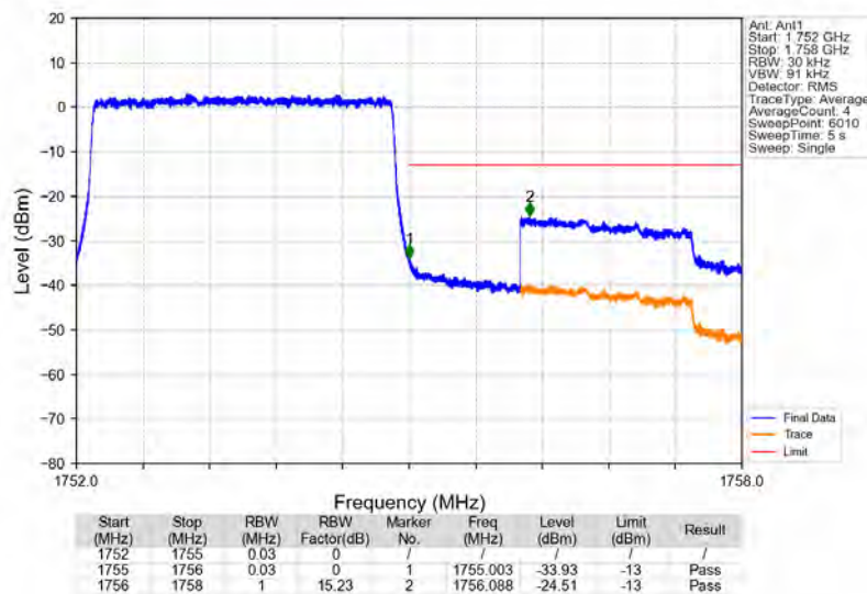
Band4_3MHz_QPSK_HCH_1753.5MHz_RB_15_0_NTNV
