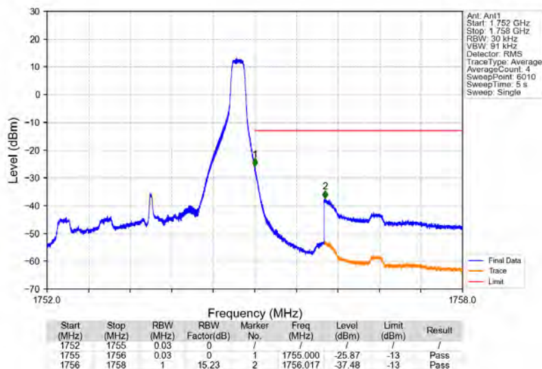
Band4_3MHz_64QAM_HCH_1753.5MHz_RB_1_14_NTNV
