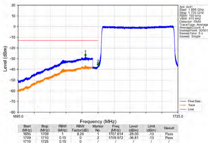
Band4_15MHz_64QAM_LCH_1717.5MHz_RB_75_0_NTNV
