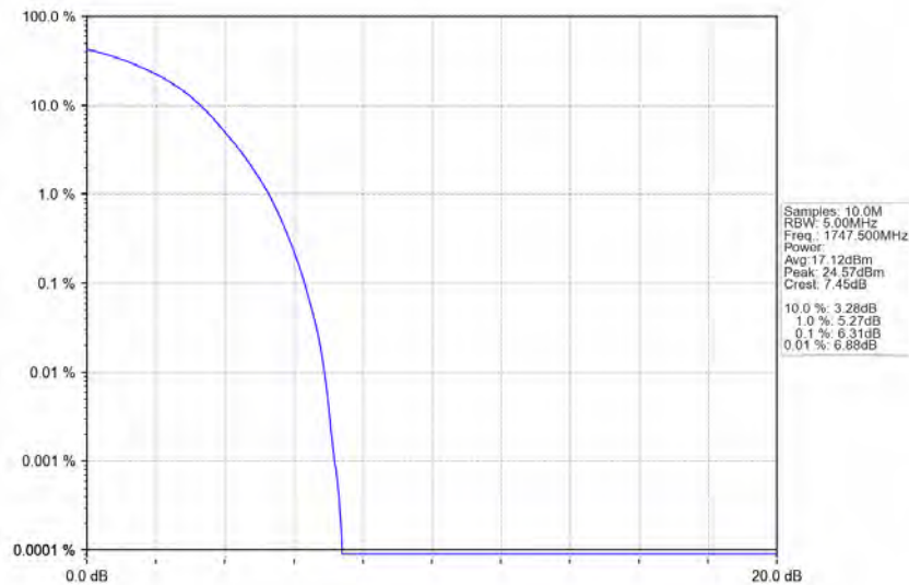
Band4_15MHz_QPSK_HCH_1747.5MHz_RB_75_0_NTNV
