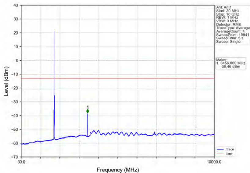
Band4_10MHz_QPSK_MCH_1732.5MHz_RB_1_0_NTNV
