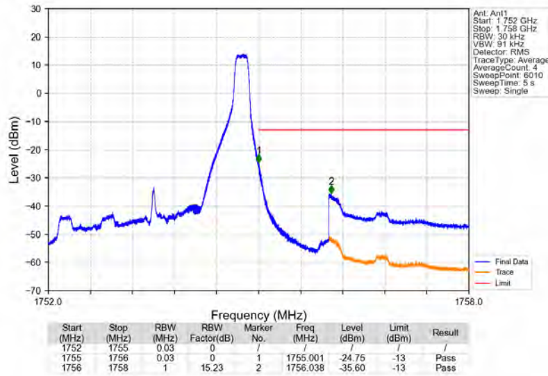
Band4_3MHz_16QAM_HCH_1753.5MHz_RB_1_14_NTNV
