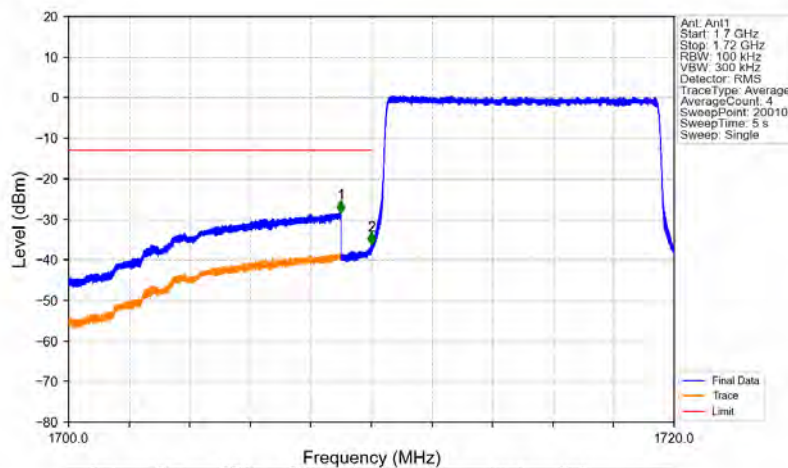
Band4_10MHz_64QAM_LCH_1715MHz_RB_50_0_NTNV
