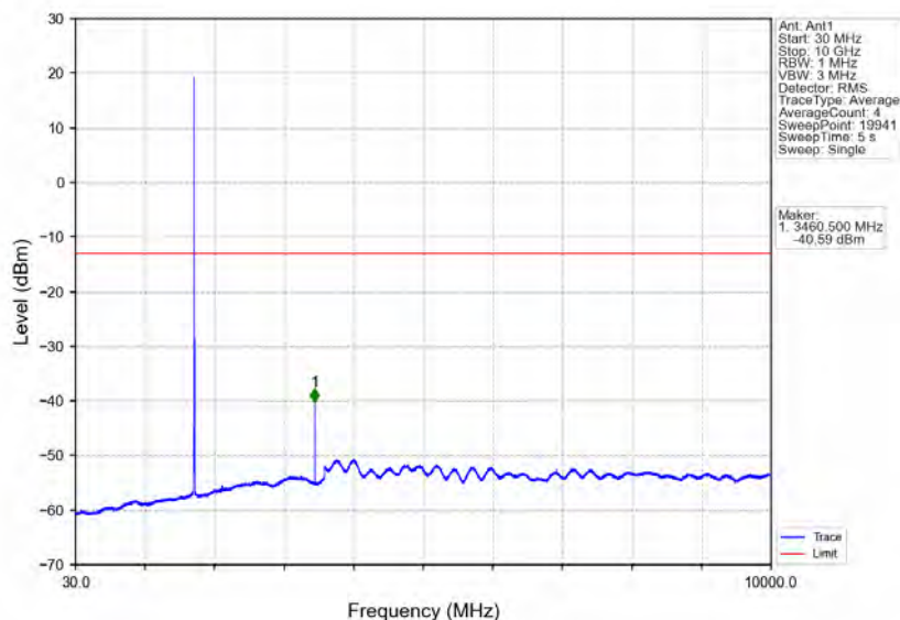
Band4_5MHz_64QAM_MCH_1732.5MHz_RB_1_0_NTNV
