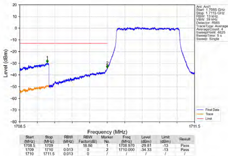
Band4_1.4MHz_64QAM_LCH_1710.7MHz_RB_6_0_NTNV
