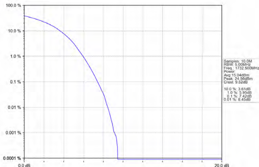
Band4_20MHz_16QAM_MCH_1732.5MHz_RB_100_0_NTNV
