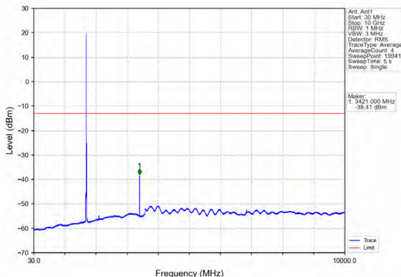
Band4_10MHz_64QAM_LCH_1715MHz_RB_1_0_NTNV
