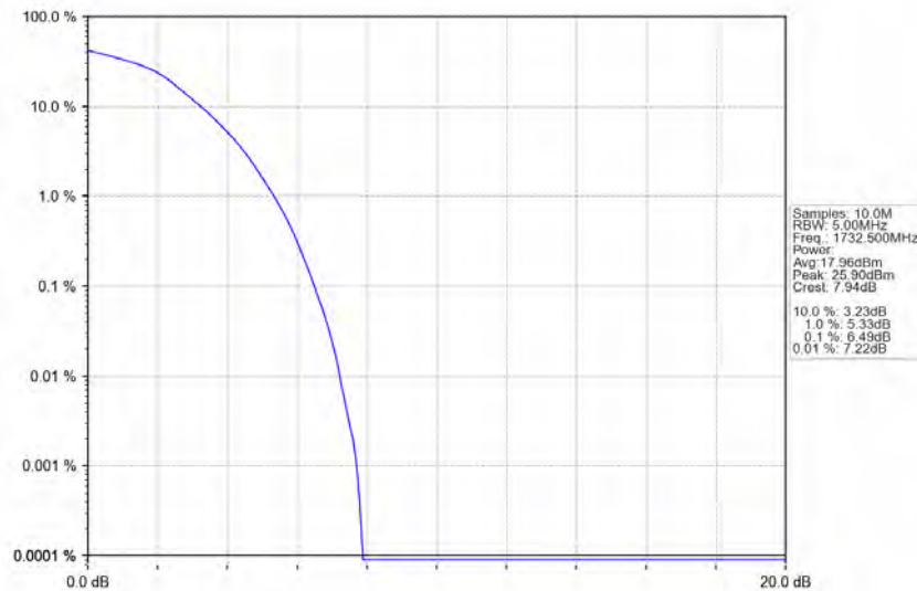
Band4_10MHz_16QAM_MCH_1732.5MHz_RB_50_0_NTNV
