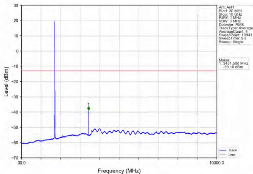
Band4_15MHz_64QAM_MCH_1732.5MHz_RB_1_0_NTNV
