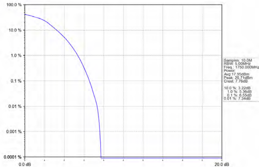
Band4_10MHz_16QAM_HCH_1750MHz_RB_50_0_NTNV
