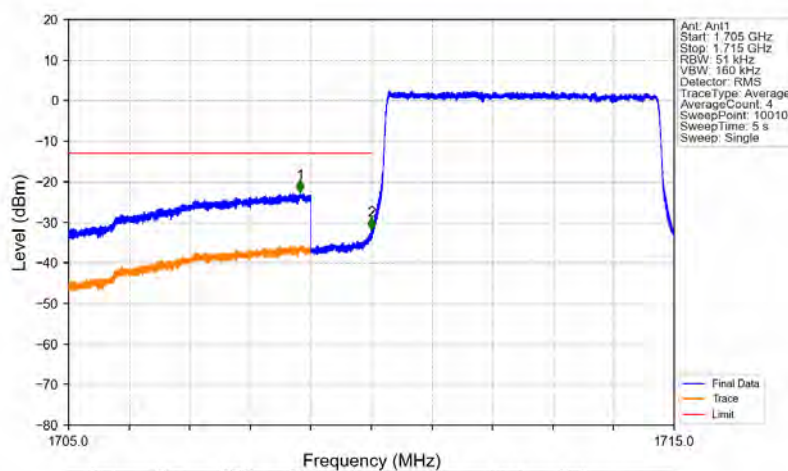
Band4_5MHz_QPSK_LCH_1712.5MHz_RB_25_0_NTNV
