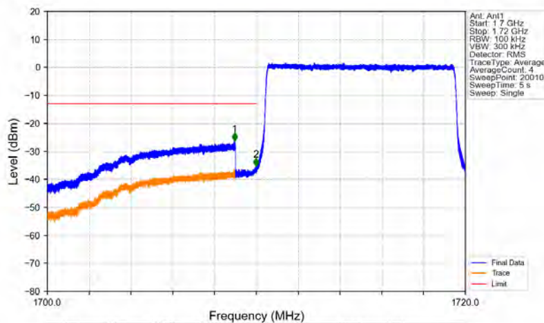
Band4_10MHz_16QAM_LCH_1715MHz_RB_50_0_NTNV
