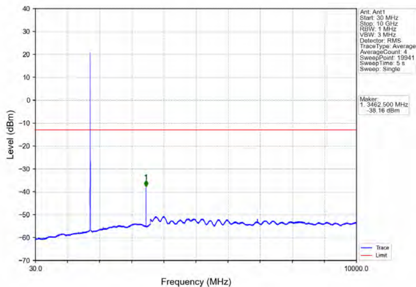
Band4_3MHz_QPSK_MCH_1732.5MHz_RB_1_0_NTNV
