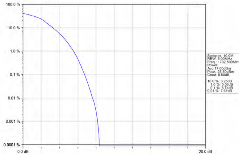
Band4_10MHz_64QAM_MCH_1732.5MHz_RB_50_0_NTNV
