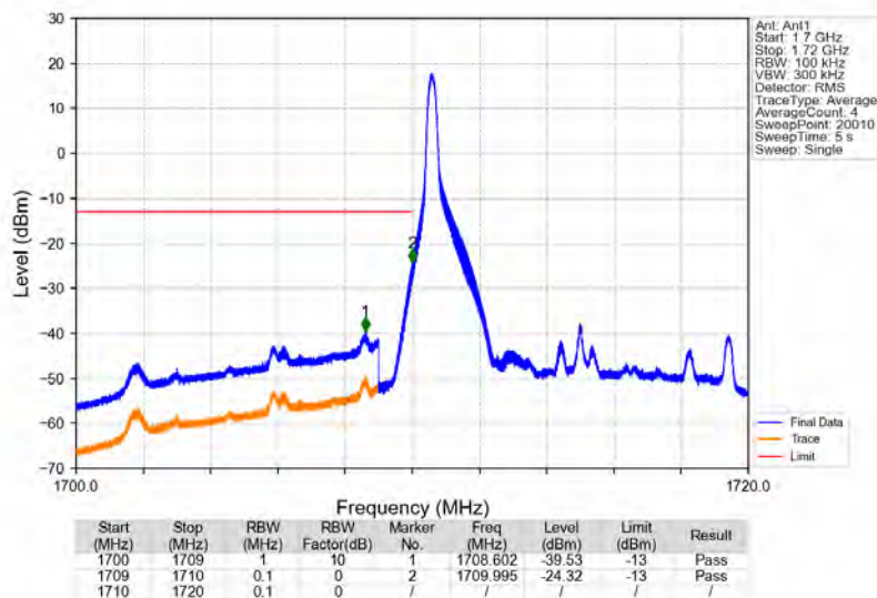
Band4_10MHz_64QAM_LCH_1715MHz_RB_1_0_NTNV
