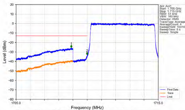
Band4_5MHz_64QAM_LCH_1712.5MHz_RB_25_0_NTNV
