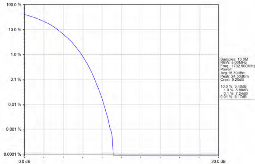
Band4_15MHz_64QAM_MCH_1732.5MHz_RB_75_0_NTNV
