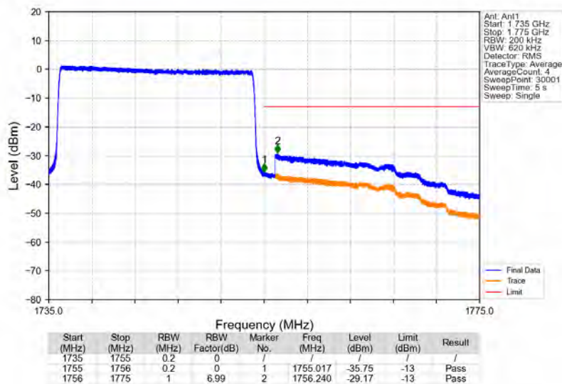
Band4_20MHz_64QAM_HCH_1745MHz_RB_100_0_NTNV
