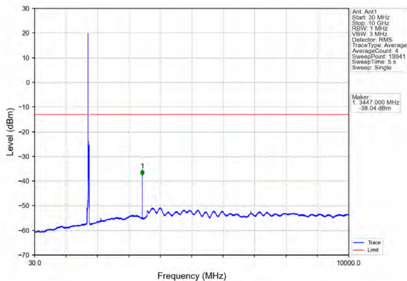
Band4_20MHz_16QAM_MCH_1732.5MHz_RB_1_0_NTNV
