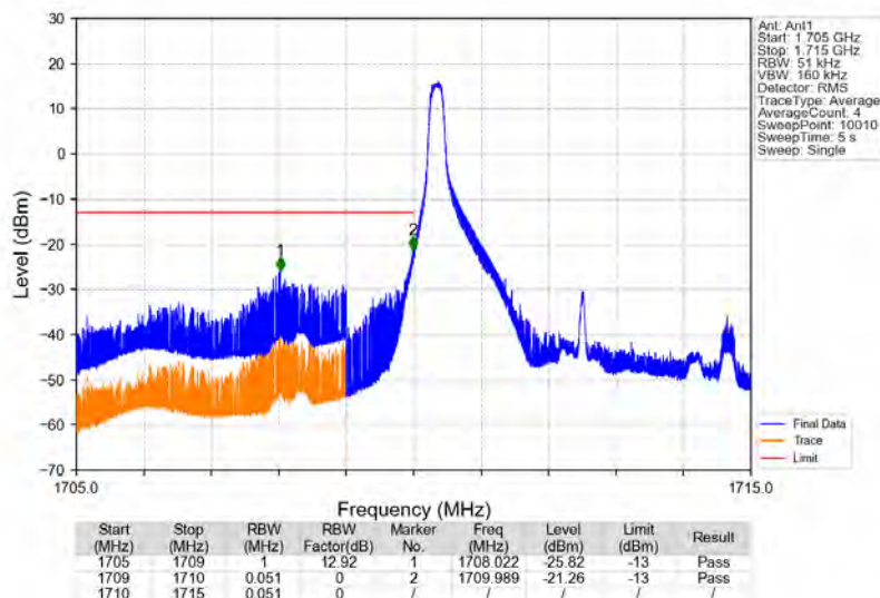
Band4_5MHz_16QAM_LCH_1712.5MHz_RB_1_0_NTNV
