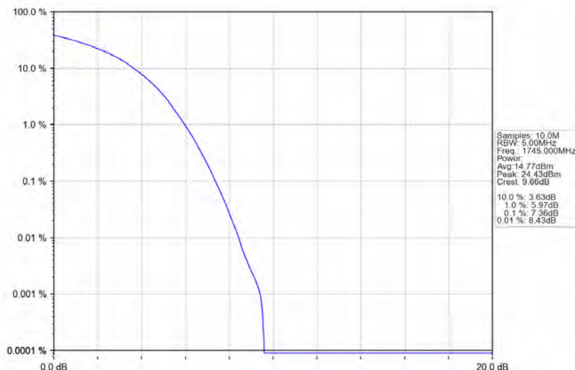
Band4_20MHz_16QAM_HCH_1745MHz_RB_100_0_NTNV
