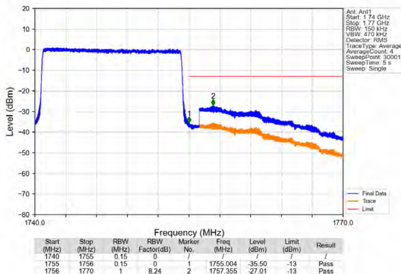
Band4_15MHz_64QAM_HCH_1747.5MHz_RB_75_0_NTNV
