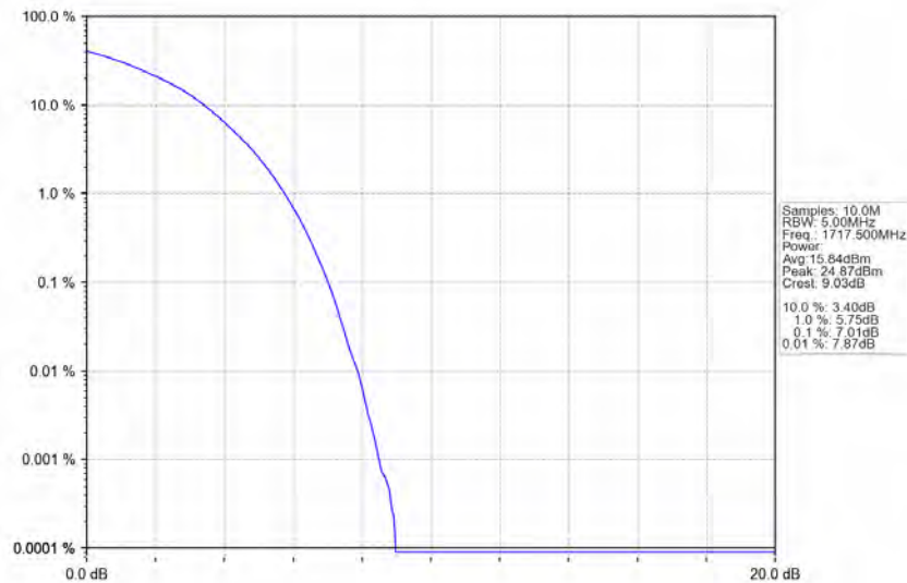
Band4_15MHz_16QAM_LCH_1717.5MHz_RB_75_0_NTNV
