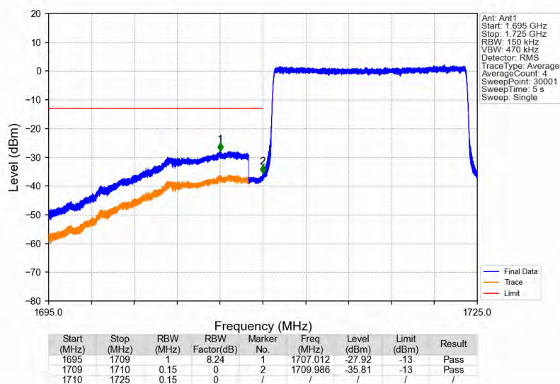
Band4_15MHz_16QAM_LCH_1717.5MHz_RB_75_0_NTNV
