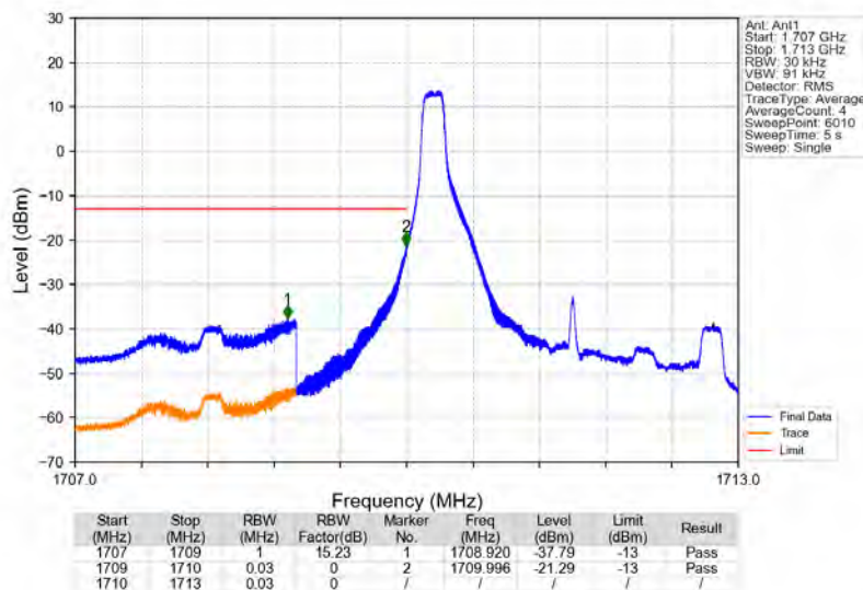
Band4_3MHz_16QAM_LCH_1711.5MHz_RB_1_0_NTNV
