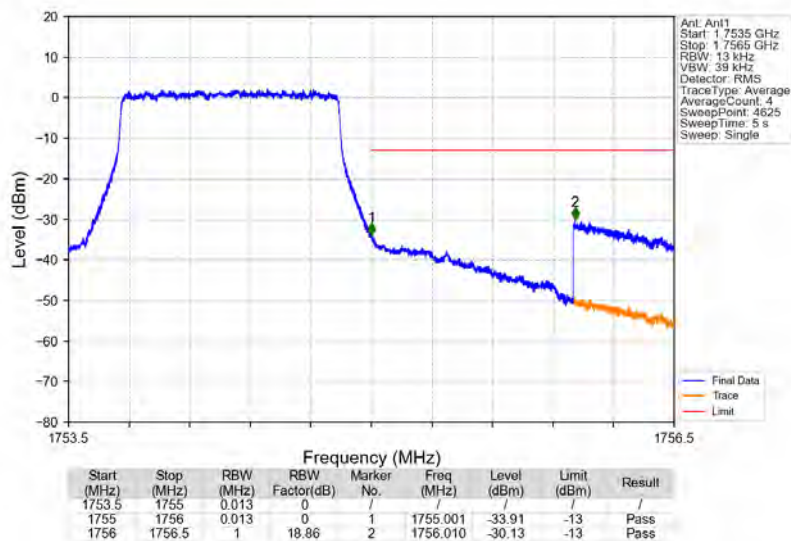
Band4_1.4MHz_16QAM_HCH_1754.3MHz_RB_6_0_NTNV
