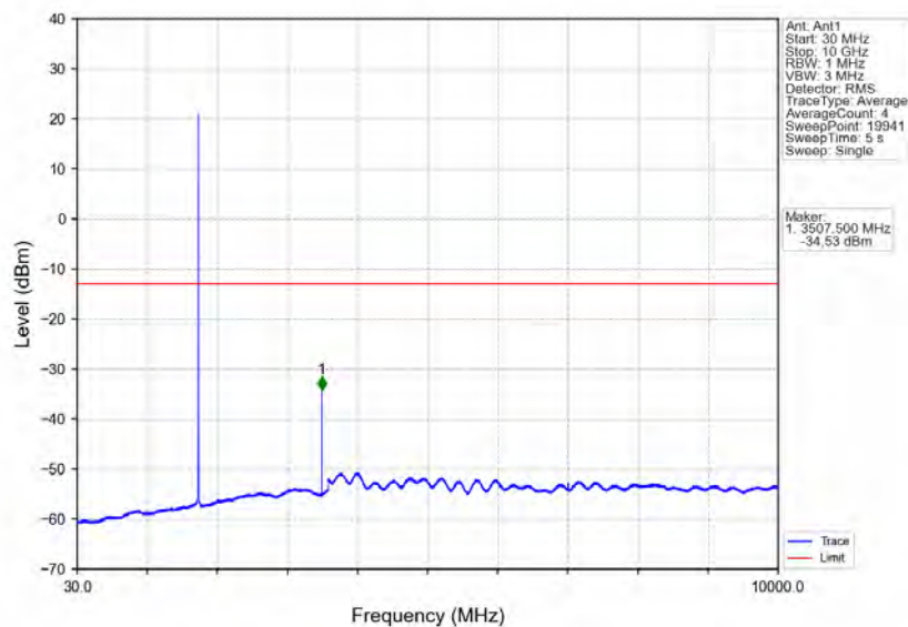
Band4_1.4MHz_QPSK_HCH_1754.3MHz_RB_1_0_NTNV
