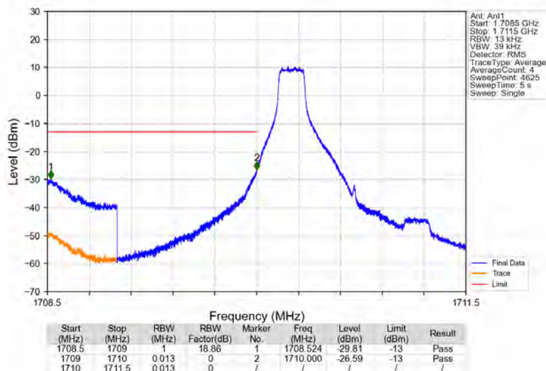
Band4_1.4MHz_16QAM_LCH_1710.7MHz_RB_1_0_NTNV
