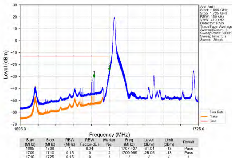
Band4_15MHz_16QAM_LCH_1717.5MHz_RB_1_0_NTNV
