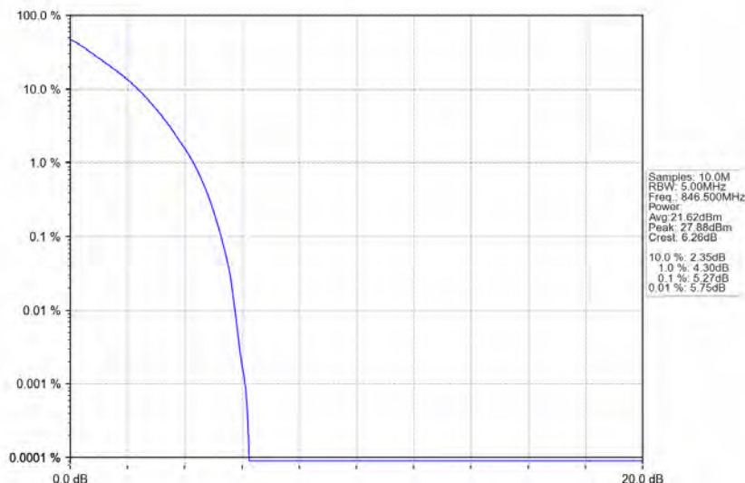
Band5_5MHz_QPSK_HCH_846.5MHz_RB_25_0_NTNV
