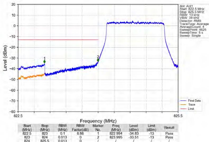
Band5_1.4MHz_QPSK_LCH_824.7MHz_RB_6_0_NTNV
