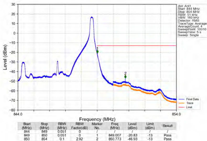
Band5_5MHz_16QAM_HCH_846.5MHz_RB_1_24_NTNV
