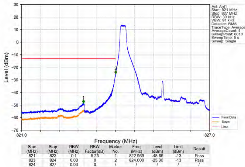
Band5_3MHz_64QAM_LCH_825.5MHz_RB_1_0_NTNV
