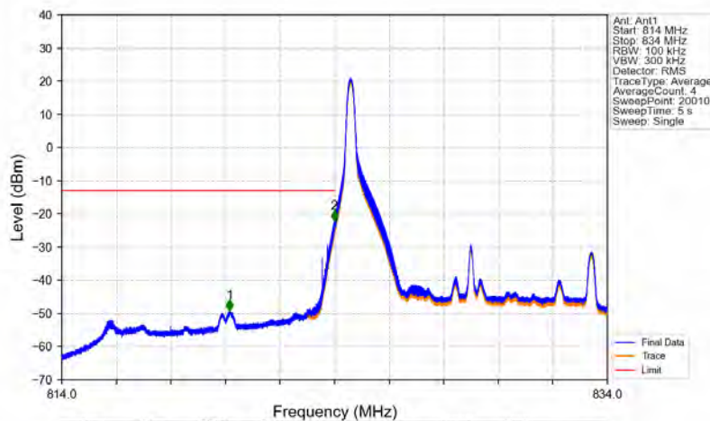
Band5_10MHz_16QAM_LCH_829MHz_RB_1_0_NTNV
