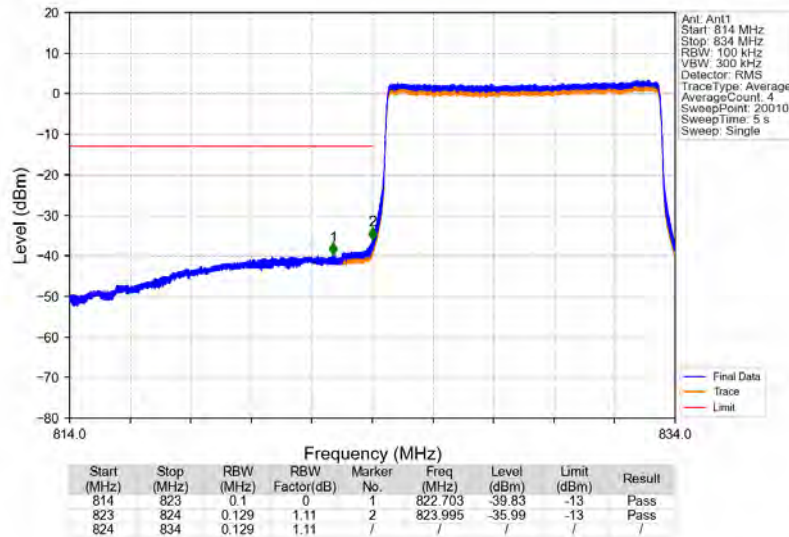
Band5_10MHz_64QAM_LCH_829MHz_RB_50_0_NTNV
