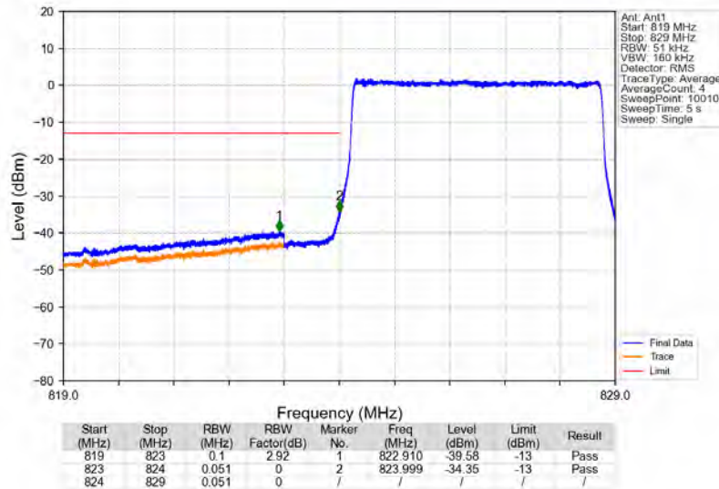
Band5_5MHz_64QAM_LCH_826.5MHz_RB_25_0_NTNV
