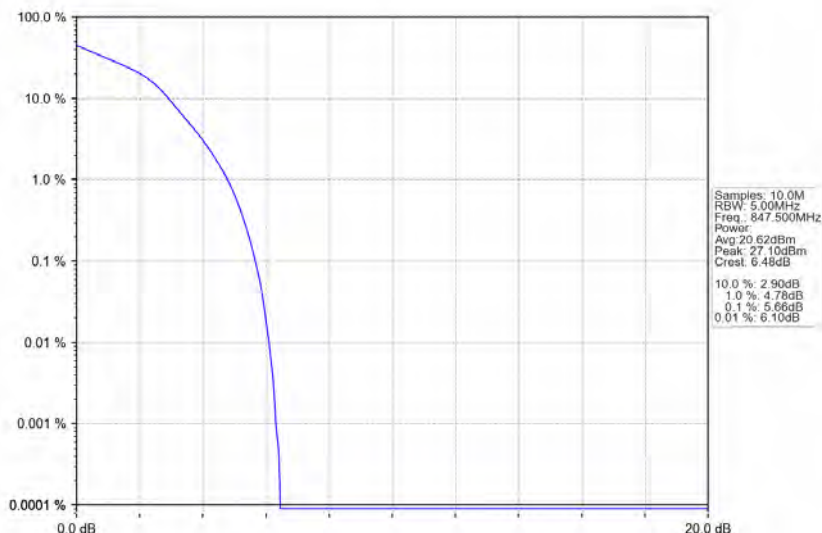
Band5_3MHz_16QAM_HCH_847.5MHz_RB_15_0_NTNV
