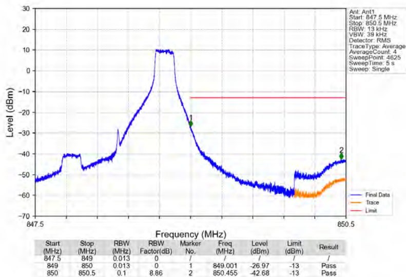
Band5_1.4MHz_64QAM_HCH_848.3MHz_RB_1_5_NTNV
