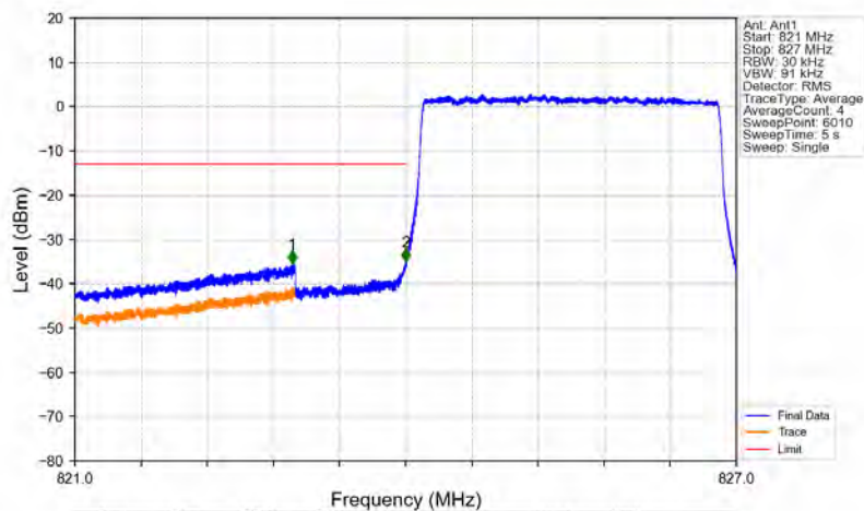
Band5_3MHz_16QAM_LCH_825.5MHz_RB_15_0_NTNV
