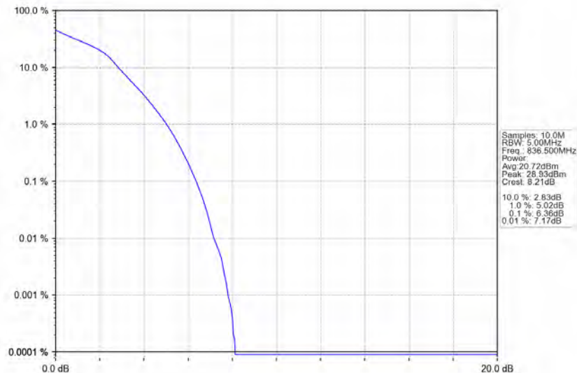
Band5_5MHz_16QAM_MCH_836.5MHz_RB_25_0_NTNV
