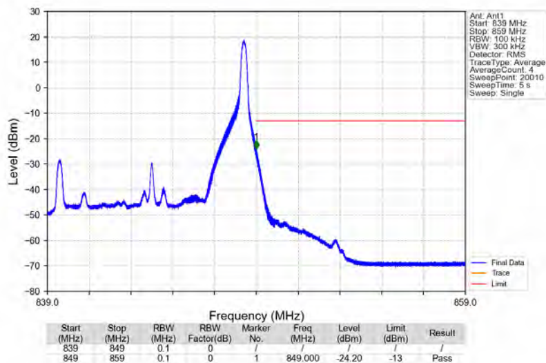
Band5_10MHz_64QAM_HCH_844MHz_RB_1_49_NTNV
