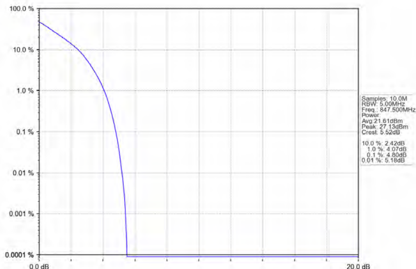
Band5_3MHz_QPSK_HCH_847.5MHz_RB_15_0_NTNV
