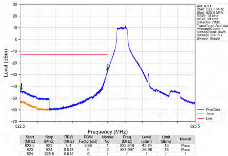
Band5 1.4MHz 64QAM LCH 824.7MHz_RB_1_0_NTNV
