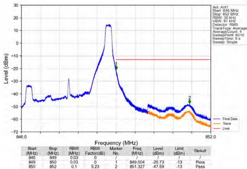
Band5_3MHz_16QAM_HCH_847.5MHz_RB_1_14_NTNV
