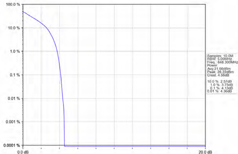
Band5_1.4MHz_QPSK_HCH_848.3MHz_RB_6_0_NTNV
