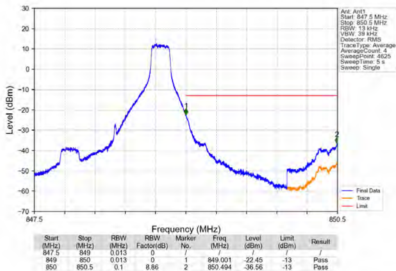
Band5_1.4MHz_QPSK_HCH_848.3MHz_RB_1_5_NTNV
