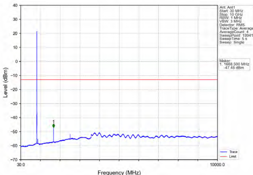
Band5_5MHz_16QAM_HCH_846.5MHz_RB_1_0_NTNV
