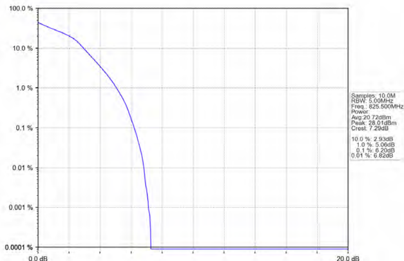
Band5_3MHz_16QAM_LCH_825.5MHz_RB_15_0_NTNV
