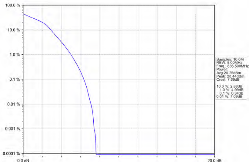
Band5_3MHz_16QAM_MCH_836.5MHz_RB_15_0_NTNV
