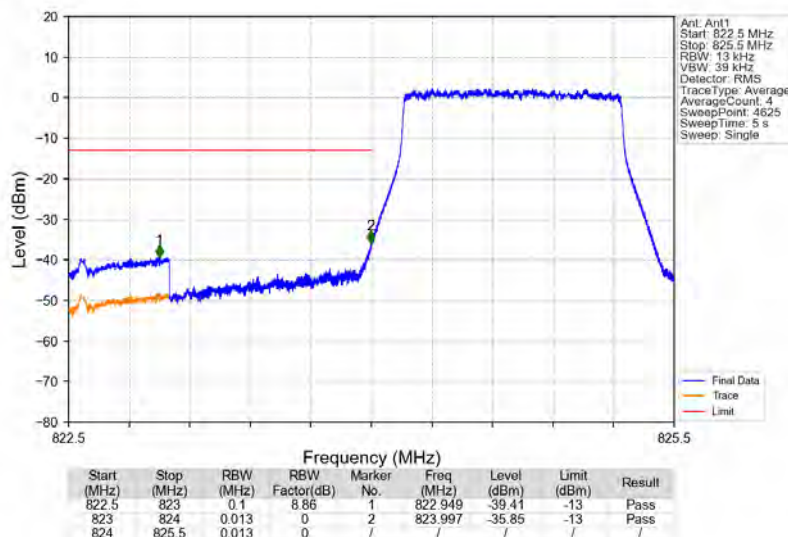
Band5_1.4MHz_64QAM_LCH_824.7MHz_RB_6_0_NTNV
