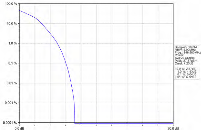
Band5_5MHz_16QAM_HCH_846.5MHz_RB_25_0_NTNV
