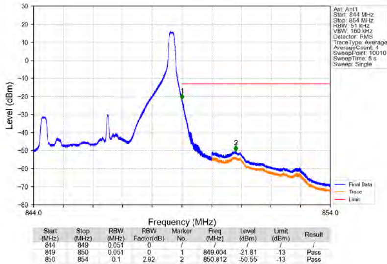
Band5_5MHz_64QAM_HCH_846.5MHz_RB_1_24_NTNV
