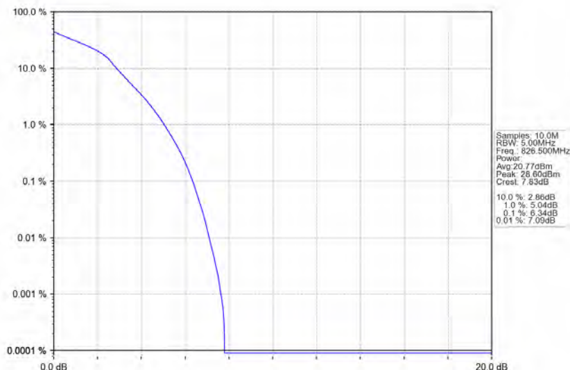
Band5_5MHz_16QAM_LCH_826.5MHz_RB_25_0_NTNV
