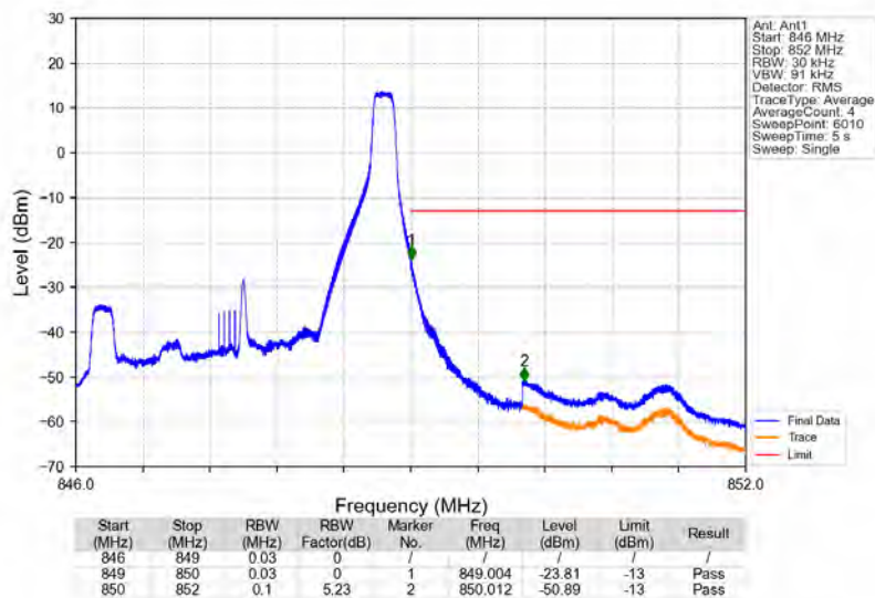
Band5_3MHz_64QAM_HCH_847.5MHz_RB_1_14_NTNV
