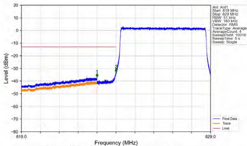
Band5_5MHz_16QAM_LCH_826.5MHz_RB_25_0_NTNV
