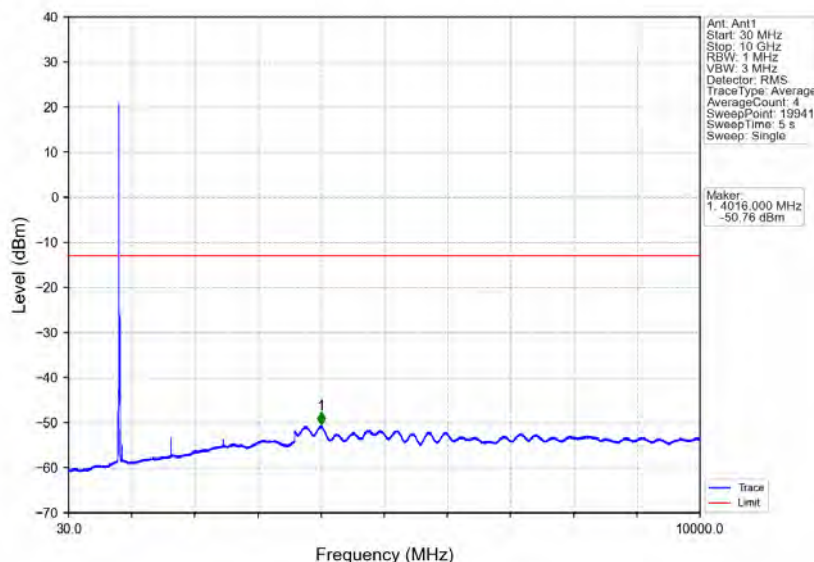
Band5_10MHz_64QAM_LCH_829MHz_RB_1_0_NTNV
