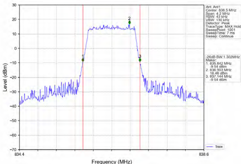
Band5_1.4MHz_64QAM_MCH_836.5MHz_RB_6_0_NTNV
