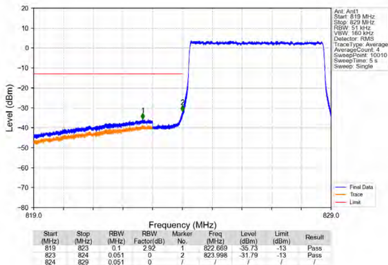
Band5_5MHz_QPSK_LCH_826.5MHz_RB_25_0_NTNV
