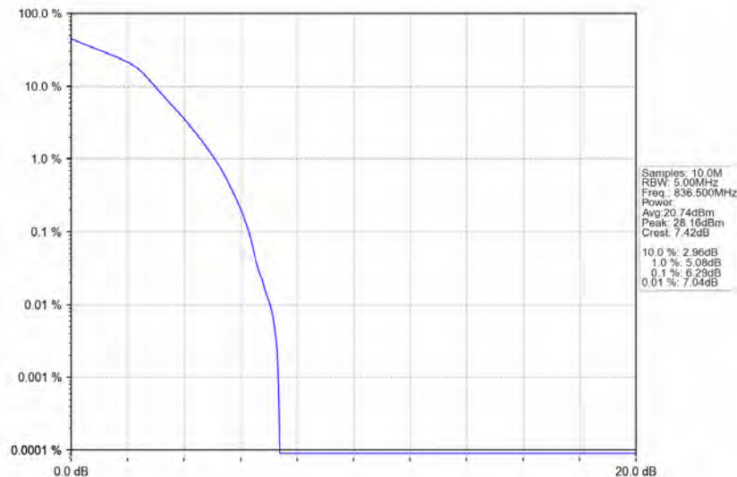
Band5_1.4MHz_16QAM_MCH_836.5MHz_RB_6_0_NTNV
