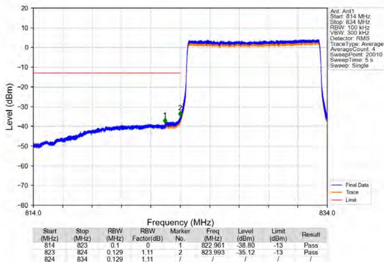
Band5_10MHz_16QAM_LCH_829MHz_RB_50_0_NTNV
