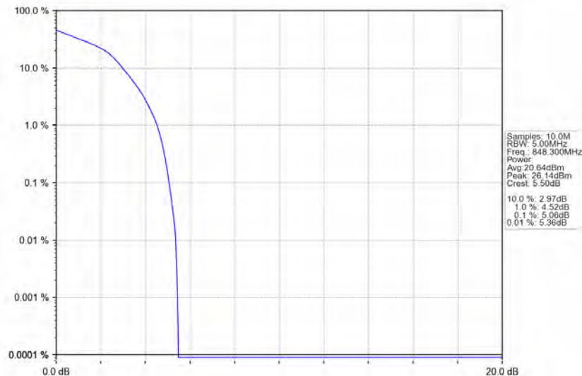
Band5_1.4MHz_16QAM_HCH_848.3MHz_RB_6_0_NTNV
