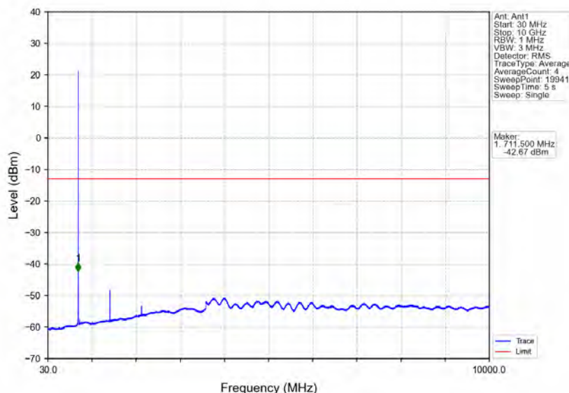
Band12_1.4MHz_16QAM_HCH_715.3MHz_RB_1_0_NTNV
