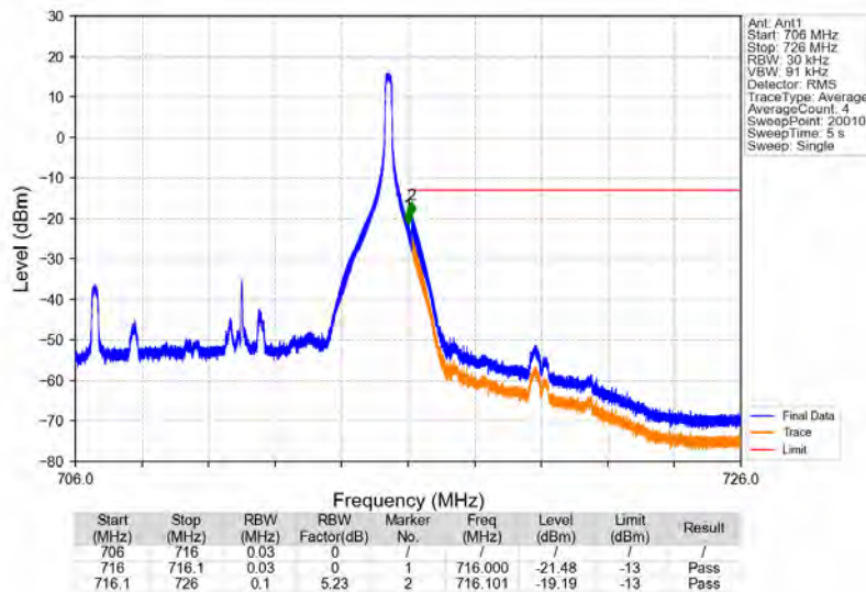
Band12_10MHz_QPSK_HCH_711MHz_RB_1_49_NTNV
