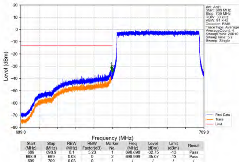
Band12_10MHz_QPSK_LCH_704MHz_RB_50_0_NTNV
