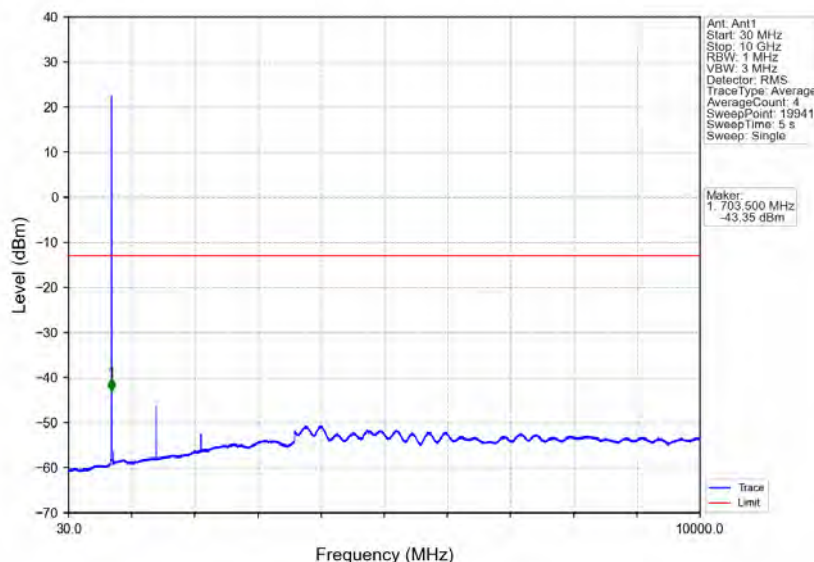
Band12_1.4MHz_QPSK_MCH_707.5MHz_RB_1_0_NTNV
