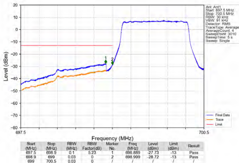
Band12_1.4MHz_QPSK_LCH_699.7MHz_RB_6_0_NTNV
