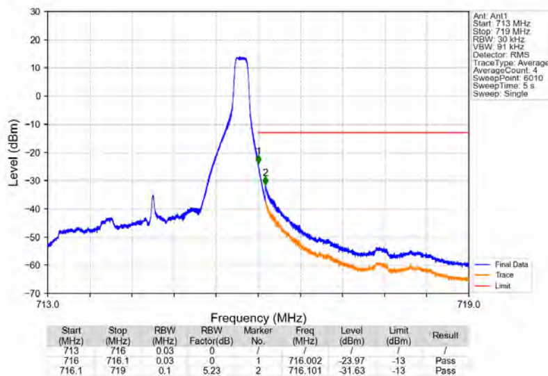
Band12_3MHz_64QAM_HCH_714.5MHz_RB_1_14_NTNV
