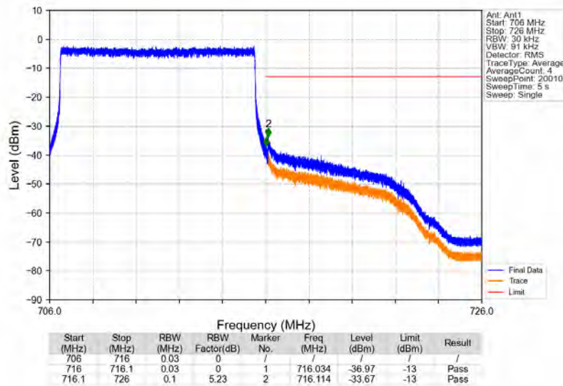
Band12_10MHz_64QAM_HCH_711MHz_RB_50_0_NTNV
