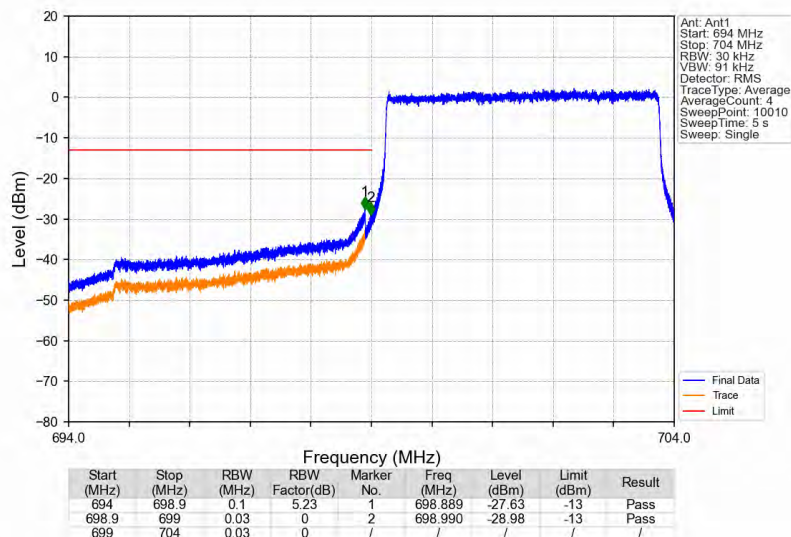
Band12_5MHz_QPSK_LCH_701.5MHz_RB_25_0_NTNV
