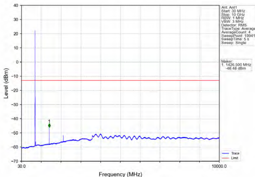
Band12_3MHz_QPSK_HCH_714.5MHz_RB_1_14_NTNV
