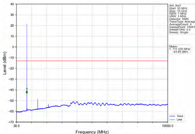
Band12_1.4MHz_64QAM_HCH_715.3MHz_RB_1_5_NTNV
