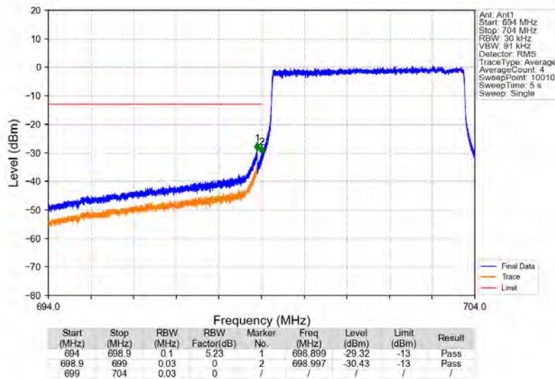
Band12_5MHz_64QAM_LCH_701.5MHz_RB_25_0_NTNV
