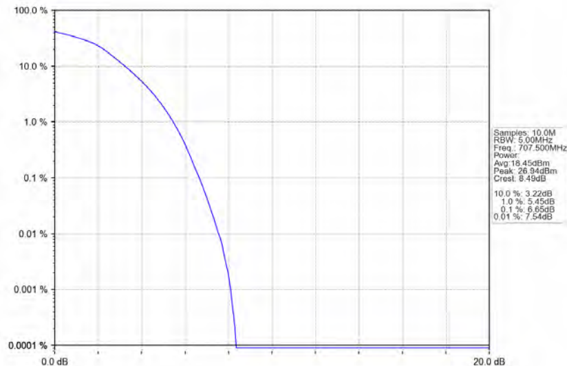
Band12_10MHz_64QAM_MCH_707.5MHz_RB_50_0_NTNV
