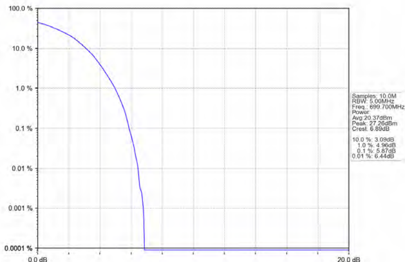
Band12_1.4MHz_64QAM_LCH_699.7MHz_RB_6_0_NTNV
