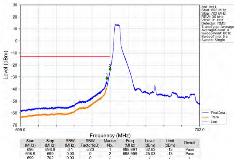
Band12_3MHz_64QAM_LCH_700.5MHz_RB_1_0_NTNV
