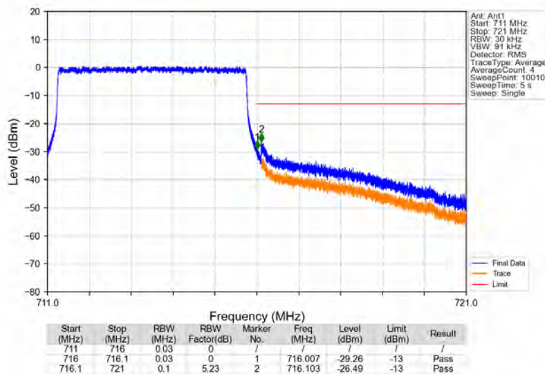
Band12_5MHz_16QAM_HCH_713.5MHz_RB_25_0_NTNV
