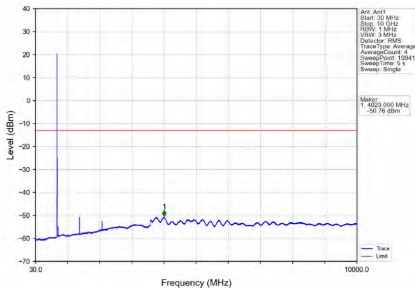
Band12_5MHz_64QAM_LCH_701.5MHz_RB_1_0_NTNV
