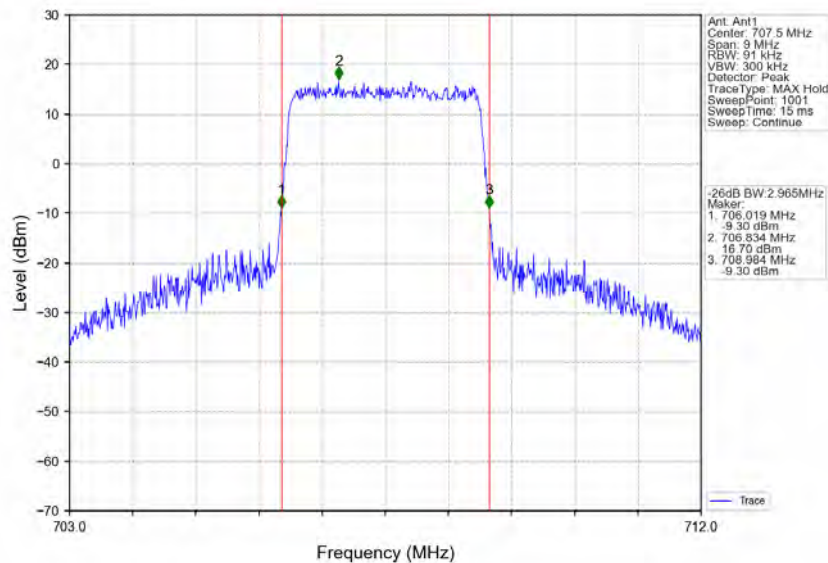
Band12_3MHz_16QAM_MCH_707.5MHz_RB_15_0_NTNV
