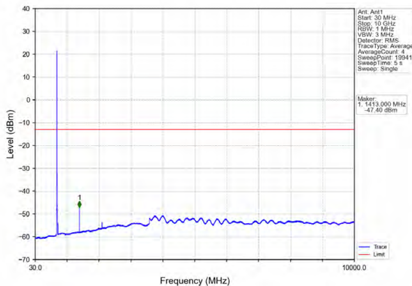
Band12_10MHz_16QAM_HCH_711MHz_RB_1_0_NTNV
