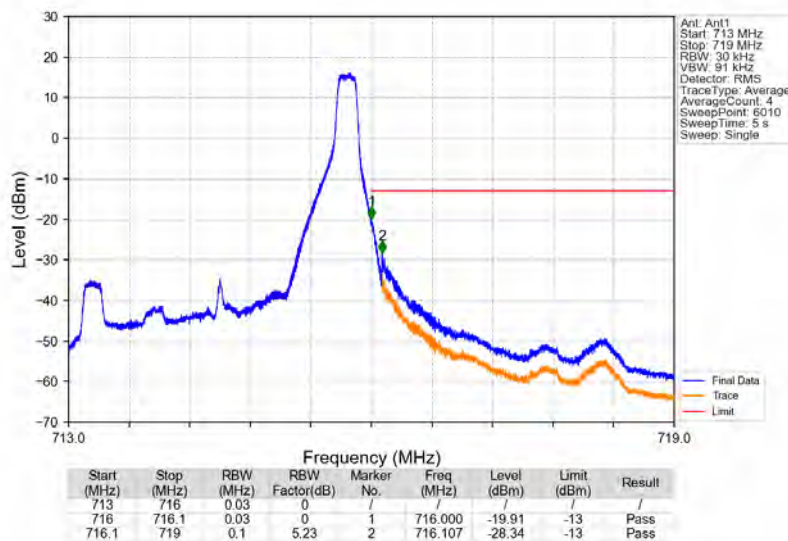
Band12_3MHz_QPSK_HCH_714.5MHz_RB_1_14_NTNV
