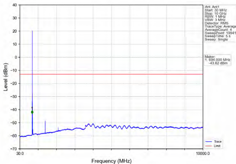
Band12_5MHz_64QAM_MCH_707.5MHz_RB_1_0_NTNV
