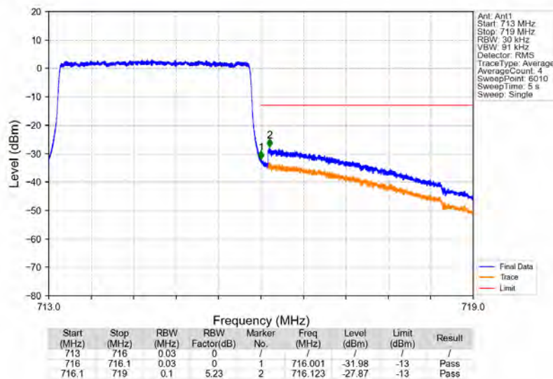
Band12_3MHz_16QAM_HCH_714.5MHz_RB_15_0_NTNV
