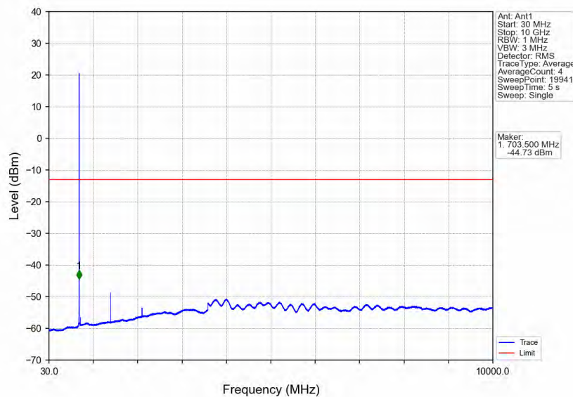
Band12_1.4MHz_64QAM_MCH_707.5MHz_RB_1_0_NTNV
