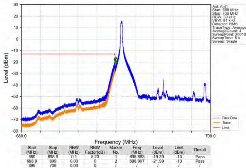
Band12_10MHz_16QAM_LCH_704MHz_RB_1_0_NTNV
