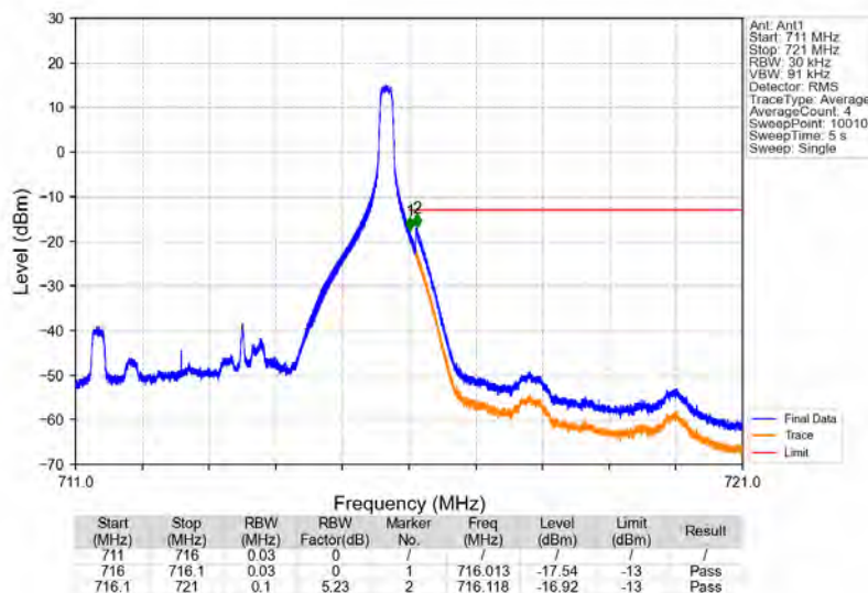
Band12_5MHz_16QAM_HCH_713.5MHz_RB_1_24_NTNV
