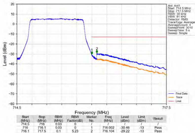
Band12_1.4MHz_64QAM_HCH_715.3MHz_RB_6_0_NTNV
