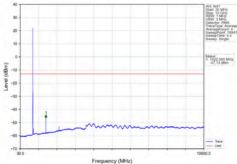
Band12_5MHz_QPSK_HCH_713.5MHz_RB_1_24_NTNV
