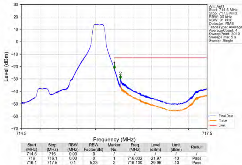
Band12_1.4MHz_16QAM_HCH_715.3MHz_RB_1_5_NTNV
