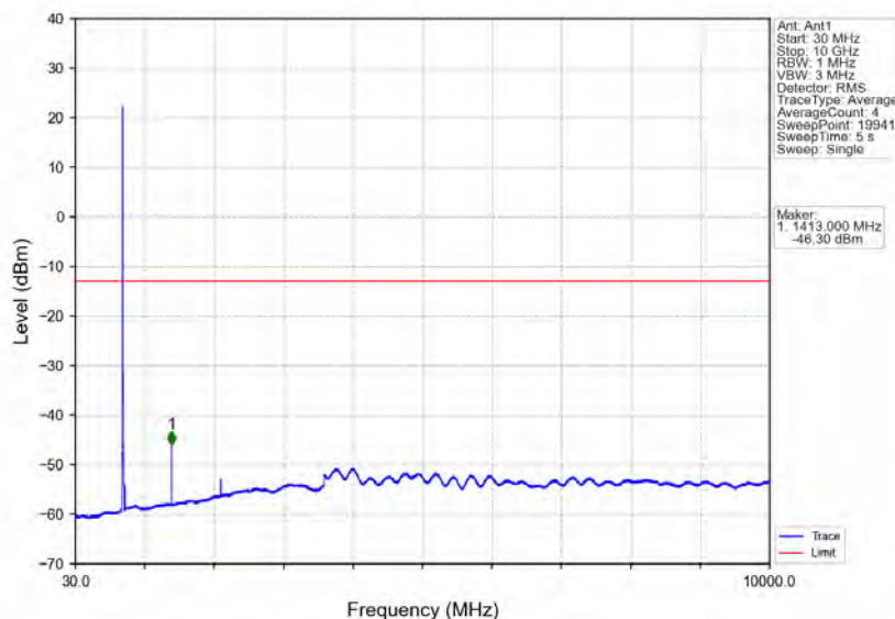
Band12_10MHz_QPSK_HCH_711MHz_RB_1_49_NTNV
