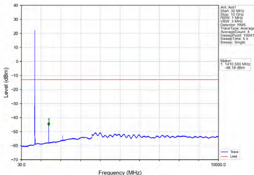
Band12_5MHz_QPSK_MCH_707.5MHz_RB_1_0_NTNV
