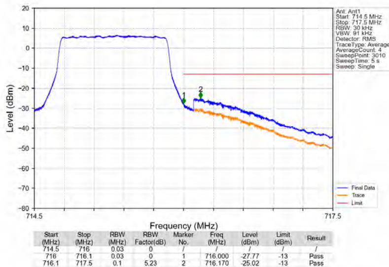
Band12_1.4MHz_16QAM_HCH_715.3MHz_RB_6_0_NTNV
