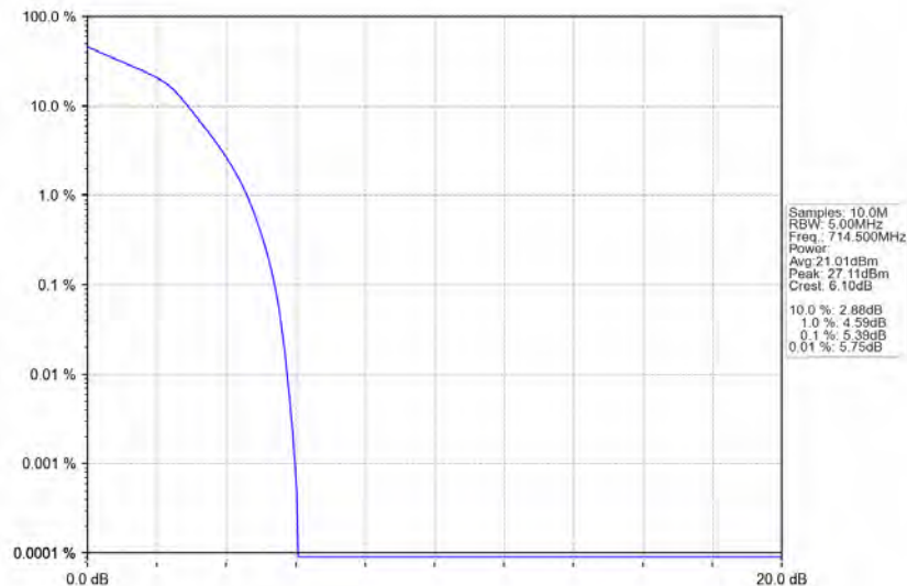
Band12_3MHz_16QAM_HCH_714.5MHz_RB_15_0_NTNV
