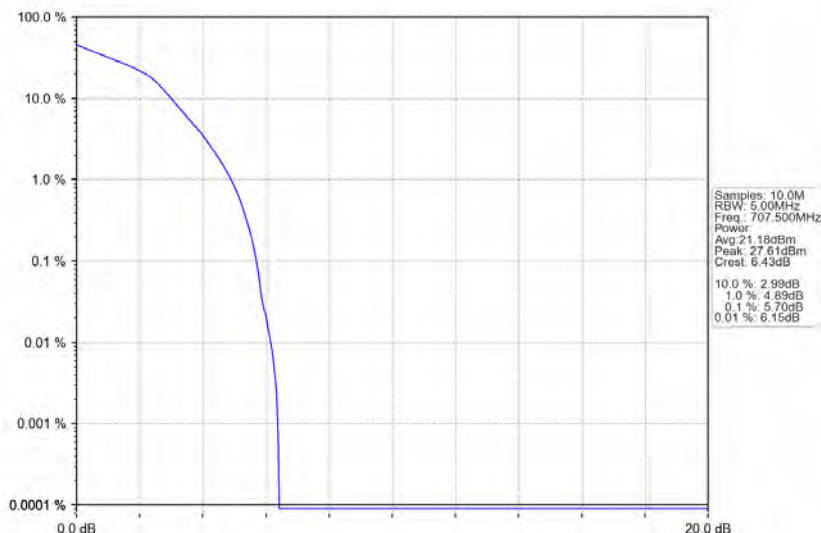
Band12_1.4MHz_16QAM_MCH_707.5MHz_RB_6_0_NTNV
