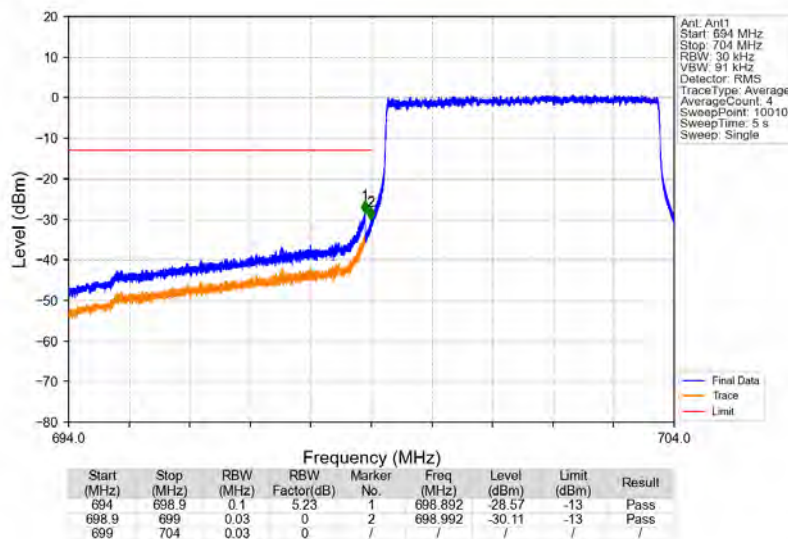
Band12_5MHz_16QAM_LCH_701.5MHz_RB_25_0_NTNV
