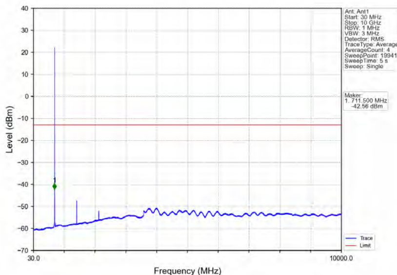
Band12_1.4MHz_QPSK_HCH_715.3MHz_RB_1_5_NTNV
