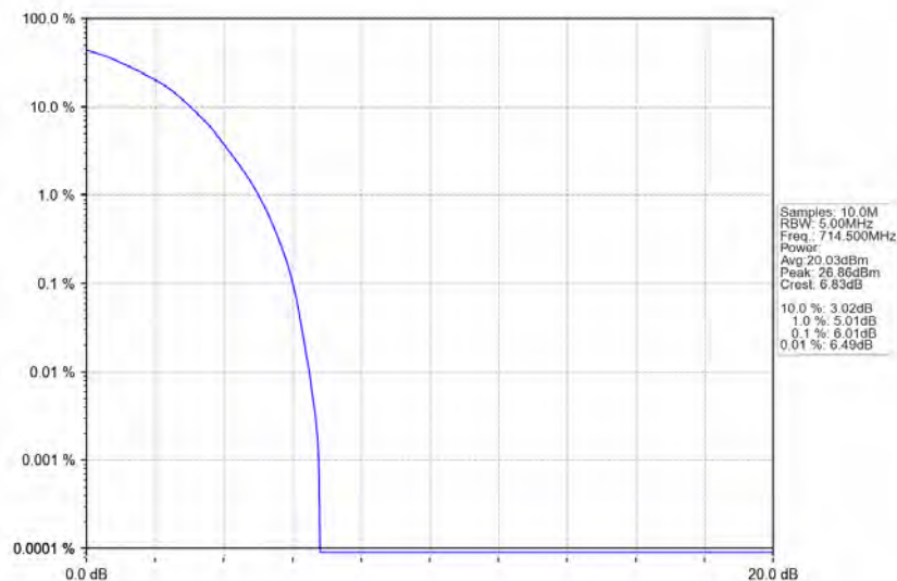
Band12_3MHz_64QAM_HCH_714.5MHz_RB_15_0_NTNV
