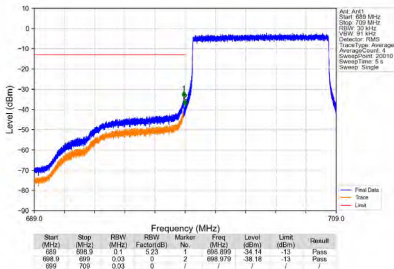
Band12_10MHz_64QAM_LCH_704MHz_RB_50_0_NTNV
