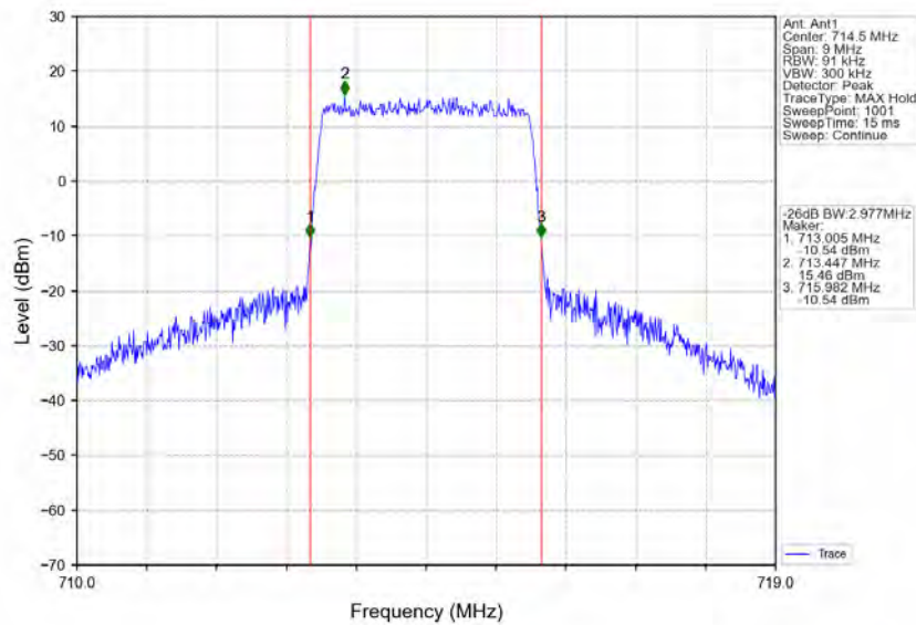
Band12_3MHz_64QAM_HCH_714.5MHz_RB_15_0_NTNV
