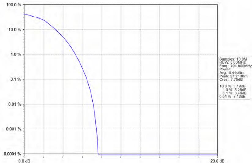
Band12_10MHz_16QAM_LCH_704MHz_RB_50_0_NTNV
