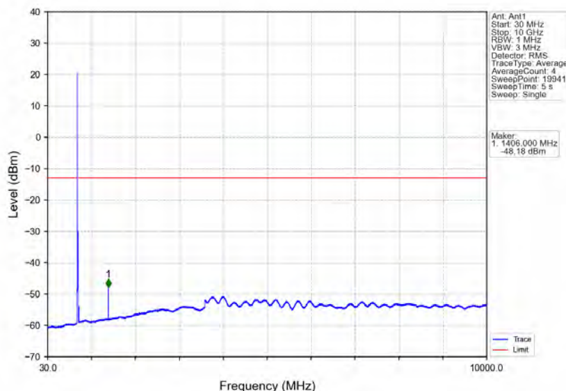
Band12_10MHz_64QAM_MCH_707.5MHz_RB_1_0_NTNV
