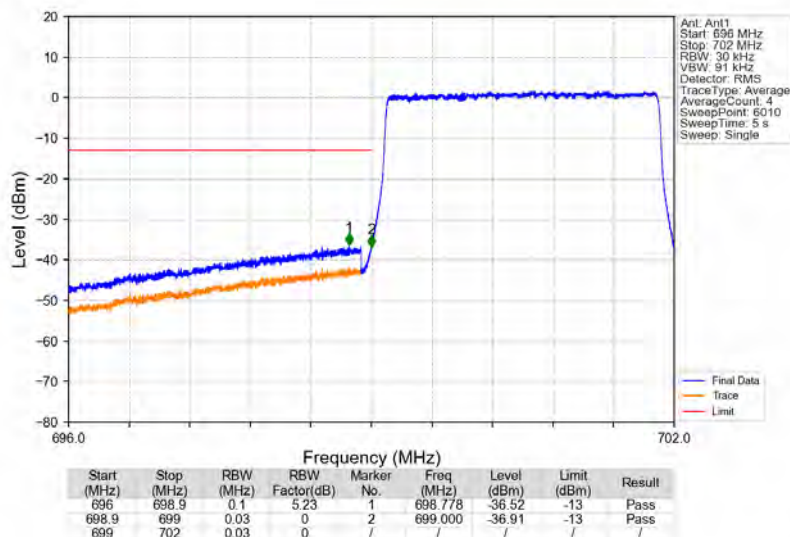
Band12_3MHz_64QAM_LCH_700.5MHz_RB_15_0_NTNV
