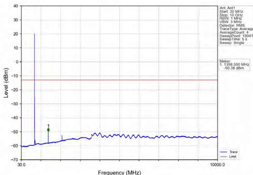
Band12_3MHz_64QAM_LCH_700.5MHz_RB_1_0_NTNV
