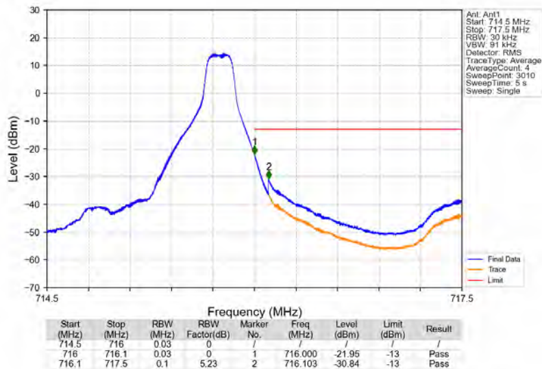
Band12_1.4MHz_64QAM_HCH_715.3MHz_RB_1_5_NTNV
