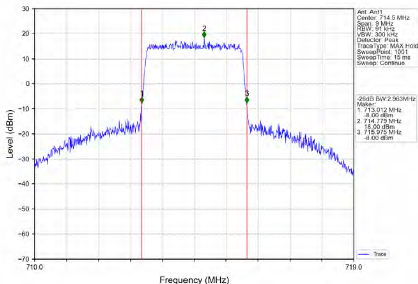
Band12_3MHz_QPSK_HCH_714.5MHz_RB_15_0_NTNV
