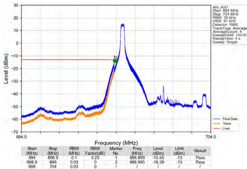
Band12_5MHz_16QAM_LCH_701.5MHz_RB_1_0_NTNV
