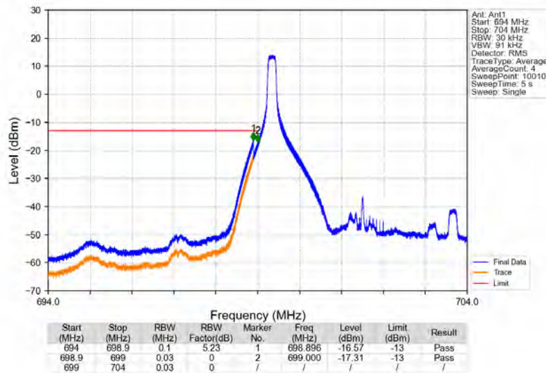
Band12_5MHz_64QAM_LCH_701.5MHz_RB_1_0_NTNV
