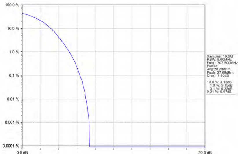
Band12_1.4MHz_64QAM_MCH_707.5MHz_RB_6_0_NTNV
