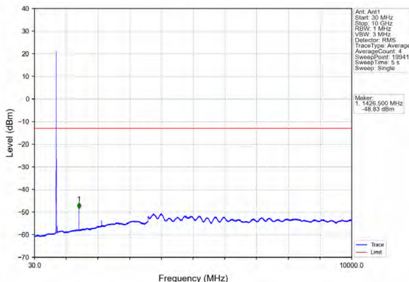
Band12_3MHz_16QAM_HCH_714.5MHz_RB_1_0_NTNV
