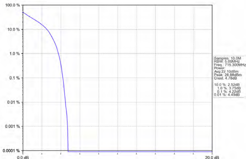
Band12_1.4MHz_QPSK_HCH_715.3MHz_RB_6_0_NTNV
