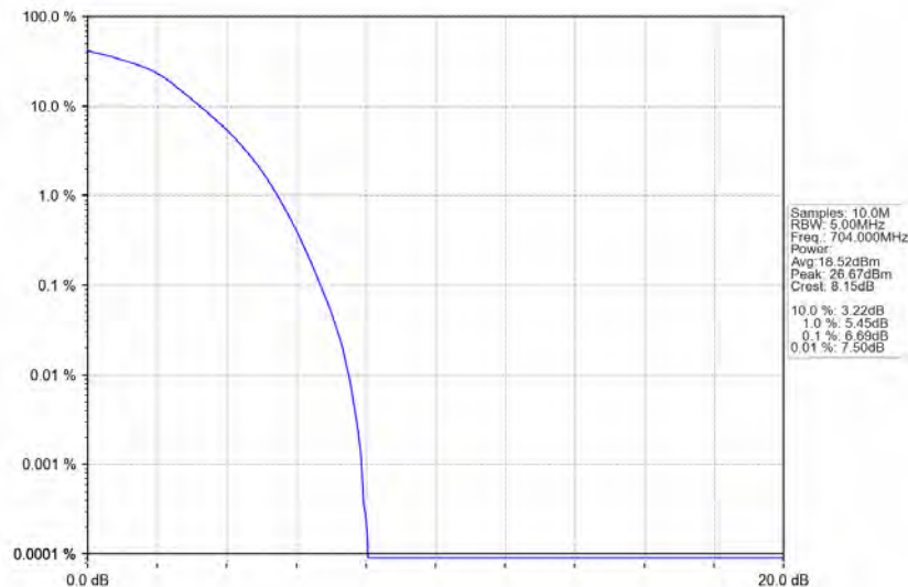
Band12_10MHz_64QAM_LCH_704MHz_RB_50_0_NTNV
