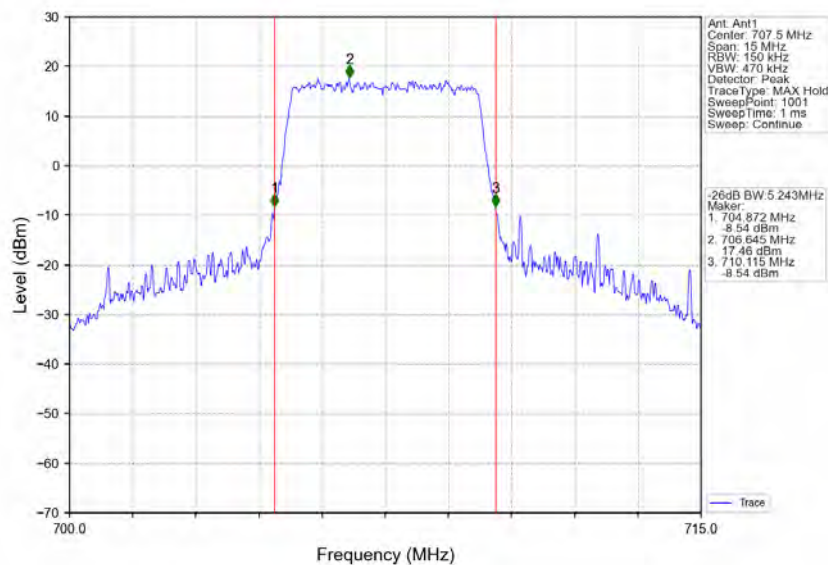
Band12_5MHz_QPSK_MCH_707.5MHz_RB_25_0_NTNV
