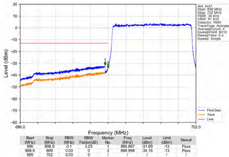
Band12_3MHz_QPSK_LCH_700.5MHz_RB_15_0_NTNV
