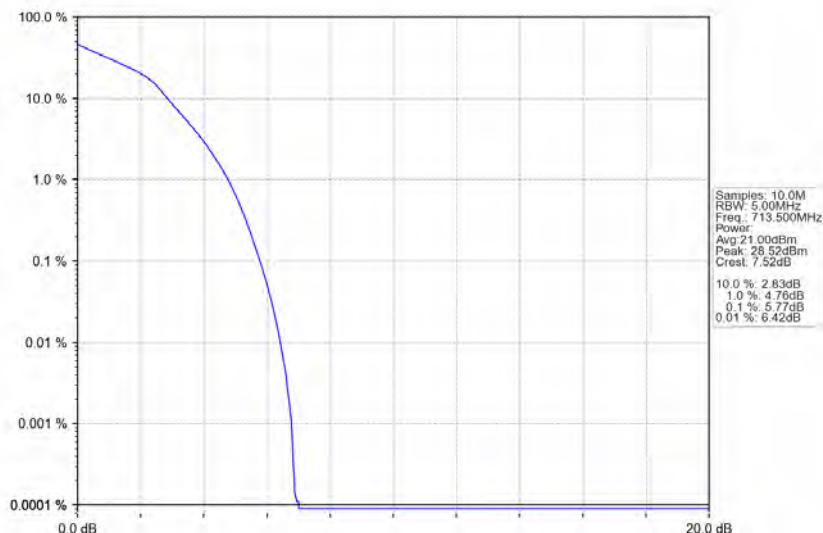
Band12_5MHz_16QAM_HCH_713.5MHz_RB_25_0_NTNV
