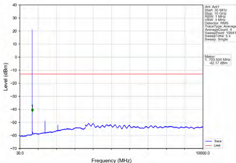
Band12_1.4MHz_16QAM_LCH_699.7MHz_RB_6_0_NTNV
