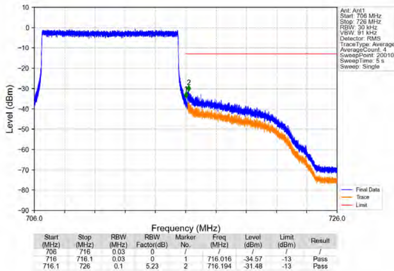
Band12_10MHz_QPSK_HCH_711MHz_RB_50_0_NTNV
