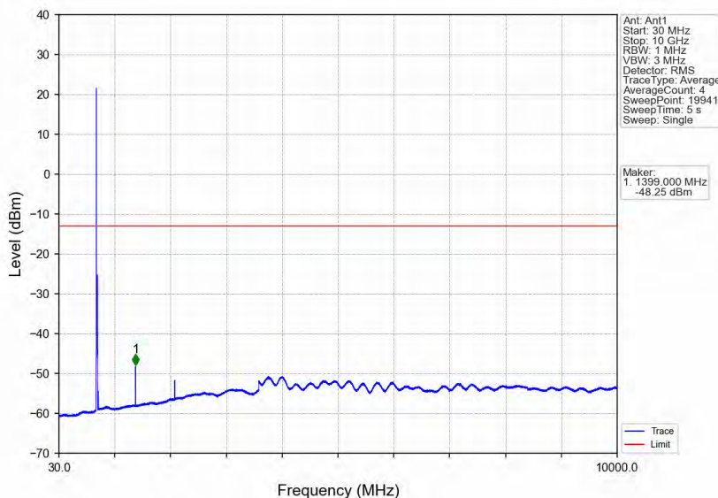
Band12_10MHz_16QAM_LCH_704MHz_RB_50_0_NTNV
