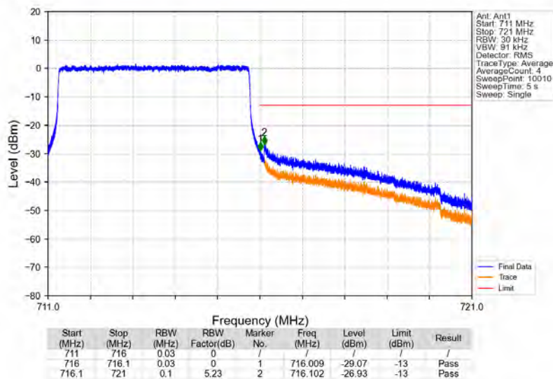
Band12_5MHz_QPSK_HCH_713.5MHz_RB_25_0_NTNV
