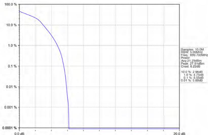
Band12_1.4MHz_16QAM_LCH_699.7MHz_RB_6_0_NTNV
