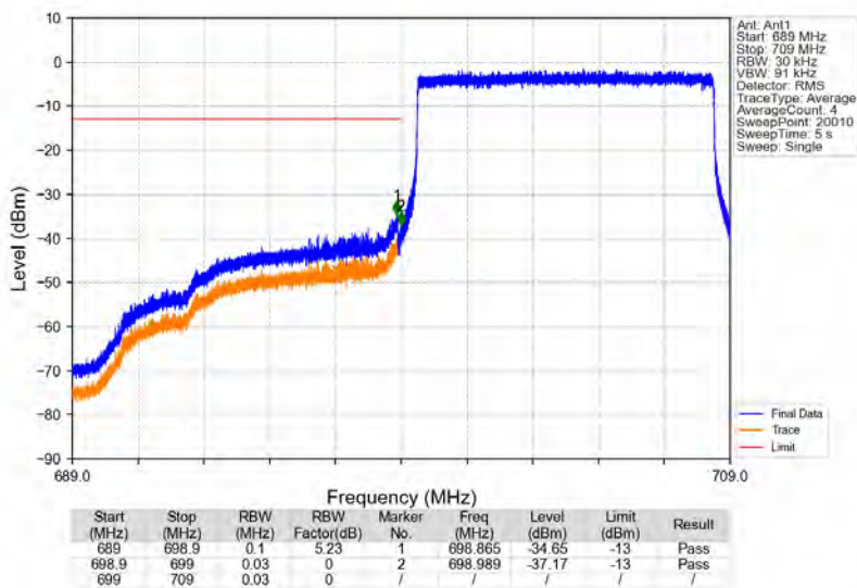
Band12_10MHz_16QAM_LCH_704MHz_RB_50_0_NTNV
