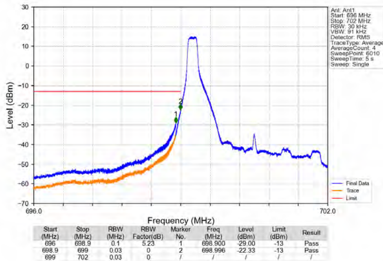
Band12_3MHz_16QAM_LCH_700.5MHz_RB_1_0_NTNV
