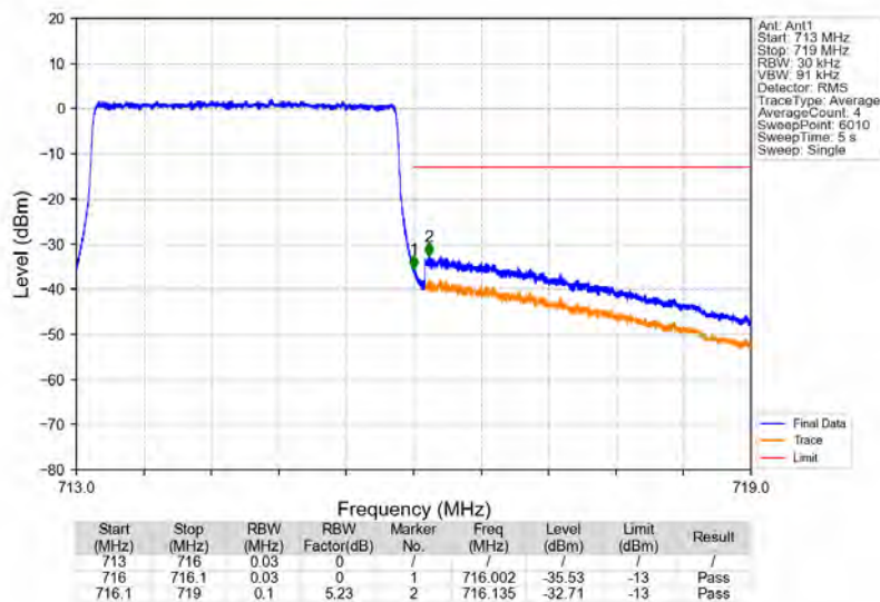
Band12_3MHz_64QAM_HCH_714.5MHz_RB_15_0_NTNV
