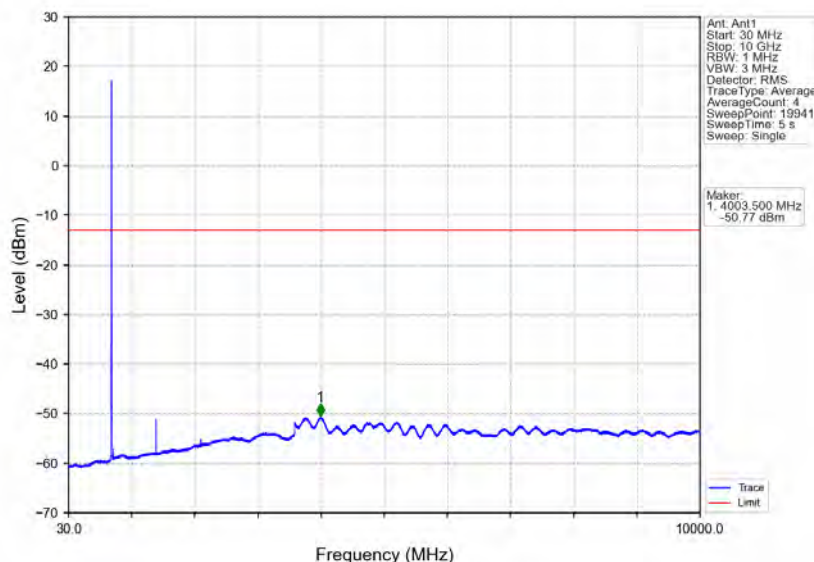
Band12_3MHz_64QAM_MCH_707.5MHz_RB_1_0_NTNV
