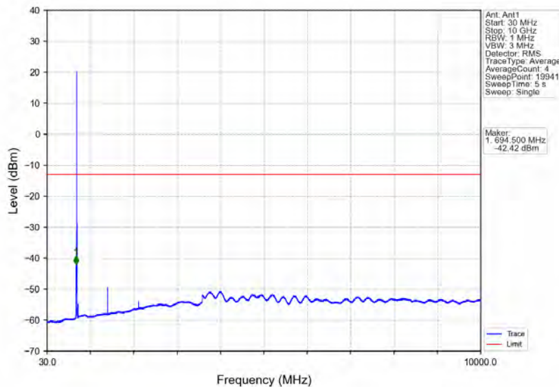
Band12_5MHz_64QAM_HCH_713.5MHz_RB_1_24_NTNV
