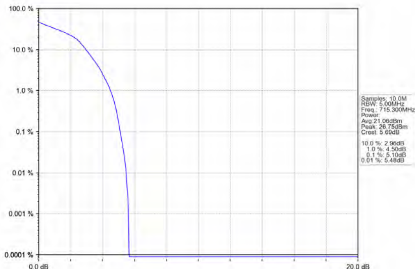
Band12_1.4MHz_16QAM_HCH_715.3MHz_RB_6_0_NTNV
