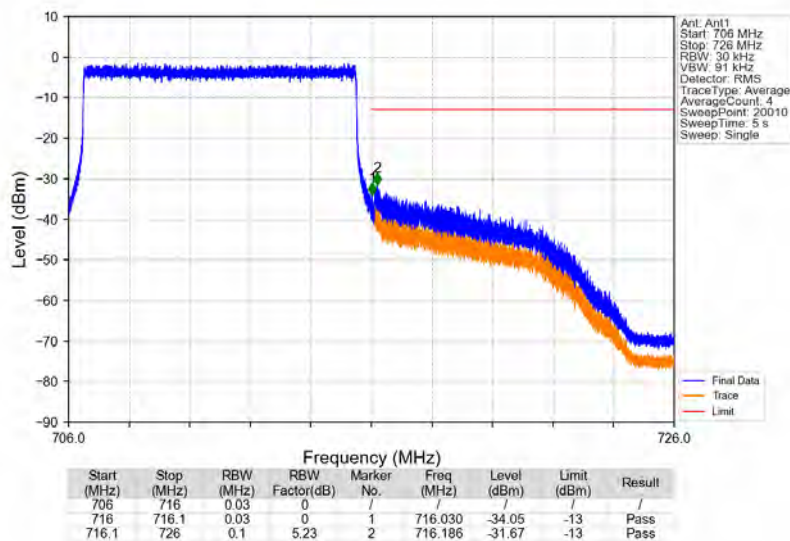
Band12_10MHz_16QAM_HCH_711MHz_RB_50_0_NTNV
