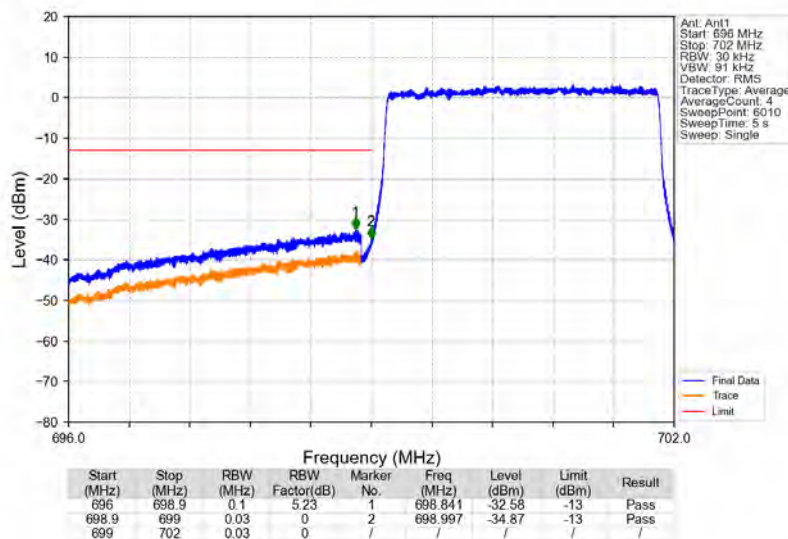
Band12_3MHz_16QAM_LCH_700.5MHz_RB_15_0_NTNV
