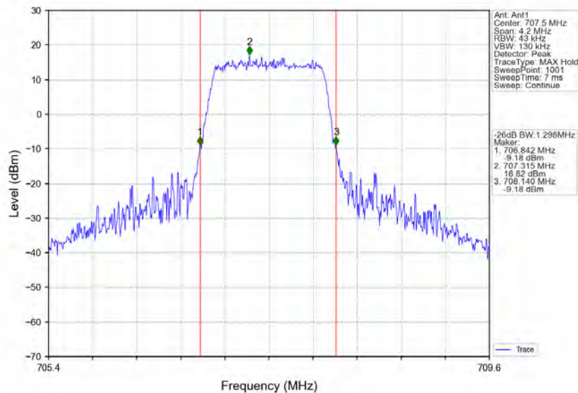
Band12_1.4MHz_64QAM_MCH_707.5MHz_RB_6_0_NTNV
