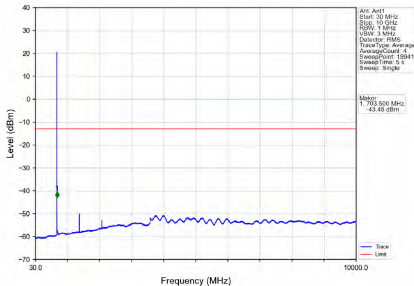
Band12_1.4MHz_64QAM_LCH_699.7MHz_RB_1_0_NTNV
