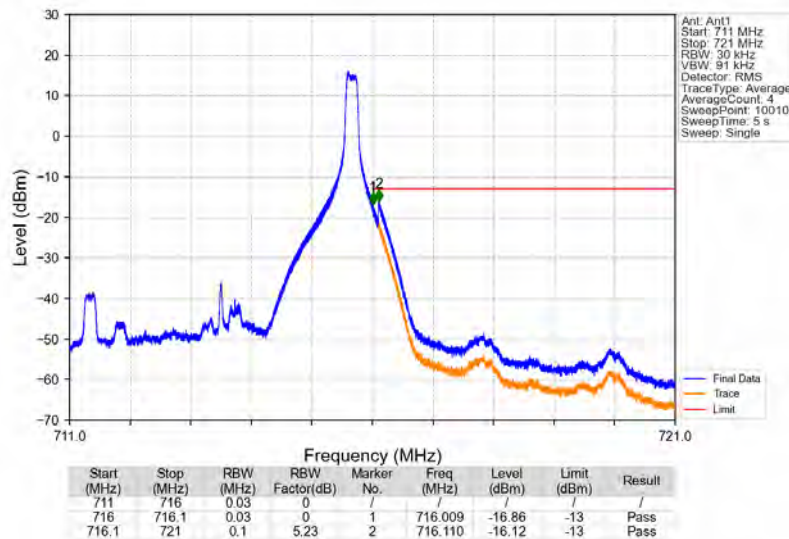
Band12_5MHz_QPSK_HCH_713.5MHz_RB_1_24_NTNV
