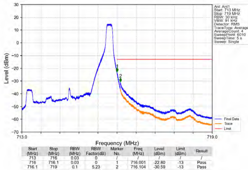
Band12_3MHz_16QAM_HCH_714.5MHz_RB_1_14_NTNV
