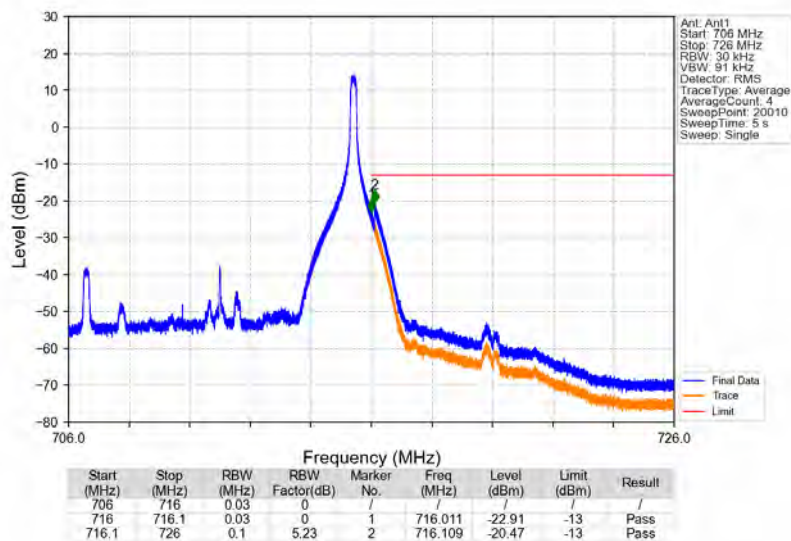
Band12_10MHz_64QAM_HCH_711MHz_RB_1_49_NTNV
