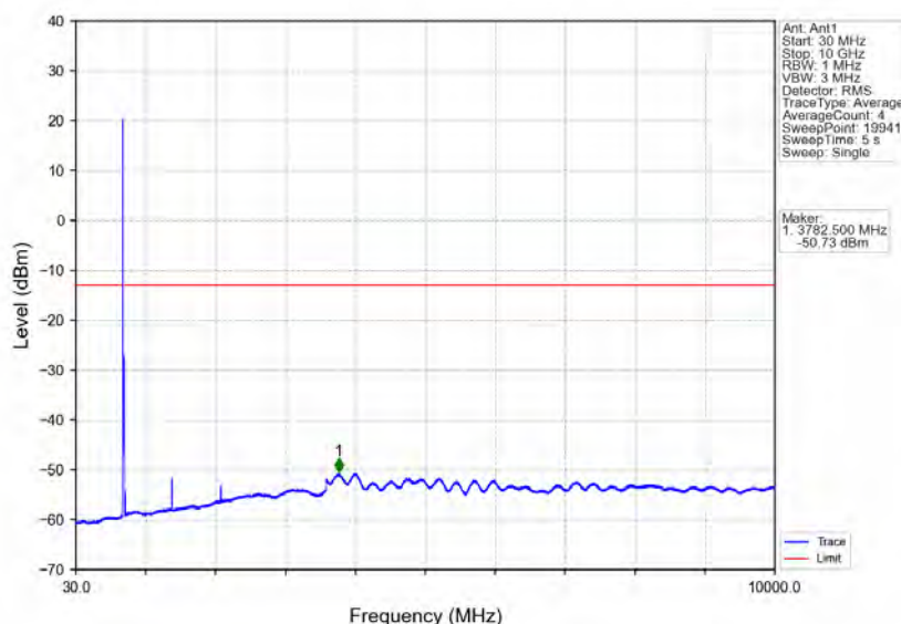
Band12_10MHz_64QAM_LCH_704MHz_RB_1_0_NTNV
