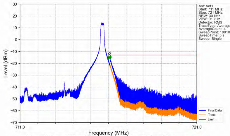
Band12_5MHz_64QAM_HCH_713.5MHz_RB_1_24_NTNV
