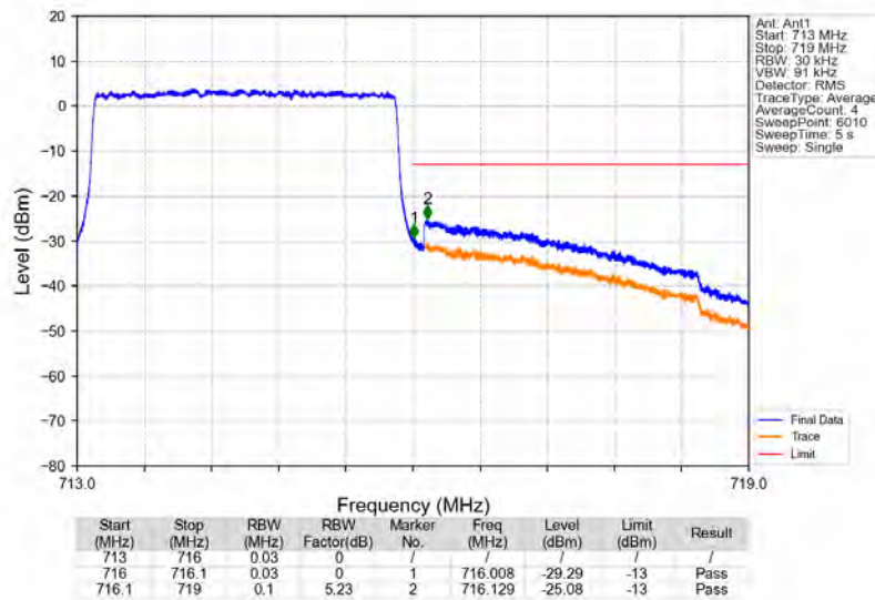
Band12_3MHz_QPSK_HCH_714.5MHz_RB_15_0_NTNV
