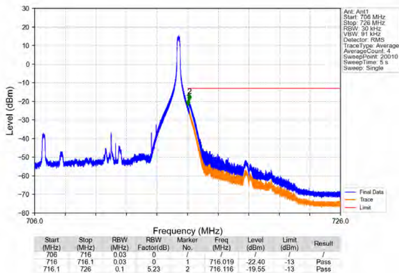
Band12_10MHz_16QAM_HCH_711MHz_RB_1_49_NTNV
