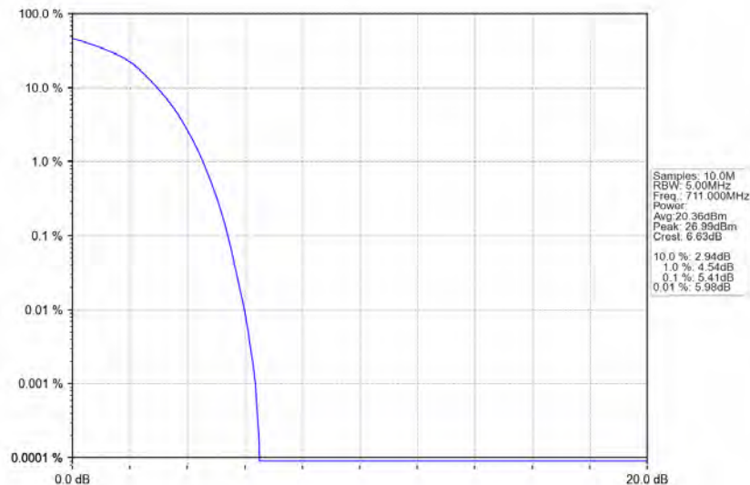
Band12_10MHz_QPSK_HCH_711MHz_RB_50_0_NTNV
