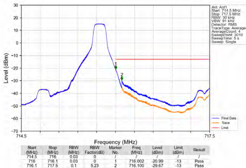
Band12_1.4MHz_QPSK_HCH_715.3MHz_RB_1_5_NTNV
