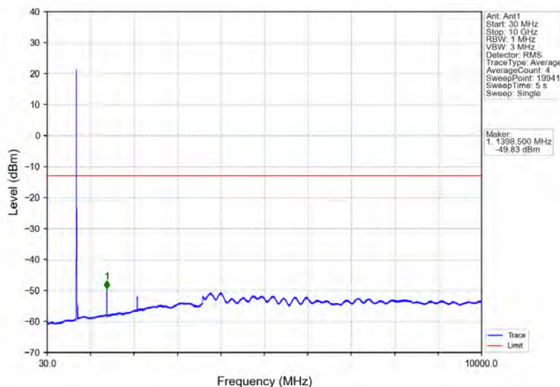
Band12_5MHz_16QAM_LCH_701.5MHz_RB_25_0_NTNV
