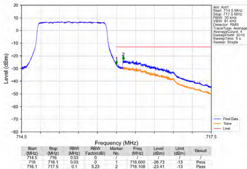
Band12_1.4MHz_QPSK_HCH_715.3MHz_RB_6_0_NTNV
