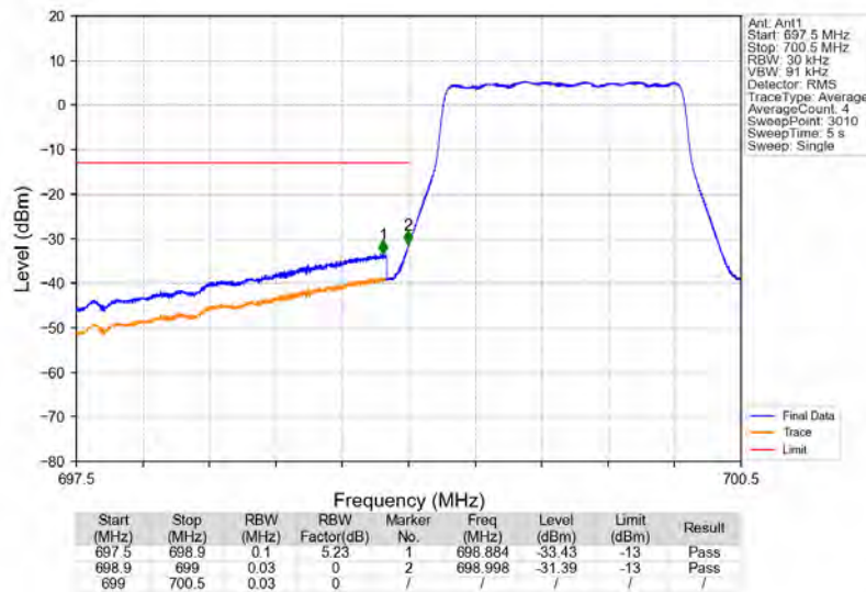
Band12_1.4MHz_64QAM_LCH_699.7MHz_RB_6_0_NTNV
