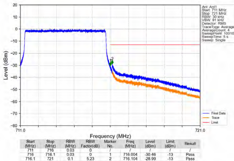
Band12_5MHz_64QAM_HCH_713.5MHz_RB_25_0_NTNV
