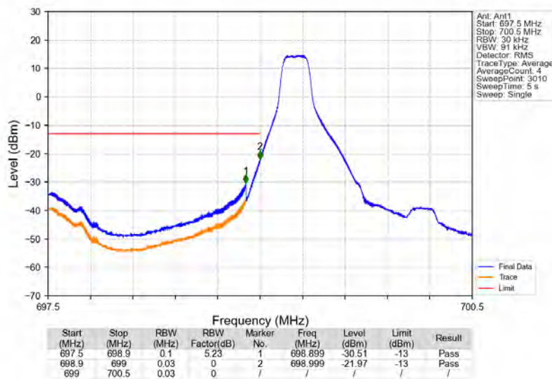
Band12_1.4MHz_16QAM_LCH_699.7MHz_RB_1_0_NTNV
