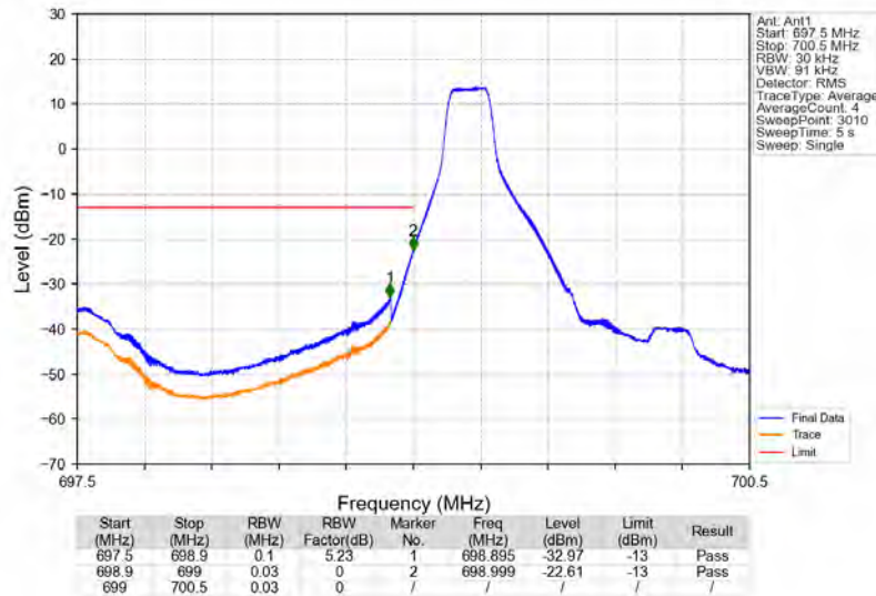
Band12_1.4MHz_64QAM_LCH_699.7MHz_RB_1_0_NTNV
