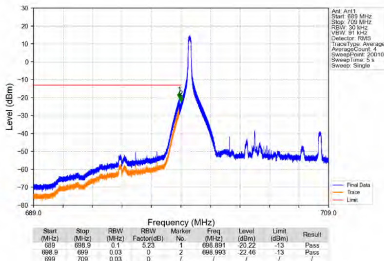
Band12_10MHz_64QAM_LCH_704MHz_RB_1_0_NTNV
