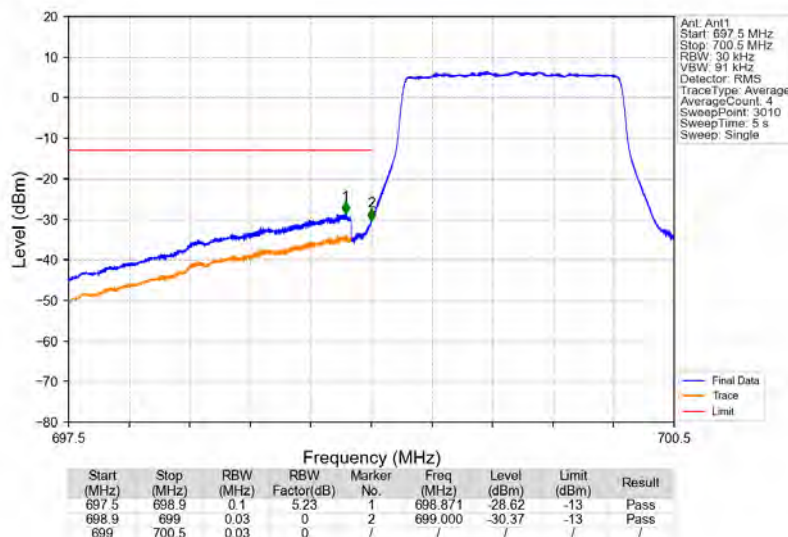
Band12_1.4MHz_16QAM_LCH_699.7MHz_RB_6_0_NTNV
