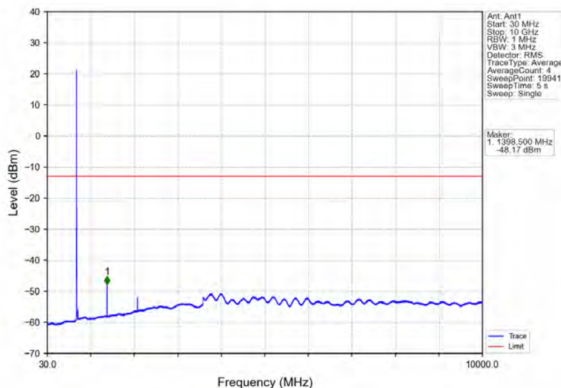
Band12_3MHz_16QAM_LCH_700.5MHz_RB_15_0_NTNV
