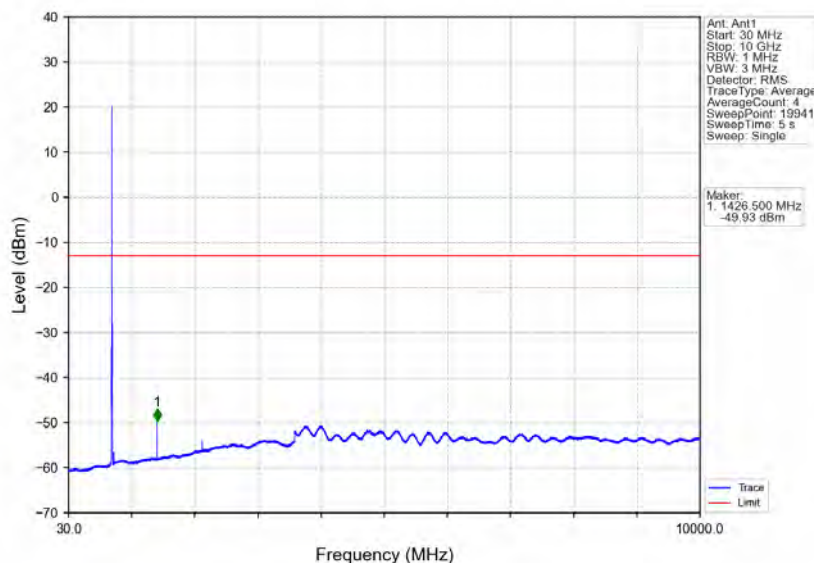
Band12_3MHz_64QAM_HCH_714.5MHz_RB_1_14_NTNV
