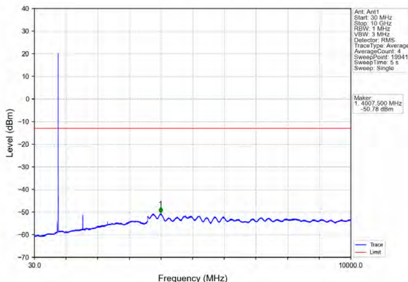
Band13_5MHz_64QAM_LCH_779.5MHz_RB_1_0_NTNV
