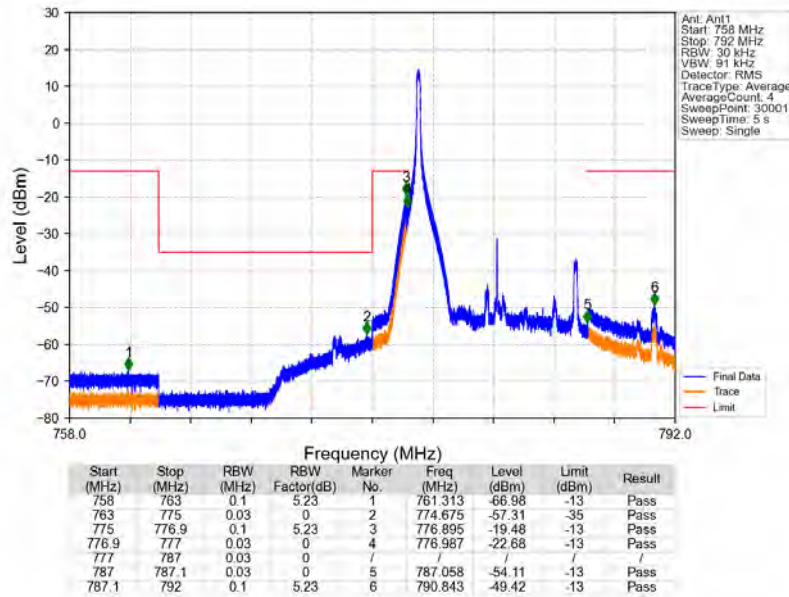
Band13_10MHz_64QAM_LCH_782MHz_RB_1_0_NTNV
