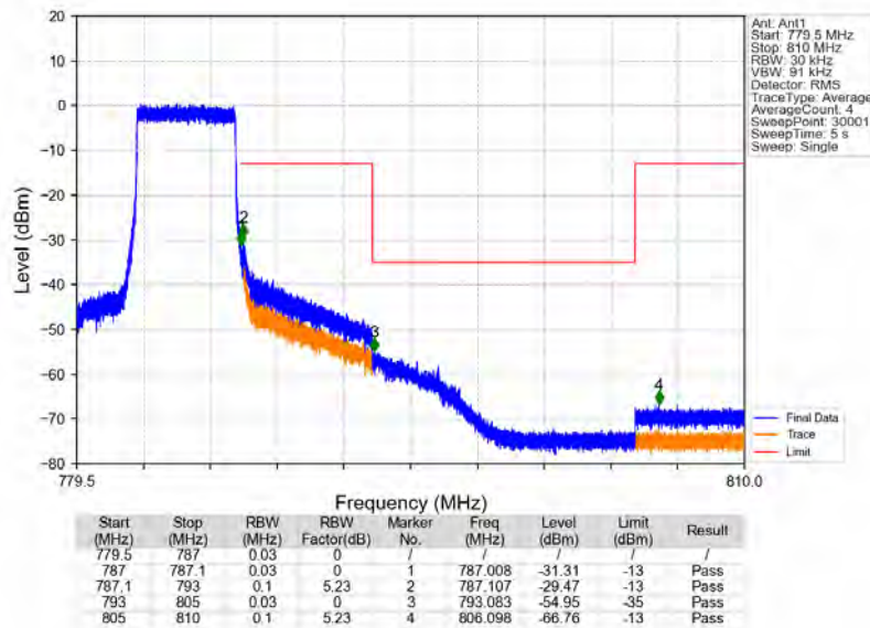
Band13_5MHz_64QAM_HCH_784.5MHz_RB_25_0_NTNV
