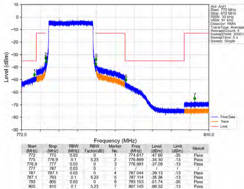
Band13_10MHz_64QAM_HCH_782MHz_RB_50_0_NTNV
