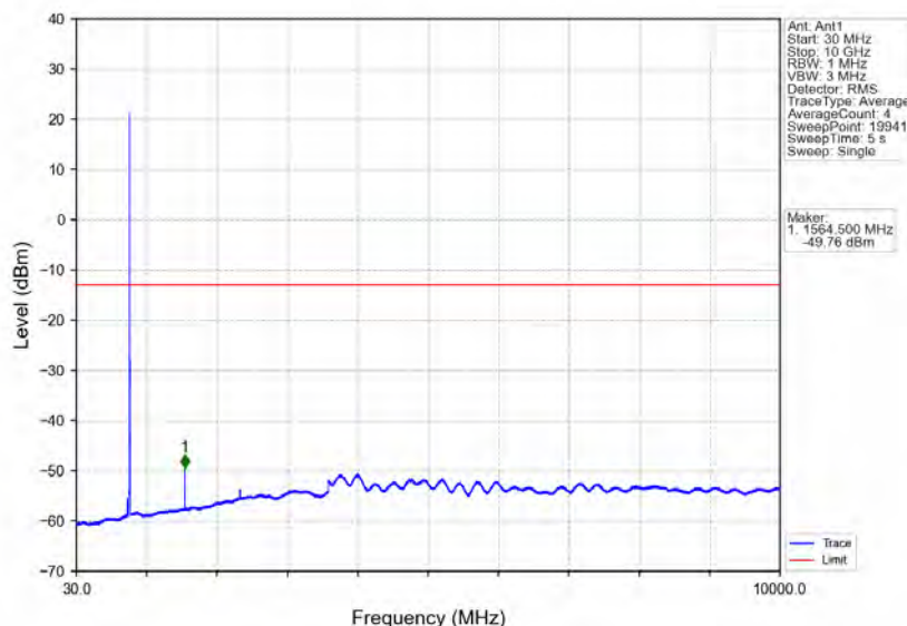
Band13_5MHz_16QAM_HCH_784.5MHz_RB_1_0_NTNV
