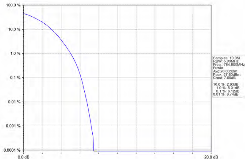
Band13_5MHz_64QAM_HCH_784.5MHz_RB_25_0_NTNV
