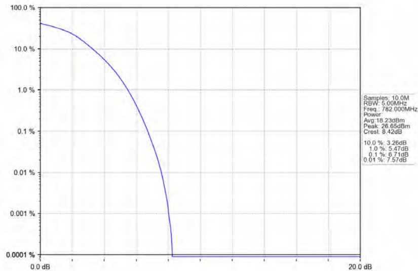
Band13_10MHz_64QAM_MCH_782MHz_RB_50_0_NTNV
