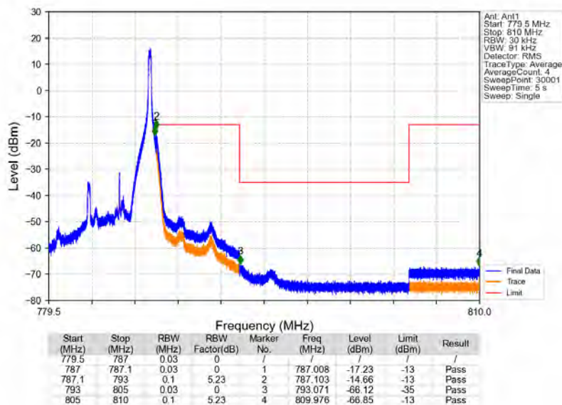
Band13_5MHz_16QAM_HCH_784.5MHz_RB_25_0_NTNV
