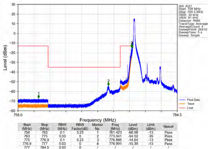
Band13_5MHz_16QAM_LCH_779.5MHz_RB_1_0_NTNV
