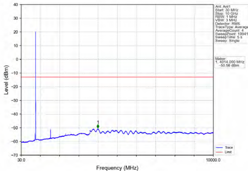
Band13_10MHz_64QAM_LCH_782MHz_RB_1_0_NTNV
