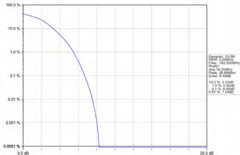
Band13_10MHz_64QAM_HCH_782MHz_RB_50_0_NTNV
