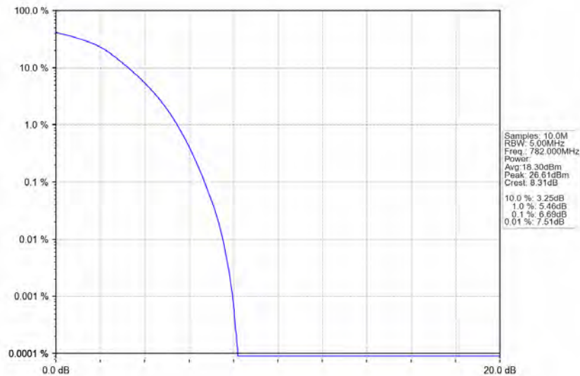
Band13_10MHz_64QAM_LCH_782MHz_RB_50_0_NTNV
