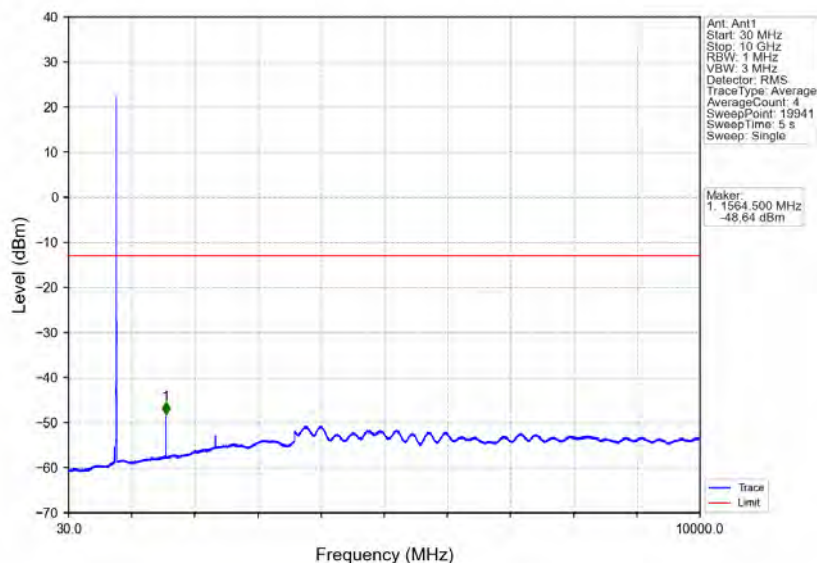
Band13_5MHz_QPSK_HCH_784.5MHz_RB_1_24_NTNV
