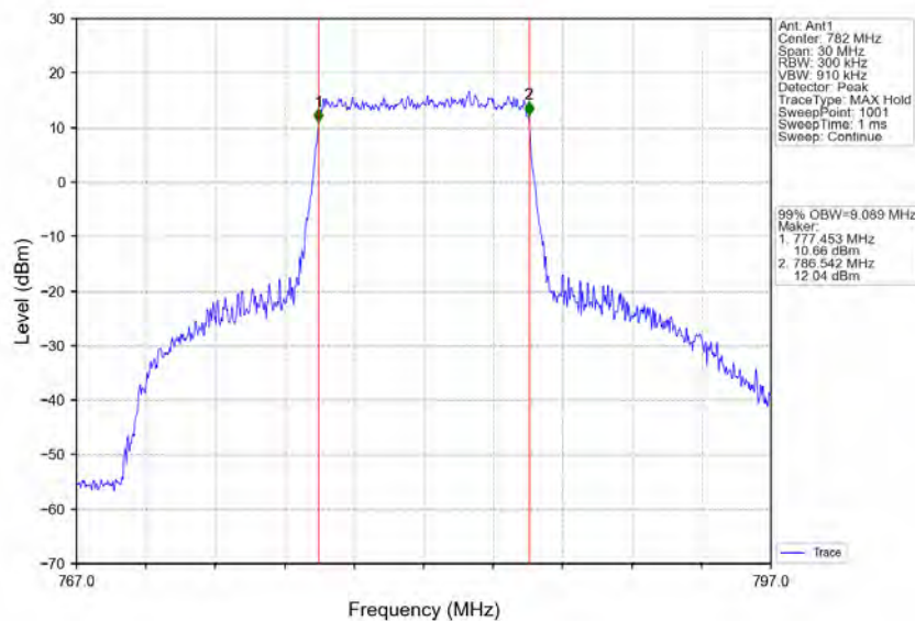
Band13_10MHz_64QAM_LCH_782MHz_RB_50_0_NTNV
