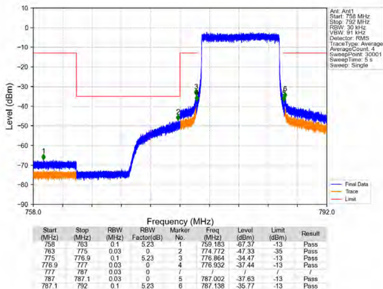
Band13_10MHz_64QAM_MCH_782MHz_RB_1_0_NTNV
