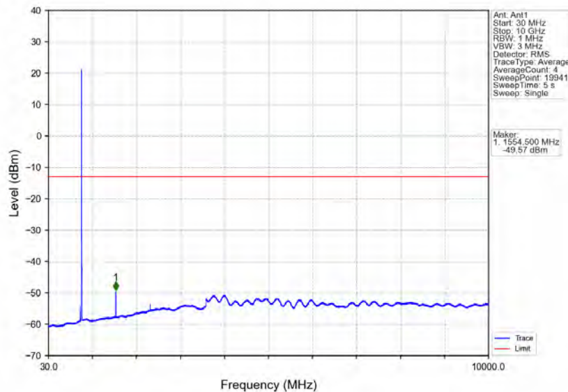
Band13_5MHz_16QAM_LCH_779.5MHz_RB_25_0_NTNV
