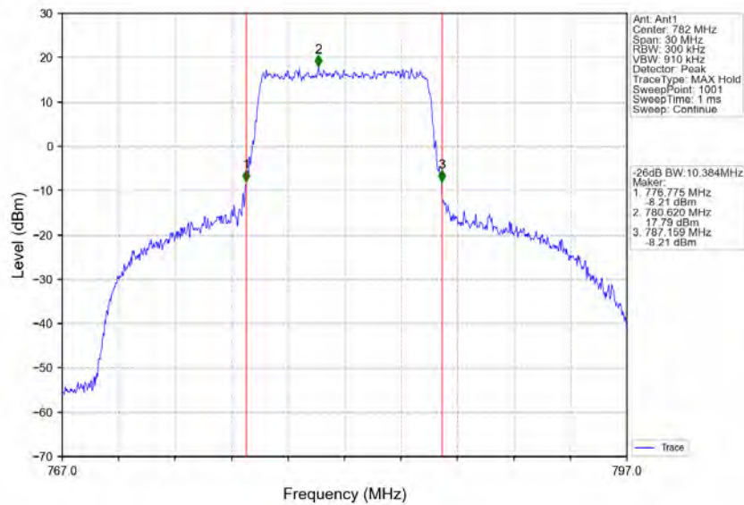
Band13_10MHz_QPSK_HCH_782MHz_RB_50_0_NTNV
