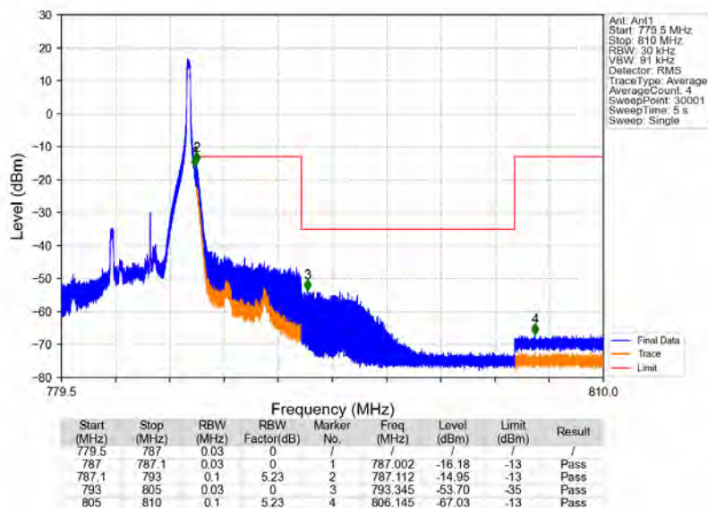
Band13_5MHz_QPSK_HCH_784.5MHz_RB_1_24_NTNV
