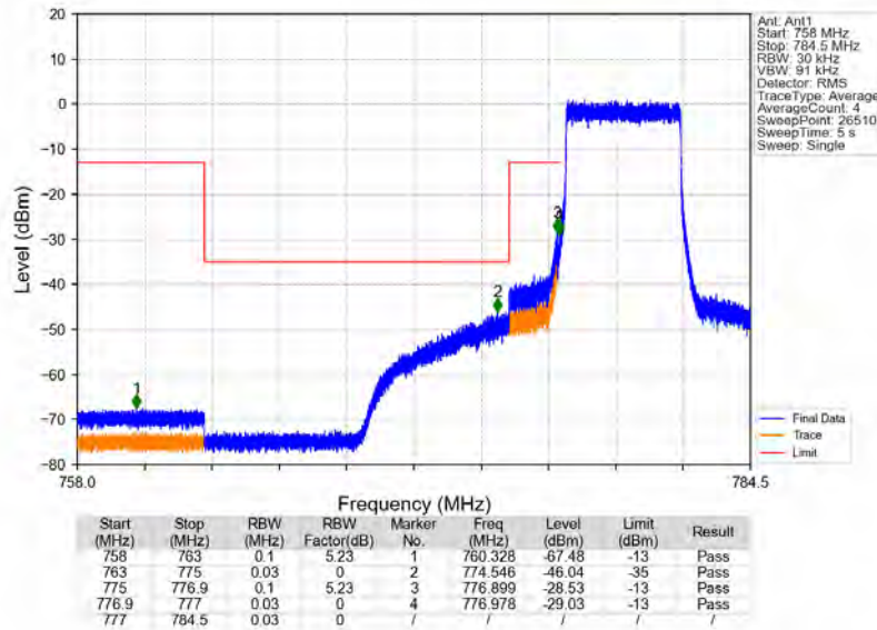
Band13_5MHz_64QAM_MCH_782MHz_RB_1_0_NTNV
