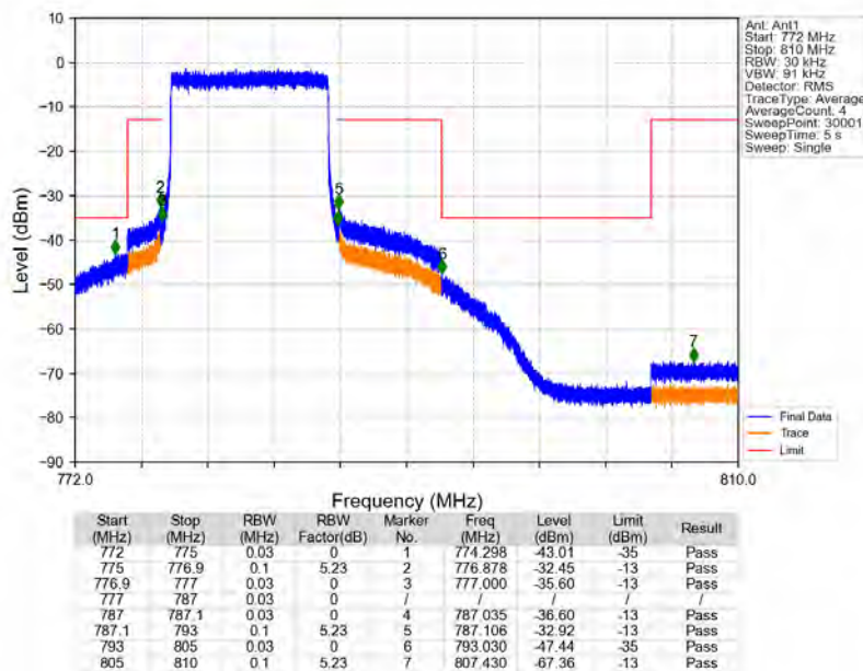
Band13_10MHz_16QAM_HCH_782MHz_RB_50_0_NTNV
