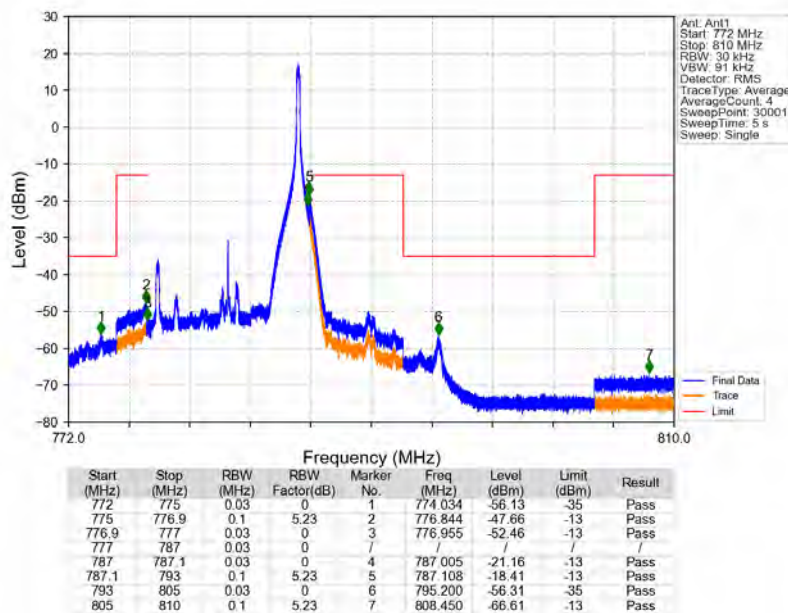
Band13_10MHz_QPSK_HCH_782MHz_RB_1_49_NTNV
