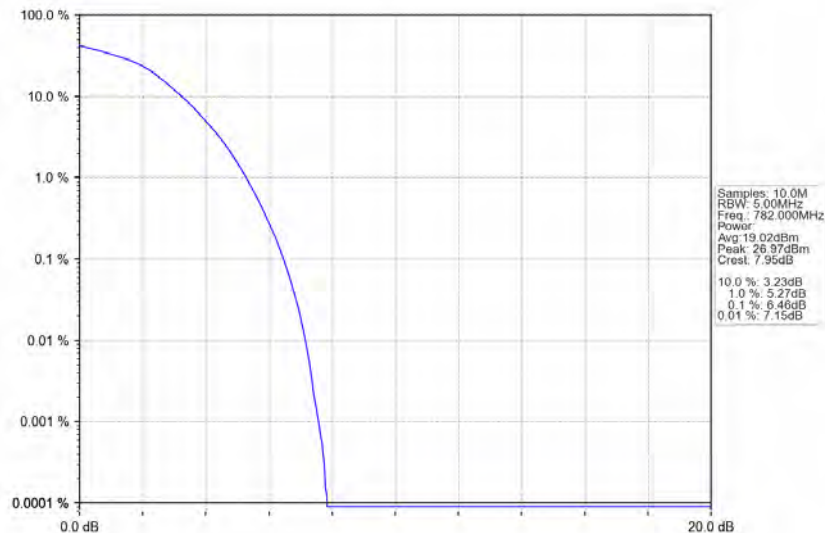
Band13_10MHz_16QAM_MCH_782MHz_RB_50_0_NTNV
