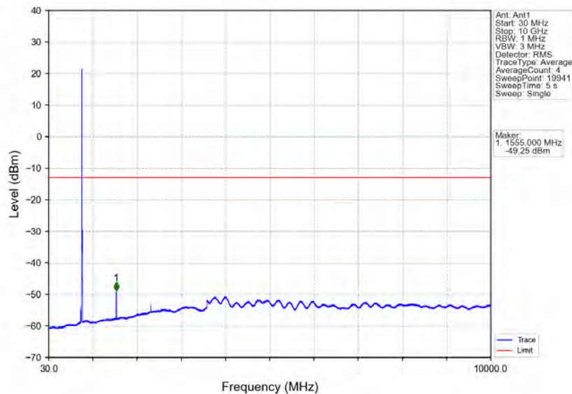
Band13_10MHz_16QAM_LCH_782MHz_RB_50_0_NTNV
