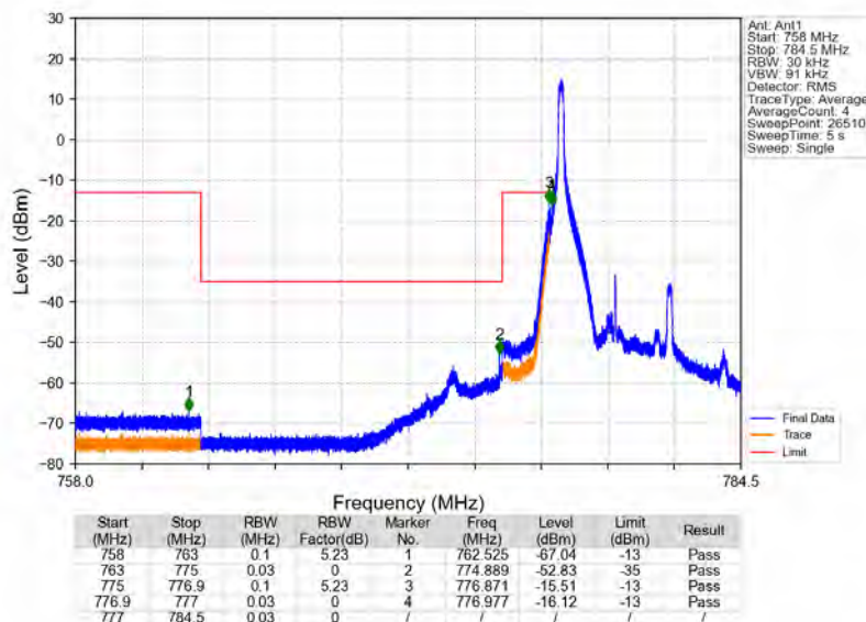
Band13_5MHz_64QAM_LCH_779.5MHz_RB_1_0_NTNV
