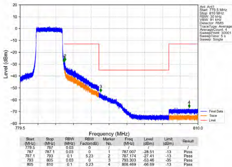
Band13_5MHz_16QAM_HCH_784.5MHz_RB_25_0_NTNV
