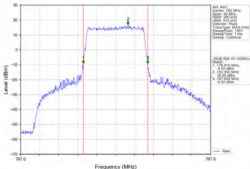
Band13_10MHz_64QAM_HCH_782MHz_RB_50_0_NTNV
