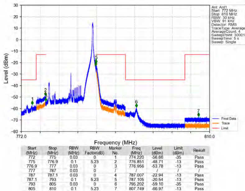
Band13_10MHz_64QAM_HCH_782MHz_RB_1_49_NTNV
