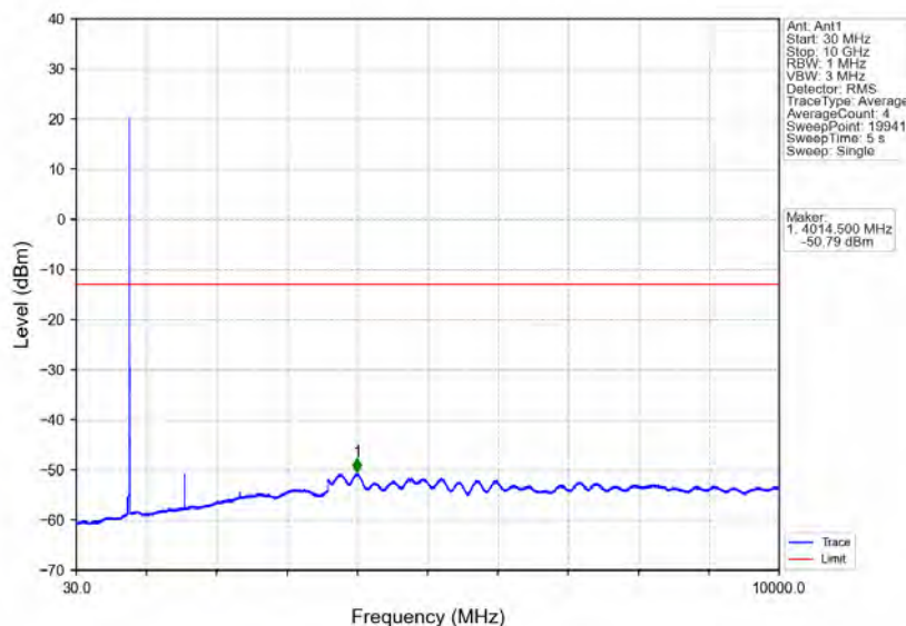
Band13_5MHz_64QAM_HCH_784.5MHz_RB_1_24_NTNV
