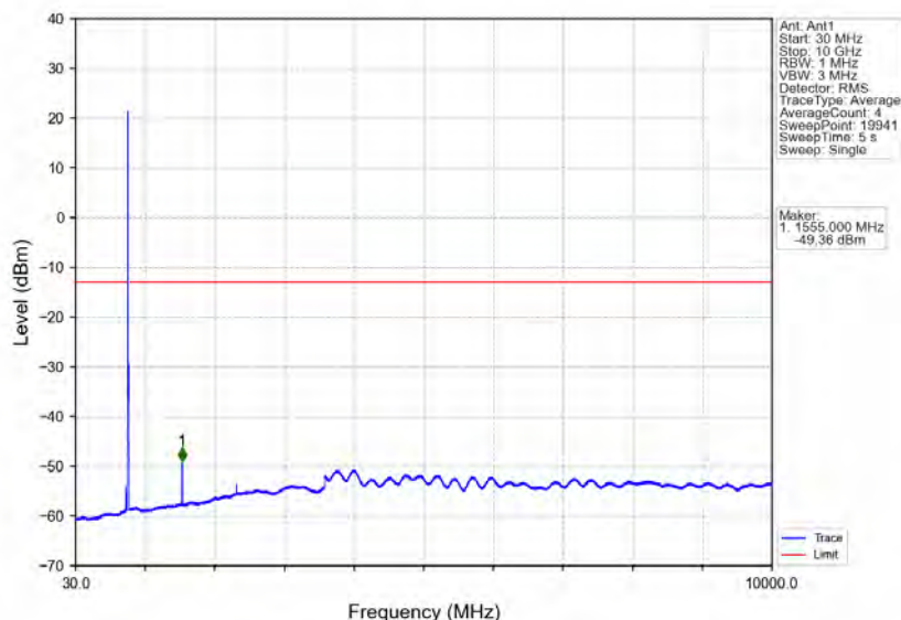
Band13_10MHz_16QAM_HCH_782MHz_RB_1_0_NTNV
