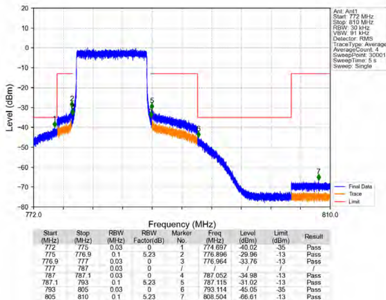
Band13_10MHz_16QAM_LCH_782MHz_RB_1_0_NTNV
