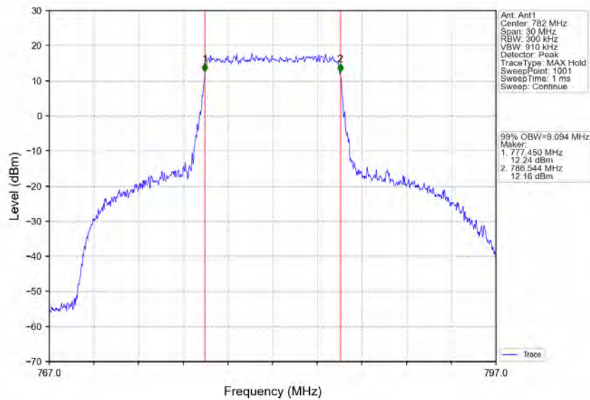
Band13_10MHz_QPSK_HCH_782MHz_RB_50_0_NTNV
