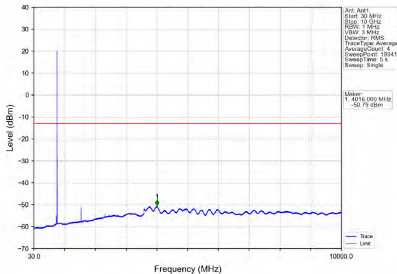
Band13_5MHz_64QAM_MCH_782MHz_RB_1_0_NTNV
