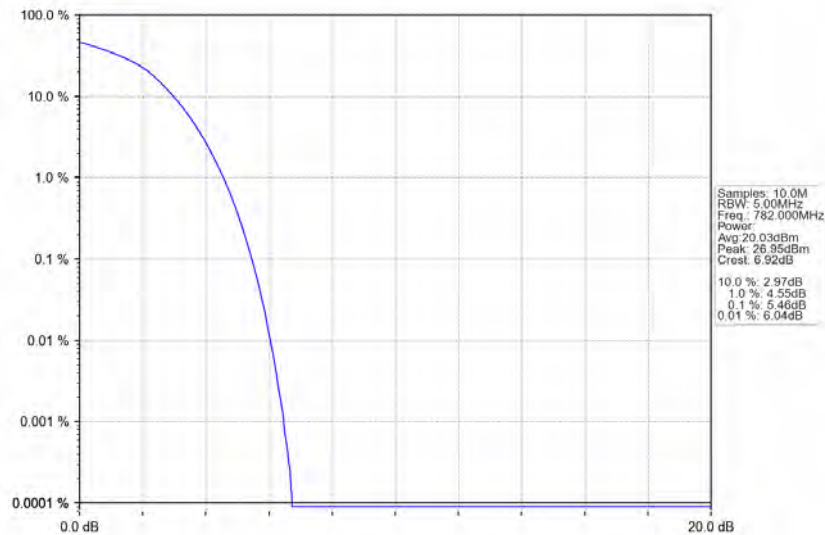
Band13_10MHz_QPSK_HCH_782MHz_RB_50_0_NTNV
