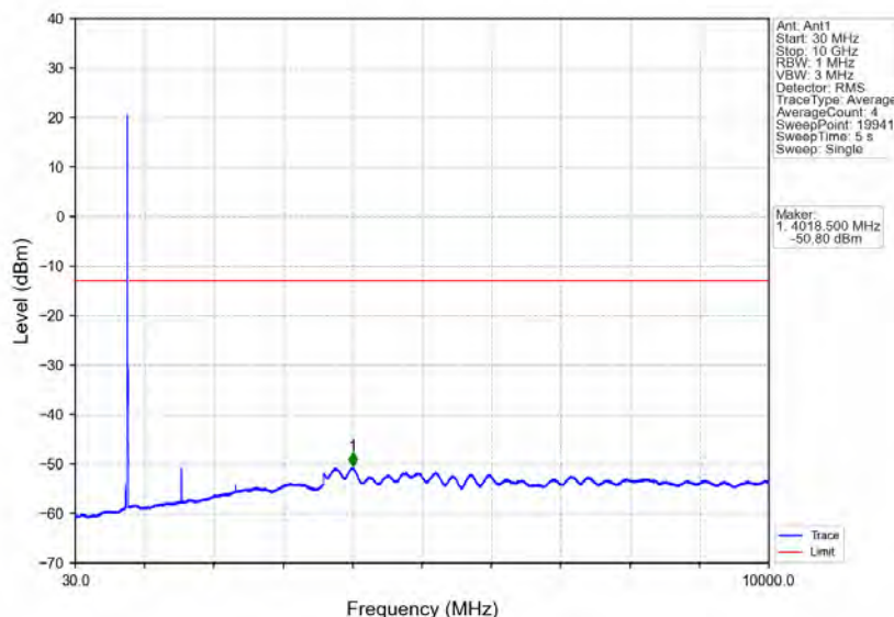
Band13_10MHz_64QAM_MCH_782MHz_RB_1_0_NTNV
