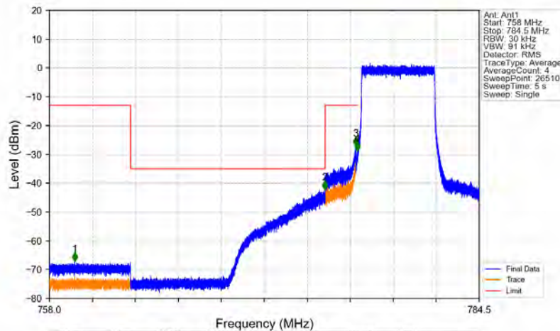
Band13_5MHz_16QAM_LCH_779.5MHz_RB_25_0_NTNV
