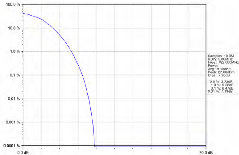
Band13_10MHz_16QAM_LCH_782MHz_RB_50_0_NTNV
