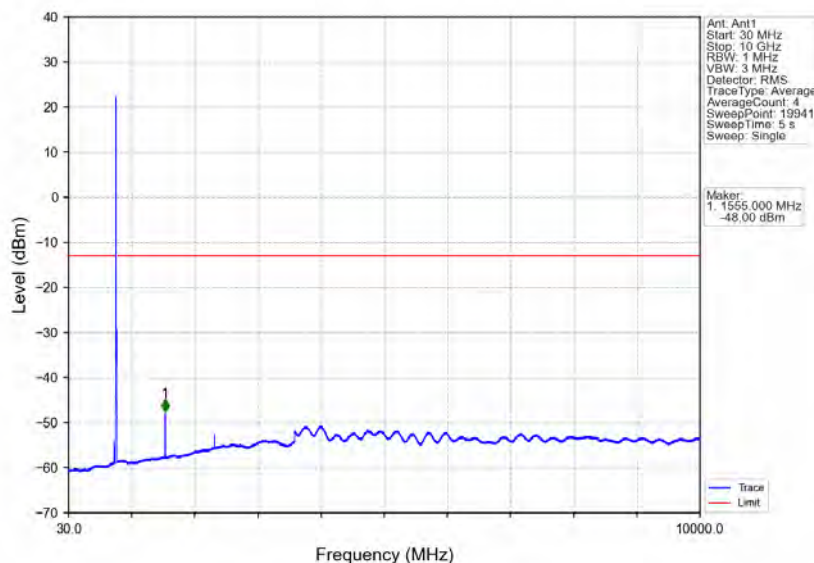
Band13_10MHz_QPSK_HCH_782MHz_RB_1_49_NTNV
