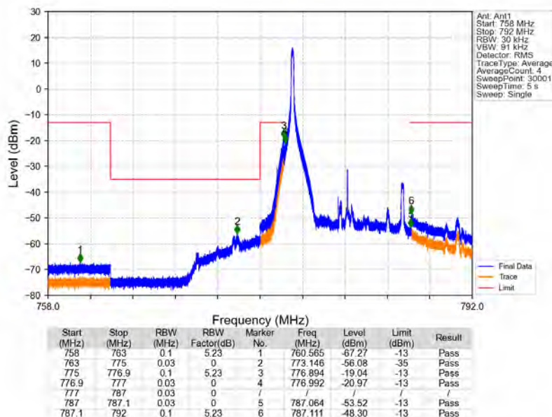
Band13_10MHz_16QAM_LCH_782MHz_RB_1_0_NTNV
