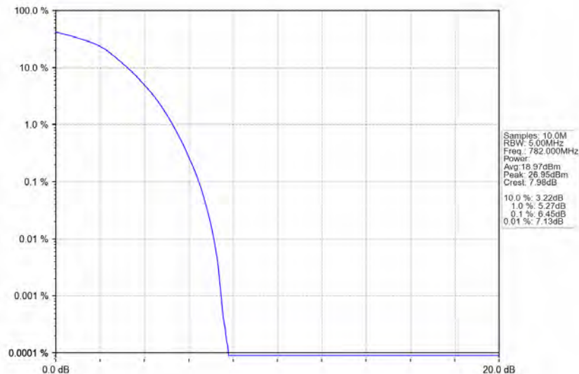
Band13_10MHz_16QAM_HCH_782MHz_RB_50_0_NTNV
