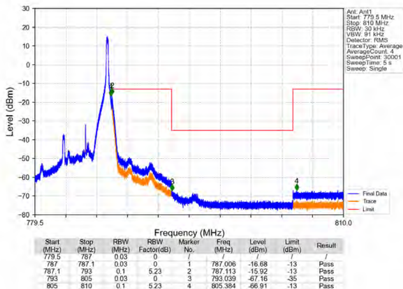
Band13_5MHz_64QAM_HCH_784.5MHz_RB_1_24_NTNV
