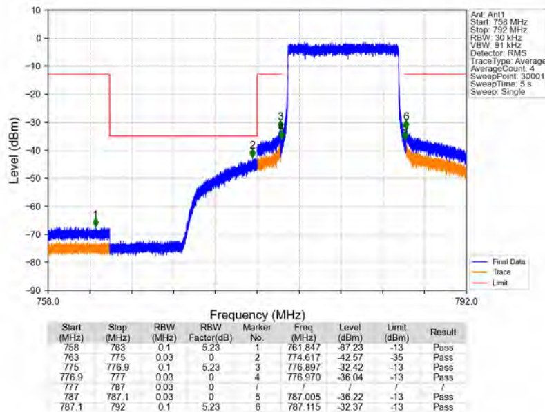
Band13_10MHz_16QAM_LCH_782MHz_RB_50_0_NTNV
