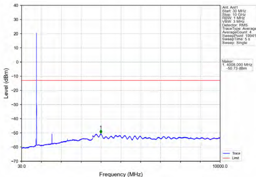
Band13_10MHz_64QAM_HCH_782MHz_RB_1_49_NTNV
