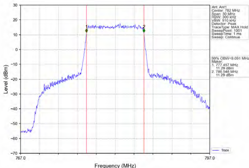
Band13_10MHz_16QAM_MCH_782MHz_RB_50_0_NTNV
