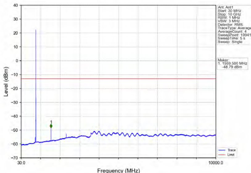
Band13_5MHz_QPSK_MCH_782MHz_RB_1_0_NTNV
