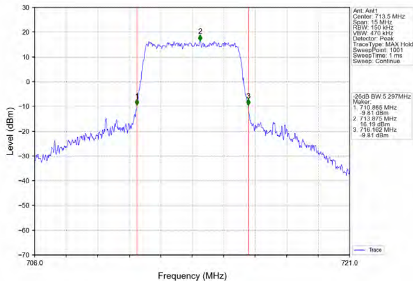
Band17_5MHz_16QAM_HCH_713.5MHz_RB_25_0_NTNV
