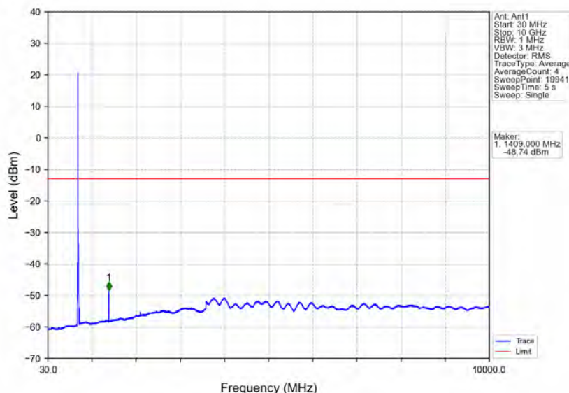
Band17_10MHz_64QAM_LCH_709MHz_RB_1_0_NTNV
