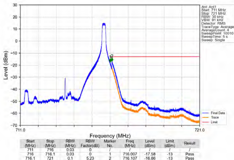
Band17_5MHz_16QAM_HCH_713.5MHz_RB_1_24_NTNV
