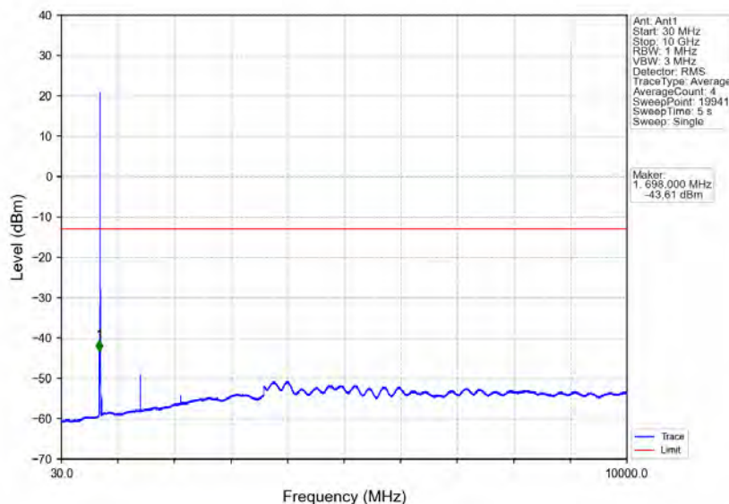
Band17_5MHz_64QAM_HCH_713.5MHz_RB_1_24_NTNV
