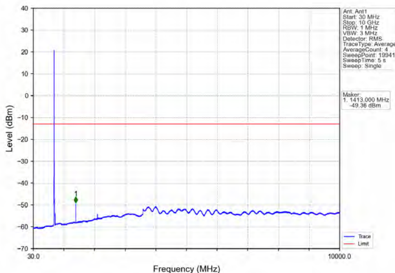
Band17_10MHz_64QAM_HCH_711MHz_RB_1_49_NTNV
