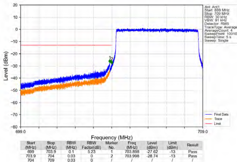
Band17_5MHz_16QAM_LCH_706.5MHz_RB_25_0_NTNV
