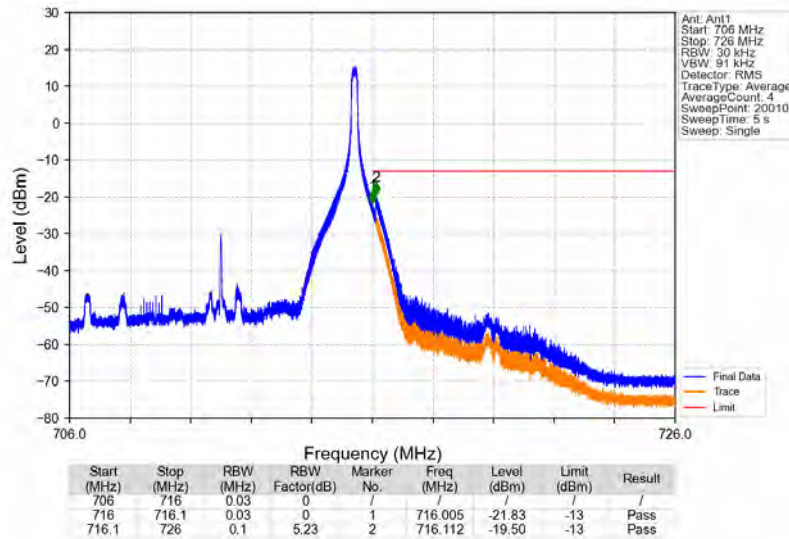
Band17_10MHz_16QAM_HCH_711MHz_RB_1_49_NTV
