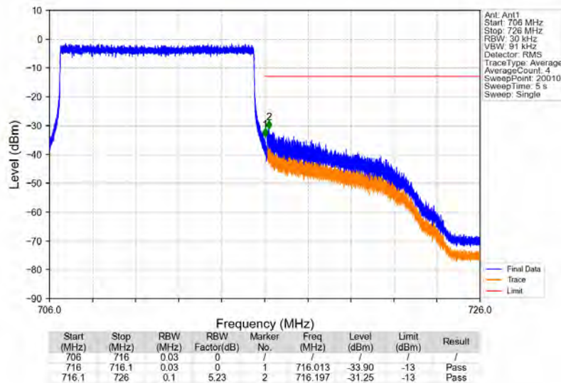
Band17_10MHz_16QAM_HCH_711MHz_RB_50_0_NTV
