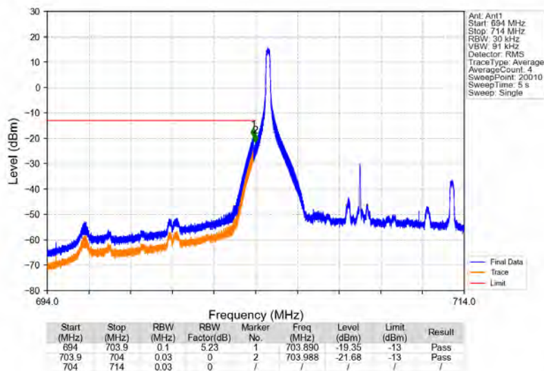
Band17_10MHz_16QAM_LCH_709MHz_RB_1_0_NTNV
