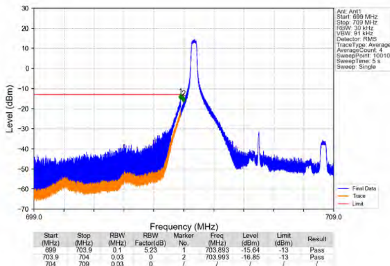
Band17_5MHz_64QAM_LCH_706.5MHz_RB_1_0_NTNV
