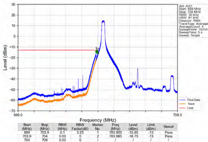
Band17_5MHz_16QAM_LCH_706.5MHz_RB_1_0_NTNV
