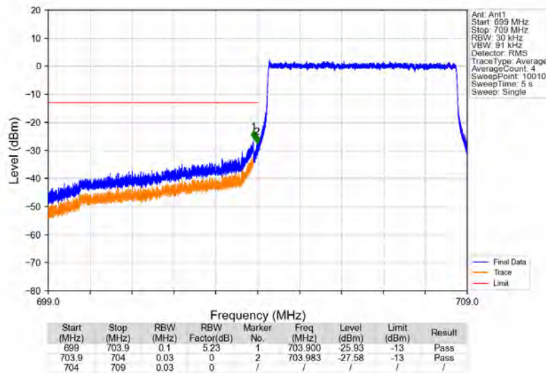
Band17_5MHz_QPSK_LCH_706.5MHz_RB_25_0_NTNV
