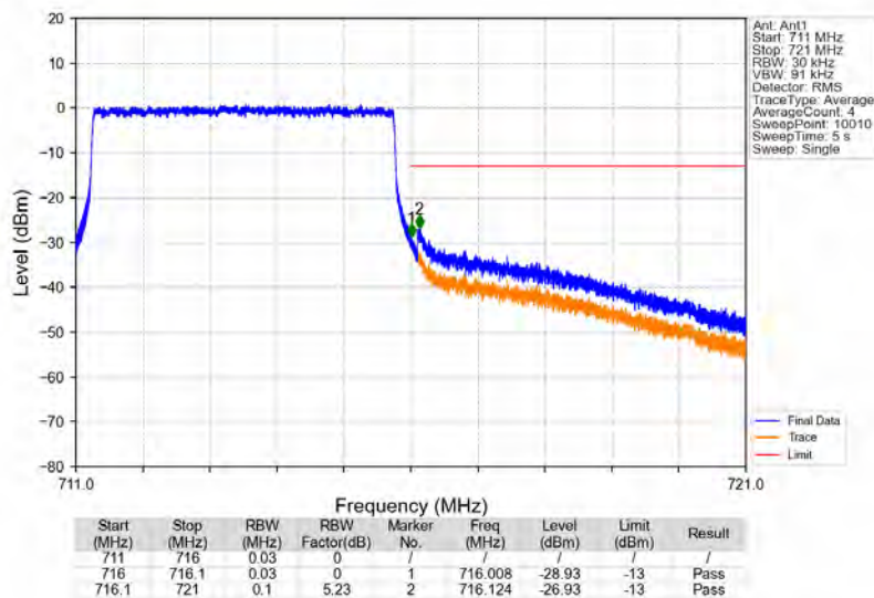
Band17_5MHz_16QAM_HCH_713.5MHz_RB_25_0_NTNV
