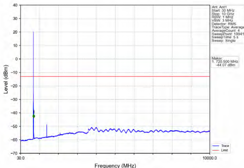
Band17_5MHz_64QAM_LCH_706.5MHz_RB_1_0_NTNV
