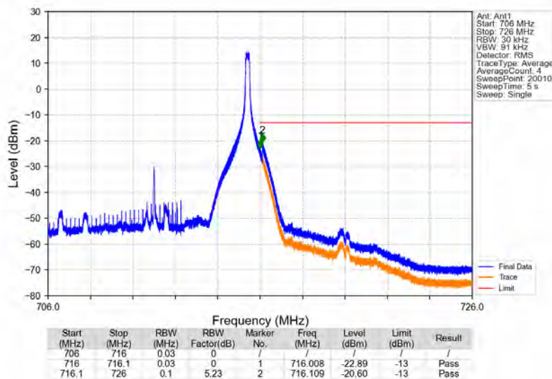
Band17_10MHz_64QAM_HCH_711MHz_RB_1_49_NTNV
