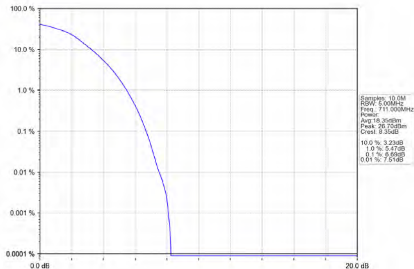
Band17_10MHz_64QAM_HCH_711MHz_RB_50_0_NTNV
