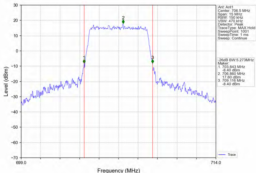
Band17_5MHz_16QAM_LCH_706.5MHz_RB_25_0_NTNV
