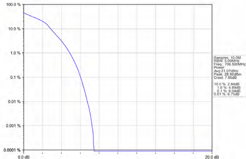
Band17_5MHz_16QAM_LCH_706.5MHz_RB_25_0_NTNV
