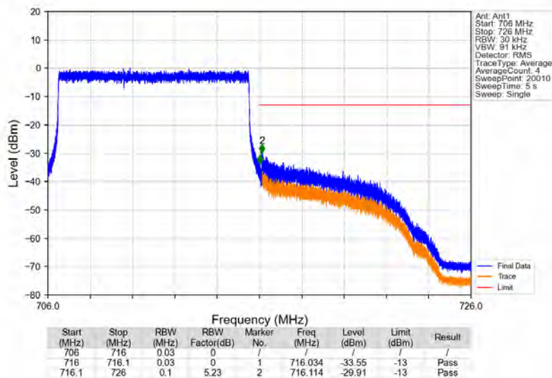
Band17_10MHz_QPSK_HCH_711MHz_RB_50_0_NTNV
