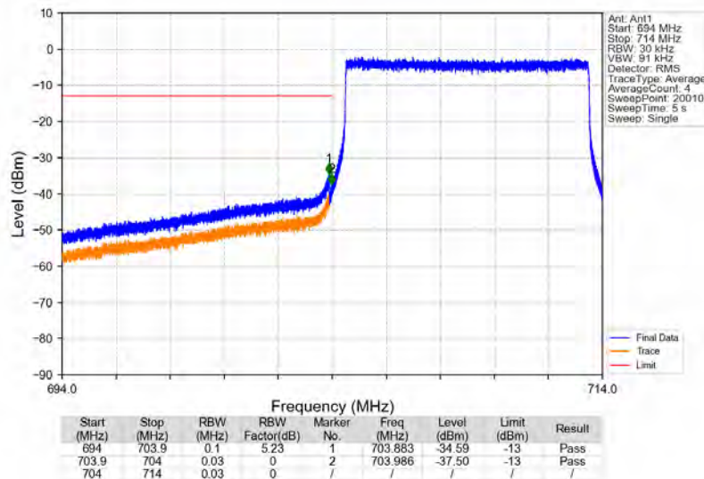
Band17_10MHz_64QAM_LCH_709MHz_RB_50_0_NTNV
