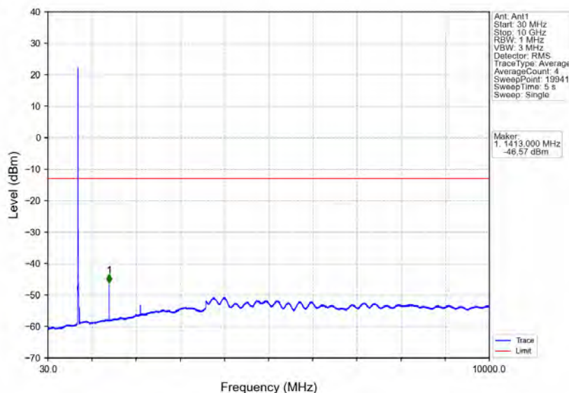
Band17_10MHz_QPSK_HCH_711MHz_RB_1_49_NTNV
