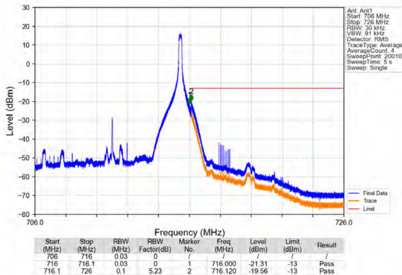
Band17_10MHz_QPSK_HCH_711MHz_RB_1_49_NTNV
