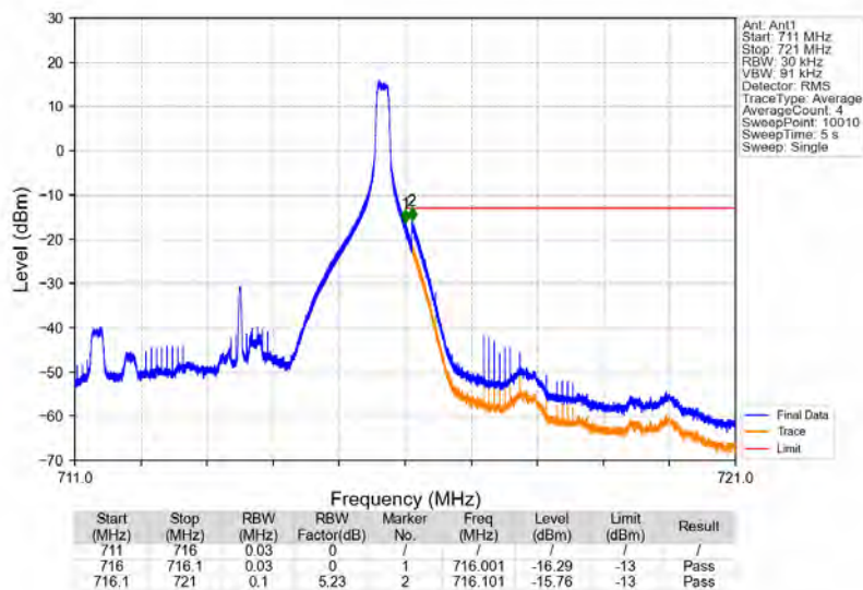
Band17_5MHz_QPSK_HCH_713.5MHz_RB_1_24_NTNV
