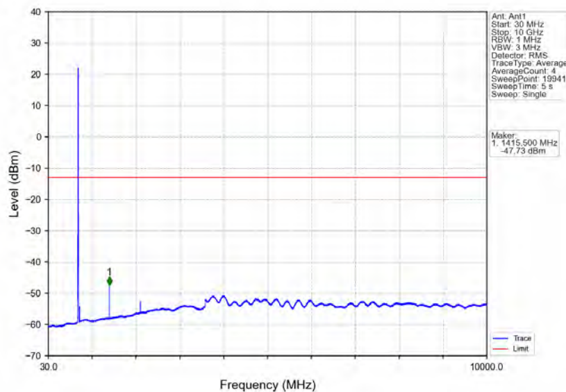
Band17_5MHz_QPSK_MCH_710MHz_RB_1_0_NTNV
