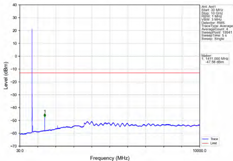
Band17_10MHz_16QAM_HCH_711MHz_RB_1_0_NTNV
