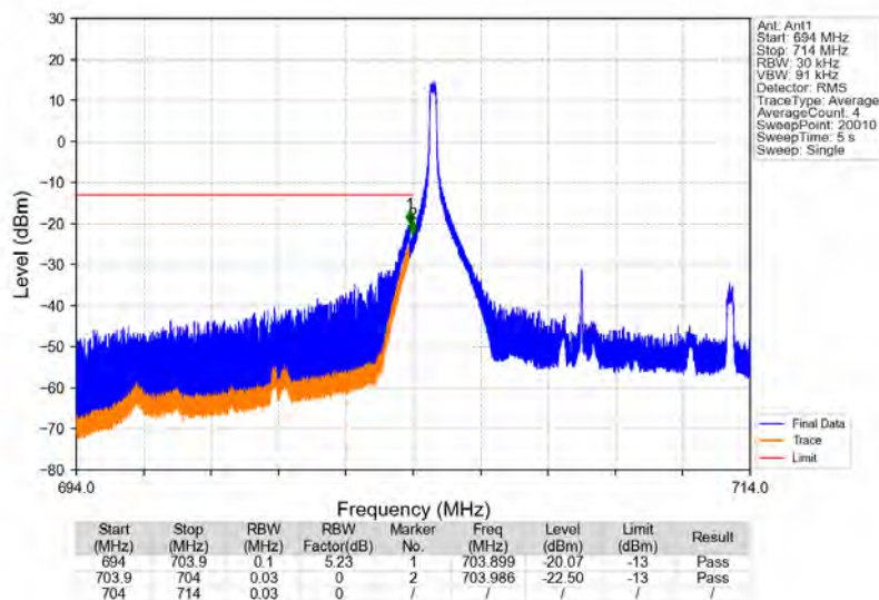
Band17_10MHz_64QAM_LCH_709MHz_RB_1_0_NTNV
