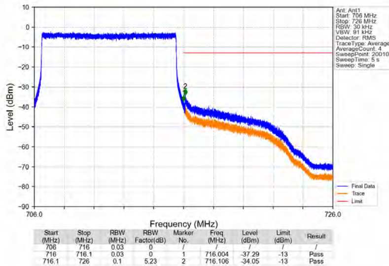
Band17_10MHz_64QAM_HCH_711MHz_RB_50_0_NTNV
