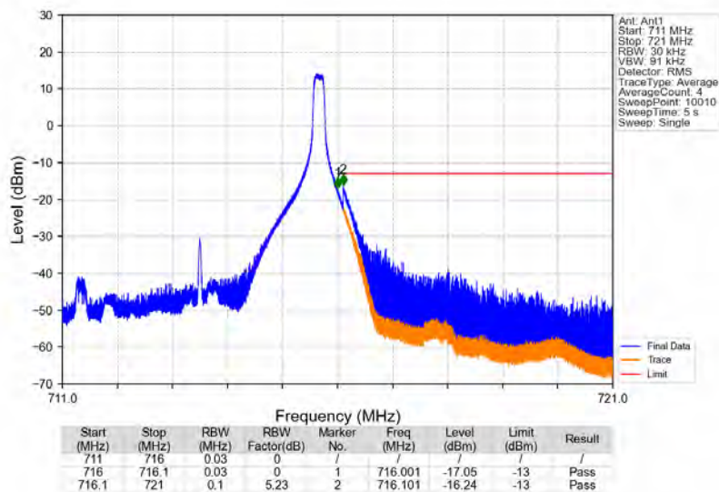
Band17_5MHz_64QAM_HCH_713.5MHz_RB_1_24_NTNV
