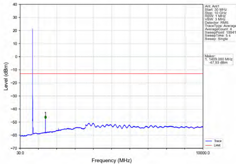
Band17_10MHz_16QAM_LCH_709MHz_RB_50_0_NTNV
