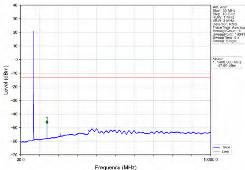
Band17_5MHz_16QAM_LCH_706.5MHz_RB_25_0_NTNV
