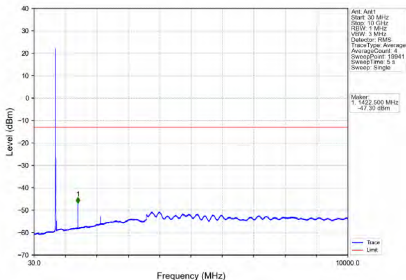
Band17_5MHz_QPSK_HCH_713.5MHz_RB_1_24_NTNV
