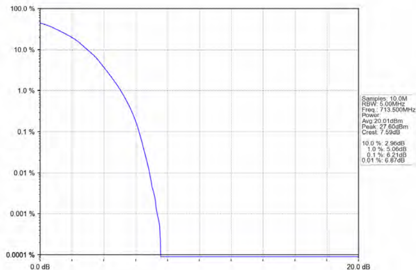
Band17_5MHz_64QAM_HCH_713.5MHz_RB_25_0_NTNV
