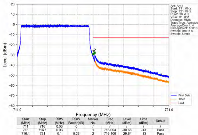
Band17_5MHz_64QAM_HCH_713.5MHz_RB_25_0_NTNV
