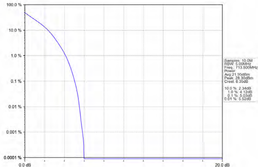
Band17_5MHz_QPSK_HCH_713.5MHz_RB_25_0_NTNV
