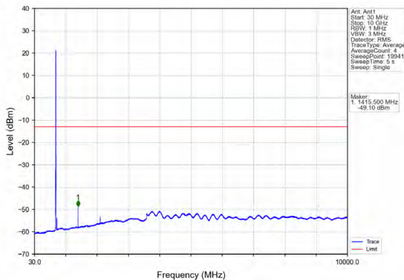
Band17_5MHz_16QAM_HCH_713.5MHz_RB_1_0_NTNV
