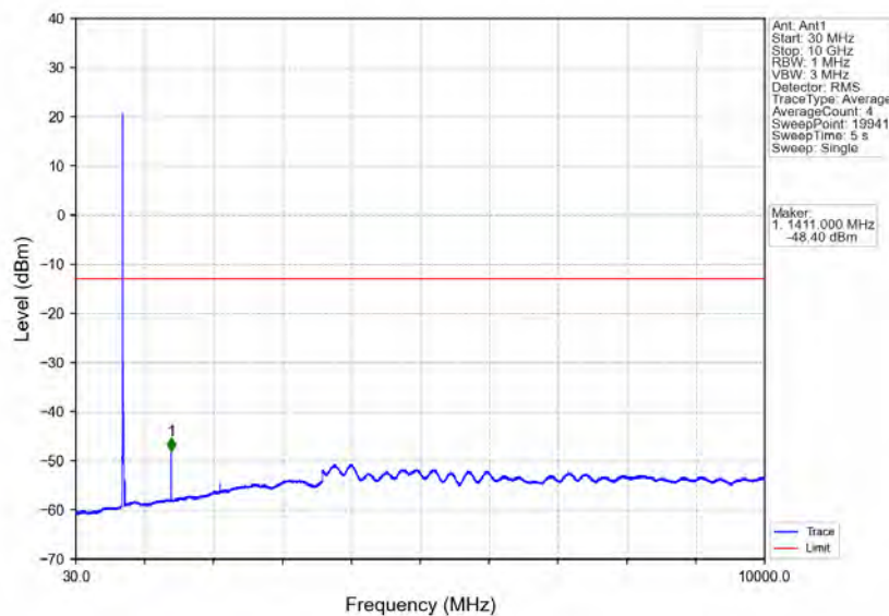
Band17_10MHz_64QAM_MCH_710MHz_RB_1_0_NTNV
