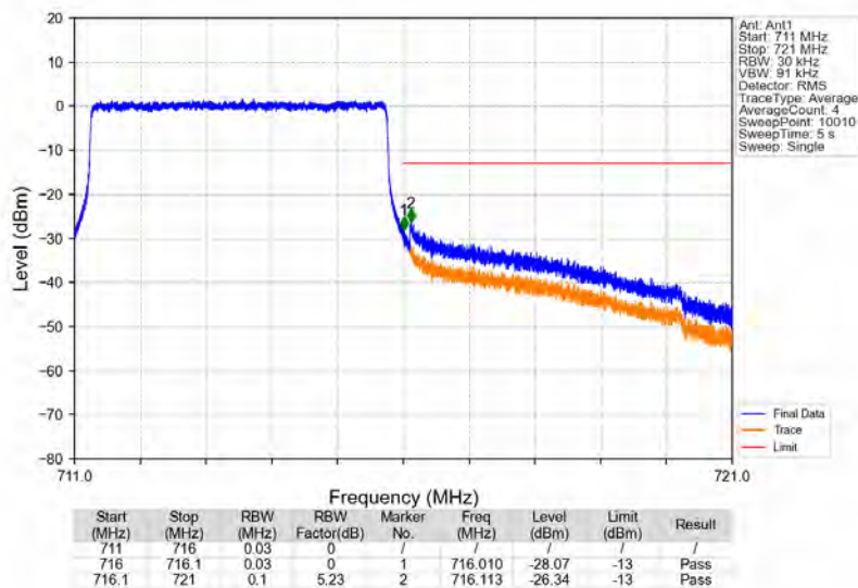
Band17_5MHz_QPSK_HCH_713.5MHz_RB_25_0_NTNV
