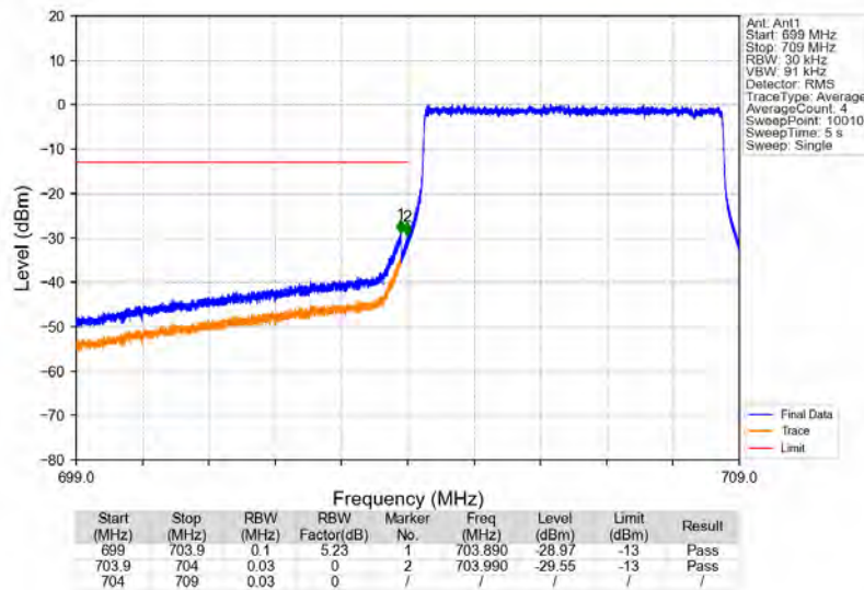
Band17_5MHz_64QAM_LCH_706.5MHz_RB_25_0_NTNV
