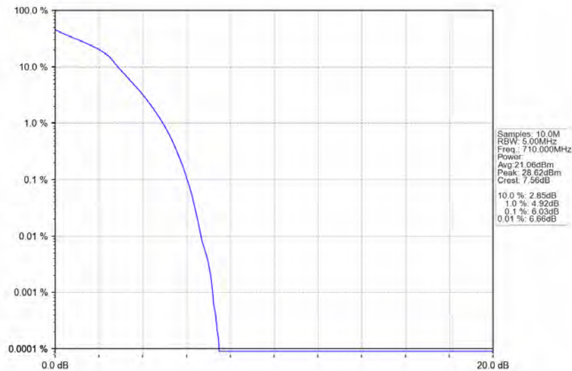
Band17_5MHz_16QAM_MCH_710MHz_RB_25_0_NTNV
