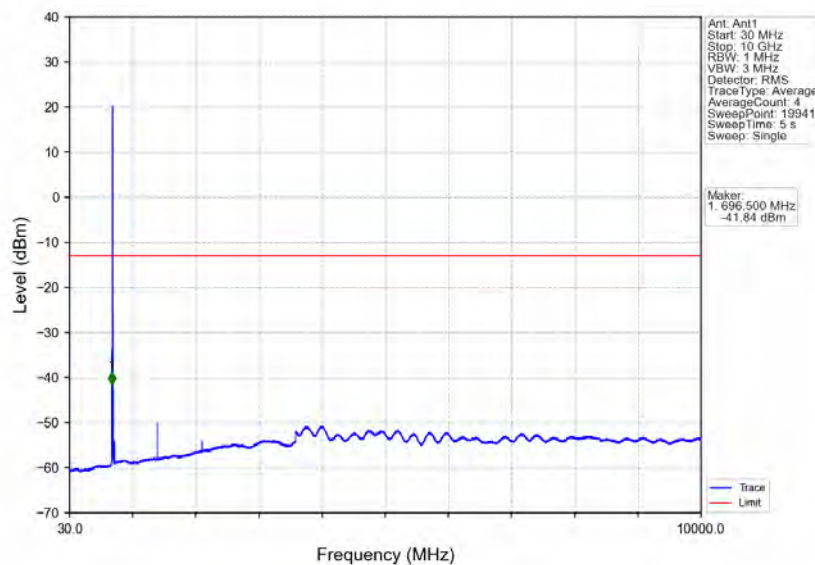
Band17_5MHz_64QAM_MCH_710MHz_RB_1_0_NTNV
