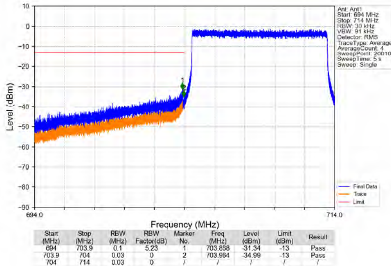
Band17_10MHz_16QAM_LCH_709MHz_RB_50_0_NTNV
