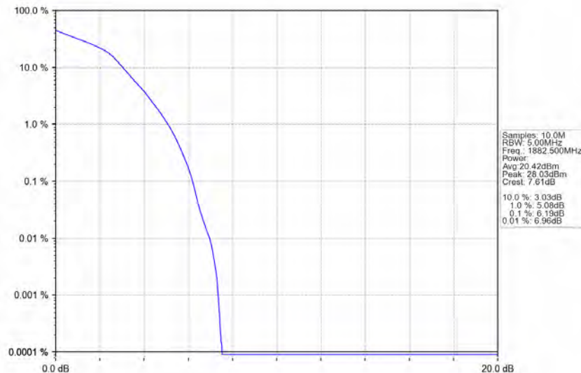
Band25_1.4MHz_16QAM_MCH_1882.5MHz_RB_6_0_NTNV
