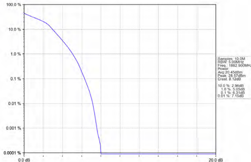
Band25_3MHz_16QAM_MCH_1882.5MHz_RB_15_0_NTNV
