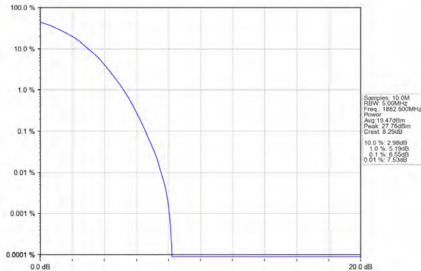
Band25_5MHz_64QAM_MCH_1882.5MHz_RB_25_0_NTNV
