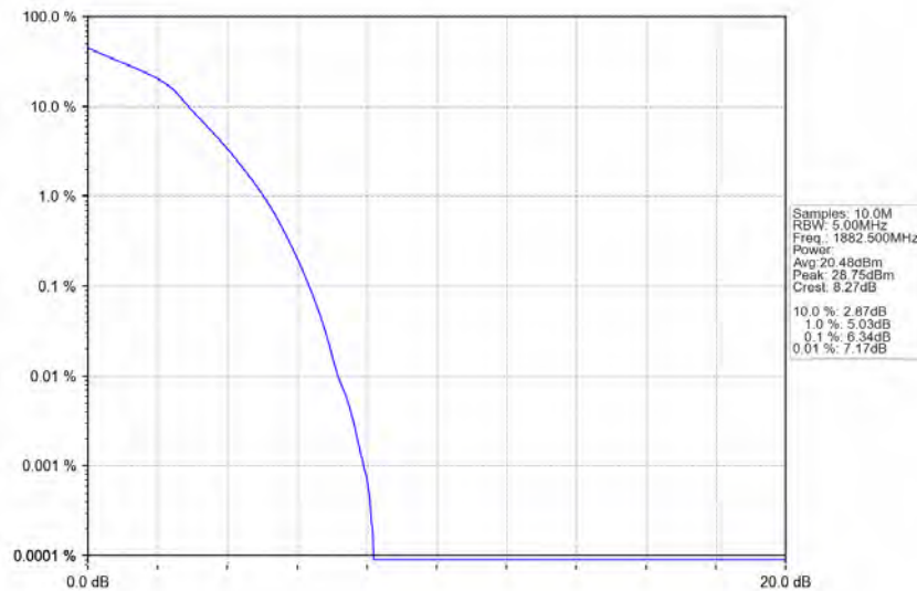
Band25_5MHz_16QAM_MCH_1882.5MHz_RB_25_0_NTNV
