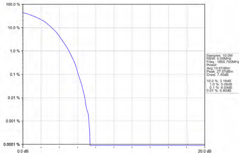
Band25_1.4MHz_64QAM_LCH_1850.7MHz_RB_6_0_NTNV
