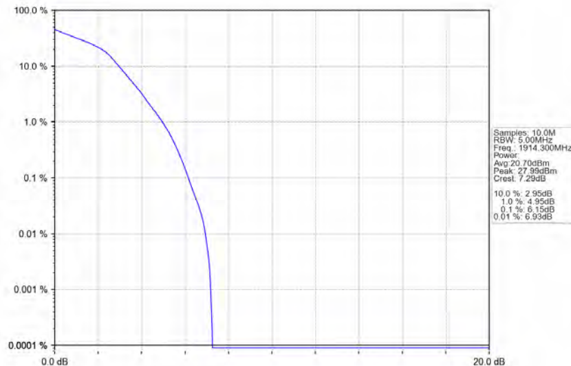
Band25_1.4MHz_16QAM_HCH_1914.3MHz_RB_6_0_NTNV
