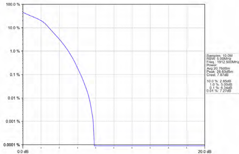
Band25_5MHz_16QAM_HCH_1912.5MHz_RB_25_0_NTNV
