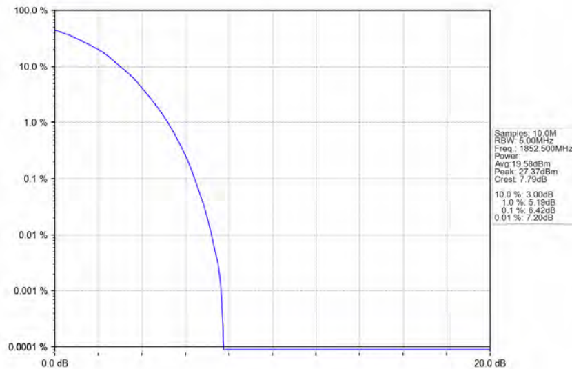
Band25_5MHz_64QAM_LCH_1852.5MHz_RB_25_0_NTNV
