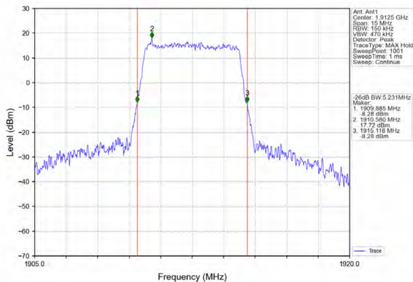
Band25_5MHz_16QAM_HCH_1912.5MHz_RB_25_0_NTNV
