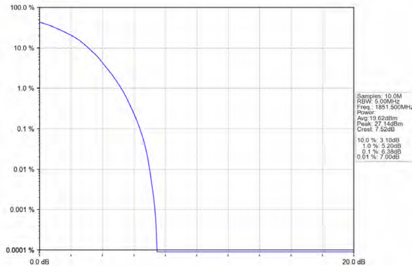
Band25_3MHz_64QAM_LCH_1851.5MHz_RB_15_0_NTNV
