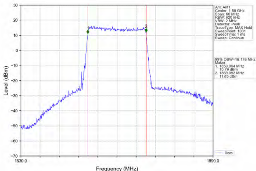
Band25_20MHz_64QAM_LCH_1860MHz_RB_100_0_NTNV
