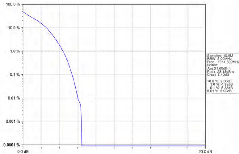
Band25_1.4MHz_QPSK_HCH_1914.3MHz_RB_6_0_NTNV
