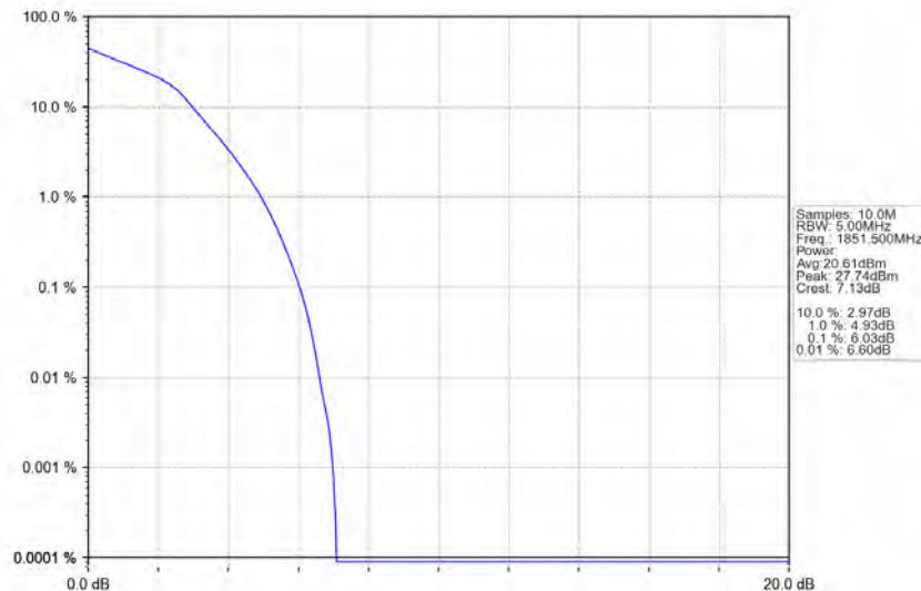
Band25_3MHz_16QAM_LCH_1851.5MHz_RB_15_0_NTNV
