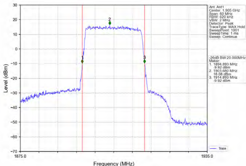
Band25_20MHz_64QAM_HCH_1905MHz_RB_100_0_NTNV
