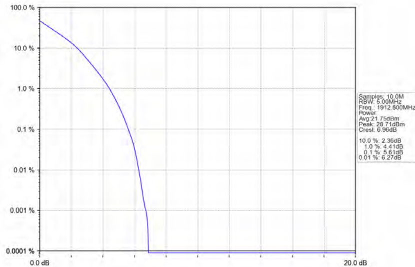
Band25_5MHz_QPSK_HCH_1912.5MHz_RB_25_0_NTNV
