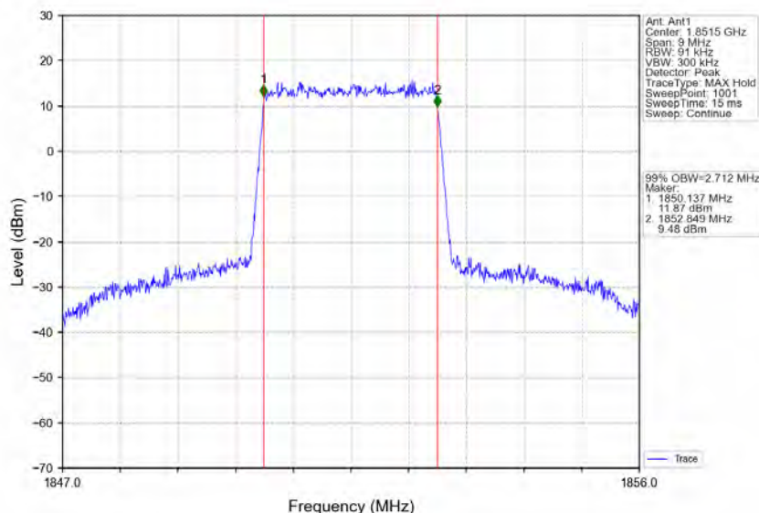
Band25_3MHz_64QAM_LCH_1851.5MHz_RB_15_0_NTNV
