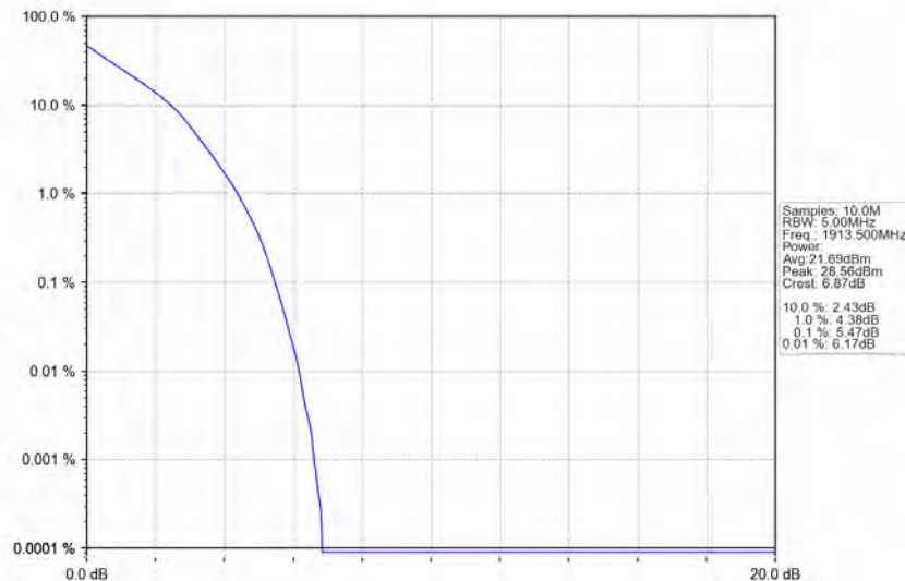
Band25_3MHz_QPSK_HCH_1913.5MHz_RB_15_0_NTNV
