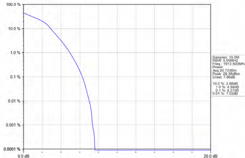
Band25_3MHz_16QAM_HCH_1913.5MHz_RB_15_0_NTNV
