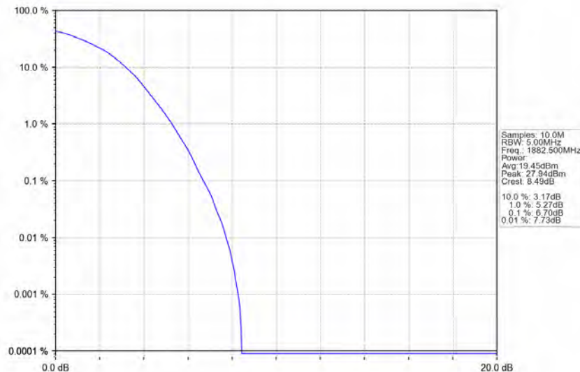
Band25_1.4MHz_64QAM_MCH_1882.5MHz_RB_6_0_NTNV
