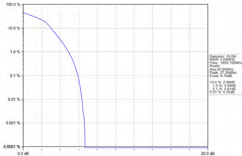
Band25_1.4MHz_16QAM_LCH_1850.7MHz_RB_6_0_NTNV
