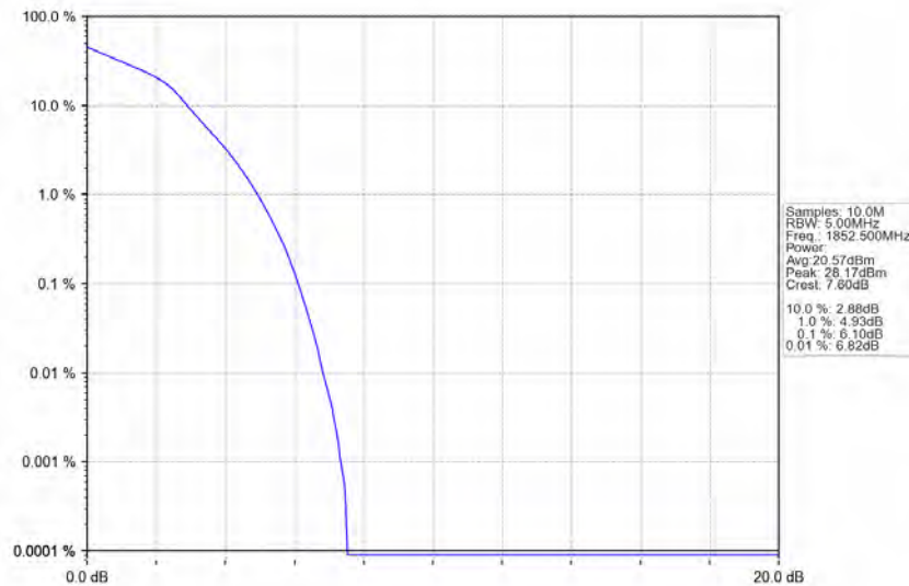
Band25_5MHz_16QAM_LCH_1852.5MHz_RB_25_0_NTNV
