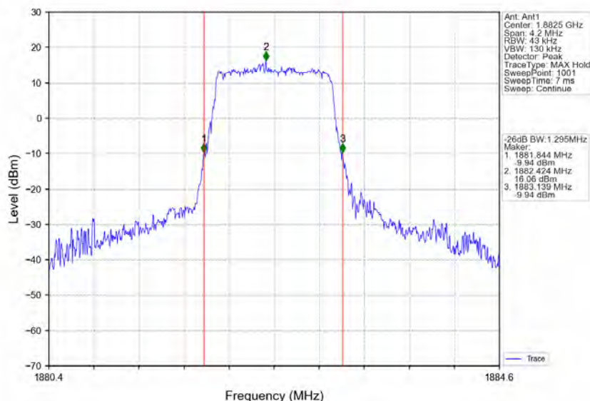
Band25_1.4MHz_64QAM_MCH_1882.5MHz_RB_6_0_NTNV
