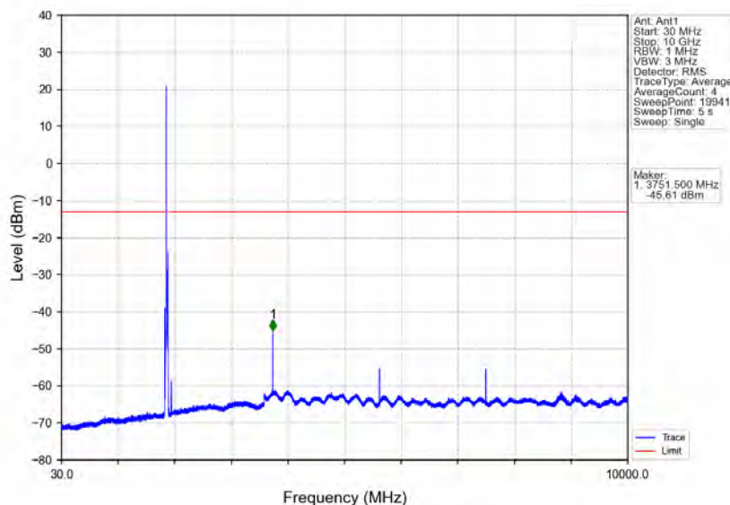
Band25_15MHz_16QAM_MCH_1882.5MHz_RB_1_0_NTNV
