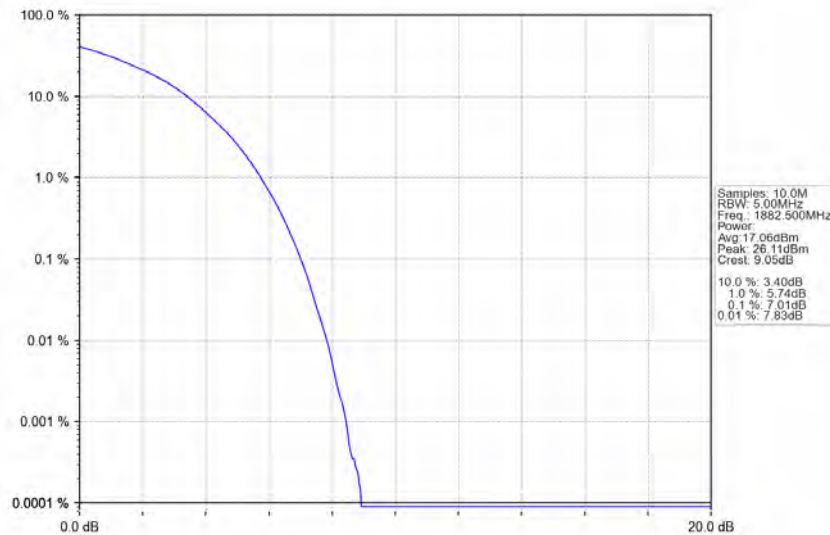
Band25_15MHz_16QAM_MCH_1882.5MHz_RB_75_0_NTNV
