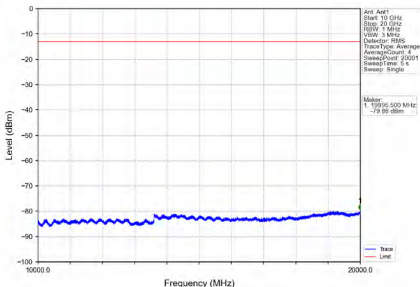
Band25_5MHz_QPSK_MCH_1882.5MHz_RB_1_0_NTNV
