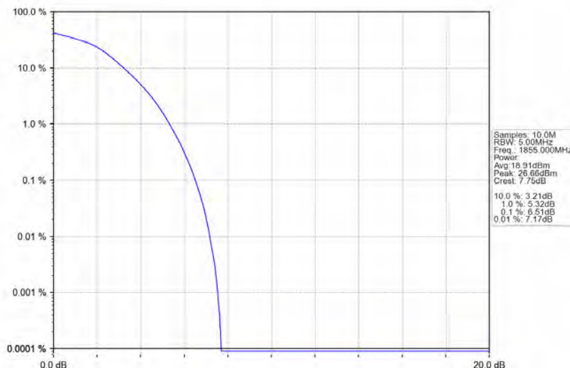
Band25_10MHz_16QAM_LCH_1855MHz_RB_50_0_NTNV
