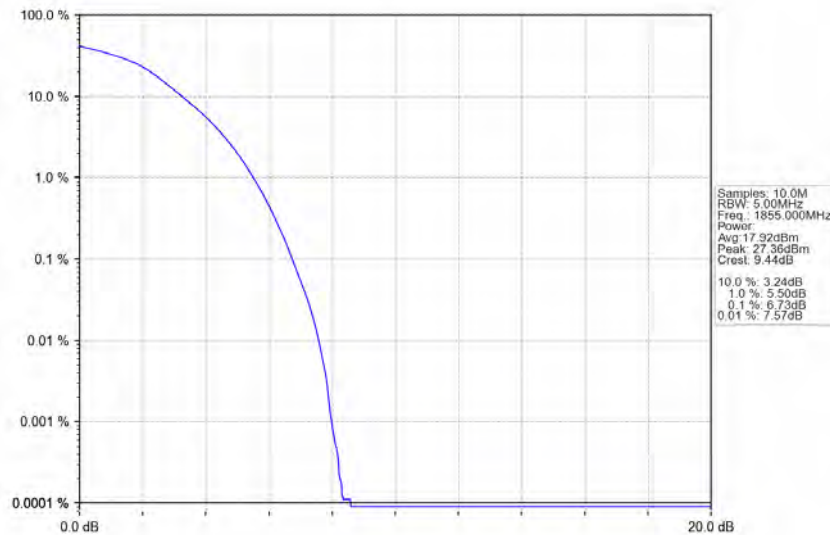
Band25_10MHz_64QAM_LCH_1855MHz_RB_50_0_NTNV
