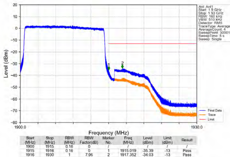
Band25_15MHz_64QAM_HCH_1907.5MHz_RB_75_0_NTNV
