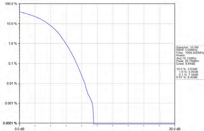
Band25_20MHz_16QAM_HCH_1905MHz_RB_100_0_NTNV
