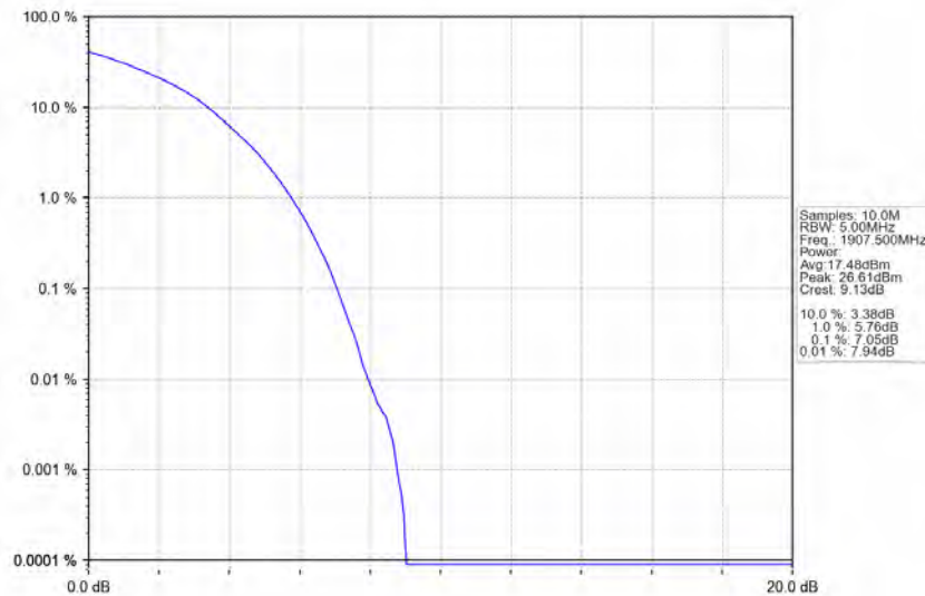
Band25_15MHz_16QAM_HCH_1907.5MHz_RB_75_0_NTNV
