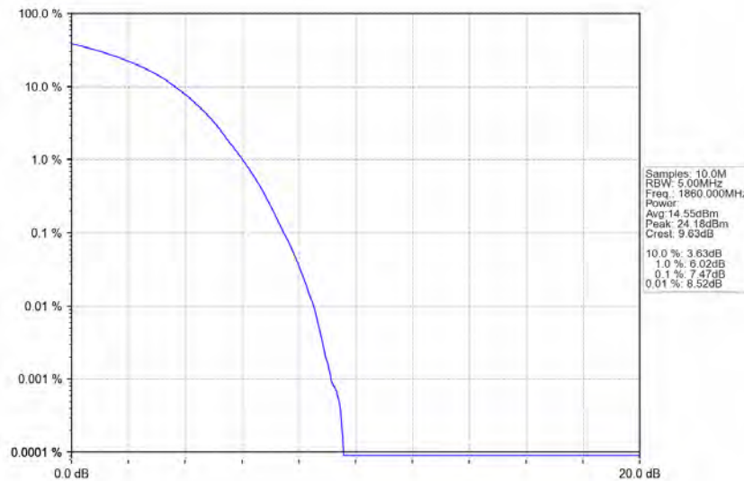
Band25_20MHz_64QAM_LCH_1860MHz_RB_100_0_NTNV
