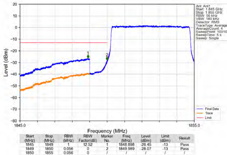
Band25_5MHz_64QAM_LCH_1852.5MHz_RB_25_0_NTNV
