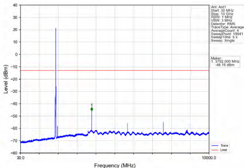
Band25_20MHz_16QAM_HCH_1905MHz_RB_1_0_NTNV
