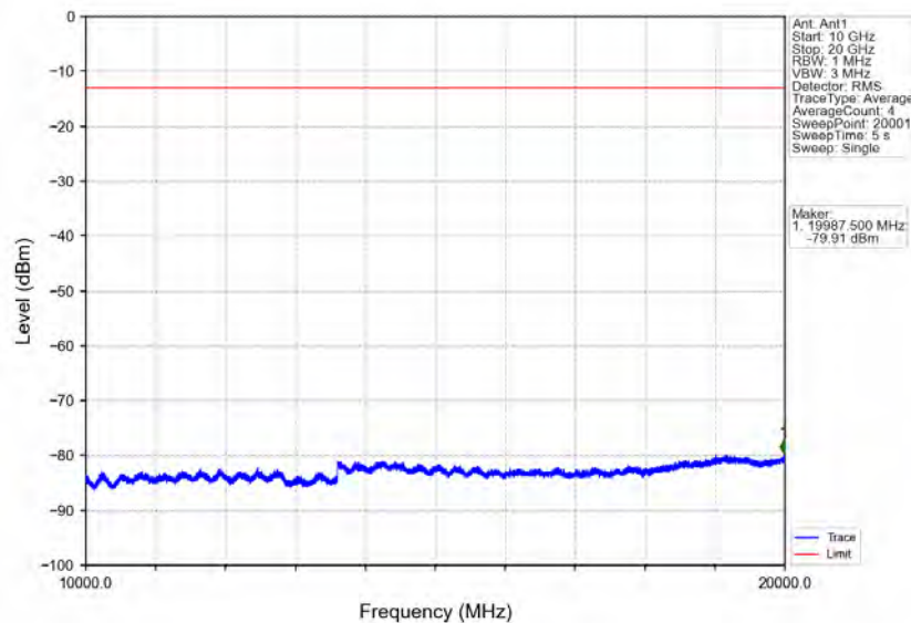
Band25_15MHz_16QAM_LCH_1857.5MHz_RB_75_0_NTNV
