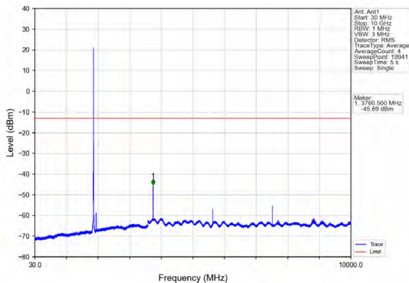
Band25_5MHz_16QAM_MCH_1882.5MHz_RB_1_0_NTNV
