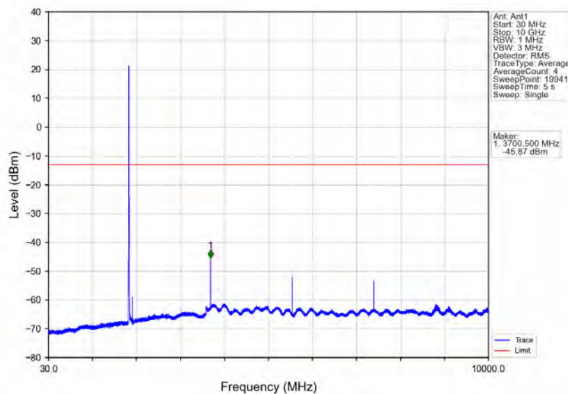
Band25_5MHz_16QAM_LCH_1852.5MHz_RB_1_0_NTNV
