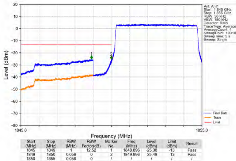
Band25_5MHz_QPSK_LCH_1852.5MHz_RB_25_0_NTNV
