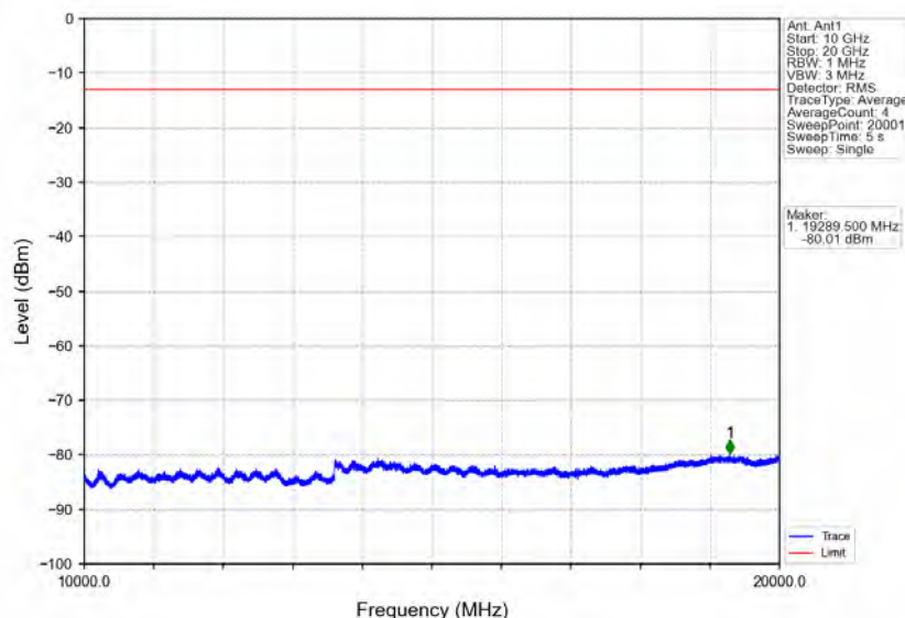
Band25_15MHz_16QAM_MCH_1882.5MHz_RB_1_0_NTNV
