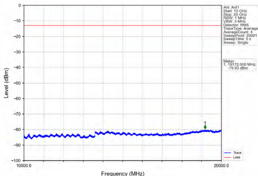
Band25_3MHz_QPSK_HCH_1913.5MHz_RB_1_0_NTNV
