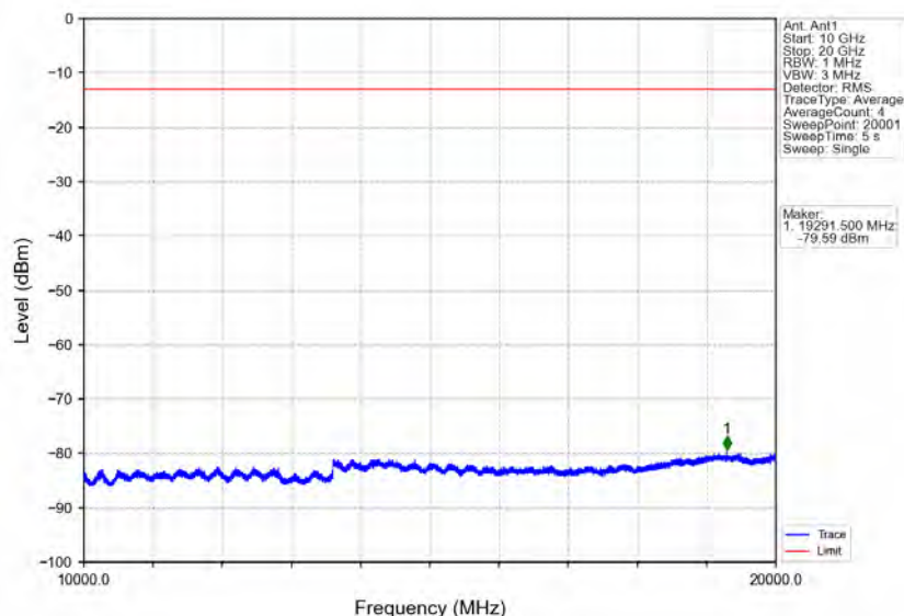
Band25_15MHz_16QAM_HCH_1907.5MHz_RB_1_0_NTNV
