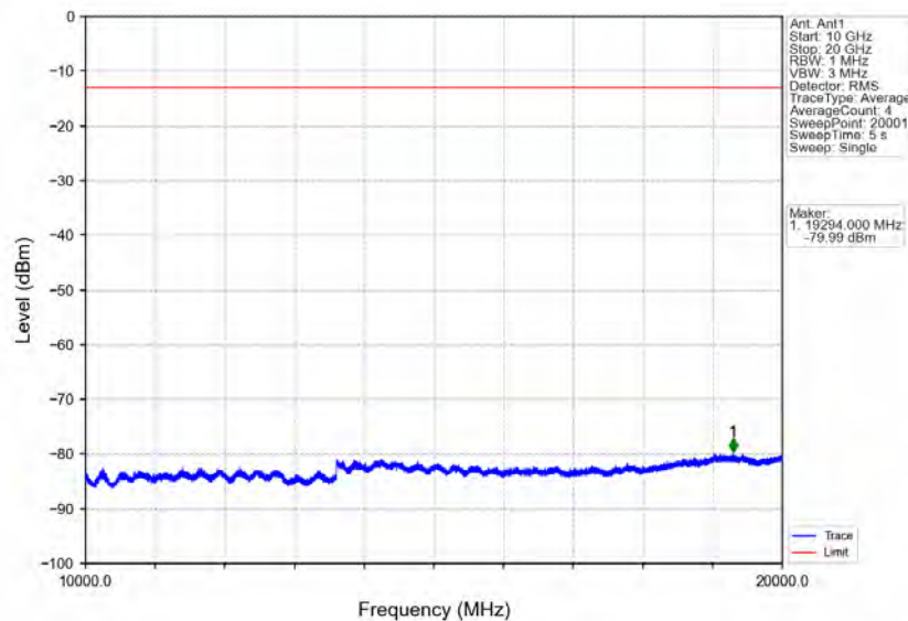
Band25_15MHz_64QAM_LCH_1857.5MHz_RB_75_0_NTNV
