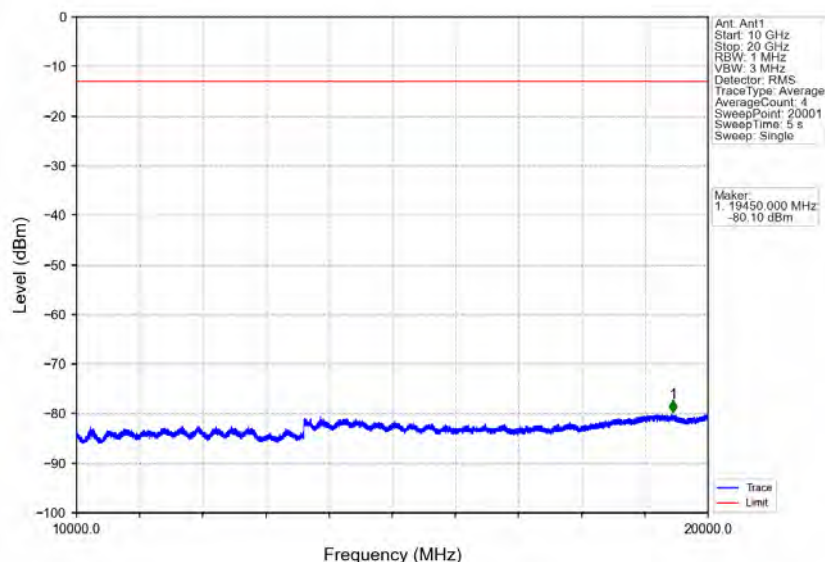
Band25_20MHz_16QAM_HCH_1905MHz_RB_1_0_NTNV
