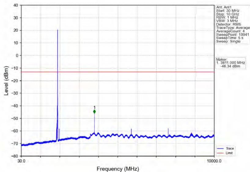
Band25_10MHz_64QAM_HCH_1910MHz_RB_1_0_NTNV
