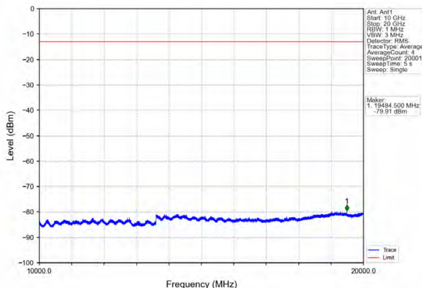
Band25_20MHz_64QAM_MCH_1882.5MHz_RB_1_0_NTNV
