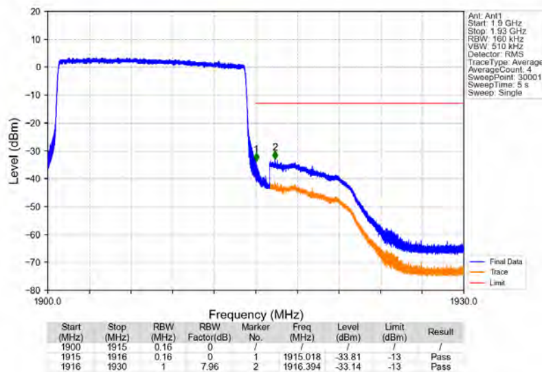
Band25_15MHz_16QAM_HCH_1907.5MHz_RB_75_0_NTNV
