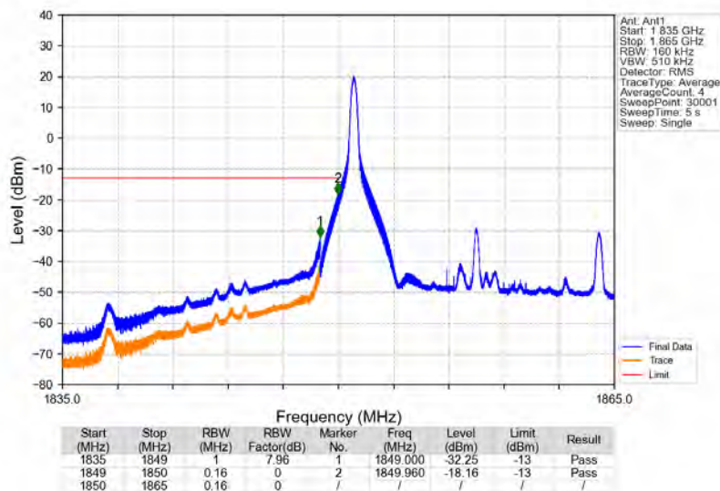
Band25_15MHz_64QAM_LCH_1857.5MHz_RB_1_0_NTNV
