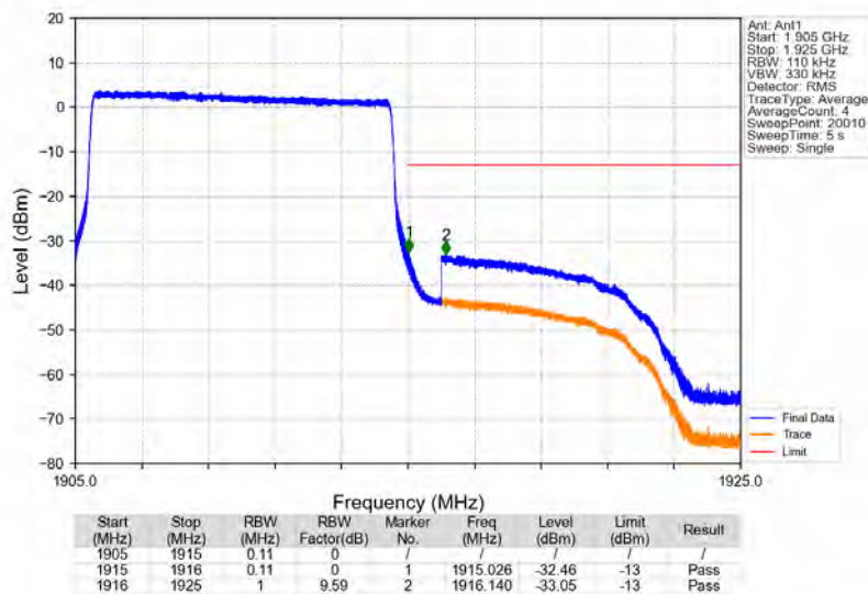
Band25_10MHz_16QAM_HCH_1910MHz_RB_50_0_NTNV
