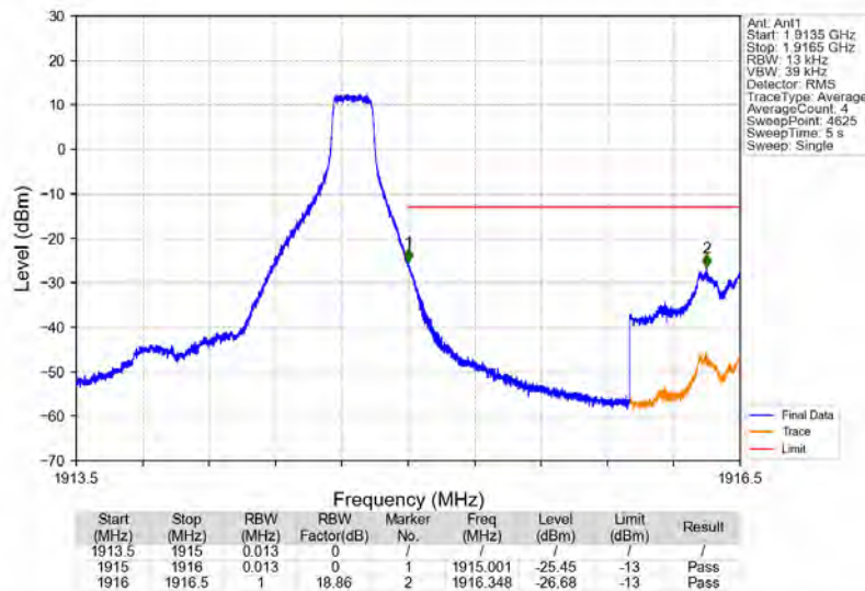
Band25_1.4MHz_QPSK_HCH_1914.3MHz_RB_1_5_NTNV
