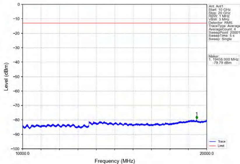
Band25_5MHz_64QAM_LCH_1852.5MHz_RB_25_0_NTNV
