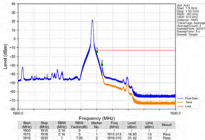
Band25_15MHz_QPSK_HCH_1907.5MHz_RB_1_74_NTNV
