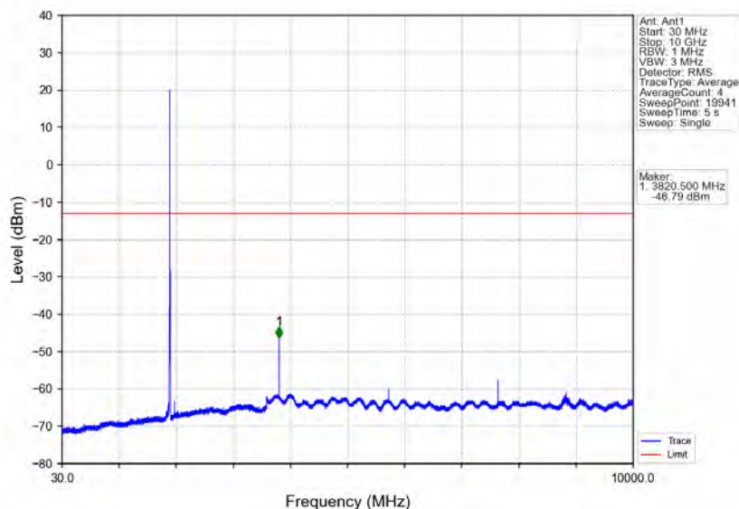
Band25_5MHz_64QAM_HCH_1912.5MHz_RB_1_0_NTNV
