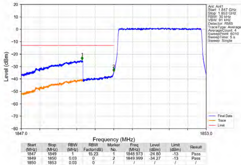
Band25_3MHz_64QAM_LCH_1851.5MHz_RB_15_0_NTNV
