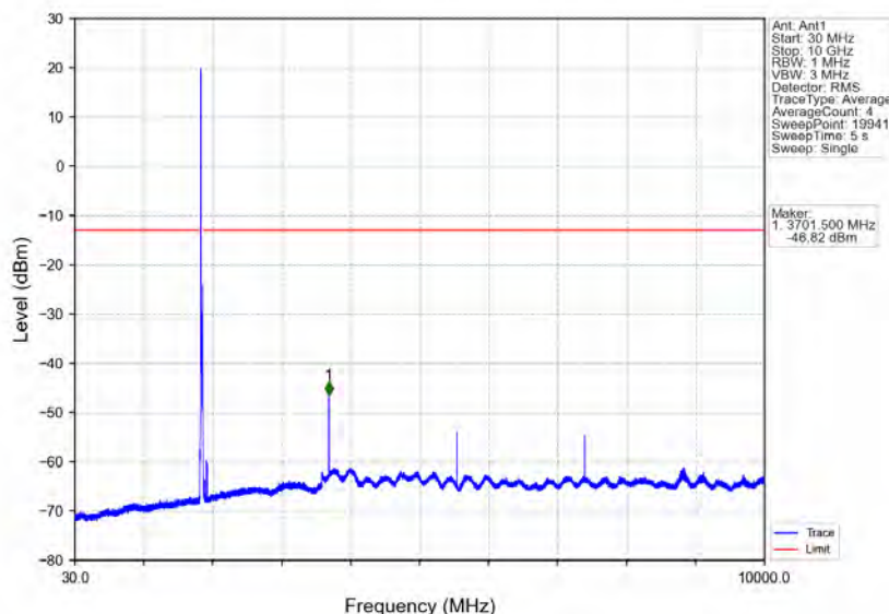
Band25_15MHz_64QAM_LCH_1857.5MHz_RB_1_0_NTNV
