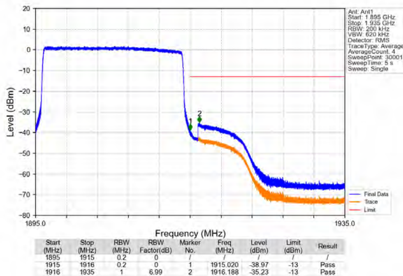
Band25_20MHz_64QAM_HCH_1905MHz_RB_100_0_NTNV
