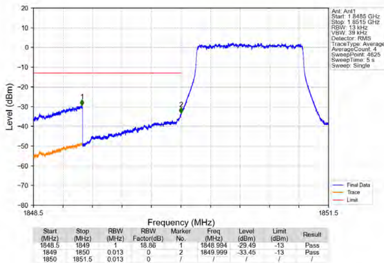
Band25 1.4MHz 64QAM LCH 1850.7MHz RB 6 0 NTN
