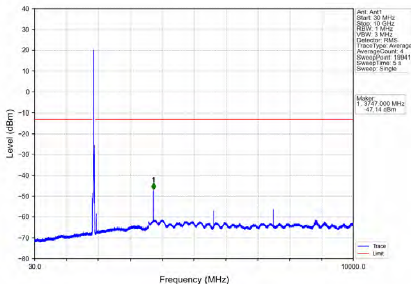
Band25_20MHz_64QAM_MCH_1882.5MHz_RB_1_0_NTNV
