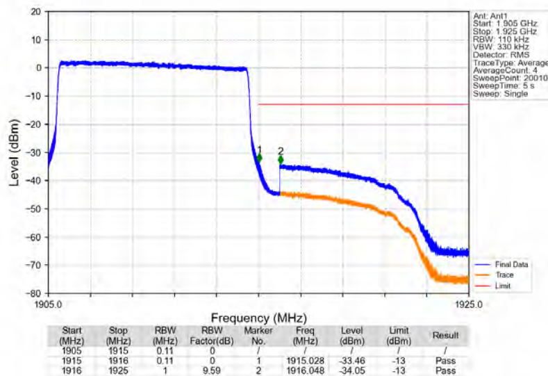
Band25_10MHz_64QAM_HCH_1910MHz_RB_50_0_NTNV
