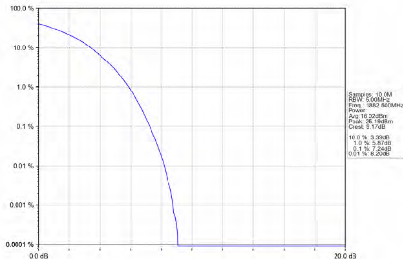
Band25_15MHz_64QAM_MCH_1882.5MHz_RB_75_0_NTNV
