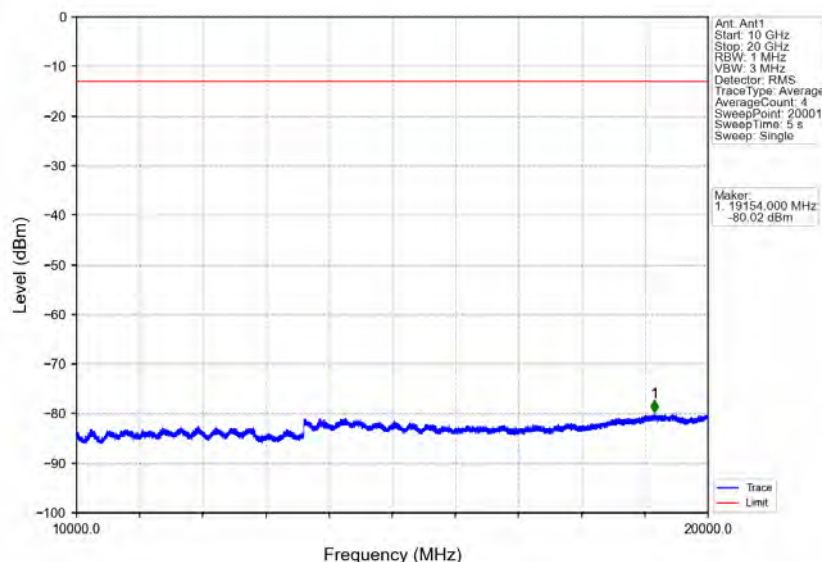
Band25_1.4MHz_QPSK_HCH_1914.3MHz_RB_1_0_NTNV
