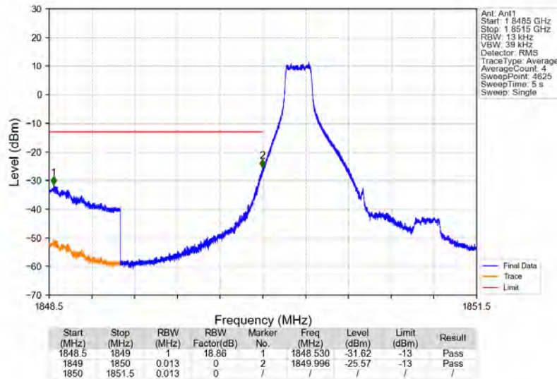
Band25 1.4MHz 64QAM LCH 1850.7MHz RB 1 0 NTN
