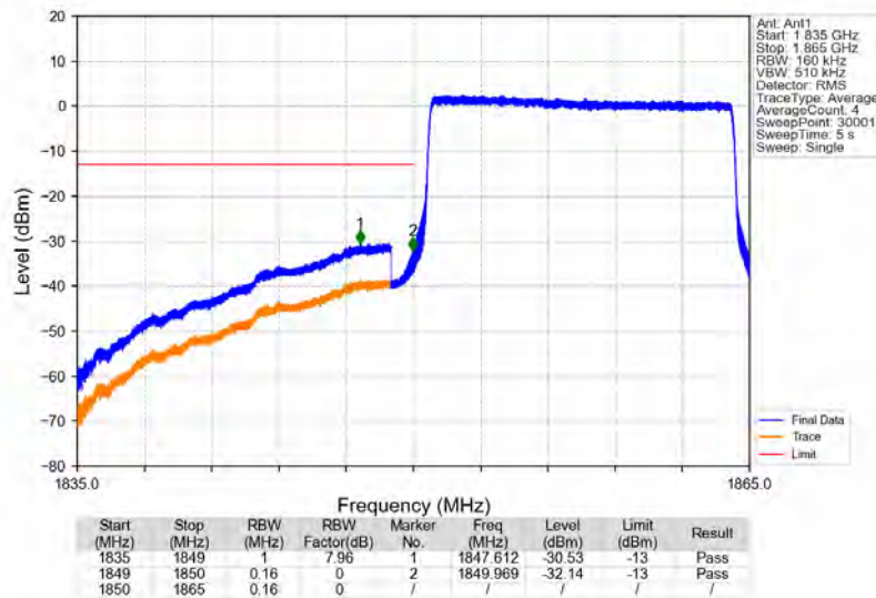
Band25_15MHz_64QAM_LCH_1857.5MHz_RB_75_0_NTNV
