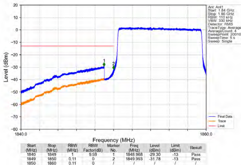
Band25_10MHz_64QAM_LCH_1855MHz_RB_50_0_NTNV
