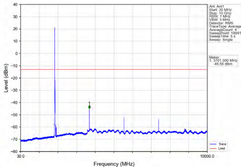
Band25_15MHz_16QAM_LCH_1857.5MHz_RB_1_0_NTNV
