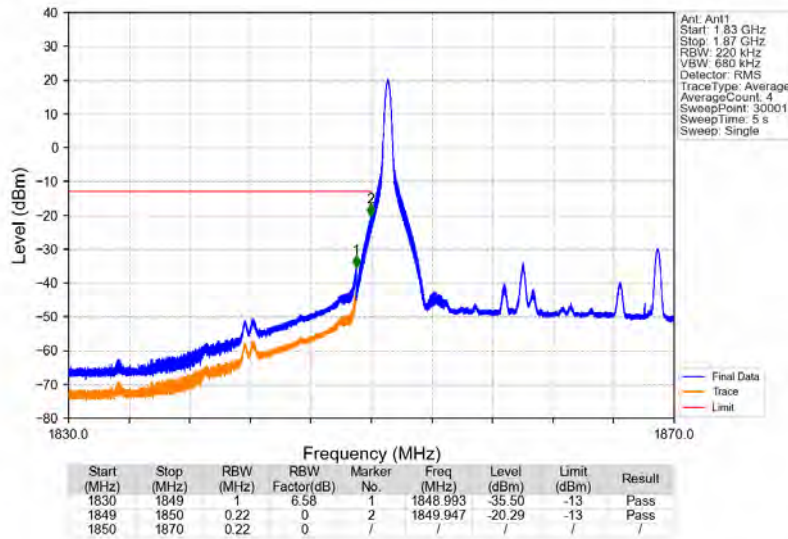
Band25_20MHz_64QAM_LCH_1860MHz_RB_1_0_NTNV
