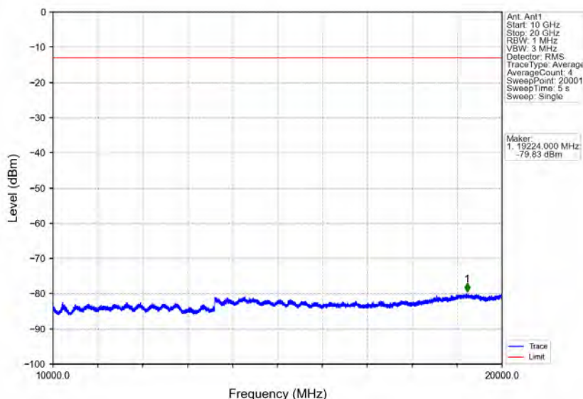
Band25_10MHz_16QAM_HCH_1910MHz_RB_1_0_NTNV
