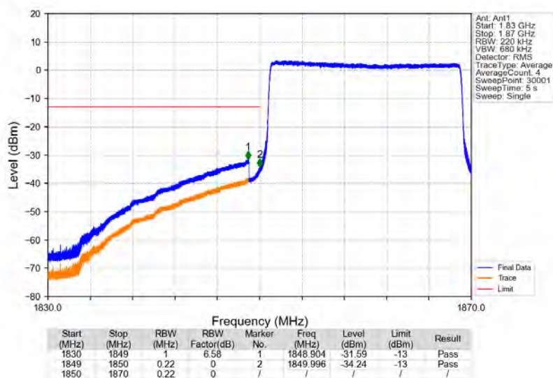
Band25_20MHz_16QAM_LCH_1860MHz_RB_100_0_NTNV
