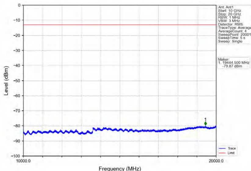
Band25_15MHz_QPSK_MCH_1882.5MHz_RB_1_0_NTNV
