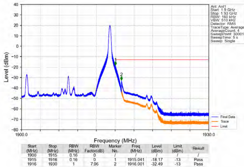
Band25_15MHz_64QAM_HCH_1907.5MHz_RB_1_74_NTNV
