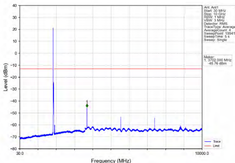
Band25_20MHz_16QAM_LCH_1860MHz_RB_1_0_NTNV
