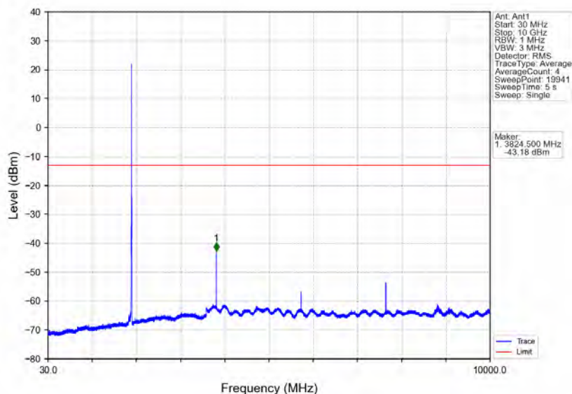
Band25_3MHz_QPSK_HCH_1913.5MHz_RB_1_0_NTNV
