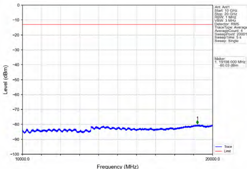
Band25_3MHz_64QAM_HCH_1913.5MHz_RB_1_0_NTNV
