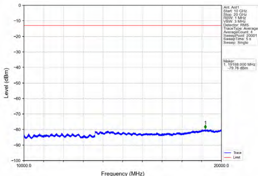
Band25_3MHz_64QAM_MCH_1882.5MHz_RB_1_0_NTNV
