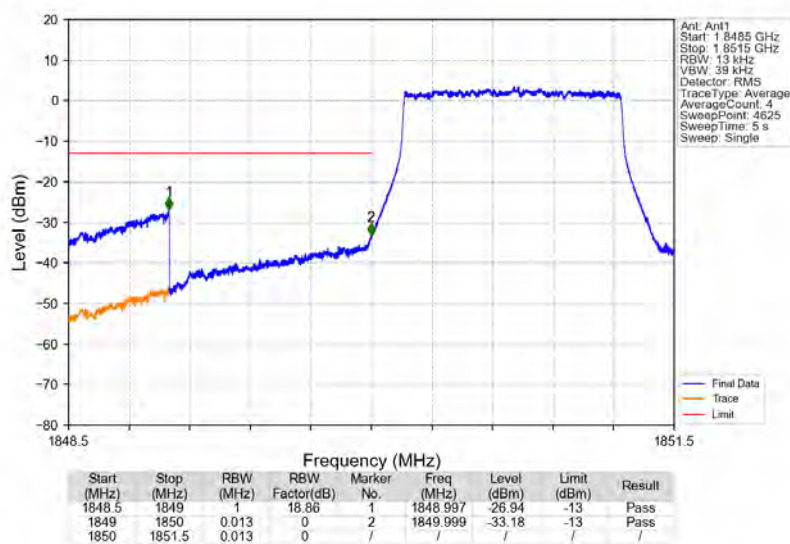
Band25 1.4MHz 16QAM LCH 1850.7MHz RB 6 0 NTN
