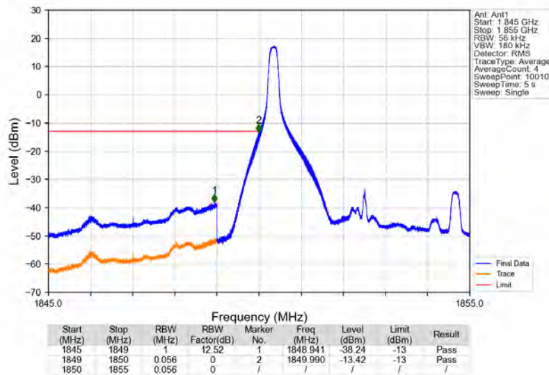
Band25_5MHz_16QAM_LCH_1852.5MHz_RB_1_0_NTNV
