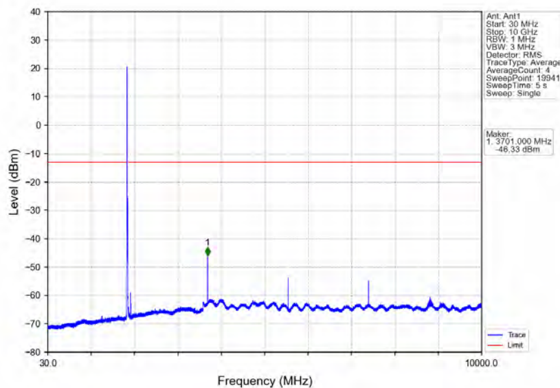
Band25_10MHz_64QAM_LCH_1855MHz_RB_1_0_NTNV
