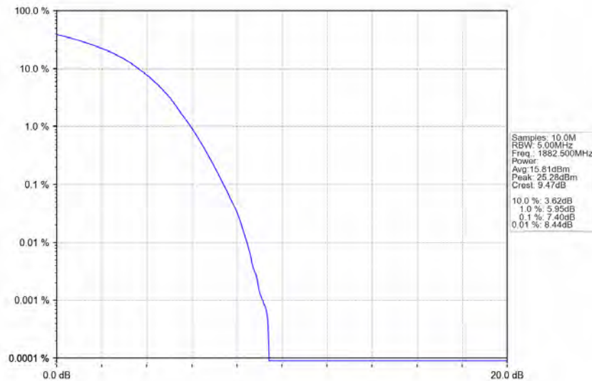
Band25_20MHz_16QAM_MCH_1882.5MHz_RB_100_0_NTNV
