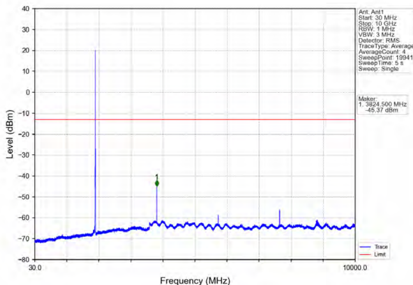
Band25_3MHz_64QAM_HCH_1913.5MHz_RB_1_0_NTNV
