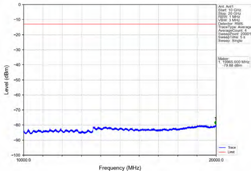
Band25_10MHz_16QAM_LCH_1855MHz_RB_50_0_NTNV
