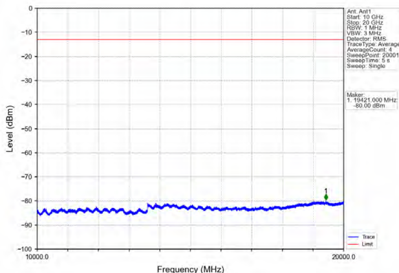
Band25_3MHz_16QAM_HCH_1913.5MHz_RB_1_0_NTNV
