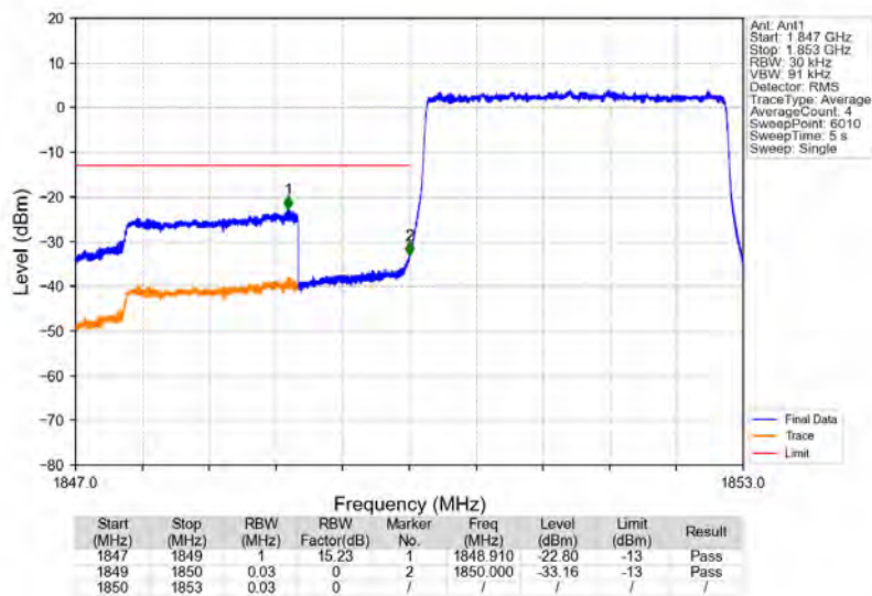
Band25_3MHz_QPSK_LCH_1851.5MHz_RB_15_0_NTNV
