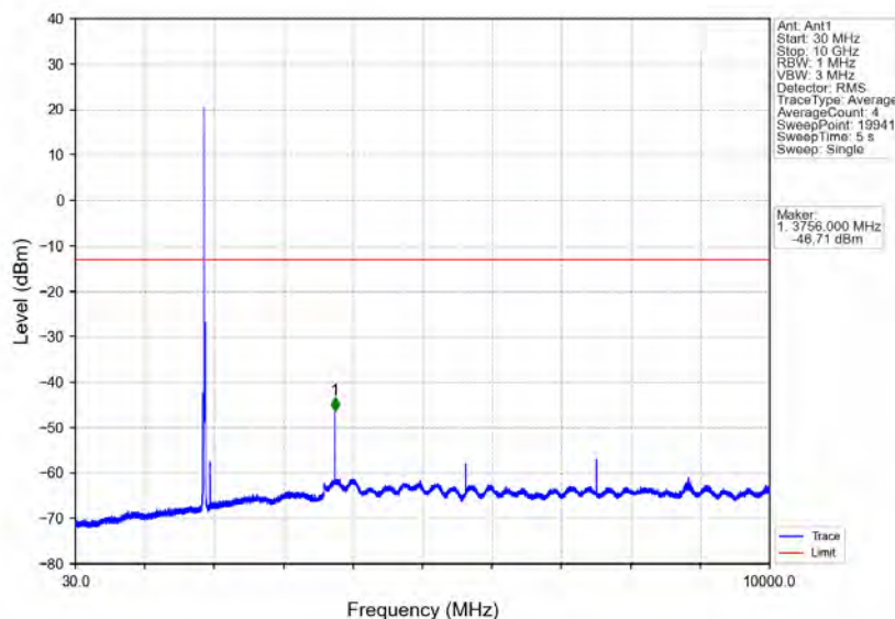
Band25_10MHz_64QAM_MCH_1882.5MHz_RB_1_0_NTNV
