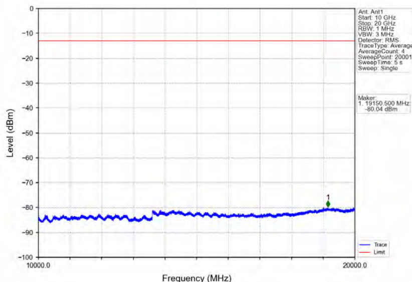
Band25_1.4MHz_16QAM_MCH_1882.5MHz_RB_1_0_NTNV
