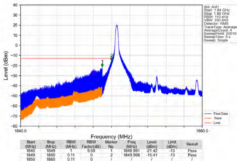
Band25_10MHz_16QAM_LCH_1855MHz_RB_1_0_NTNV
