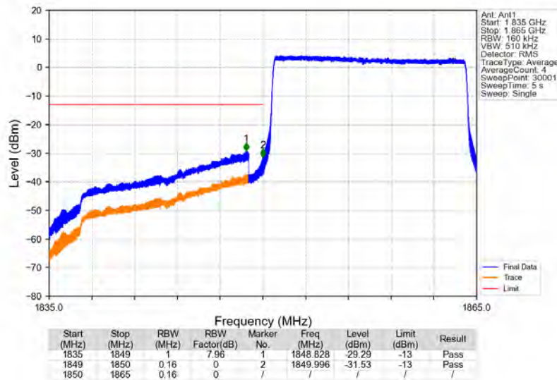
Band25_15MHz_QPSK_LCH_1857.5MHz_RB_75_0_NTNV
