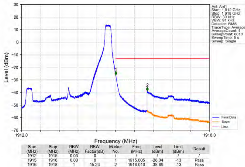
Band25_3MHz_64QAM_HCH_1913.5MHz_RB_1_14_NTNV
