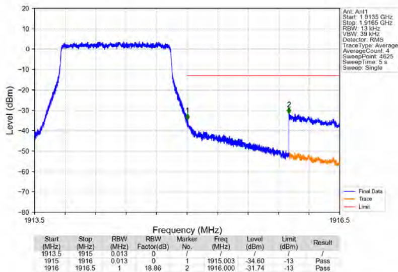
Band25 1.4MHz 16QAM HCH 1914.3MHz RB 6 0 NTNV
