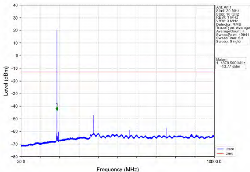
Band25_1.4MHz_64QAM_MCH_1882.5MHz_RB_1_0_NTNV
