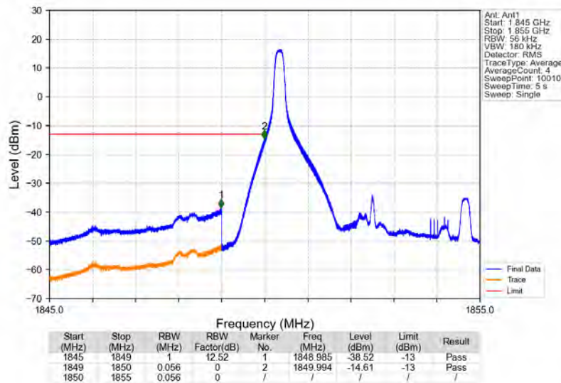
Band25_5MHz_64QAM_LCH_1852.5MHz_RB_1_0_NTNV
