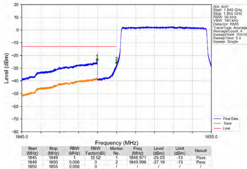
Band25_5MHz_16QAM_LCH_1852.5MHz_RB_25_0_NTNV
