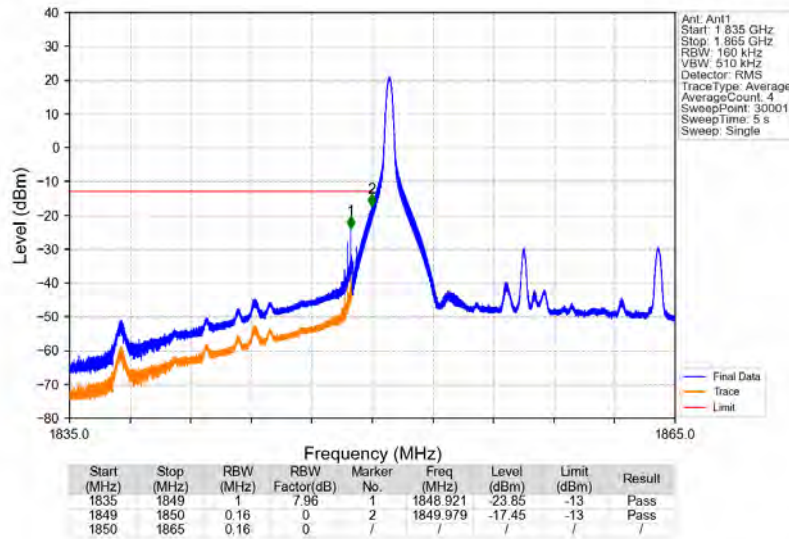
Band25_15MHz_16QAM_LCH_1857.5MHz_RB_1_0_NTNV
