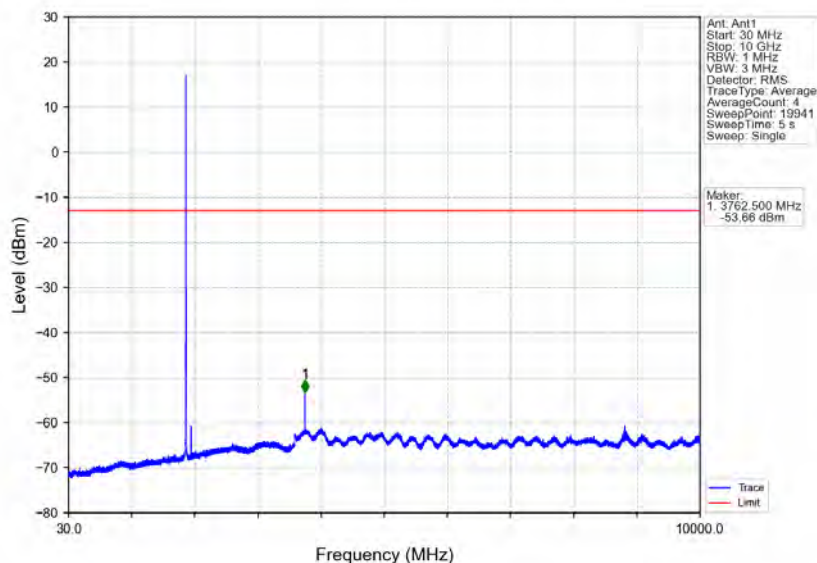
Band25_3MHz_64QAM_MCH_1882.5MHz_RB_1_0_NTNV
