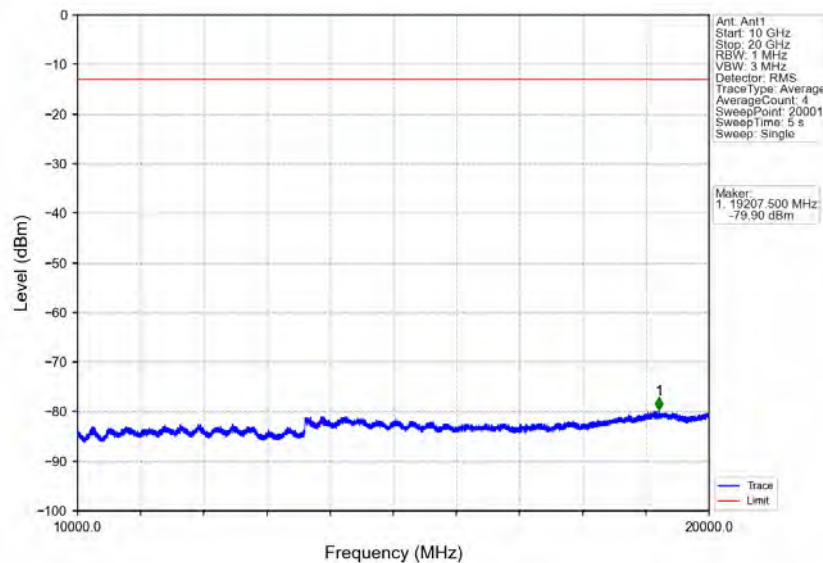
Band25_5MHz_QPSK_LCH_1852.5MHz_RB_25_0_NTNV
