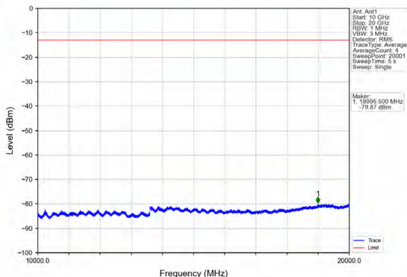
Band25_15MHz_64QAM_HCH_1907.5MHz_RB_1_0_NTNV
