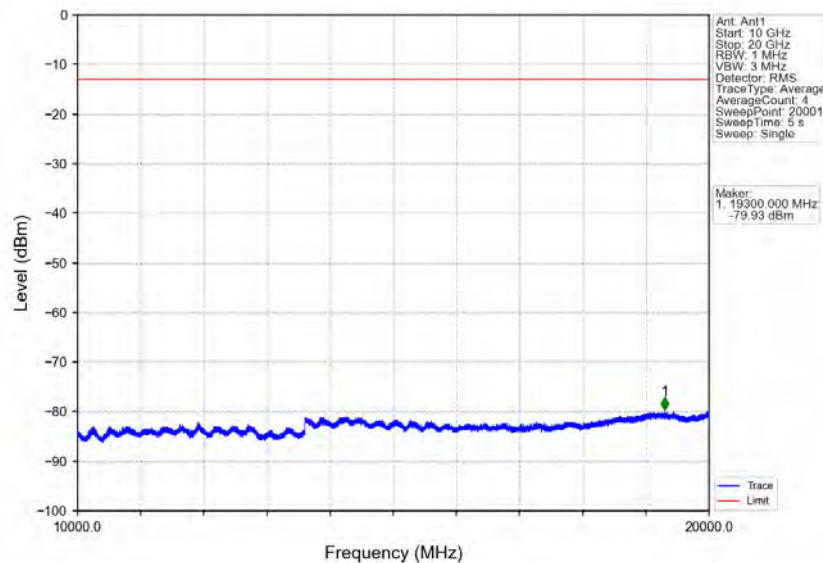
Band25_15MHz_QPSK_LCH_1857.5MHz_RB_75_0_NTNV
