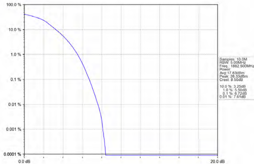
Band25_10MHz_64QAM_MCH_1882.5MHz_RB_50_0_NTNV
