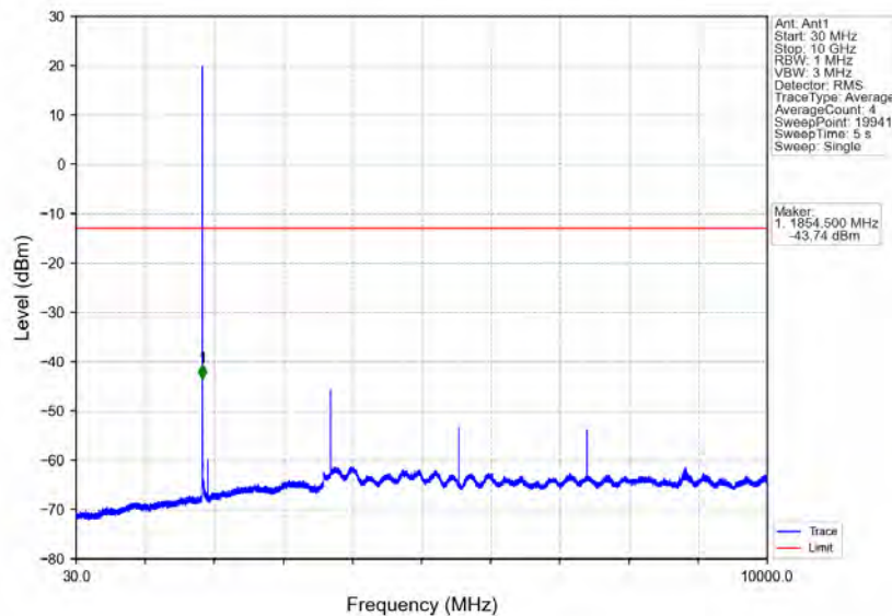
Band25 1.4MHz 64QAM LCH 1850.7MHz RB 1 0 NTN
