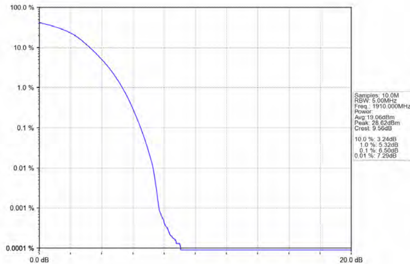
Band25_10MHz_16QAM_HCH_1910MHz_RB_50_0_NTNV
