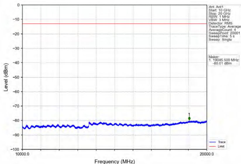
Band25 1.4MHz 16QAM LCH 1850.7MHz RB 6 0 NTN
