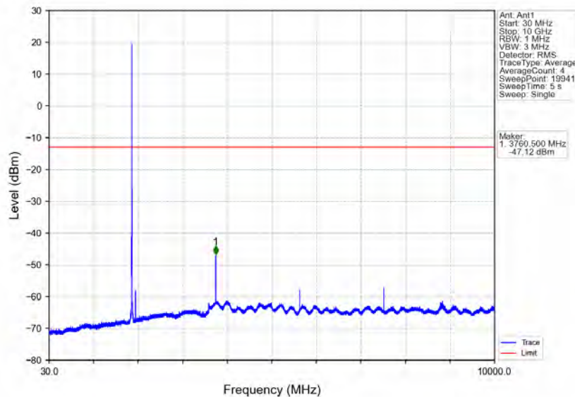
Band25_5MHz_64QAM_MCH_1882.5MHz_RB_1_0_NTNV
