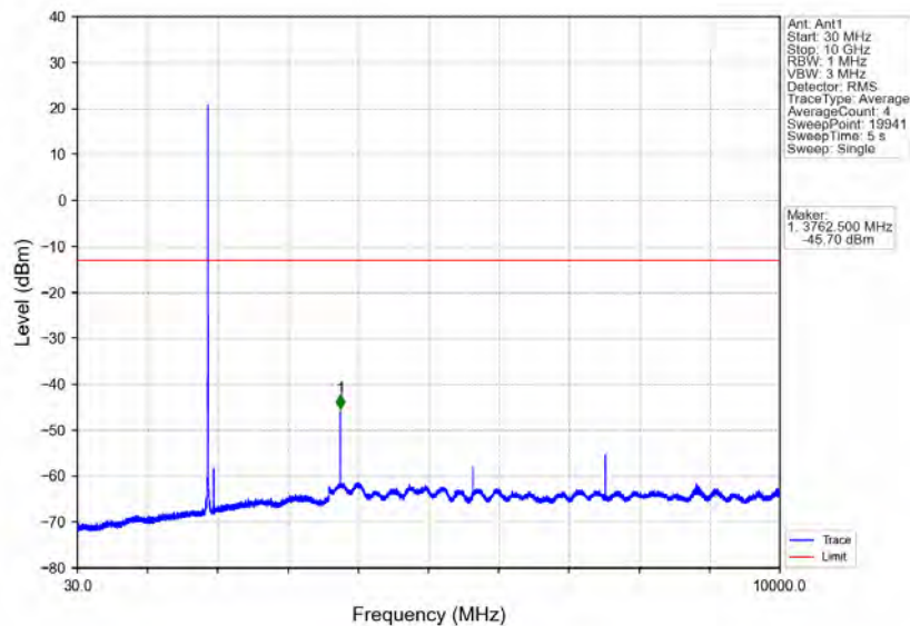
Band25_3MHz_16QAM_MCH_1882.5MHz_RB_1_0_NTNV
