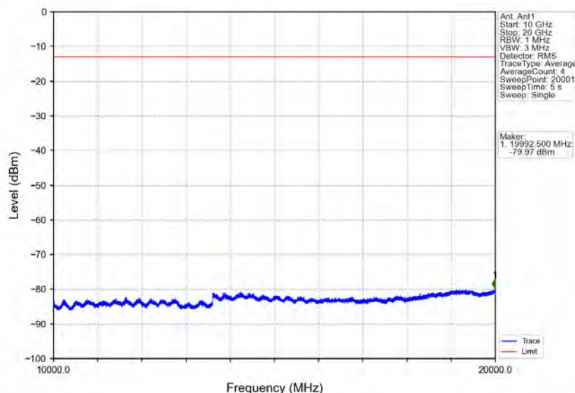
Band25 1.4MHz 64QAM HCH 1914.3MHz RB 1 0 NTN
