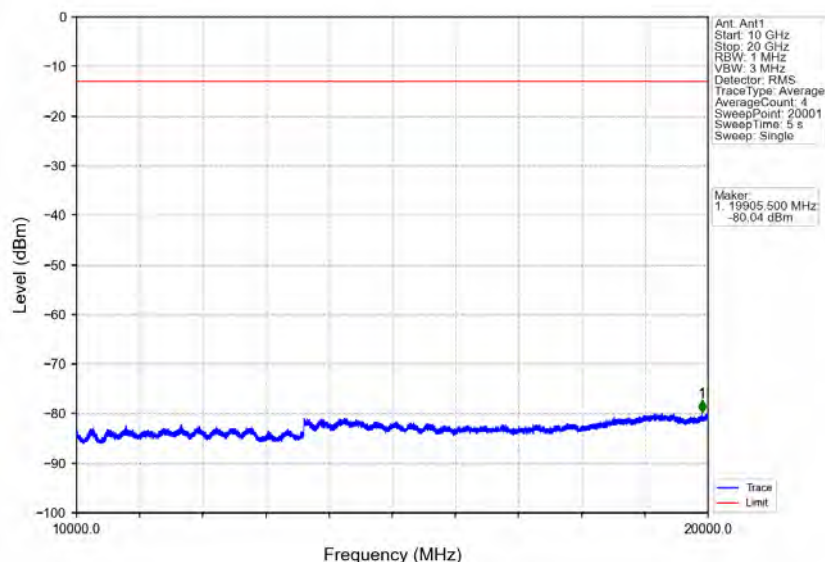
Band25_20MHz_QPSK_MCH_1882.5MHz_RB_1_0_NTNV
