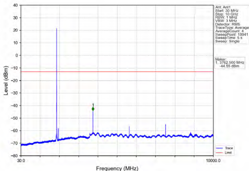
Band25_3MHz_QPSK_MCH_1882.5MHz_RB_1_0_NTNV
