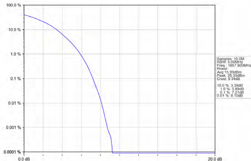
Band25_15MHz_64QAM_LCH_1857.5MHz_RB_75_0_NTNV
