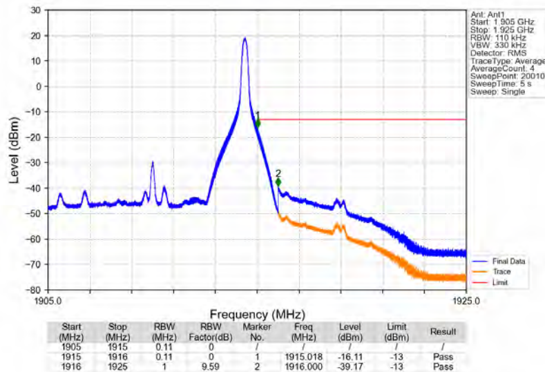
Band25_10MHz_64QAM_HCH_1910MHz_RB_1_49_NTNV
