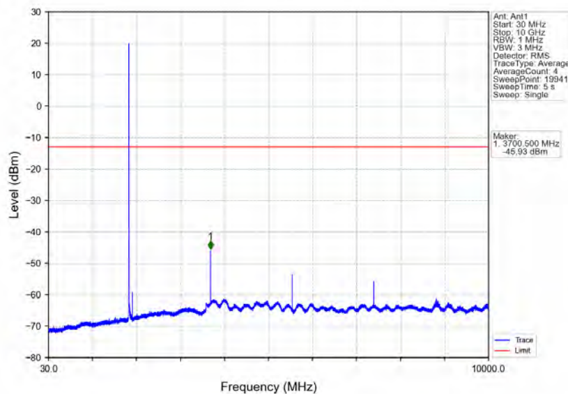
Band25_3MHz_64QAM_LCH_1851.5MHz_RB_1_0_NTNV
