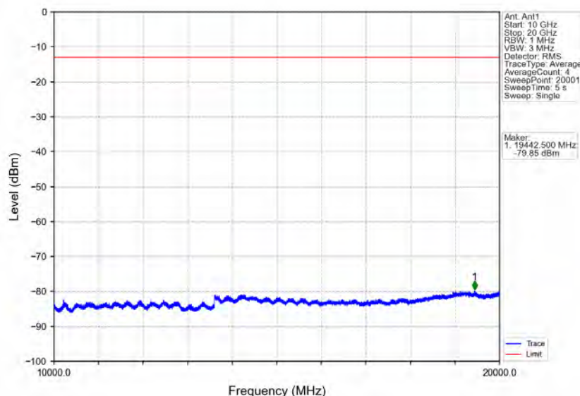
Band25_10MHz_QPSK_MCH_1882.5MHz_RB_1_0_NTNV
