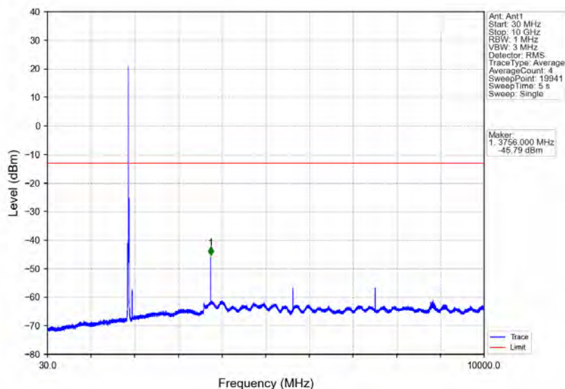
Band25_10MHz_16QAM_MCH_1882.5MHz_RB_1_0_NTNV
