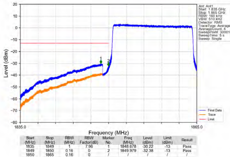
Band25_15MHz_16QAM_LCH_1857.5MHz_RB_75_0_NTNV
