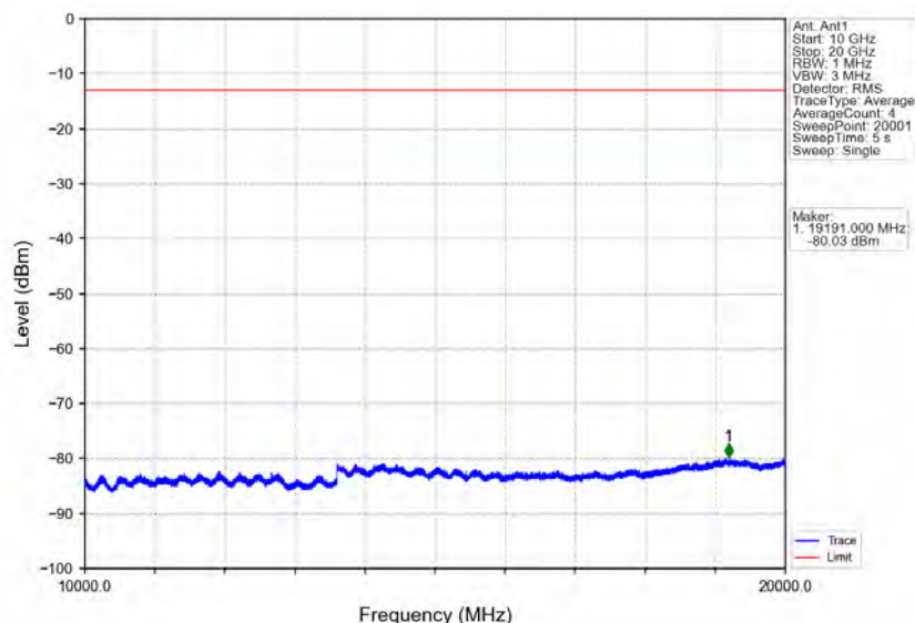
Band25_20MHz_16QAM_MCH_1882.5MHz_RB_1_0_NTNV
