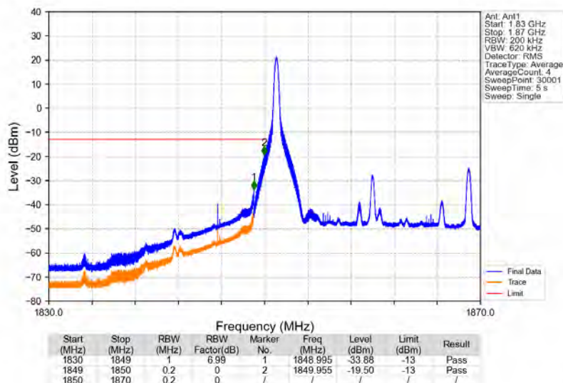
Band25_20MHz_16QAM_LCH_1860MHz_RB_1_0_NTNV
