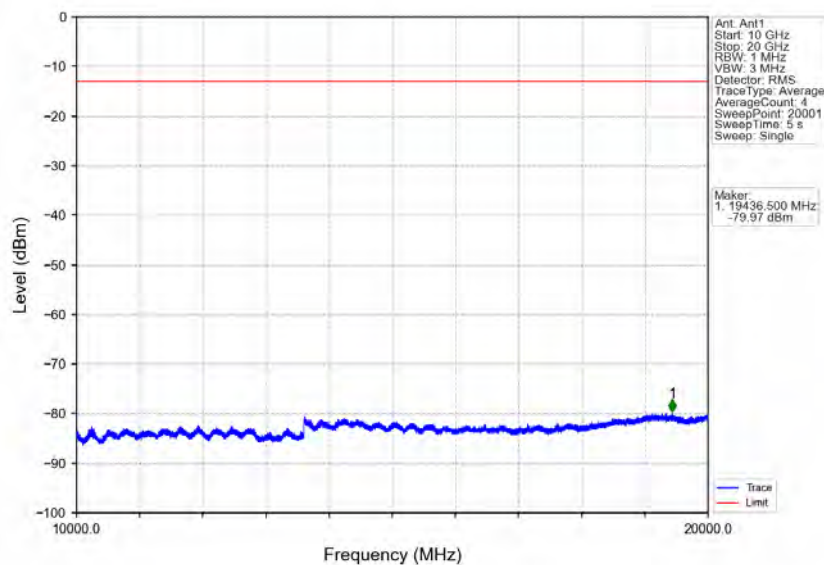
Band25_5MHz_16QAM_HCH_1912.5MHz_RB_1_0_NTNV
