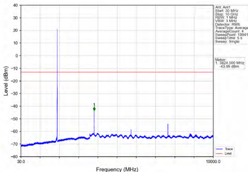
Band25_3MHz_16QAM_HCH_1913.5MHz_RB_1_0_NTNV
