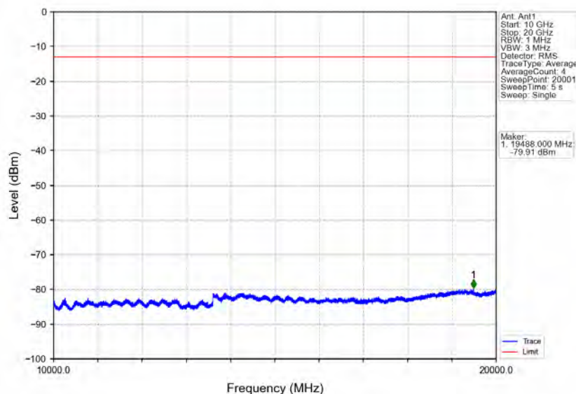
Band25_20MHz_64QAM_LCH_1860MHz_RB_100_0_NTNV
