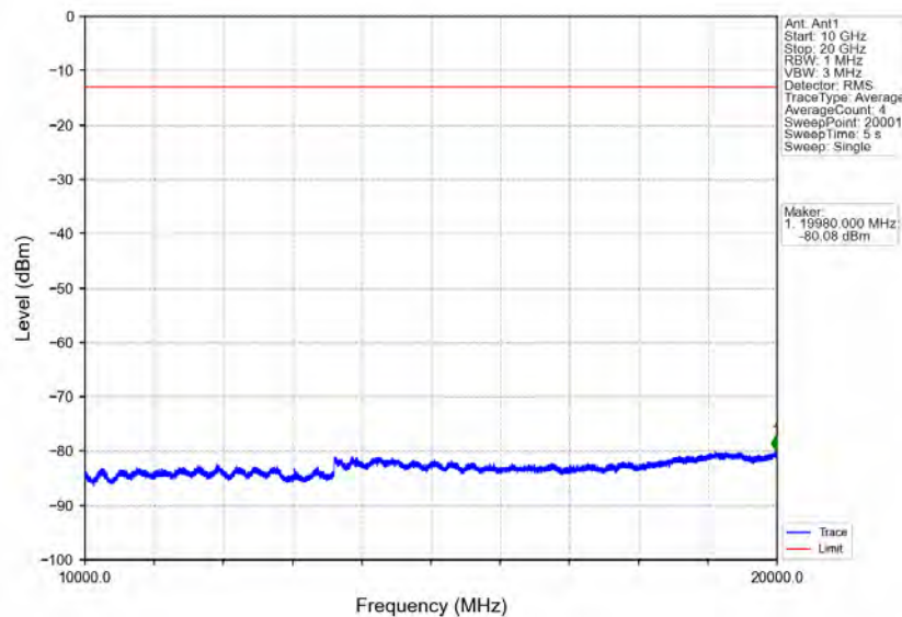
Band25_3MHz_64QAM_LCH_1851.5MHz_RB_15_0_NTNV
