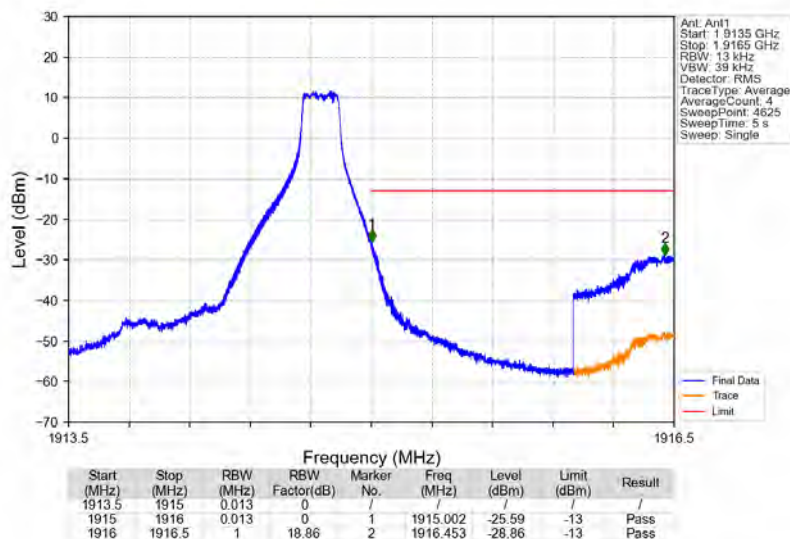
Band25 1.4MHz 16QAM HCH 1914.3MHz RB 1 5 NTNV
