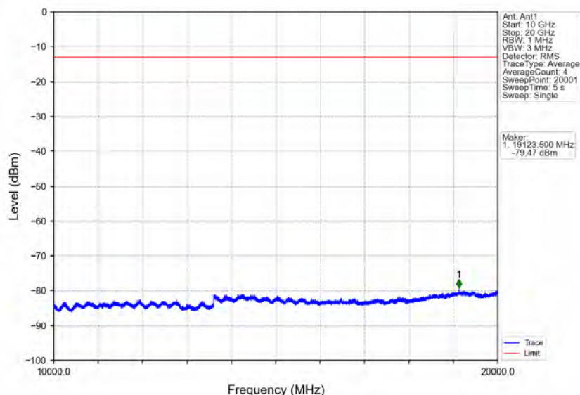
Band25_1.4MHz_64QAM_MCH_1882.5MHz_RB_1_0_NTNV
