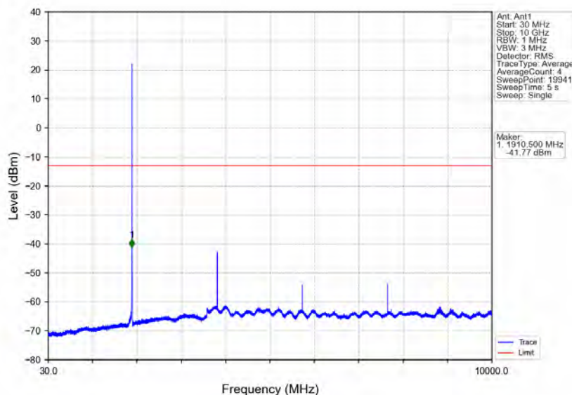
Band25_1.4MHz_QPSK_HCH_1914.3MHz_RB_1_0_NTNV
