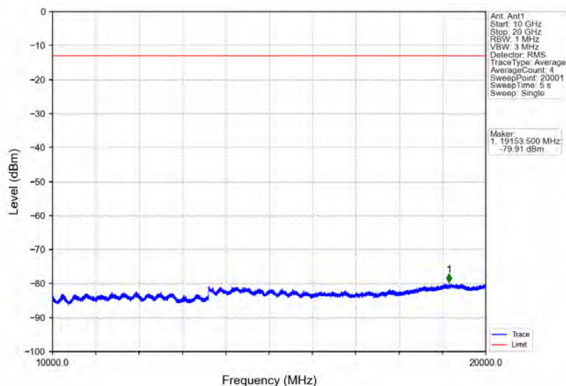
Band25_20MHz_16QAM_LCH_1860MHz_RB_100_0_NTNV
