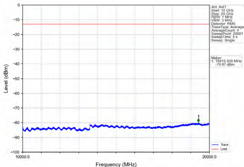
Band25_3MHz_QPSK_LCH_1851.5MHz_RB_15_0_NTNV
