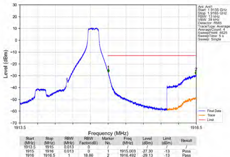
Band25 1.4MHz 64QAM HCH 1914.3MHz RB 1 5 NTNV
