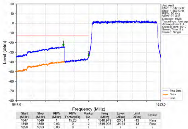
Band25_3MHz_16QAM_LCH_1851.5MHz_RB_15_0_NTNV
