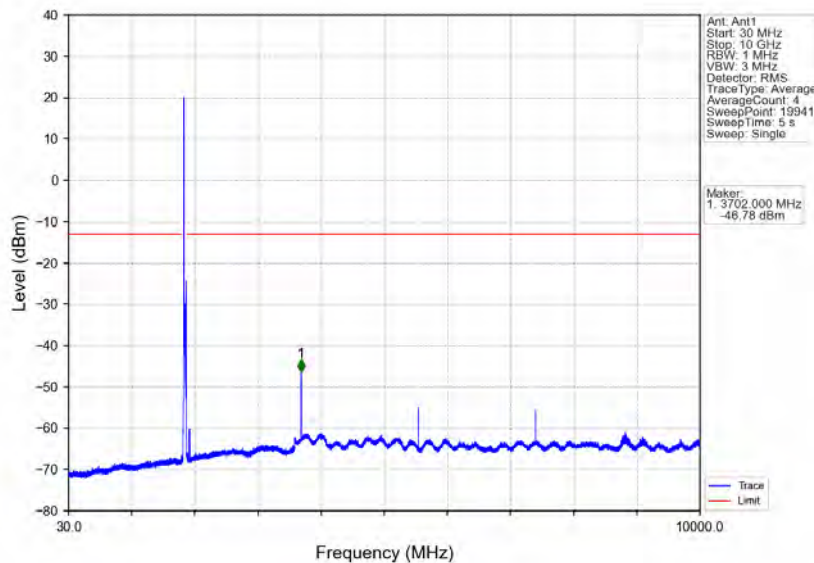
Band25_20MHz_64QAM_LCH_1860MHz_RB_1_0_NTNV
