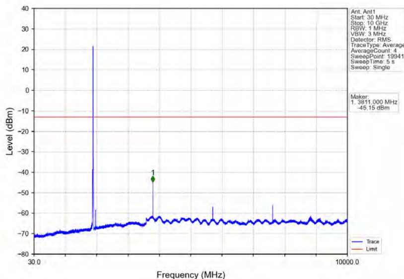
Band25_10MHz_16QAM_HCH_1910MHz_RB_1_0_NTNV
