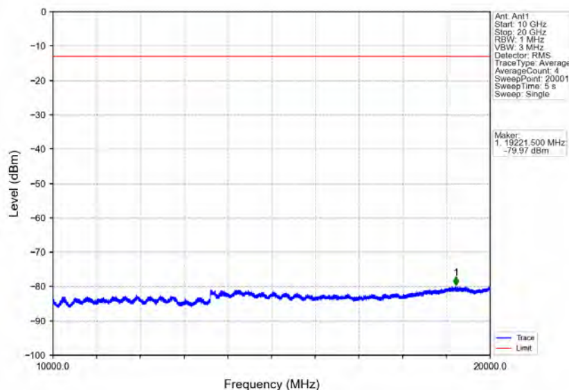
Band25_10MHz_64QAM_LCH_1855MHz_RB_50_0_NTNV
