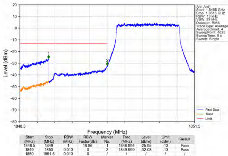
Band25_1.4MHz_QPSK_LCH_1850.7MHz_RB_6_0_NTNV
