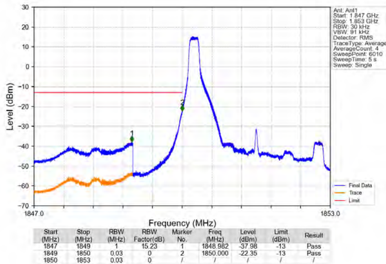
Band25_3MHz_16QAM_LCH_1851.5MHz_RB_1_0_NTNV
