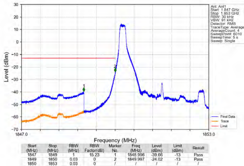
Band25_3MHz_64QAM_LCH_1851.5MHz_RB_1_0_NTNV
