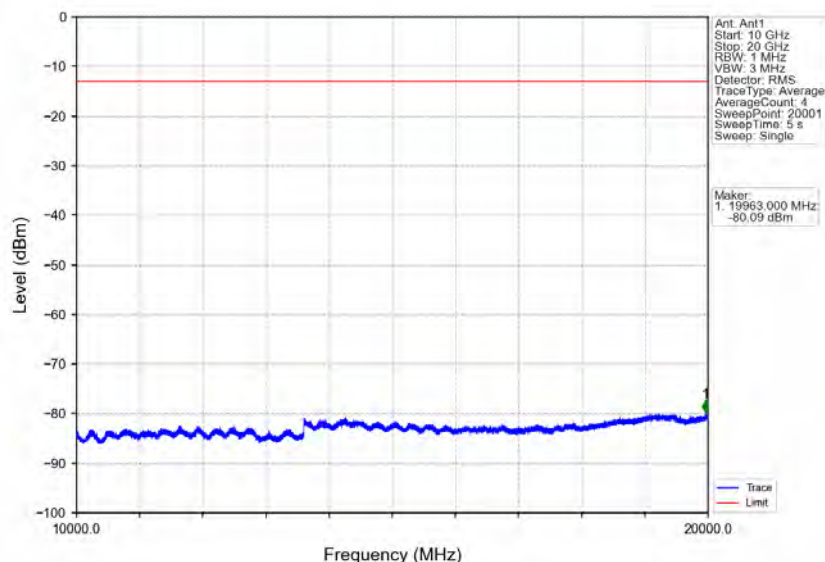
Band25_3MHz_QPSK_MCH_1882.5MHz_RB_1_0_NTNV
