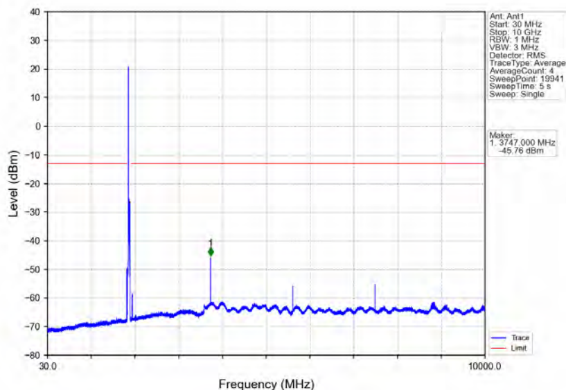
Band25_20MHz_16QAM_MCH_1882.5MHz_RB_1_0_NTNV
