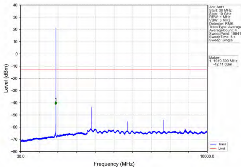
Band25_1.4MHz_16QAM_HCH_1914.3MHz_RB_1_0_NTNV
