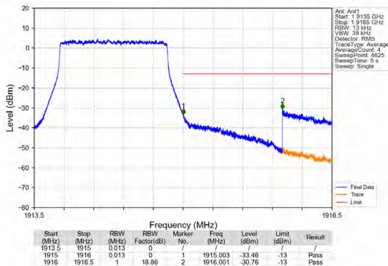
Band25_1.4MHz_QPSK_HCH_1914.3MHz_RB_6_0_NTNV
