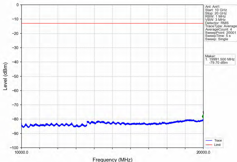
Band25_5MHz_64QAM_HCH_1912.5MHz_RB_1_0_NTNV
