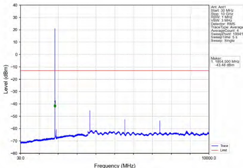
Band25 1.4MHz 16QAM LCH 1850.7MHz RB 1 0 NTN
