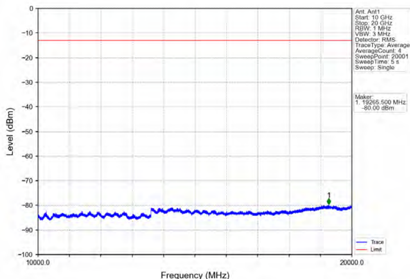
Band25_10MHz_16QAM_MCH_1882.5MHz_RB_1_0_NTNV
