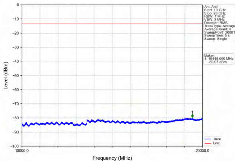
Band25_1.4MHz_16QAM_HCH_1914.3MHz_RB_1_0_NTNV
