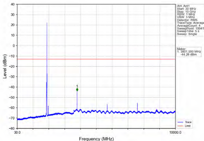
Band25_15MHz_QPSK_HCH_1907.5MHz_RB_1_0_NTNV
