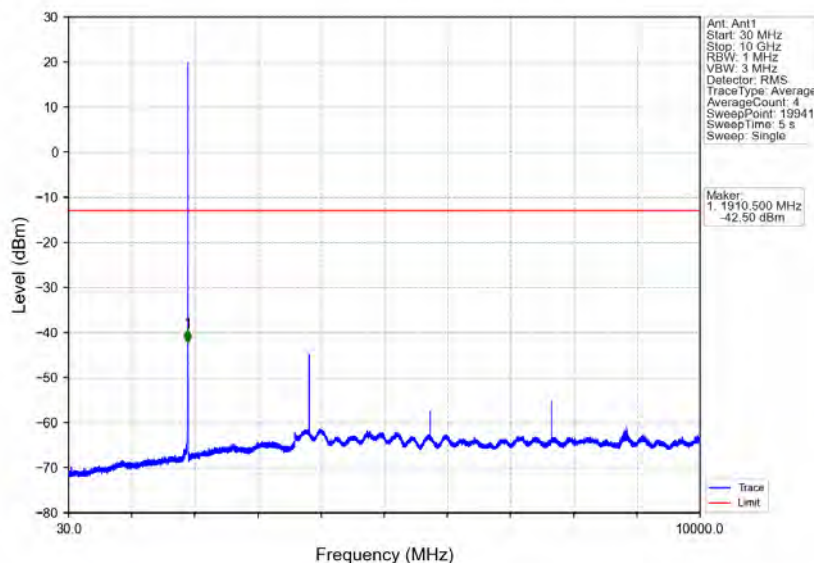
Band25 1.4MHz 64QAM HCH 1914.3MHz RB 1 0 NTN
