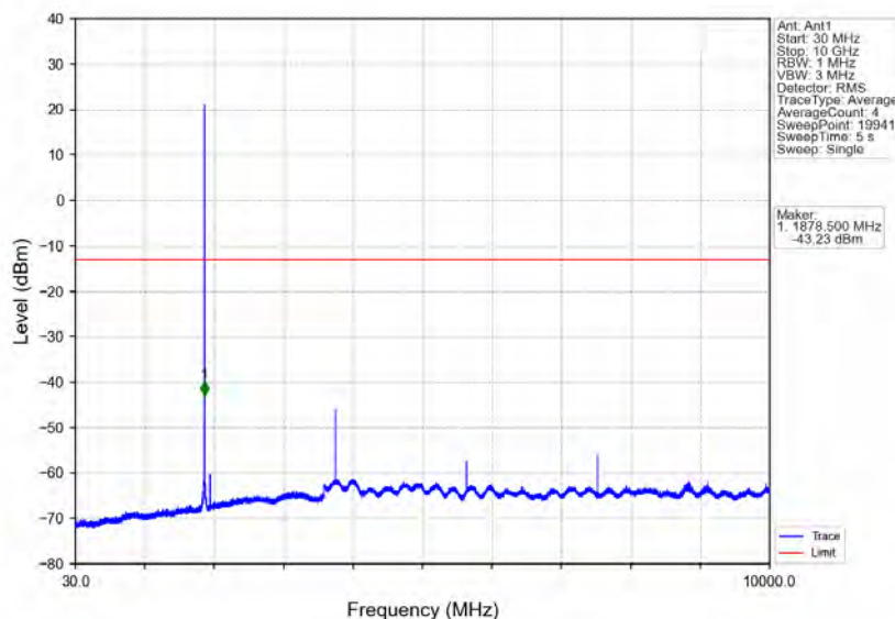
Band25_1.4MHz_16QAM_MCH_1882.5MHz_RB_1_0_NTNV
