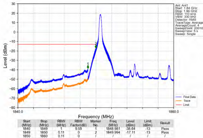
Band25_10MHz_64QAM_LCH_1855MHz_RB_1_0_NTNV
