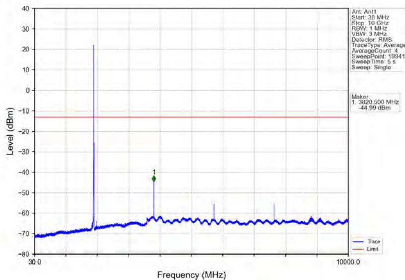
Band25_5MHz_QPSK_HCH_1912.5MHz_RB_1_0_NTNV
