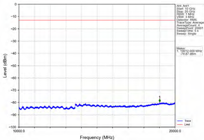
Band25_10MHz_64QAM_HCH_1910MHz_RB_1_0_NTNV
