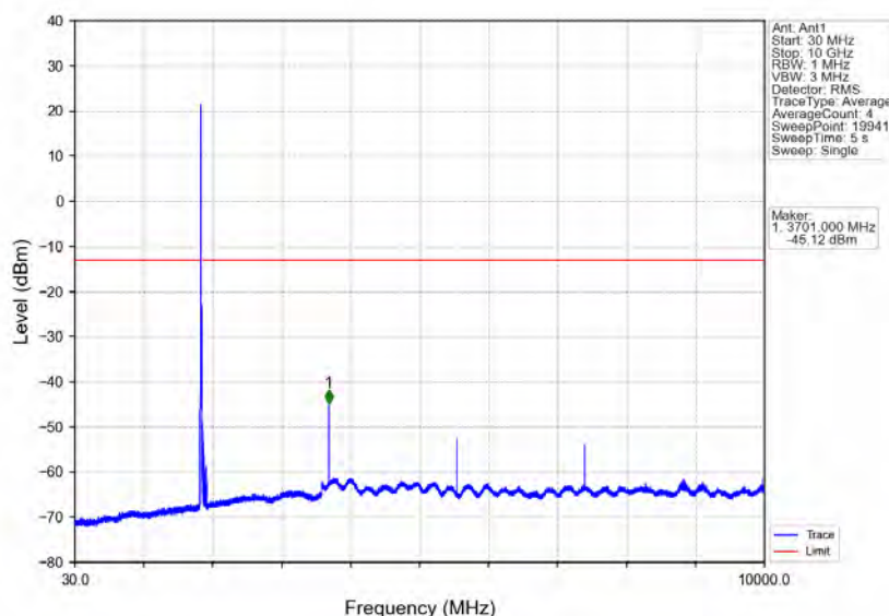
Band25_10MHz_16QAM_LCH_1855MHz_RB_1_0_NTNV
