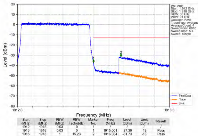
Band25_3MHz_64QAM_HCH_1913.5MHz_RB_15_0_NTNV
