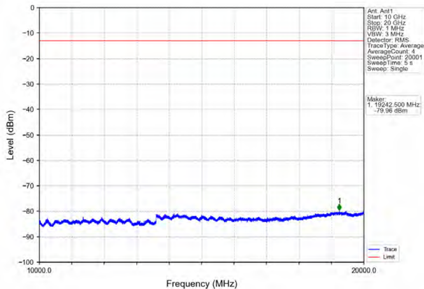
Band25_3MHz_16QAM_MCH_1882.5MHz_RB_1_0_NTNV
