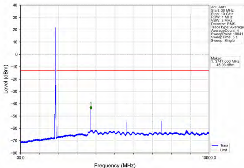
Band25_20MHz_QPSK_MCH_1882.5MHz_RB_1_0_NTNV
