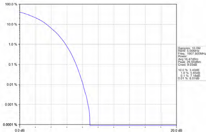
Band25_15MHz_64QAM_HCH_1907.5MHz_RB_75_0_NTNV
