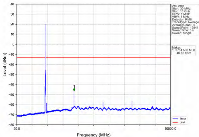
Band25_15MHz_64QAM_MCH_1882.5MHz_RB_1_0_NTNV
