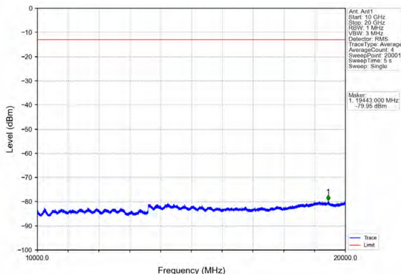
Band25_10MHz_64QAM_MCH_1882.5MHz_RB_1_0_NTNV
