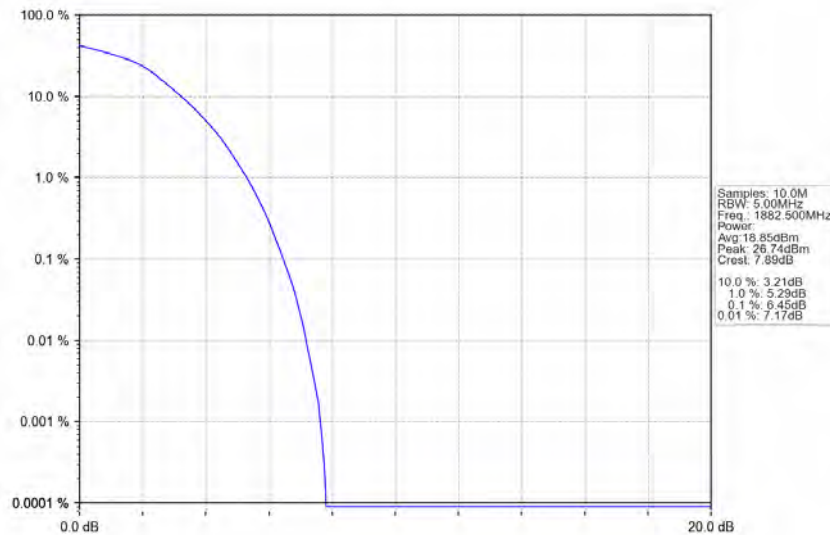
Band25_10MHz_16QAM_MCH_1882.5MHz_RB_50_0_NTNV
