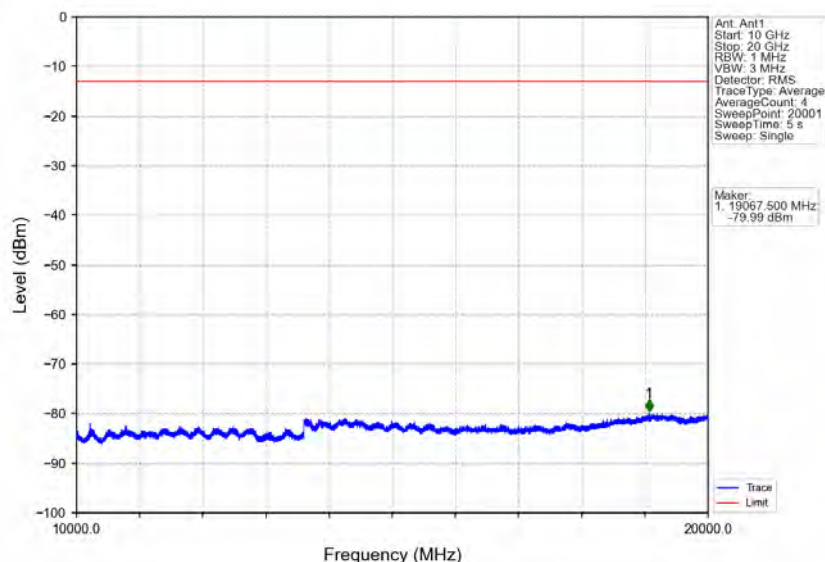
Band25_15MHz_64QAM_MCH_1882.5MHz_RB_1_0_NTNV
