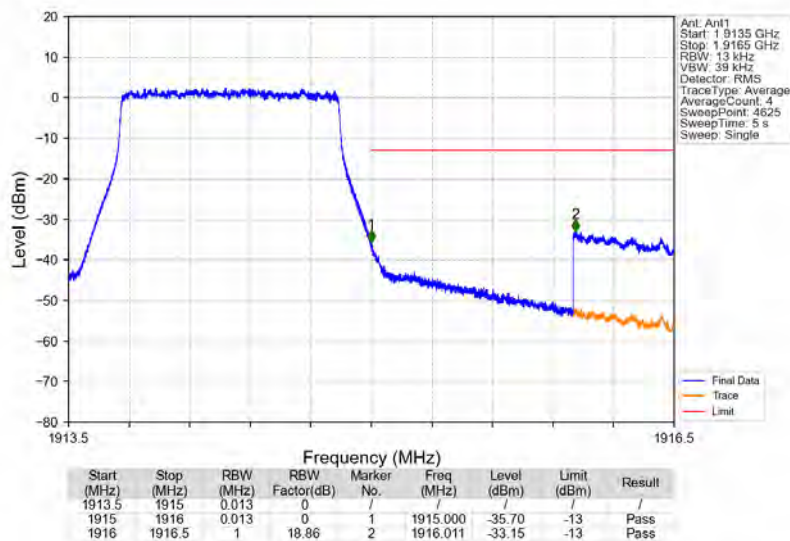
Band25 1.4MHz 64QAM HCH 1914.3MHz RB 6 0 NTNV
