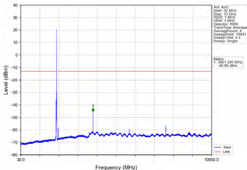
Band25_15MHz_64QAM_HCH_1907.5MHz_RB_1_0_NTNV
