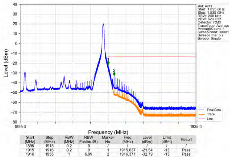
Band25_20MHz_64QAM_HCH_1905MHz_RB_1_99_NTNV
