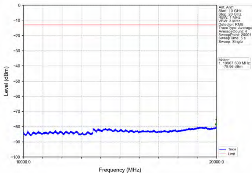
Band25_5MHz_16QAM_MCH_1882.5MHz_RB_1_0_NTNV
