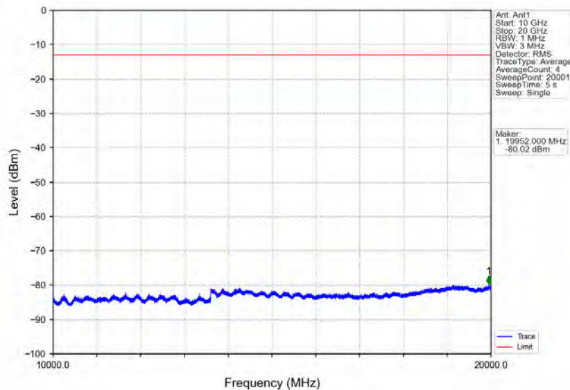
Band25_5MHz_64QAM_MCH_1882.5MHz_RB_1_0_NTNV
