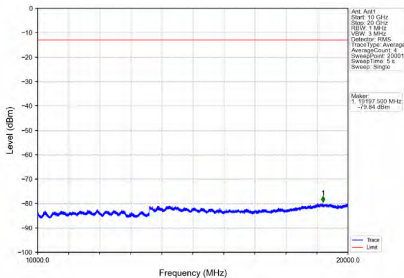
Band25_5MHz_QPSK_HCH_1912.5MHz_RB_1_0_NTNV
