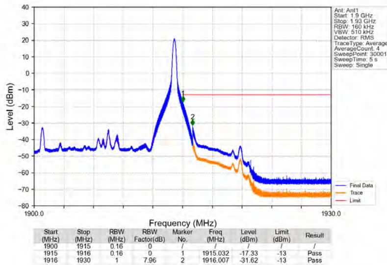
Band25_15MHz_16QAM_HCH_1907.5MHz_RB_1_74_NTNV
