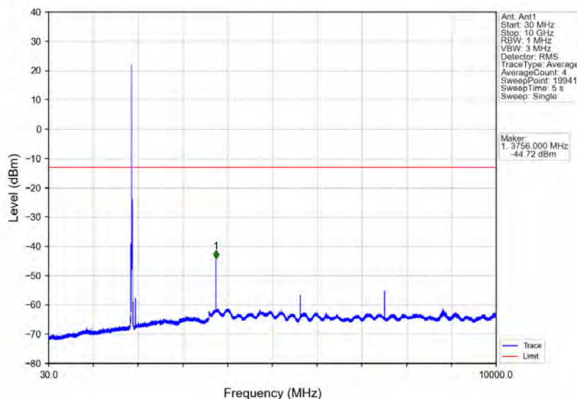
Band25_10MHz_QPSK_MCH_1882.5MHz_RB_1_0_NTNV
