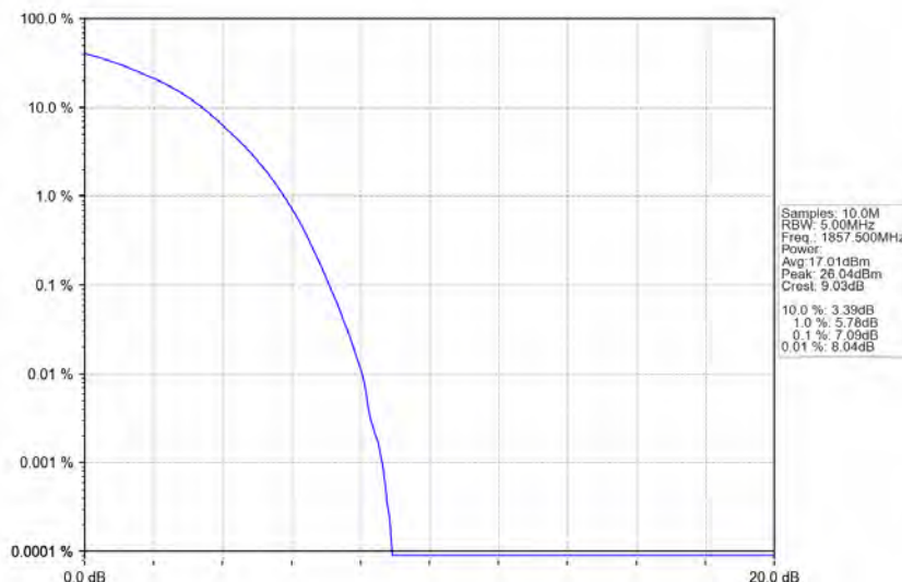
Band25_15MHz_16QAM_LCH_1857.5MHz_RB_75_0_NTNV
