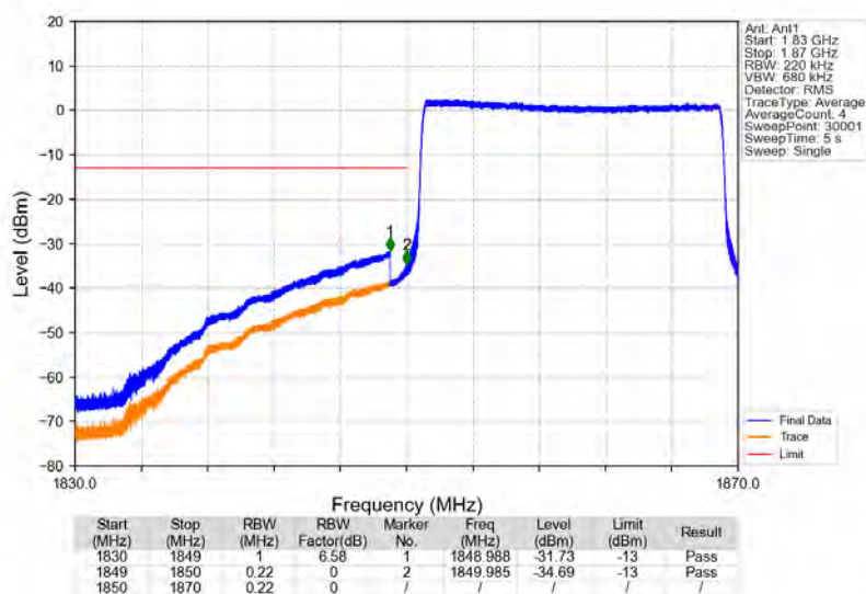
Band25_20MHz_64QAM_LCH_1860MHz_RB_100_0_NTNV
