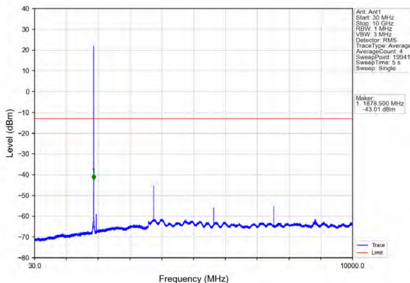
Band25_1.4MHz_QPSK_MCH_1882.5MHz_RB_1_0_NTNV
