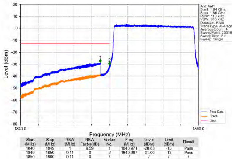
Band25_10MHz_16QAM_LCH_1855MHz_RB_50_0_NTNV
