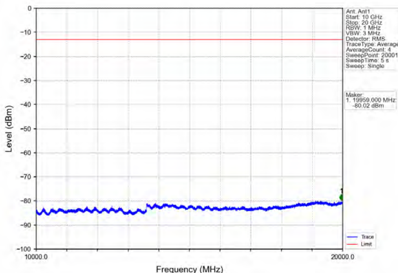
Band25_15MHz_QPSK_HCH_1907.5MHz_RB_1_0_NTNV
