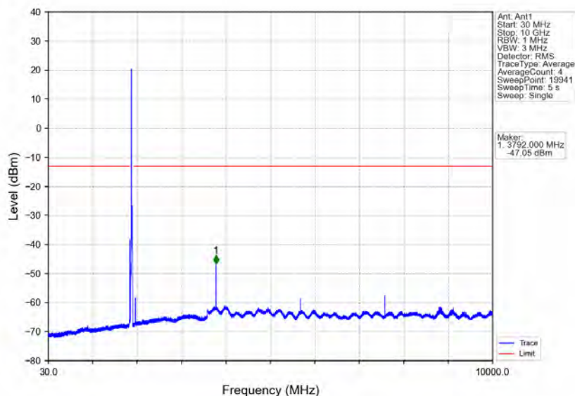
Band25_20MHz_64QAM_HCH_1905MHz_RB_1_0_NTNV
