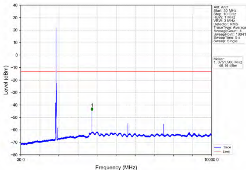
Band25_15MHz_QPSK_MCH_1882.5MHz_RB_1_0_NTNV
