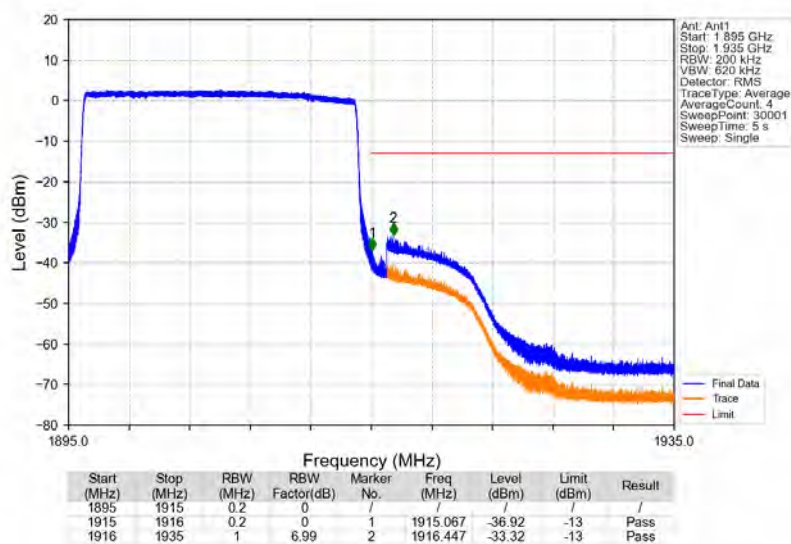
Band25_20MHz_16QAM_HCH_1905MHz_RB_100_0_NTNV
