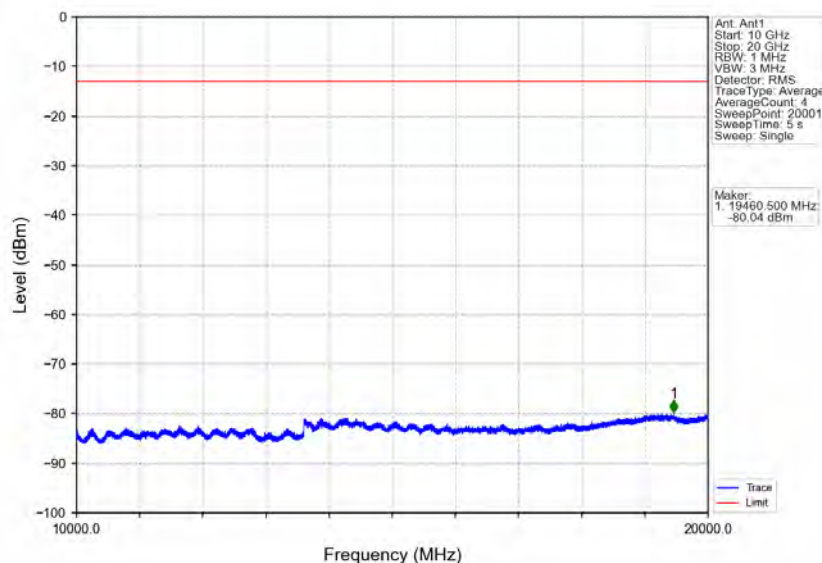
Band25_3MHz_16QAM_LCH_1851.5MHz_RB_15_0_NTNV
