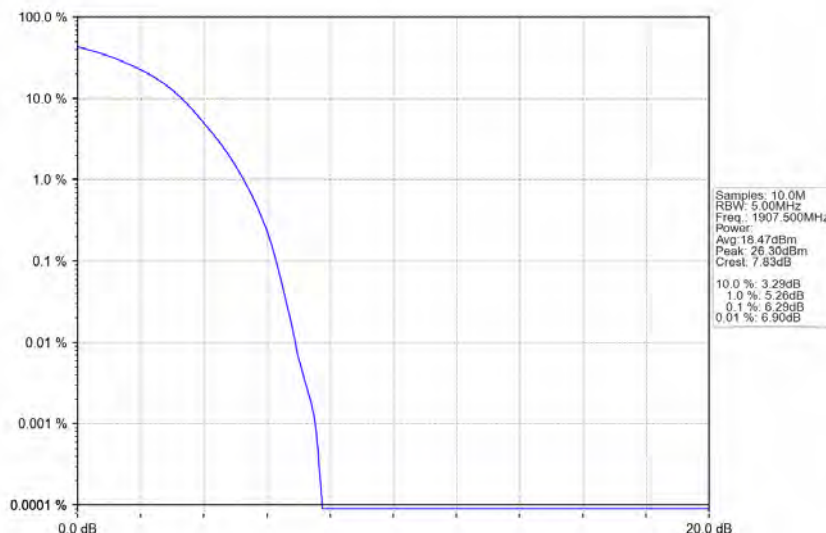
Band25_15MHz_QPSK_HCH_1907.5MHz_RB_75_0_NTNV
