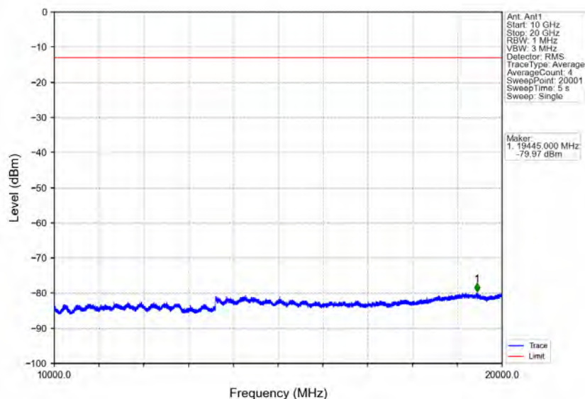
Band25_1.4MHz_QPSK_LCH_1850.7MHz_RB_6_0_NTNV
