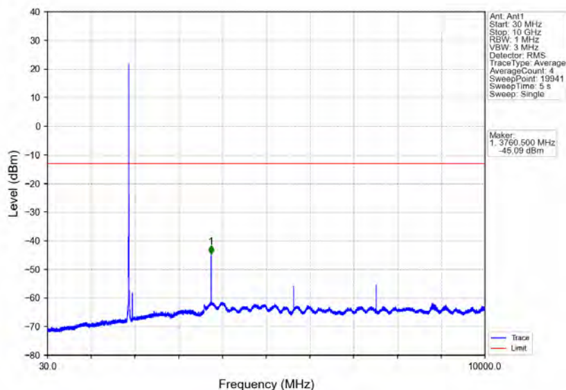
Band25_5MHz_QPSK_MCH_1882.5MHz_RB_1_0_NTNV
