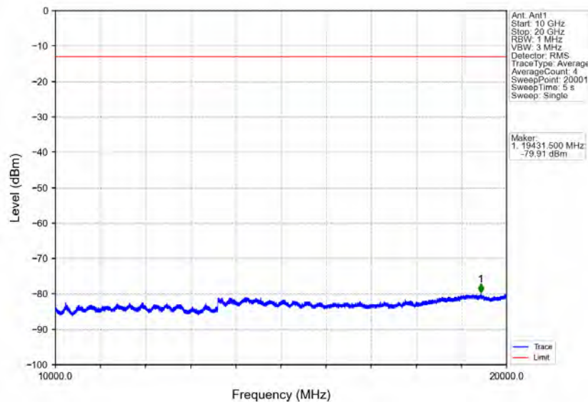
Band25_5MHz_16QAM_LCH_1852.5MHz_RB_25_0_NTNV
