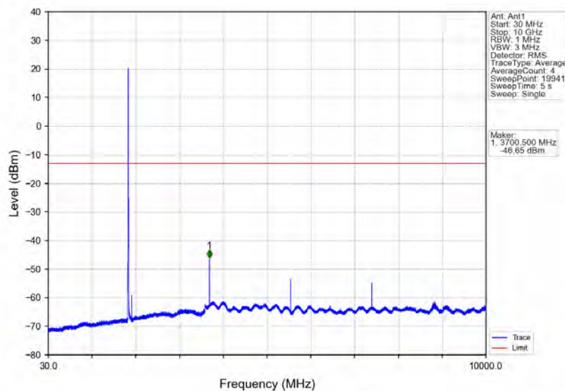
Band25_5MHz_64QAM_LCH_1852.5MHz_RB_1_0_NTNV
