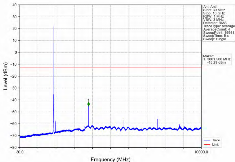
Band25_15MHz_16QAM_HCH_1907.5MHz_RB_1_0_NTNV
