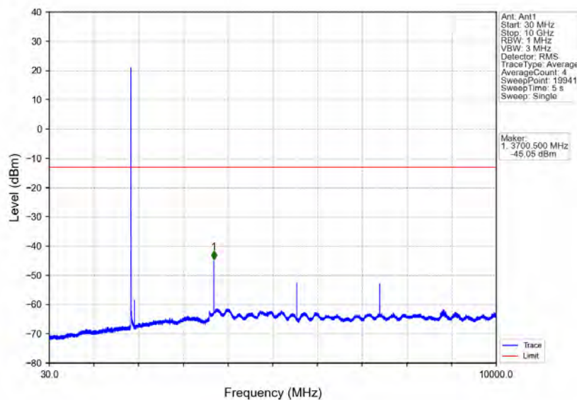
Band25_3MHz_16QAM_LCH_1851.5MHz_RB_1_0_NTNV
