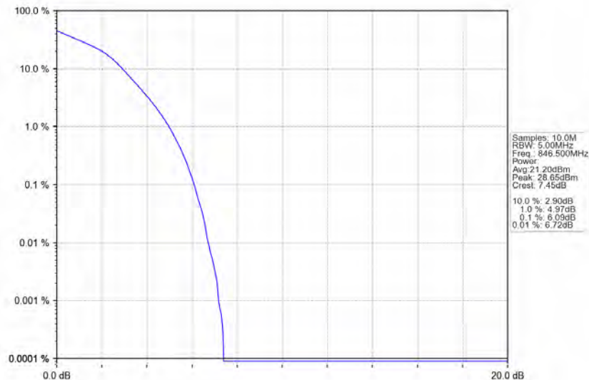
Band26b_5MHz_16QAM_HCH_846.5MHz_RB_25_0_NTNV
