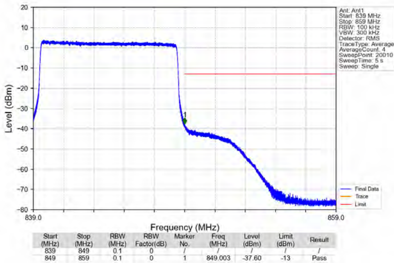
Band26b_10MHz_16QAM_HCH_844MHz_RB_50_0_NTNV
