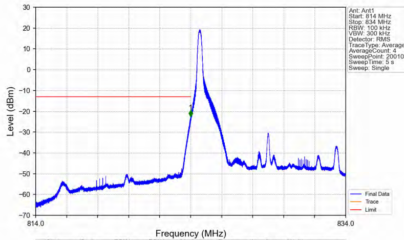
Band26b_10MHz_64QAM_LCH_829MHz_RB_1_0_NTNV
