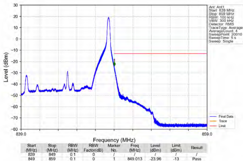
Band26b_10MHz_64QAM_HCH_844MHz_RB_1_49_NTNV
