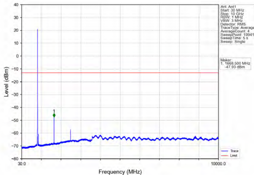
Band26b 5MHz 64QAM MCH 836.5MHz RB 1 0 NTN
