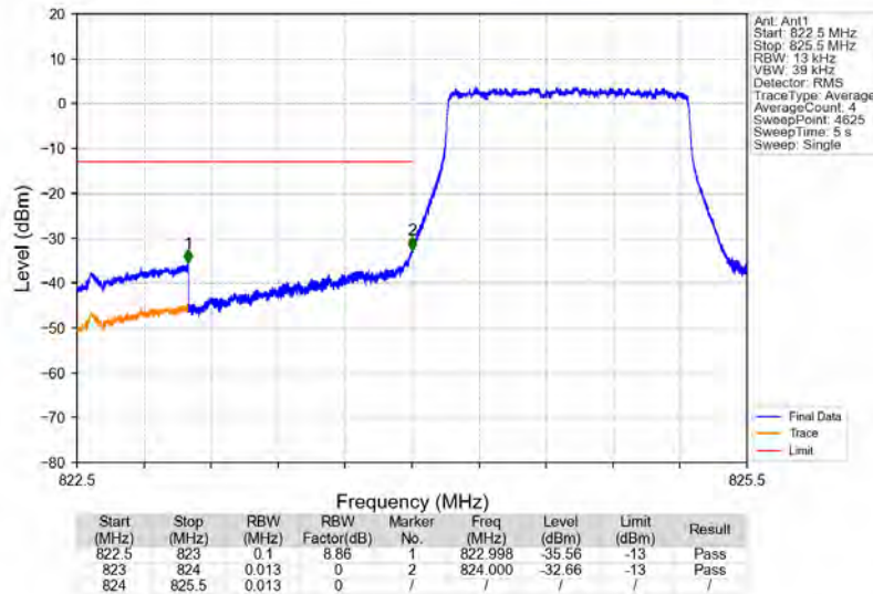
Band26b_1.4MHz_16QAM_LCH_824.7MHz_RB_6_0_NTNV
