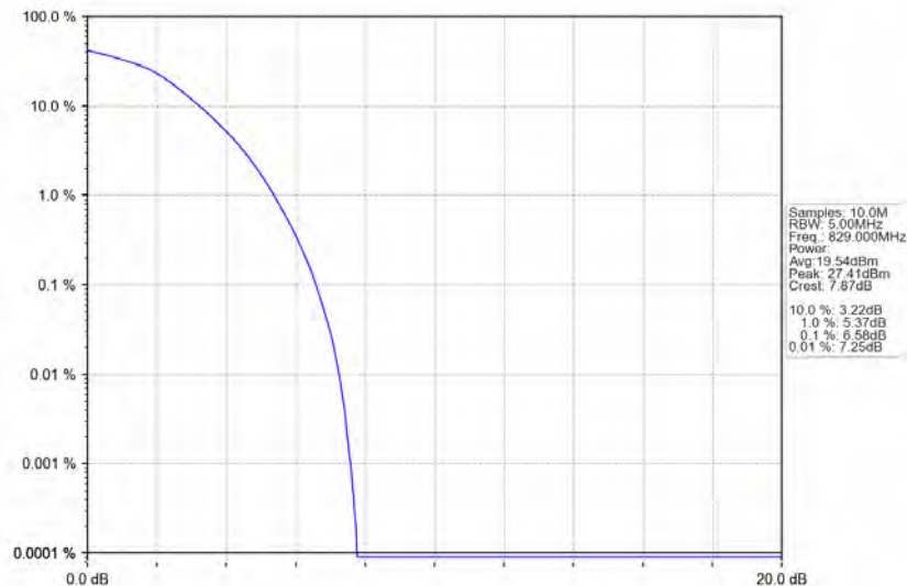
Band26b_10MHz_16QAM_LCH_829MHz_RB_50_0_NTNV
