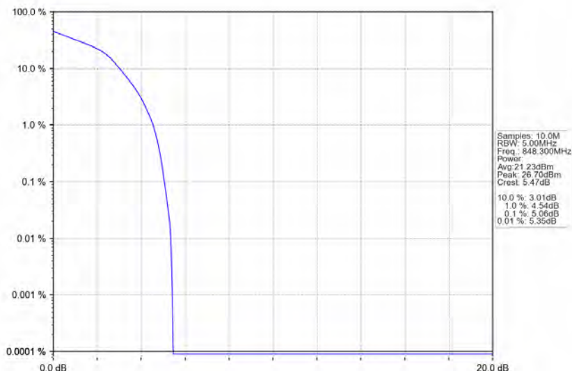
Band26b_1.4MHz_16QAM_HCH_848.3MHz_RB_6_0_NTNV
