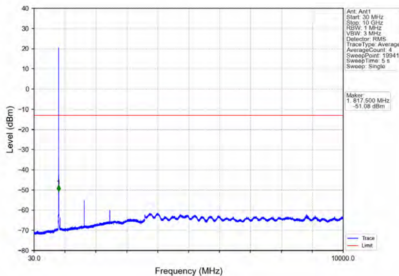
Band26b_3MHz_64QAM_LCH_825.5MHz_RB_1_0_NTNV
