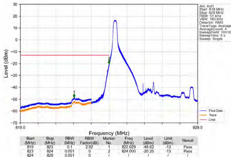
Band26b_5MHz_64QAM_LCH_826.5MHz_RB_1_0_NTNV
