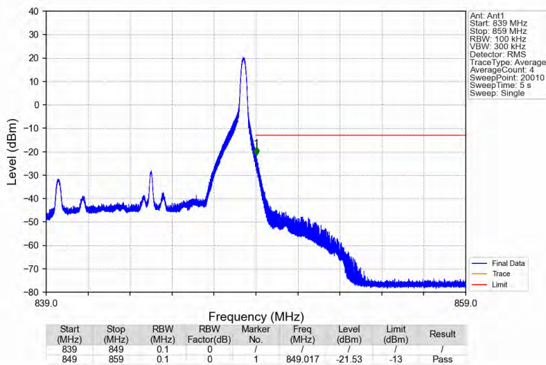
Band26b_10MHz_16QAM_HCH_844MHz_RB_1_49_NTNV
