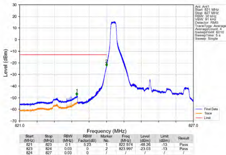
Band26b_3MHz_16QAM_LCH_825.5MHz_RB_1_0_NTNV
