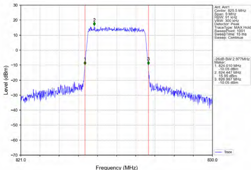
Band26b_3MHz_64QAM_LCH_825.5MHz_RB_15_0_NTNV
