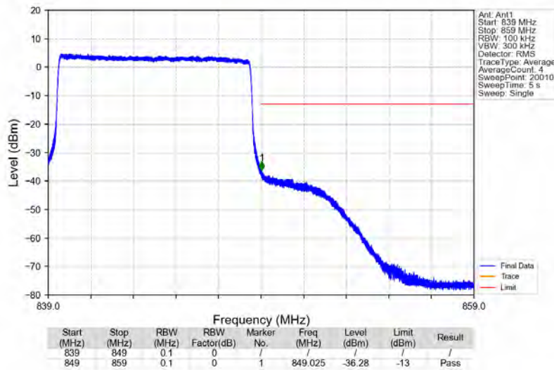
Band26b_10MHz_QPSK_HCH_844MHz_RB_50_0_NTNV
