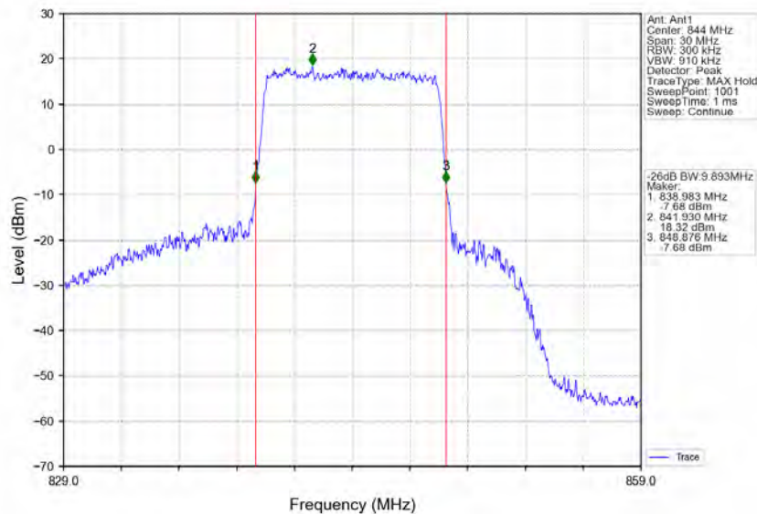
Band26b_10MHz_QPSK_HCH_844MHz_RB_50_0_NTNV
