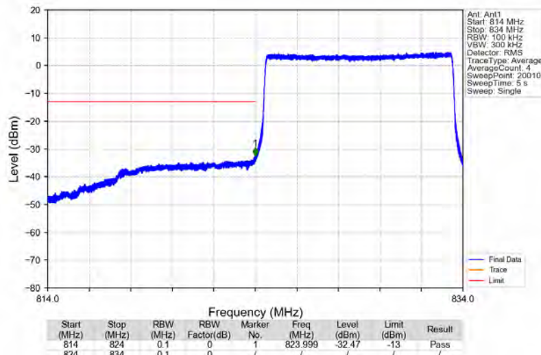
Band26b_10MHz_QPSK_LCH_829MHz_RB_50_0_NTNV
