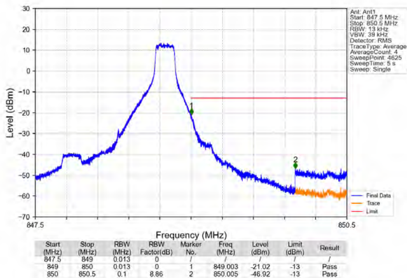
Band26b 1.4MHz QPSK HCH 848.3MHz RB 1_5 NTN
