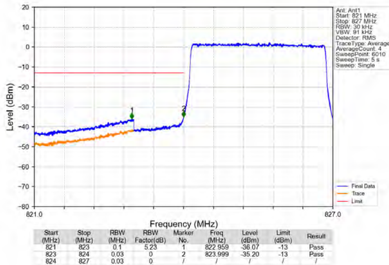
Band26b_3MHz_64QAM_LCH_825.5MHz_RB_15_0_NTNV
