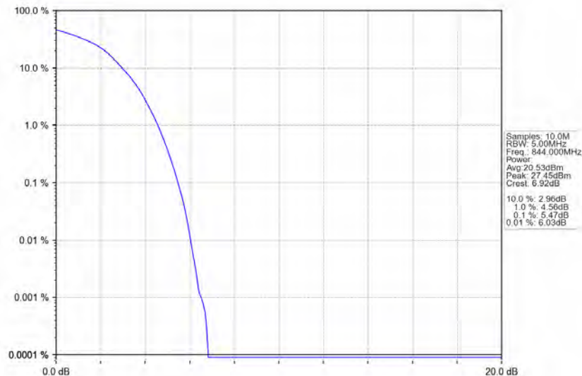
Band26b_10MHz_QPSK_HCH_844MHz_RB_50_0_NTNV
