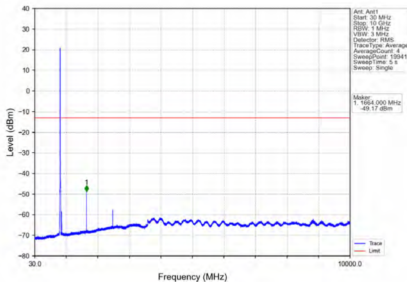
Band26b_10MHz_64QAM_MCH_836.5MHz_RB_1_0_NTNV
