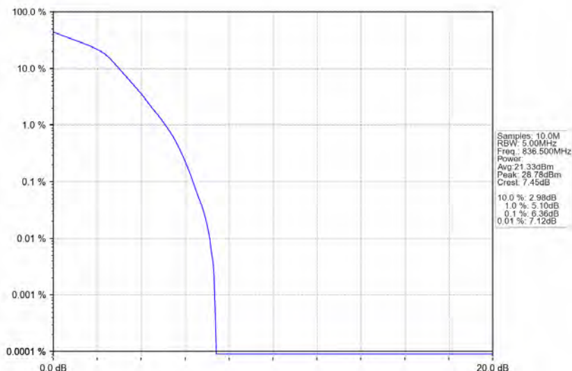
Band26b_1.4MHz_16QAM_MCH_836.5MHz_RB_6_0_NTNV
