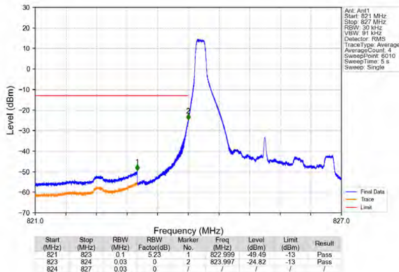
Band26b_3MHz_64QAM_LCH_825.5MHz_RB_1_0_NTNV
