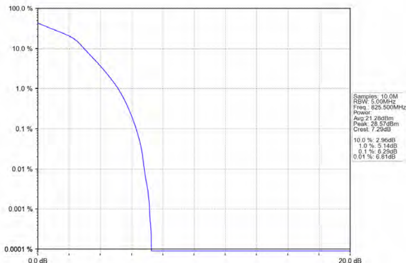
Band26b_3MHz_16QAM_LCH_825.5MHz_RB_15_0_NTNV
