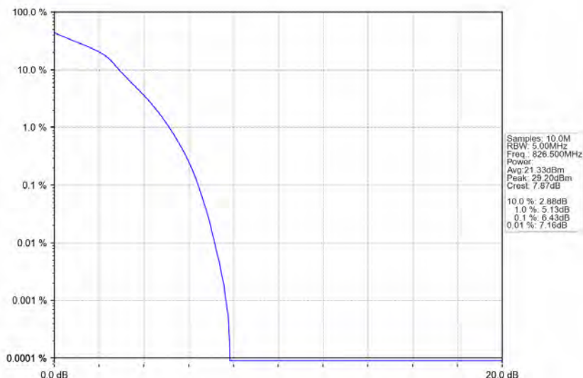
Band26b_5MHz_16QAM_LCH_826.5MHz_RB_25_0_NTNV
