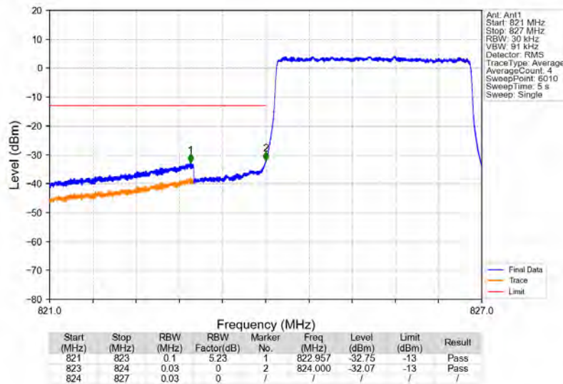
Band26b_3MHz_QPSK_LCH_825.5MHz_RB_15_0_NTNV
