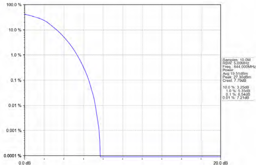
Band26b_10MHz_16QAM_HCH_844MHz_RB_50_0_NTNV
