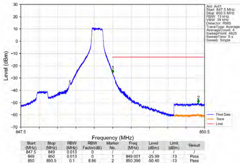
Band26b_1.4MHz_64QAM_HCH_848.3MHz_RB_1_5_NTNV
