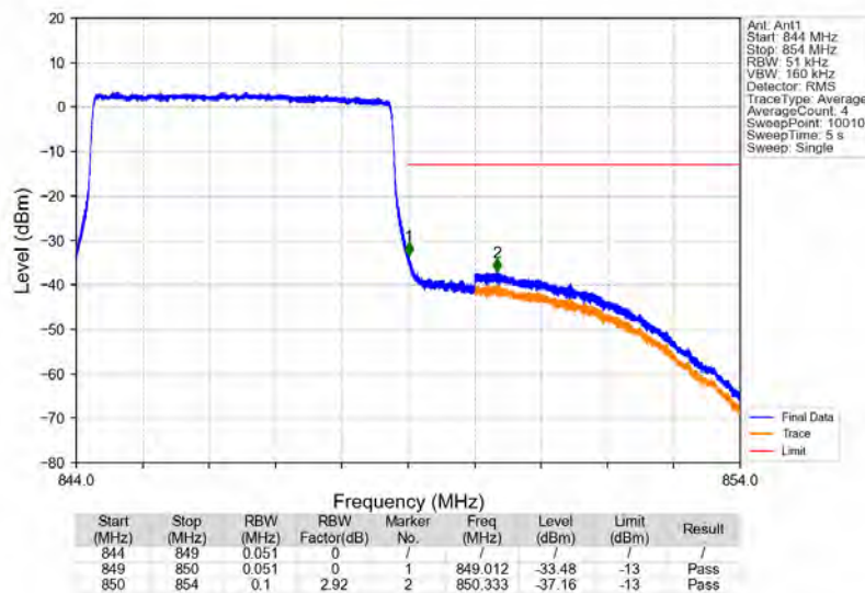
Band26b_5MHz_16QAM_HCH_846.5MHz_RB_25_0_NTNV
