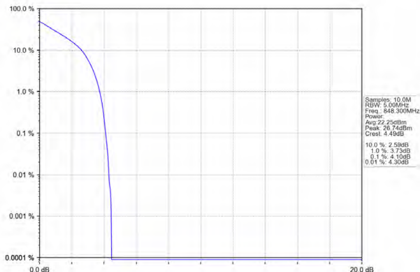
Band26b 1.4MHz QPSK HCH 848.3MHz RB 6_0 NTN
