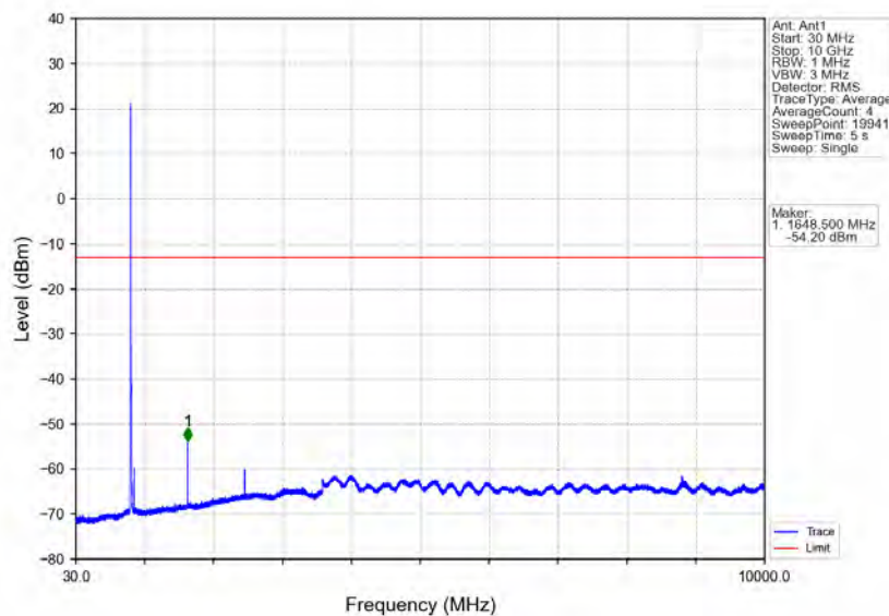
Band26b_5MHz_64QAM_LCH_826.5MHz_RB_1_0_NTNV
