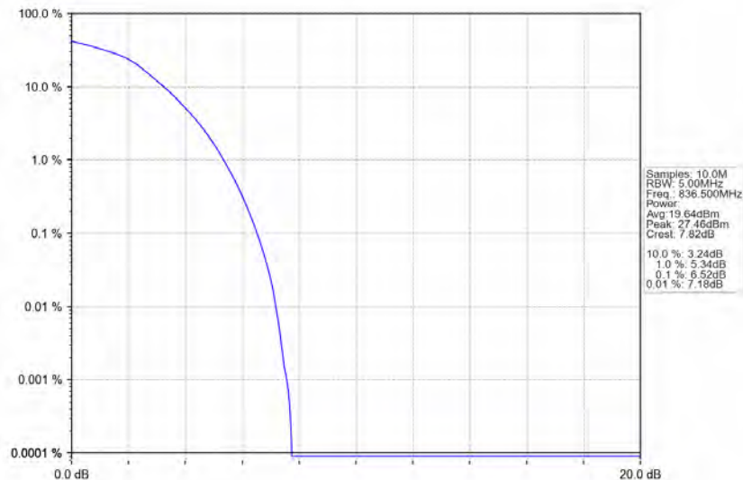
Band26b_10MHz_16QAM_MCH_836.5MHz_RB_50_0_NTNV
