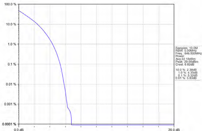
Band26b_5MHz_QPSK_HCH_846.5MHz_RB_25_0_NTNV
