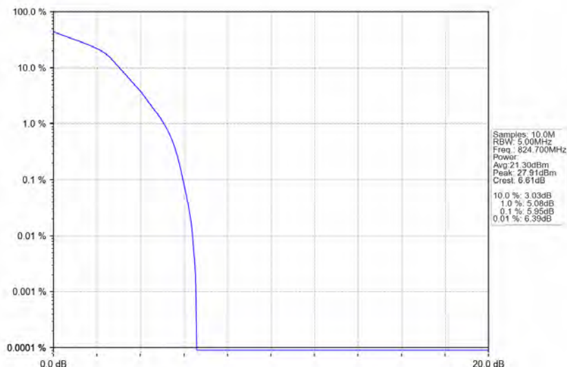
Band26b 1.4MHz 16QAM LCH 824.7MHz RB 6_0 NTN
