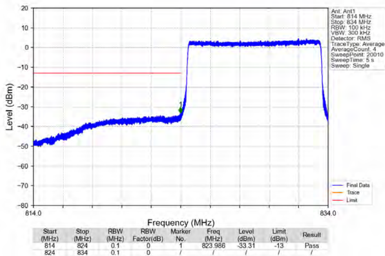
Band26b_10MHz_16QAM_LCH_829MHz_RB_50_0_NTNV
