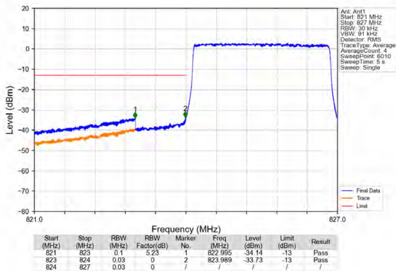
Band26b_3MHz_16QAM_LCH_825.5MHz_RB_15_0_NTNV
