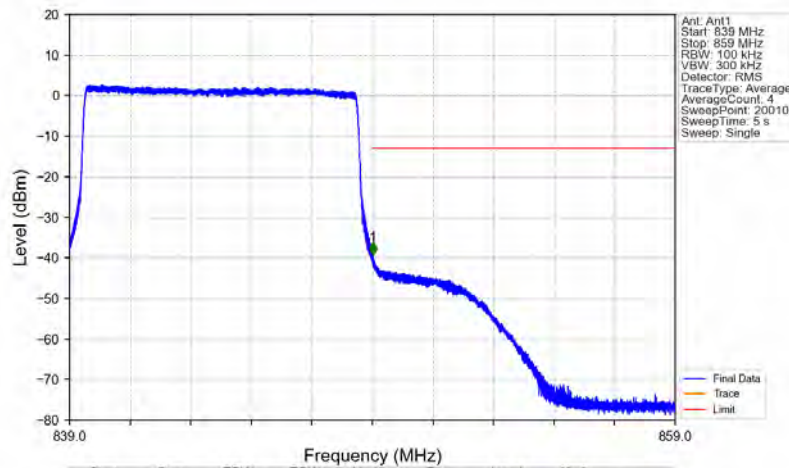
Band26b_10MHz_64QAM_HCH_844MHz_RB_50_0_NTNV
