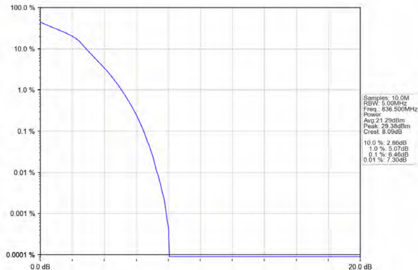
Band26b_5MHz_16QAM_MCH_836.5MHz_RB_25_0_NTNV
