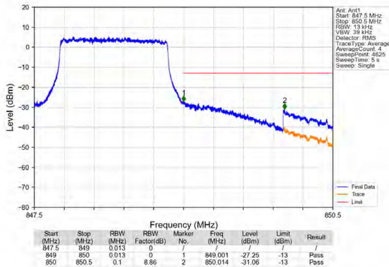
Band26b 1.4MHz QPSK HCH 848.3MHz RB 6 0 NTNV
