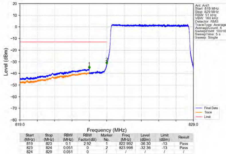
Band26b 5MHz 64QAM LCH 826.5MHz RB 25 0 NTN
