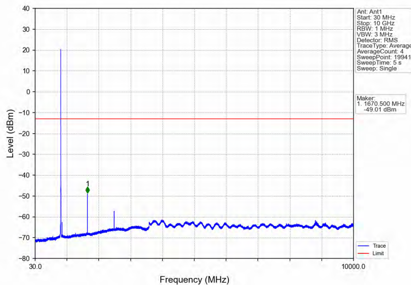
Band26b_3MHz_64QAM_MCH_836.5MHz_RB_1_0_NTNV
