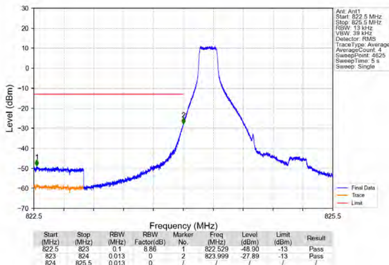
Band26b_1.4MHz_64QAM_LCH_824.7MHz_RB_1_0_NTNV
