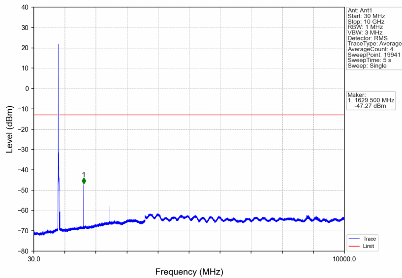
Band26c_15MHz_16QAM_LCH_821.5MHz_RB_75_0_NTNV
