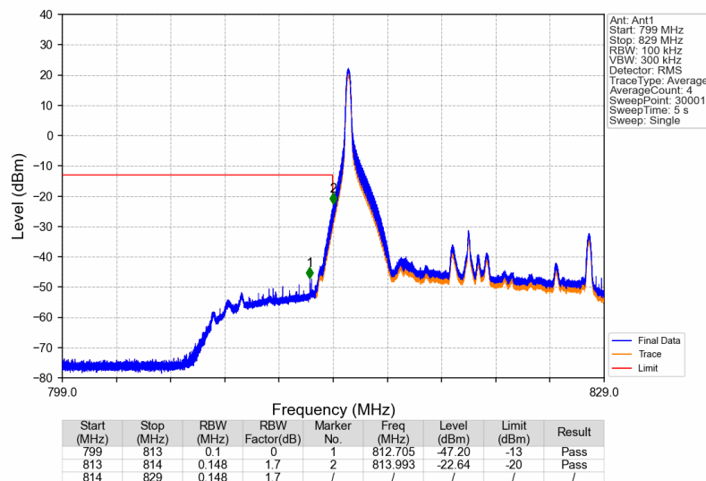
Band26c_15MHz_16QAM_LCH_821.5MHz_RB_1_0_NTNV
