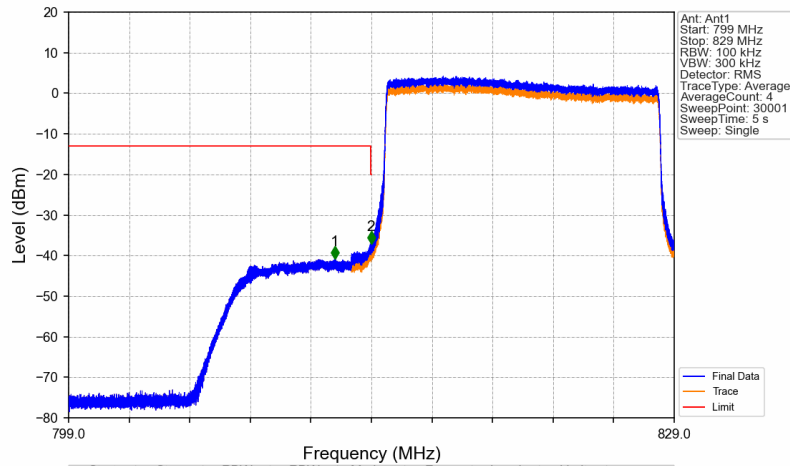
Band26c_15MHz_16QAM_LCH_821.5MHz_RB_75_0_NTNV
