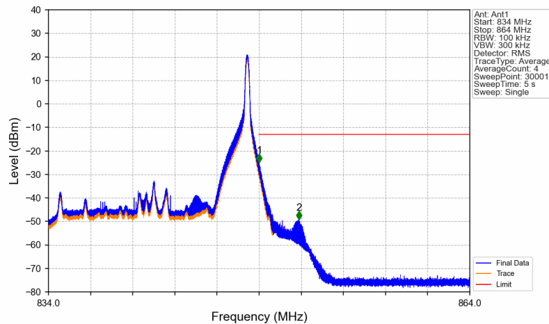
Band26c_15MHz_64QAM_HCH_841.5MHz_RB_1_74_NTNV
