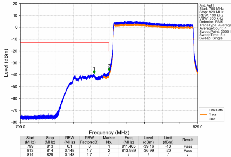
Band26c_15MHz_QPSK_LCH_821.5MHz_RB_75_0_NTNV
