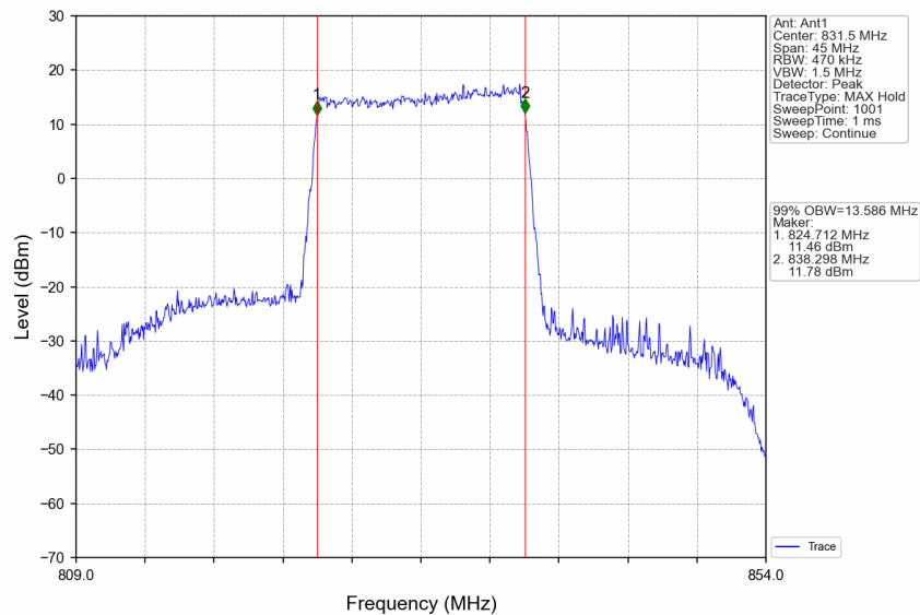
Band26c_15MHz_64QAM_MCH_831.5MHz_RB_75_0_NTNV
