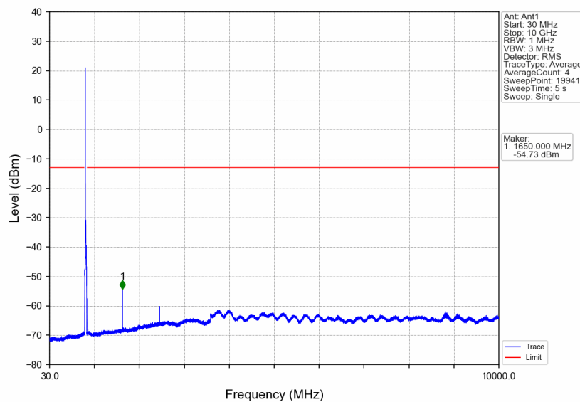
Band26c_15MHz_64QAM_MCH_831.5MHz_RB_1_0_NTNV
