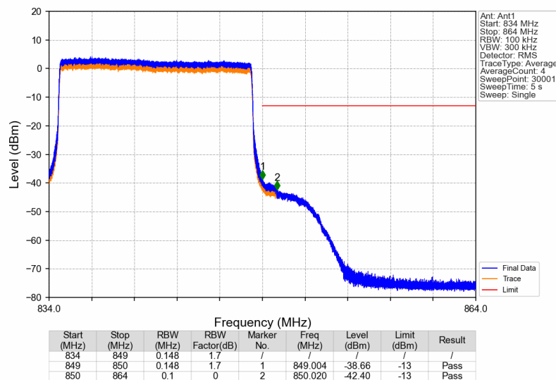
Band26c_15MHz_16QAM_HCH_841.5MHz_RB_75_0_NTNV
