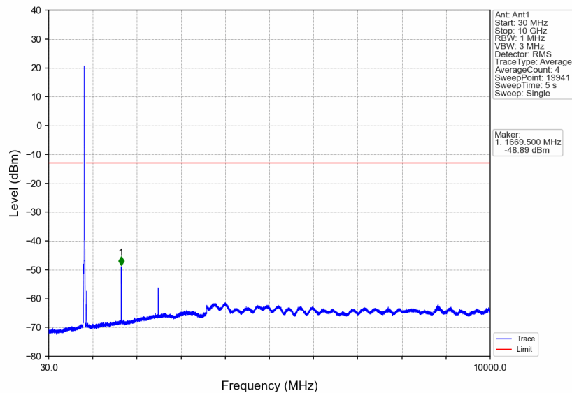
Band26c_15MHz_64QAM_HCH_841.5MHz_RB_1_74_NTNV
