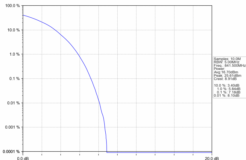
Band26c_15MHz_64QAM_HCH_841.5MHz_RB_75_0_NTNV
