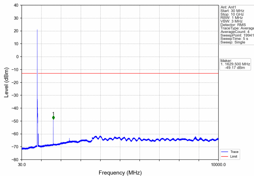
Band26c_15MHz_64QAM_LCH_821.5MHz_RB_1_0_NTNV
