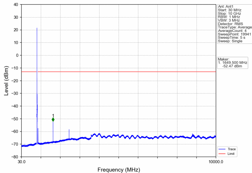
Band26c_15MHz_16QAM_HCH_841.5MHz_RB_1_0_NTNV
