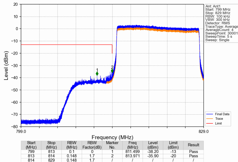
Band26c_15MHz_64QAM_LCH_821.5MHz_RB_75_0_NTNV
