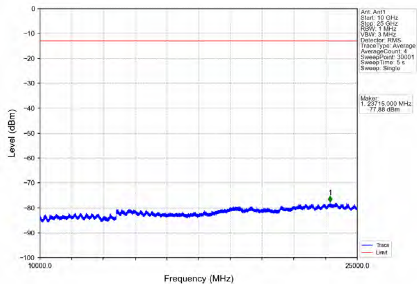
Band30_10MHz_16QAM_HCH_2310MHz_RB_1_0_NTNV
