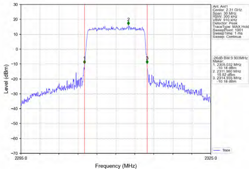
Band30_10MHz_64QAM_HCH_2310MHz_RB_50_0_NTNV
