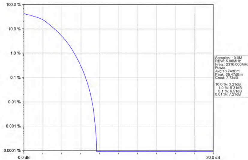
Band30_10MHz_16QAM_HCH_2310MHz_RB_50_0_NTNV
