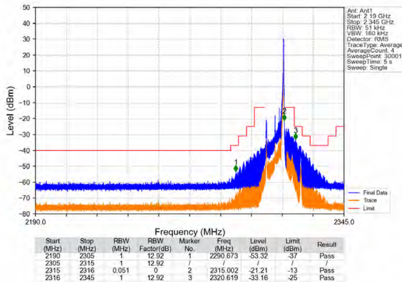
Band30_5MHz_16QAM_HCH_2312.5MHz_RB_1_24_NTNV
