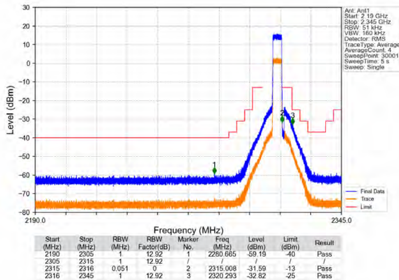
Band30_5MHz_16QAM_HCH_2312.5MHz_RB_25_0_NTNV
