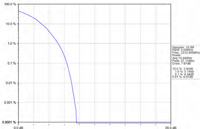
Band30_5MHz_64QAM_HCH_2312.5MHz_RB_25_0_NTNV
