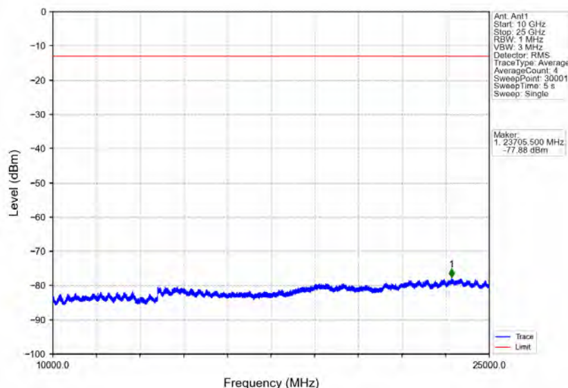
Band30_5MHz_QPSK_HCH_2312.5MHz_RB_1_0_NTNV
