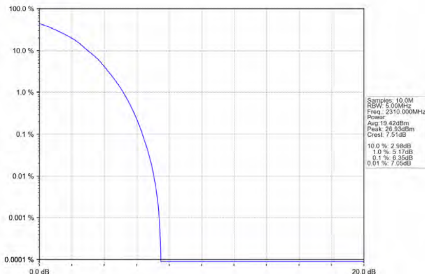
Band30_5MHz_64QAM_MCH_2310MHz_RB_25_0_NTNV
