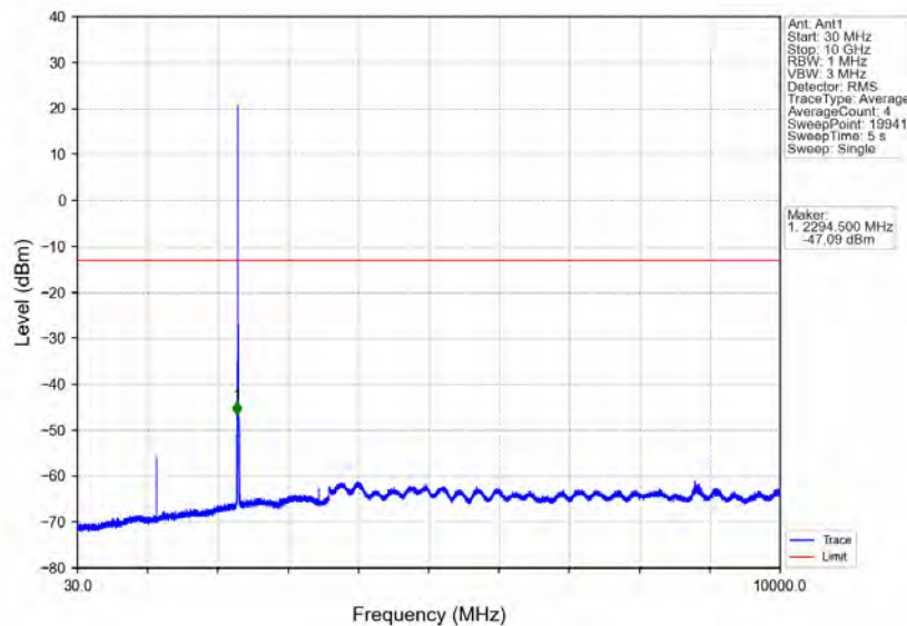
Band30_5MHz_16QAM_LCH_2307.5MHz_RB_1_0_NTNV
