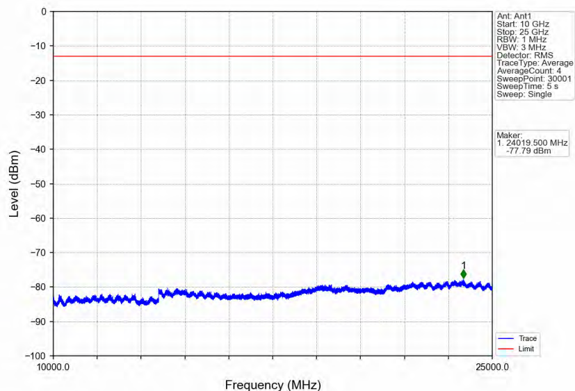
Band30_10MHz_64QAM_MCH_2310MHz_RB_1_0_NTNV
