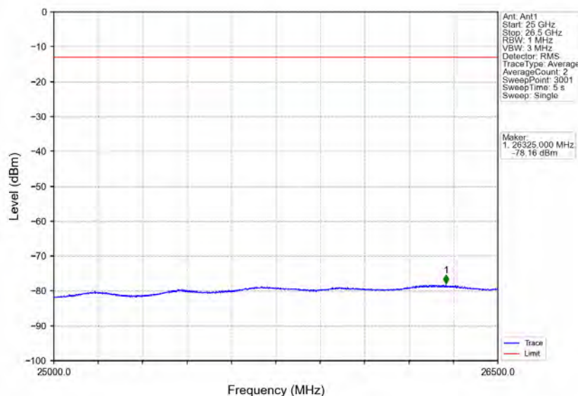
Band30_5MHz_64QAM_HCH_2312.5MHz_RB_1_24_NTNV
