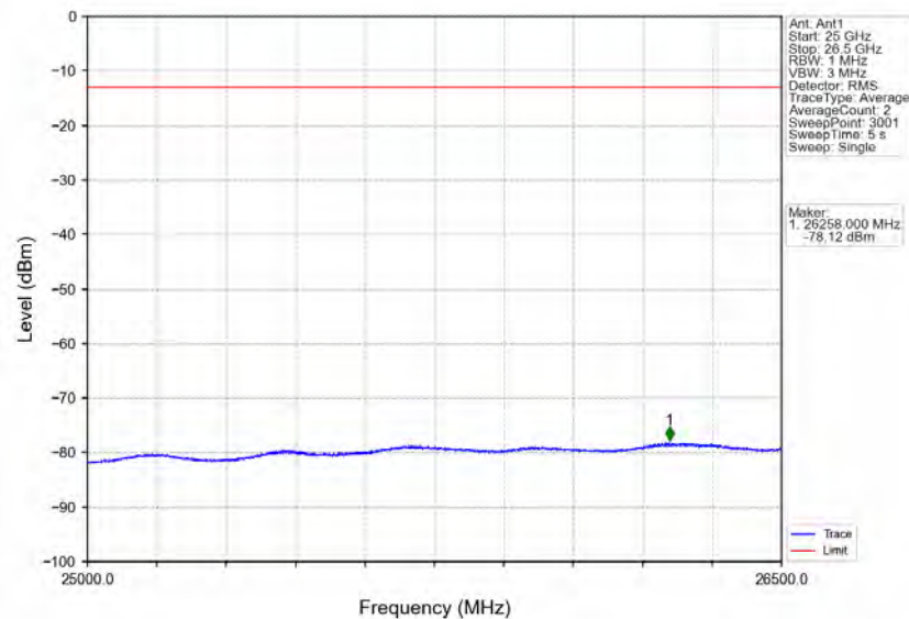
Band30_5MHz_16QAM_HCH_2312.5MHz_RB_1_0_NTNV
