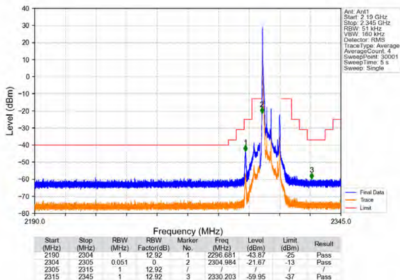
Band30_5MHz_64QAM_LCH_2307.5MHz_RB_1_0_NTNV
