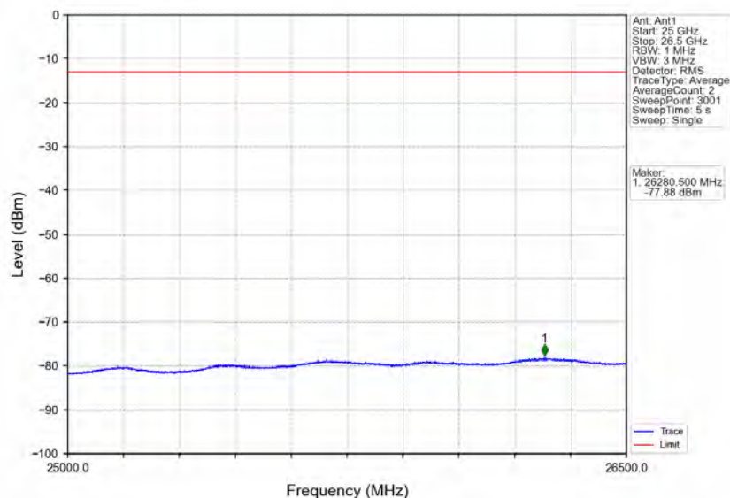
Band30_10MHz_16QAM_HCH_2310MHz_RB_1_0_NTNV
