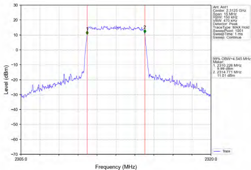
Band30_5MHz_16QAM_HCH_2312.5MHz_RB_25_0_NTNV
