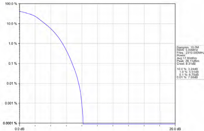
Band30_10MHz_64QAM_MCH_2310MHz_RB_50_0_NTNV
