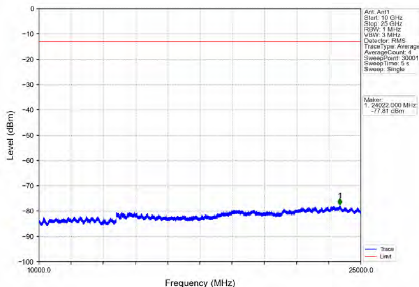
Band30_5MHz_64QAM_HCH_2312.5MHz_RB_1_0_NTNV
