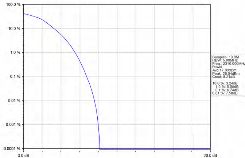
Band30_10MHz_64QAM_LCH_2310MHz_RB_50_0_NTNV
