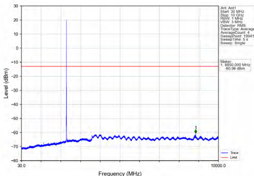
Band30_5MHz_64QAM_MCH_2310MHz_RB_1_0_NTNV
