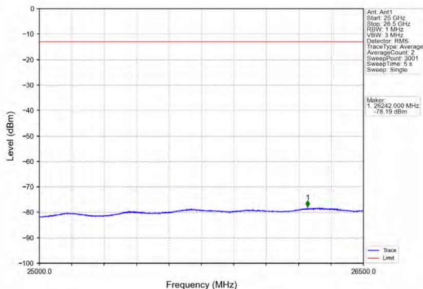
Band30_10MHz_64QAM_HCH_2310MHz_RB_1_49_NTNV
