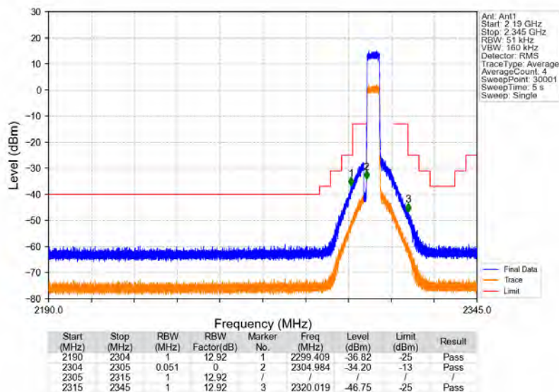
Band30_5MHz_64QAM_MCH_2310MHz_RB_1_0_NTNV
