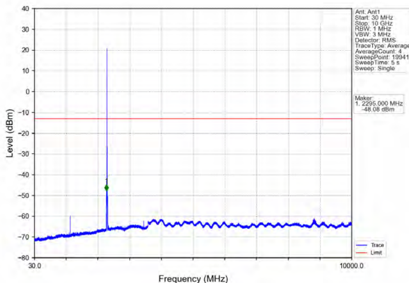
Band30_5MHz_16QAM_MCH_2310MHz_RB_1_0_NTNV
