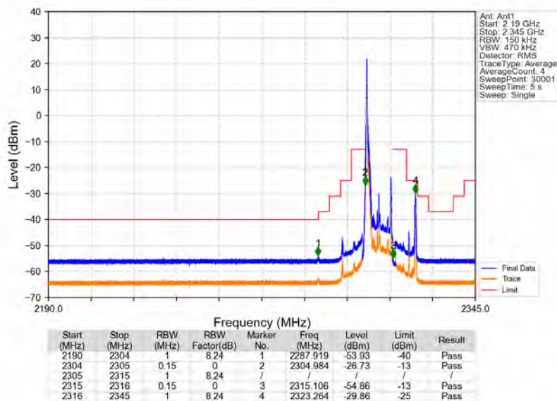
Band30_10MHz_64QAM_LCH_2310MHz_RB_1_0_NTNV
