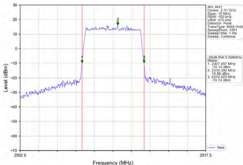
Band30_5MHz_64QAM_MCH_2310MHz_RB_25_0_NTNV
