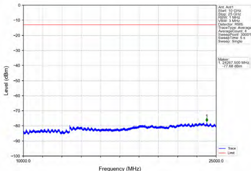
Band30_5MHz_16QAM_MCH_2310MHz_RB_1_0_NTNV
