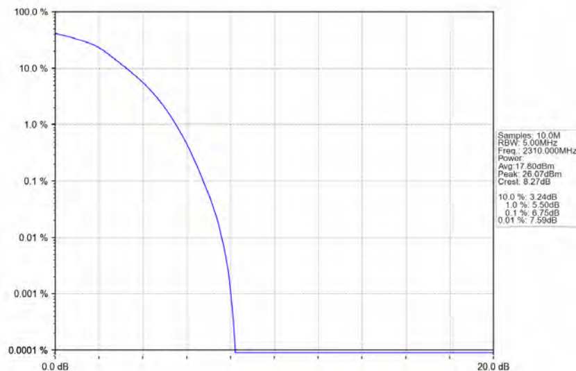
Band30_10MHz_64QAM_HCH_2310MHz_RB_50_0_NTNV
