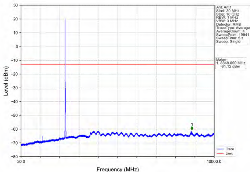
Band30_10MHz_64QAM_HCH_2310MHz_RB_1_0_NTNV
