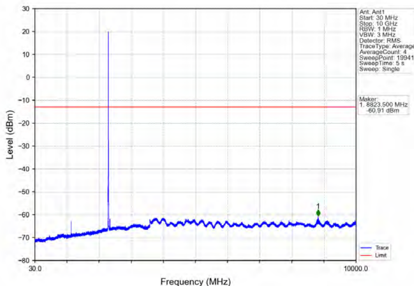
Band30_5MHz_64QAM_HCH_2312.5MHz_RB_1_0_NTNV
