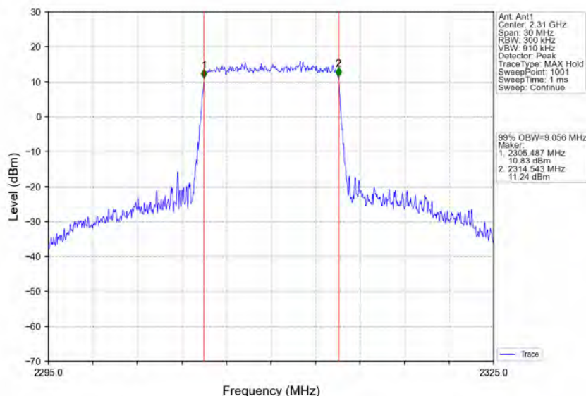
Band30_10MHz_64QAM_HCH_2310MHz_RB_50_0_NTNV
