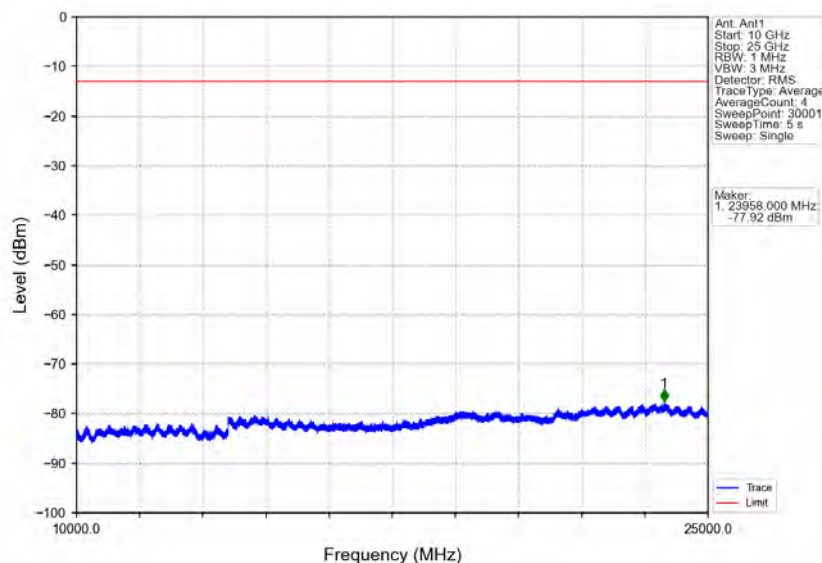
Band30_5MHz_64QAM_LCH_2307.5MHz_RB_1_0_NTNV
