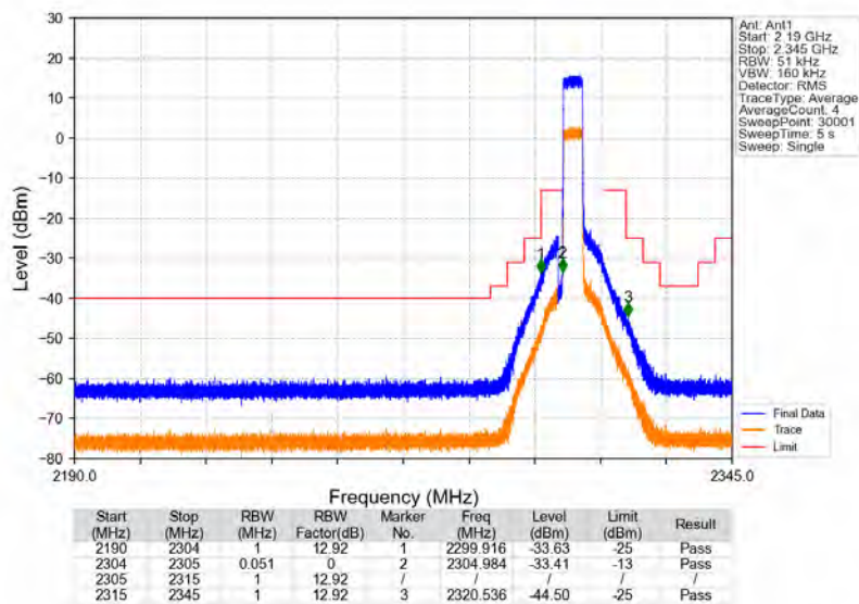
Band30_5MHz_16QAM_LCH_2307.5MHz_RB_25_0_NTNV
