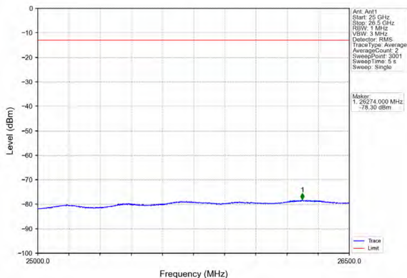
Band30_5MHz_QPSK_HCH_2312.5MHz_RB_1_24_NTNV
