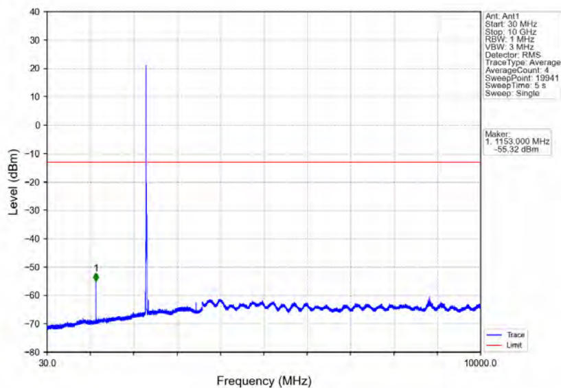
Band30_10MHz_16QAM_HCH_2310MHz_RB_1_0_NTNV
