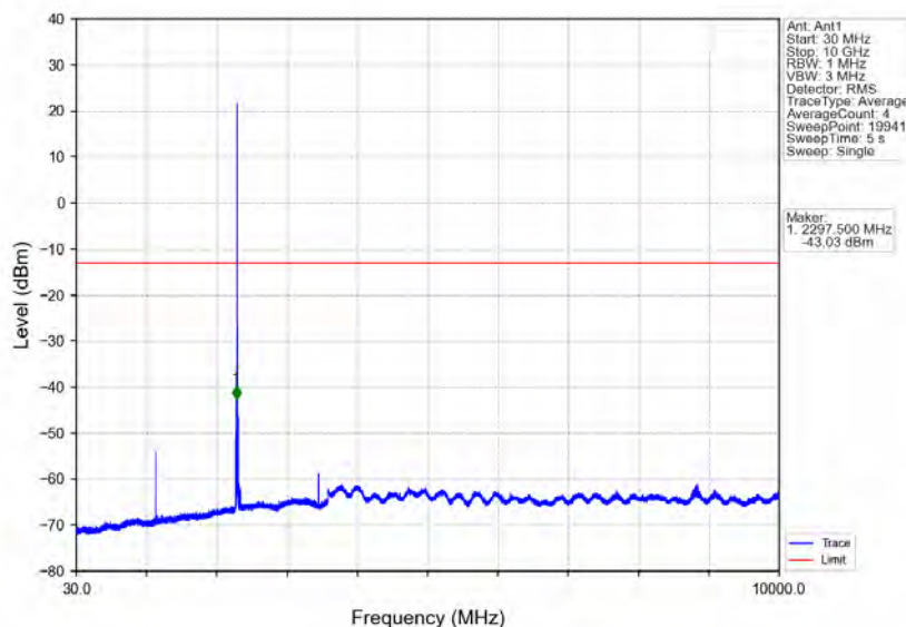
Band30_5MHz_QPSK_HCH_2312.5MHz_RB_1_0_NTNV
