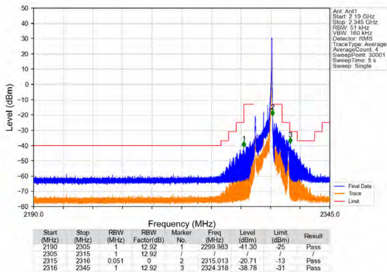
Band30_5MHz_QPSK_HCH_2312.5MHz_RB_1_24_NTNV
