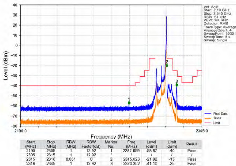
Band30_5MHz_64QAM_HCH_2312.5MHz_RB_1_24_NTNV
