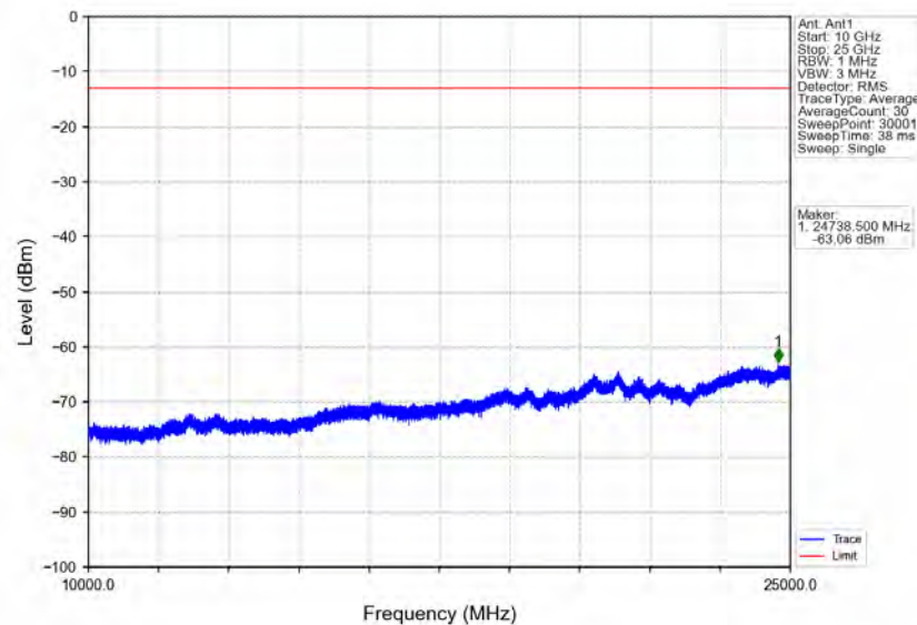
Band30_10MHz_64QAM_LCH_2310MHz_RB_1_0_NTNV
