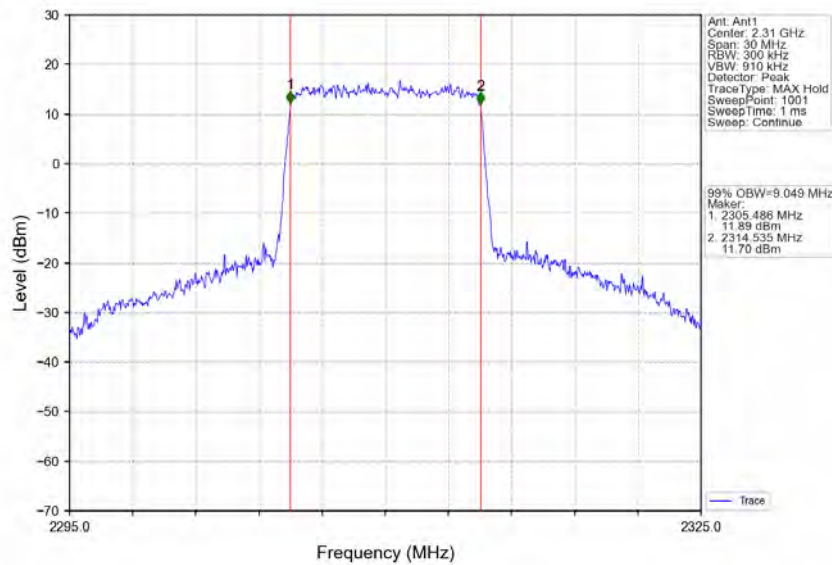
Band30_10MHz_64QAM_LCH_2310MHz_RB_50_0_NTNV
