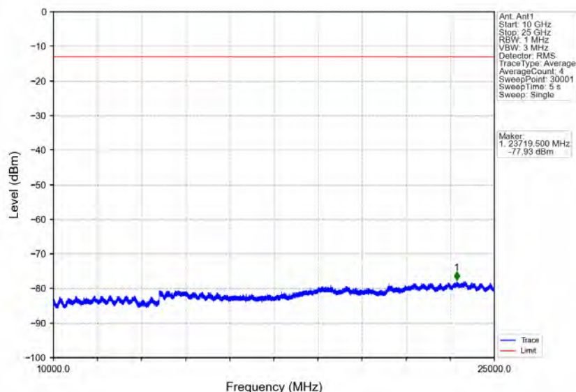
Band30_10MHz_64QAM_HCH_2310MHz_RB_1_0_NTNV
