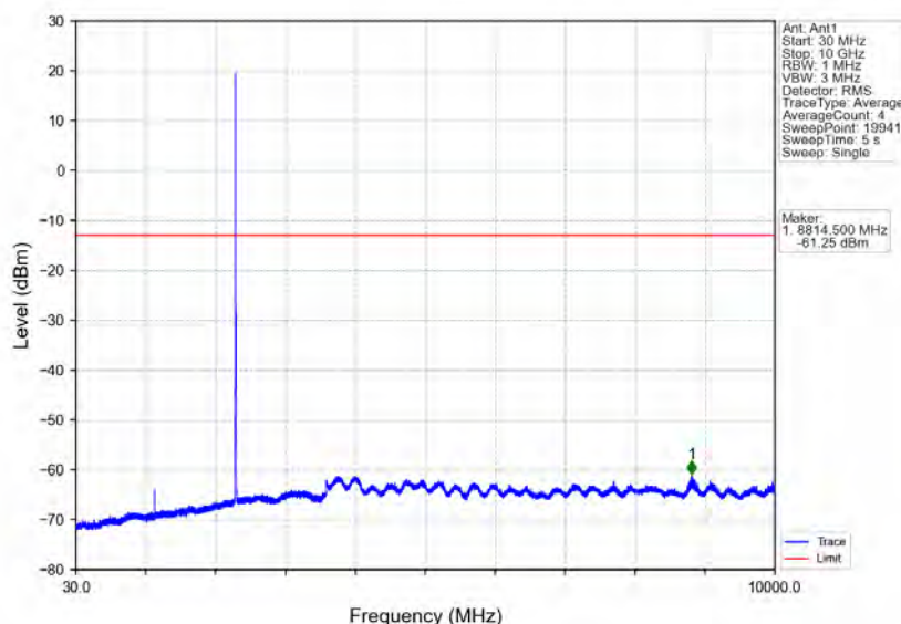
Band30_5MHz_64QAM_LCH_2307.5MHz_RB_1_0_NTNV
