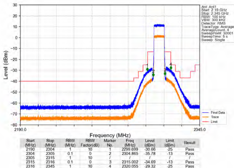
Band30_10MHz_16QAM_HCH_2310MHz_RB_50_0_NTNV
