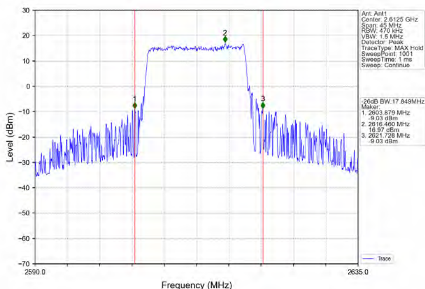
Band38_15MHz 16QAM HCH 2612.5MHz RB 75 0 NTNV
