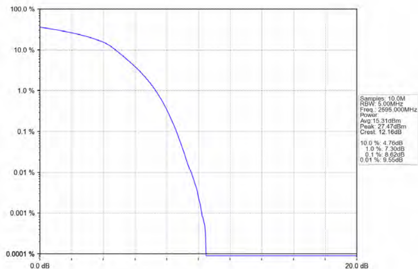
Band38 10MHz 64QAM MCH 2595MHz RB 50 0 NTN
