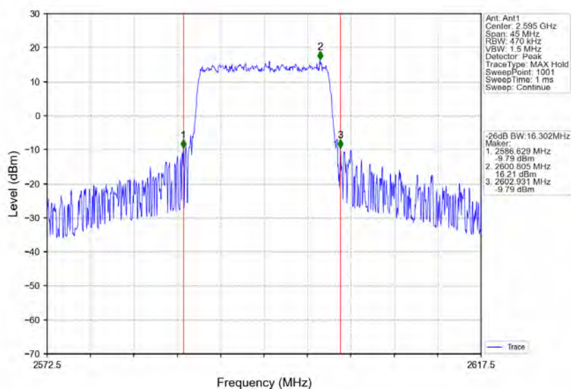
Band38 15MHz 64QAM MCH 2595MHz RB 75 0 NTN
