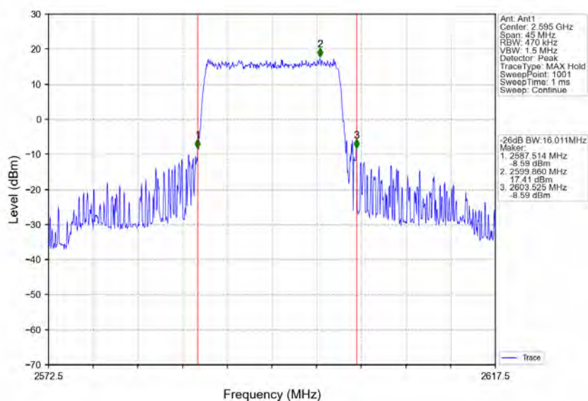
Band38_15MHz_QPSK_MCH_2595MHz_RB_75_0_NTNV
