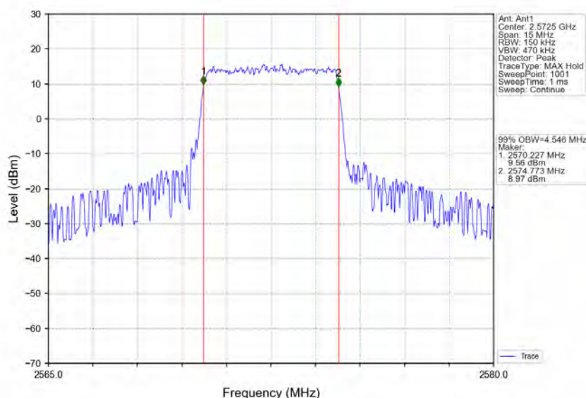
Band38 5MHz 16QAM LCH 2572.5MHz RB 25 0 NTN
