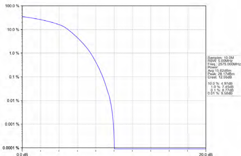
Band38 10MHz 16QAM LCH 2575MHz RB 50 0 NTV
