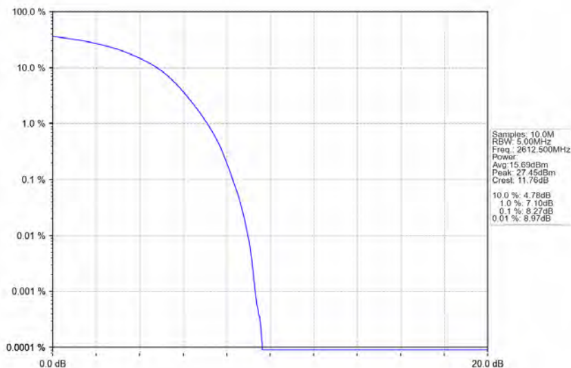
Band38 15MHz QPSK HCH 2612.5MHz RB 75 0 NTNV
