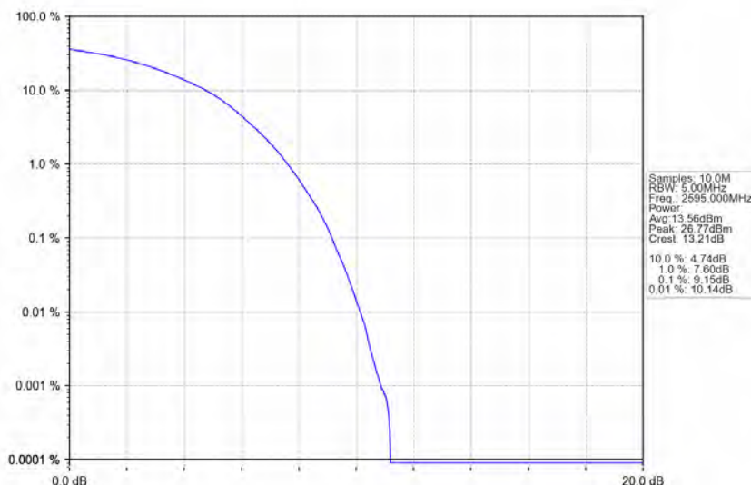
Band38 15MHz 64QAM MCH 2595MHz RB 75 0 NTNV
