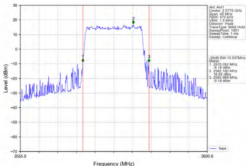
Band38 15MHz 16QAM LCH 2577.5MHz RB 75 0 NTNV
