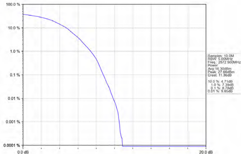
Band38 5MHz 64QAM LCH 2572.5MHz RB 25 0 NTNV
