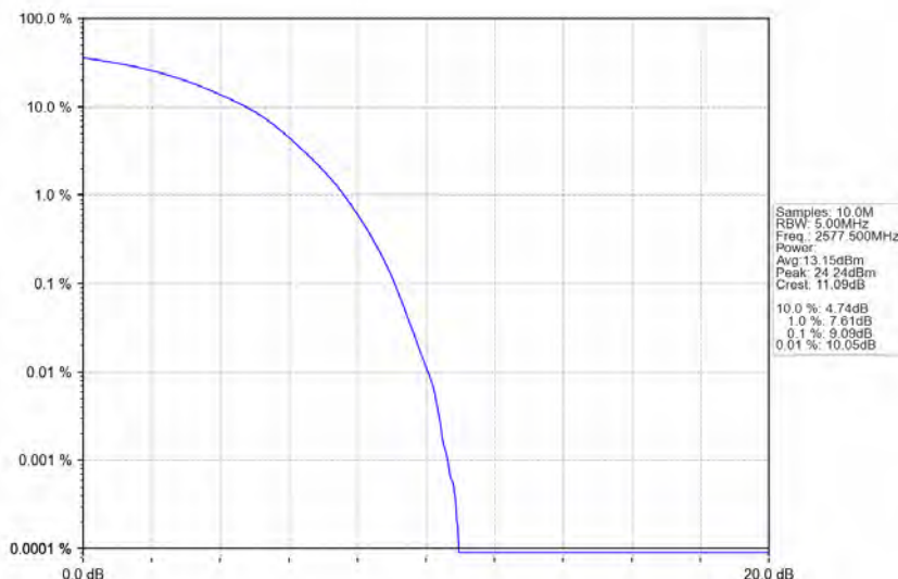
Band38 15MHz 64QAM LCH 2577.5MHz RB 75 0 NTNV
