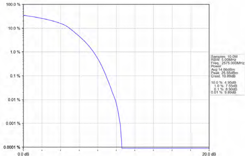
Band38 10MHz 64QAM LCH 2575MHz RB 50 0 NTN
