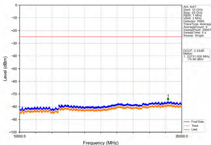
Band38_20MHz_64QAM_MCH_2595MHz_RB_1_0_NTNV
