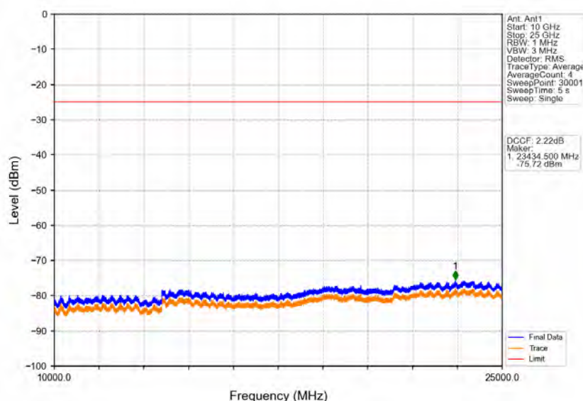
Band38_20MHz_64QAM_HCH_2610MHz_RB_1_0_NTNV
