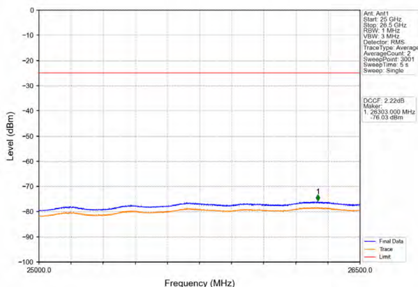
Band38_20MHz_64QAM_LCH_2580MHz_RB_1_0_NTNV
