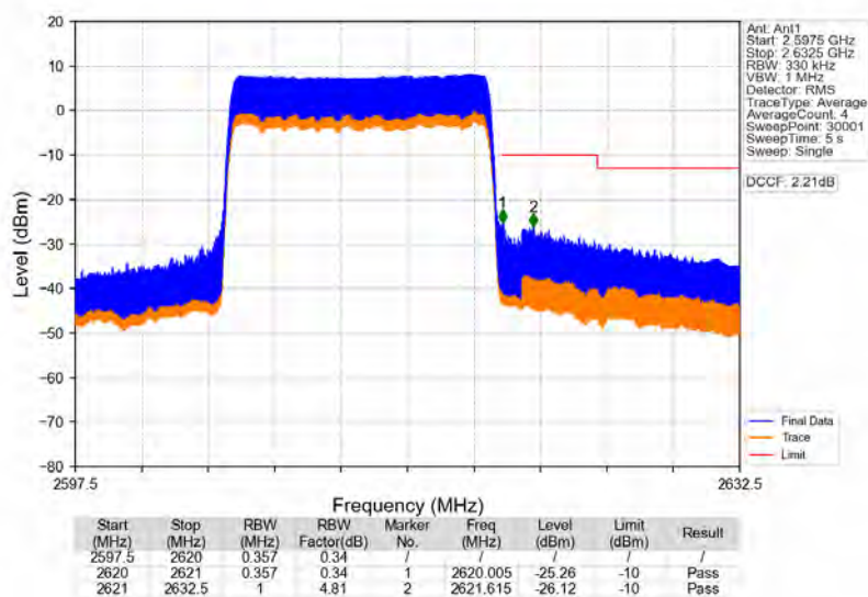
Band38_15MHz_16QAM_HCH_2612.5MHz_RB_75_0_NTNV
