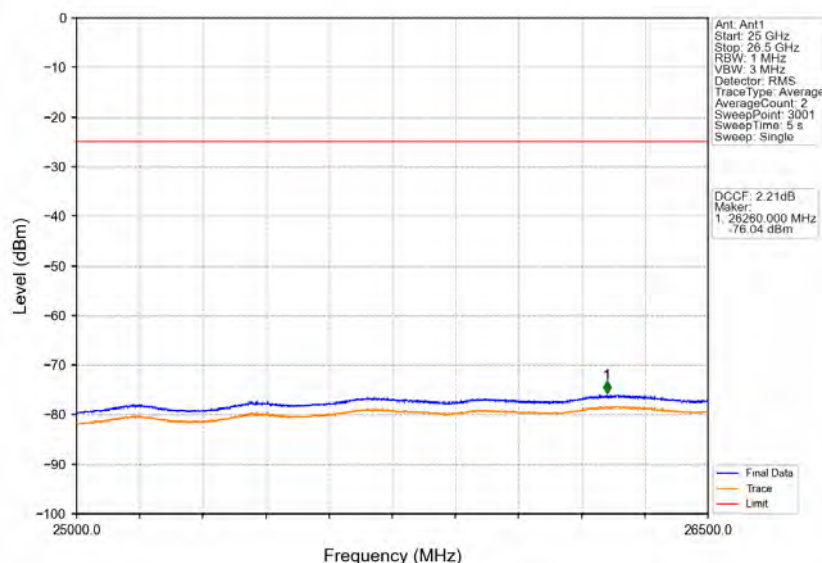
Band38_5MHz_64QAM_LCH_2572.5MHz_RB_1_0 NTN
