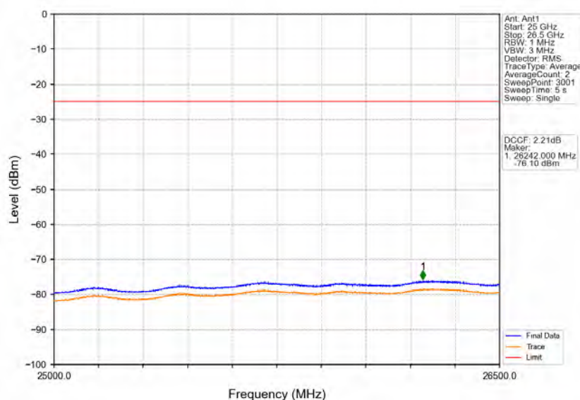
Band38_15MHz_64QAM_HCH_2612.5MHz_RB_1_74_NTNV
