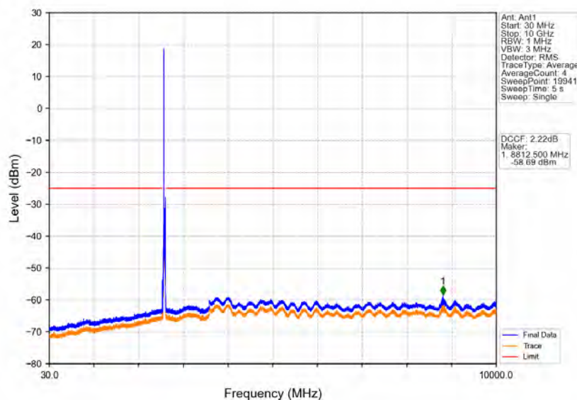
Band38_20MHz_64QAM_MCH_2595MHz_RB_1_0_NTNV
