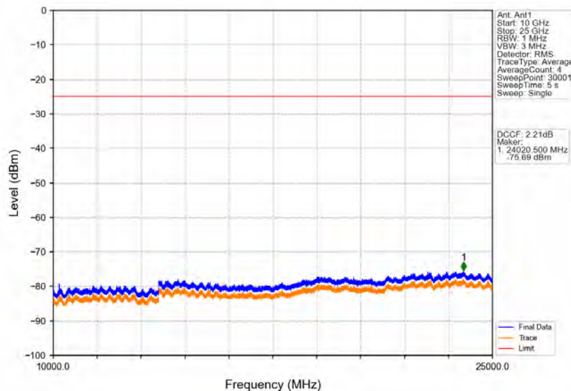
Band38_10MHz_16QAM_LCH_2575MHz_RB_1_0_NTNV
