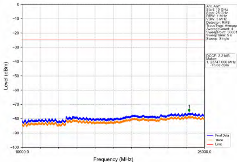
Band38_10MHz_16QAM_MCH_2595MHz_RB_1_0_NTNV
