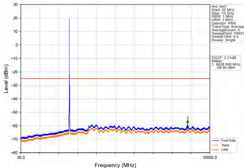
Band38_15MHz_64QAM_MCH_2595MHz_RB_1_0_NTNV
