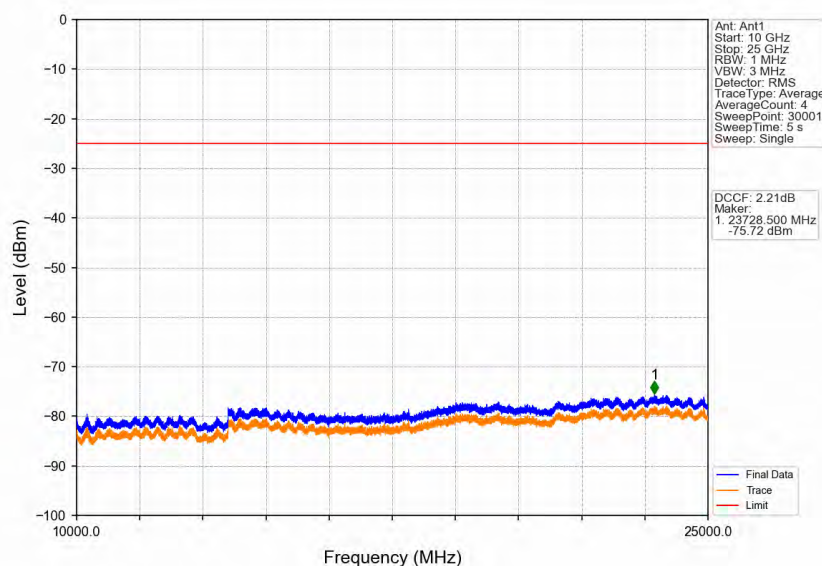
Band38_15MHz_QPSK_LCH_2577.5MHz_RB_1_0_NTNV
