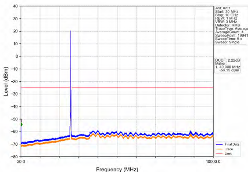
Band38_20MHz_64QAM_HCH_2610MHz_RB_1_0_NTNV
