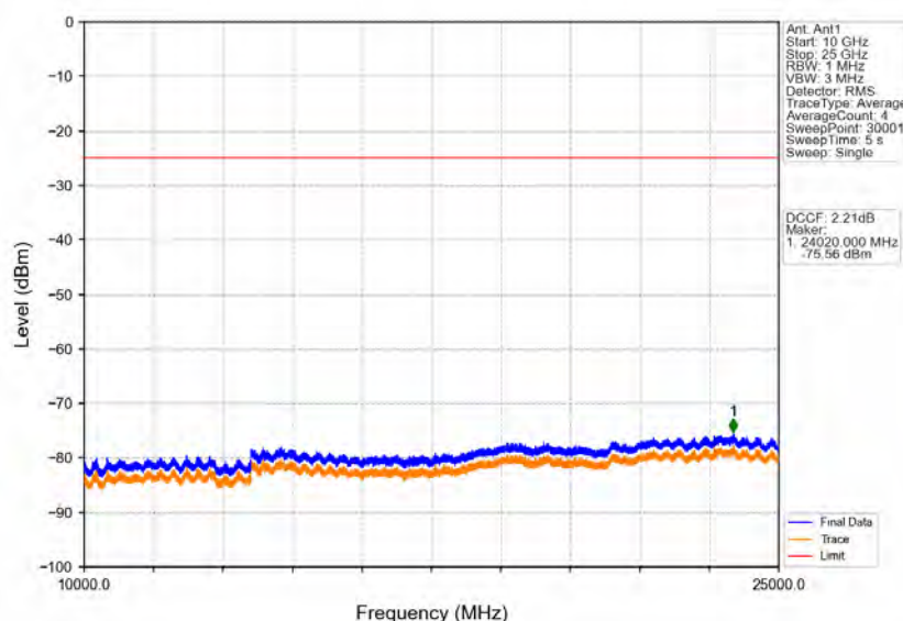
Band38_15MHz_QPSK_HCH_2612.5MHz_RB_1_0_NTNV
