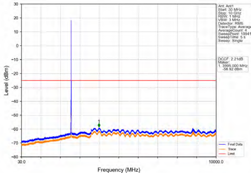
Band38_10MHz_16QAM_LCH_2575MHz_RB_1_0_NTNV
