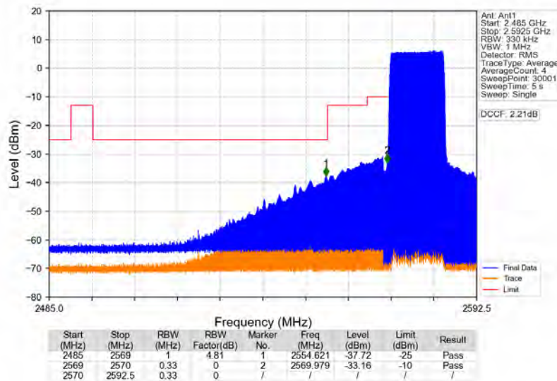
Band38_15MHz_64QAM_LCH_2577.5MHz_RB_75_0_NTNV
