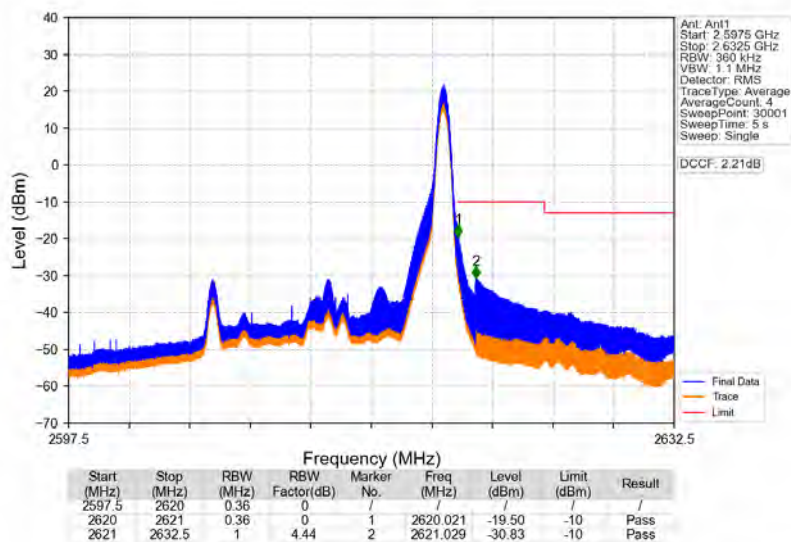
Band38_15MHz_64QAM_HCH_2612.5MHz_RB_1_74_NTNV
