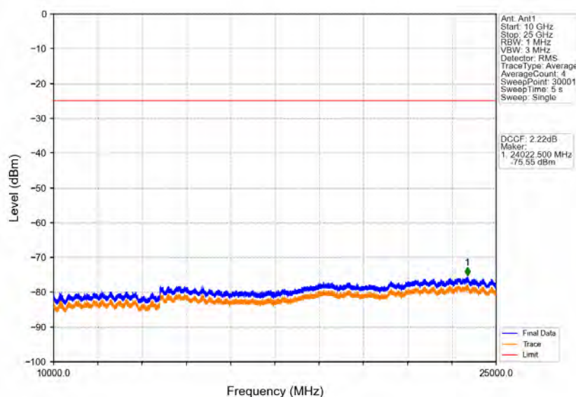
Band38_20MHz_64QAM_LCH_2580MHz_RB_1_0_NTNV
