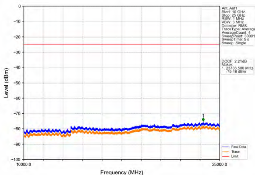
Band38_10MHz_64QAM_LCH_2575MHz_RB_1_0_NTNV
