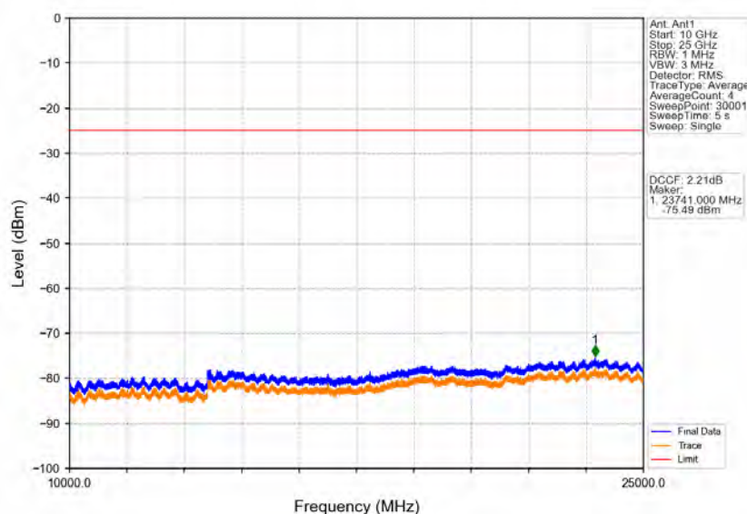
Band38_10MHz_16QAM_HCH_2615MHz_RB_1_0_NTNV
