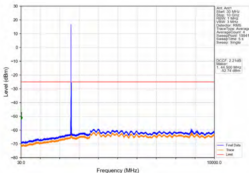
Band38_15MHz_QPSK_HCH_2612.5MHz_RB_1_0_NTNV
