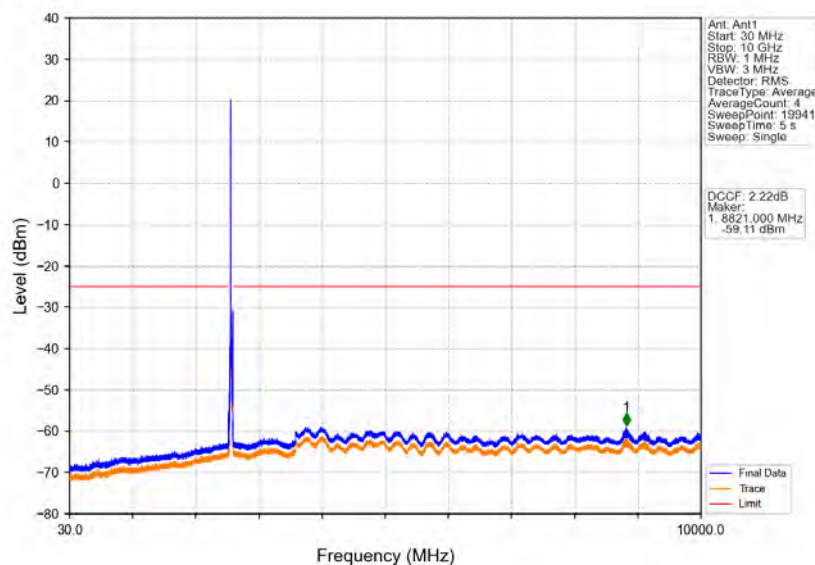
Band38_20MHz_64QAM_LCH_2580MHz_RB_1_0_NTNV
