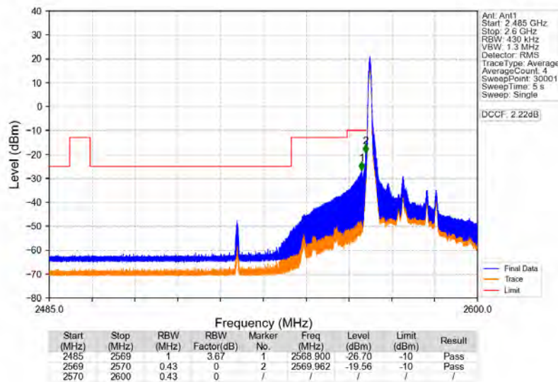
Band38_20MHz_64QAM_LCH_2580MHz_RB_1_0_NTNV
