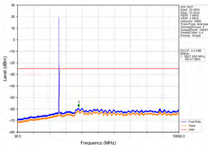
Band38_15MHz_16QAM_MCH_2595MHz_RB_1_0_NTNV
