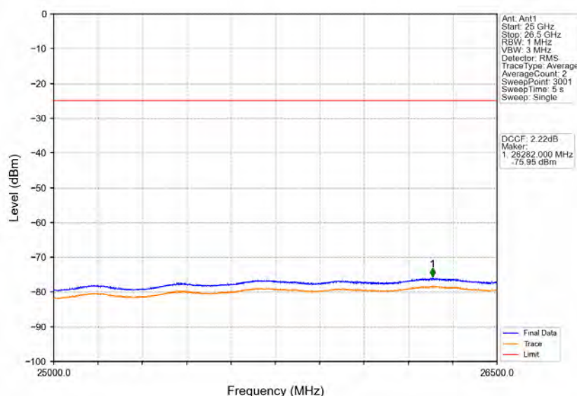
Band38_20MHz_64QAM_MCH_2595MHz_RB_1_0_NTNV
