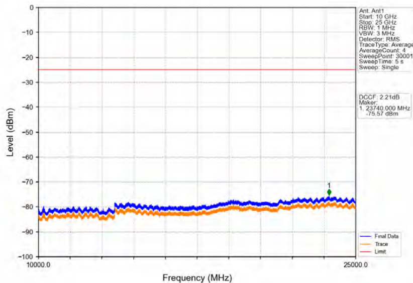
Band38_15MHz_64QAM_MCH_2595MHz_RB_1_0_NTNV
