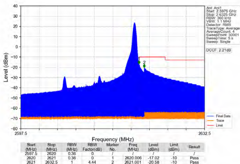
Band38_15MHz_16QAM_HCH_2612.5MHz_RB_1_74_NTNV
