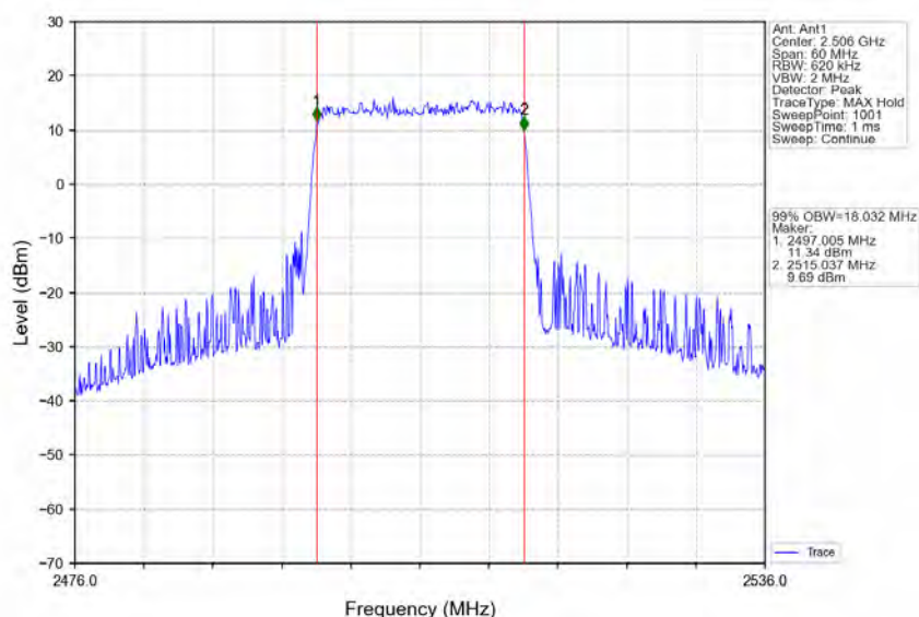
Band41 20MHz 64QAM LCH 2506MHz RB 100 0 NTN
