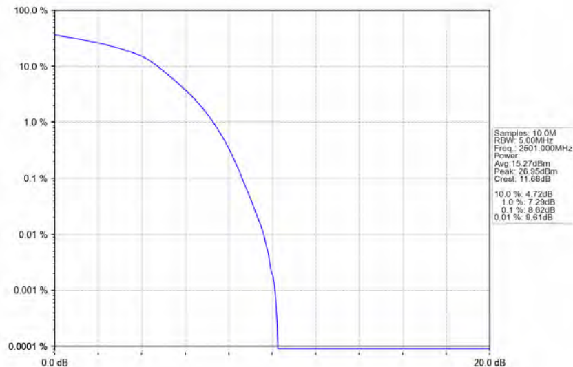
Band41 10MHz 64QAM LCH 2501MHz RB 50 0 NTN
