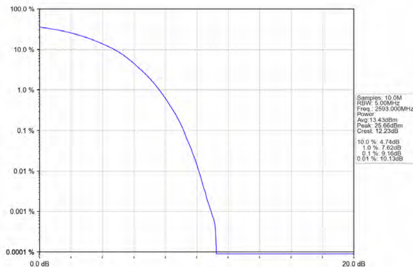
Band41_15MHz_64QAM_MCH_2593MHz_RB_75_0_NTNV
