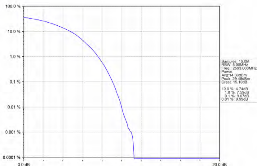
Band41_15MHz_16QAM_MCH_2593MHz_RB_75_0_NTNV
