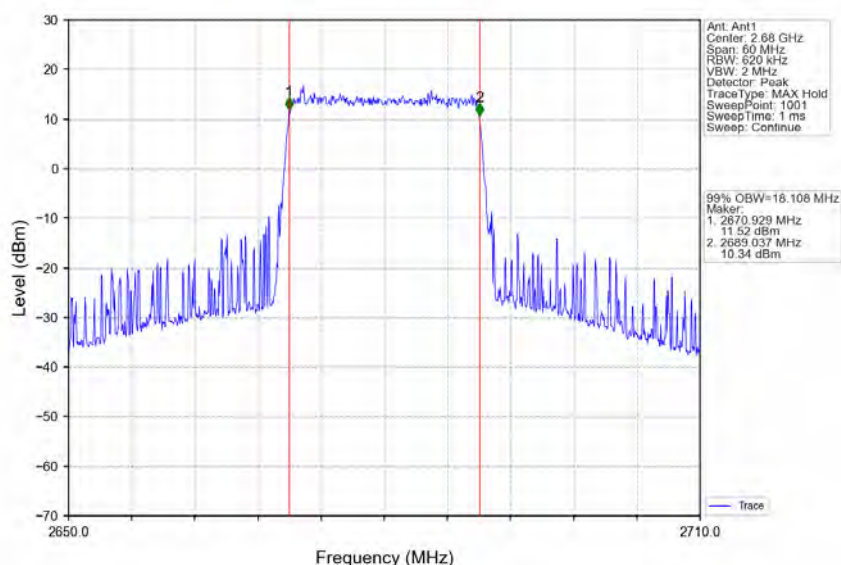
Band41_20MHz_64QAM_HCH_2680MHz_RB_100_0_NTNV
