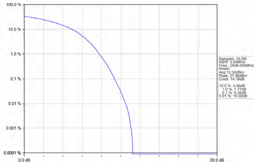
Band41_20MHz_64QAM_LCH_2506MHz_RB_100_0_NTNV
