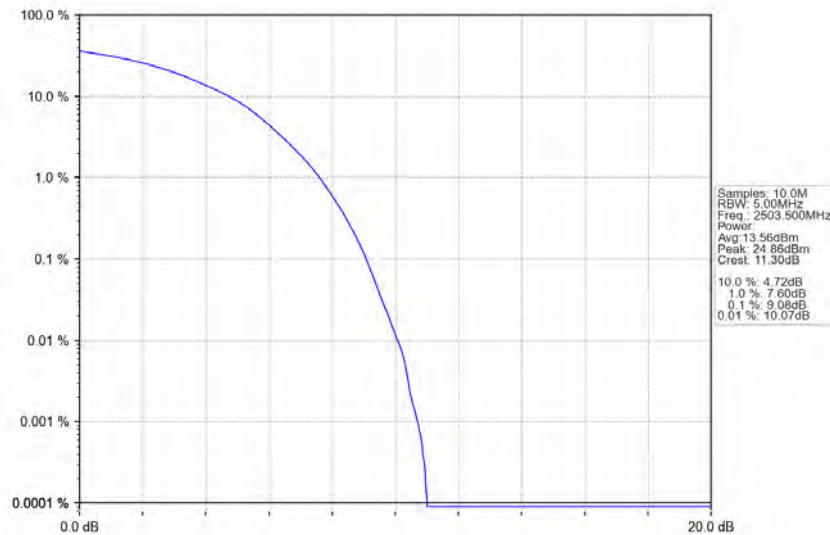
Band41_15MHz_64QAM_LCH_2503.5MHz_RB_75_0_NTNV
