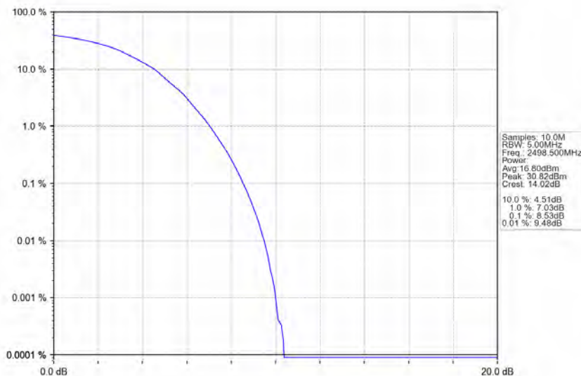
Band41 5MHz 64QAM LCH 2498.5MHz RB 25 0 NTNV
