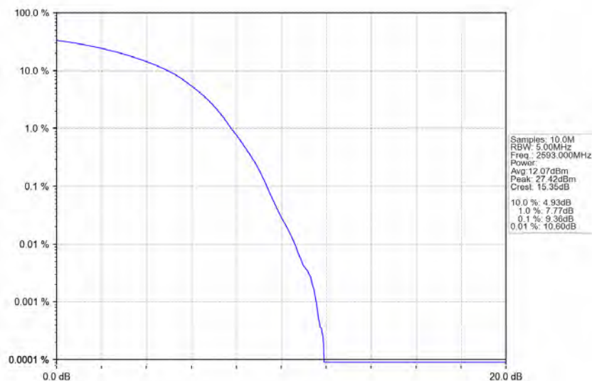
Band41_20MHz_64QAM_MCH_2593MHz_RB_100_0_NTNV
