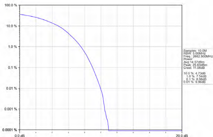
Band41_15MHz_16QAM_HCH_2682.5MHz_RB_75_0_NTNV
