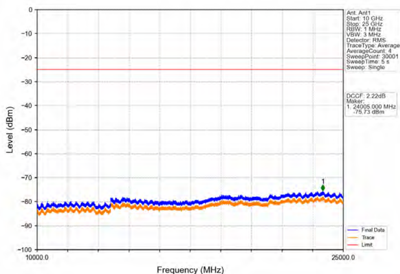
Band41_20MHz_64QAM_MCH_2593MHz_RB_1_0_NTNV
