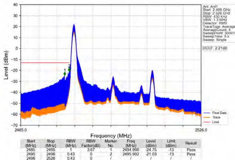
Band41_20MHz_64QAM_LCH_2506MHz_RB_1_0_NTNV
