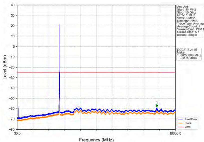
Band41_15MHz_64QAM_HCH_2682.5MHz_RB_1_0_NTNV
