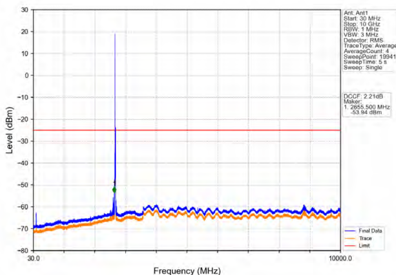
Band41_10MHz_64QAM_HCH_2685MHz_RB_1_0_NTNV
