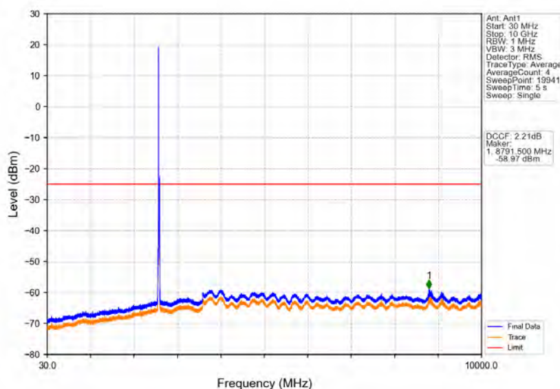
Band41_15MHz_16QAM_MCH_2593MHz_RB_1_0_NTNV
