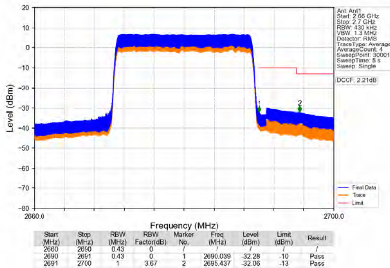
Band41 20MHz 16QAM HCH 2680MHz RB 100 0 NTNV
