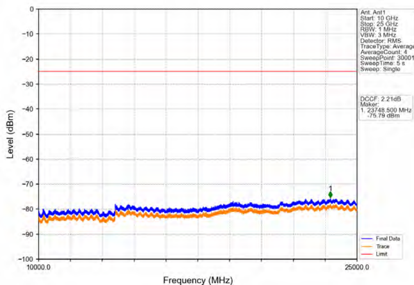
Band41_5MHz_16QAM_MCH_2593MHz_RB_1_0_NTNV
