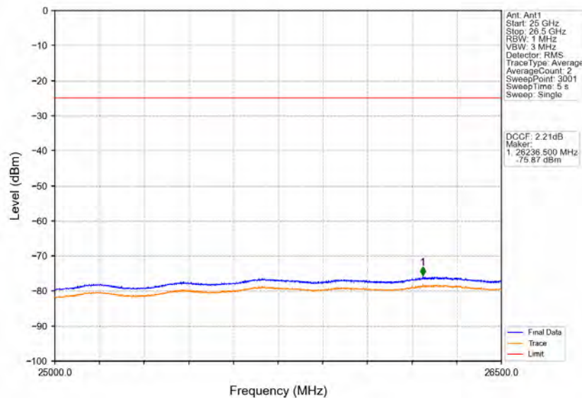
Band41 5MHz 64QAM HCH 2687.5MHz RB 1 24 NTNV
