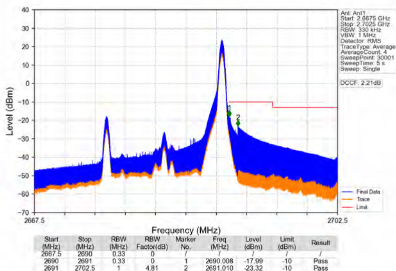
Band41_15MHz_16QAM_HCH_2682.5MHz_RB_1_74_NTNV
