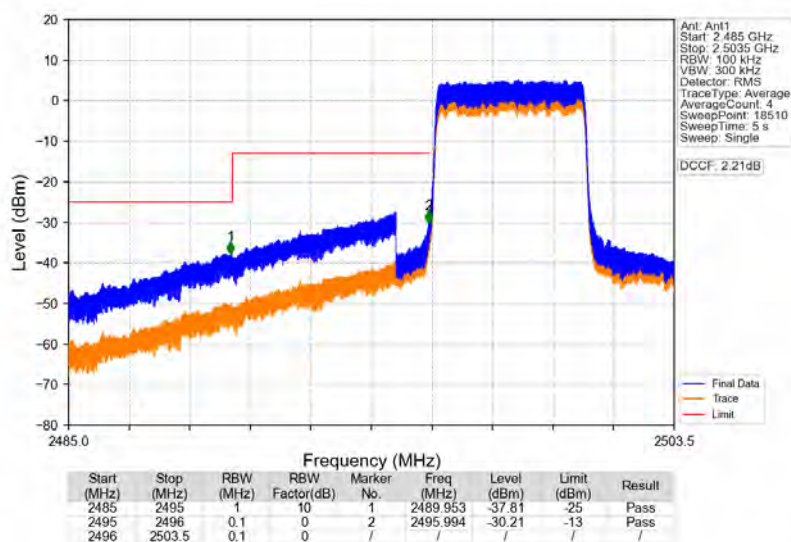
Band41 5MHz 64QAM LCH 2498.5MHz RB 25 0 NTNV
