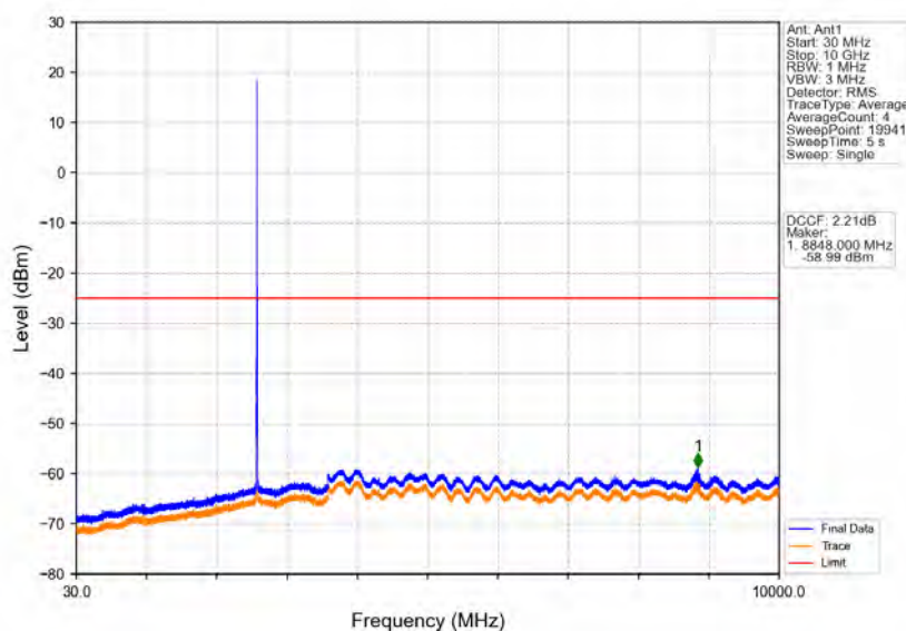
Band41 5MHz 64QAM MCH 2593MHz RB 1 0 NTNV
