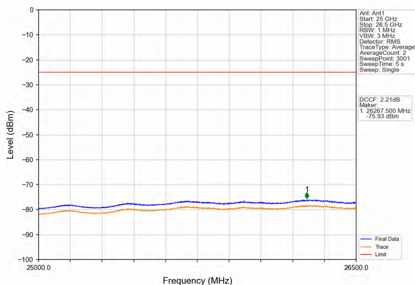
Band41 5MHz 16QAM LCH 2498.5MHz RB 25 0 NTNV
