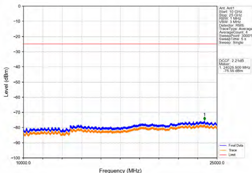
Band41 15MHz 16QAM LCH 2503.5MHz RB 1 0 NTNV
