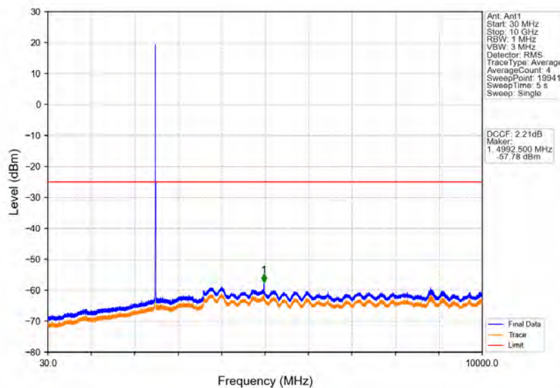
Band41 5MHz 16QAM LCH 2498.5MHz RB 1 0 NTNV
