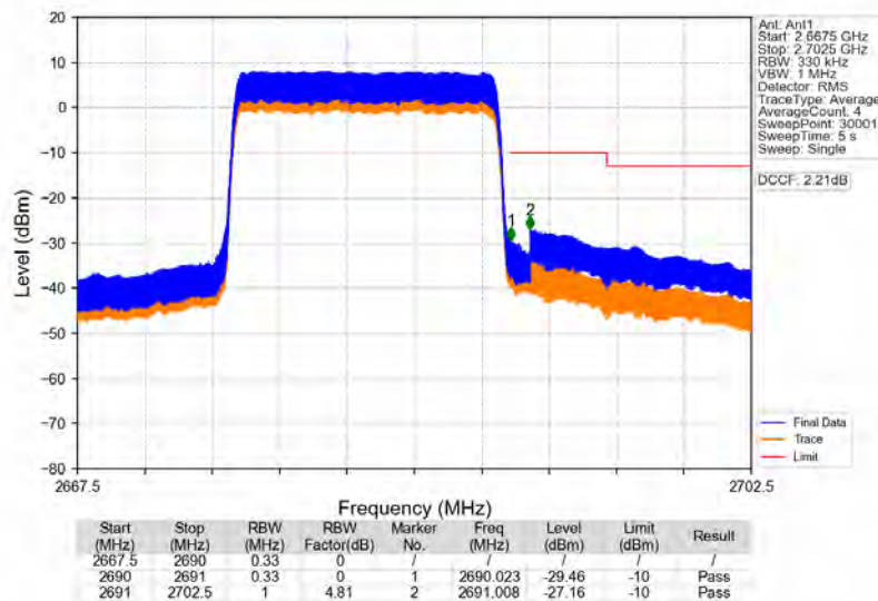
Band41 15MHz QPSK HCH 2682.5MHz RB 75 0 NTNV
