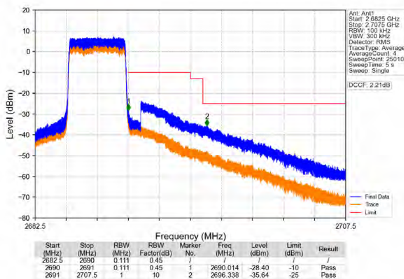
Band41 5MHz 16QAM HCH 2687.5MHz RB 25_0 NTNV
