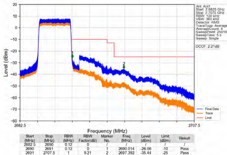
Band41 5MHz QPSK HCH 2687.5MHz RB 25 0 NTN
