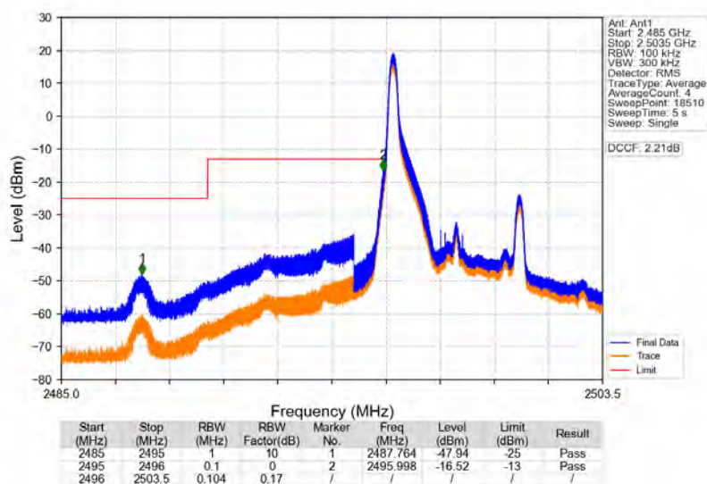
Band41 5MHz 64QAM LCH 2498.5MHz RB 1 0 NTNV
