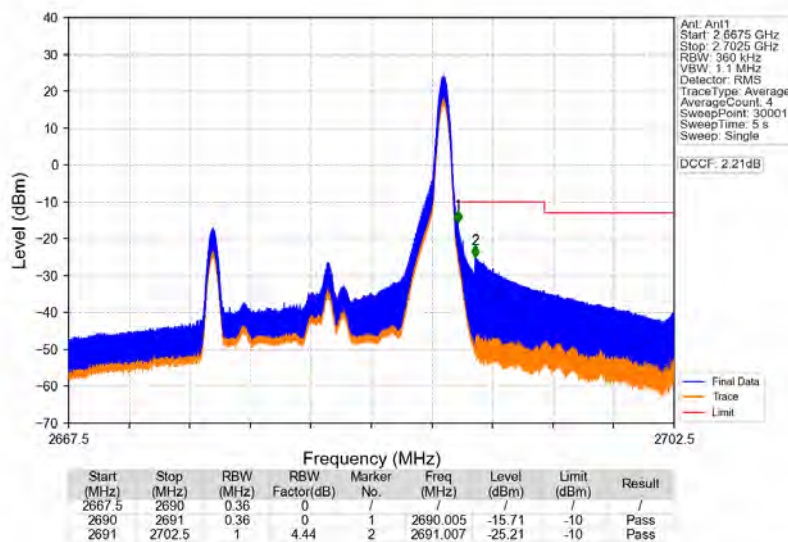
Band41 15MHz QPSK HCH 2682.5MHz RB 1 74 NTNV
