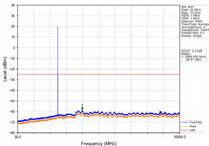
Band41 5MHz 64QAM LCH 2498.5MHz RB 1 0 NTNV
