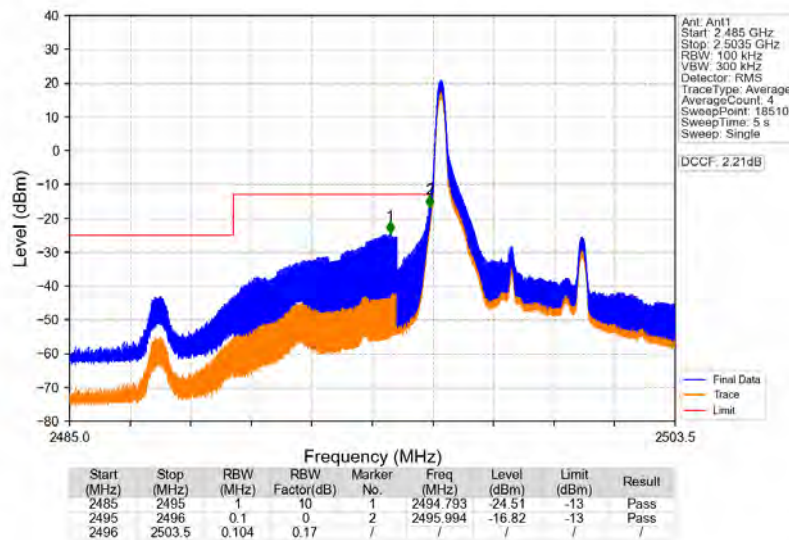
Band41 5MHz 16QAM LCH 2498.5MHz RB 1 0 NTN
