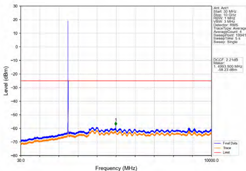
Band41_10MHz_64QAM_LCH_2501MHz_RB_1_0_NTNV
