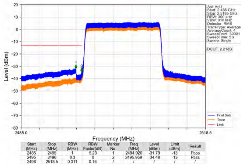
Band41_15MHz_64QAM_LCH_2503.5MHz_RB_75_0_NTNV
