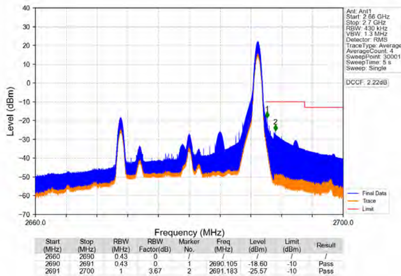
Band41 20MHz 16QAM HCH 2680MHz RB 1 99 NTNV
