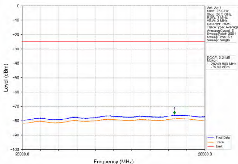
Band41_15MHz_16QAM_LCH_2503.5MHz_RB_75_0_NTNV
