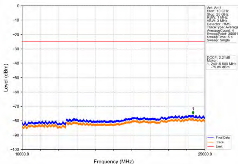
Band41_15MHz_64QAM_MCH_2593MHz_RB_1_0_NTNV
