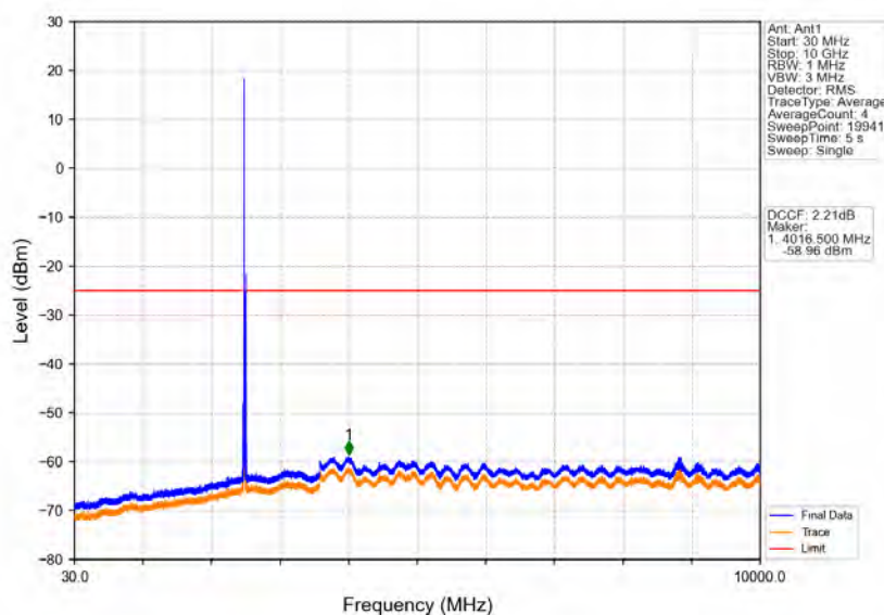
Band41 15MHz 64QAM LCH 2503.5MHz RB 1 0 NTNV
