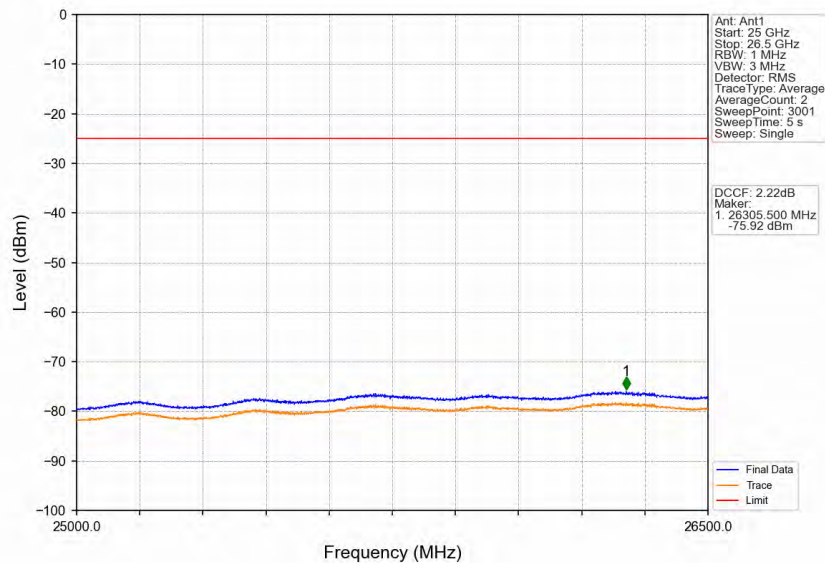
Band41_20MHz_64QAM_HCH_2680MHz_RB_1_99_NTNV
