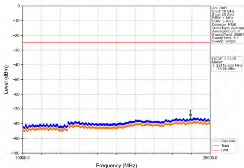
Band41_20MHz_64QAM_LCH_2506MHz_RB_1_0_NTNV
