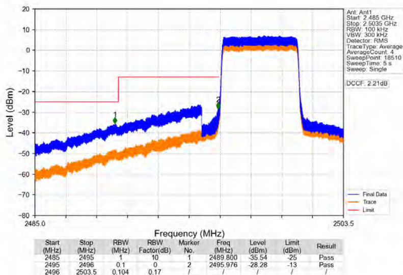
Band41 5MHz 16QAM LCH 2498.5MHz RB 25 0 NTNV
