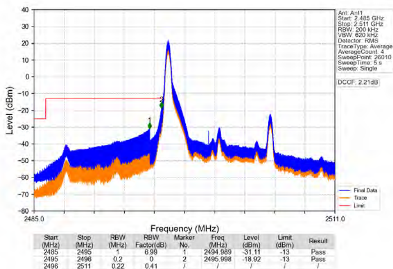
Band41_10MHz_64QAM_LCH_2501MHz_RB_1_0_NTNV
