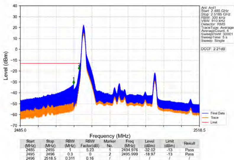
Band41 15MHz 64QAM LCH 2503.5MHz RB 1 0 NTNV
