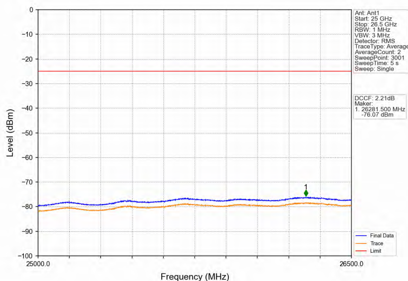
Band41 15MHz QPSK HCH 2682.5MHz RB 1 74 NTNV
