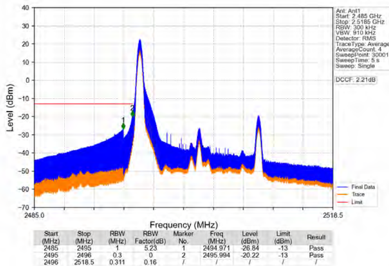
Band41 15MHz 16QAM LCH 2503.5MHz RB 1 0 NTNV
