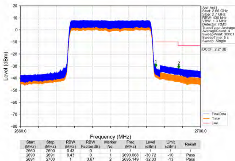
Band41 20MHz QPSK HCH 2680MHz RB 100 0 NTN
