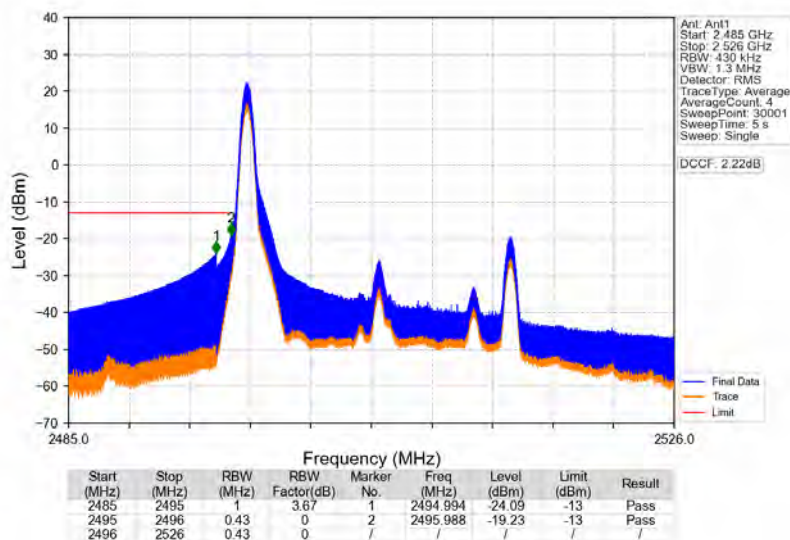
Band41 20MHz 16QAM LCH 2506MHz RB 1 0 NTN
