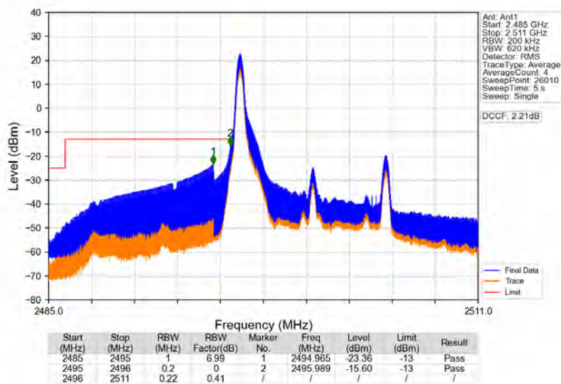
Band41 10MHz 16QAM LCH 2501MHz RB 1 0 NTNV
