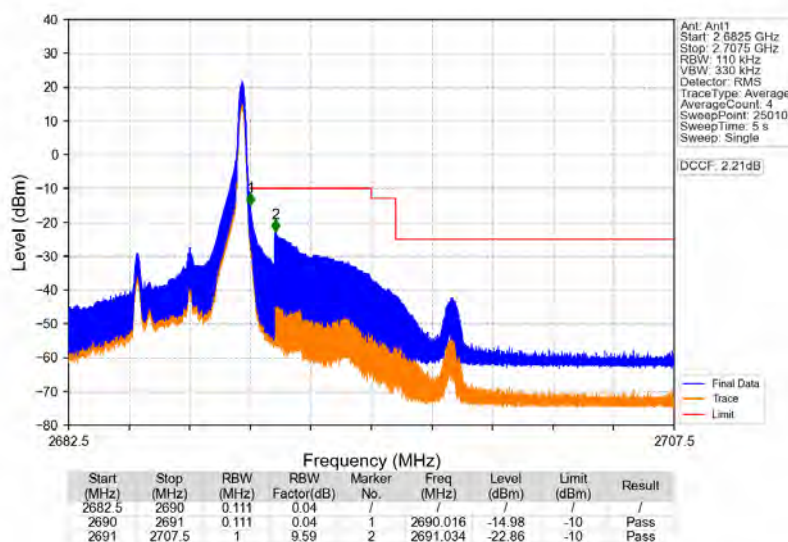
Band41 5MHz 16QAM HCH 2687.5MHz RB 1 24 NTNV
