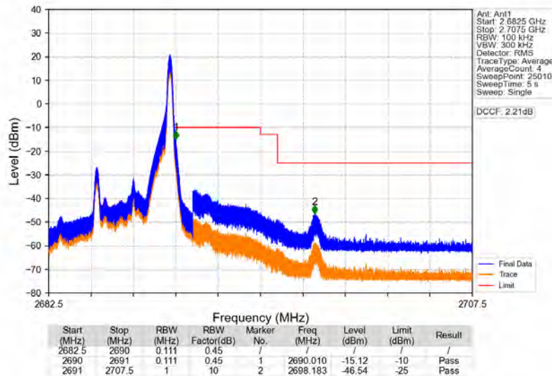
Band41 5MHz 64QAM HCH 2687.5MHz RB 1 24 NTNV
