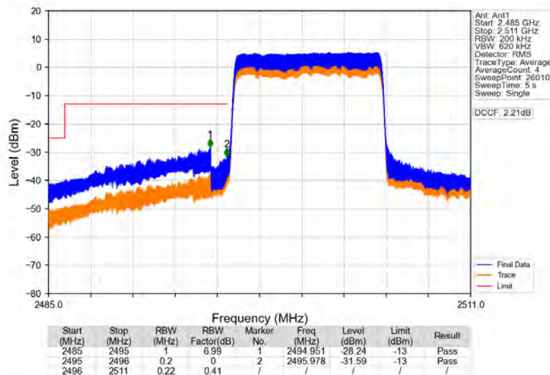
Band41_10MHz_64QAM_LCH_2501MHz_RB_50_0_NTNV
