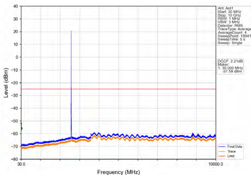
Band41 5MHz QPSK MCH 2593MHz RB 1 0 NTN
