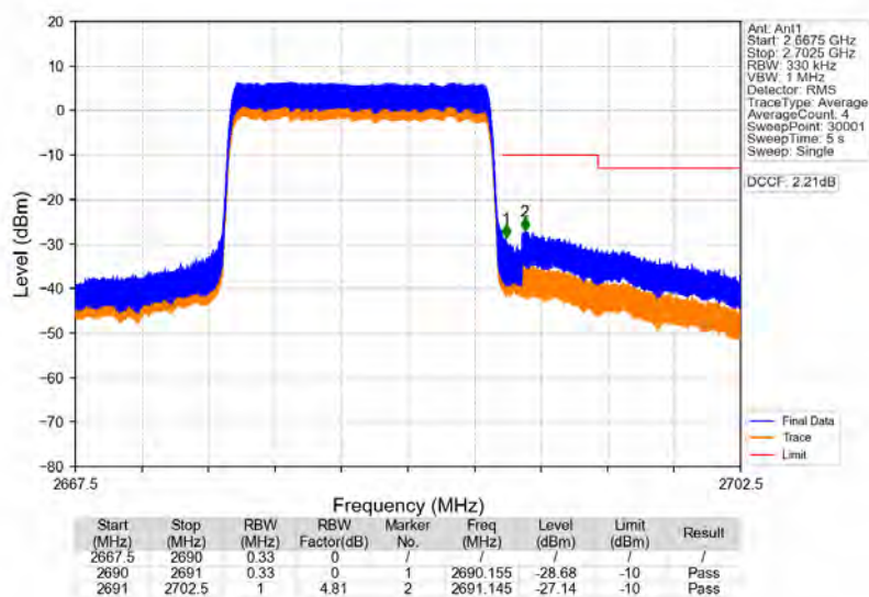
Band41_15MHz_16QAM_HCH_2682.5MHz_RB_75_0_NTNV
