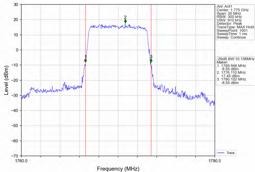
Band66_10MHz_QPSK_HCH_1775MHz_RB_50_0_NTNV
