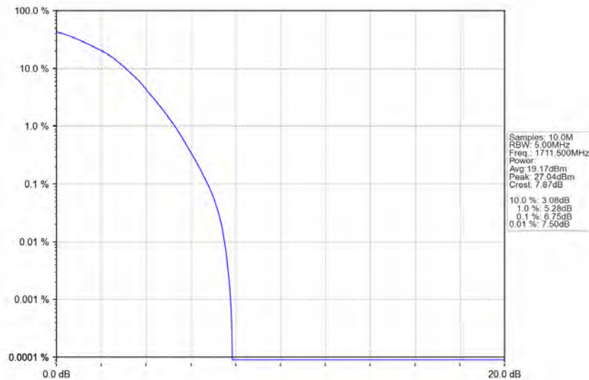
Band66_3MHz_64QAM_LCH_1711.5MHz_RB_15_0_NTNV
