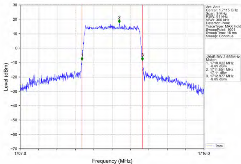
Band66_3MHz_QPSK_LCH_1711.5MHz_RB_15_0_NTNV
