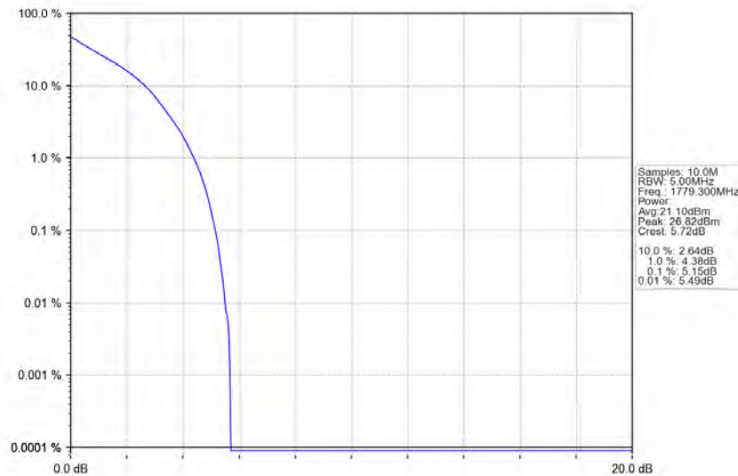
Band66_1.4MHz_QPSK_HCH_1779.3MHz_RB_6_0_NTNV
