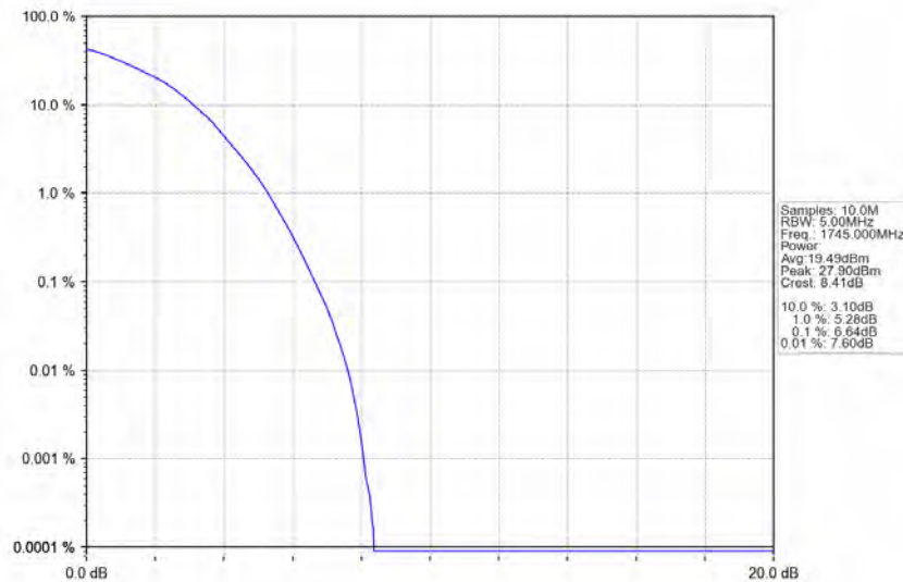
Band66_3MHz_64QAM_MCH_1745MHz_RB_15_0_NTNV
