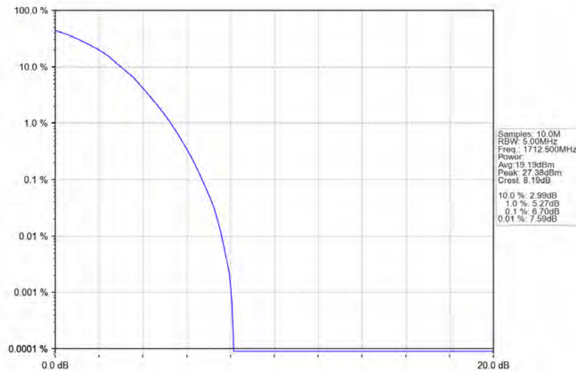
Band66_5MHz_64QAM_LCH_1712.5MHz_RB_25_0_NTNV
