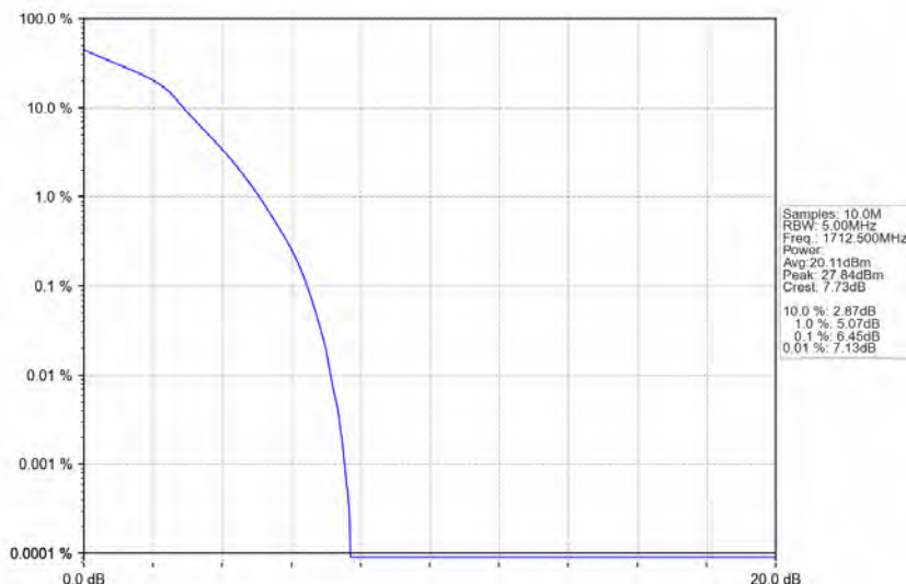
Band66_5MHz_16QAM_LCH_1712.5MHz_RB_25_0_NTNV
