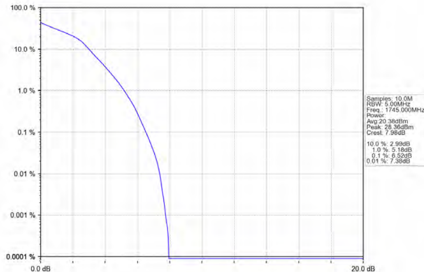
Band66_3MHz_16QAM_MCH_1745MHz_RB_15_0_NTNV
