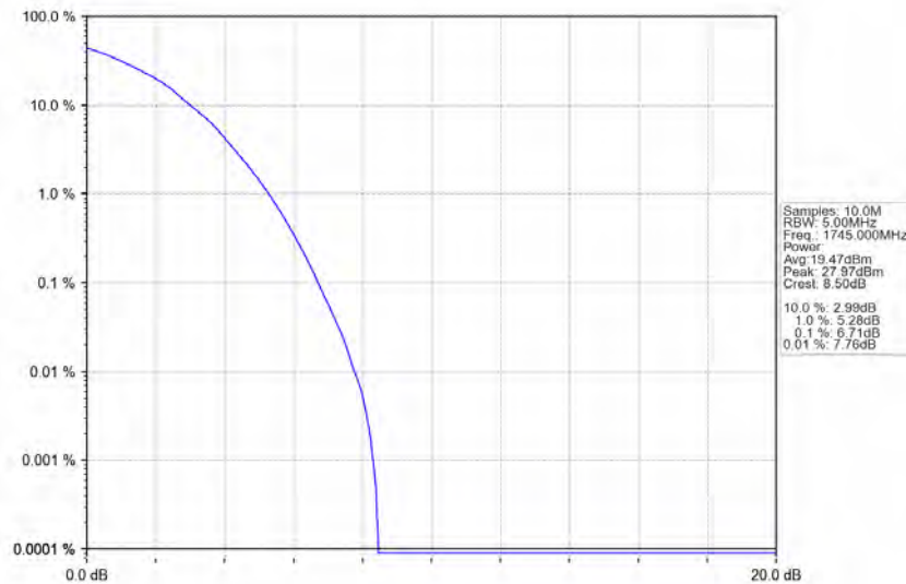
Band66_5MHz_64QAM_MCH_1745MHz_RB_25_0_NTNV
