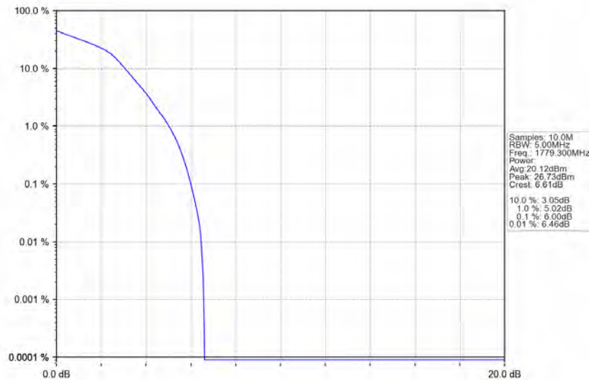
Band66_1.4MHz_16QAM_HCH_1779.3MHz_RB_6_0_NTNV
