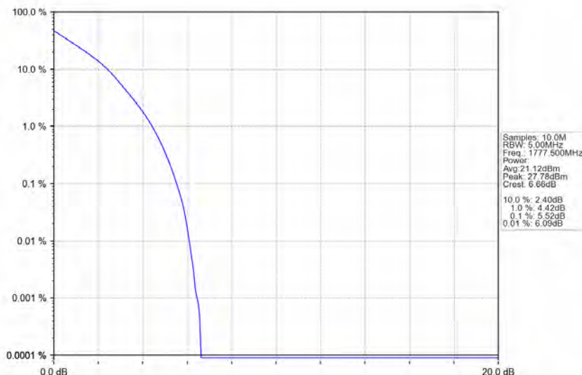
Band66_5MHz_QPSK_HCH_1777.5MHz_RB_25_0_NTNV
