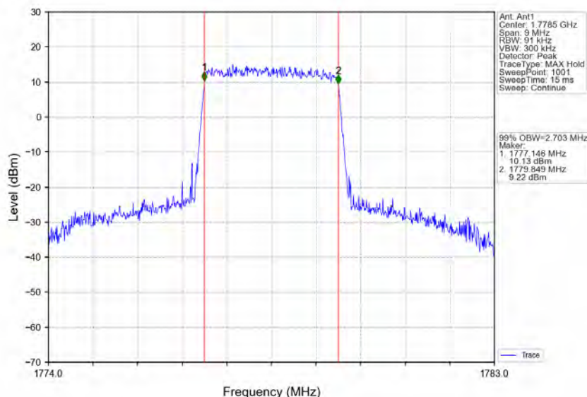
Band66_3MHz_64QAM_HCH_1778.5MHz_RB_15_0_NTNV
