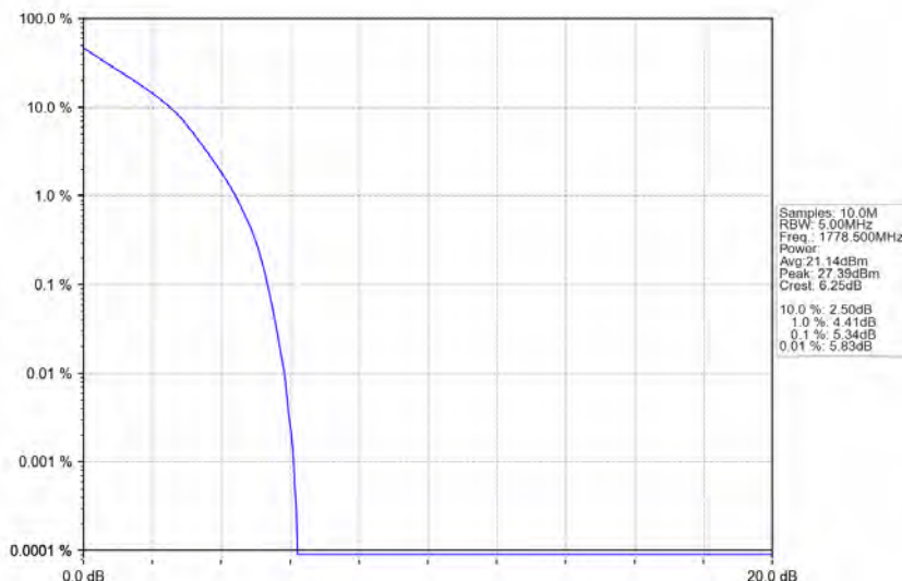
Band66_3MHz_QPSK_HCH_1778.5MHz_RB_15_0_NTNV
