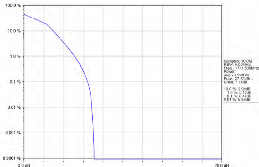
Band66_3MHz_16QAM_LCH_1711.5MHz_RB_15_0_NTNV
