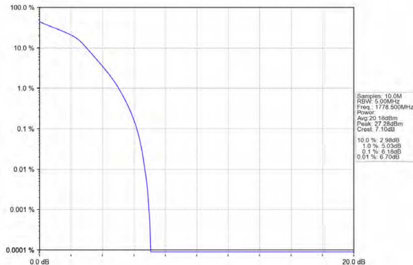
Band66_3MHz_16QAM_HCH_1778.5MHz_RB_15_0_NTNV
