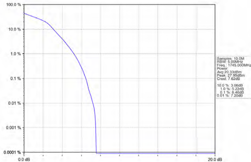
Band66_1.4MHz_16QAM_MCH_1745MHz_RB_6_0_NTNV
