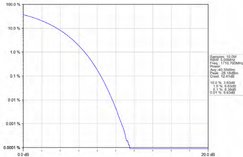
Band66_1.4MHz_16QAM_LCH_1710.7MHz_RB_6_0_NTNV
