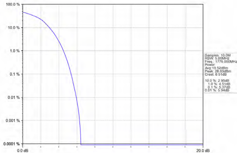
Band66_10MHz_QPSK_HCH_1775MHz_RB_50_0_NTNV
