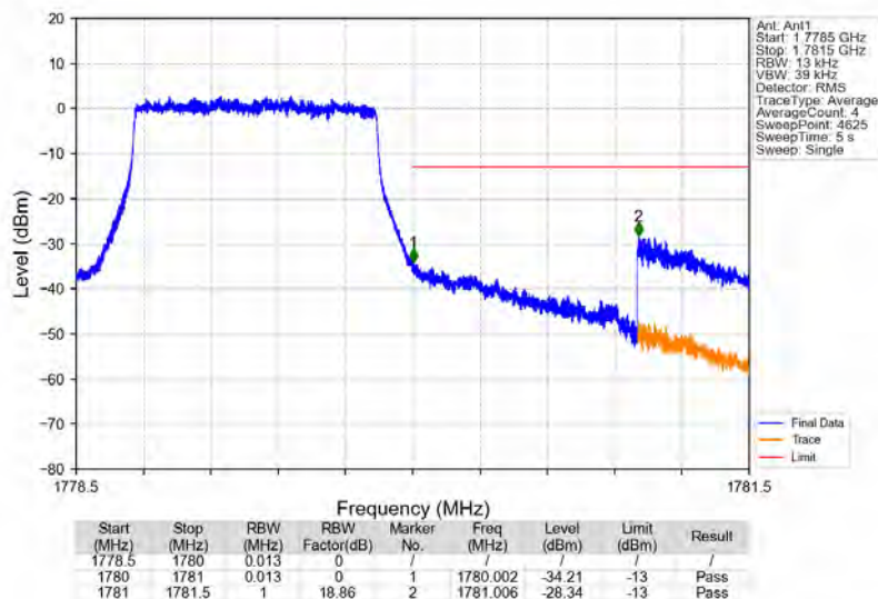
Band66_1.4MHz_64QAM_HCH_1779.3MHz_RB_6_0_NTNV
