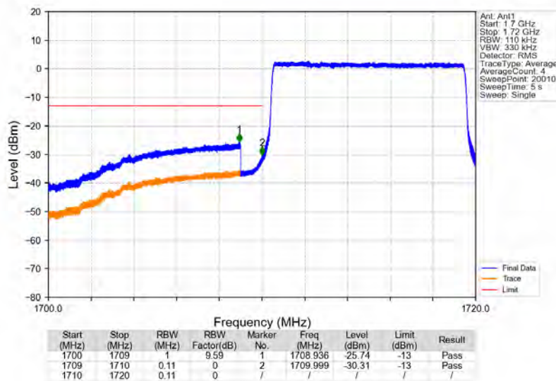
Band66_10MHz_16QAM_LCH_1715MHz_RB_50_0_NTNV
