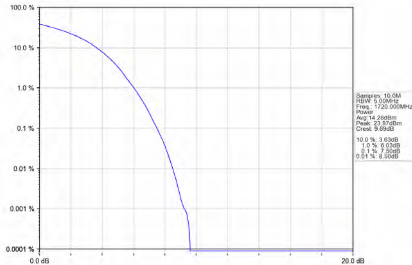
Band66_20MHz_64QAM_LCH_1720MHz_RB_100_0_NTNV
