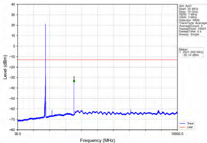
Band66_10MHz_16QAM_HCH_1775MHz_RB_1_0_NTNV
