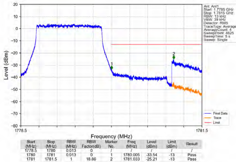
Band66_1.4MHz_QPSK_HCH_1779.3MHz_RB_6_0_NTNV
