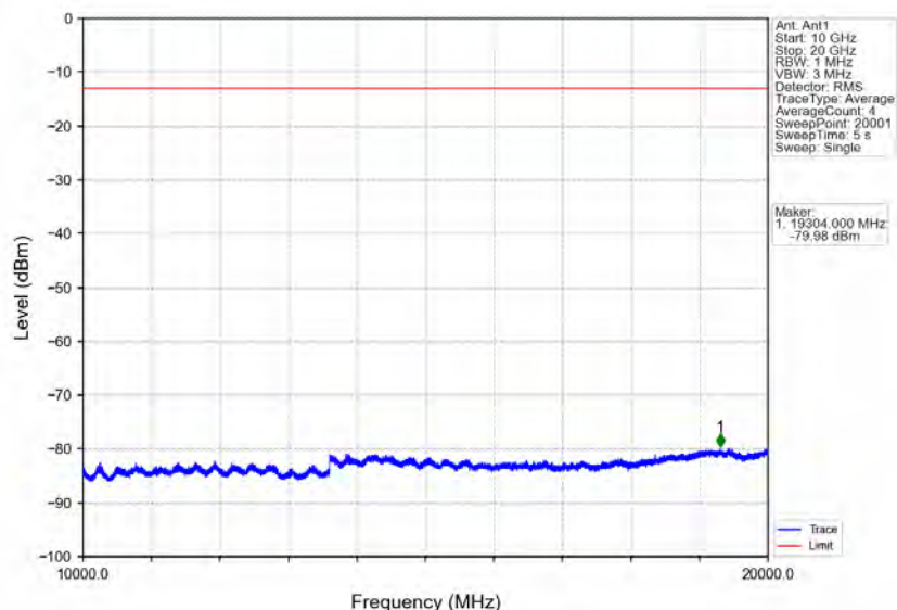
Band66_5MHz_QPSK_HCH_1777.5MHz_RB_1_0_NTNV
