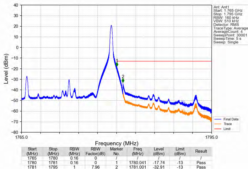
Band66_15MHz_QPSK_HCH_1772.5MHz_RB_1_74_NTNV
