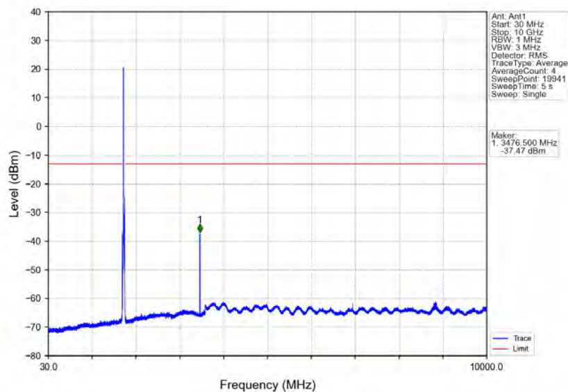
Band66_15MHz_16QAM_MCH_1745MHz_RB_1_0_NTNV
