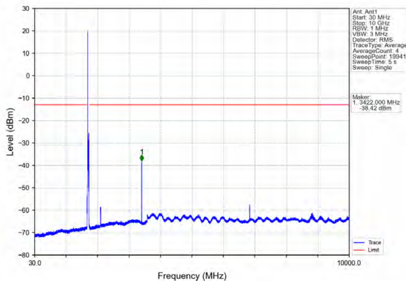
Band66_20MHz_64QAM_LCH_1720MHz_RB_1_0_NTNV
