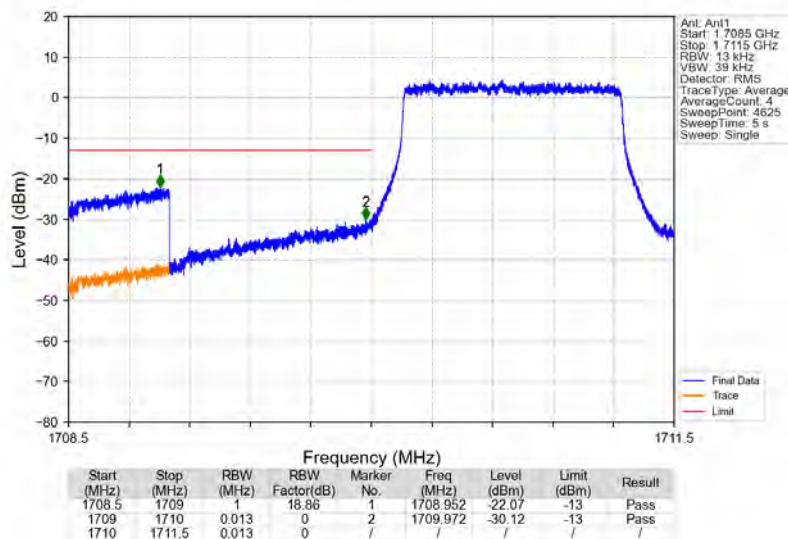
Band66_1.4MHz_QPSK_LCH_1710.7MHz_RB_6_0_NTNV
