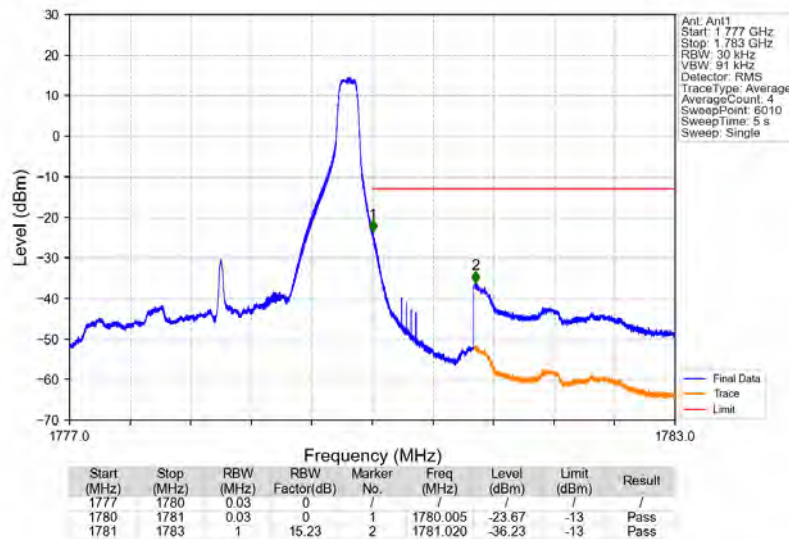
Band66_3MHz_16QAM_HCH_1778.5MHz_RB_1_14_NTNV
