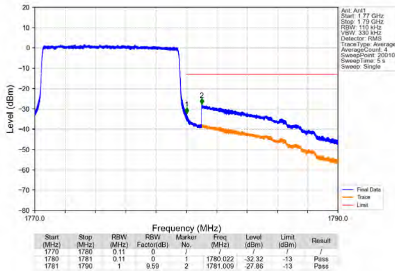
Band66_10MHz_64QAM_HCH_1775MHz_RB_50_0_NTNV
