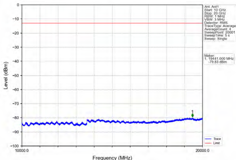
Band66_1.4MHz_16QAM_HCH_1779.3MHz_RB_1_0_NTNV
