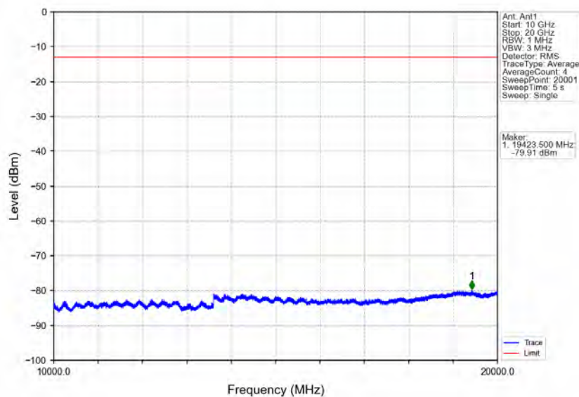
Band66_3MHz_16QAM_MCH_1745MHz_RB_1_0_NTNV
