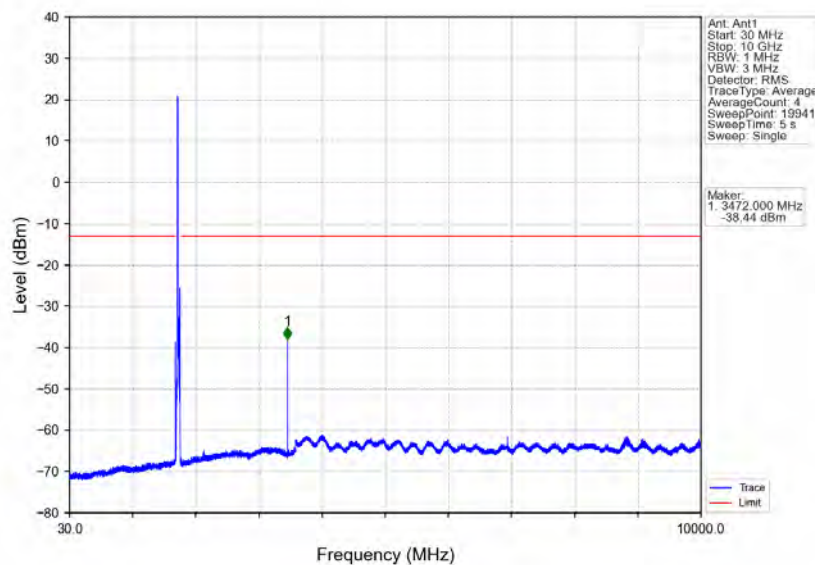
Band66_20MHz_16QAM_MCH_1745MHz_RB_1_0_NTNV
