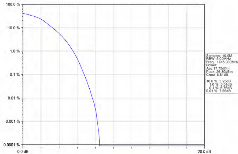
Band66_10MHz_64QAM_MCH_1745MHz_RB_50_0_NTNV
