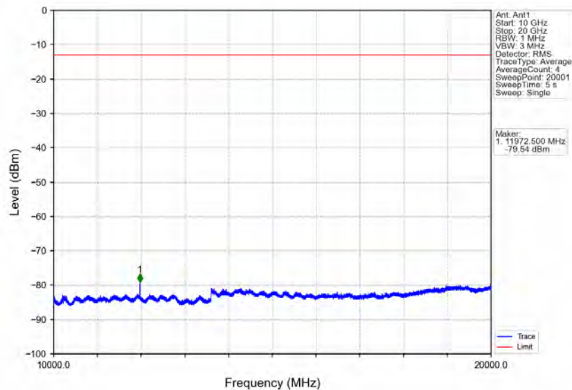
Band66_5MHz_64QAM_LCH_1712.5MHz_RB_25_0_NTNV
