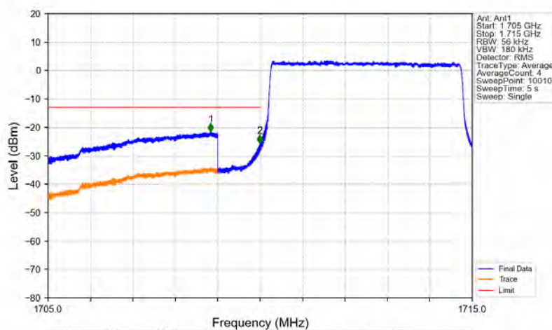
Band66_5MHz_QPSK_LCH_1712.5MHz_RB_25_0_NTNV
