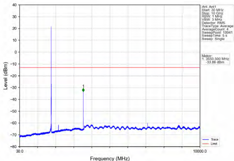
Band66_5MHz_QPSK_HCH_1777.5MHz_RB_1_0_NTNV
