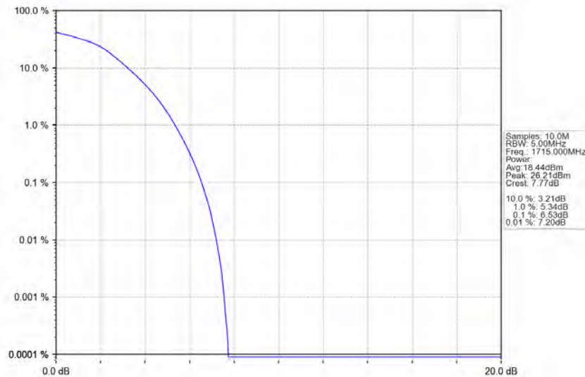
Band66_10MHz_16QAM_LCH_1715MHz_RB_50_0_NTNV
