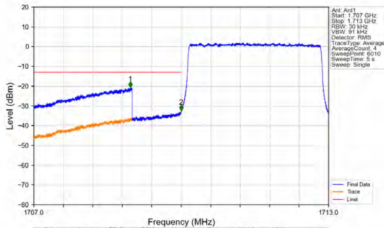
Band66_3MHz_16QAM_LCH_1711.5MHz_RB_15_0_NTNV
