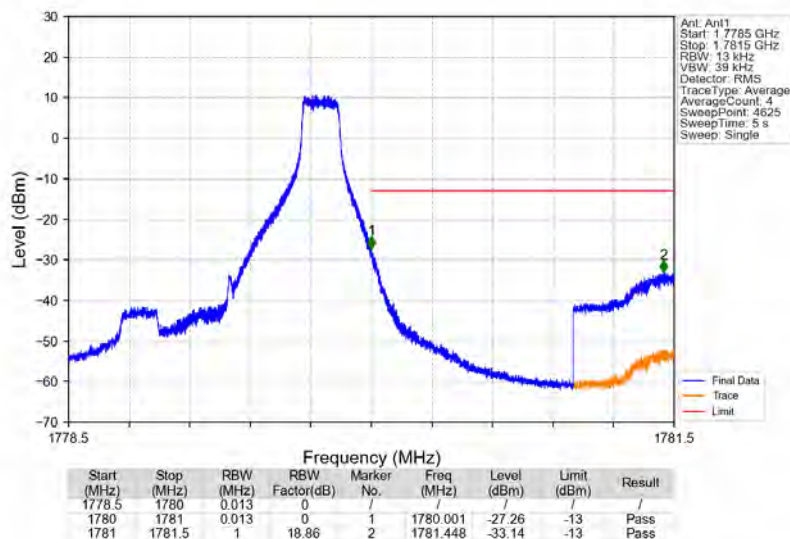
Band66_1.4MHz_64QAM_HCH_1779.3MHz_RB_1_5_NTNV
