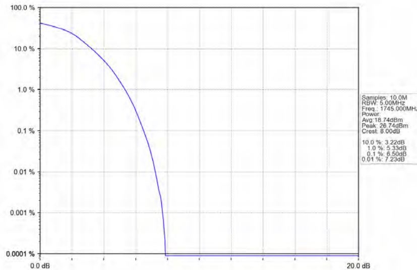
Band66_10MHz_16QAM_MCH_1745MHz_RB_50_0_NTNV
