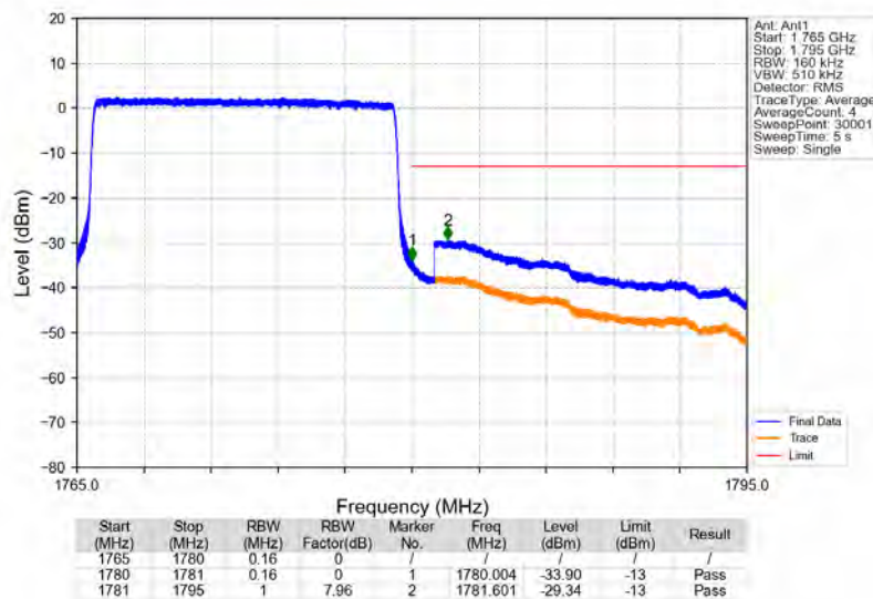
Band66_15MHz_16QAM_HCH_1772.5MHz_RB_75_0_NTNV
