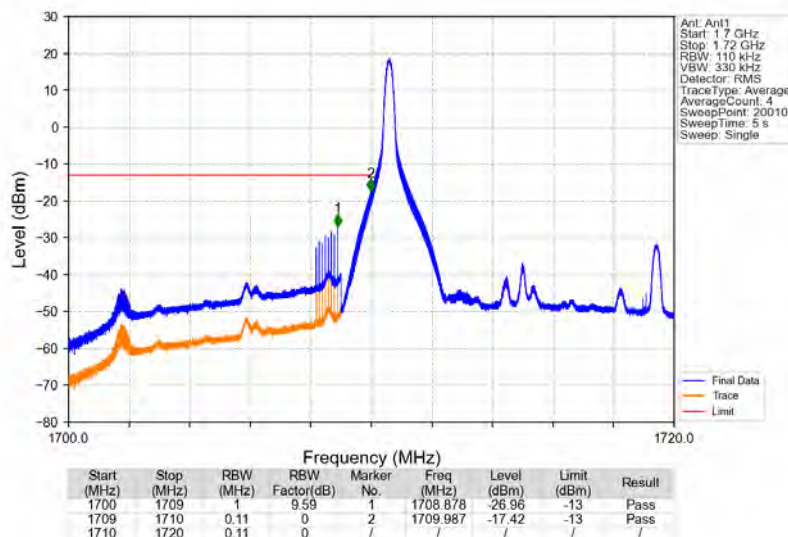
Band66_10MHz_64QAM_LCH_1715MHz_RB_1_0_NTNV
