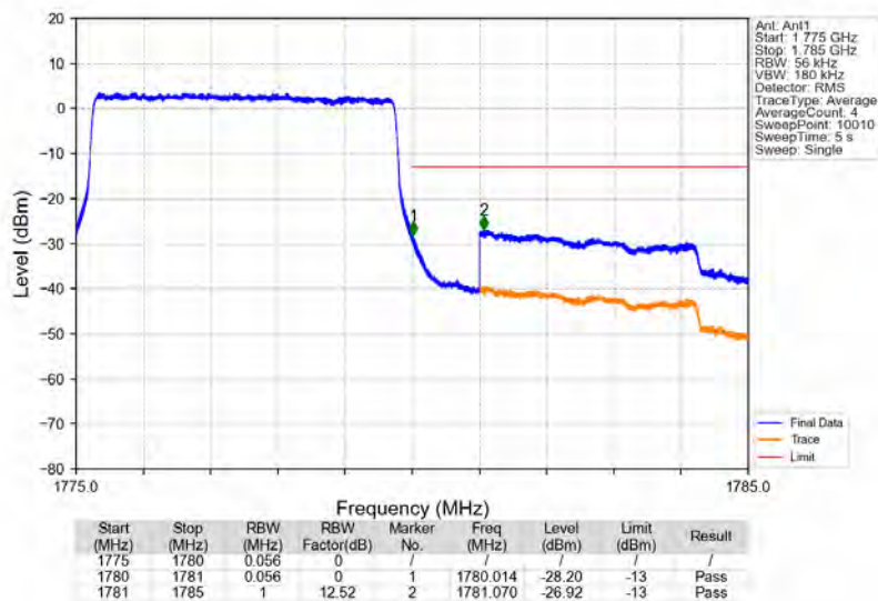
Band66_5MHz_QPSK_HCH_1777.5MHz_RB_25_0_NTNV
