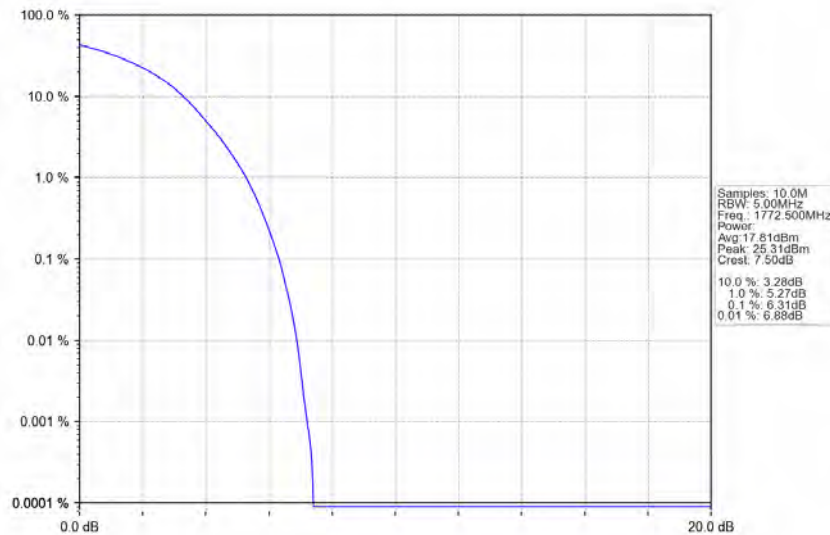
Band66_15MHz_QPSK_HCH_1772.5MHz_RB_75_0_NTNV
