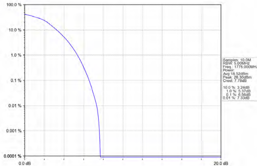
Band66_10MHz_16QAM_HCH_1775MHz_RB_50_0_NTNV
