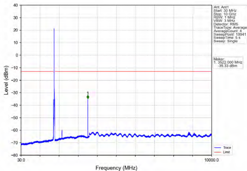
Band66_20MHz_16QAM_HCH_1770MHz_RB_1_0_NTNV
