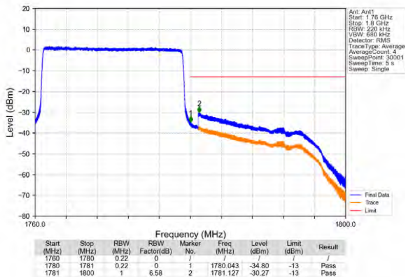
Band66_20MHz_64QAM_HCH_1770MHz_RB_100_0_NTNV
