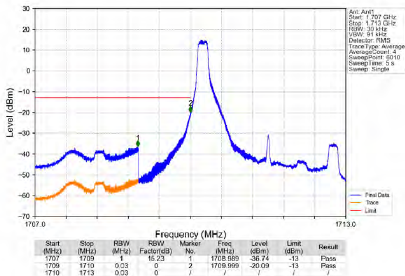
Band66_3MHz_16QAM_LCH_1711.5MHz_RB_1_0_NTNV
