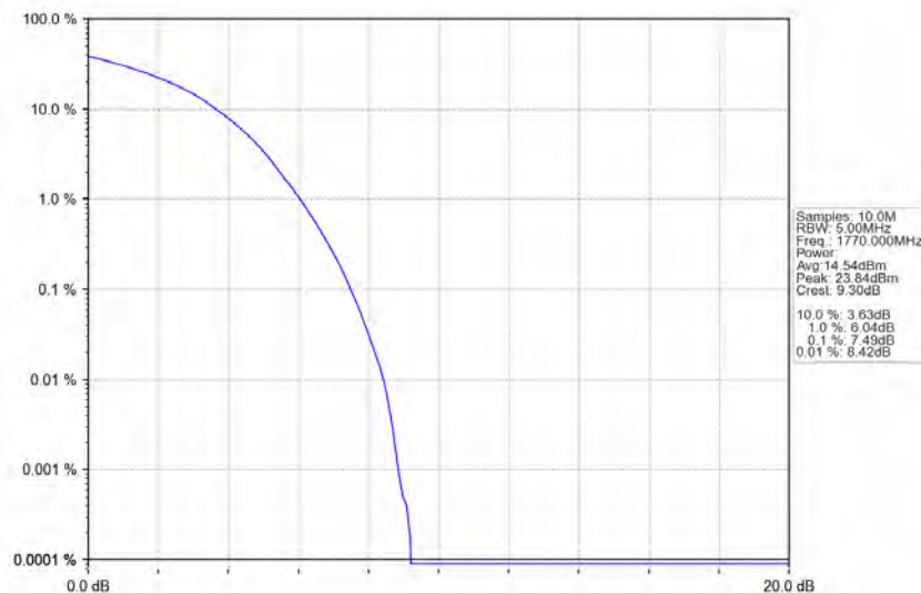
Band66_20MHz_64QAM_HCH_1770MHz_RB_100_0_NTNV
