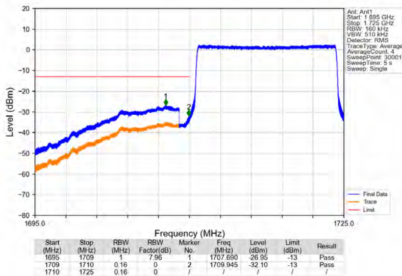
Band66_15MHz_16QAM_LCH_1717.5MHz_RB_75_0_NTNV
