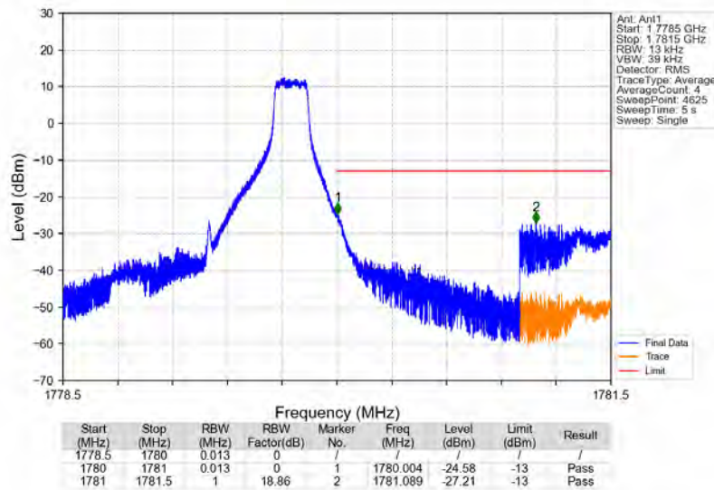
Band66_1.4MHz_QPSK_HCH_1779.3MHz_RB_1_5_NTNV
