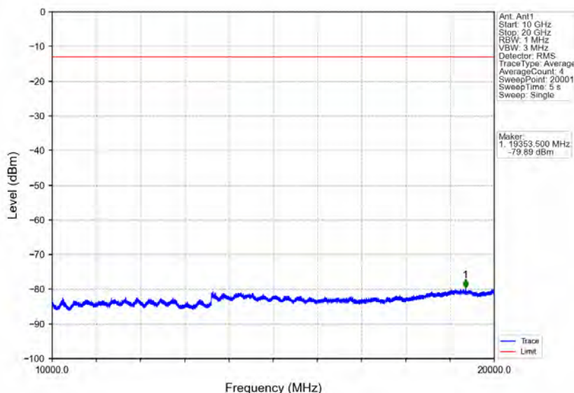
Band66_1.4MHz_64QAM_HCH_1779.3MHz_RB_1_0_NTNV
