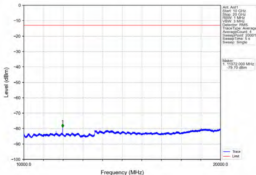
Band66_1.4MHz_QPSK_LCH_1710.7MHz_RB_6_0_NTNV
