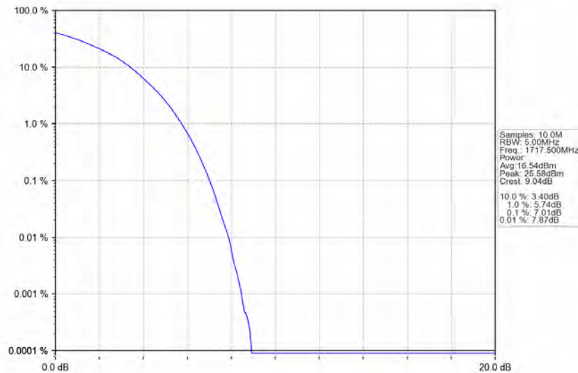
Band66_15MHz_16QAM_LCH_1717.5MHz_RB_75_0_NTNV
