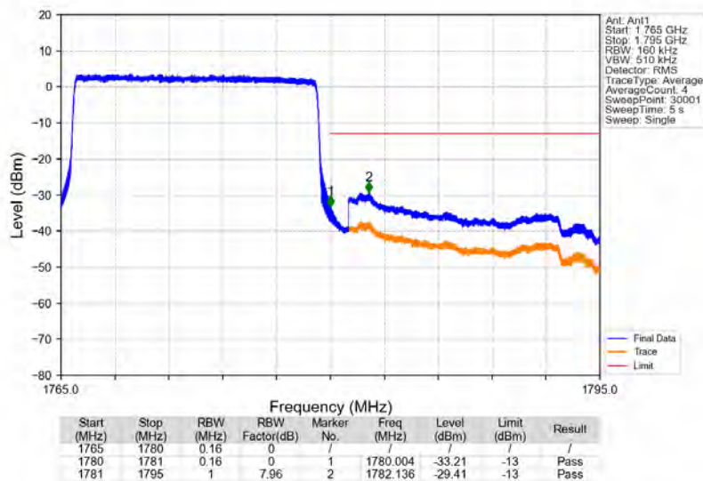
Band66_15MHz_QPSK_HCH_1772.5MHz_RB_75_0_NTNV
