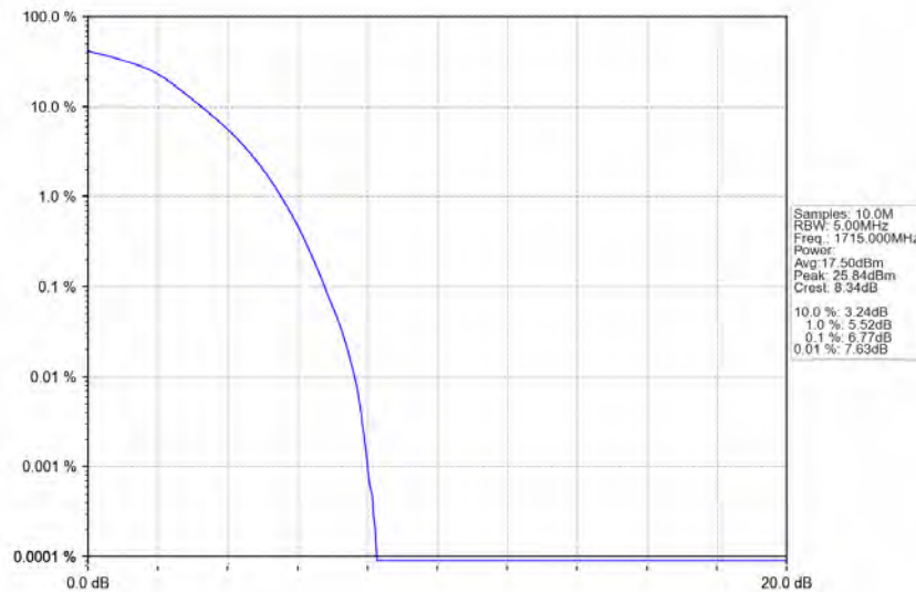
Band66_10MHz_64QAM_LCH_1715MHz_RB_50_0_NTNV
