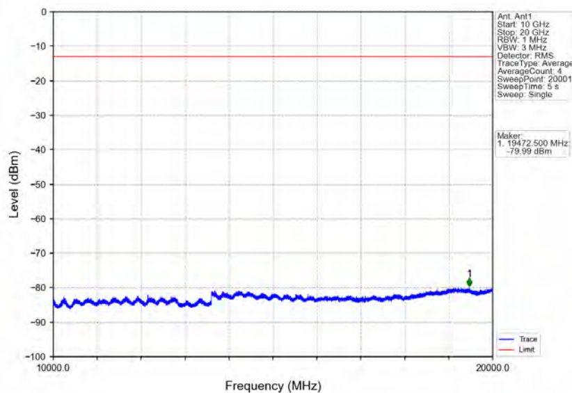
Band66_20MHz_16QAM_MCH_1745MHz_RB_1_0_NTNV
