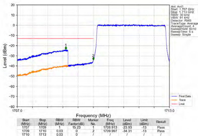
Band66_3MHz_64QAM_LCH_1711.5MHz_RB_15_0_NTNV
