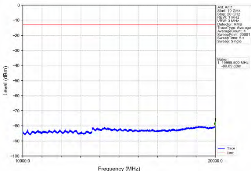
Band66_5MHz_QPSK_MCH_1745MHz_RB_1_0_NTNV
