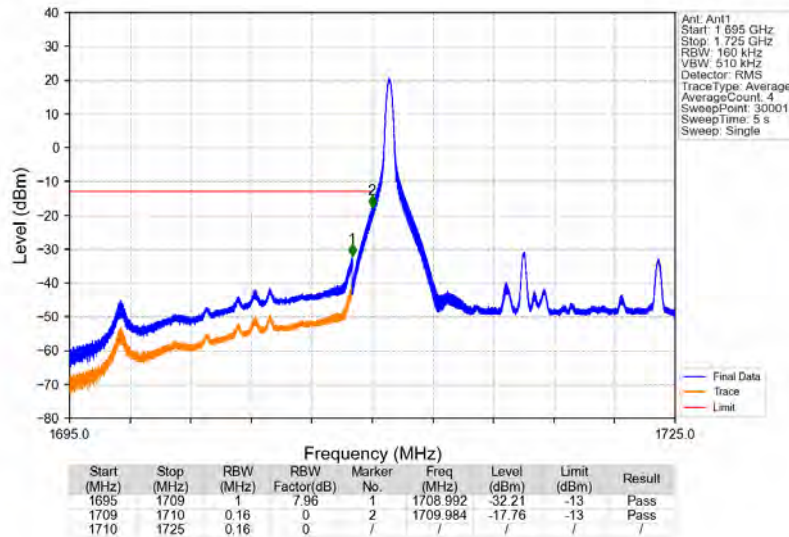
Band66_15MHz_16QAM_LCH_1717.5MHz_RB_1_0_NTNV
