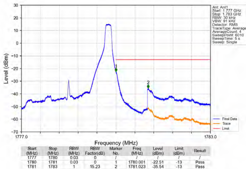
Band66_3MHz_QPSK_HCH_1778.5MHz_RB_1_14_NTNV
