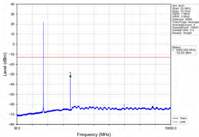
Band66_1.4MHz_QPSK_MCH_1745MHz_RB_1_0_NTNV
