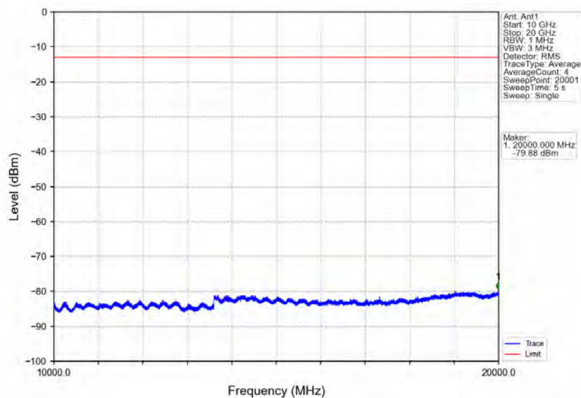
Band66_10MHz_16QAM_HCH_1775MHz_RB_1_0_NTNV
