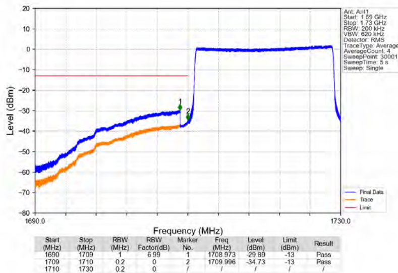
Band66_20MHz_64QAM_LCH_1720MHz_RB_100_0_NTNV
