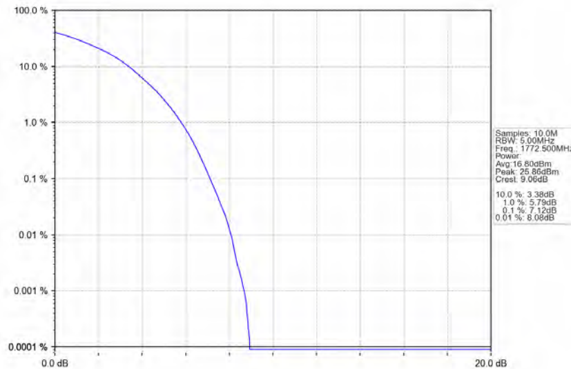
Band66_15MHz_16QAM_HCH_1772.5MHz_RB_75_0_NTNV
