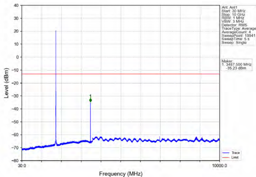
Band66_3MHz_16QAM_MCH_1745MHz_RB_1_0_NTNV
