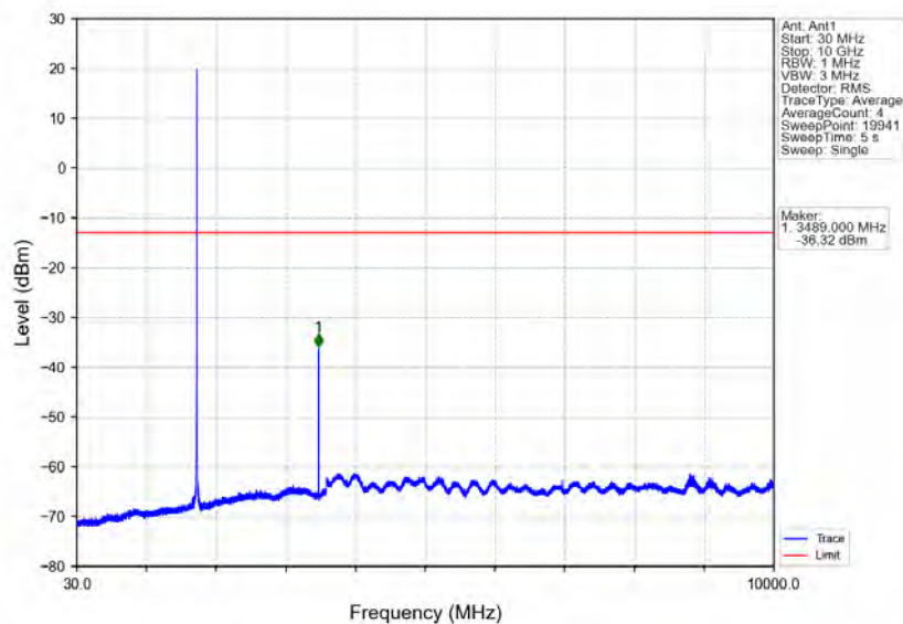
Band66_1.4MHz_64QAM_MCH_1745MHz_RB_1_0_NTNV
