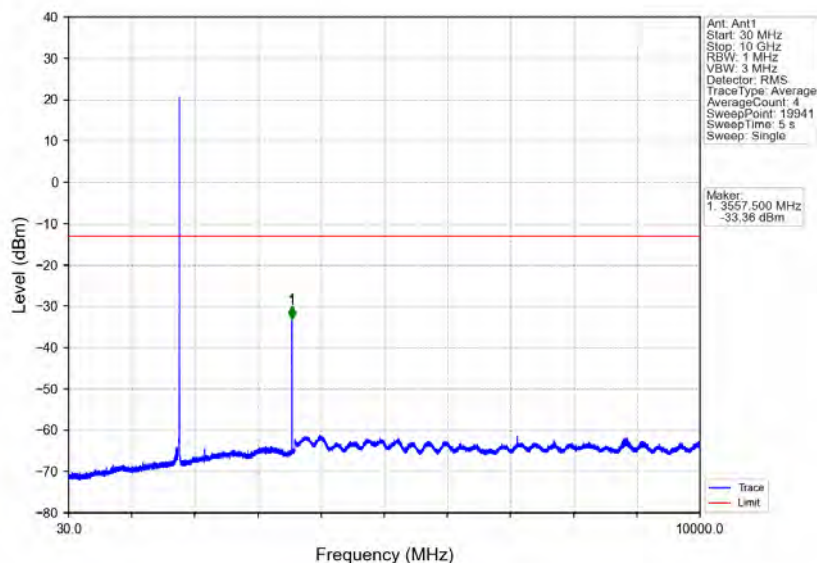
Band66_1.4MHz_16QAM_HCH_1779.3MHz_RB_1_0_NTNV
