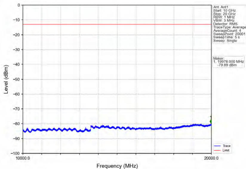
Band66_1.4MHz_QPSK_MCH_1745MHz_RB_1_0_NTNV
