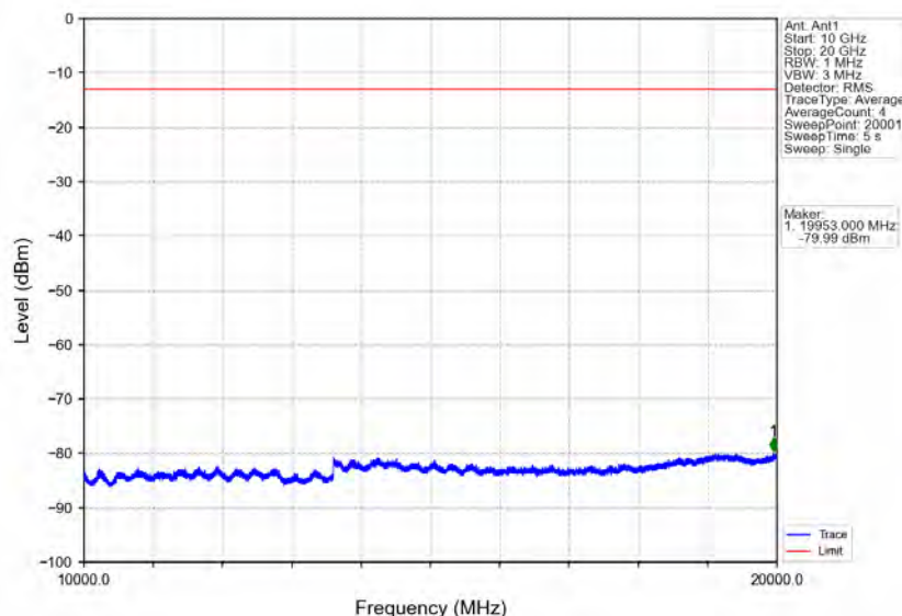
Band66_1.4MHz_QPSK_HCH_1779.3MHz_RB_1_0_NTNV
