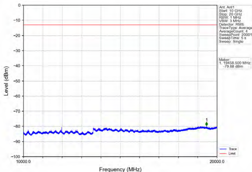
Band66_10MHz_16QAM_LCH_1715MHz_RB_50_0_NTNV
