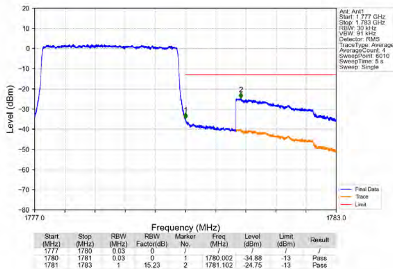
Band66_3MHz_16QAM_HCH_1778.5MHz_RB_15_0_NTNV
