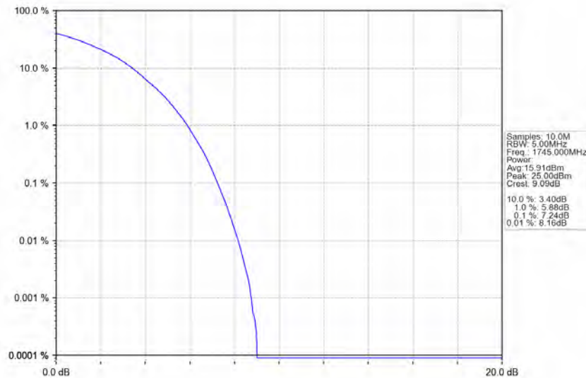
Band66_15MHz_64QAM_MCH_1745MHz_RB_75_0_NTNV
