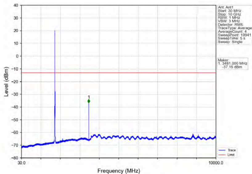
Band66_10MHz_64QAM_MCH_1745MHz_RB_1_0_NTNV
