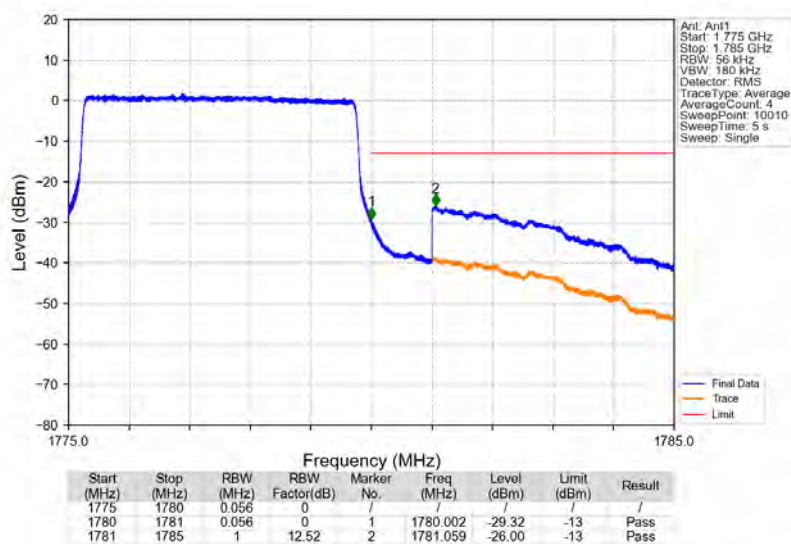
Band66_5MHz_64QAM_HCH_1777.5MHz_RB_25_0_NTNV
