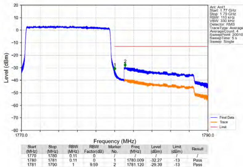
Band66_10MHz_QPSK_HCH_1775MHz_RB_50_0_NTNV
