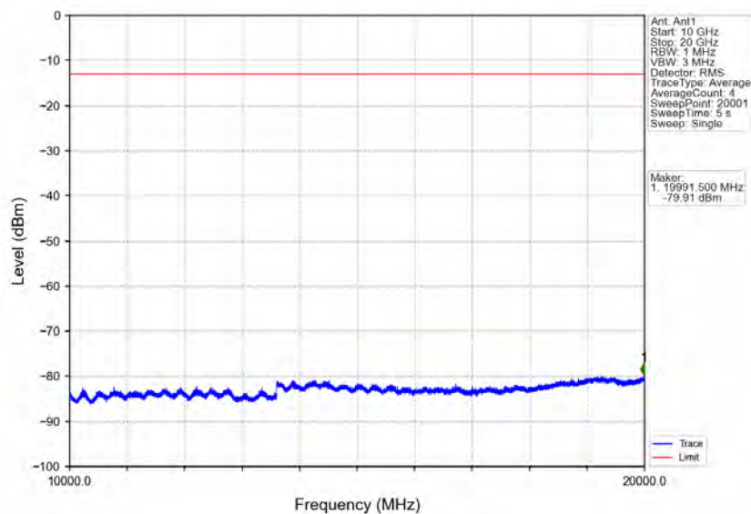
Band66_1.4MHz_16QAM_MCH_1745MHz_RB_1_0_NTNV
