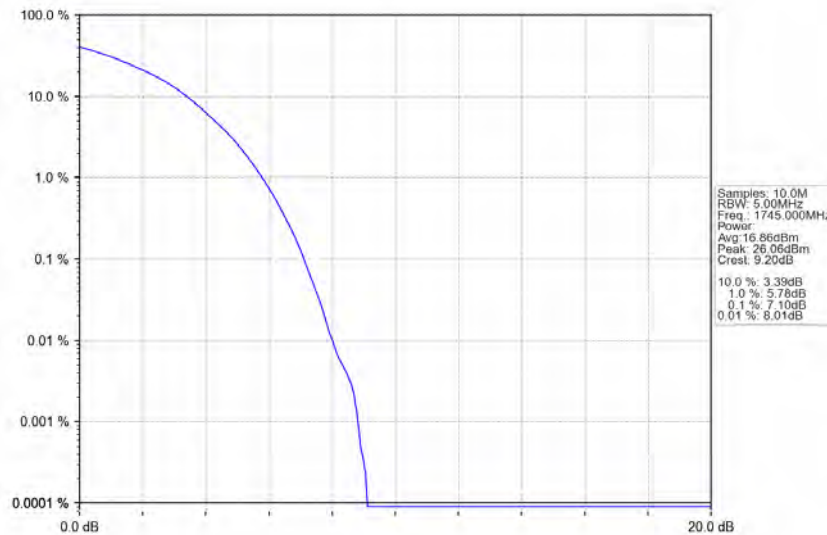
Band66_15MHz_16QAM_MCH_1745MHz_RB_75_0_NTNV
