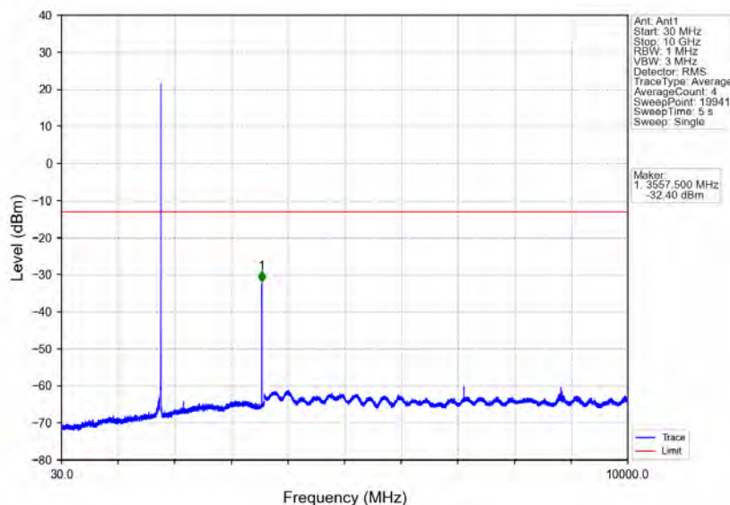
Band66_1.4MHz_QPSK_HCH_1779.3MHz_RB_1_0_NTNV
