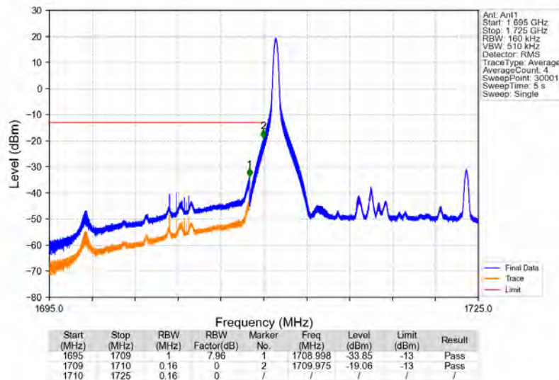
Band66_15MHz_64QAM_LCH_1717.5MHz_RB_1_0_NTNV
