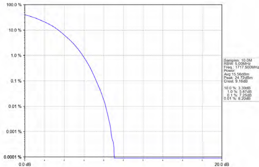
Band66_15MHz_64QAM_LCH_1717.5MHz_RB_75_0_NTNV
