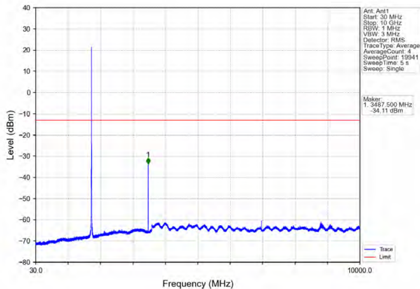
Band66_3MHz_QPSK_MCH_1745MHz_RB_1_0_NTNV
