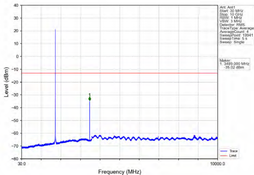
Band66_1.4MHz_16QAM_MCH_1745MHz_RB_1_0_NTNV
