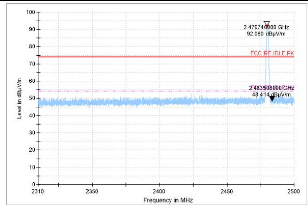
Bandedge:Ch39
