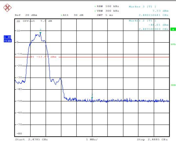
Frequency Band Edge: 8DPSK, Ch78, Hopping OFF
