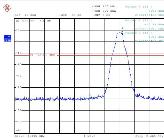
Frequency Band Edge: GFSK, Ch0, Hopping OFF
