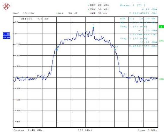
20dB Bandwidth: 8DPSK, Ch78
