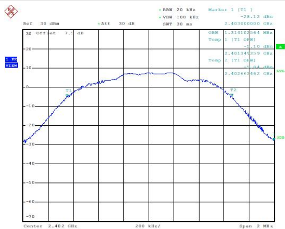
99% Bandwidth: 8DPSK, Ch0
