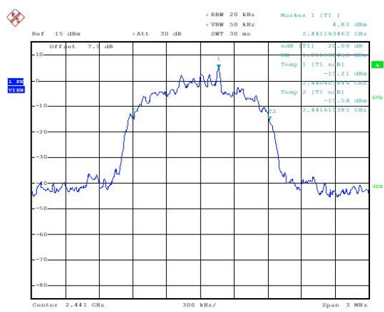
20dB Bandwidth: 8DPSK, Ch39
