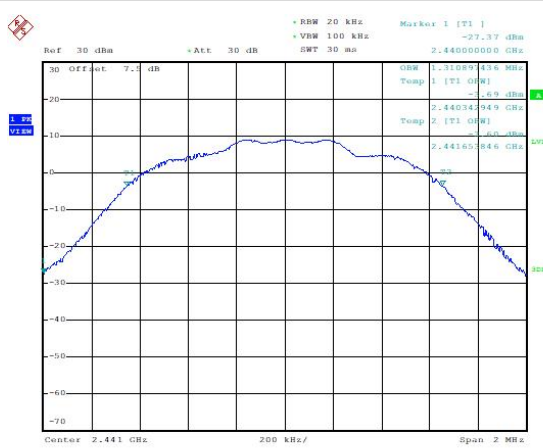
99% Bandwidth: 8DPSK, Ch39
