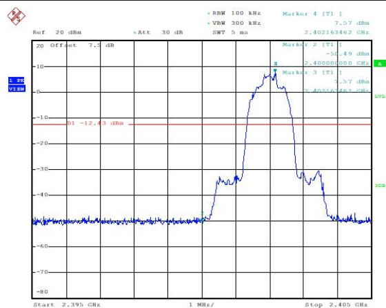
Frequency Band Edge: 8DPSK, Ch0, Hopping OFF
