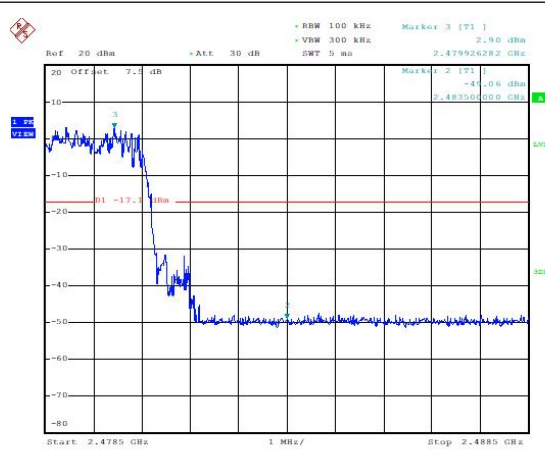
Frequency Band Edge: 8DPSK, Ch78, Hopping ON
