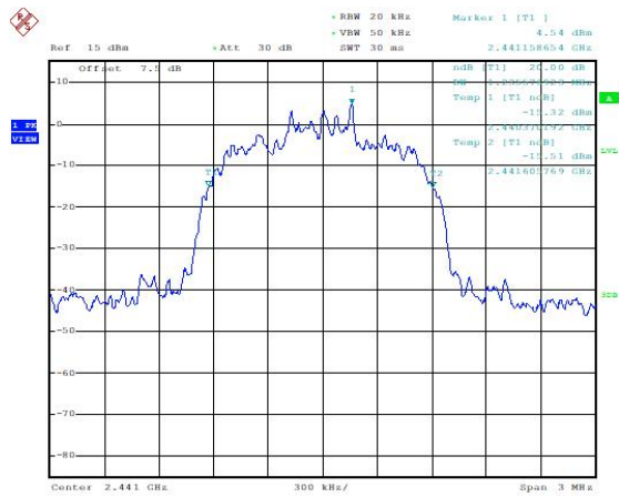
20dB Bandwidth: \pi/4 DQPSK, Ch39
