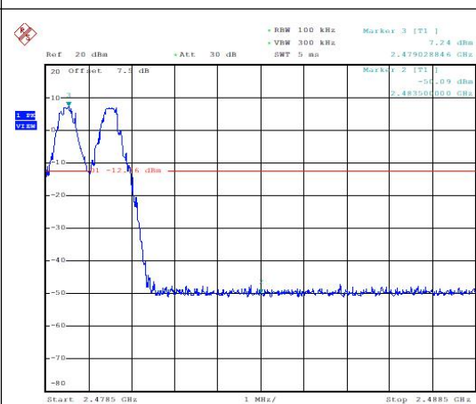
Frequency Band Edge: GFSK, Ch78, Hopping ON
