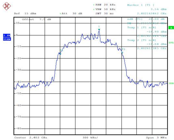
20dB Bandwidth: 8DPSK, Ch0
