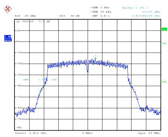
Power Spectral Density (802.11g, Ch1)
