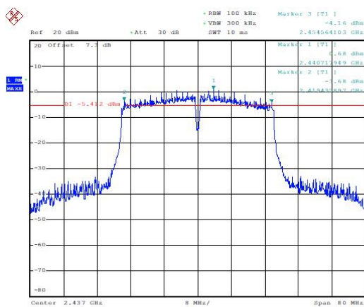
Occupied 6dB Bandwidth (MHz) (802.11n-40MHz, Ch6)
