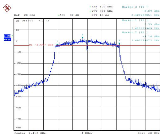
Occupied 6dB Bandwidth (MHz) (802.11n-20MHz, Ch1)
