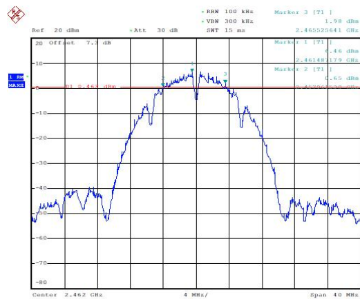
Occupied 6dB Bandwidth (MHz) (802.11b, Ch11)
