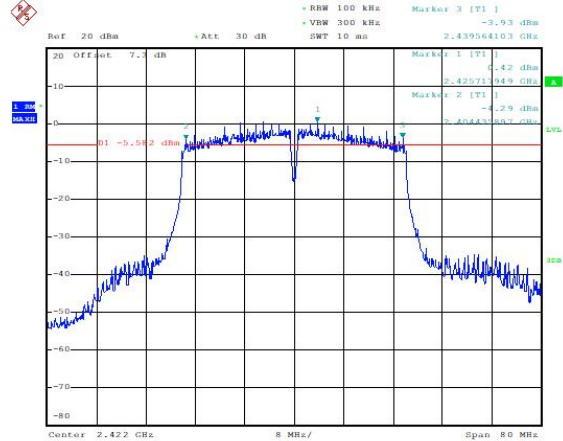
Occupied 6dB Bandwidth (MHz) (802.11n-40MHz, Ch3)
