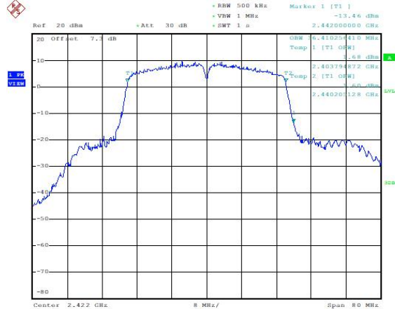
99% Occupied Bandwidth (802.11n40, Ch3)
