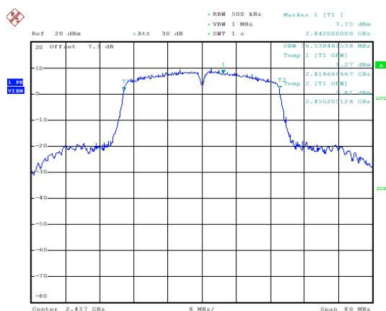
99% Occupied Bandwidth (802.11n40, Ch6)
