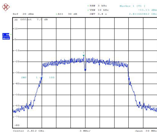
Power Spectral Density (802.11n-20MHz, Ch1)
