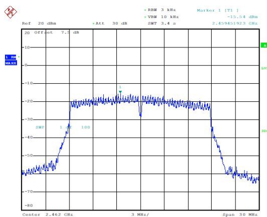
Power Spectral Density (802.11n-20MHz, Ch11)
