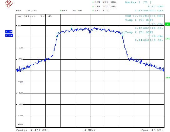
99% Occupied Bandwidth (802.11n20, Ch6)
