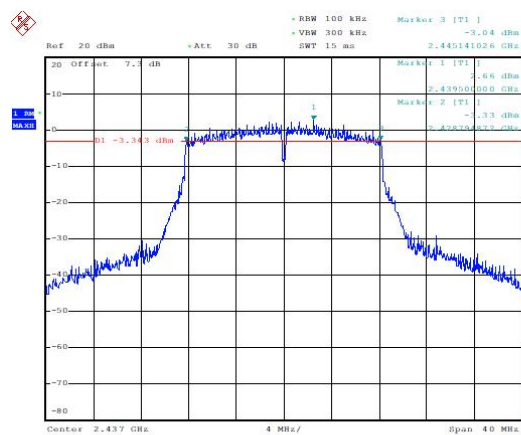
Occupied 6dB Bandwidth (MHz) (802.11g, Ch6)
