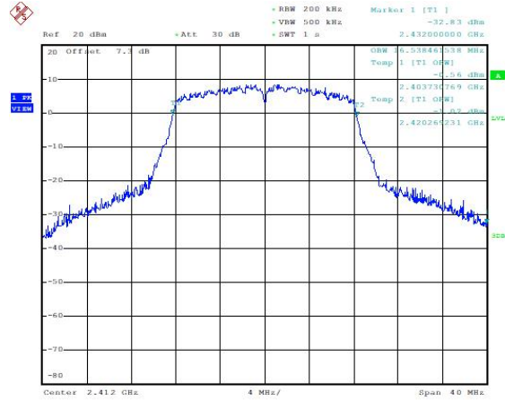
99% Occupied Bandwidth (802.11g, Ch1)
