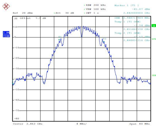
99% Occupied Bandwidth (802.11b, Ch11)
