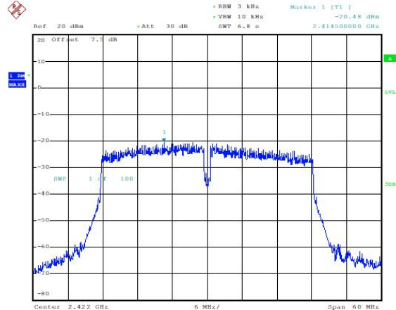
Power Spectral Density (802.11n-40MHz, Ch3)
