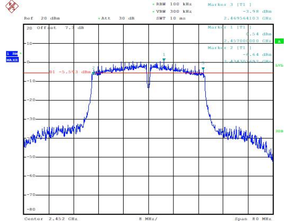
Occupied 6dB Bandwidth (MHz) (802.11n-40MHz, Ch9)
