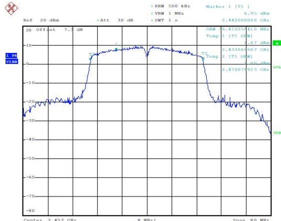
99% Occupied Bandwidth (802.11n40, Ch9)
