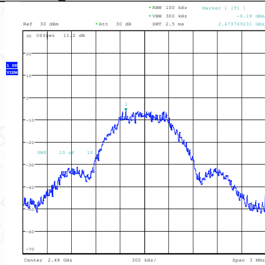
BLE_125K-Ant1-2480-0~Reference-PASS
