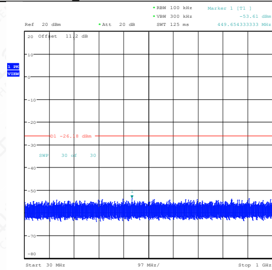
BLE_125K-Ant1-2480-30~1000-PASS
