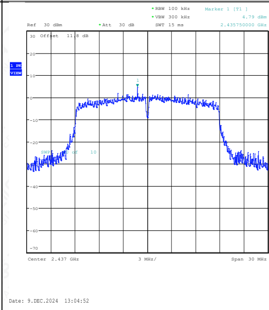
11N20SISO-Ant1-2437-0~Reference-PASS
