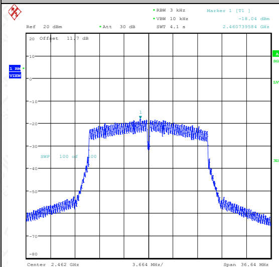
11N20SISO-Ant1-2462-PASS
