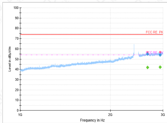
RSE-11G-CH6-1GHz-3GHz
