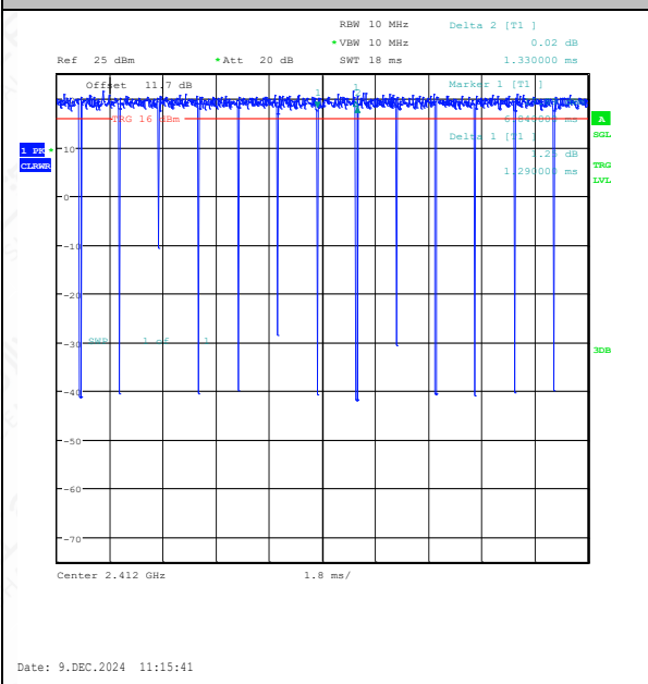
NTNV-11N20SISO-Ant1-2412
