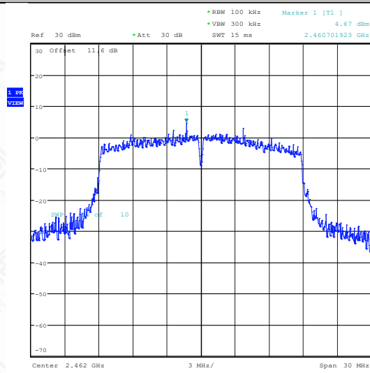
11N20SISO-Ant1-2462-0~Reference-PASS
