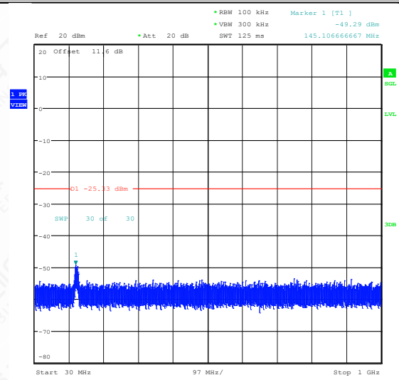
11N20SISO-Ant1-2462-30~1000-PASS
