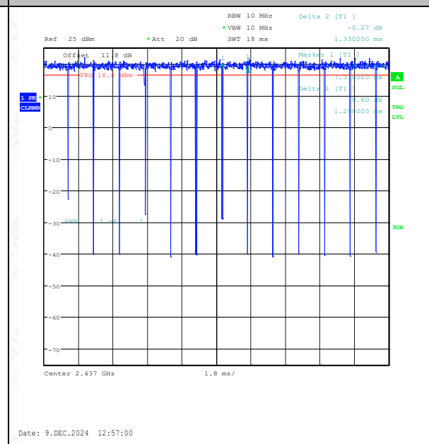
NTNV-11N20SISO-Ant1-2437
