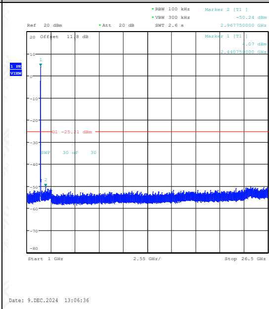
11N20SISO-Ant1-2437-1000~26500-PASS
