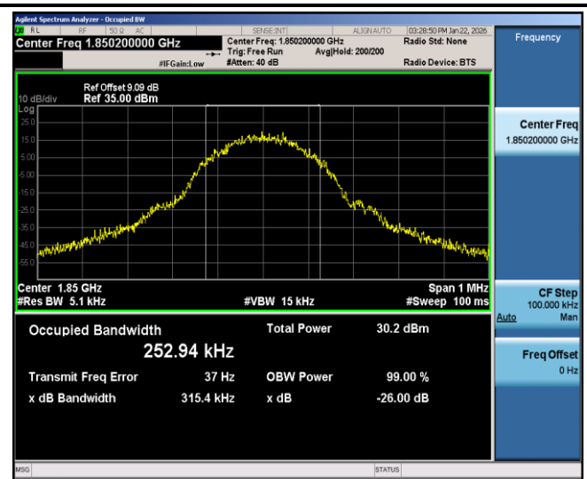
EGPRS1900-512-2-0.3154
