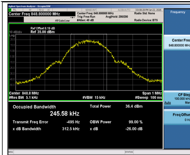
GSM850-251-3-0.3125
