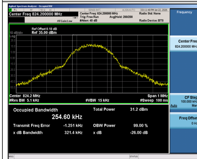
EGPRS850-128-8-0.3214
