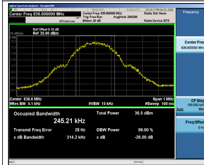
GPRS850-190-3-0.3142
