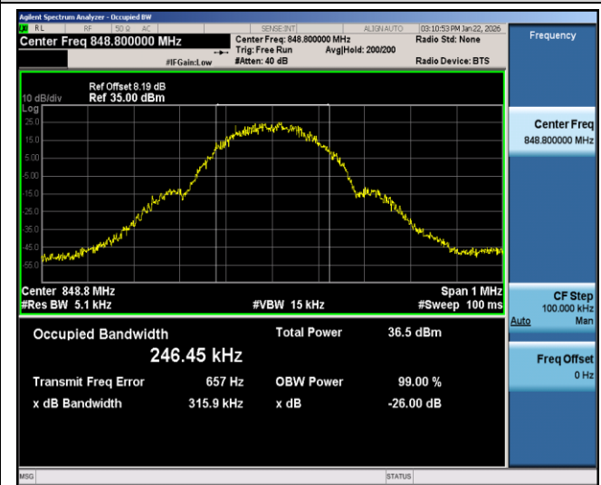
GPRS850-251-3-0.3159
