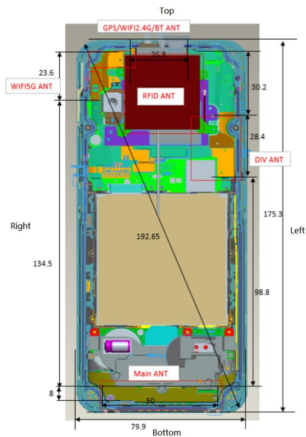
Picture 18: Antenna Locations
