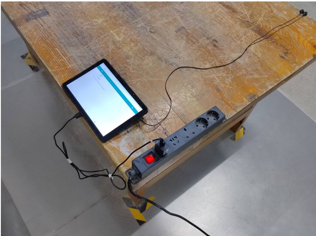
Conducted Emissions Side View Adapter 2#
