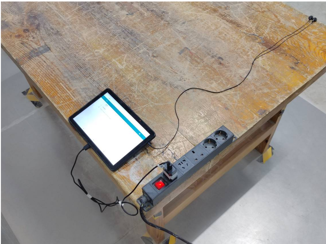
Conducted Emissions Side View Adapter 3#
